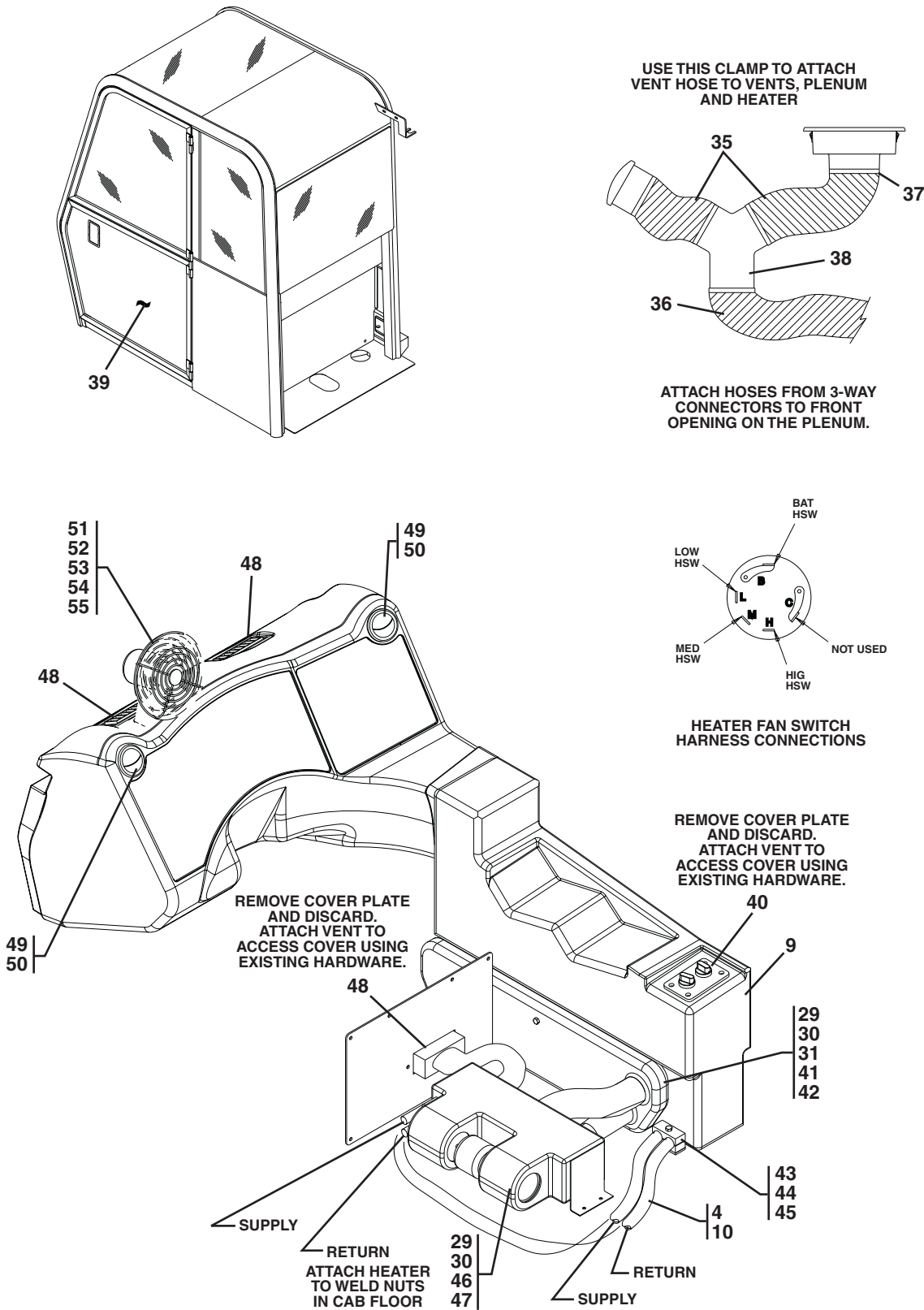
Figure 6-2 Cab Enclosure With Heater Option (Continued)
