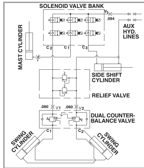
HYDRAULIC SCHEMATIC
