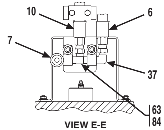
VIEW E-E
