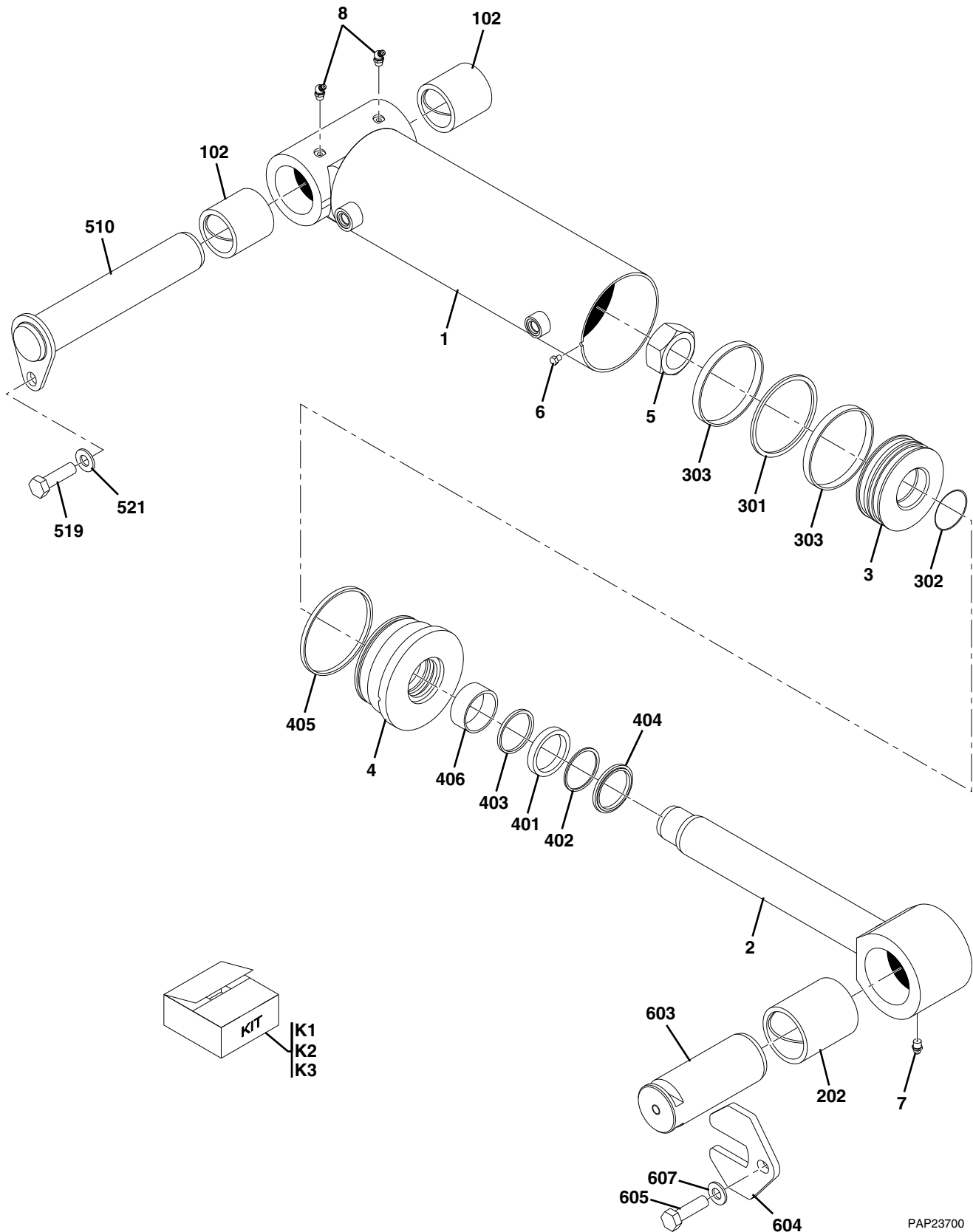
Figure 9-4 Compensating Cylinder
