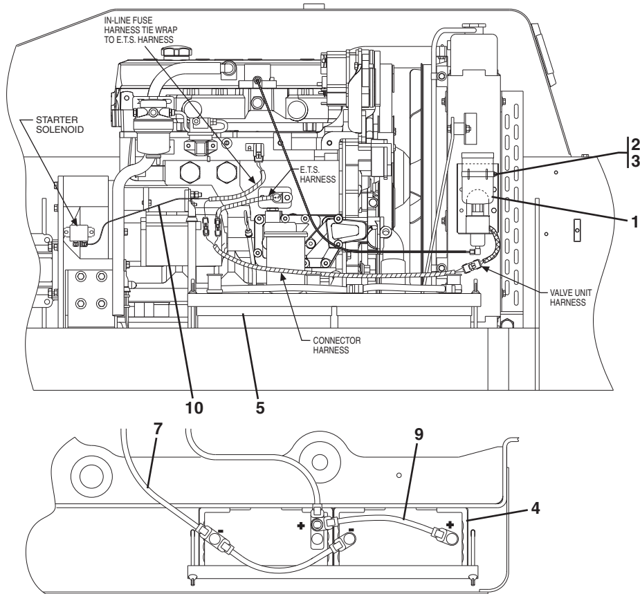
VIEW OF BATTERY AREA
