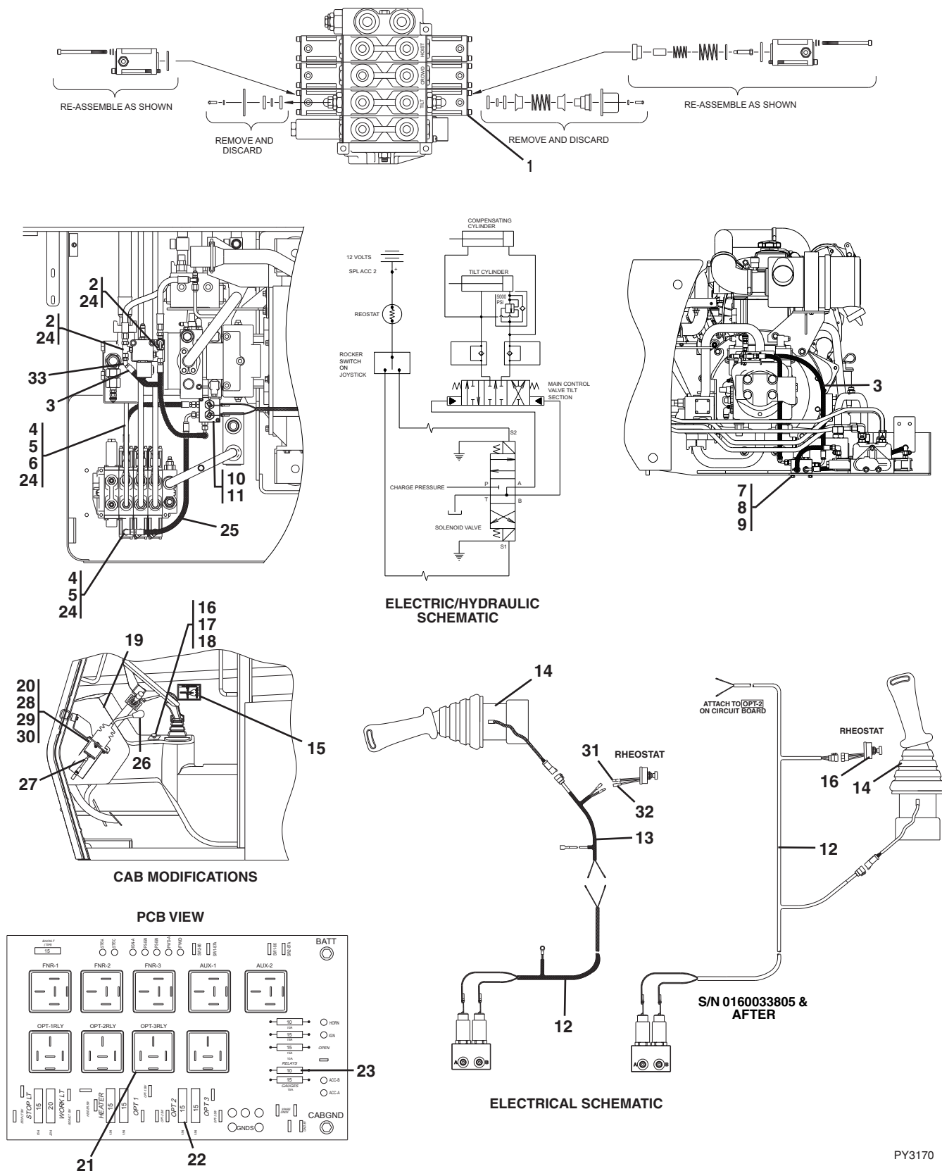
Figure 12-16 Tilt on Joystick With LH Sway
