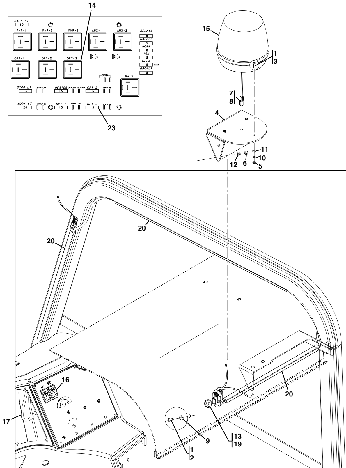
Figure 12-41 Beacon Light Installation
