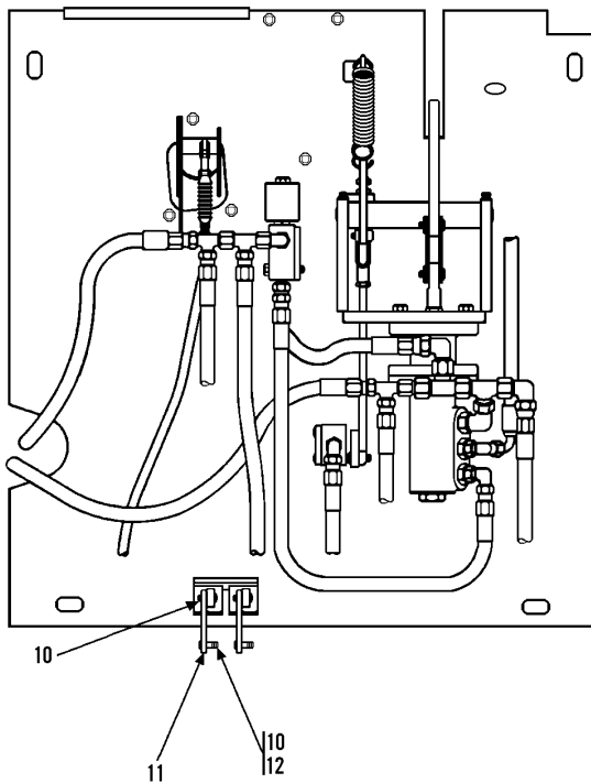
VIEW B-B
