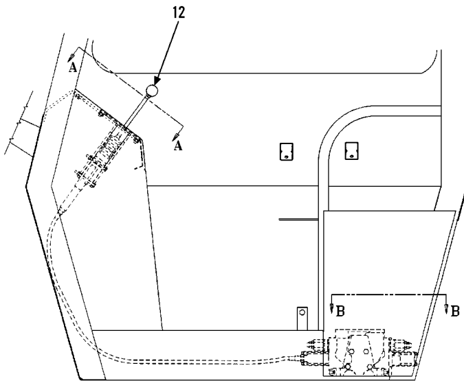
VIEW INSIDE CAB
