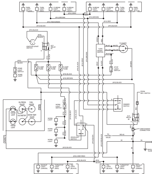
ELECTRICAL SCHEMATIC
