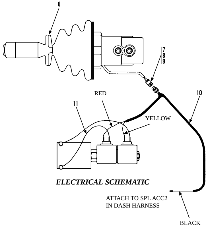
VIEW INSIDE CAB
