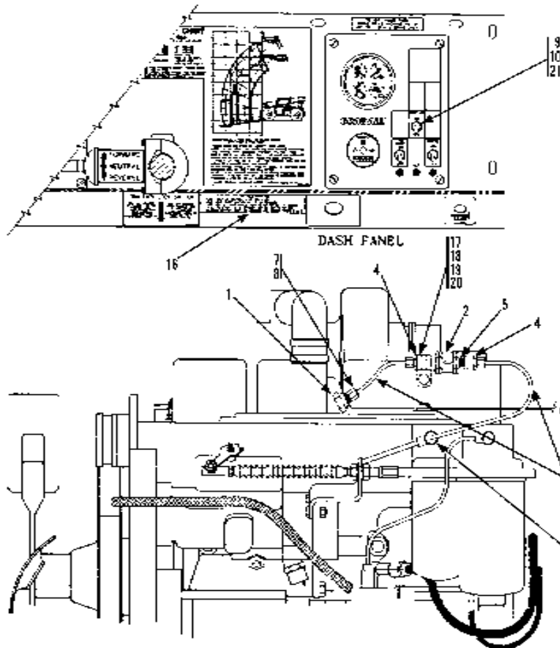
PARTIAL VIEW - ENGINE LEFT SIDE
