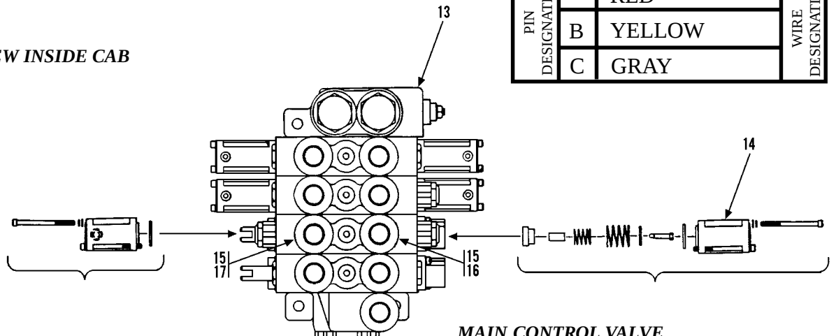
MAIN CONTROL VALVE
