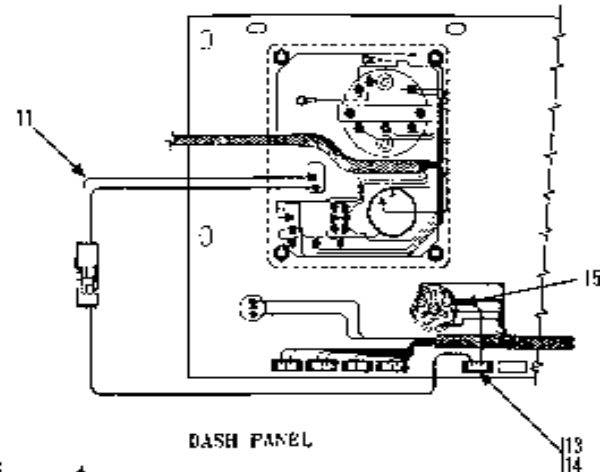
PARTIAL VIEW FROM UNDER DASH
