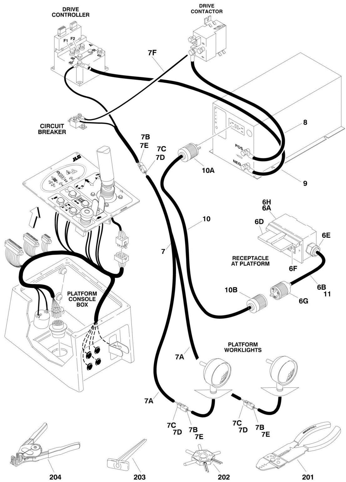
FIGURE 7-4. OPTIONAL ELECTRICAL COMPONENTS INSTALLATION
