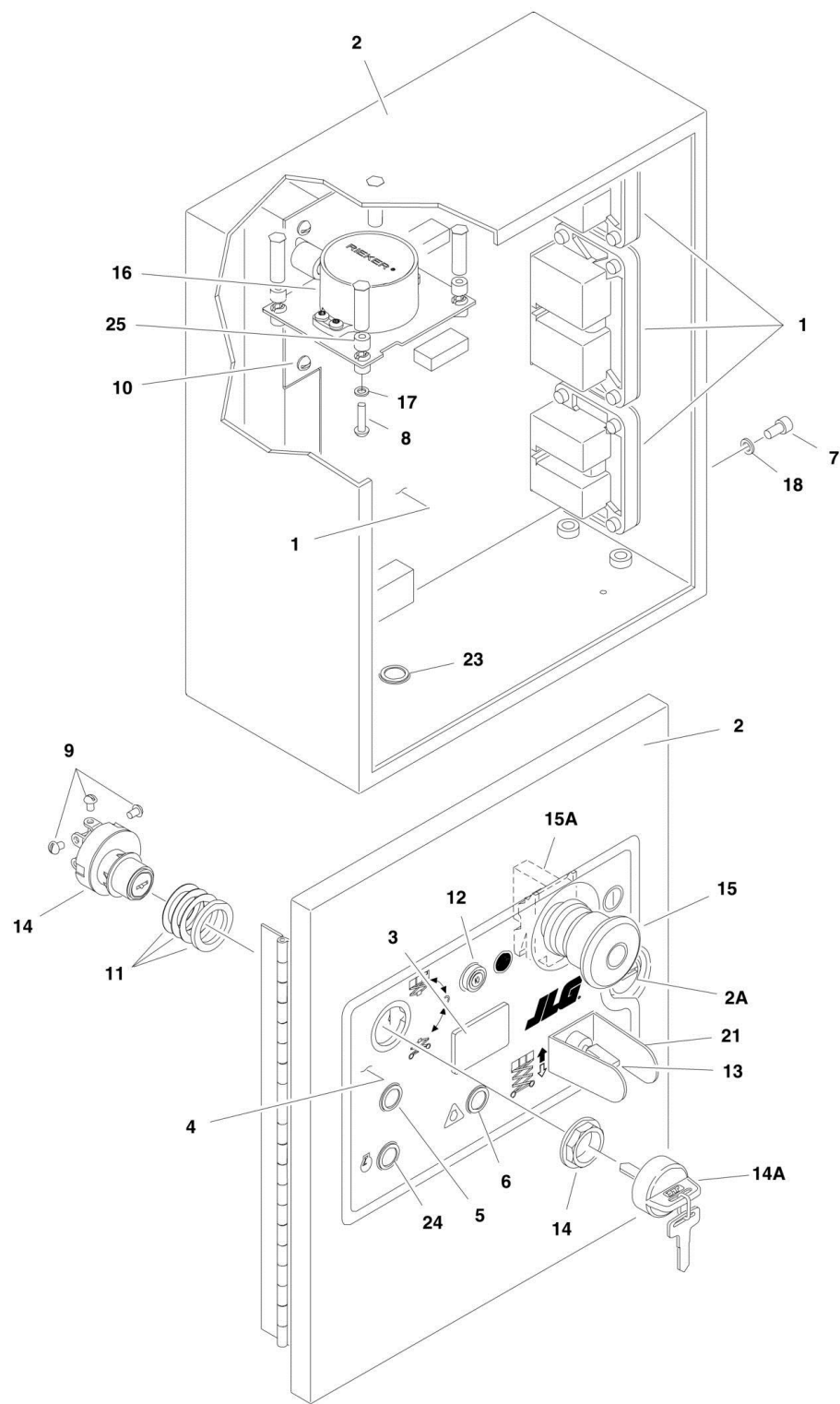
FIGURE 2-3. GROUND CONTROL BOX ASSEMBLY
