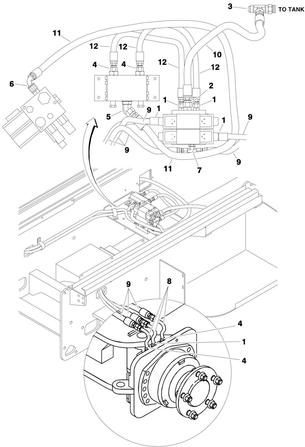
FIGURE 6-3. HYDRAULIC DIAGRAM - 4WD (OPTIONAL)
