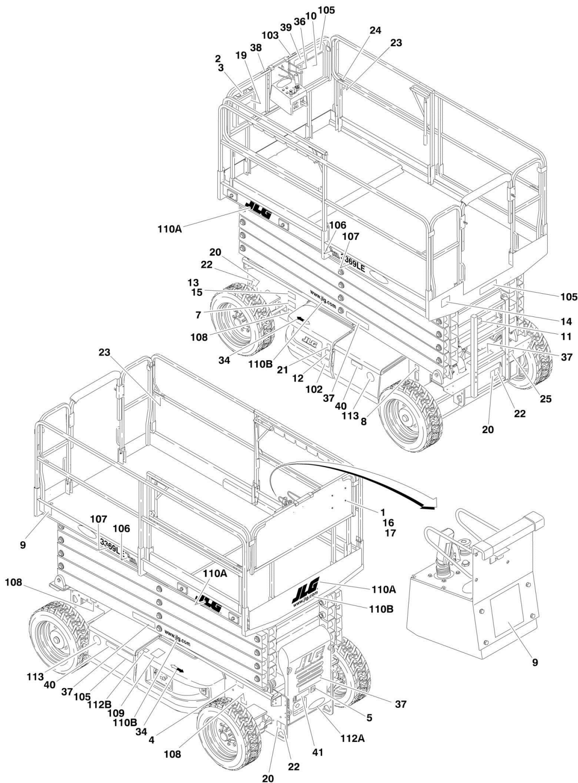
FIGURE 8-1. DECAL INSTALLATION - ANSI SPECS
