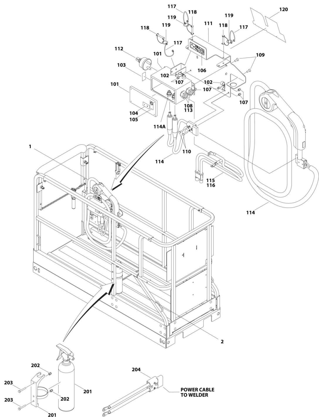
FIGURE 4-14. QUIK WELDER INSTALLATION (SN 0200123646 through 0200135154, SN 1200002324 through 1200004293)
