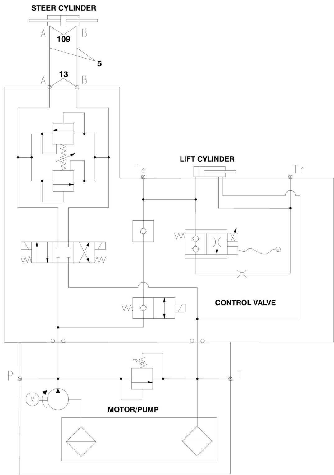
FIGURE 6-1. HYDRAULIC DIAGRAM
