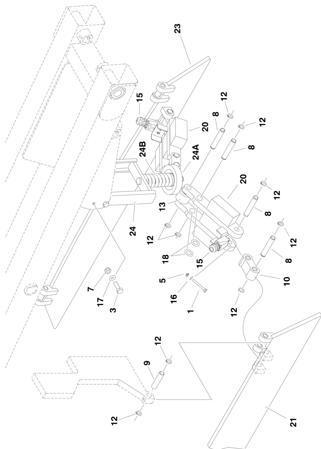
FIGURE 1-5. POTHOLE PROTECTION INSTALLATION (1930ES/2030ES/2630ES)
