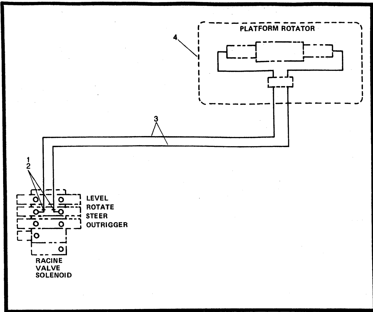
Figure 2-52. Hydraulic Rotate Circuit.
