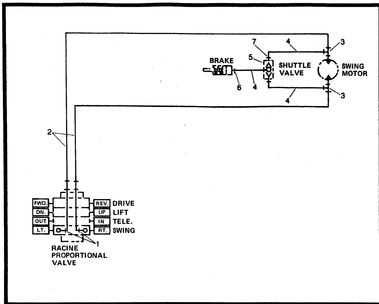
Figure 2-42. Hydraulic Swing Circuit.
