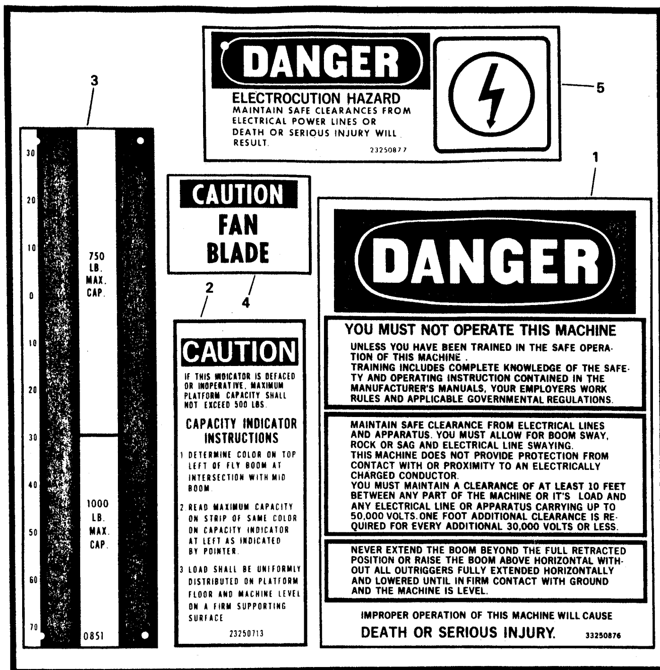
Figure 2-58. Nameplate Details.
