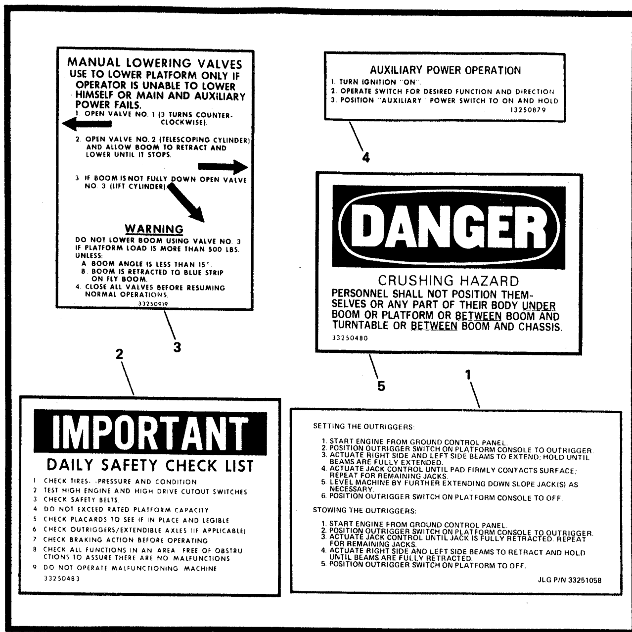
Figure 2-59. Nameplate Details.
