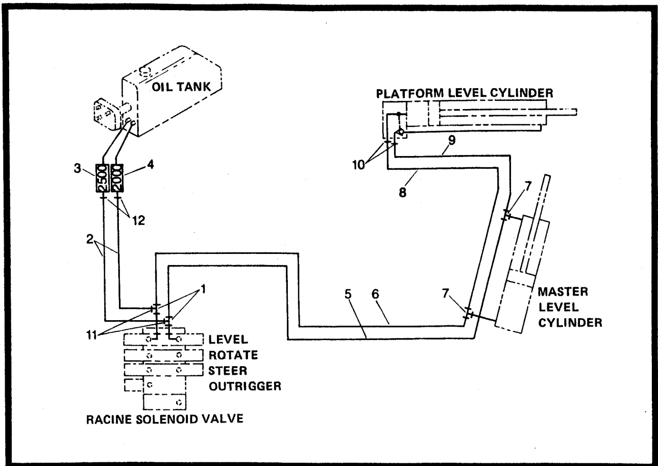
Figure 2-51. Hydraulic Level Circuit.
