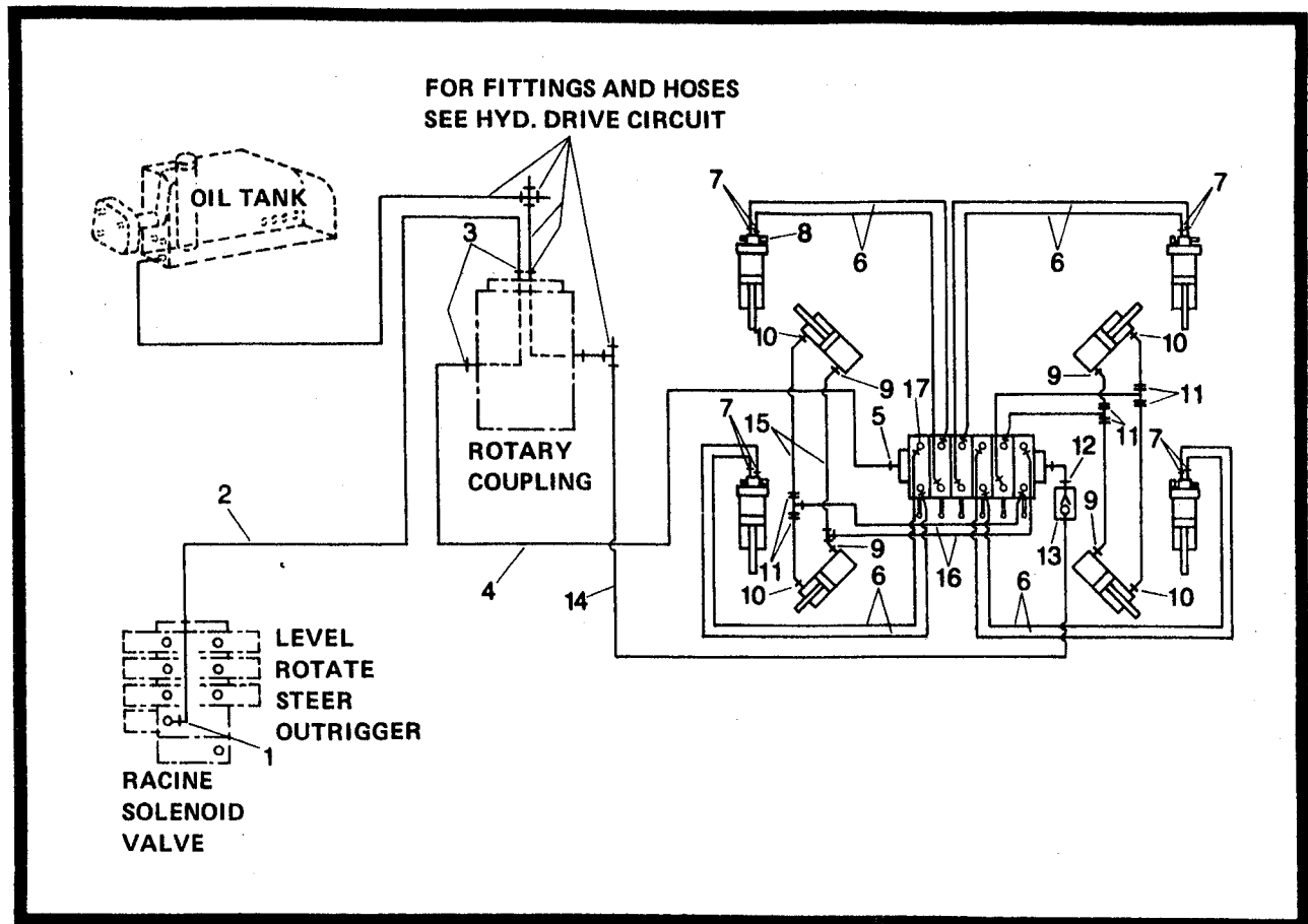
Figure 2-55. Hydraulic Outrigger Circuit.
