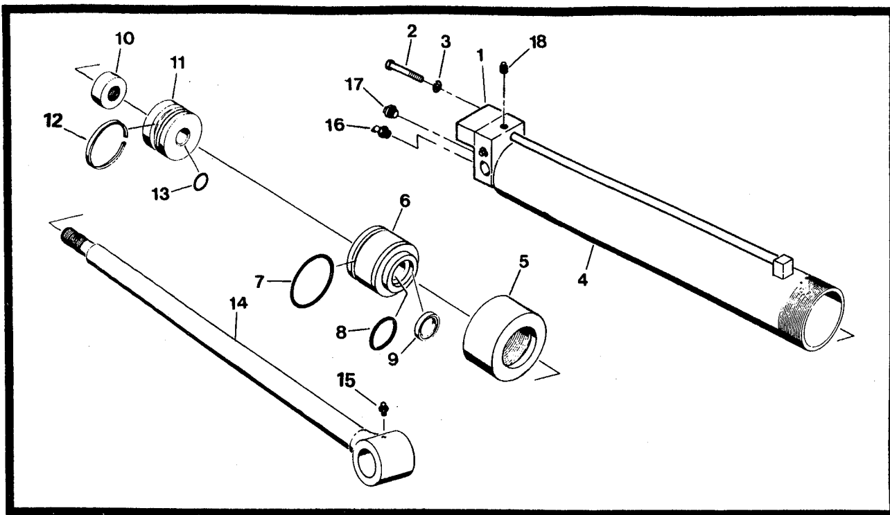
Figure 2-6. Slave Level Cylinder Assembly.
