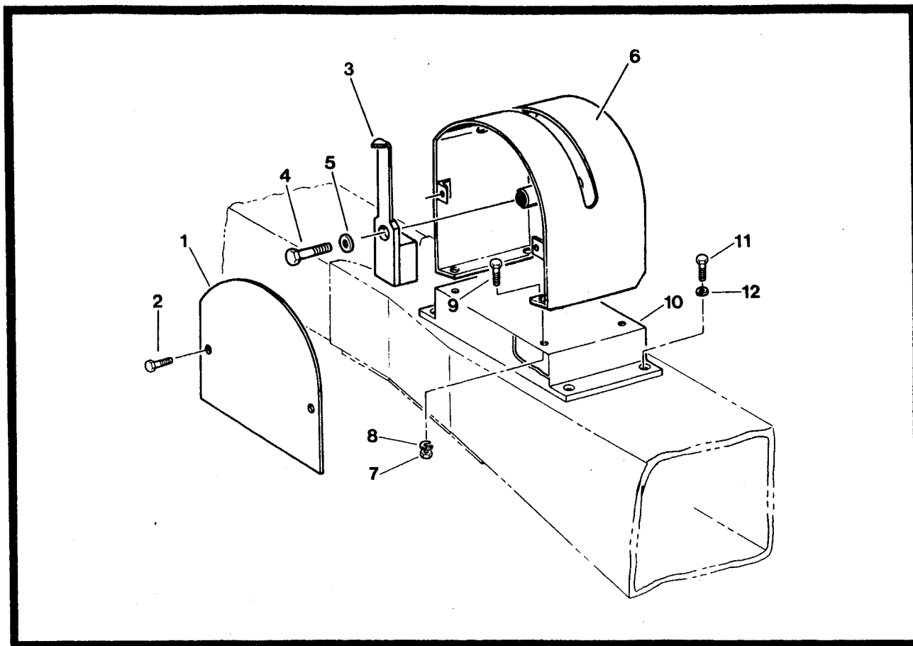
Figure 2-4. Capacity Indicator Installation.
