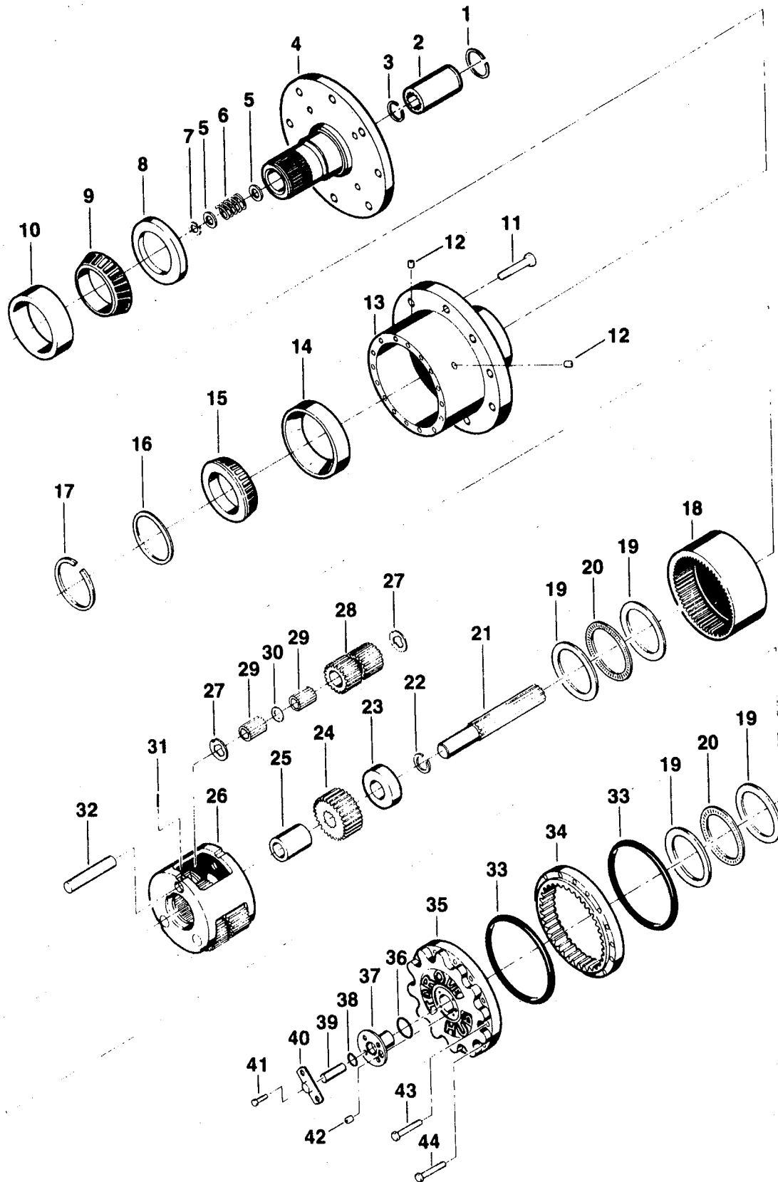
Figure 2-31. Wheel Drive Hub Assembly (Outrigger Machines).
