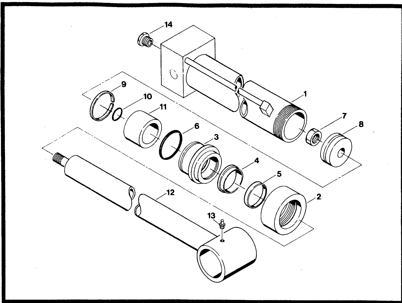
Figure 2-36. Outrigger Extension Cylinder Assembly.
