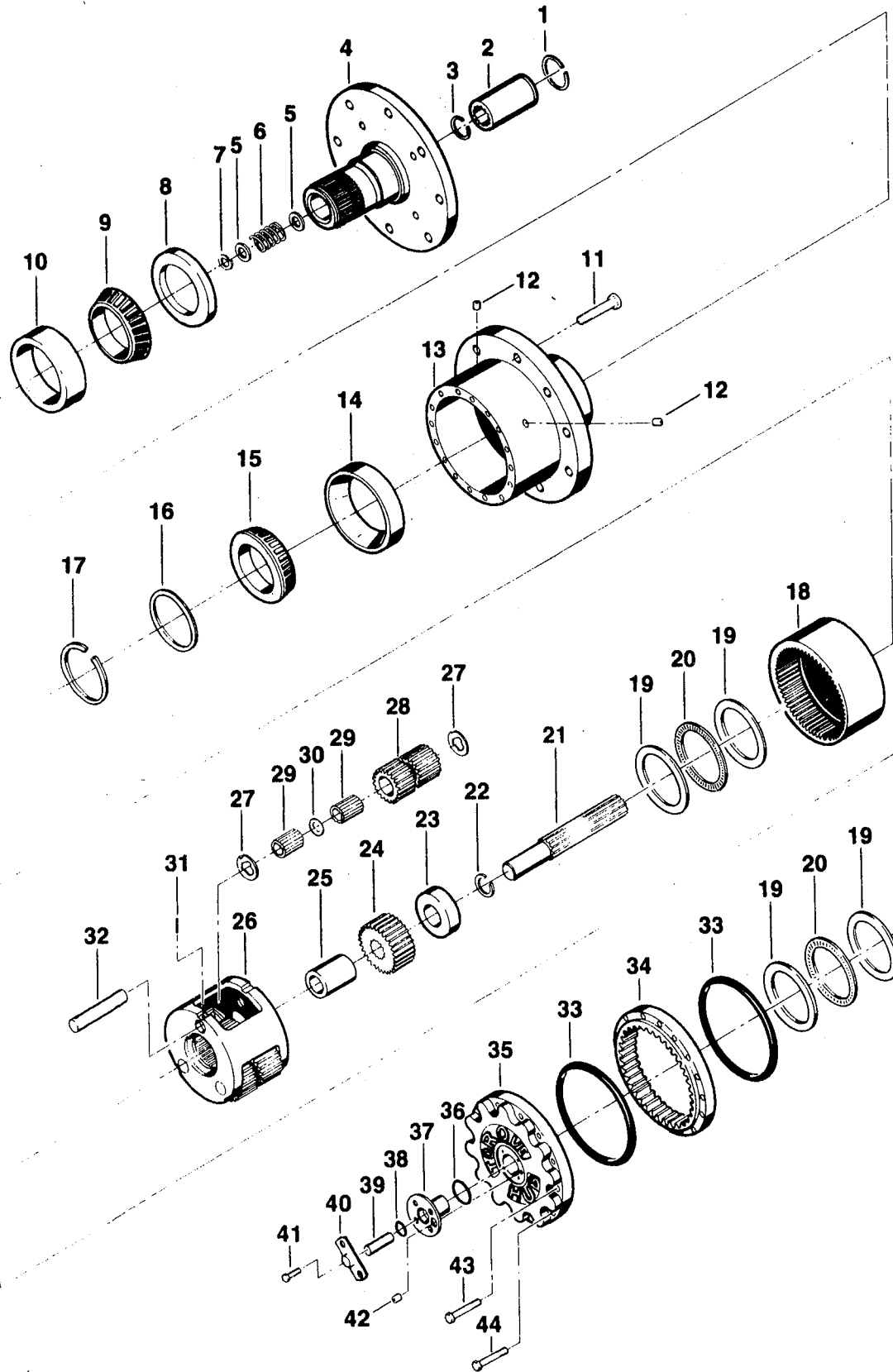
Figure 2-41. Wheel Drive Hub Assembly (Extending Axle Machines).
