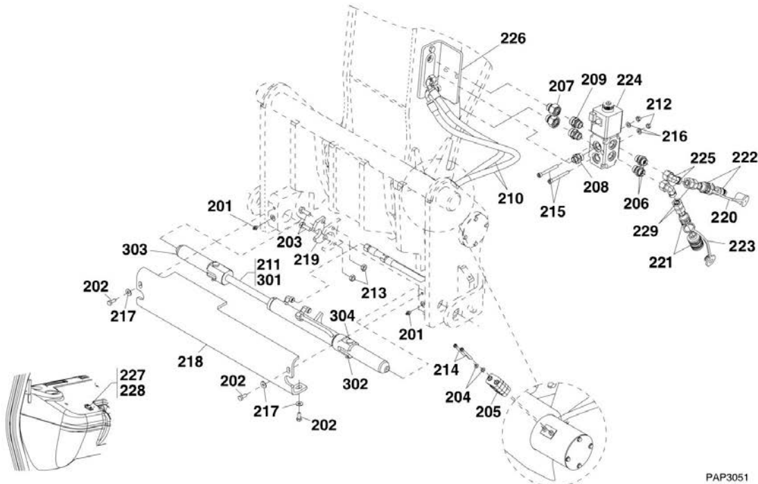
HYDRAULIC QUICK ATTACH W/ ELECTRIC VALVE
