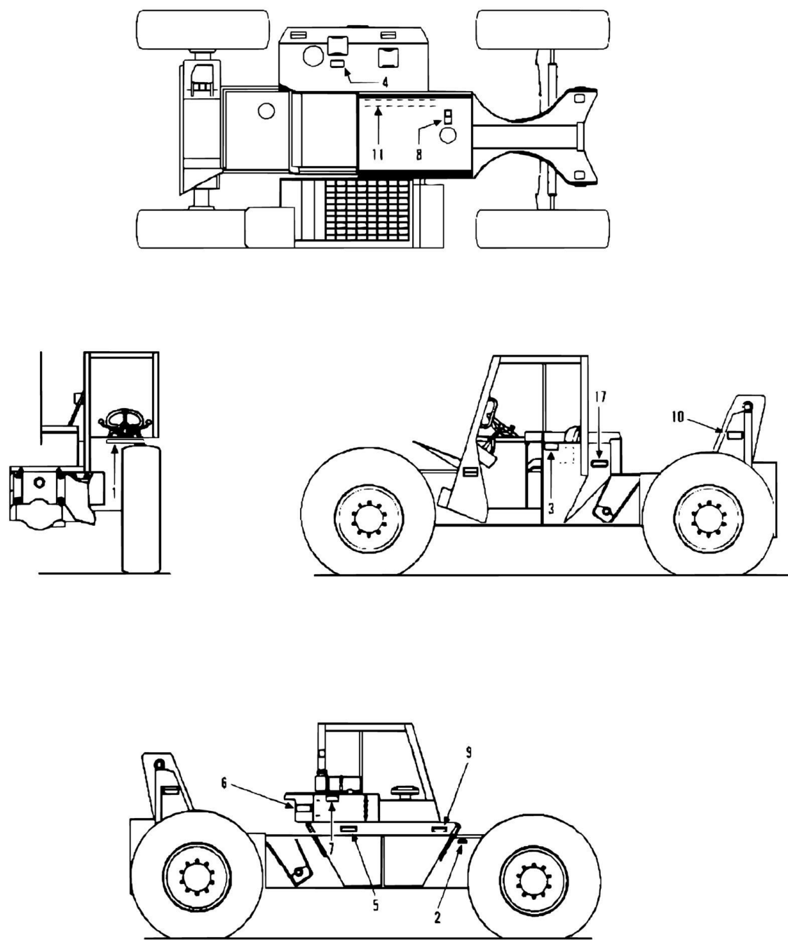
FIGURE 11-1. FRAME DECALS (SN 0144860S to Present)
