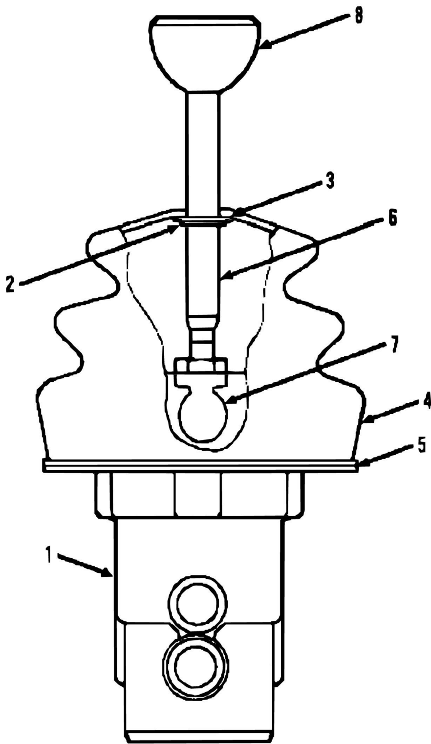
FIGURE 12-28. HYDRAULIC CONTROLLER (SN 0144860S to Present)
