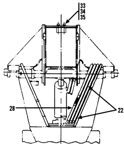
AUXILIARY VIEW OF REAR OF BOOM
