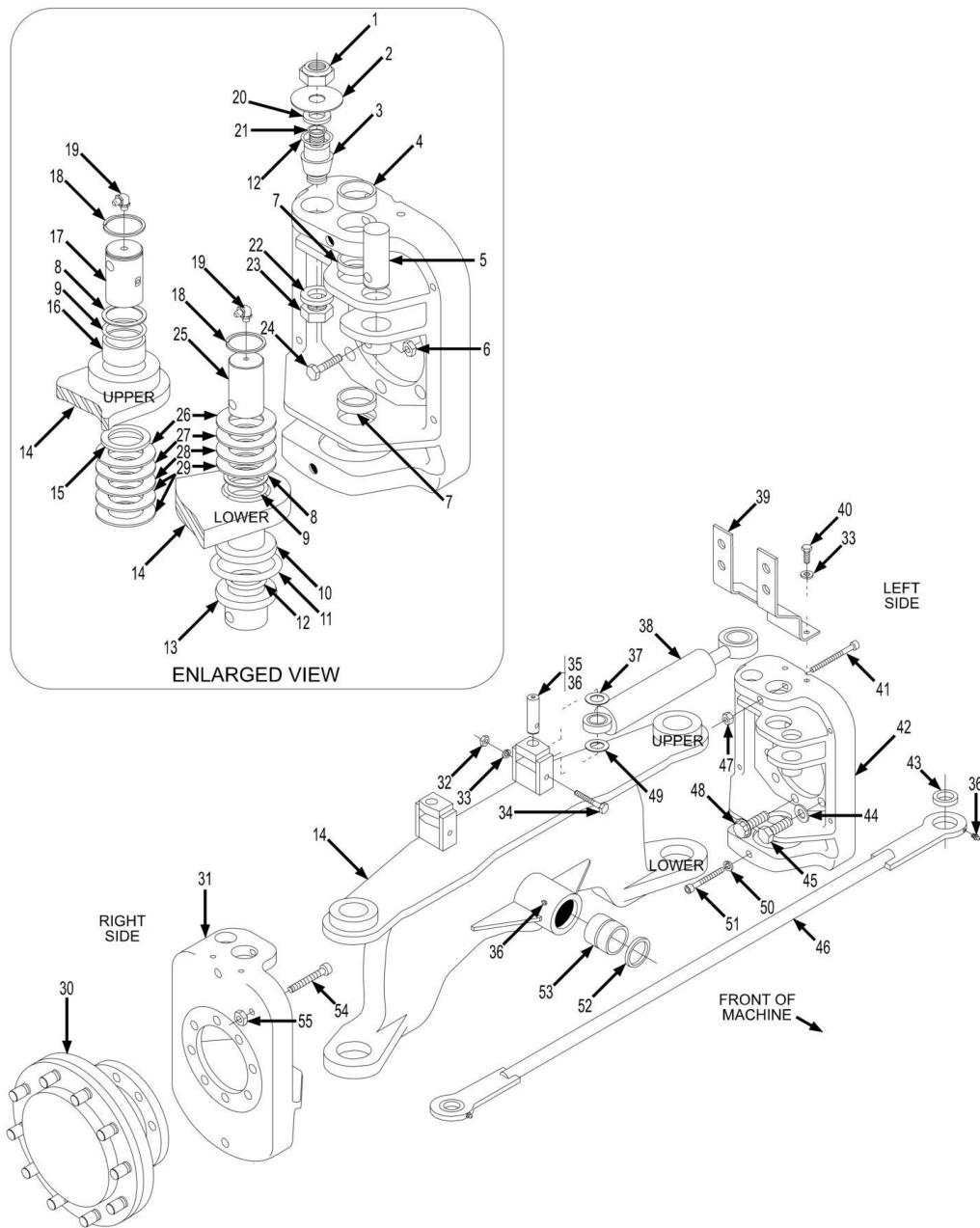
FIGURE 12-28. (91335026) REAR AXLE ADVANTAGE KIT FOR SERVICE ONLY
