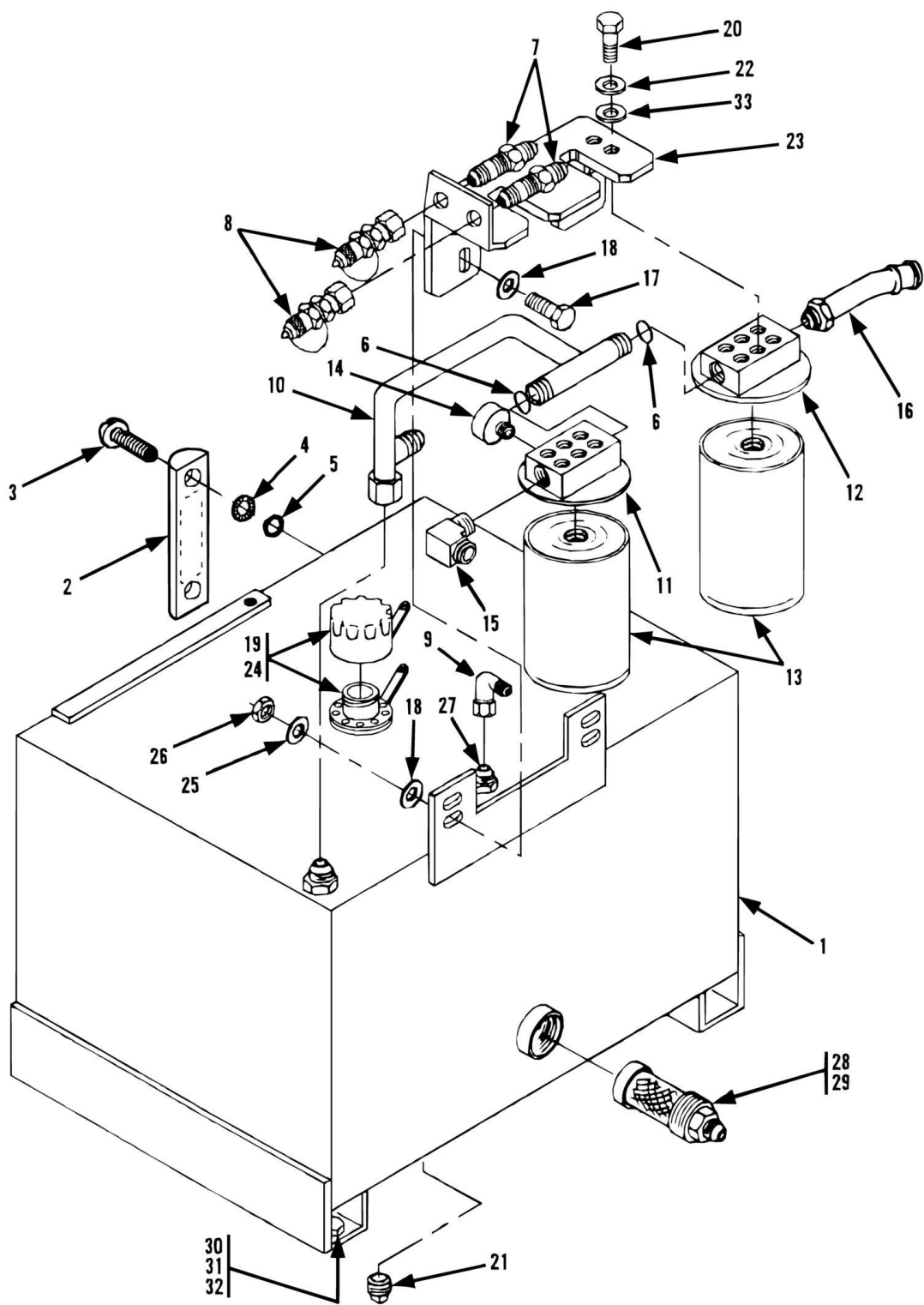
FIGURE 9-18. (91125069) HYDRAULIC RESERVOIR AND FILTER (SN 0277001 to Present)
