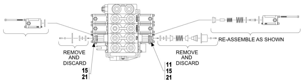
VALVE POSITIONER CONVERSION FROM MANUAL TO HYDRAULIC ACTUATION
