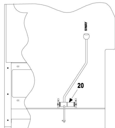
REAR VIEW OF CAB
