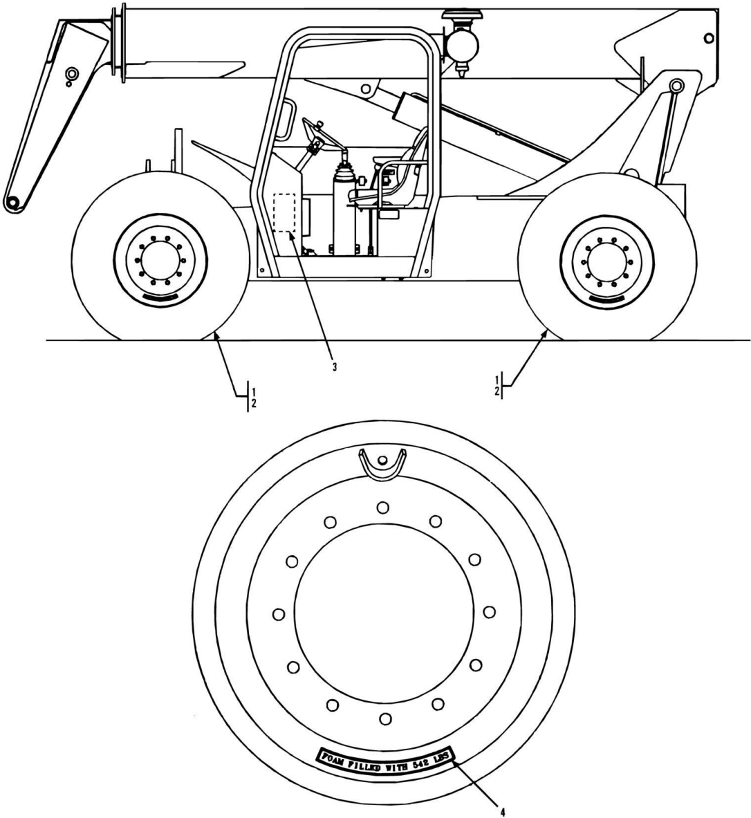
VIEW SHOWING DECAL PLACEMENT ON RIM
