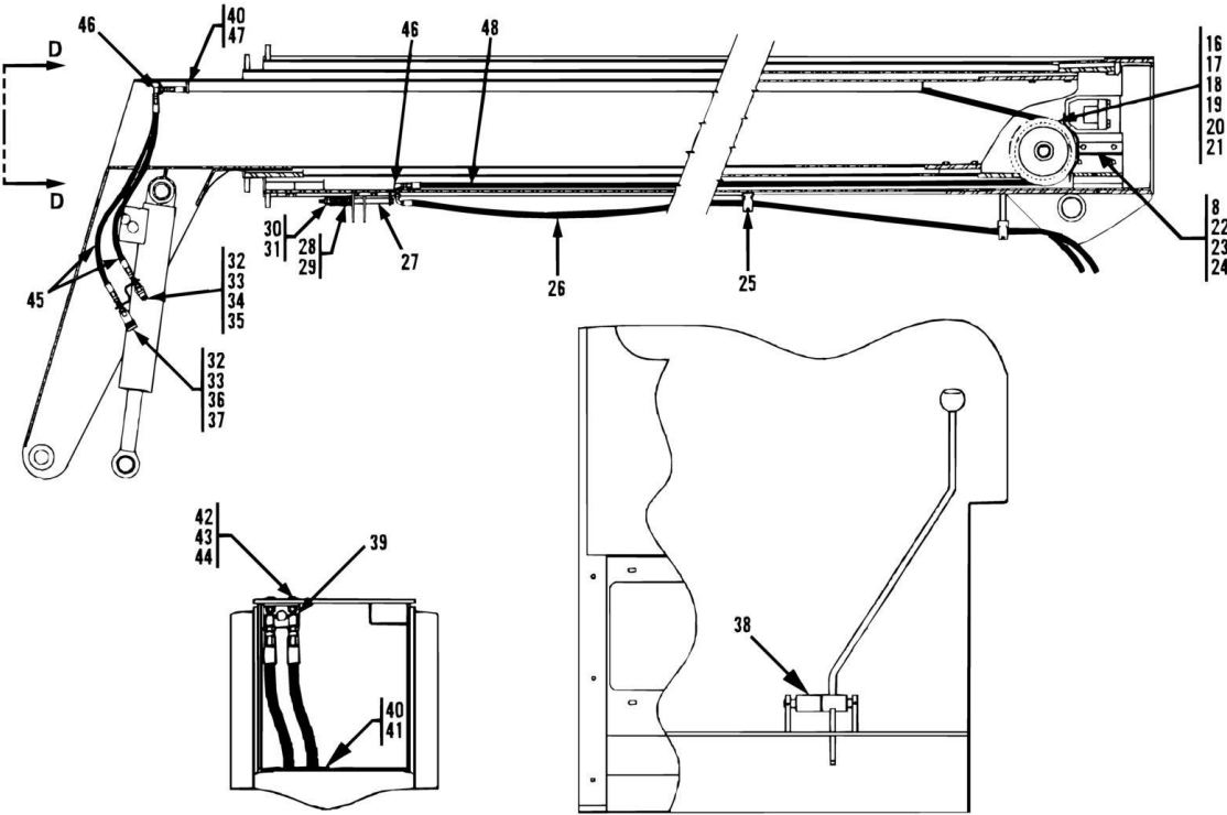
VIEW D - D
