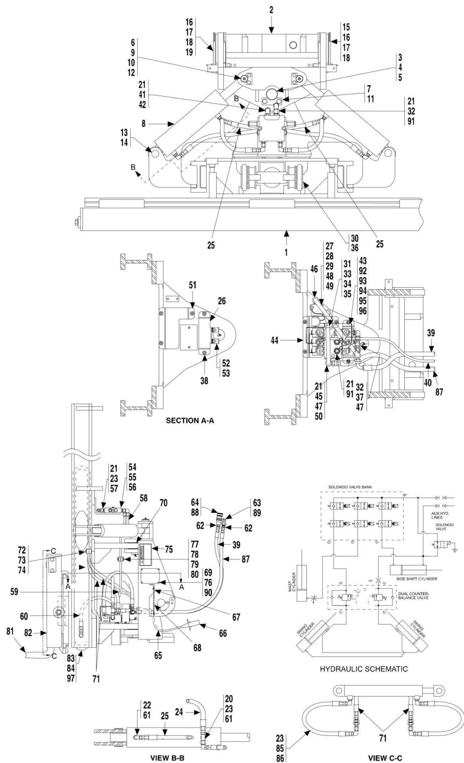
FIGURE 3-12. (90455047) 6FT SWING MAST W/SIDE SHIFT (SN 0344001 to Present, SN 0266001 to Present)
