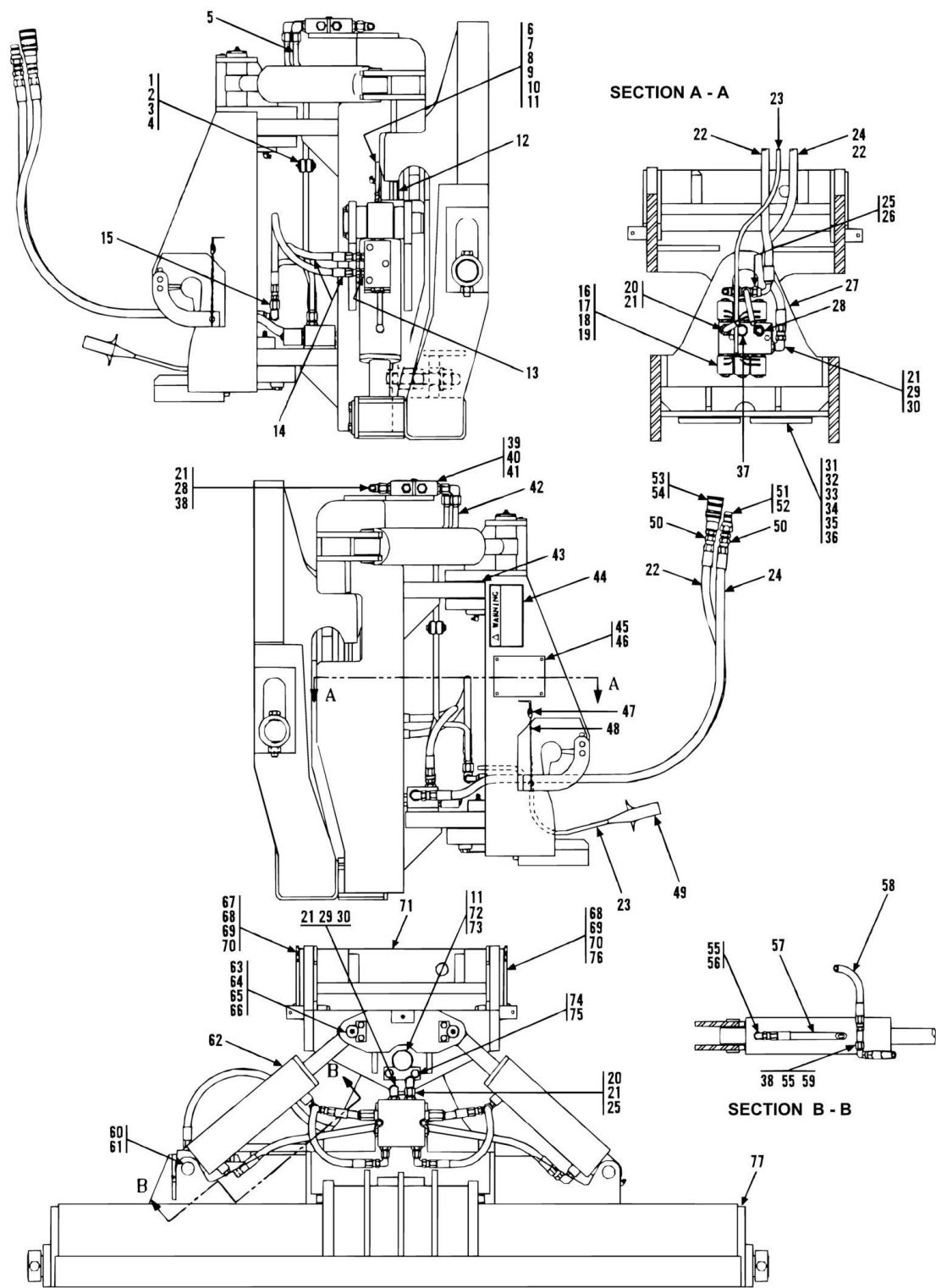
FIGURE 3-14. (91305021) SWINGING SLOPE PILER (SN 0344001 to Present, SN 0266001 to Present)
