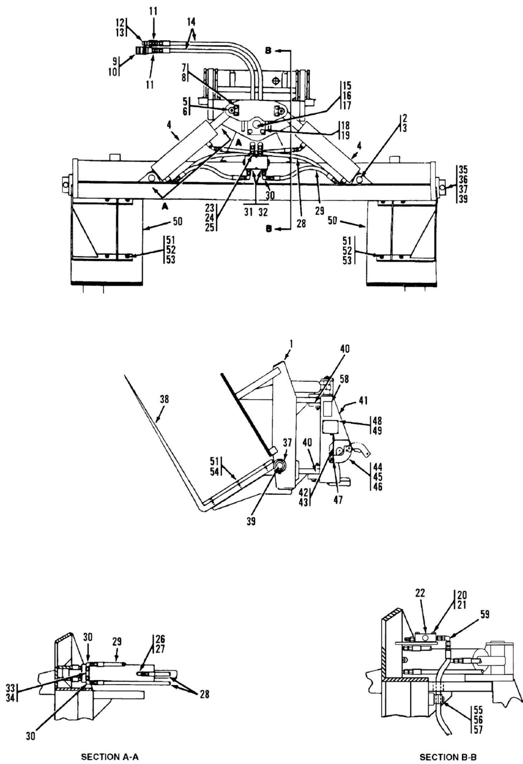
FIGURE 3-13. (90555013) 100, DRYWALL SWING FORK ASSEMBLY
