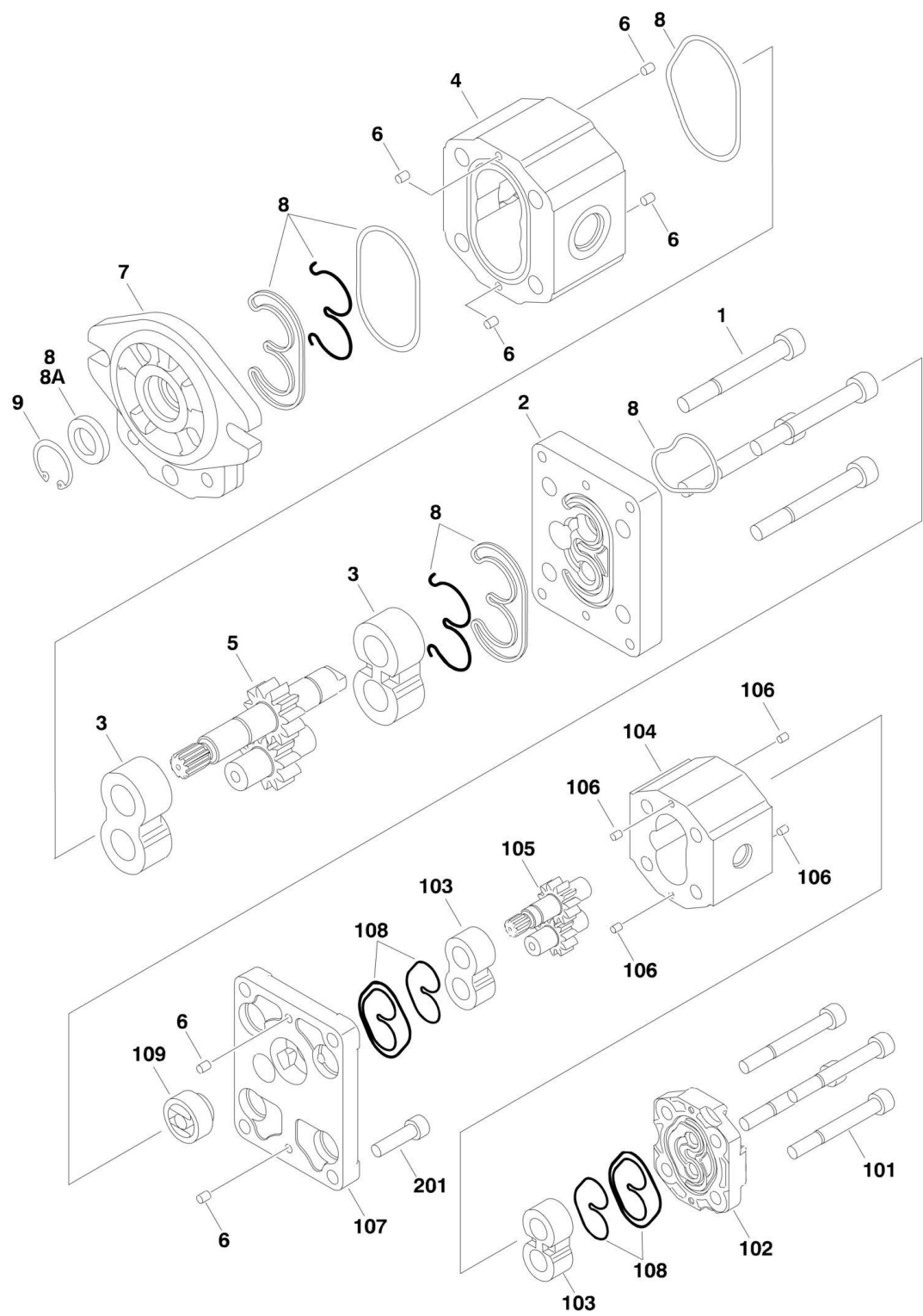
FIGURE 2-9. GEAR PUMP ASSEMBLY
