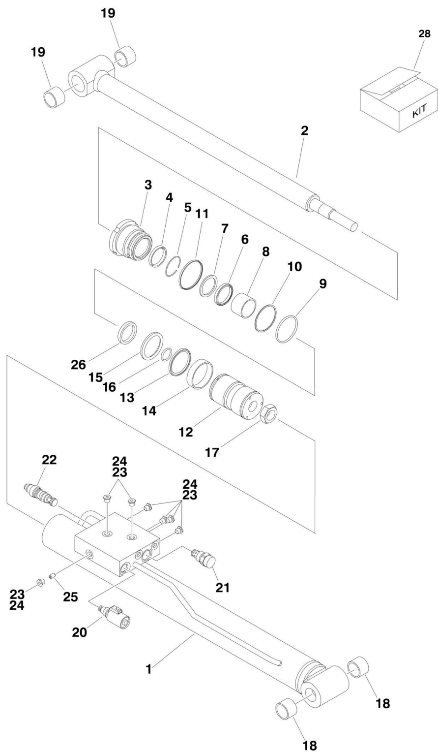
FIGURE 5-4. LIFT (JIB) CYLINDER ASSEMBLY
