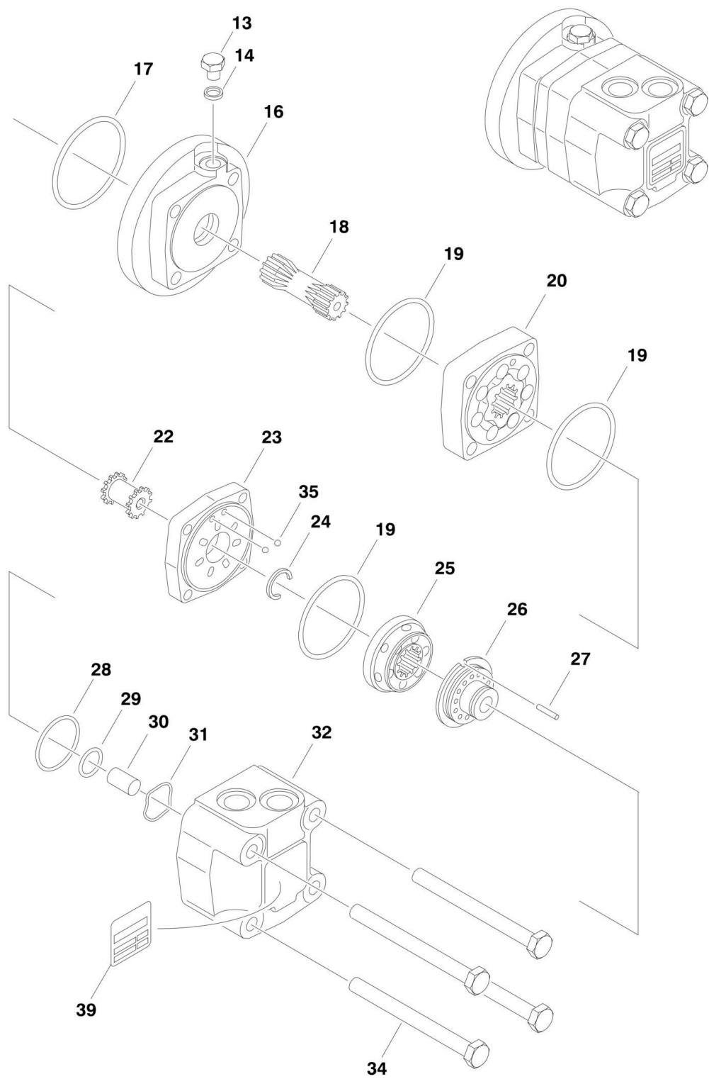
FIGURE 1-3. DRIVE MOTOR ASSEMBLY
