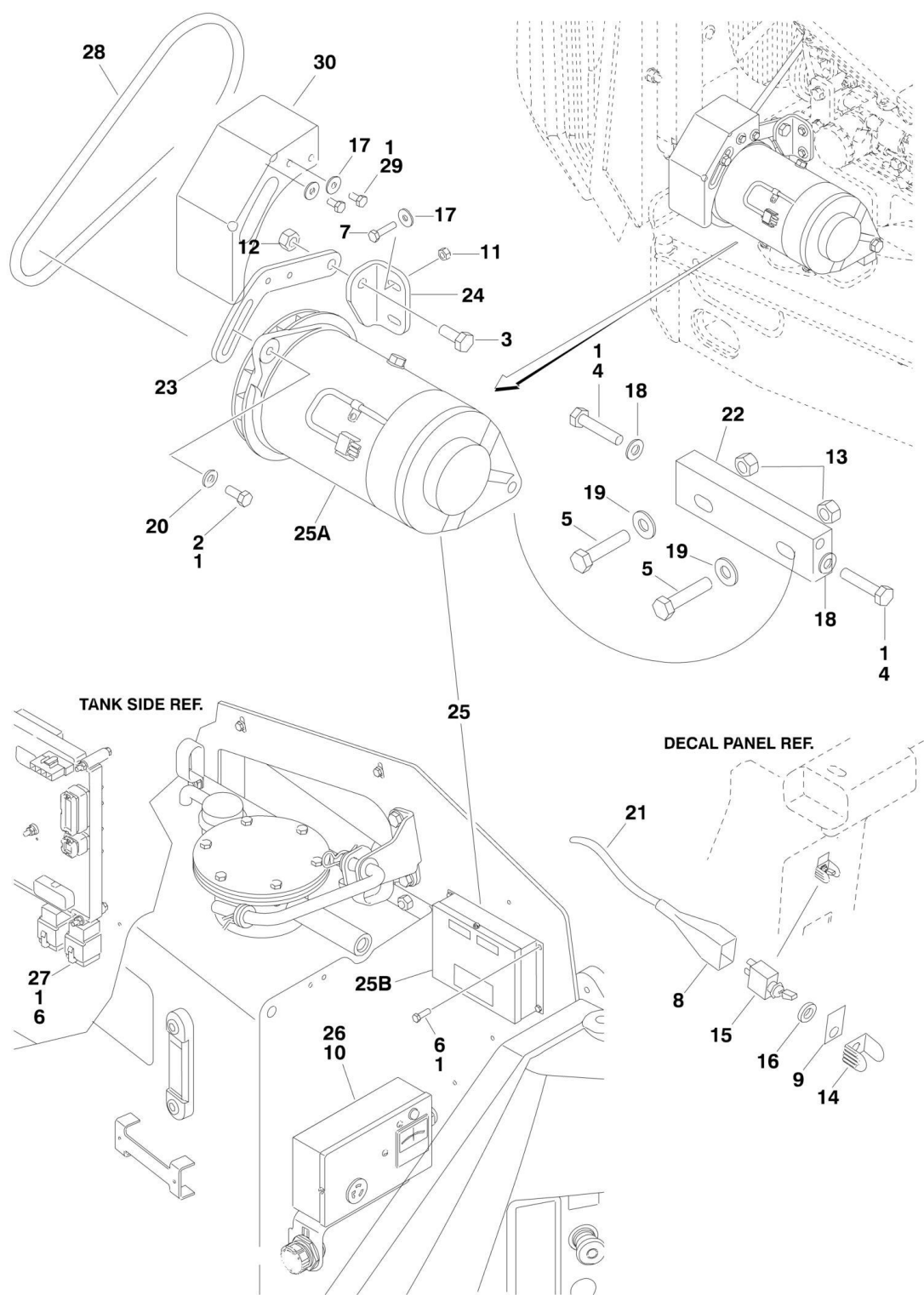
FIGURE 2-14. GENERATOR INSTALLATION - GM ENGINE MACHINES (OPTIONAL)
