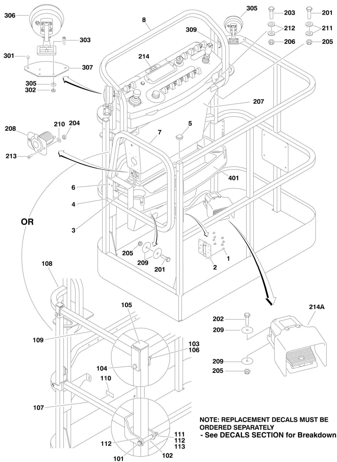
FIGURE 4-1. PLATFORM ASSEMBLY
