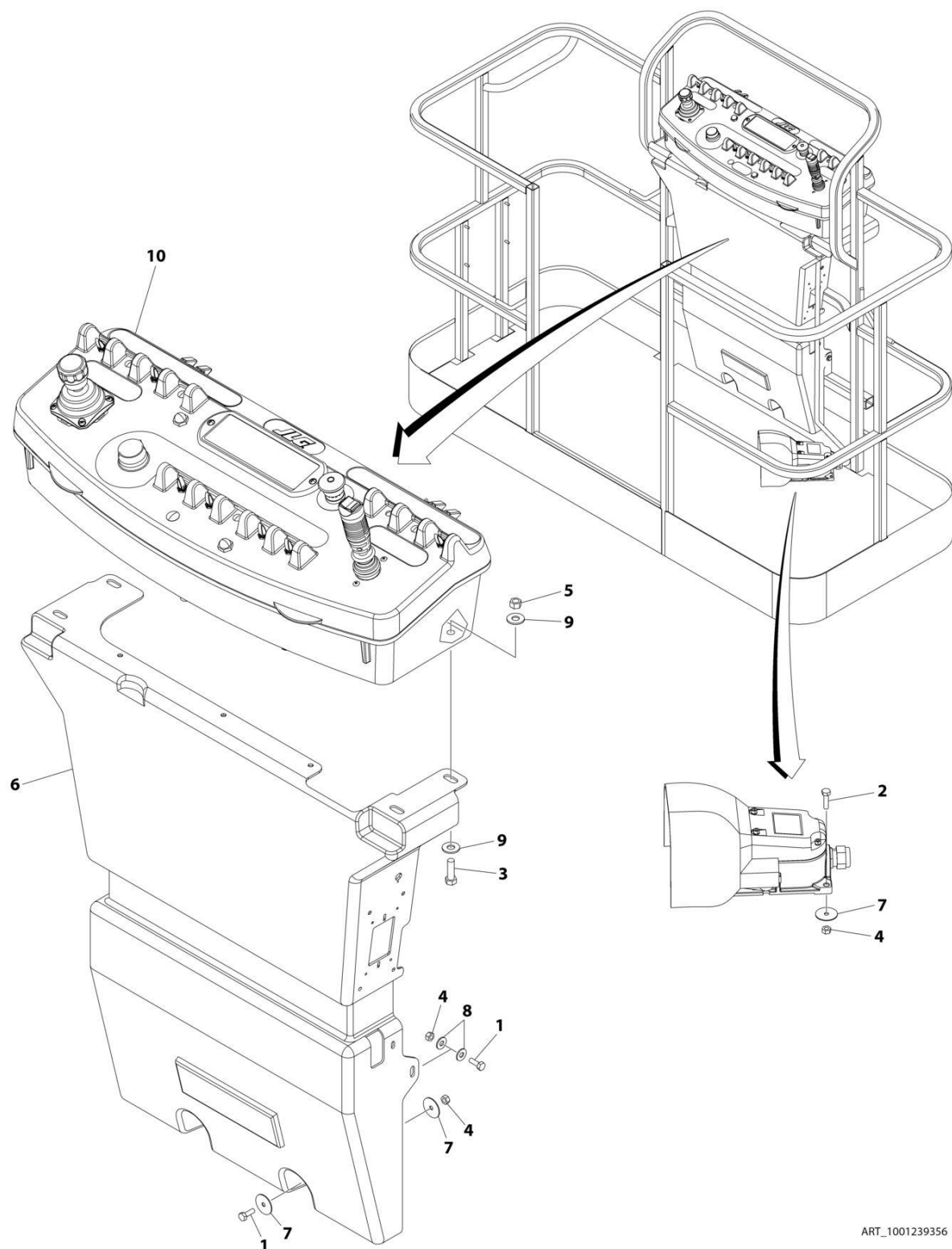
FIGURE 4-9. PLATFORM CONSOLE AND FOOTSWITCH INSTALLATION - E300AJ WITH SKYGUARD (UL SPECS) (SN 0300256384 through 0300272206)
