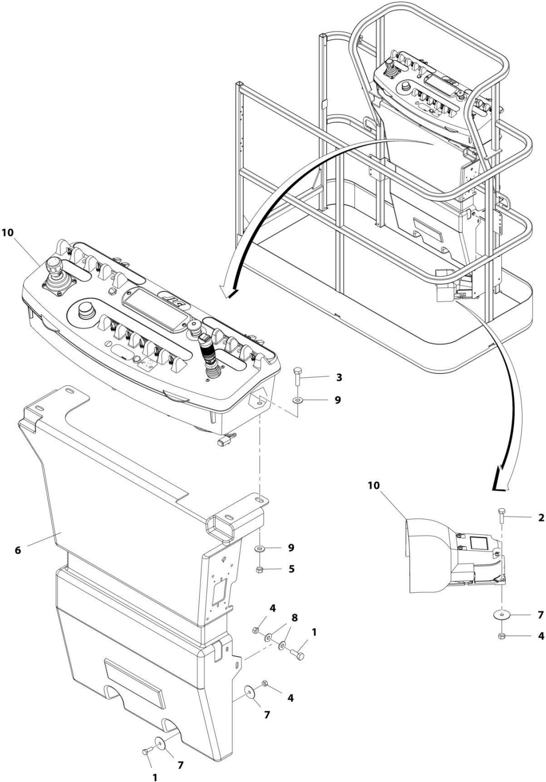
FIGURE 4-11. PLATFORM CONSOLE AND FOOTSWITCH INSTALLATION WITH 4 CELL LSS - E300AJP WITH SKYGUARD (SN 0300211844 through 0300256384)
