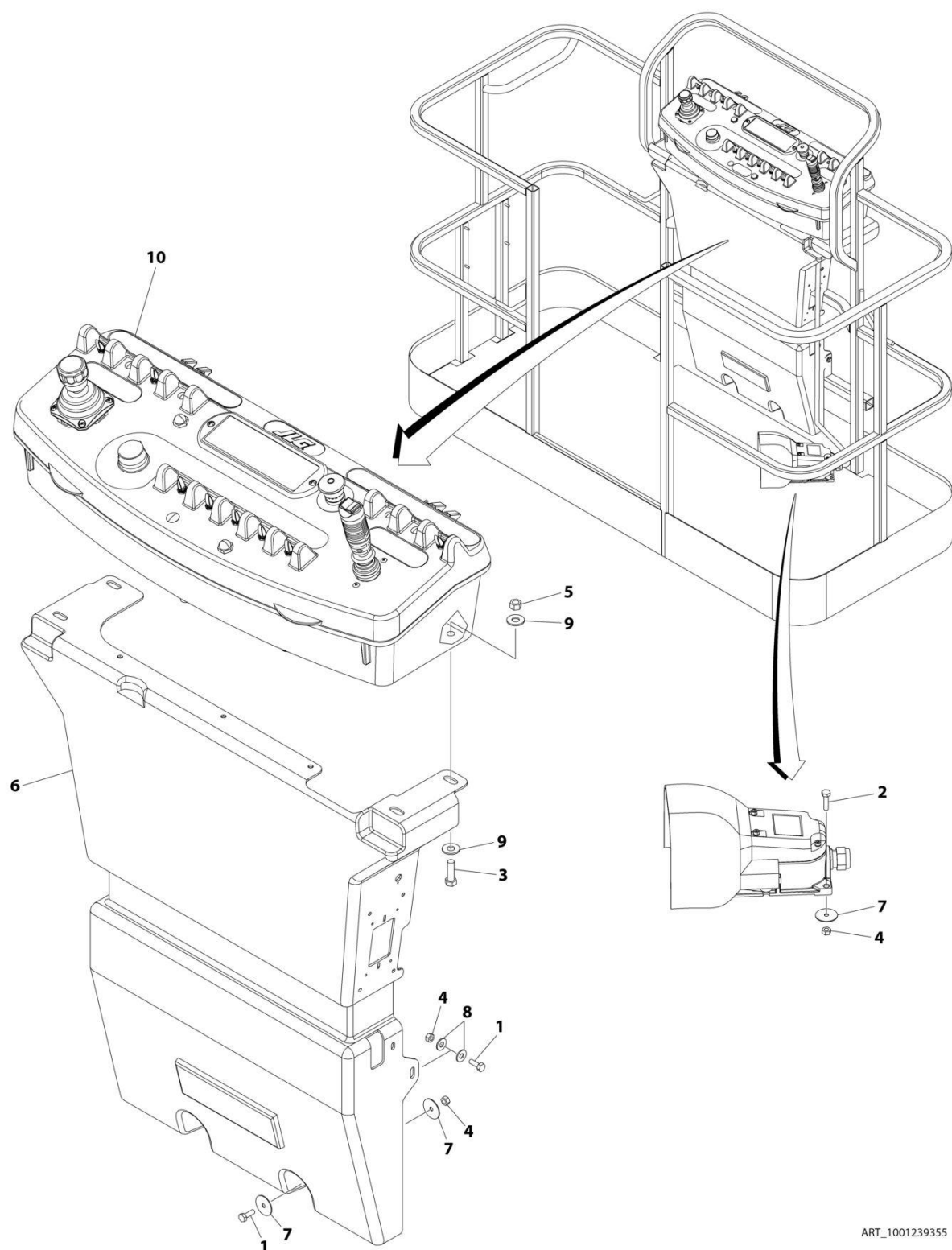
FIGURE 4-12. PLATFORM CONSOLE AND FOOTSWITCH INSTALLATION WITH 4 CELL LSS - E300AJP WITH SKYGUARD (SN 0300256384 through 0300272206)
