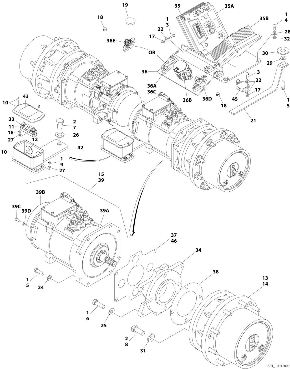
FIGURE 1-5. WHEEL DRIVE INSTALLATION (UL SPECS) (SN 0300226252 through 0300272206)
