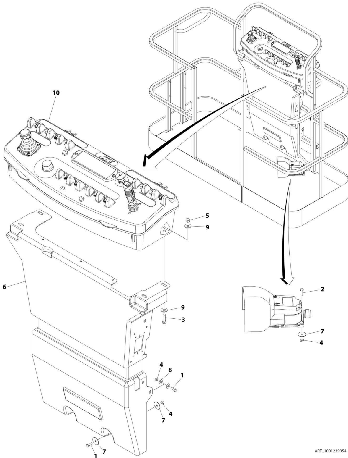
FIGURE 4-6. PLATFORM CONSOLE AND FOOTSWITCH INSTALLATION WITH 4 CELL LSS - E300AJ WITH SKYGUARD (SN 0300256384 through 0300272206)
