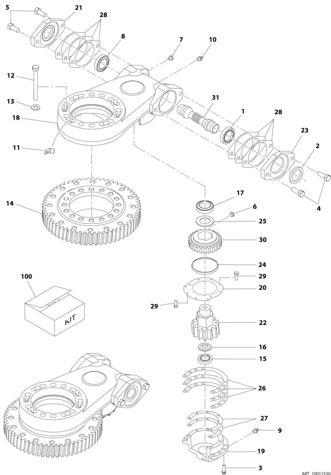
FIGURE 2-9. TURNTABLE BEARING ASSEMBLY - JING WEI
