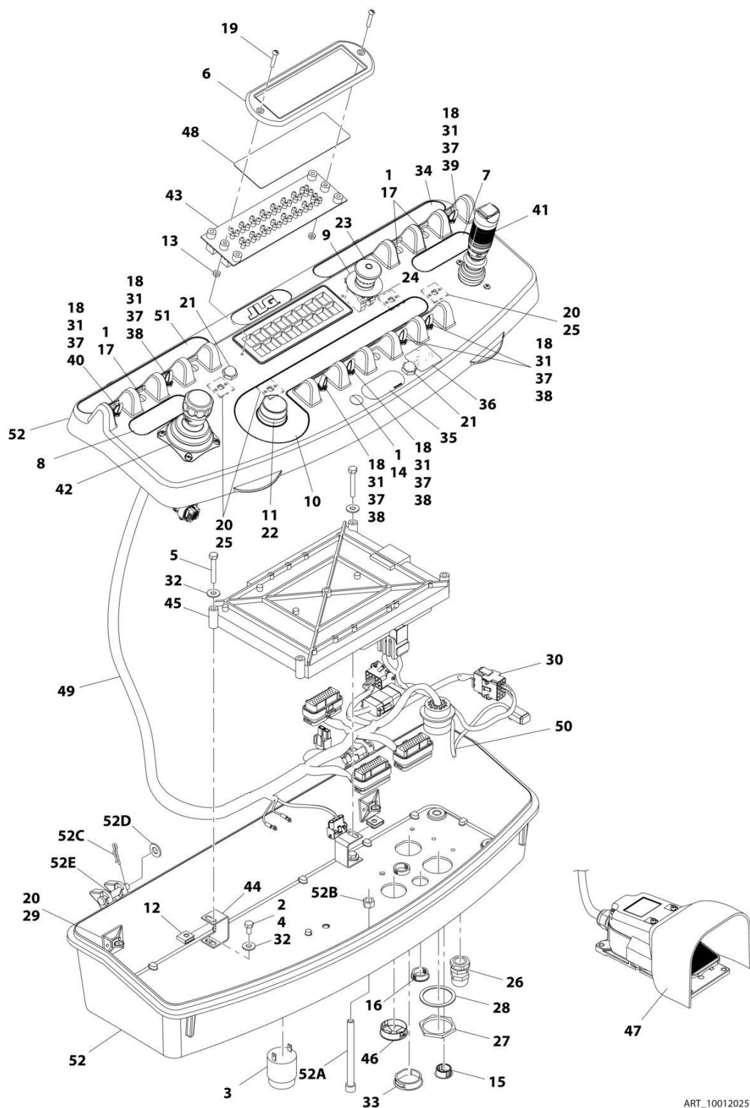
FIGURE 4-17. PLATFORM CONSOLE ASSEMBLY WITH 4 CELL LSS - E300AJ WITH SKYGUARD (SN 0300211844 through 0300256384)
