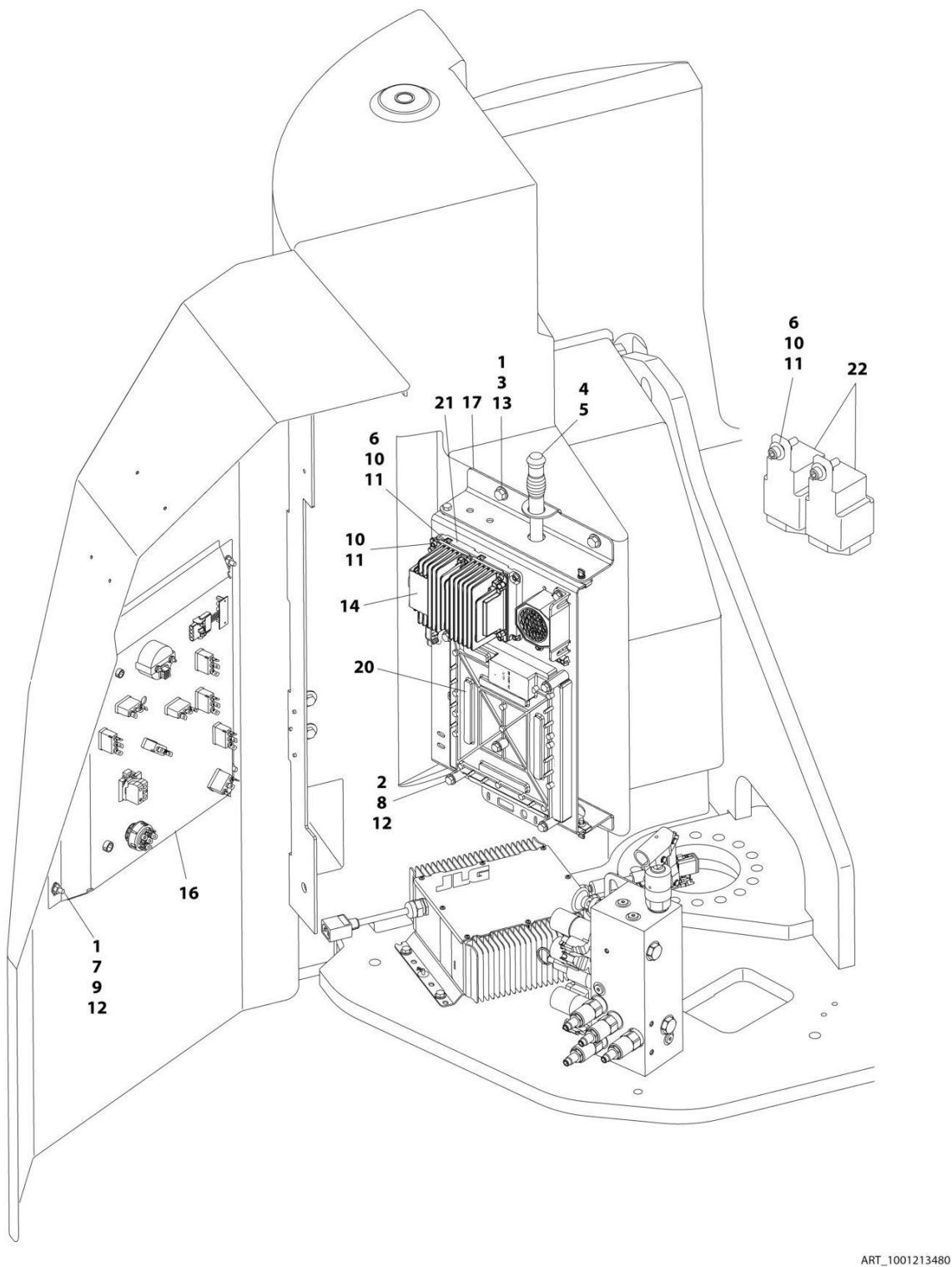
FIGURE 2-17. ELECTRICAL COMPONENTS INSTALLATION - E300AJP (UL SPECS) (SN 0300226252 through 0300272206)
