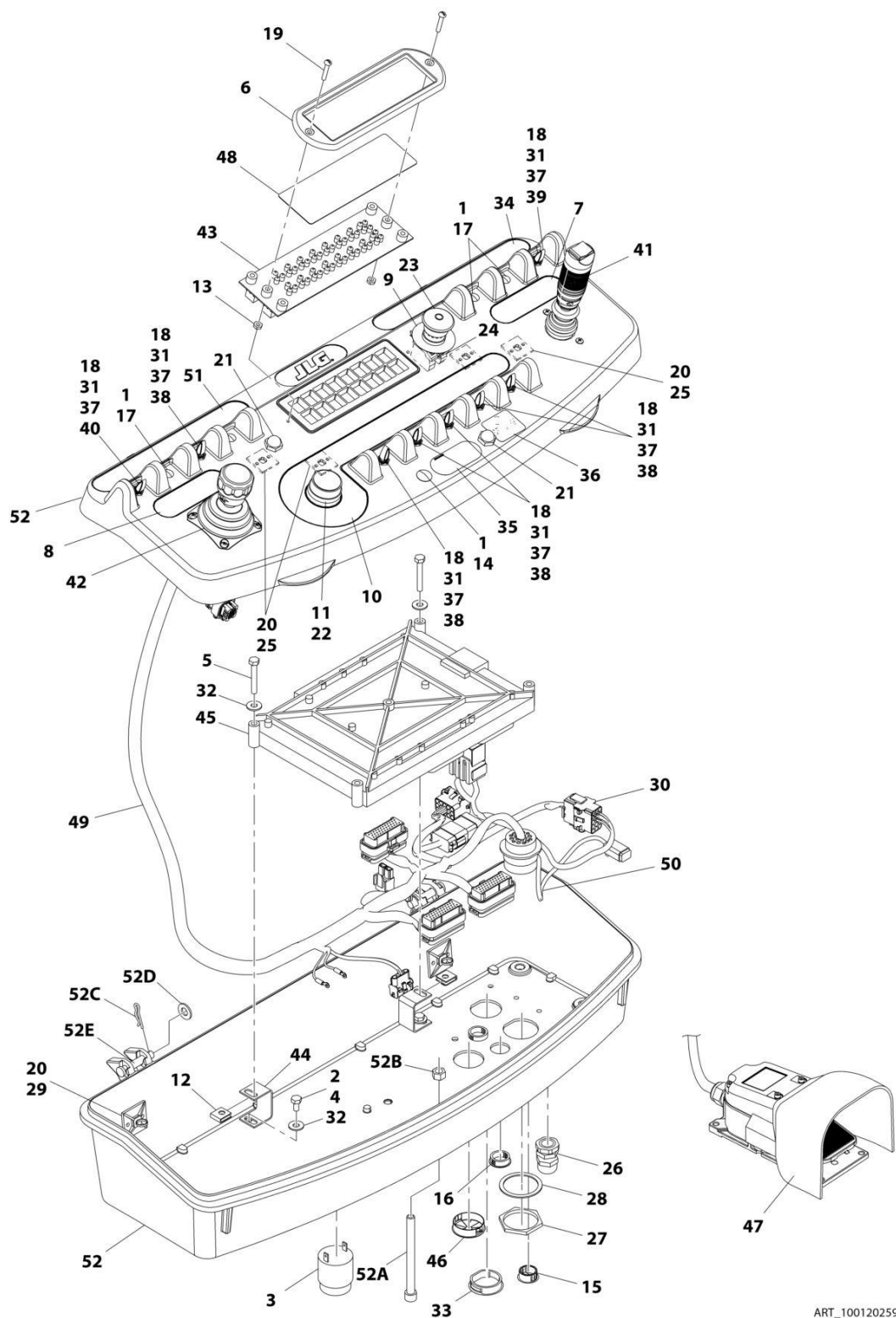
FIGURE 4-23. PLATFORM CONSOLE ASSEMBLY WITH 4 CELL LSS - E300AJP WITH SKYGUARD (SN 0300211844 through 0300256384)
