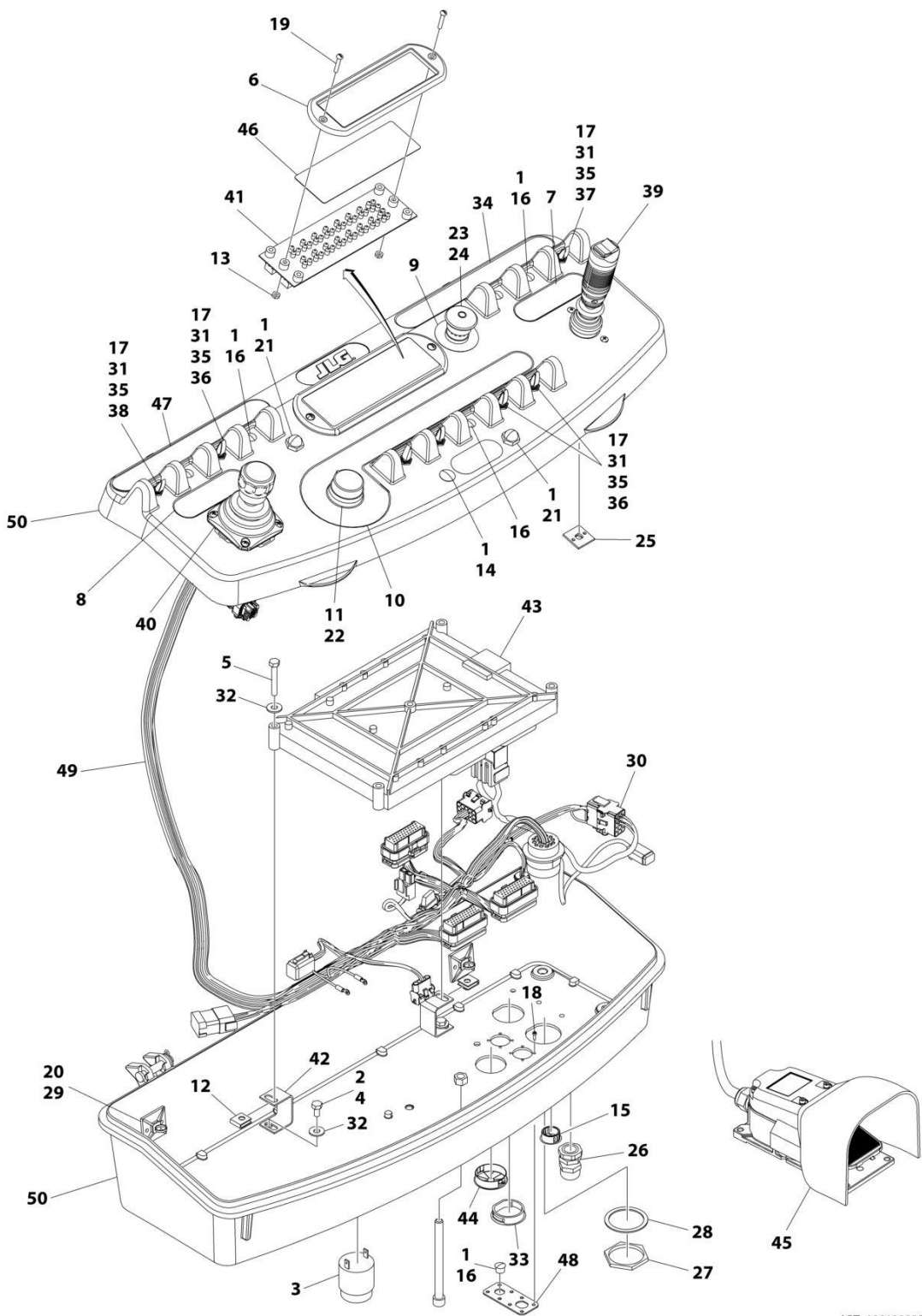
FIGURE 4-18. PLATFORM CONSOLE ASSEMBLY WITH 4 CELL LSS - E300AJ WITH SKYGUARD (SN 0300256384 through 0300272206)
