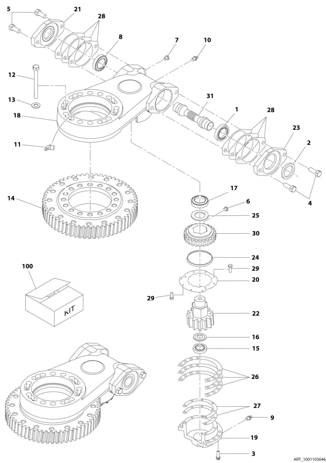
FIGURE 2-8. TURNTABLE BEARING ASSEMBLY - DOHI
