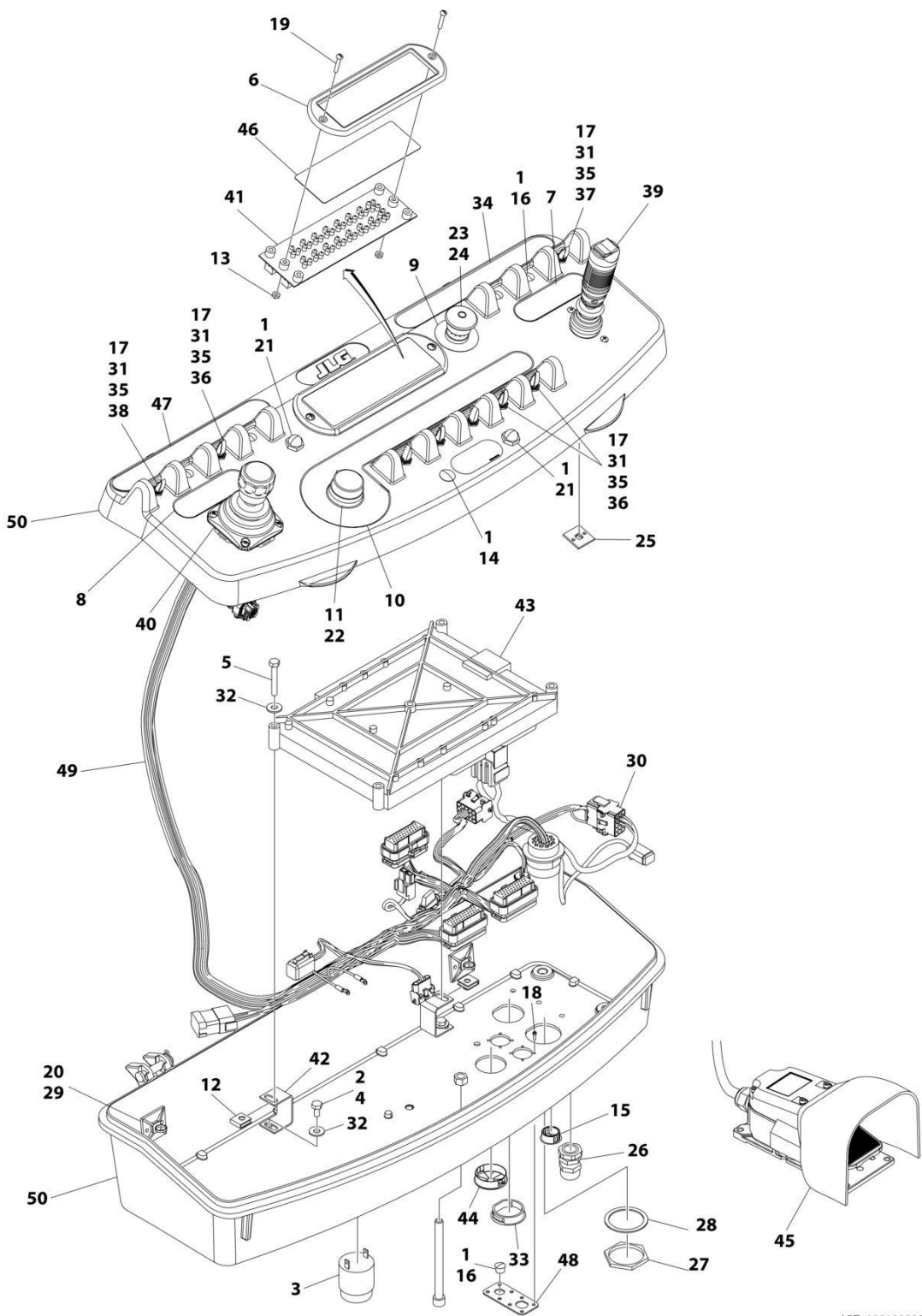
FIGURE 4-24. PLATFORM CONSOLE ASSEMBLY WITH 4 CELL LSS - E300AJP WITH SKYGUARD (SN 0300256384 through 0300272206)
