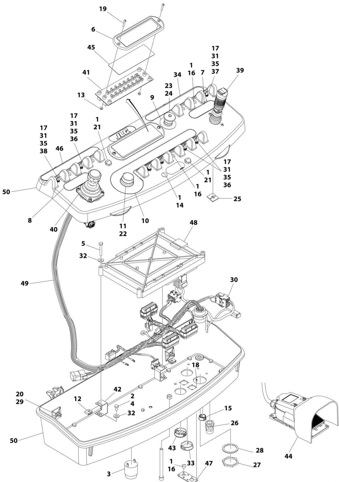
FIGURE 4-21. PLATFORM CONSOLE ASSEMBLY - E300AJ (UL SPECS) (SN 0300256384 through 0300272206)
