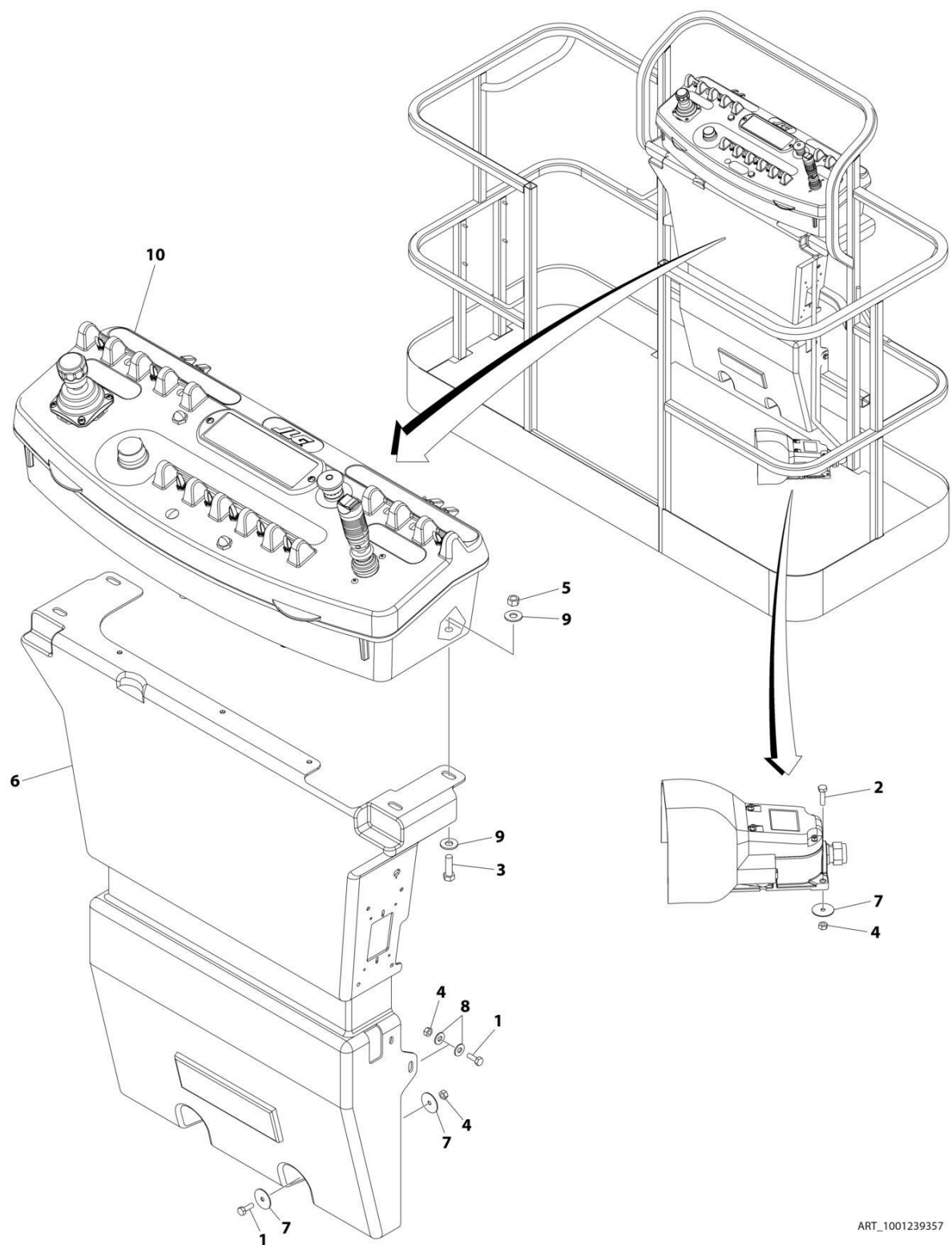
FIGURE 4-15. PLATFORM CONSOLE AND FOOTSWITCH INSTALLATION - E300AJP WITH SKYGUARD (UL SPECS) (SN 0300256384 through 0300272206)
