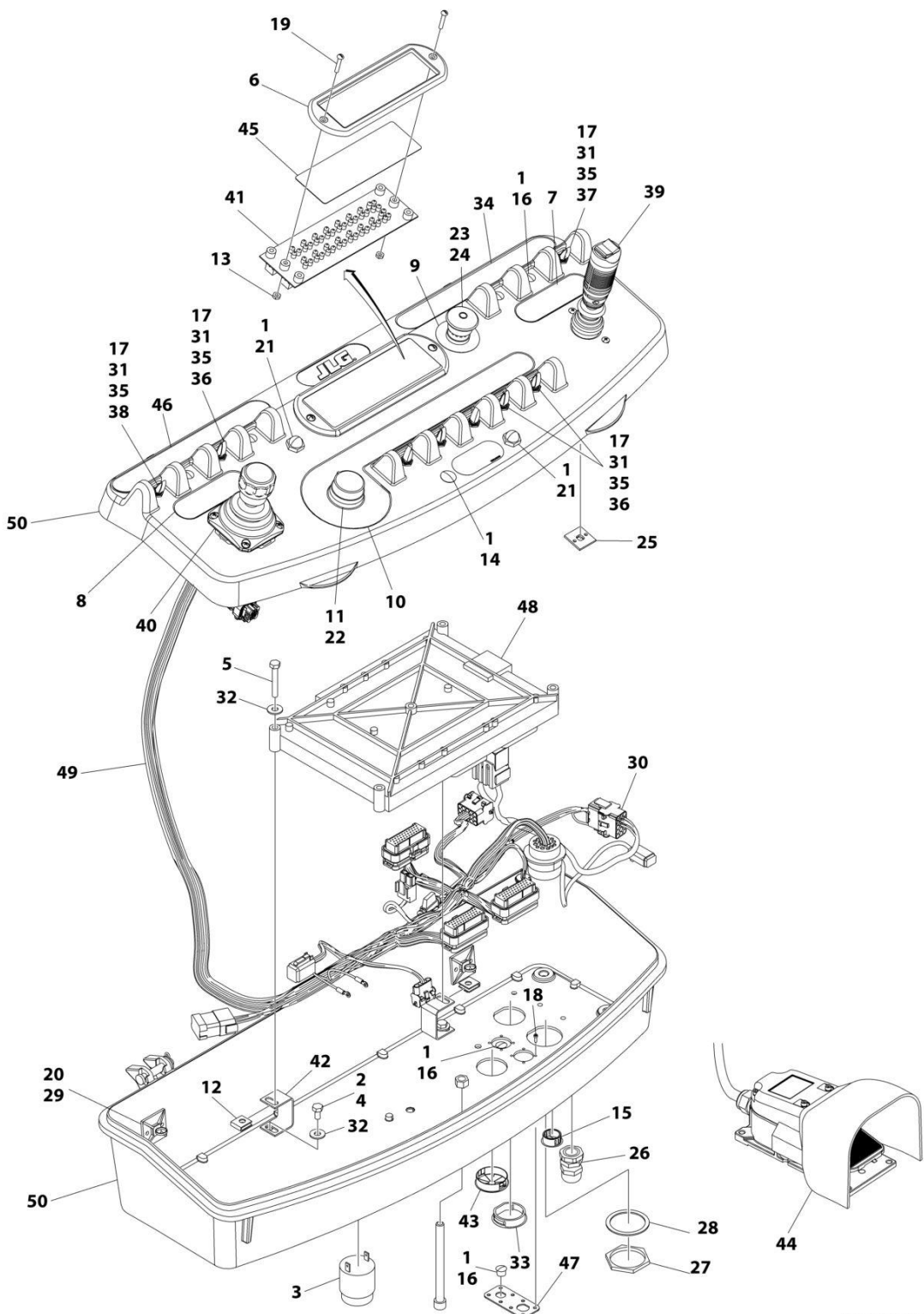
FIGURE 4-27. PLATFORM CONSOLE ASSEMBLY - E300AJP (UL SPECS) (SN 0300256384 through 0300272206)
