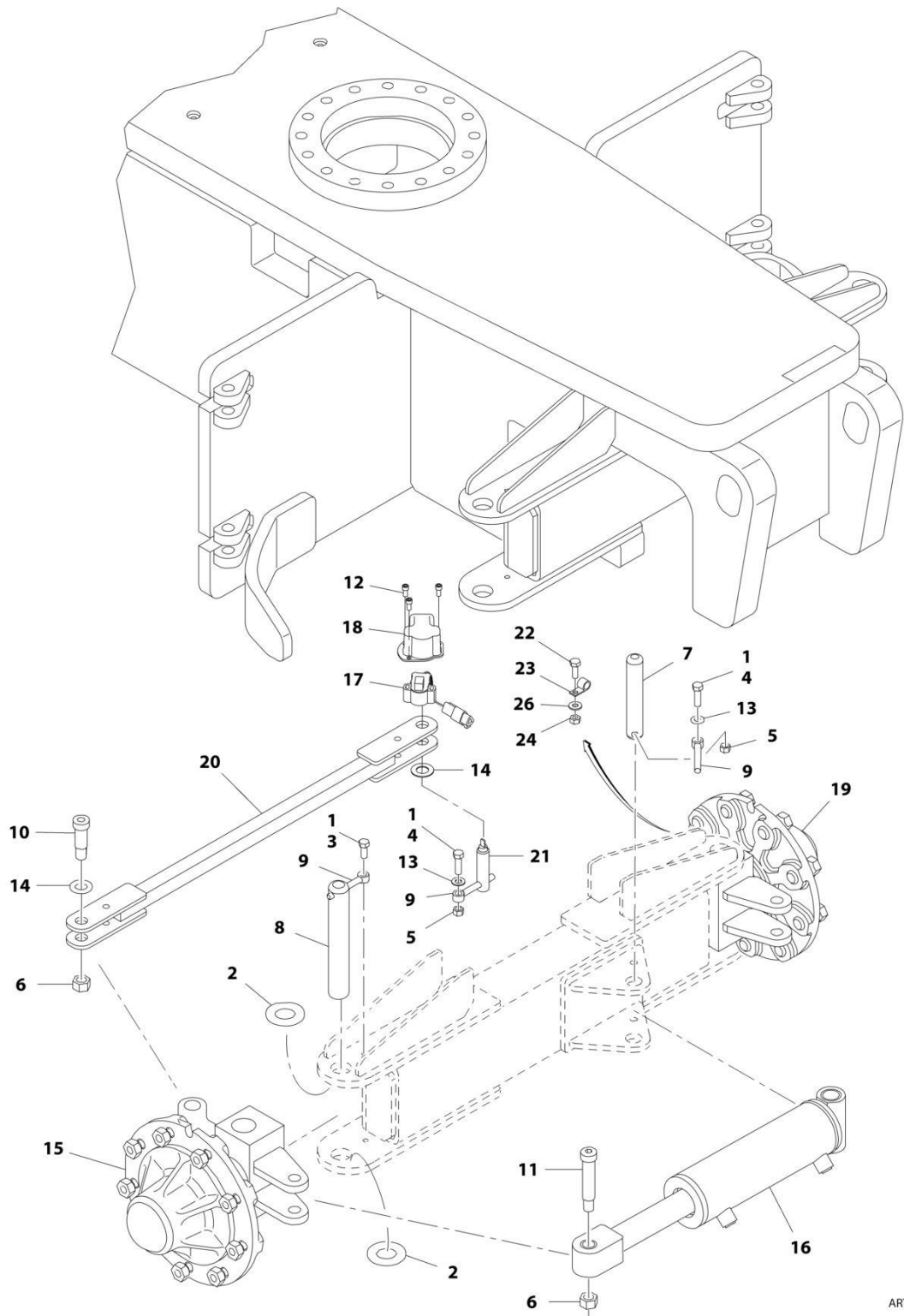
FIGURE 1-1. STEER INSTALLATION
