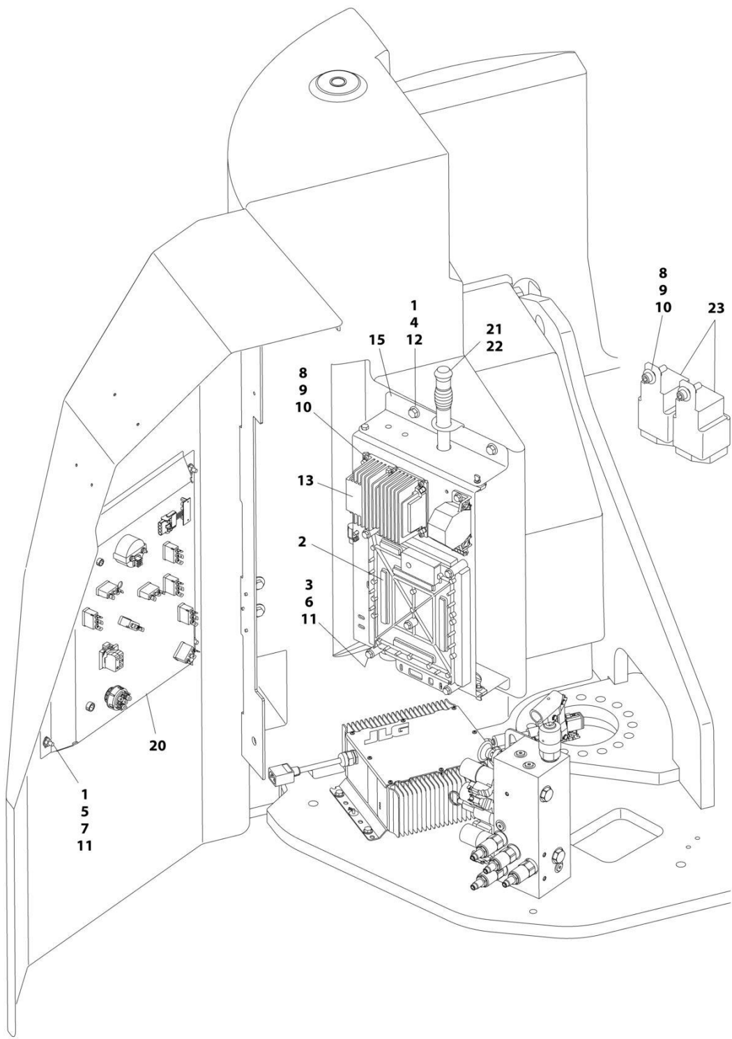
FIGURE 2-12. ELECTRICAL COMPONENTS INSTALLATION - E300AJ ALL SPECS EXCEPT CE AND UL SPECS
