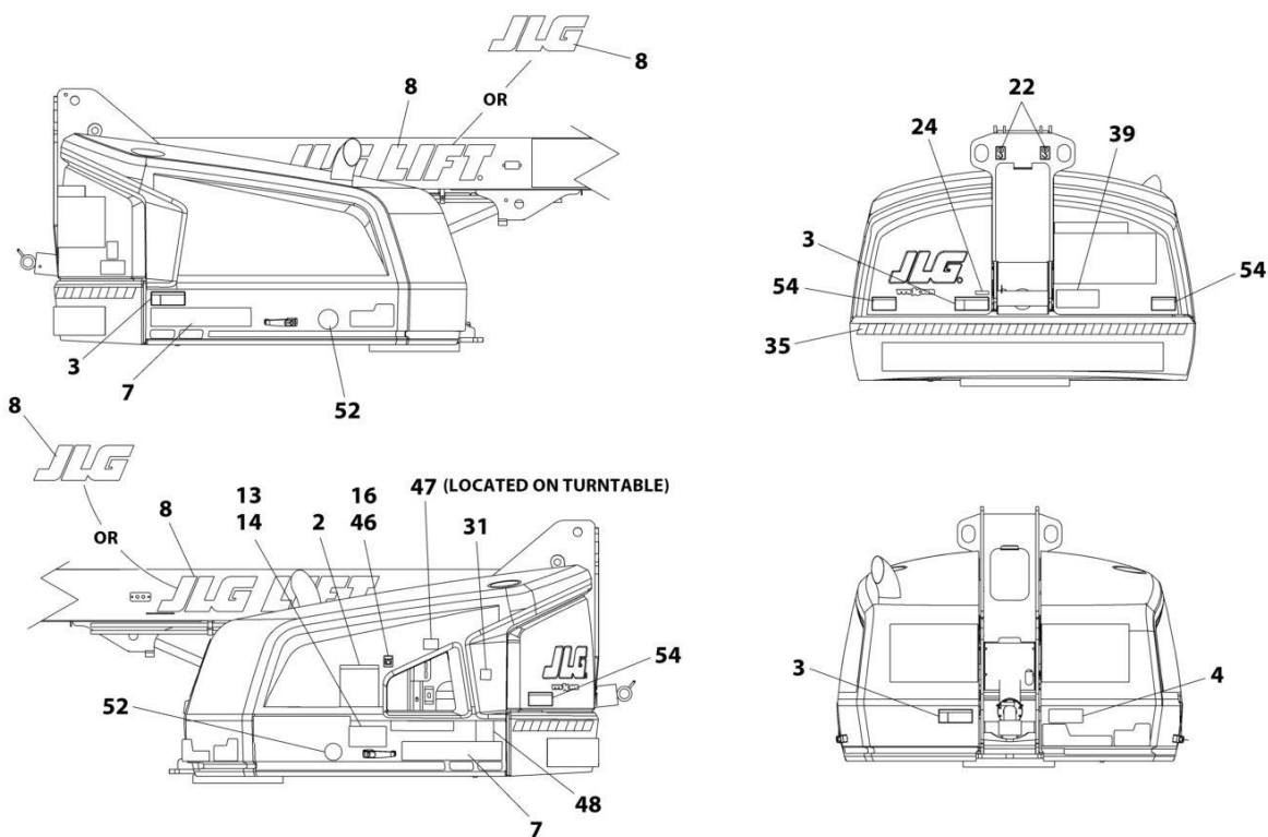
FIGURE 9-3. DECAL INSTALLATION - CE & UK CA SPEC - 400SC
