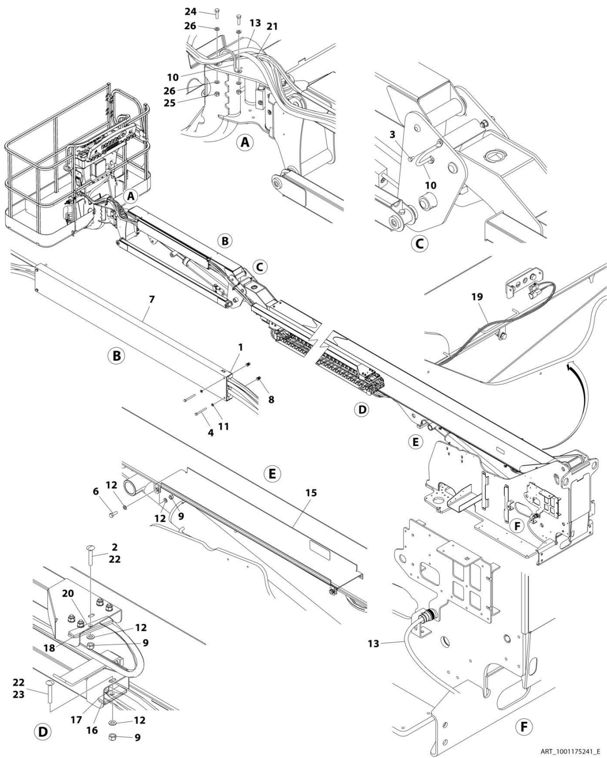
FIGURE 8-33. CABLES AND CLAMPS INSTALLATION - 460SJC WITH 4000W GENERATOR 60HZ
