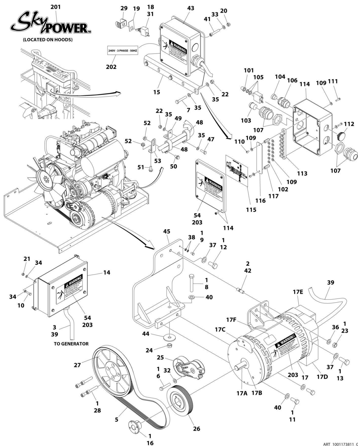
FIGURE 3-44. GENERATOR INSTALLATION - 7500W/50HZ (DEUTZ D2011 ENGINE) (ANSI EXPORT SPECS)
