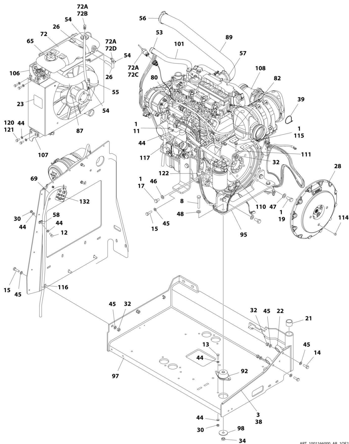
FIGURE 3-10. ENGINE ASSEMBLY - DEUTZ D2.9L4 EMR4 ENGINE (WITHOUT ARCTIC PACKAGE) (ANSI, ANSI EXPORT AND CSA SPECS)
