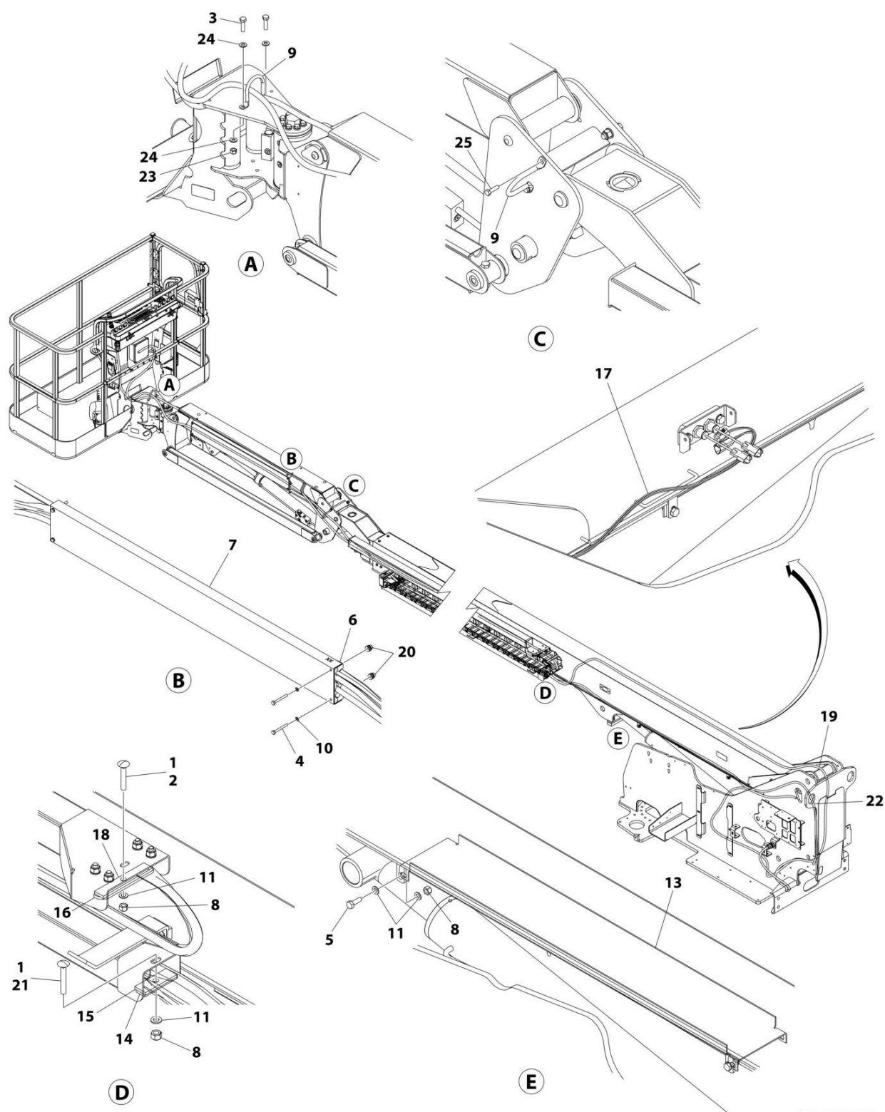
FIGURE 8-34. CABLES AND CLAMPS INSTALLATION - 460SJC WITH 7500W GENERATOR
