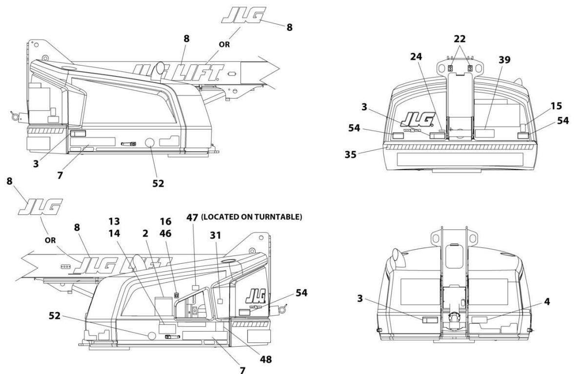
FIGURE 9-10. DECAL INSTALLATION - ANSI EXPORT SPEC - 460SJC (KOREAN SPECS)
