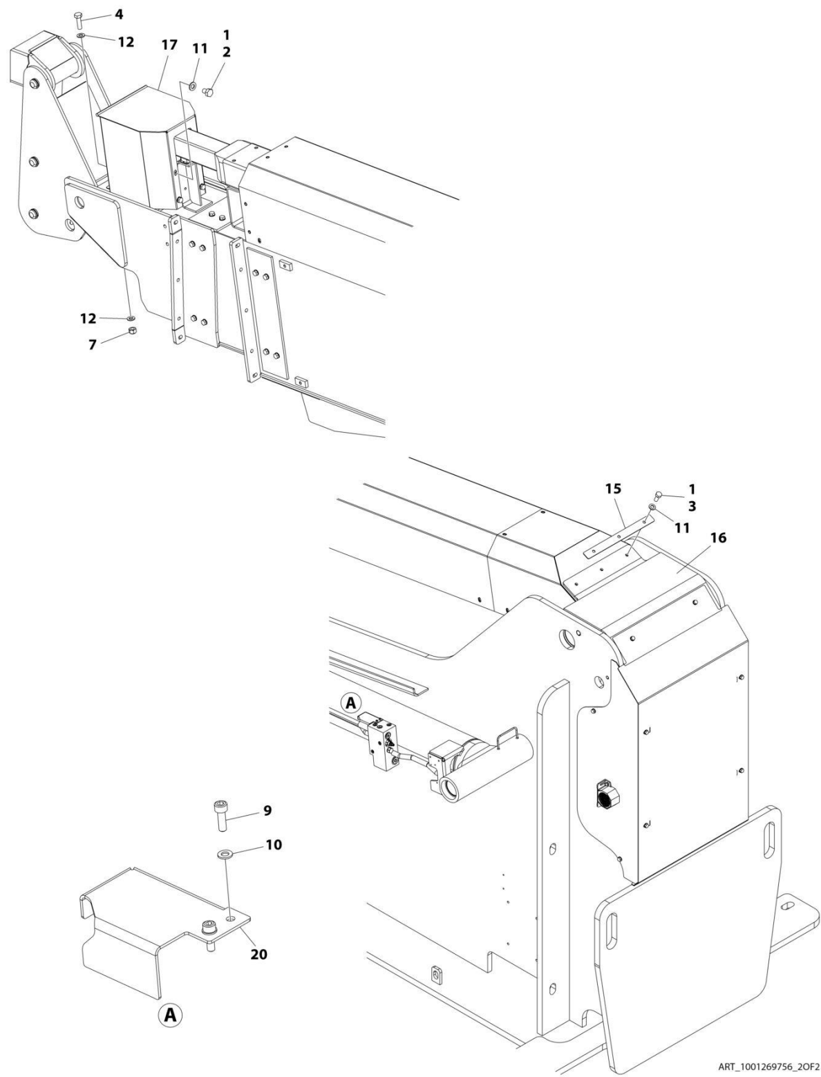
FIGURE 4-14. BOOM SHIELDS INSTALLATION
