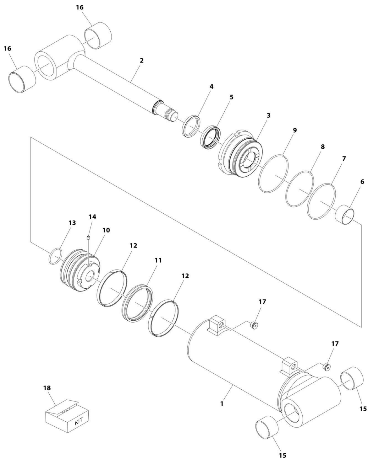
FIGURE 6-6. STEER CYLINDER ASSEMBLY
