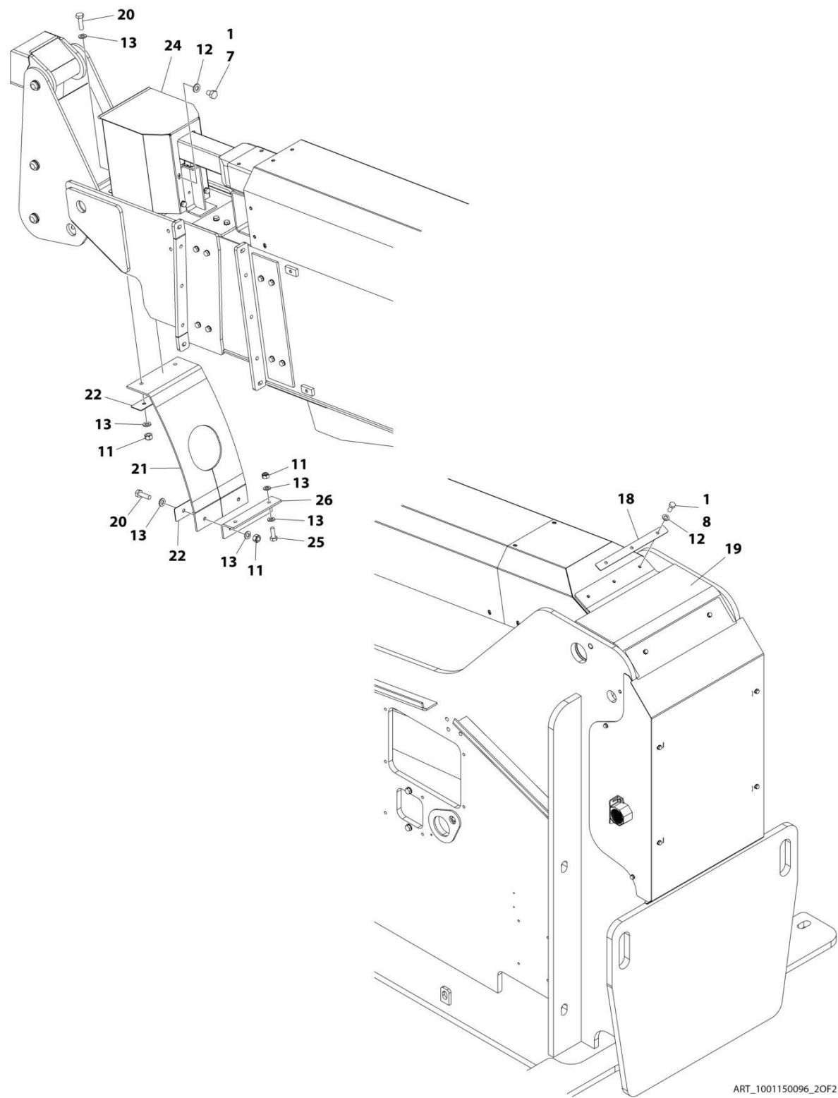
FIGURE 4-15. BOOM SHIELDS INSTALLATION - SHIPYARD MACHINES
