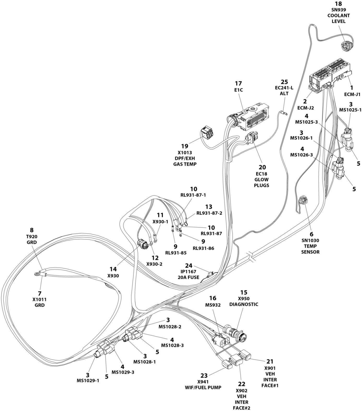
FIGURE 8-27. ENGINE HARNESS - DEUTZ TD2.9L4 ENGINES (CHINA IV SPECS)
