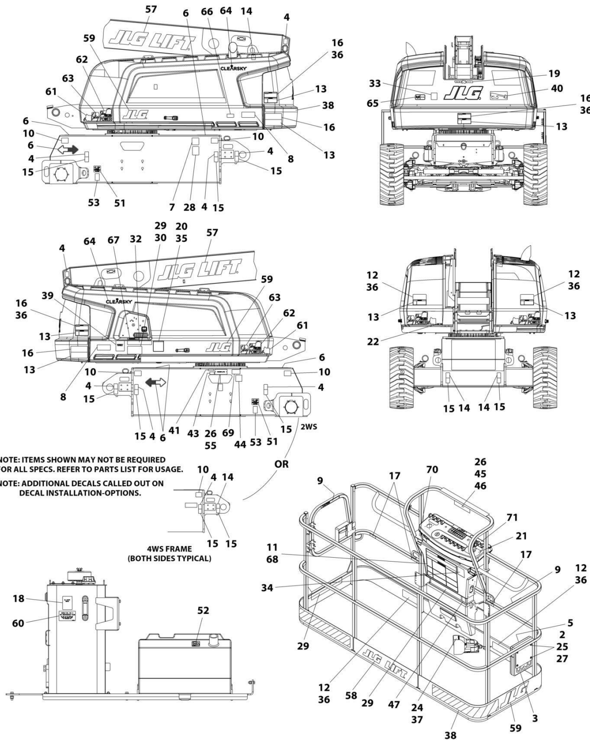
FIGURE 9-5. DECAL INSTALLATION (CHINESE SPECS - ENGLISH/TRADITIONAL CHINESE LANGUAGES) (600S)
