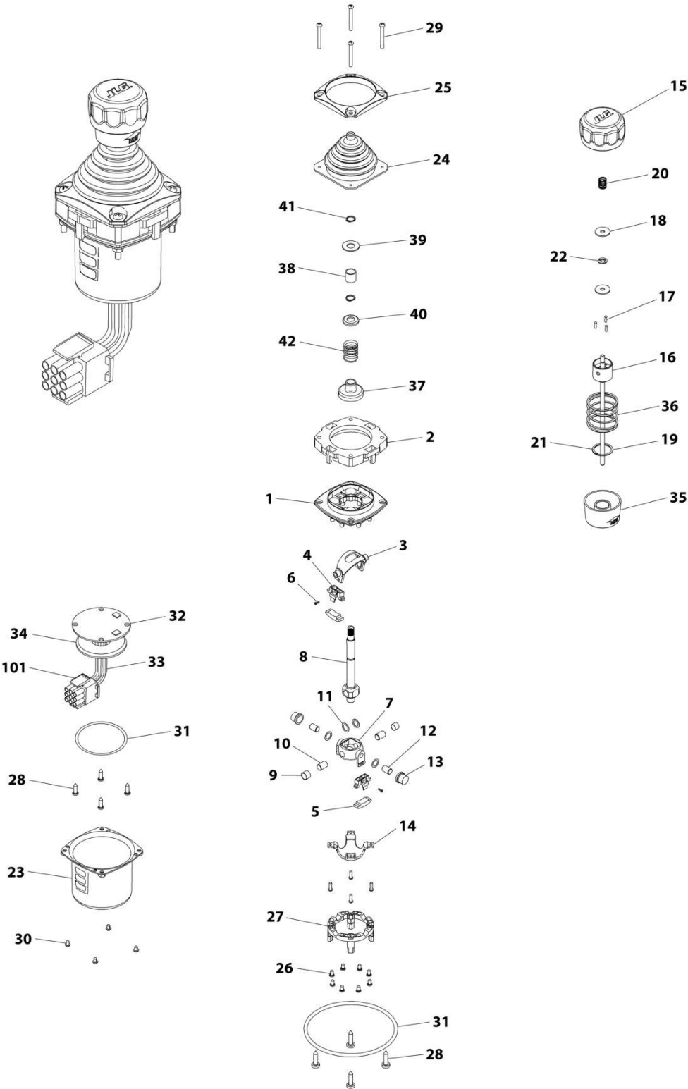
FIGURE 5-25. CONTROLLER ASSEMBLY (LIFT AND SWING)
