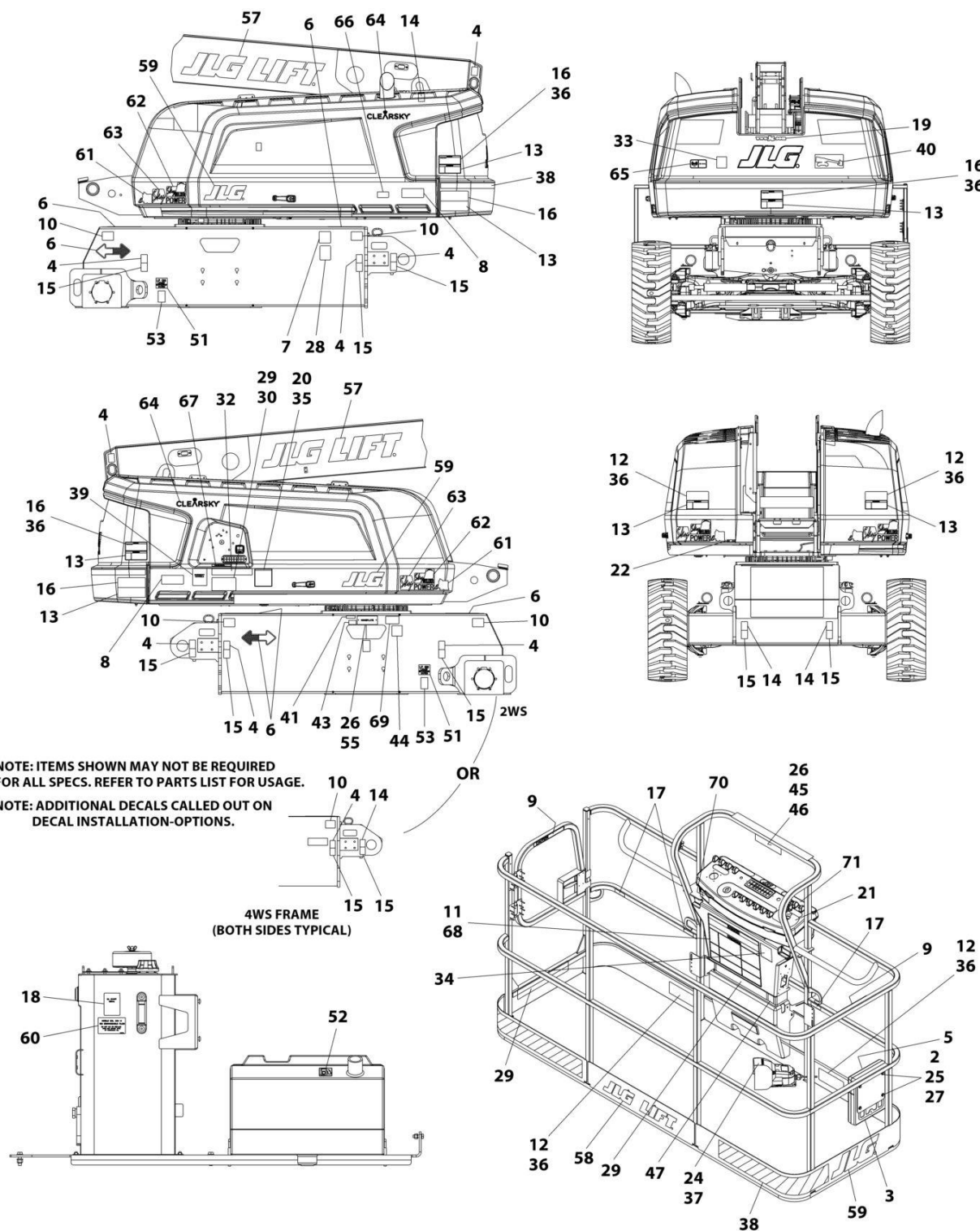
FIGURE 9-11. DECAL INSTALLATION (AUSTRALIAN SPECS - ENGLISH LANGUAGE) (660SJ)
