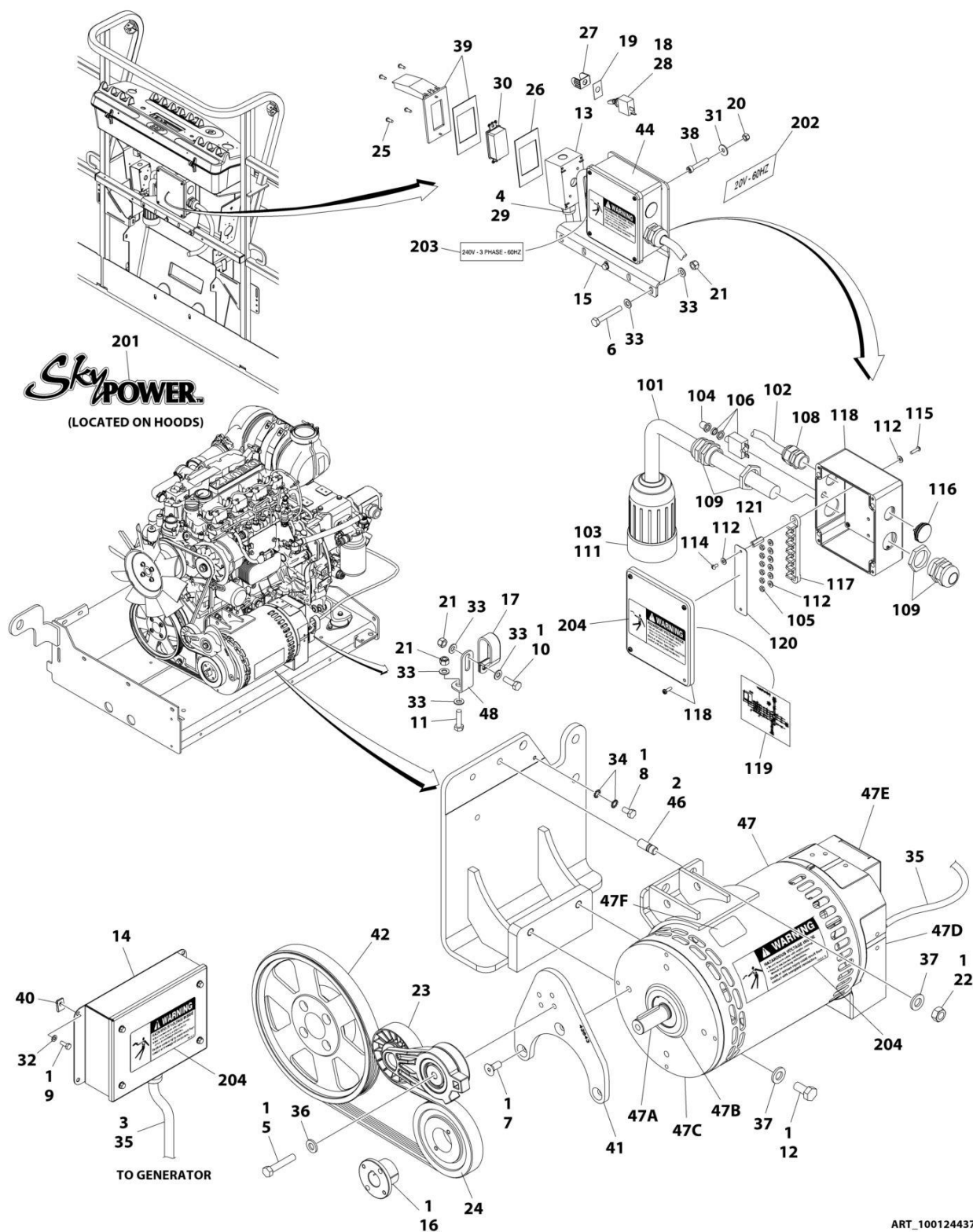
FIGURE 3-73. 7500W SKYPOWER GENERATOR INSTALLATION - 110V/60HZ (DEUTZ D2.9L4 - 49HP ENGINES) (OPTIONAL)
