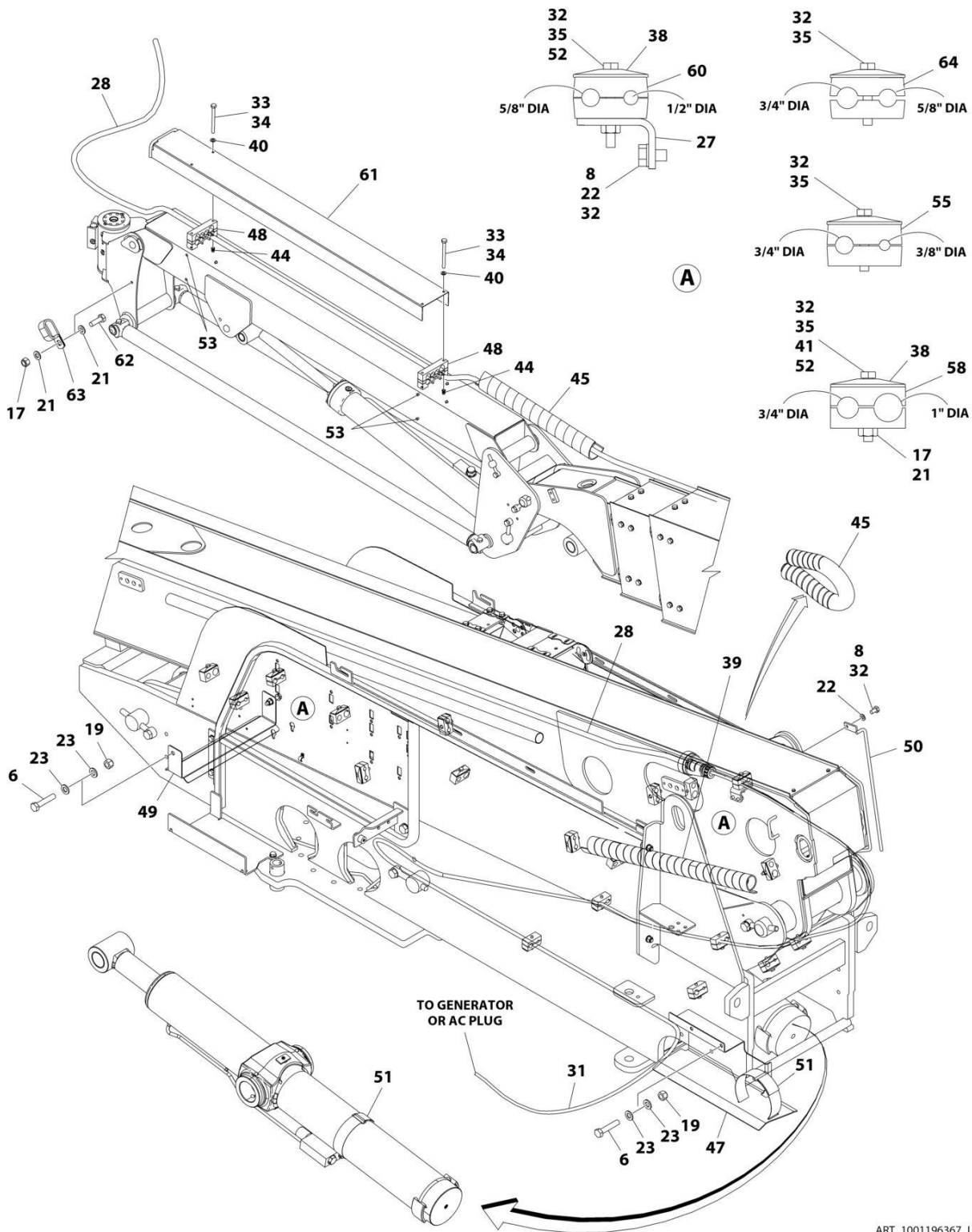
FIGURE 8-28. AC CABLES AND CLAMPS INSTALLATION - WITH 4000W/50HZ GENERATOR (ANSI EXPORT, AUSTRALIAN, CE & UK CA SPECS) (660SJ)
