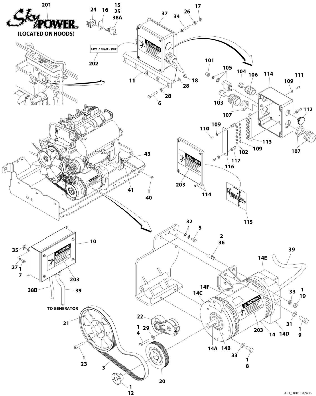
FIGURE 3-76. 7500W SKYPOWER GENERATOR INSTALLATION - 220V/50HZ (DEUTZ D2011 ENGINES) (OPTIONAL)
