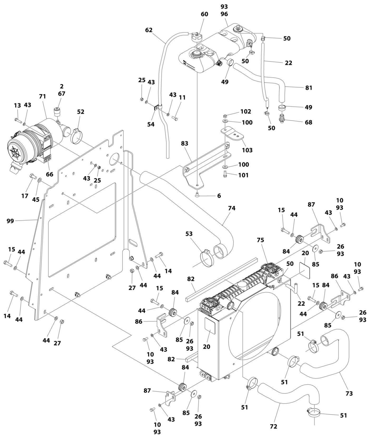
FIGURE 3-21. DEUTZ D2.9L4 - 49HP ENGINE ASSEMBLY - WITH ARCTIC PACKAGE
