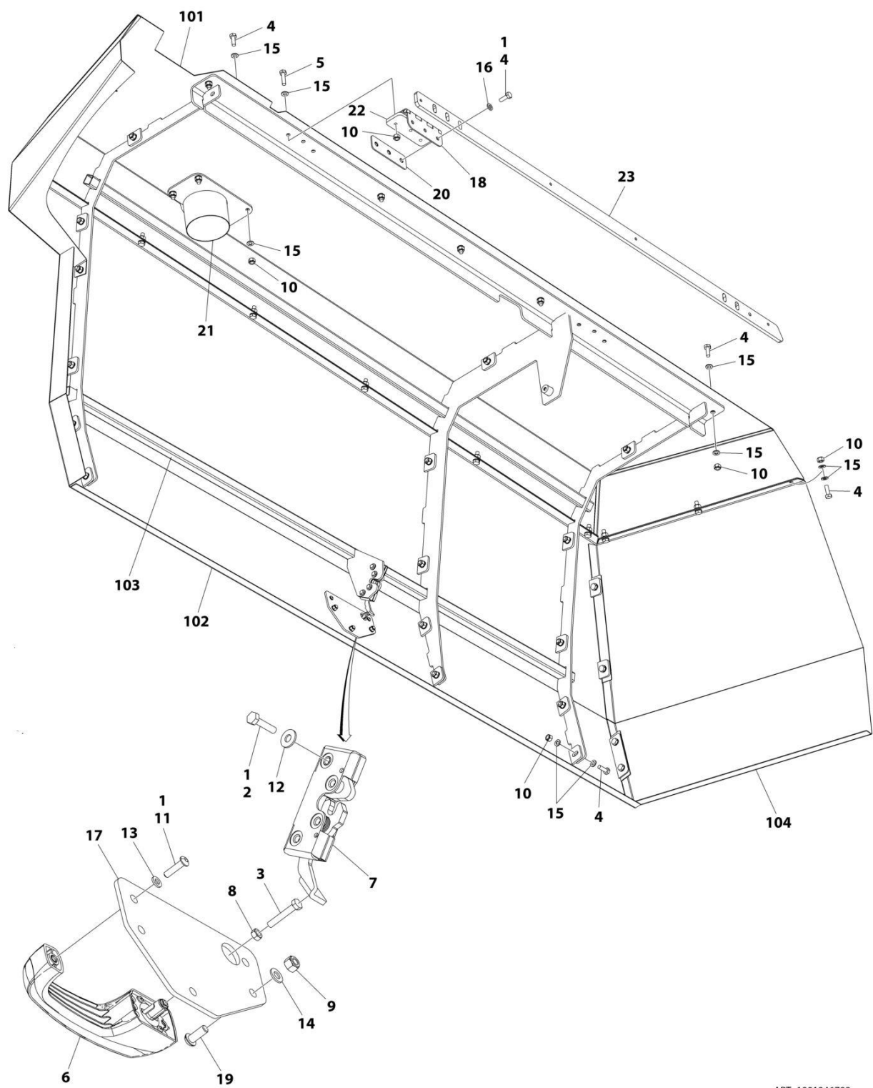
FIGURE 2-57. HOOD ASSEMBLY - ENGINE SIDE (STEEL) (MACHINES WITH SN STARTING WITH B3)
