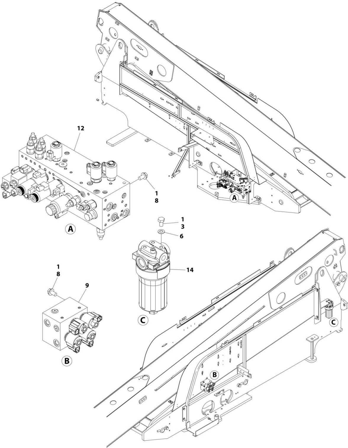
FIGURE 2-2. VALVE INSTALLATION - WITH 4WS (600S)
