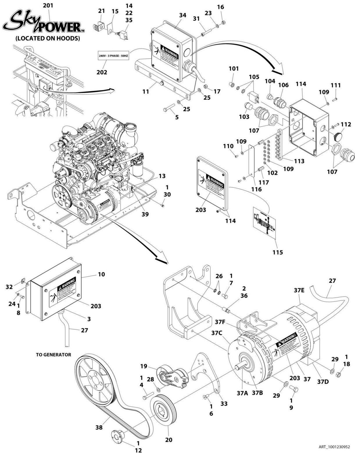
FIGURE 3-78. 7500W SKYPOWER GENERATOR INSTALLATION - 220V/50HZ (DEUTZ TD2.9L4 - 67HP ENGINES) (OPTIONAL)
