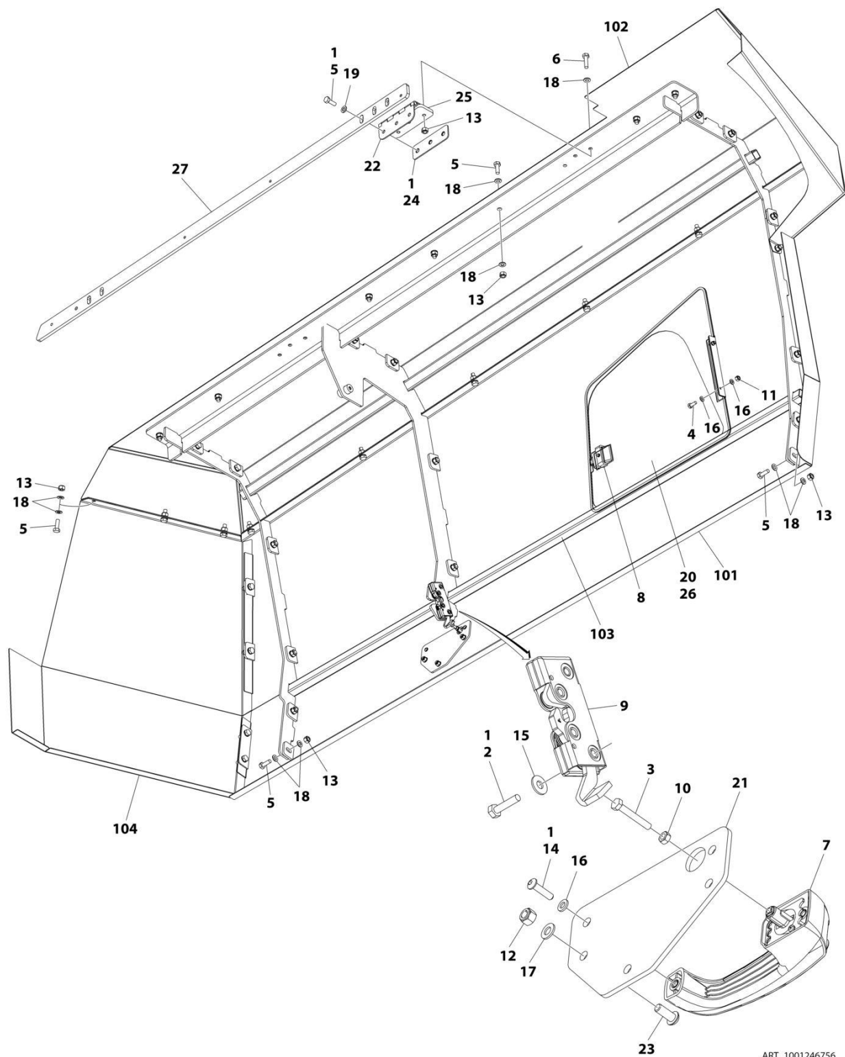
FIGURE 2-59. HOOD ASSEMBLY - TANK SIDE (STEEL) (MACHINES WITH SN STARTING WITH B3)
