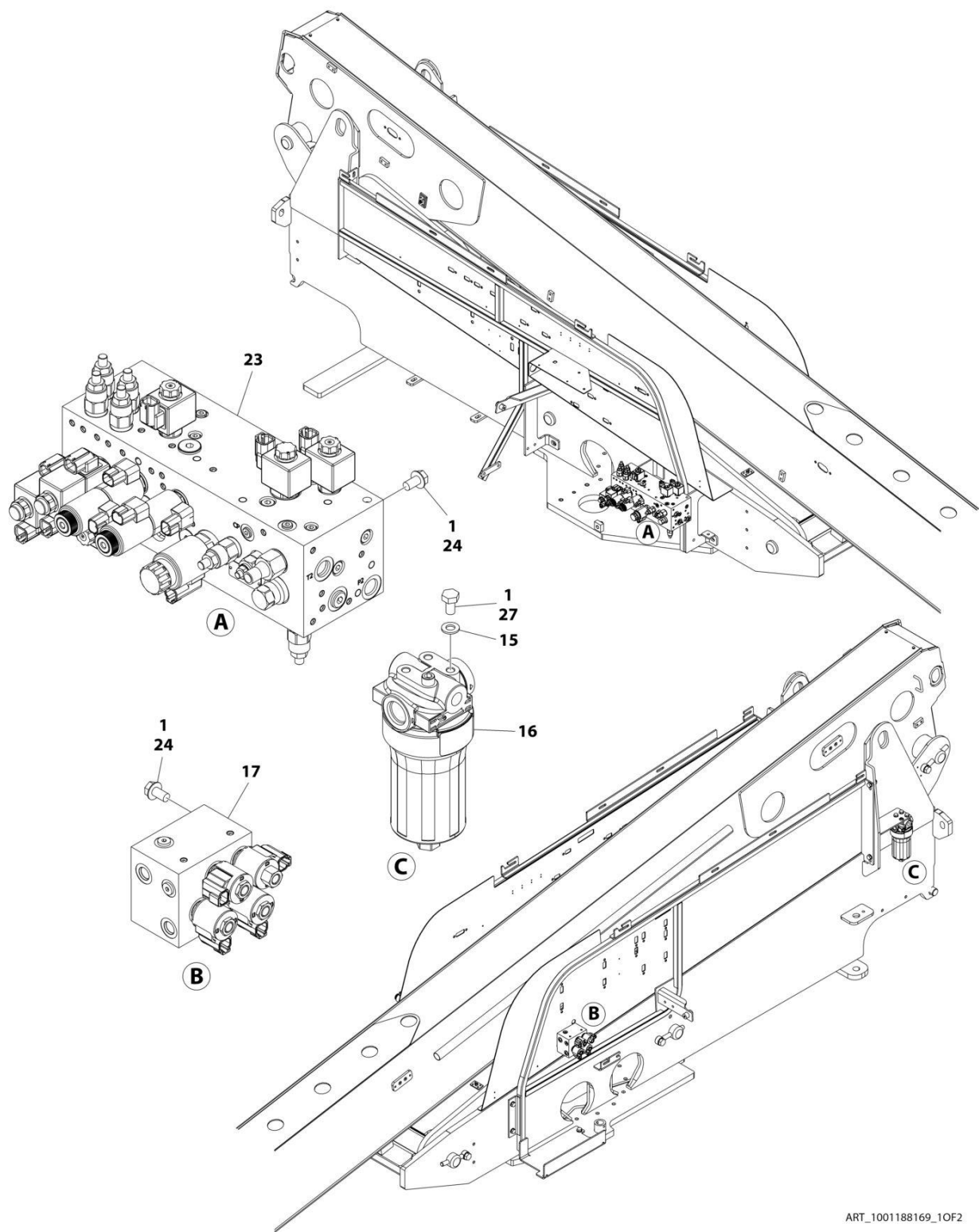
FIGURE 2-4. VALVE INSTALLATION - WITH 4WS (660SJ)
