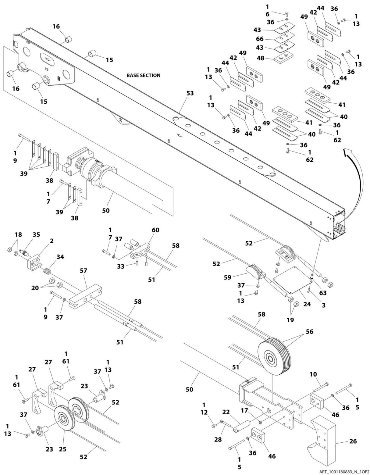
FIGURE 4-5. BOOM ASSEMBLY (600S)
