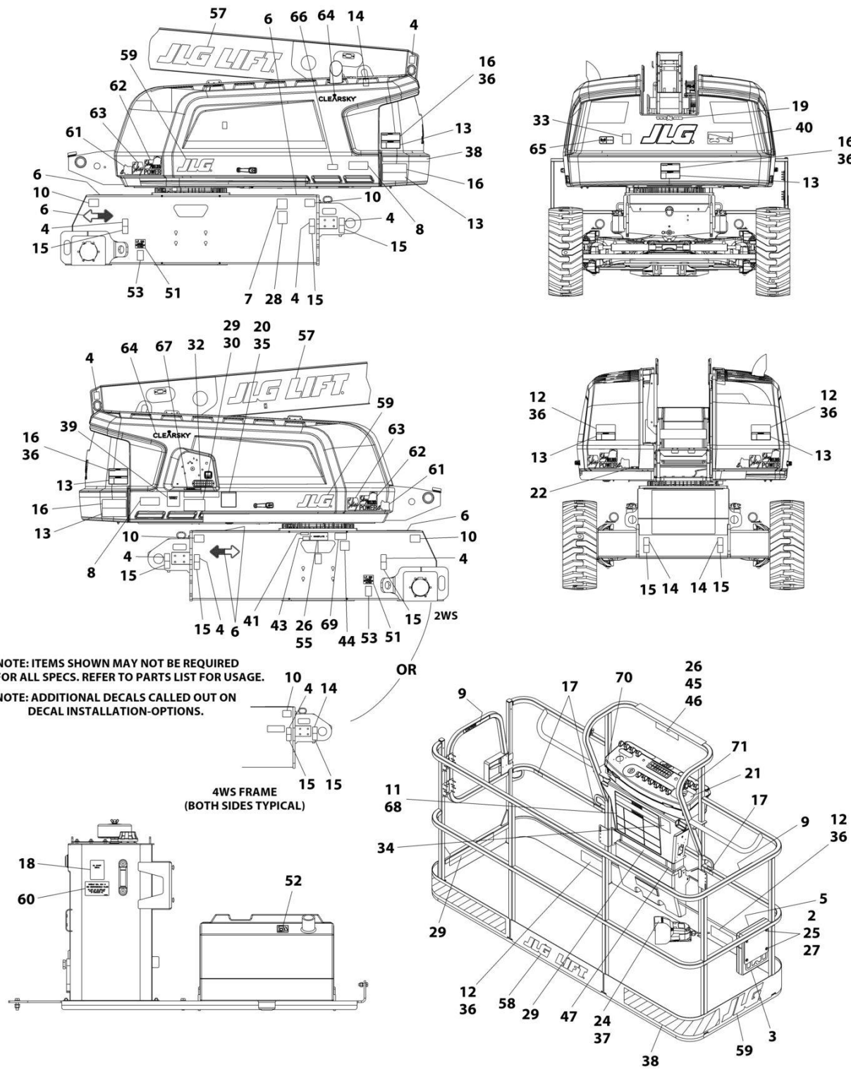
FIGURE 9-19. DECAL INSTALLATION (LATIN AMERICAN SPECS - ENGLISH/SPANISH LANGUAGES) (660SJ)
