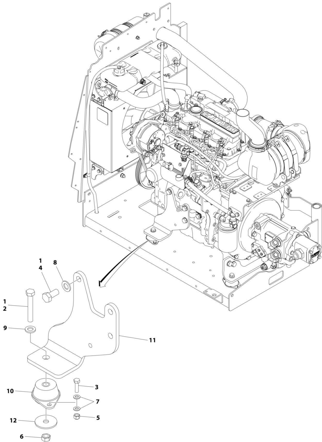
FIGURE 3-48. MOTOR MOUNT INSTALLATION - WITHOUT GENERATOR (DEUTZ TD2.9L4 - 49HP ENGINES)
