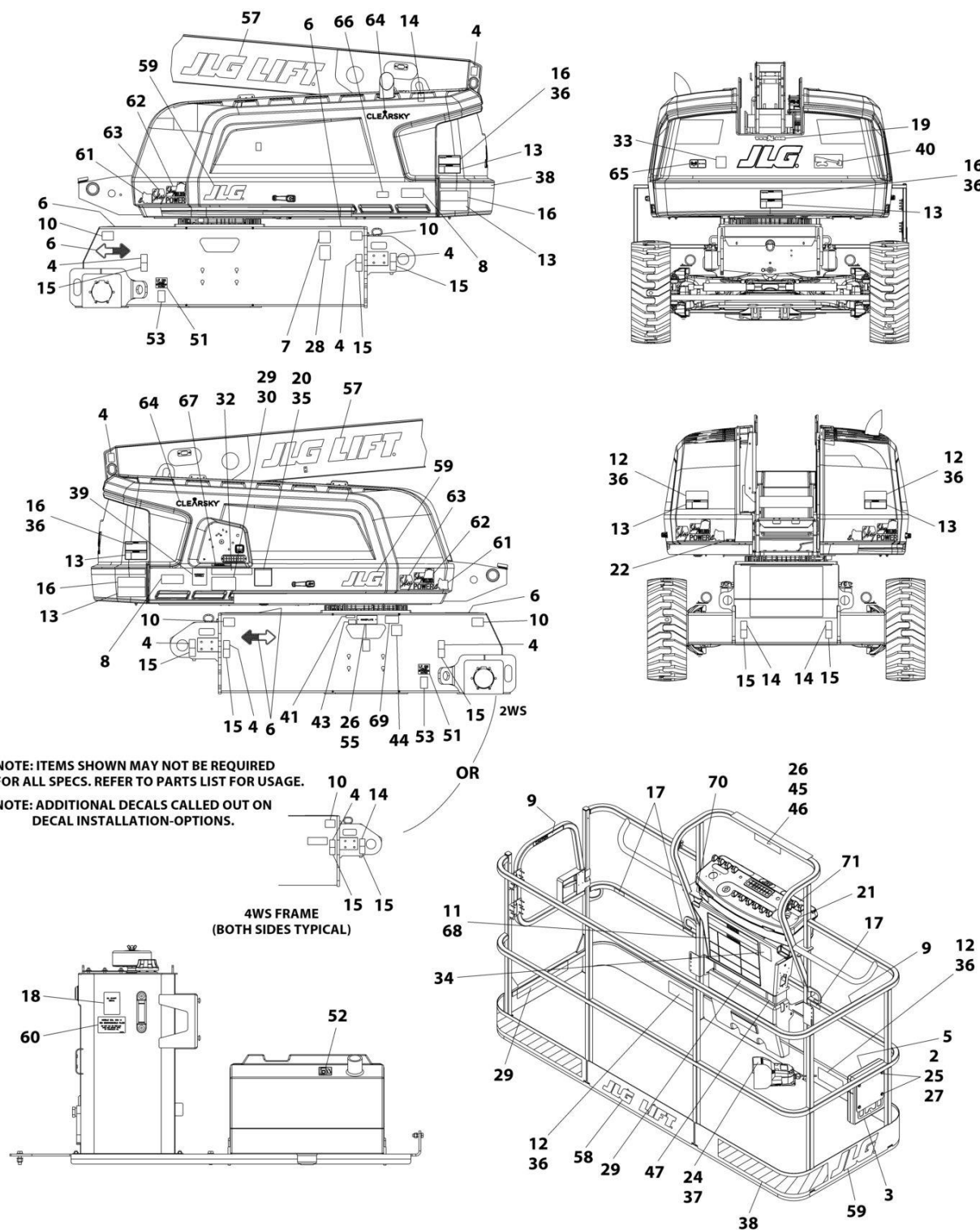
FIGURE 9-6. DECAL INSTALLATION (CSA SPECS - ENGLISH/FRENCH LANGUAGES) (600S)
