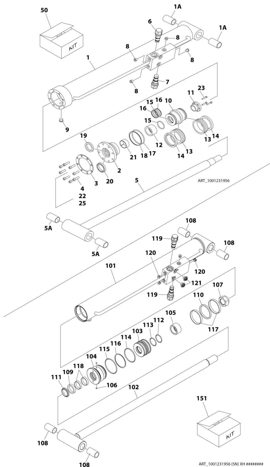
FIGURE 6-6. LIFT CYLINDER ASSEMBLY - JIB (MACHINES WITH SN STARTING WITH B3) (660SJ)
