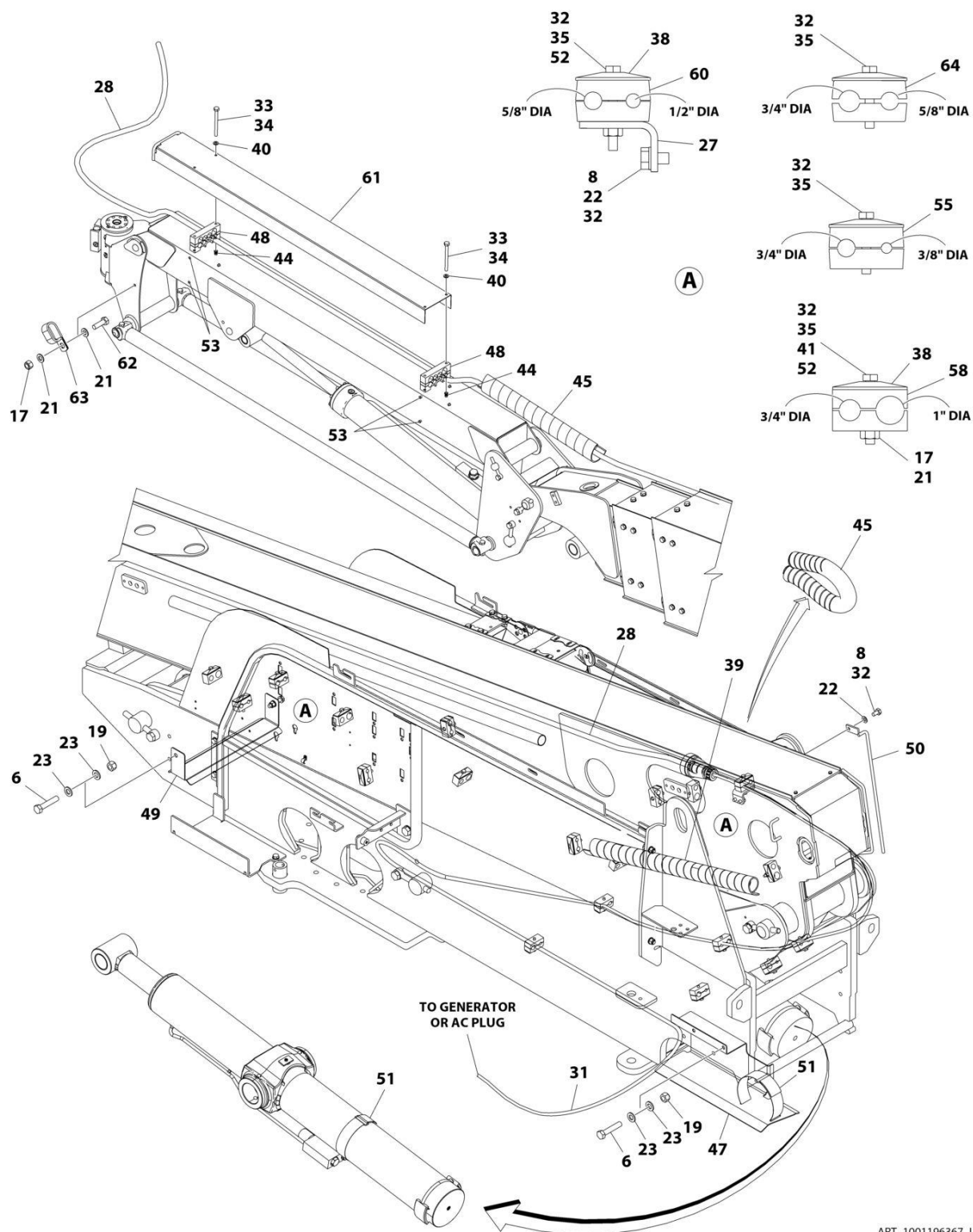
FIGURE 8-27. AC CABLES AND CLAMPS INSTALLATION - WITH 2500W GENERATOR (ALL SPECS EXCEPT CE & UK CA SPECS) (660SJ)
