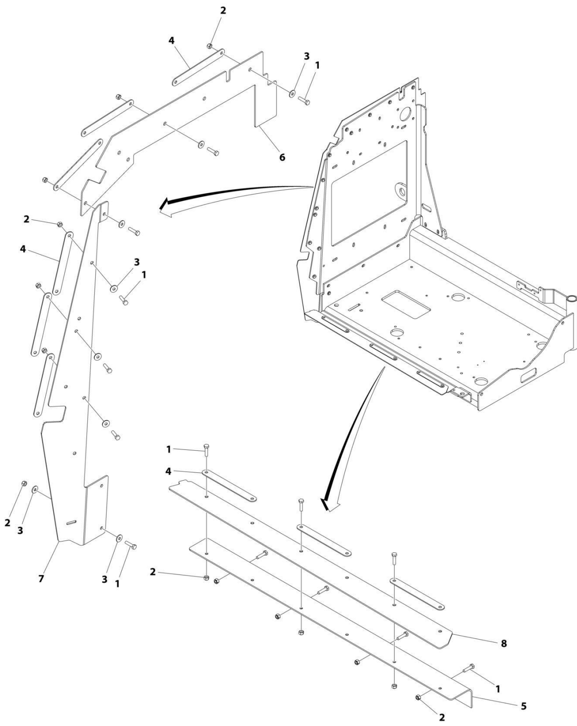
FIGURE 3-60. ENGINE HOOD Baffles INSTALLATION - STEEL HOODS (DEUTZ D2.9L4 - 49HP ENGINES)
