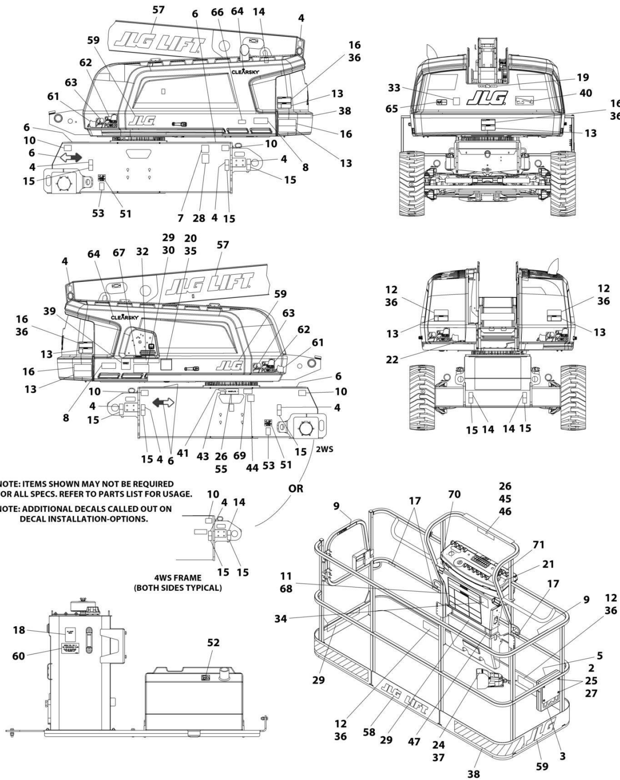
FIGURE 9-7. DECAL INSTALLATION (JAPANESE SPECS - ENGLISH/JAPANESE LANGUAGES) (600S)
