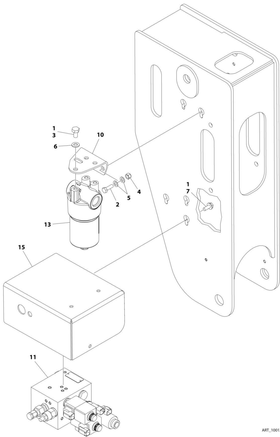
FIGURE 4-13. BOOM VALVES INSTALLATION - WITH 4WS (600S)
