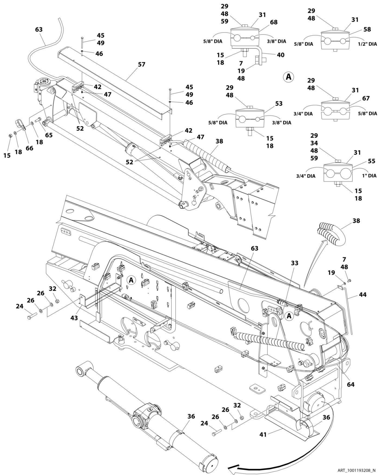
FIGURE 8-24. AC CABLES AND CLAMPS INSTALLATION - WITHOUT GENERATOR (ANSI, CSA AND JAPANESE SPECS) (660SJ)
