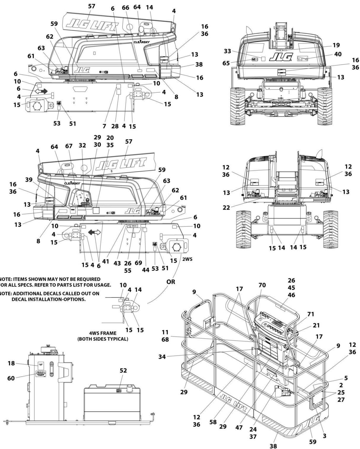
FIGURE 9-4. DECAL INSTALLATION (CHINESE SPECS - ENGLISH/SIMPLIFIED CHINESE LANGUAGES) (600S)
