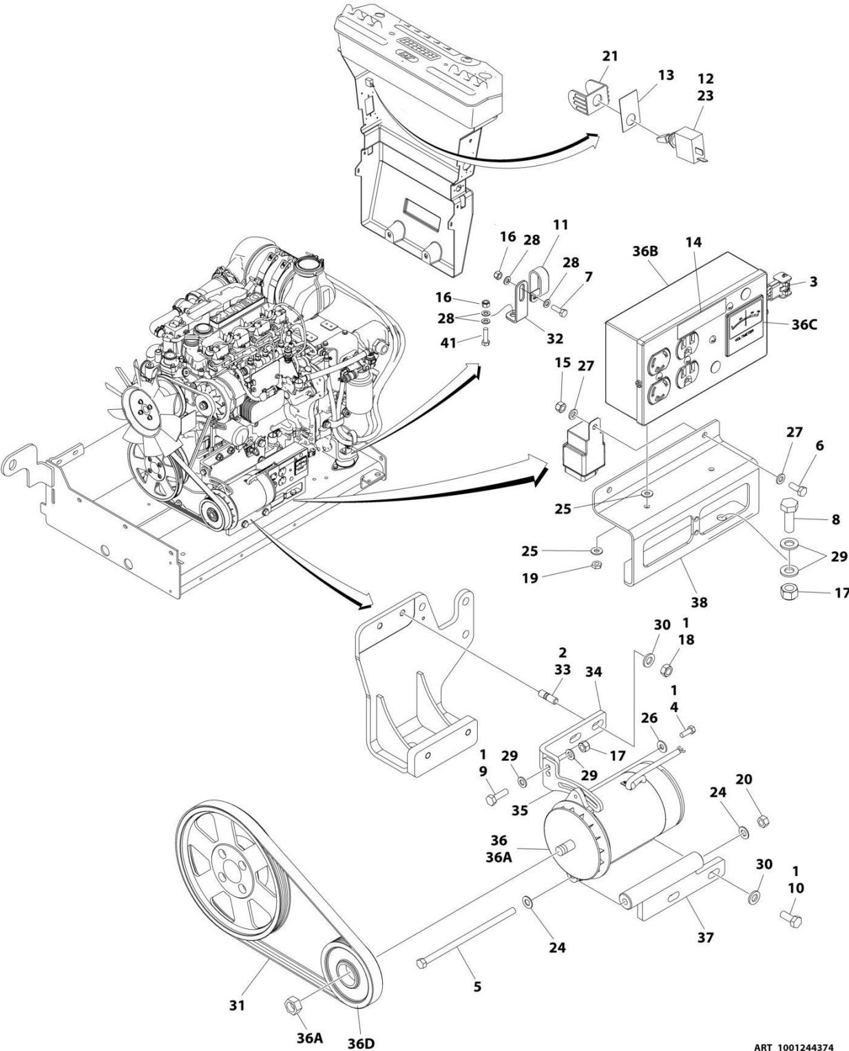
FIGURE 3-62. 2500W GENERATOR INSTALLATION - 110V/60HZ (DEUTZ D2.9L4 - 49HP ENGINES) (OPTIONAL)
