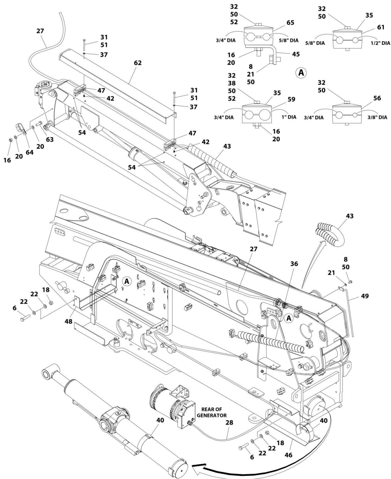
FIGURE 8-30. AC CABLES AND CLAMPS INSTALLATION - WITH 7500W SKYPOWER GENERATOR (660SJ)
