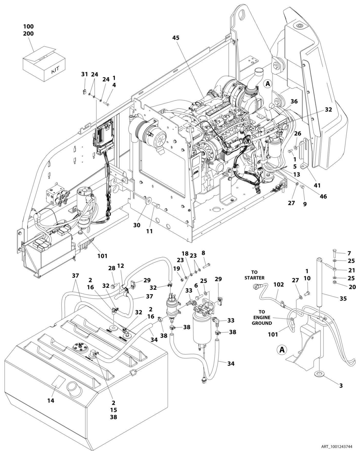
FIGURE 3-16. DEUTZ D2.9L4 - 49HP ENGINE INSTALLATION - WITHOUT ARCTIC PACKAGE
