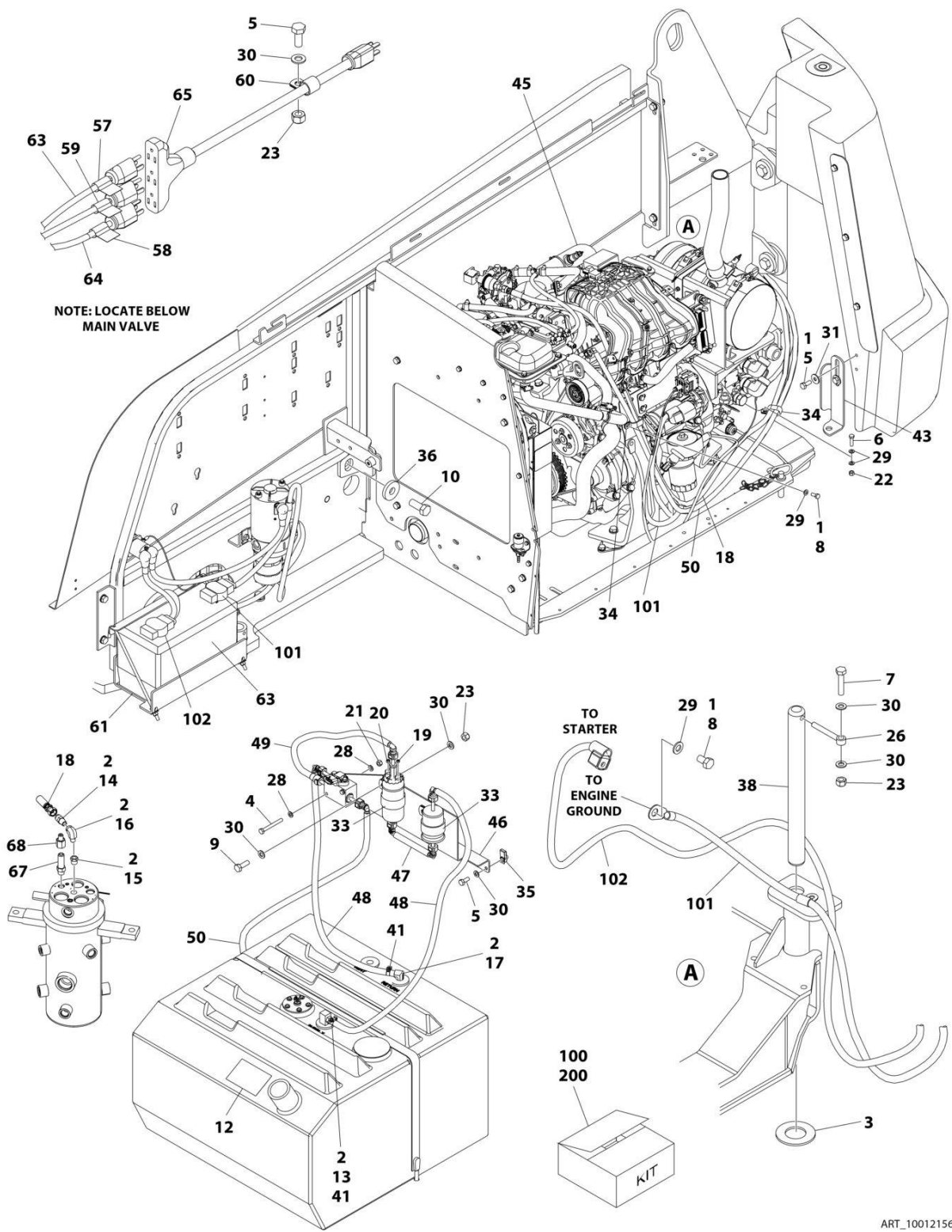
FIGURE 3-34. FORD ENGINE INSTALLATION - WITH ARCTIC PACKAGE
