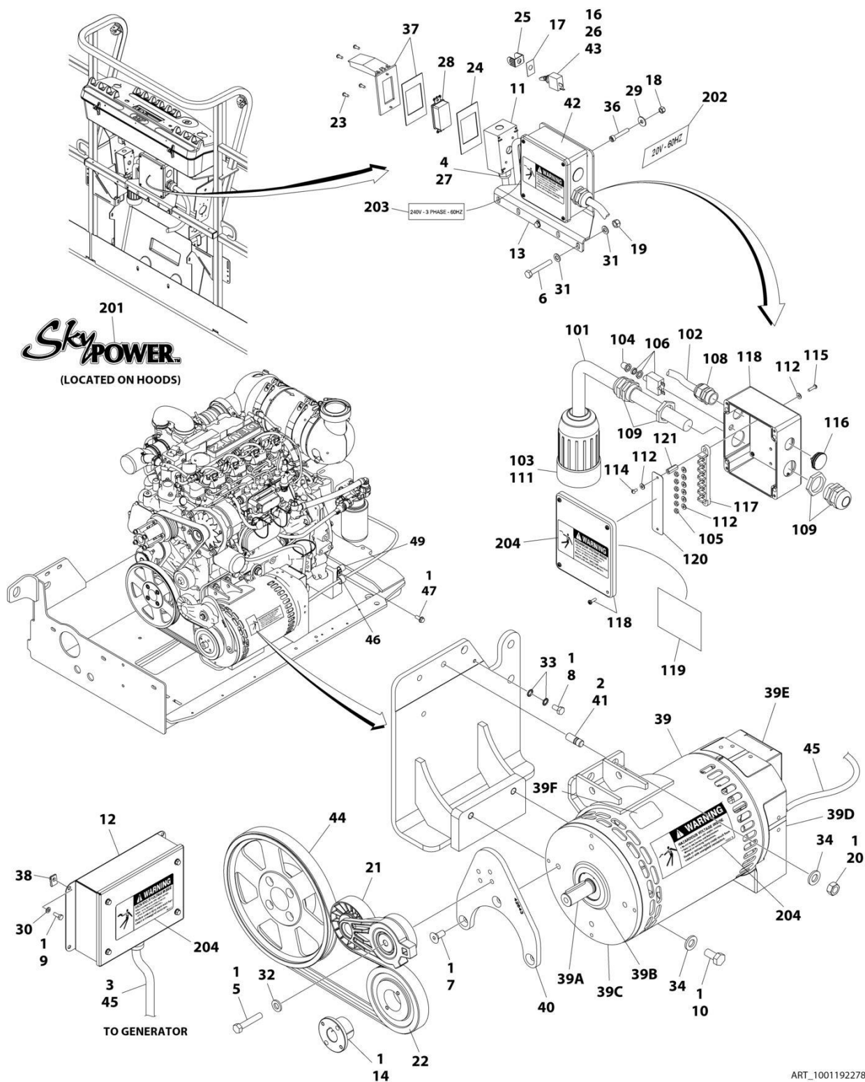
FIGURE 3-74. 7500W SKYPOWER GENERATOR INSTALLATION - 110V/60HZ (DEUTZ TD2.9L4 - 67HP ENGINES) (OPTIONAL)
