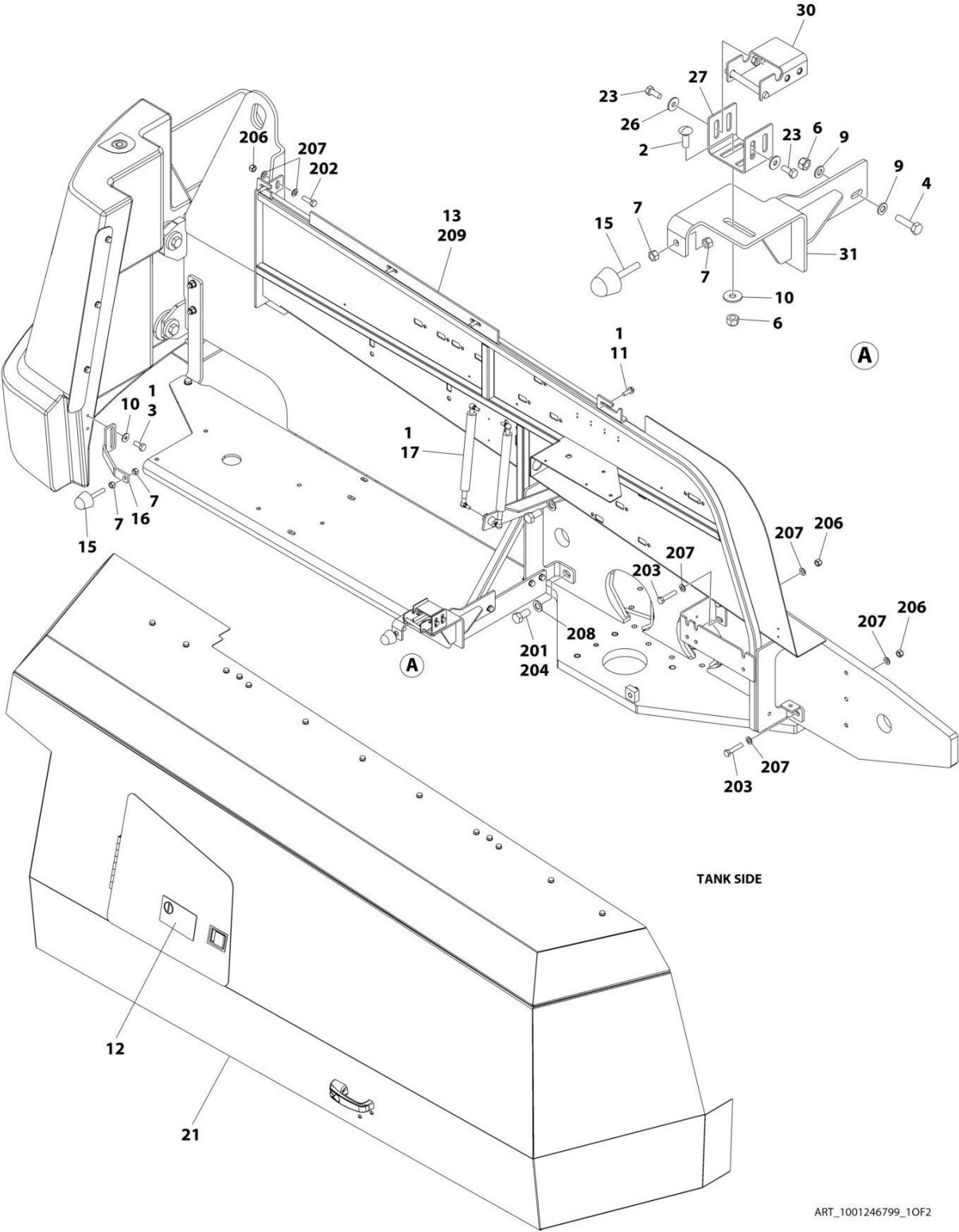
FIGURE 2-55. HOODS INSTALLATIONS - STEEL (MACHINES WITH SN STARTING WITH B3)
