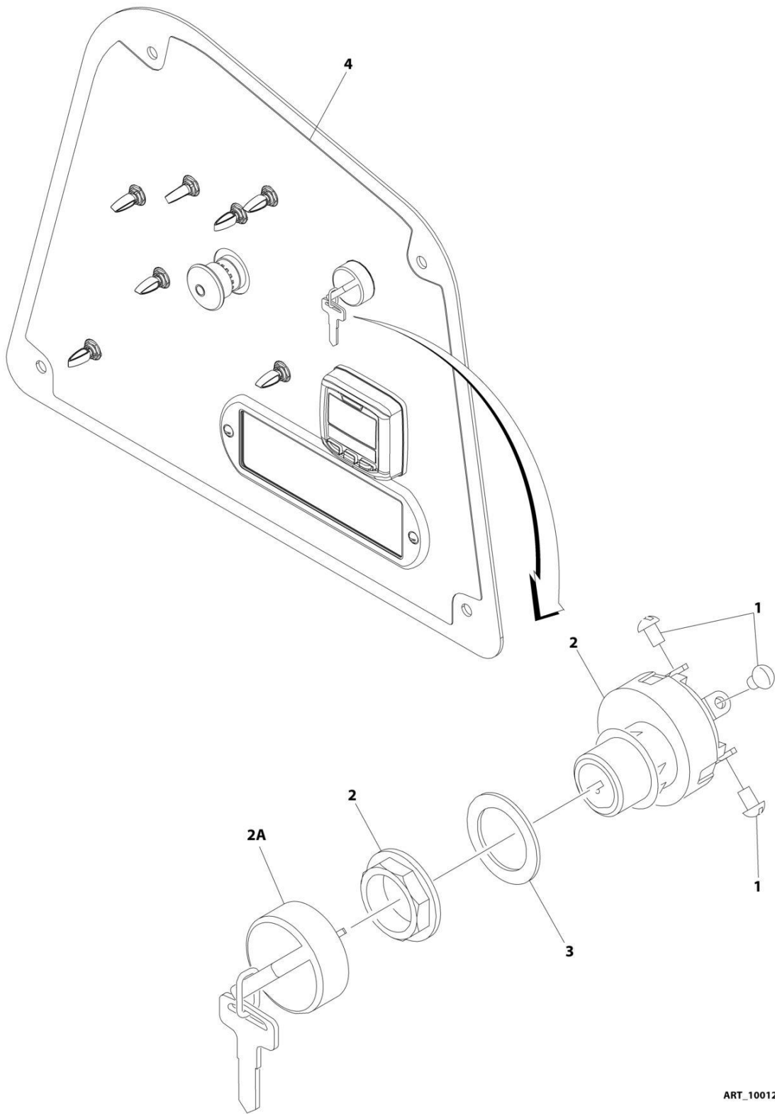
FIGURE 2-42. KEYSWITCH INSTALLATION (ALL SPECS EXCEPT CE & UK CA SPECS) (660SJ)
