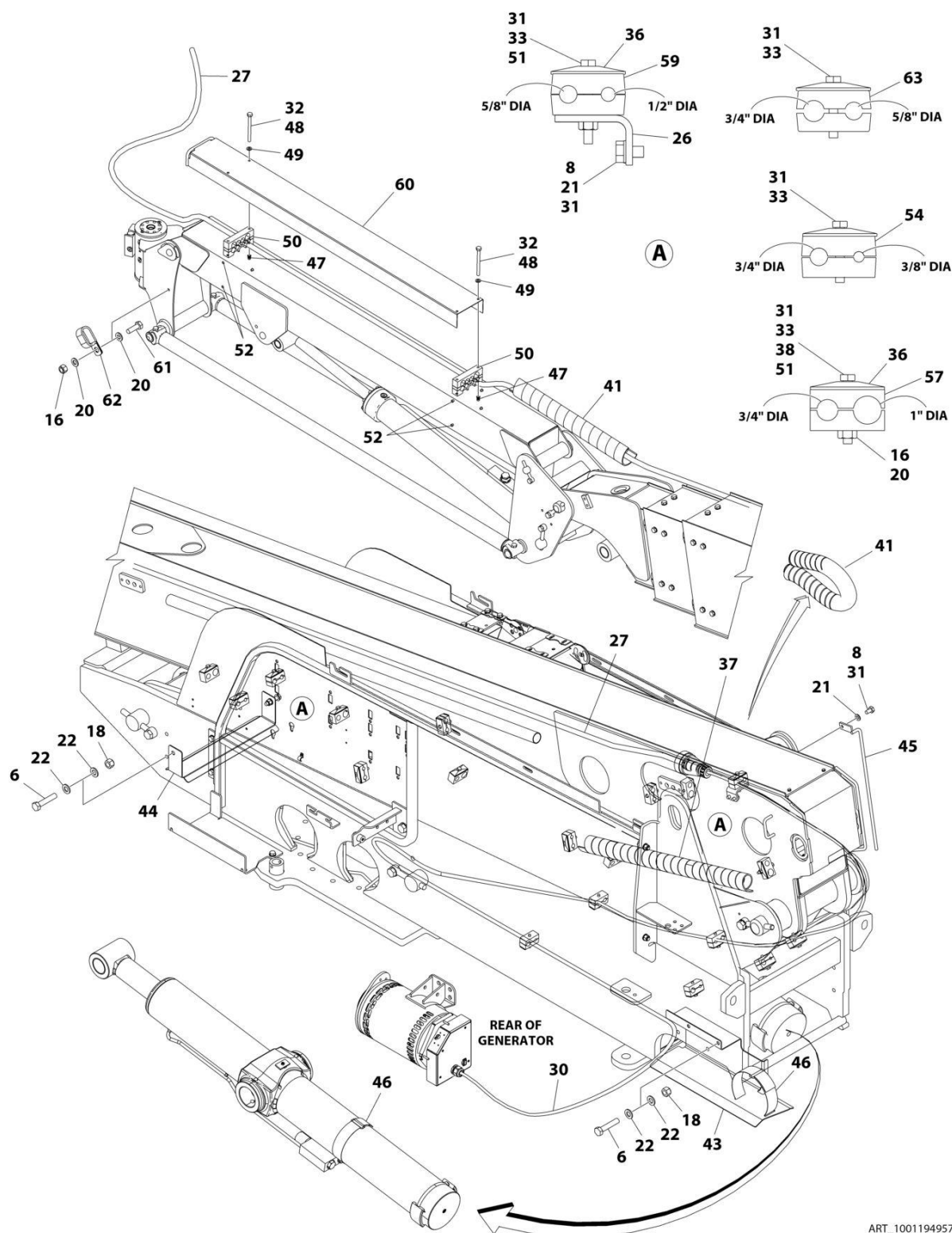
FIGURE 8-29. AC CABLES AND CLAMPS INSTALLATION - WITH 4000W/60HZ GENERATOR (ALL SPECS EXCEPT AUSTRALIAN, CHINA, CE & UK CA SPECS) (660SJ)
