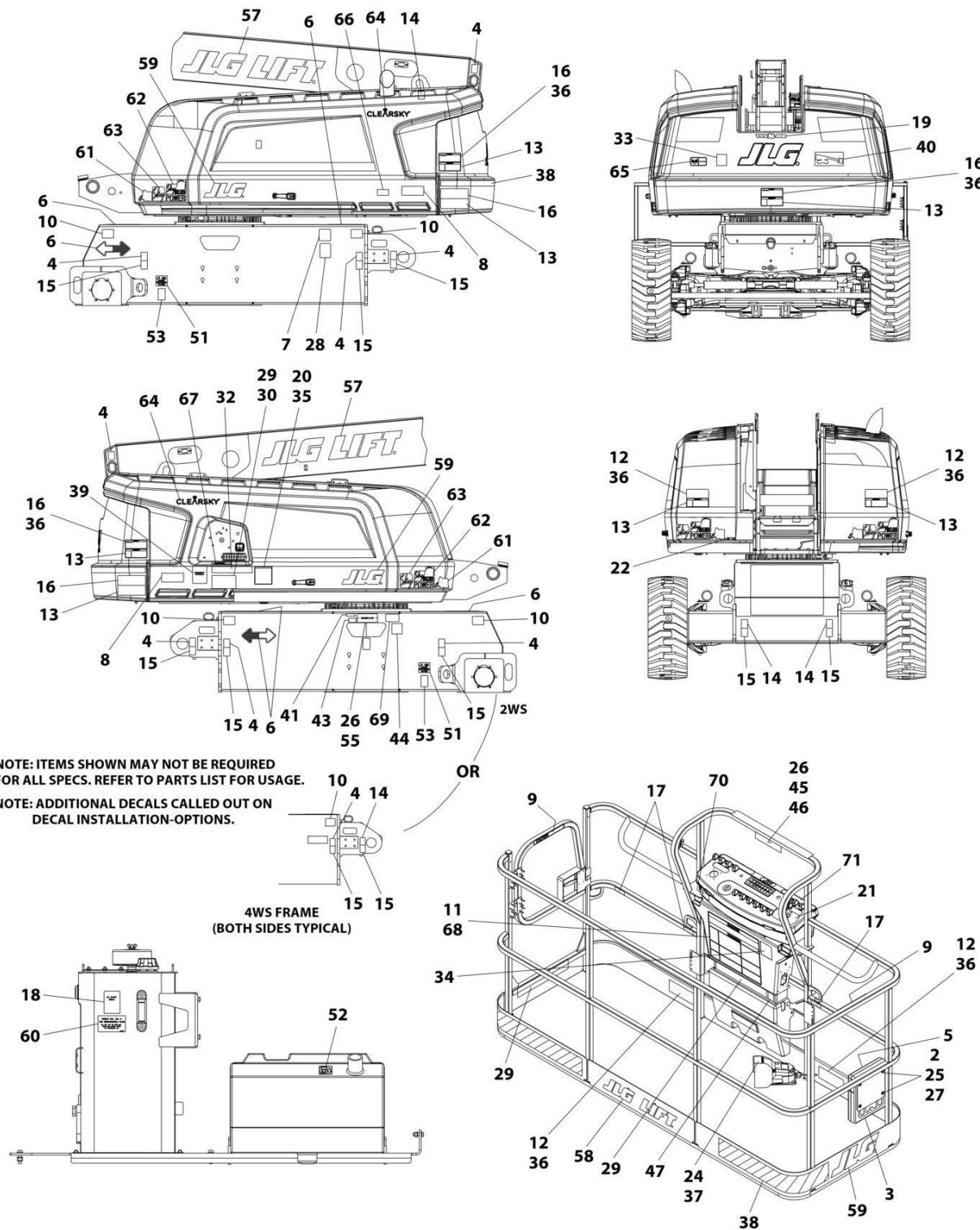
FIGURE 9-17. DECAL INSTALLATION (JAPANESE SPECS - ENGLISH/JAPANESE LANGUAGES) (660SJ)
