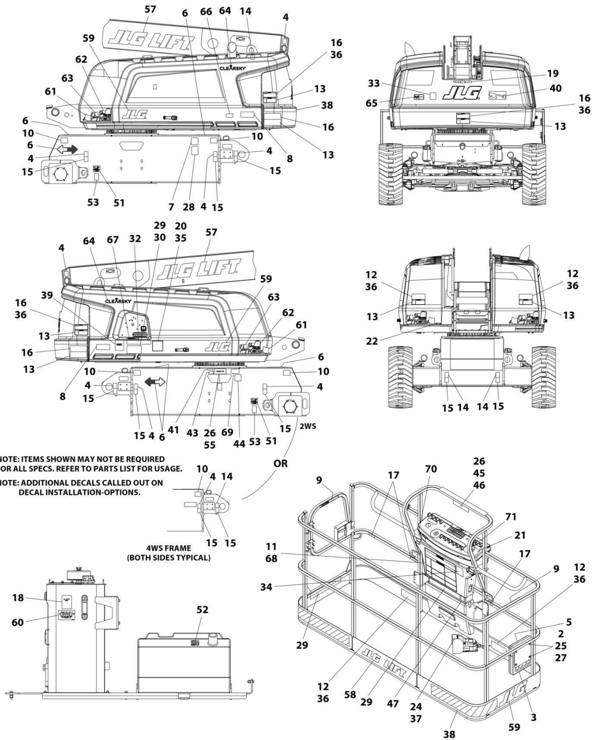
FIGURE 9-12. DECAL INSTALLATION (BRAZIL SPECS - PORTUGUESE/SPANISH LANGUAGES) (660SJ)
