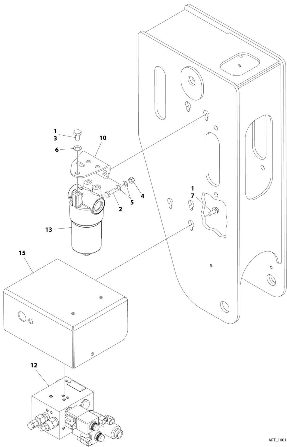
FIGURE 4-12. BOOM VALVES INSTALLATION - WITH 2WS (600S)
