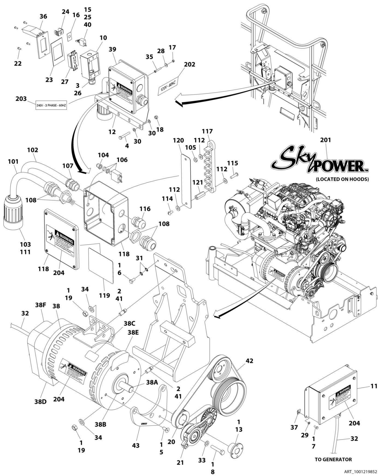
FIGURE 3-75. 7500W SKYPOWER GENERATOR INSTALLATION - 110V/60HZ (FORD ENGINES) (OPTIONAL)
