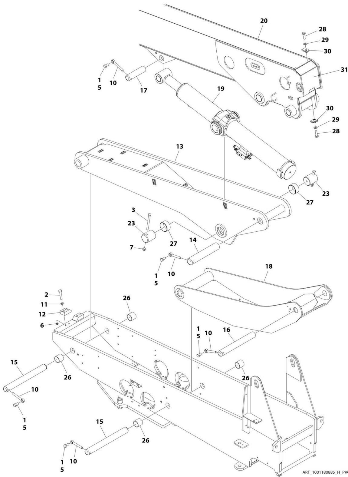
FIGURE 4-3. BOOM INSTALLATION (660SJ)
