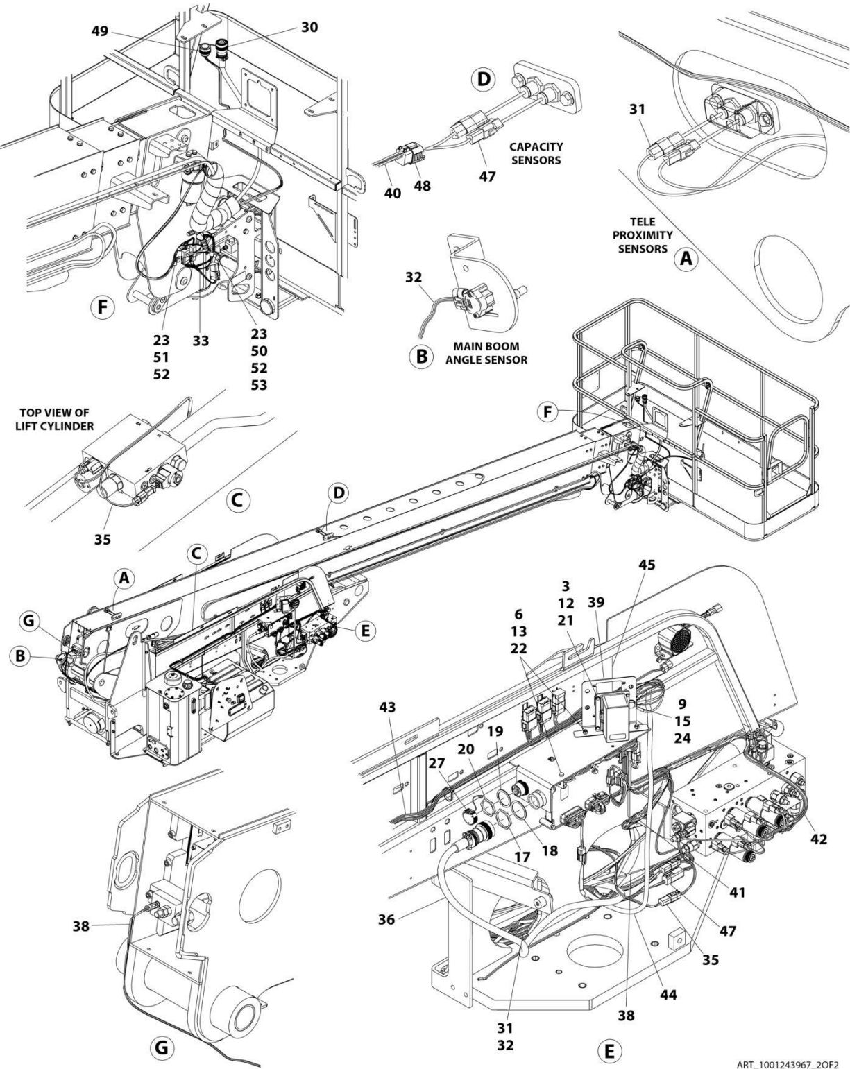
FIGURE 8-42. ELECTRICAL COMPONENTS INSTALLATION - WITH 2WS (600S)
