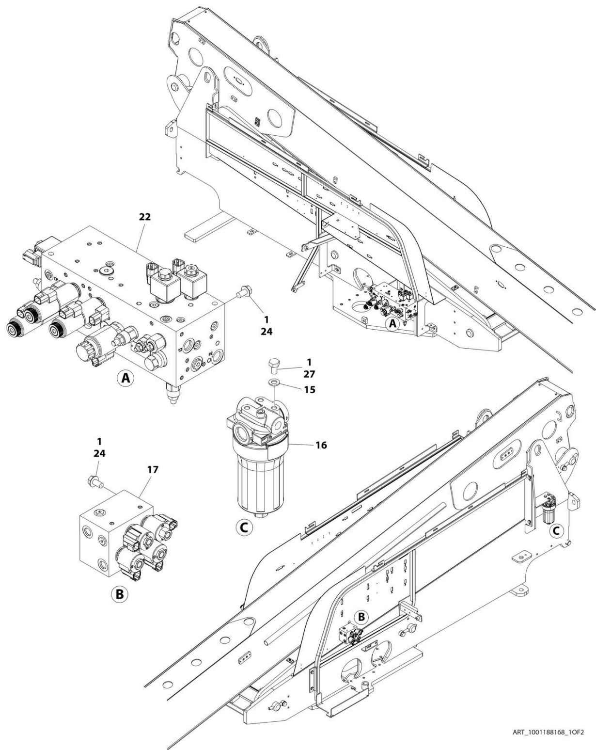
FIGURE 2-3. VALVE INSTALLATION - WITH 2WS (660SJ)
