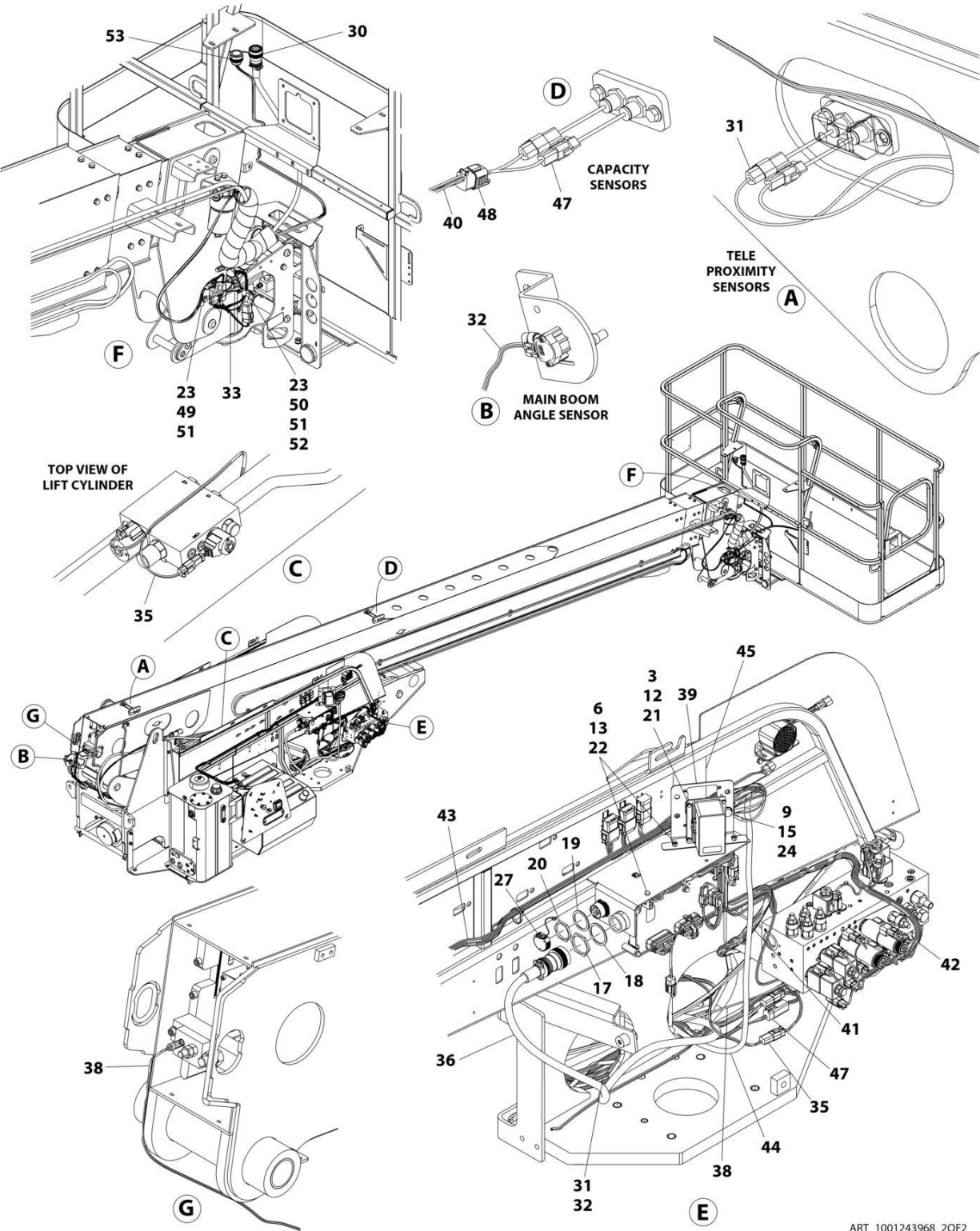
FIGURE 8-44. ELECTRICAL COMPONENTS INSTALLATION - WITH 4WS (600S)
