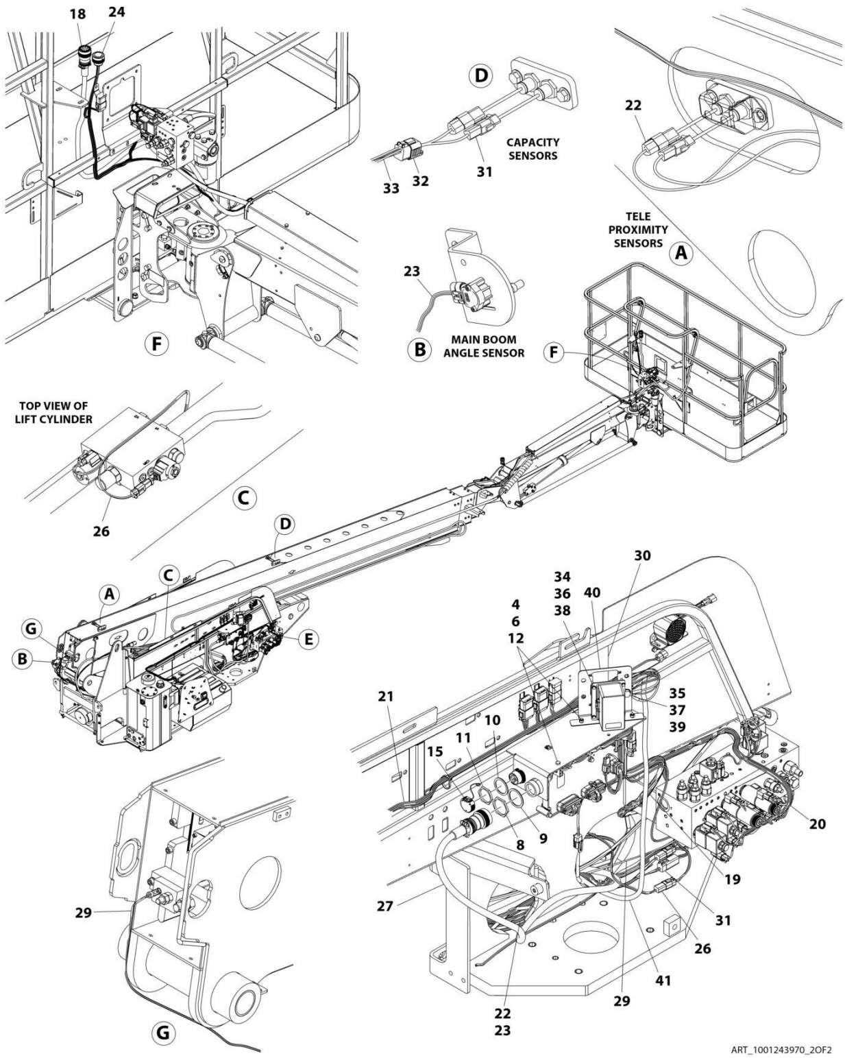
FIGURE 8-48. ELECTRICAL COMPONENTS INSTALLATION - WITH 4WS (660SJ)
