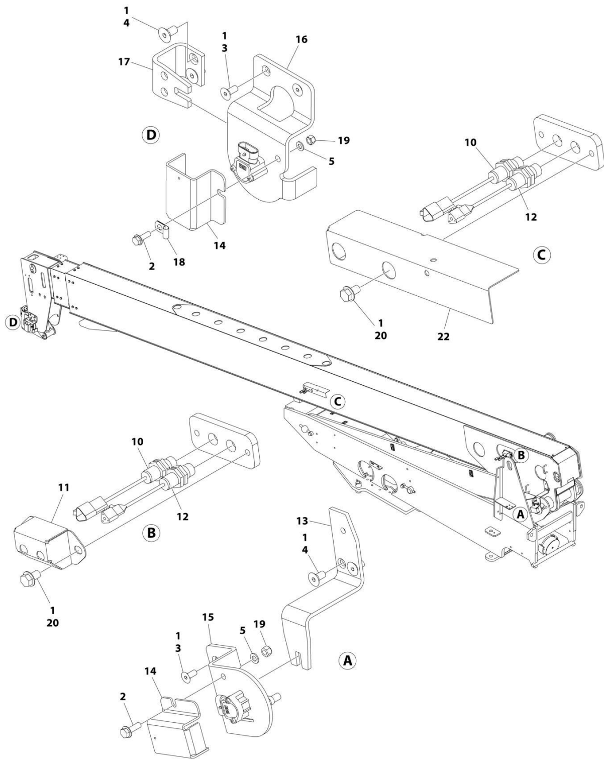
FIGURE 4-18. BOOM SENSORS INSTALLATION (MACHINES WITH SN STARTING WITH 03) (600S)
