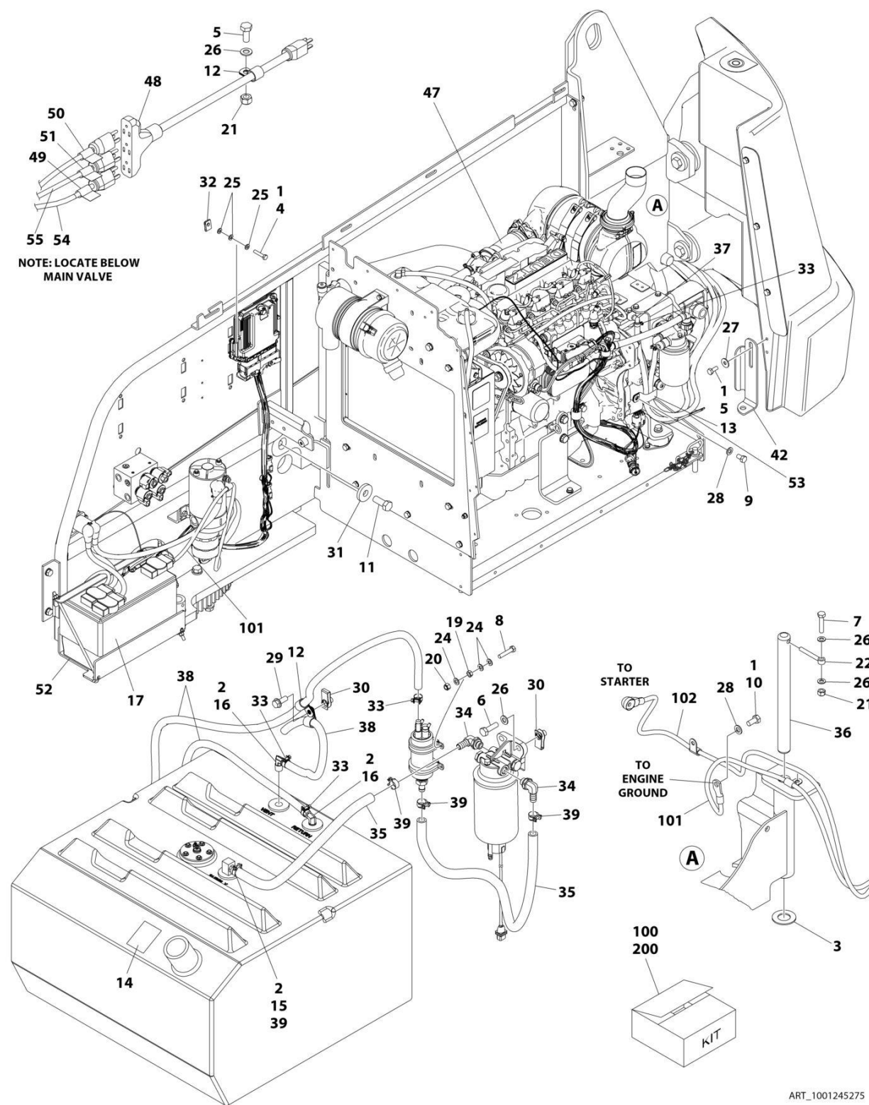
FIGURE 3-19. DEUTZ D2.9L4 - 49HP ENGINE INSTALLATION - WITH ARCTIC PACKAGE
