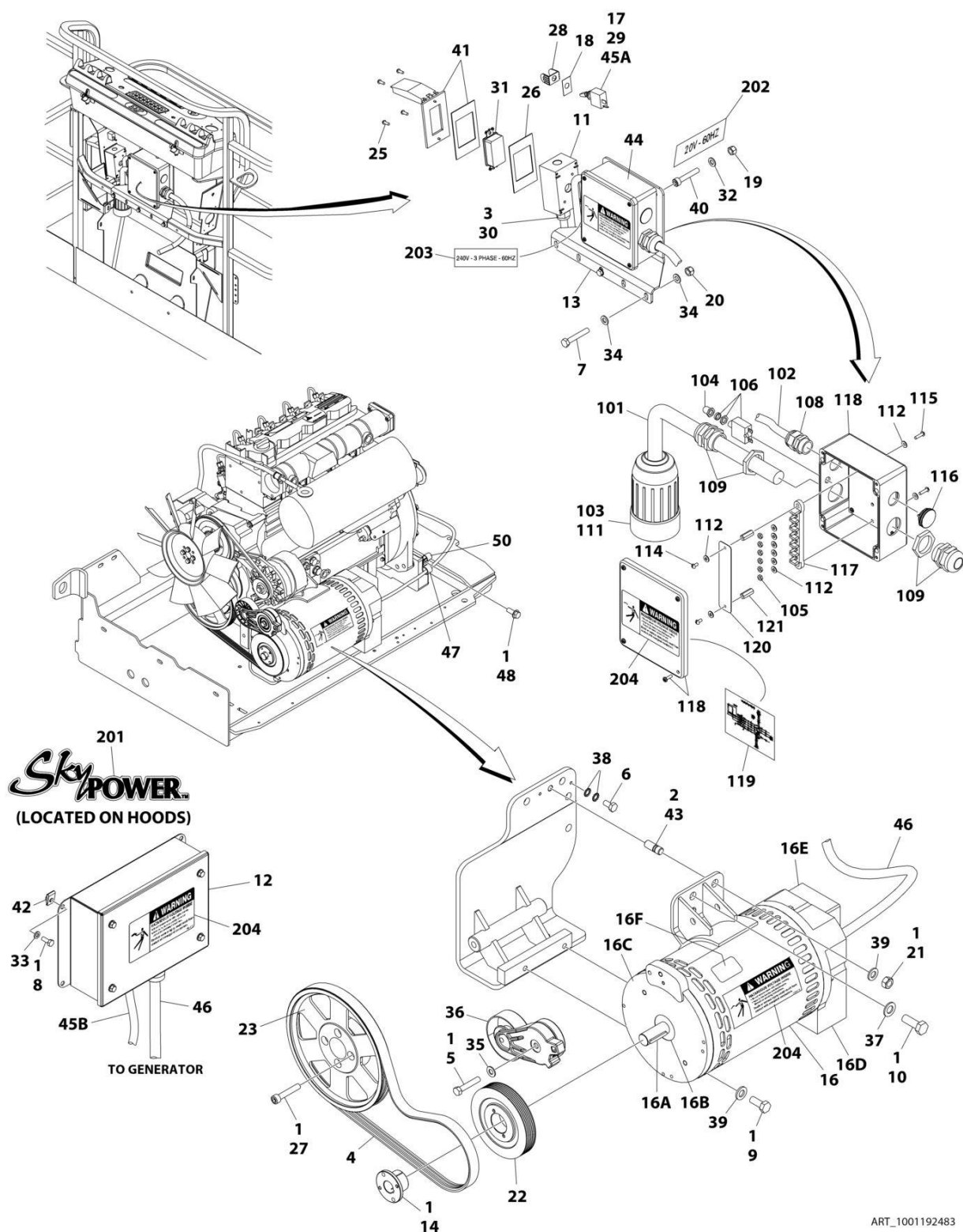
FIGURE 3-72. 7500W SKYPOWER GENERATOR INSTALLATION - 110/60HZ (DEUTZ D2011 ENGINES) (OPTIONAL)
