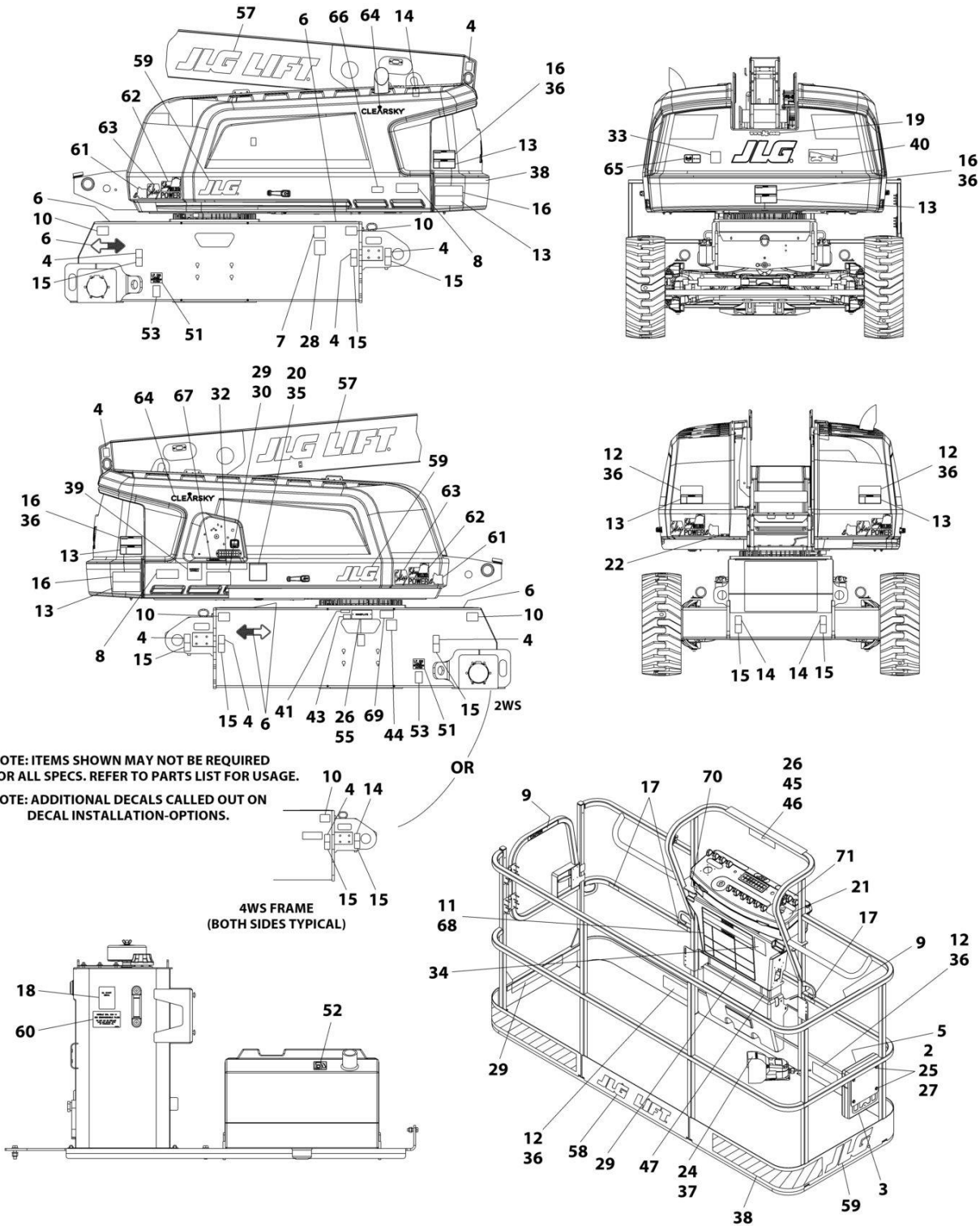
FIGURE 9-10. DECAL INSTALLATION (ANSI SPECS - ENGLISH LANGUAGE) (660SJ)
