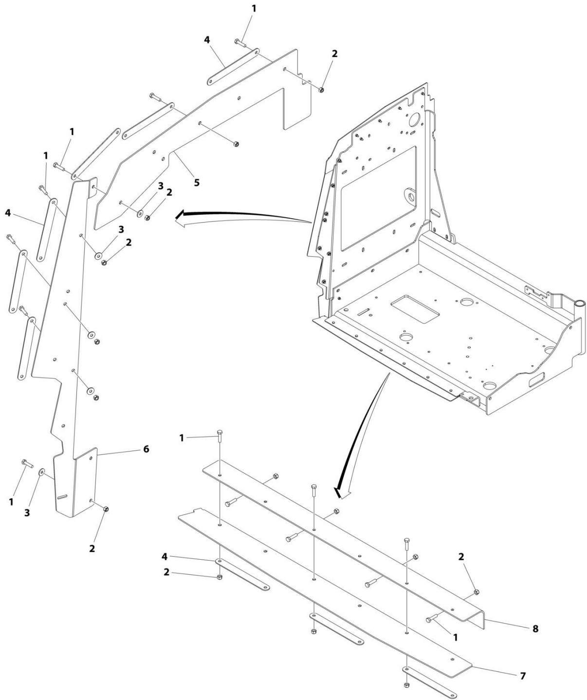
FIGURE 3-58. ENGINE HOOD BAFFLES INSTALLATION - ABS HOODS (DEUTZ D2.9L4 - 49HP ENGINES)
