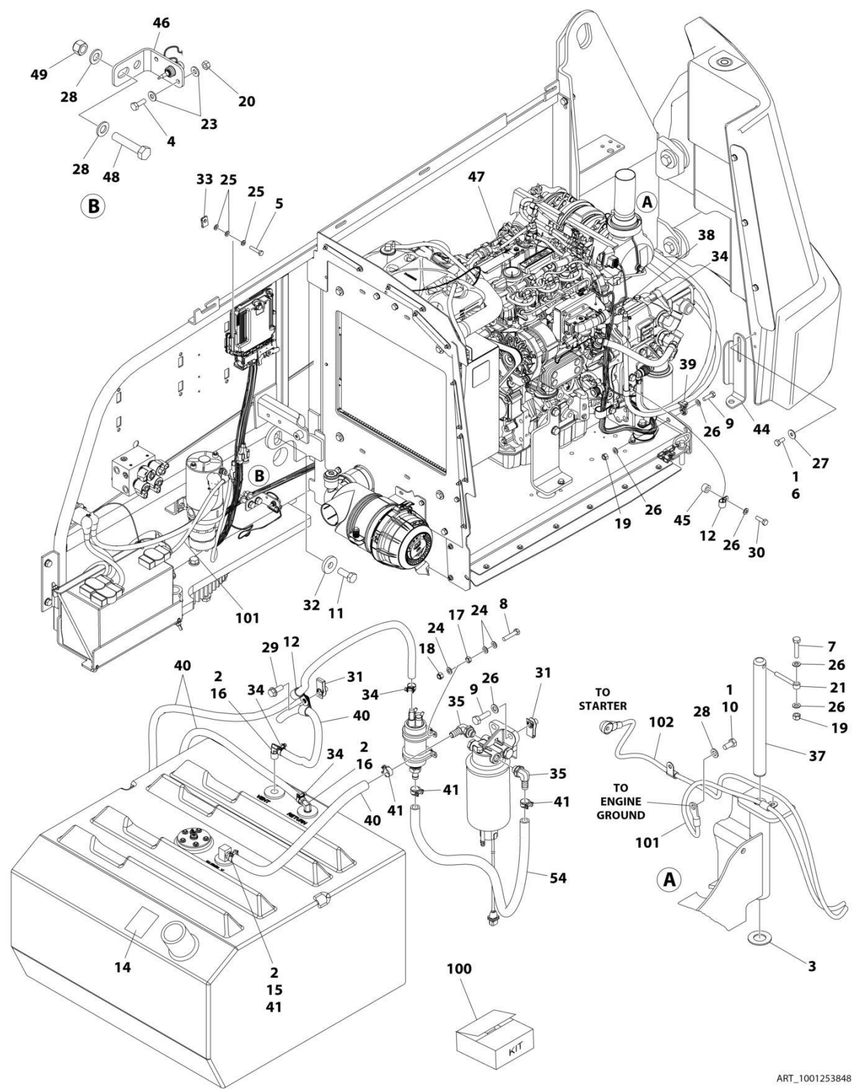
FIGURE 3-12. DEUTZ TD2.2L3 (STAGE V) ENGINE INSTALLATION
