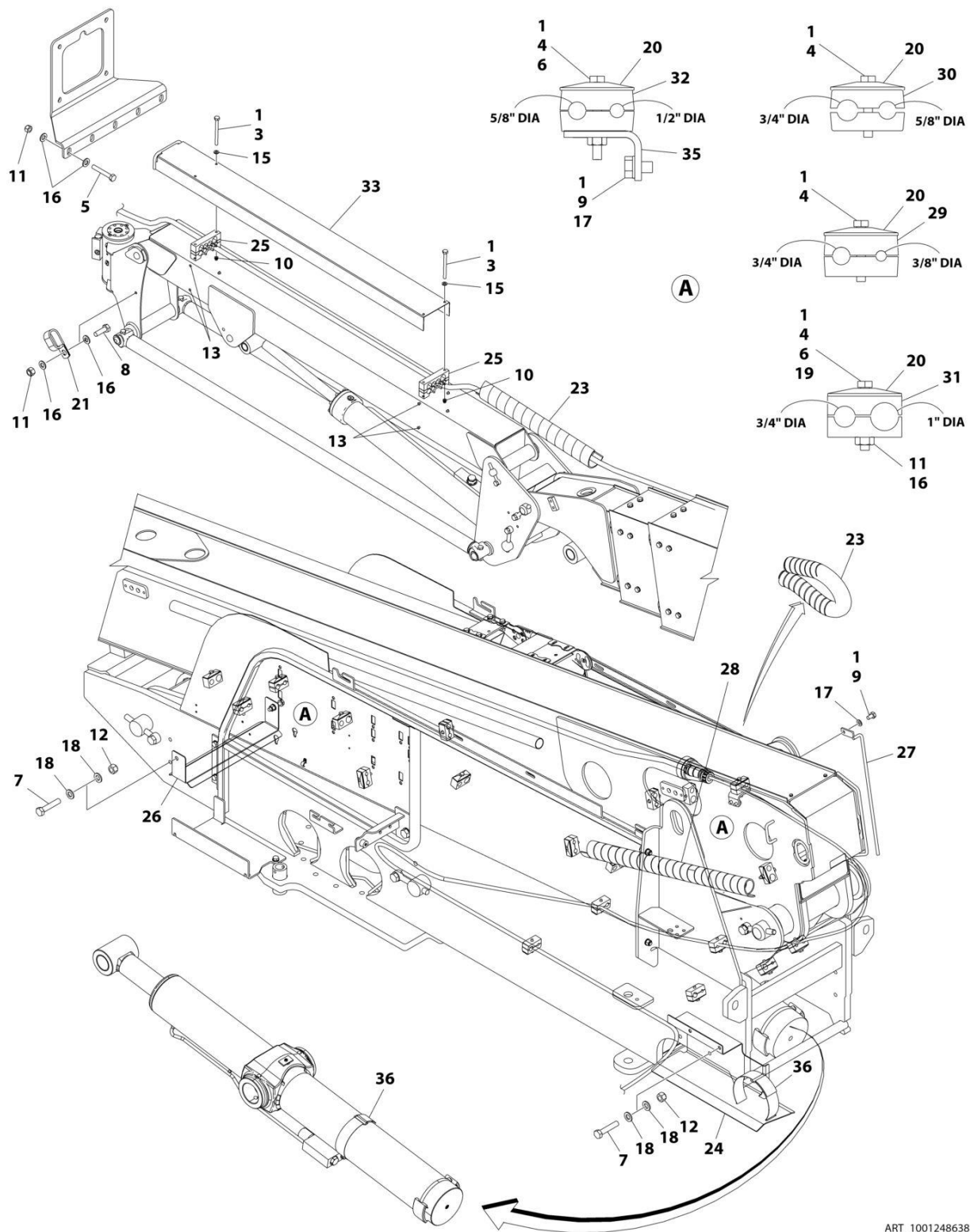
FIGURE 8-26. AC CABLES AND CLAMPS INSTALLATION - WITHOUT GENERATOR AND WITHOUT AC CABLES (MACHINES WITH SN STARTING WITH B3) (660SJ)
