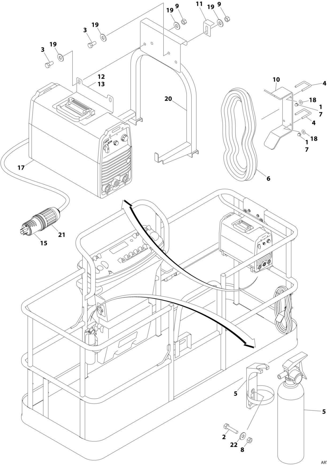
FIGURE 5-36. SKYWELDER INSTALLATION (60HZ)
