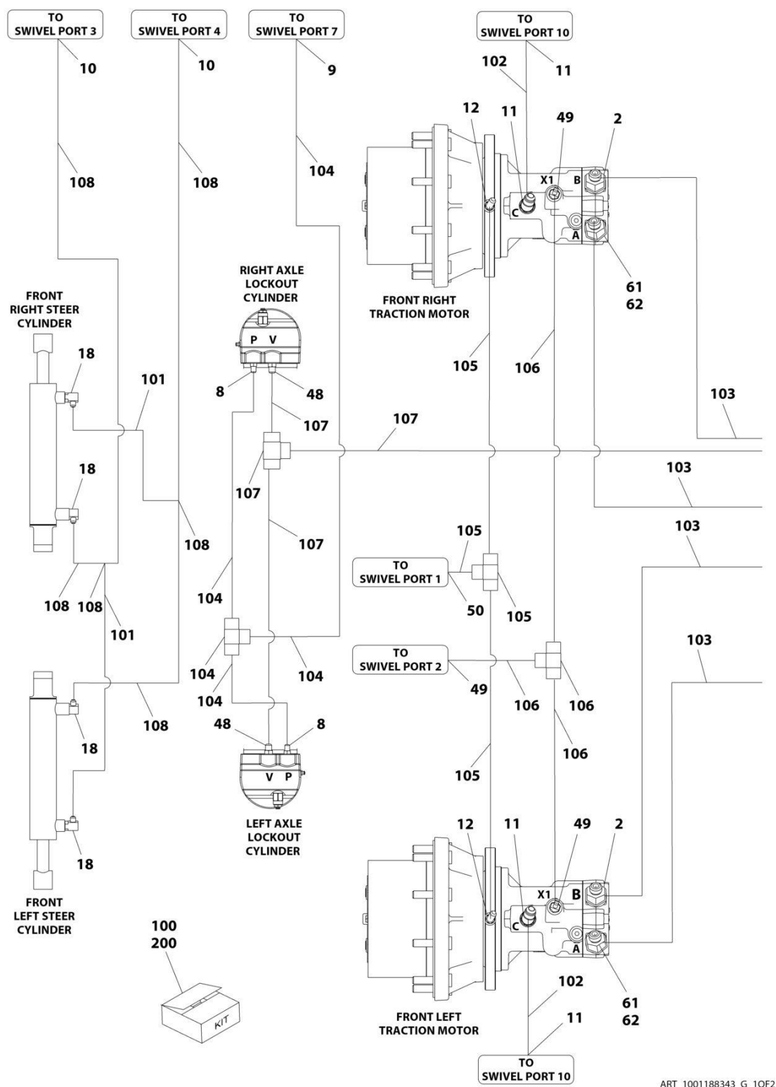
FIGURE 7-3. DRIVE HYDRAULIC DIAGRAM (4WS)
