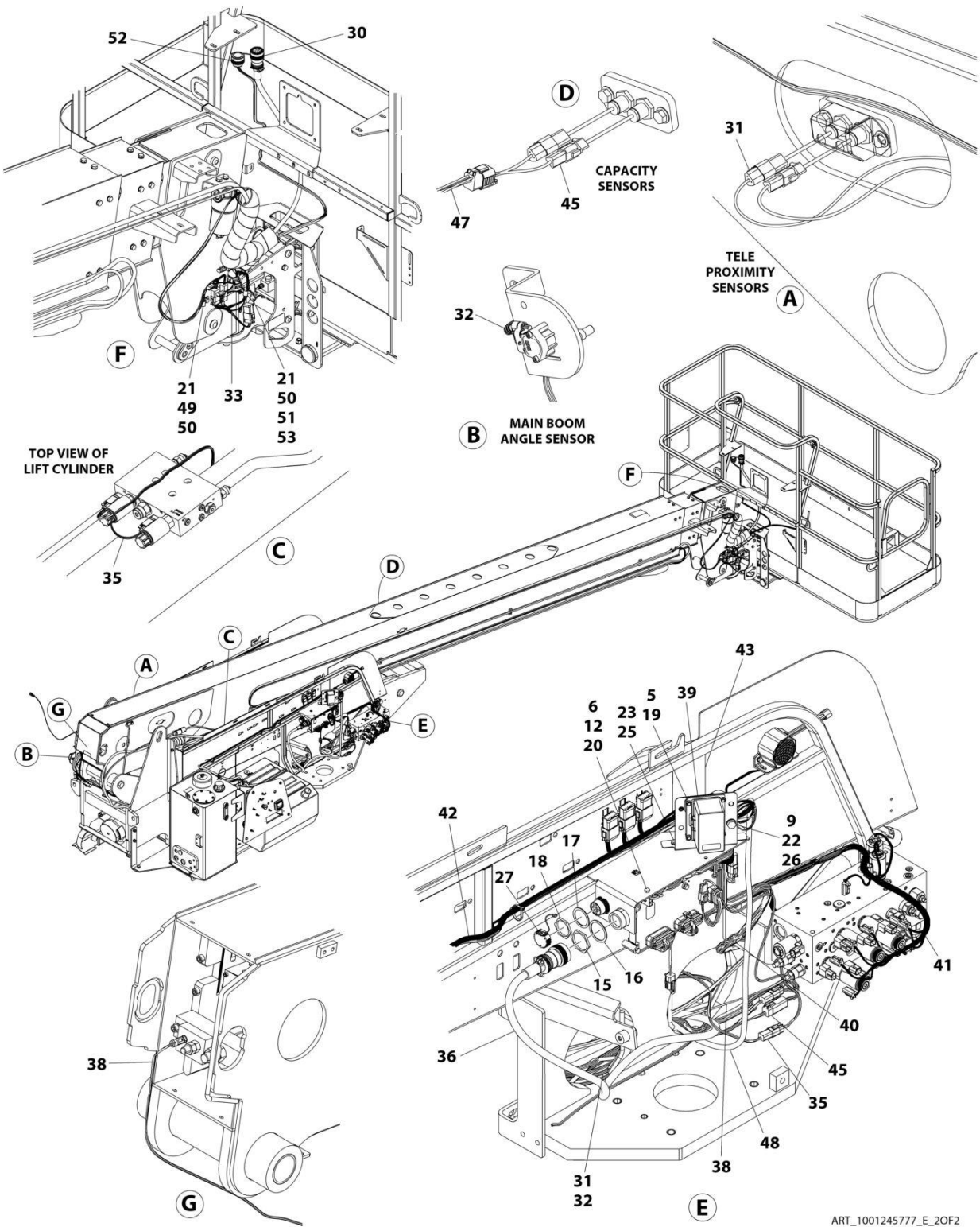
FIGURE 8-45. ELECTRICAL COMPONENTS INSTALLATION - WITH 4WS AND DEUTZ TD2.2L3 (STAGE V) ENGINE (600S)
