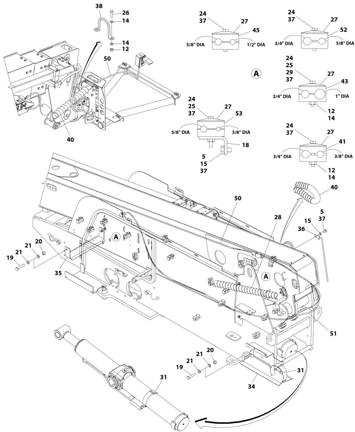
FIGURE 8-18. AC CABLES AND CLAMPS INSTALLATION - WITHOUT GENERATOR (ANSI, CSA AND JAPANESE SPECS) (600S)
