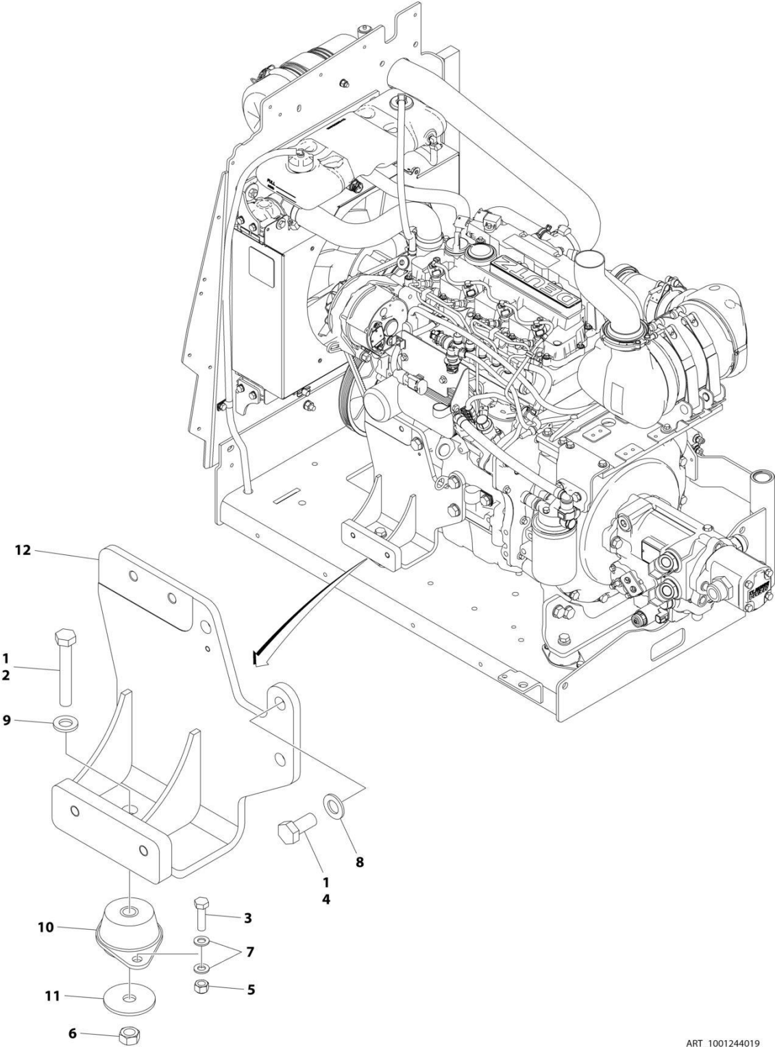
FIGURE 3-52. MOTOR MOUNT INSTALLATION - WITH GENERATOR (DEUTZ TD2.9L4 - 49HP ENGINES)
