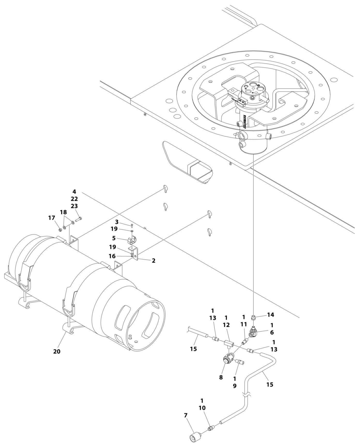
FIGURE 1-17. LP TANKS AND BRACKETS INSTALLATION (FORD ENGINES)
