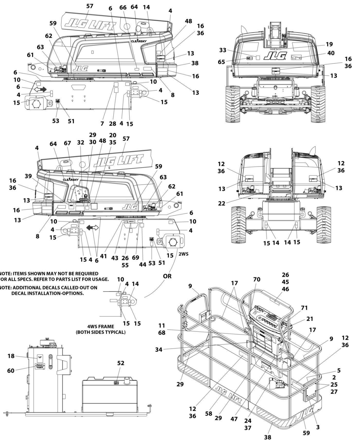
FIGURE 9-14. DECAL INSTALLATION (CHINESE SPECS - ENGLISH/SIMPLIFIED CHINESE LANGUAGES) (660SJ)
