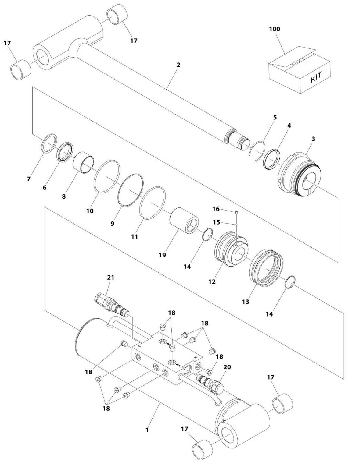
FIGURE 6-4. LEVEL CYLINDER ASSEMBLY - PLATFORM SLAVE (660SJ)
