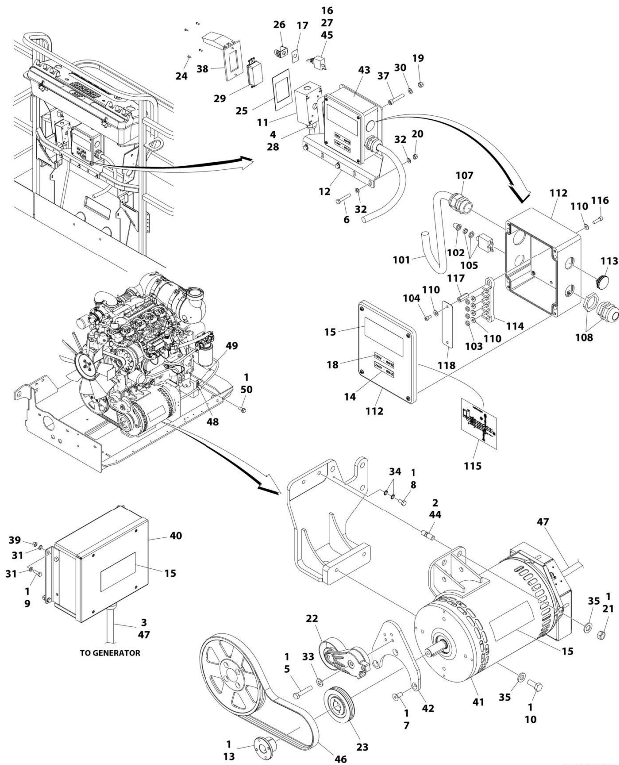
FIGURE 3-68. 4000W GENERATOR INSTALLATION - 110V/60HZ (DEUTZ TD2.9L4 - 67HP ENGINES) (OPTIONAL)
