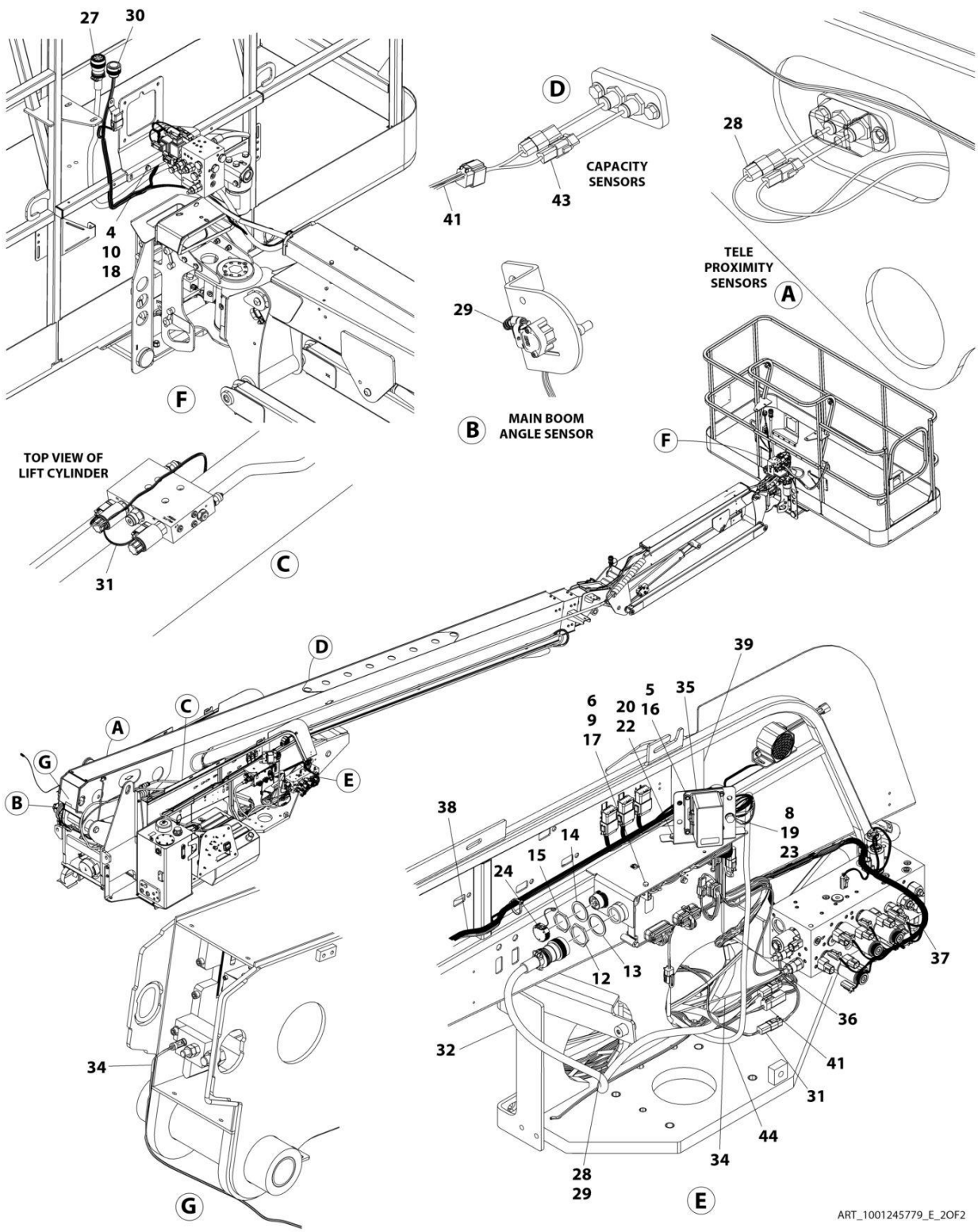
FIGURE 8-49. ELECTRICAL COMPONENTS INSTALLATION - WITH 4WS AND DEUTZ TD2.2L3 (STAGE V) ENGINE (660SJ)
