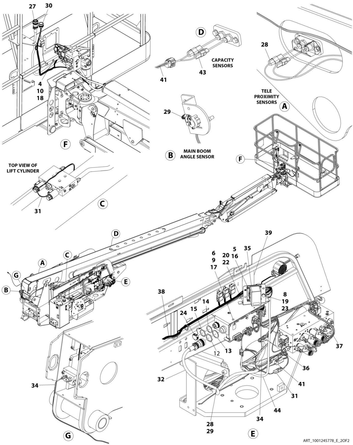
FIGURE 8-47. ELECTRICAL COMPONENTS INSTALLATION - WITH 2WS AND DEUTZ TD2.2L3 (STAGE V) ENGINE (660SJ)
