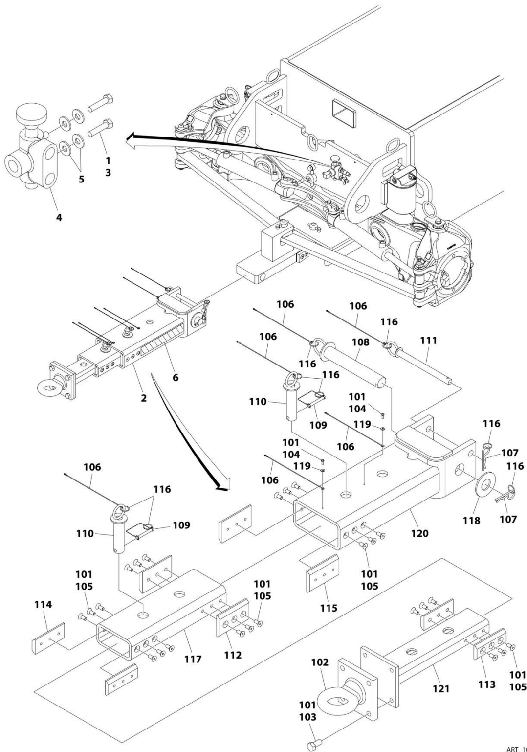
FIGURE 1-20. TOW BAR INSTALLATION
