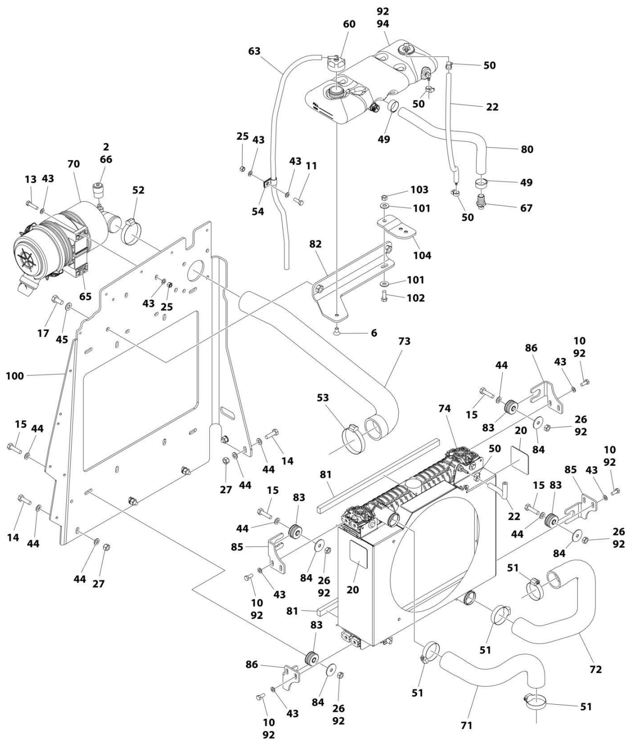
FIGURE 3-18. DEUTZ D2.9L4 - 49HP ENGINE ASSEMBLY - WITHOUT ARCTIC PACKAGE
