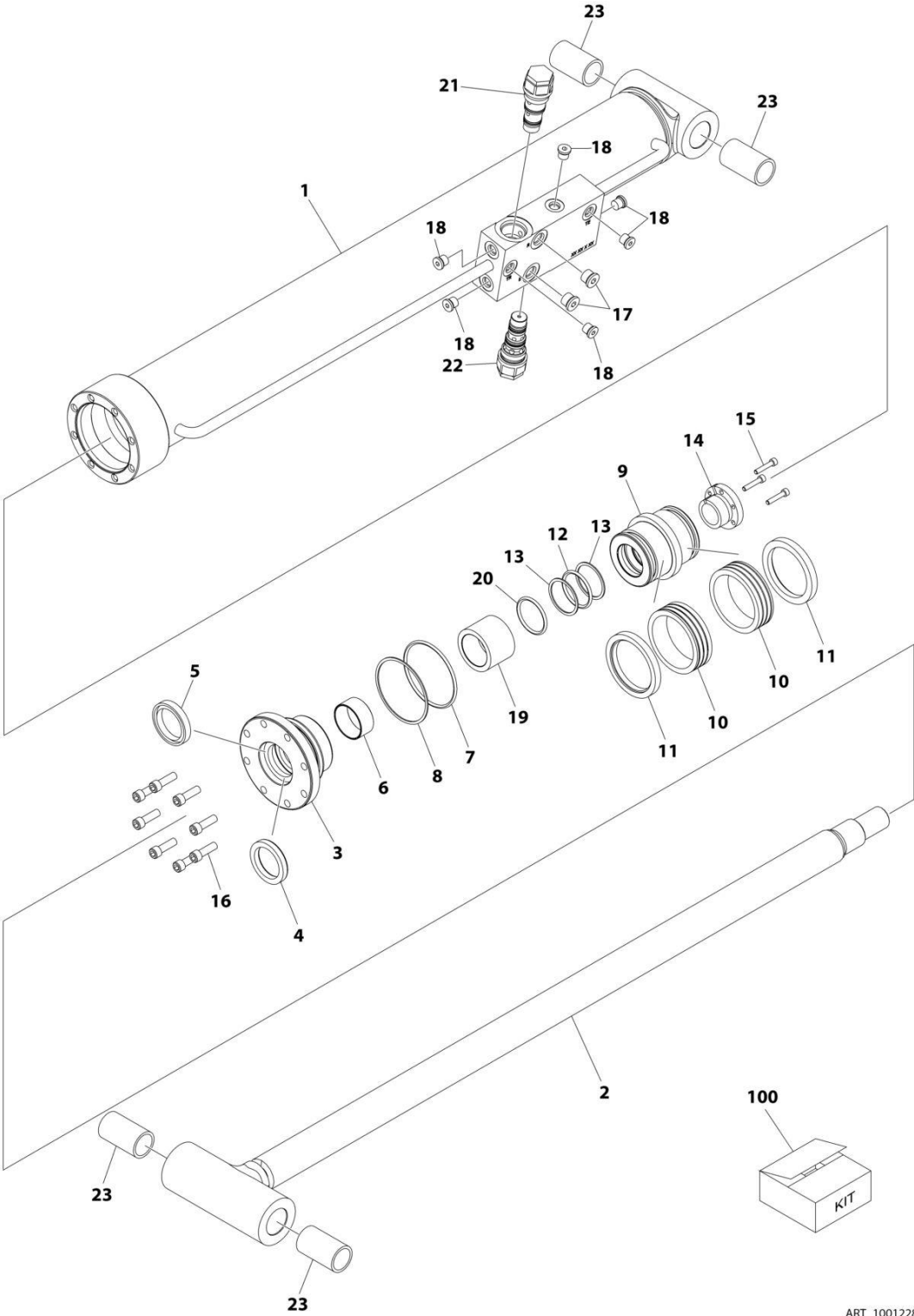
FIGURE 6-5. LIFT CYLINDER ASSEMBLY - JIB (MACHINES WITH SN STARTING WITH 03) (660SJ)
