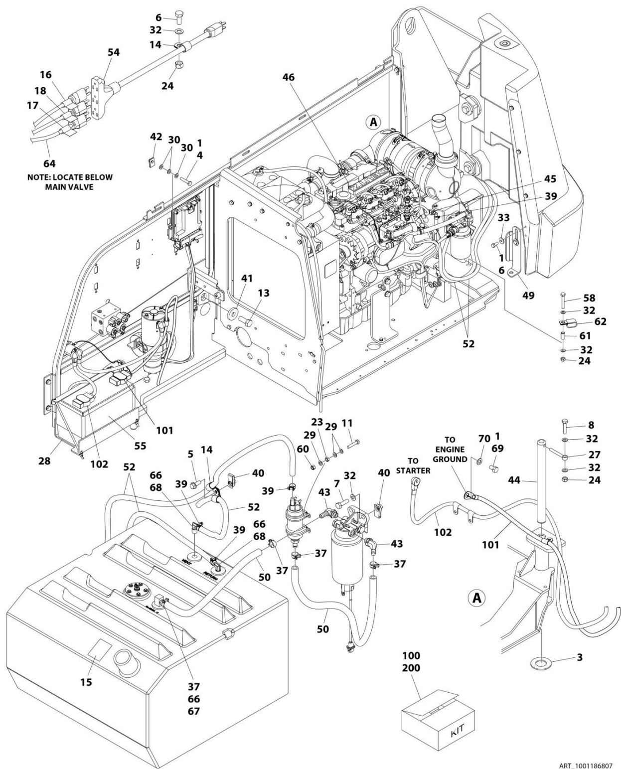
FIGURE 3-26. DEUTZ TD2.9L4 - 67HP ENGINE INSTALLATION - WITH ARCTIC PACKAGE
