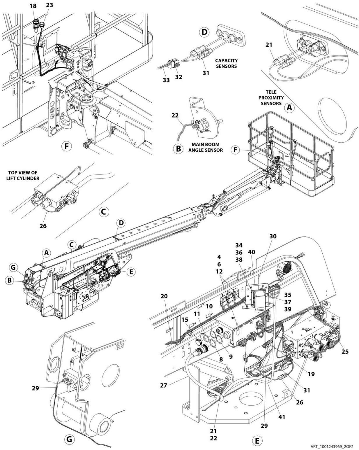
FIGURE 8-46. ELECTRICAL COMPONENTS INSTALLATION - WITH 2WS (660SJ)
