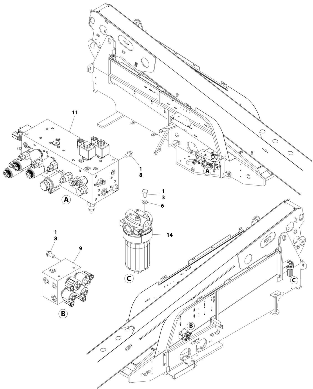
FIGURE 2-1. VALVE INSTALLATION - WITH 2WS (600S)
