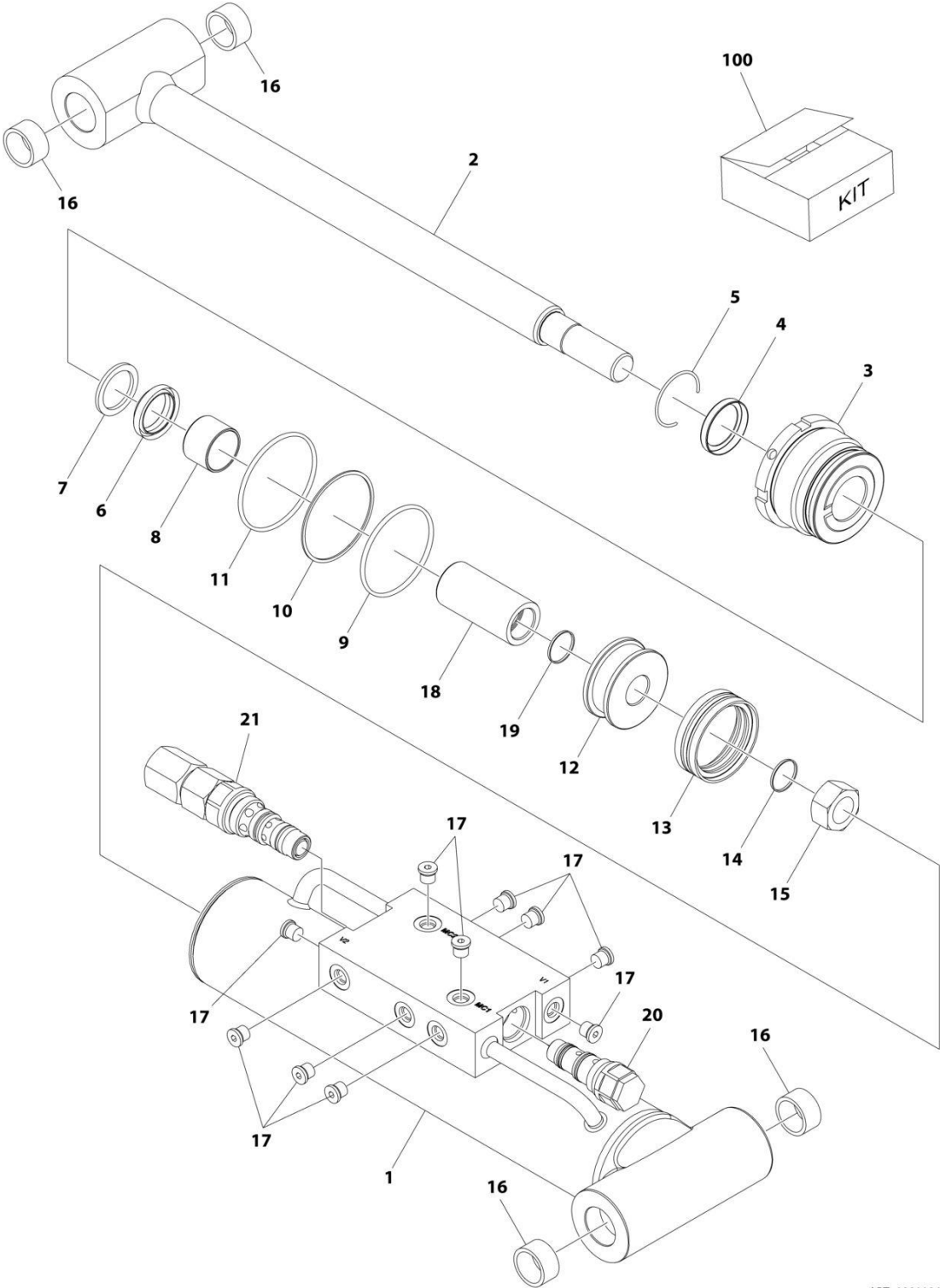
FIGURE 6-3. LEVEL CYLINDER ASSEMBLY - PLATFORM SLAVE (600S)
