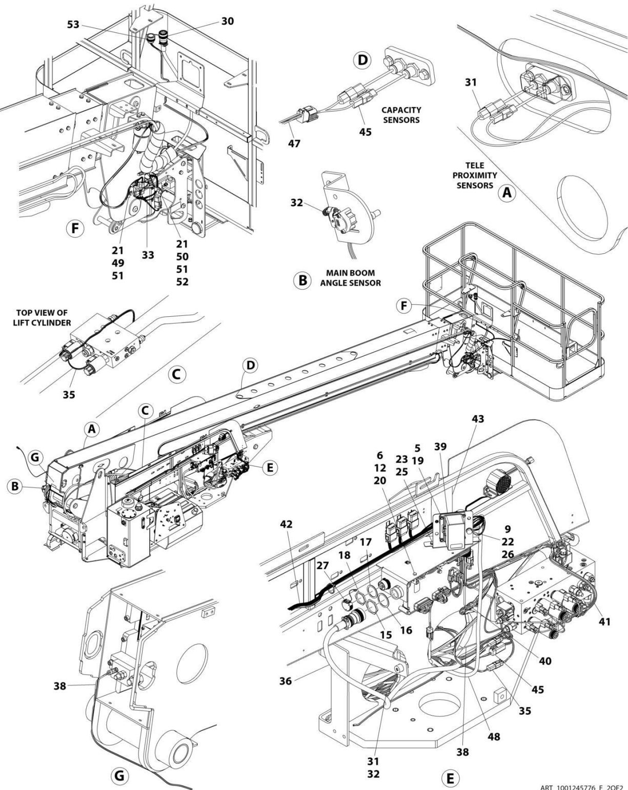
FIGURE 8-43. ELECTRICAL COMPONENTS INSTALLATION - WITH 2WS AND DEUTZ TD2.2L3 (STAGE V) ENGINE (600S)
