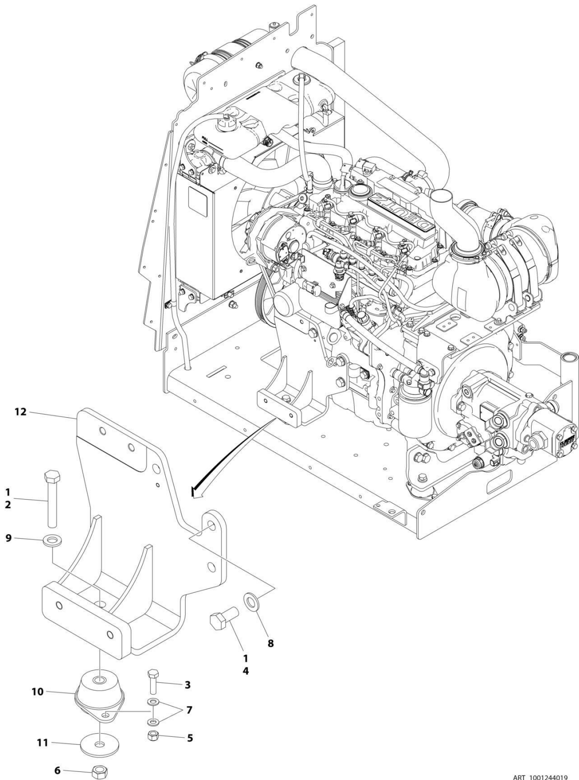
FIGURE 3-44. ENGINE MOUNT (WITH GENERATOR) - DEUTZ D2.9L4 AND DEUTZ D2.9L4 (STAGE V) ENGINES
