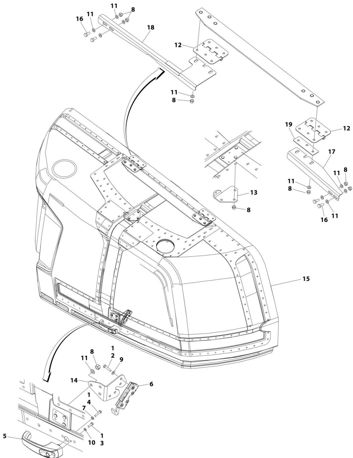
FIGURE 2-47. ABS HOOD ASSEMBLY - ENGINE SIDE (CE & UK CA SPEC)
