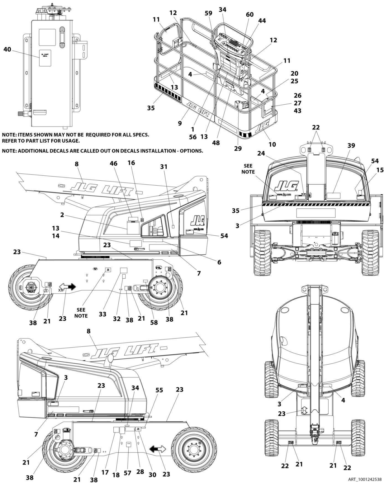
FIGURE 9-1. DECAL INSTALLATION - ANSI, ANSI EXPORT AND CSA SPECS - ENGLISH (400S)
