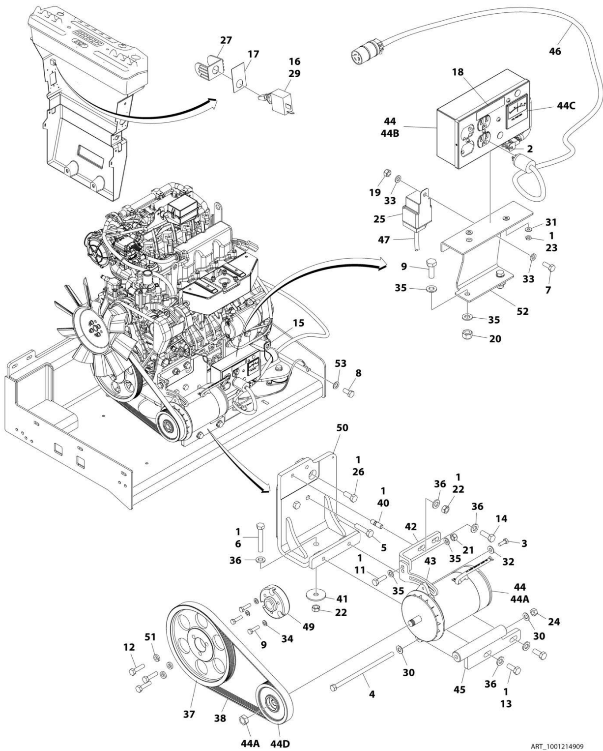
FIGURE 3-49. GENERATOR INSTALLATION - 2500W/60HZ (KUBOTA ENGINE)
