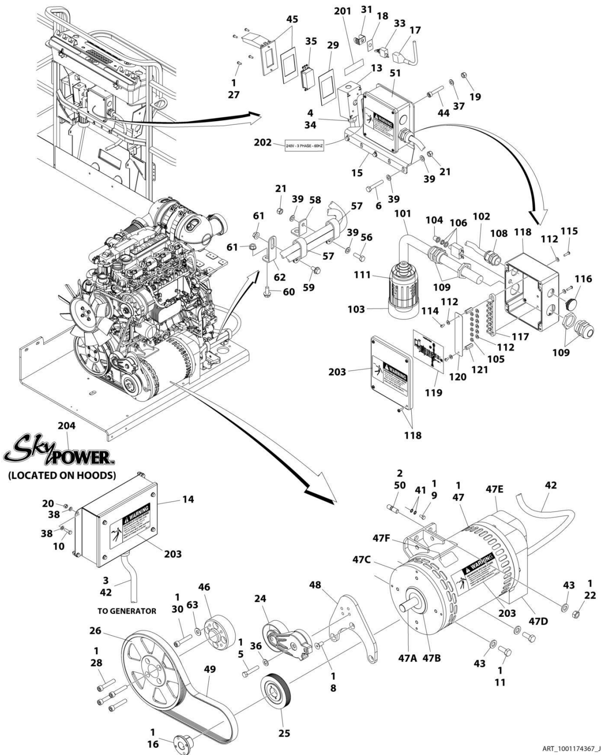
FIGURE 3-56. GENERATOR INSTALLATION - 7500W/60HZ (DEUTZ D2.9L4 ENGINE)
