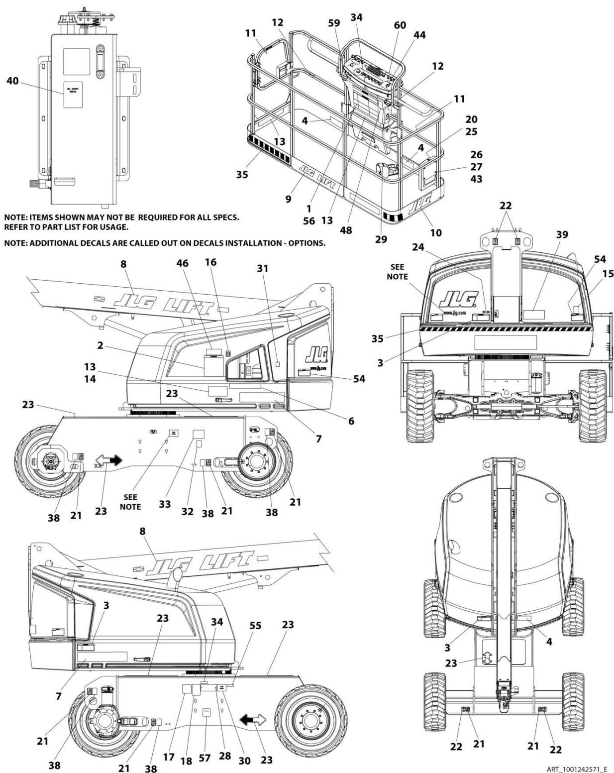
FIGURE 9-5. INSTALLATION - BRAZIL SPEC (DUAL LANGUAGE - PORTUGUESE/SPANISH) (400S)
