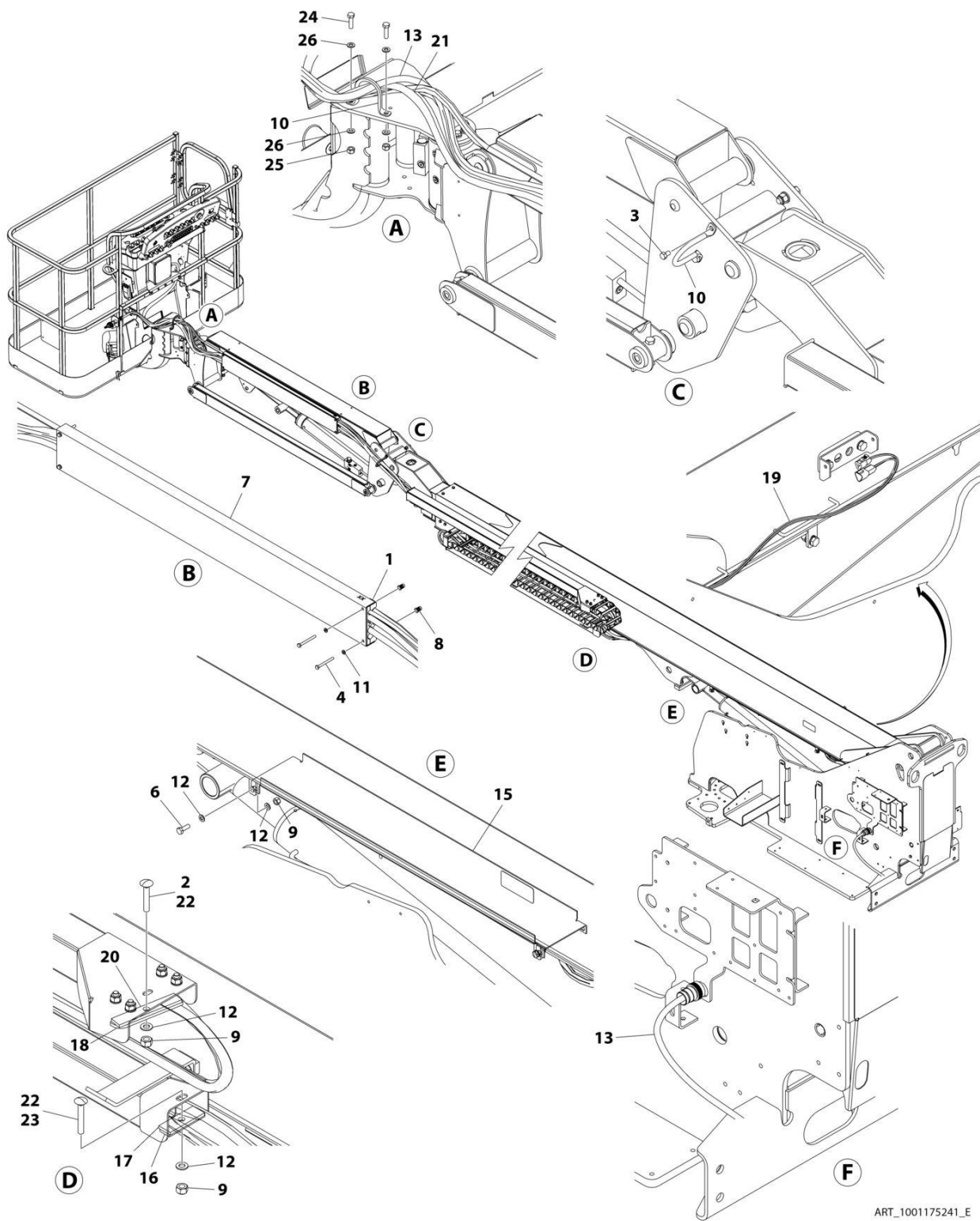
FIGURE 8-31. CABLES AND CLAMPS INSTALLATION - 460SJ (4000W GENERATOR 60HZ) (ANSI, ANSI EXPORT, CSA AND JAPANESE SPECS)
