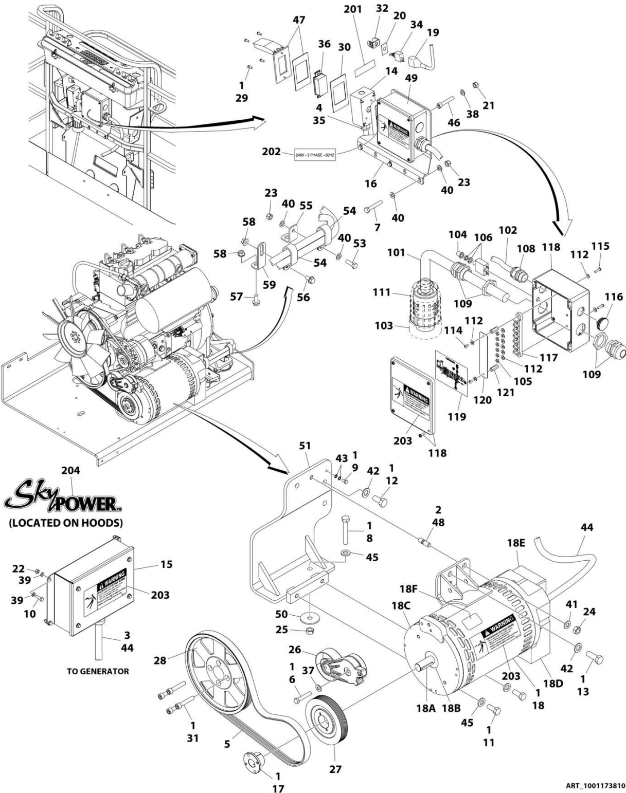
FIGURE 3-55. GENERATOR INSTALLATION - 7500W/60HZ (DEUTZ D2011 ENGINE)
