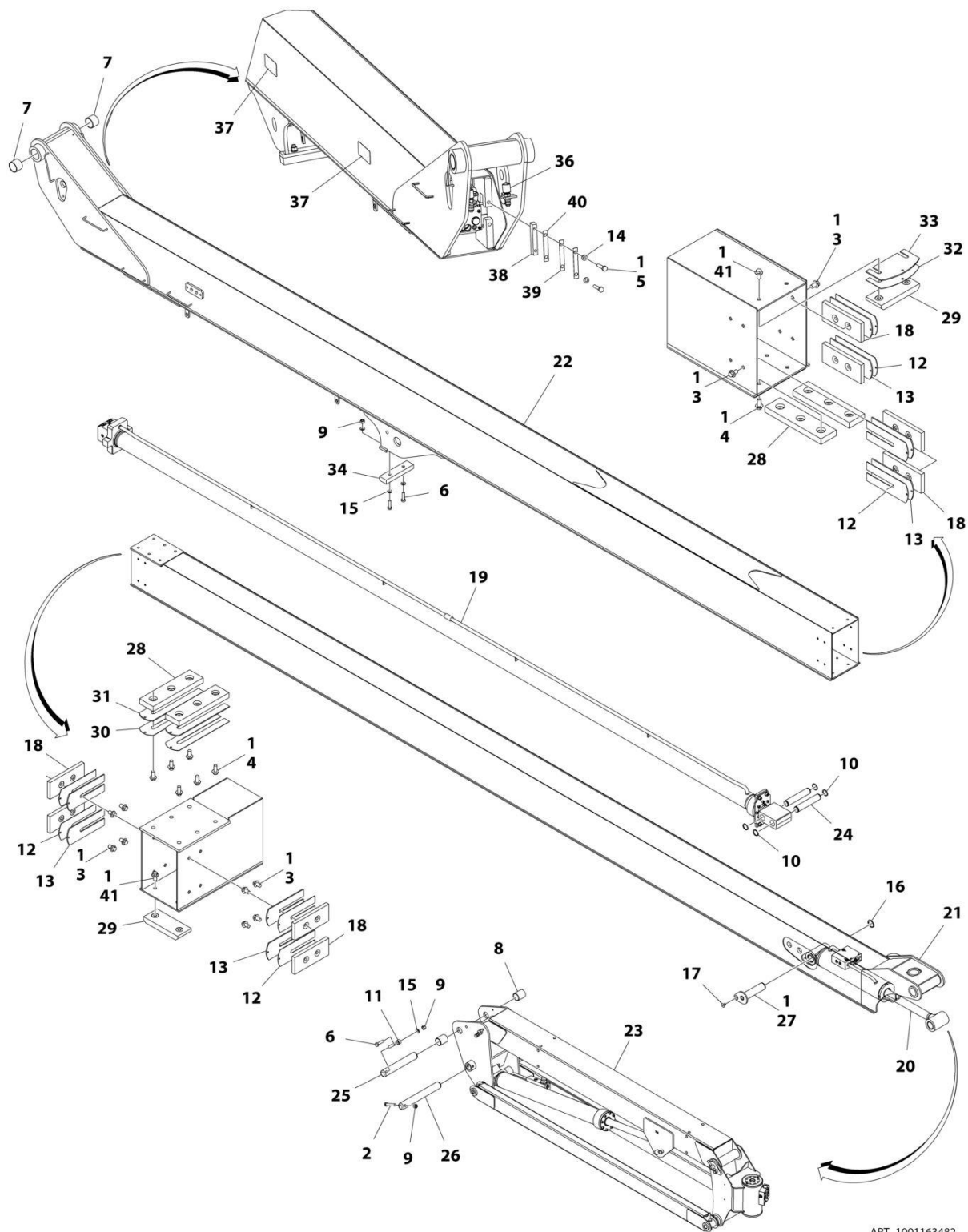
FIGURE 4-4. MAIN BOOM ASSEMBLY - 460SJ
