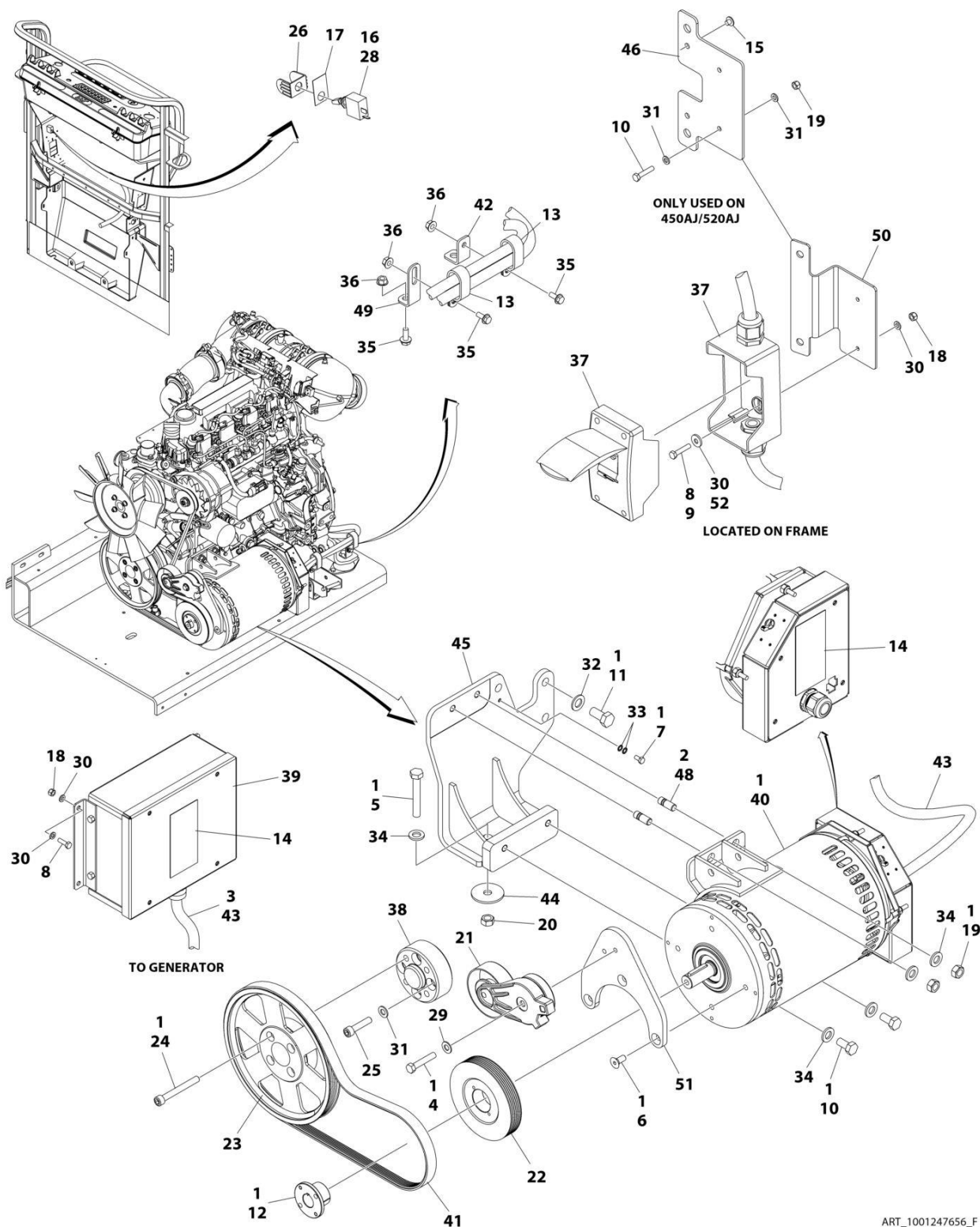
FIGURE 3-53. GENERATOR INSTALLATION - 4000W/50HZ (DEUTZ STAGE V ENGINE)
