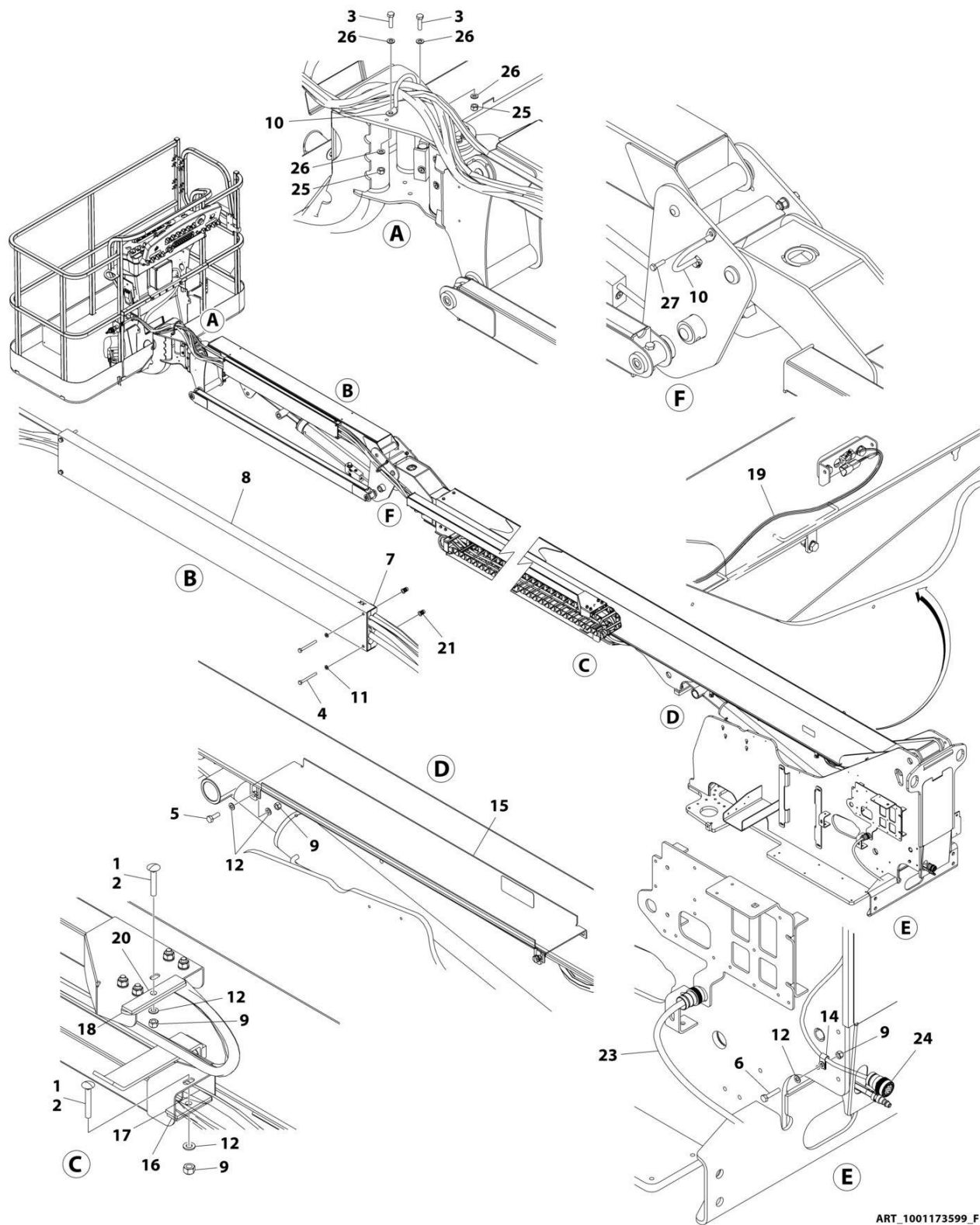
FIGURE 8-32. CABLES AND CLAMPS INSTALLATION - 460SJ (4000W GENERATOR 50HZ) (ALL SPECS)
