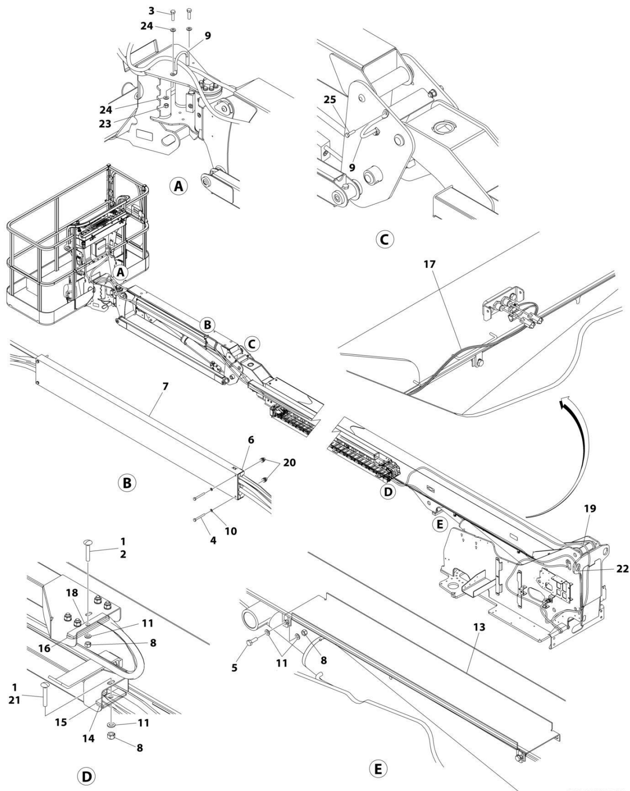
FIGURE 8-33. CABLES AND CLAMPS INSTALLATION - 460SJ (7500W GENERATOR) (ALL SPECS EXCEPT CE & UK CA SPECS)
