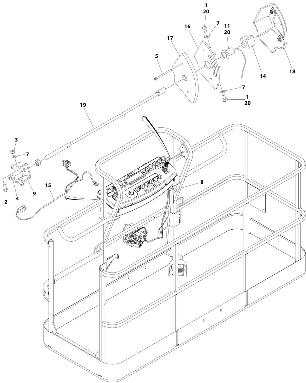
FIGURE 5-27. SKYLINE INSTALLATION
