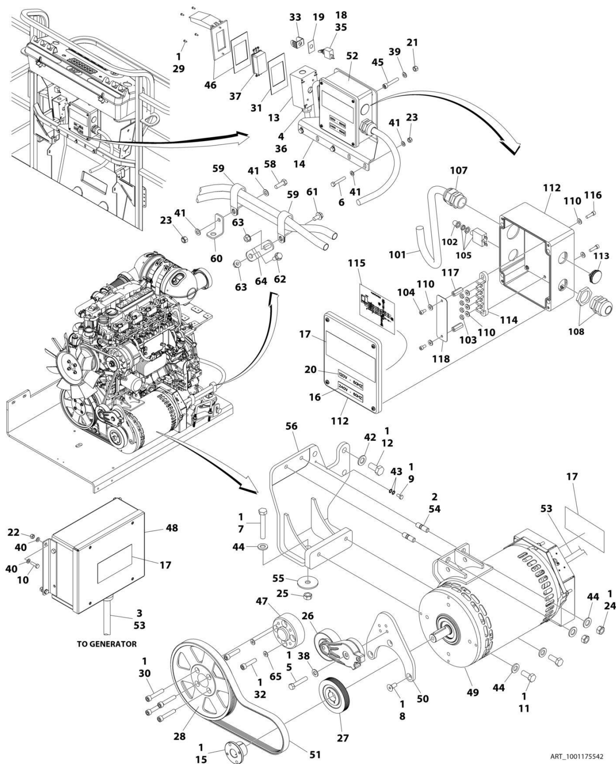
FIGURE 3-52. GENERATOR INSTALLATION - 4000W/60HZ (DEUTZ D2.9L4 ENGINE)
