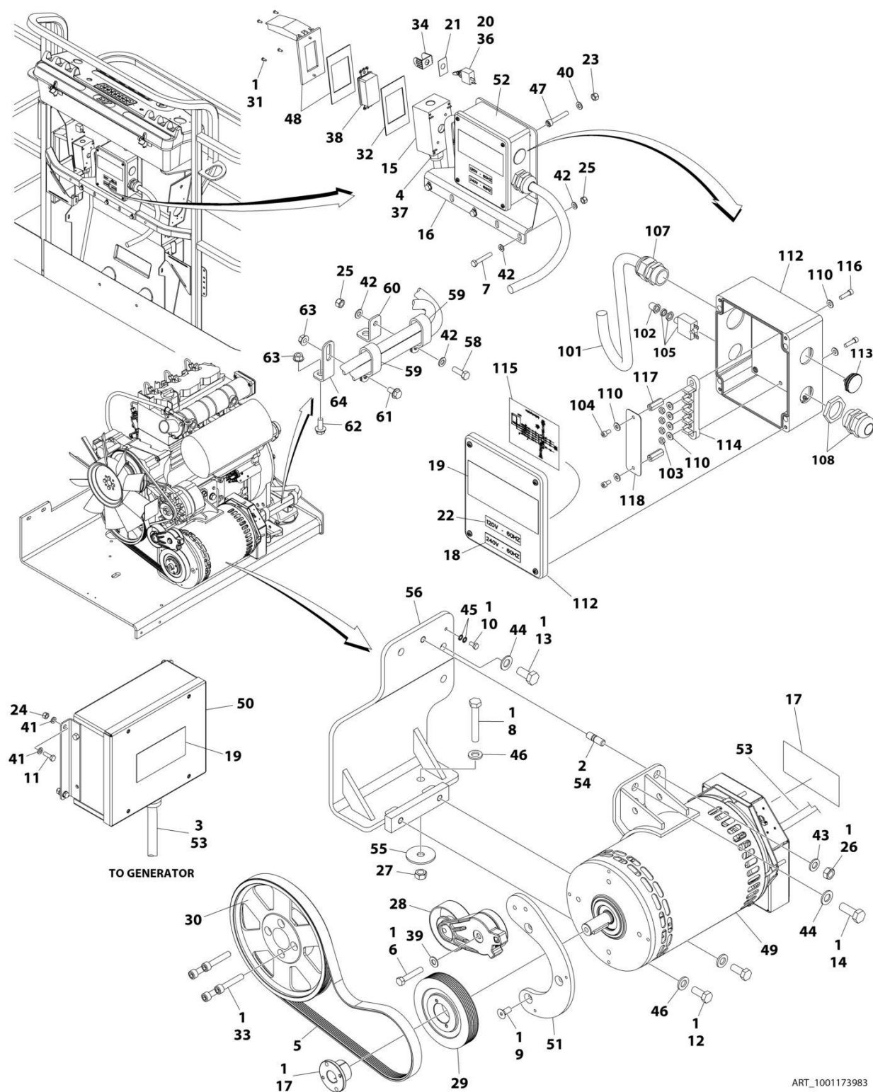
FIGURE 3-51. GENERATOR INSTALLATION - 4000W/60HZ (DEUTZ D2011 ENGINE)
