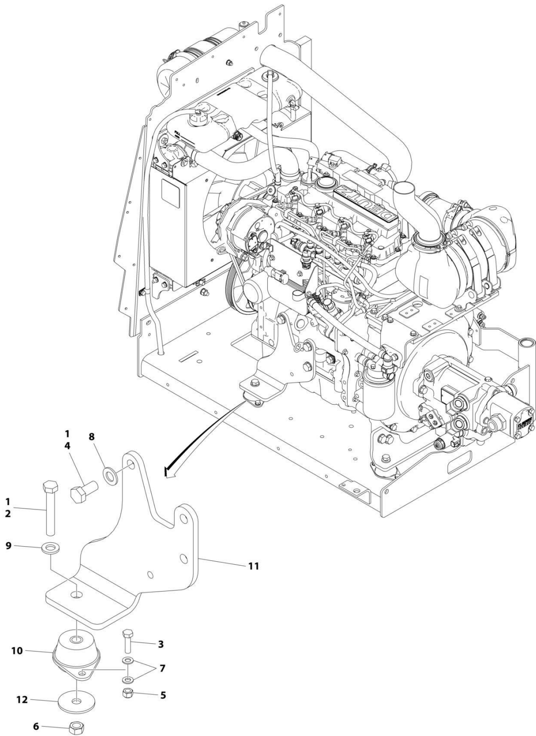
FIGURE 3-45. ENGINE MOUNT (WITHOUT GENERATOR) - DEUTZ D2.9L4, DEUTZ D2.9L4 (STAGE V) AND DEUTZ D2.9L4 (CHINA IV) ENGINES
