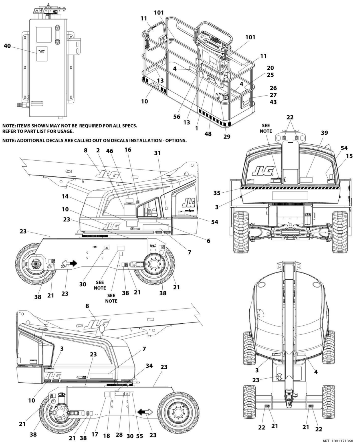
FIGURE 9-4. DECAL INSTALLATION - CE & UK CA SPEC (460SJ)
