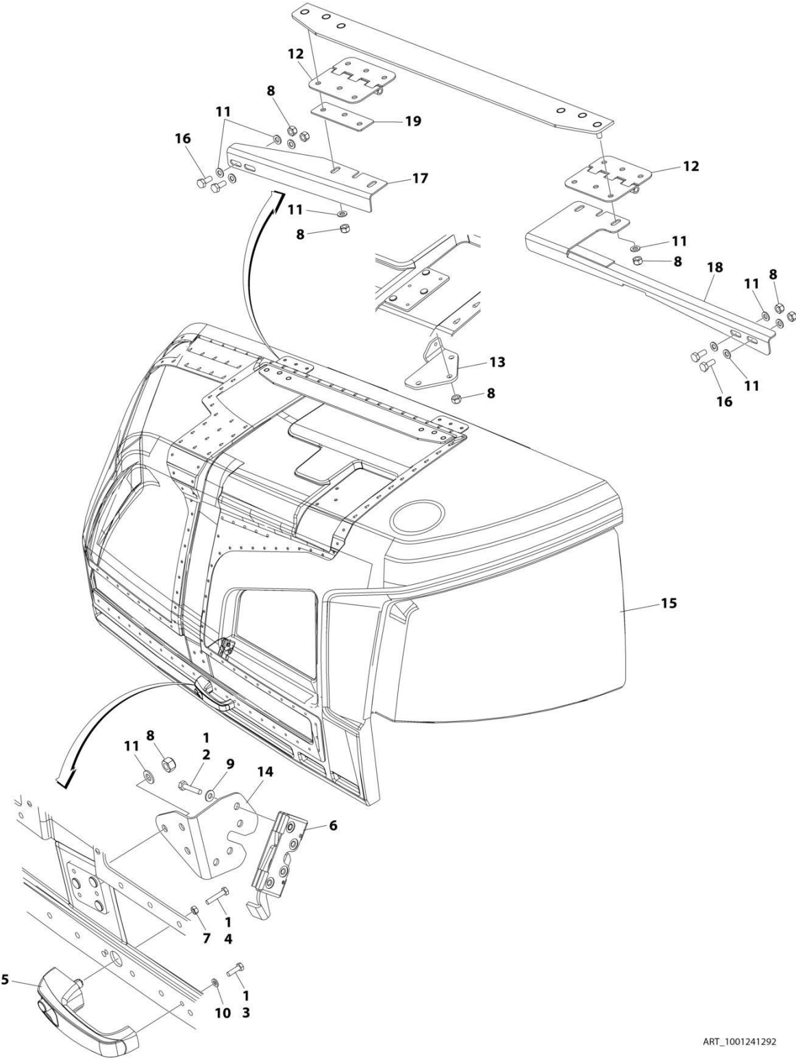
FIGURE 2-49. ABS HOOD ASSEMBLY - TANK SIDE (CE & UK CA SPEC)
