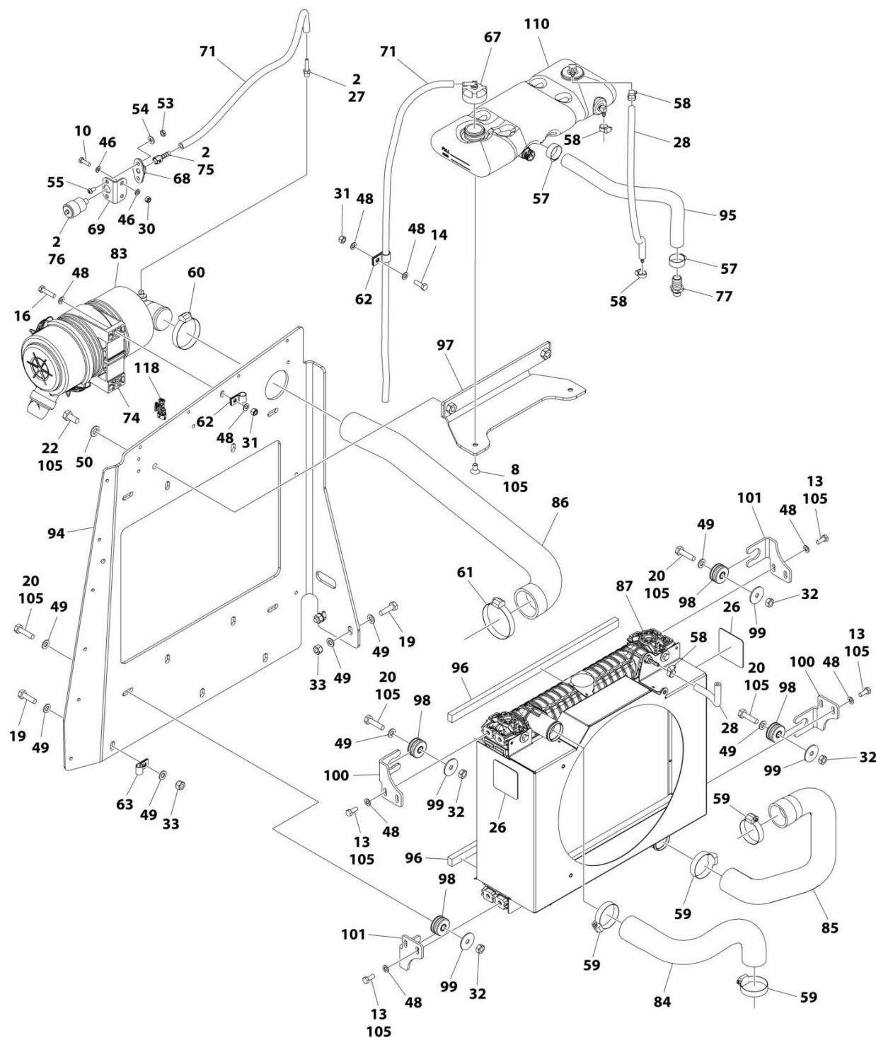
FIGURE 3-25. DEUTZ D2.9L4 ENGINE ASSEMBLY (CHINA IV)
