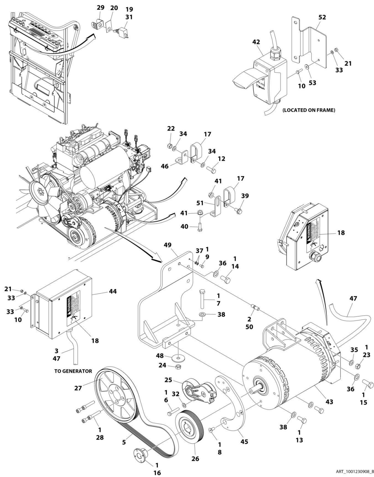
FIGURE 3-50. GENERATOR INSTALLATION - 4000W/50HZ (DEUTZ D2011 ENGINES)
