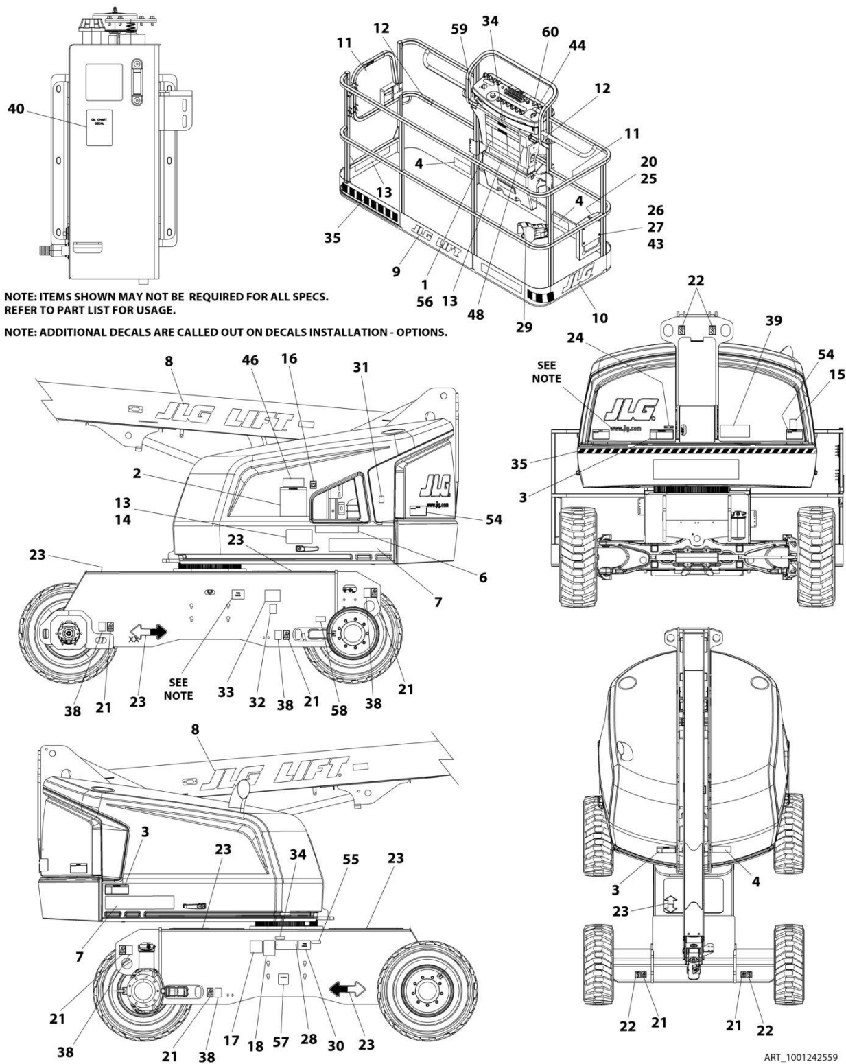
FIGURE 9-2. DECAL INSTALLATION - ANSI, ANSI EXPORT AND CSA SPECS - ENGLISH (460SJ)
