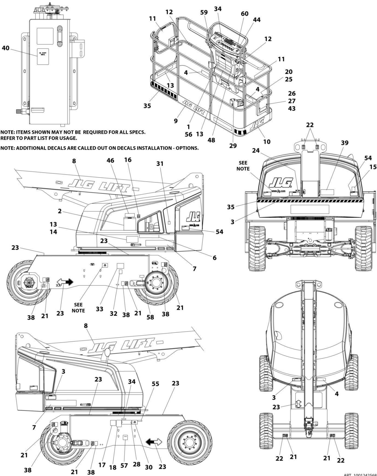
FIGURE 9-10. DECAL INSTALLATION - CSA SPEC (DUAL LANGUAGE - ENGLISH/FRENCH) (460SJ)
