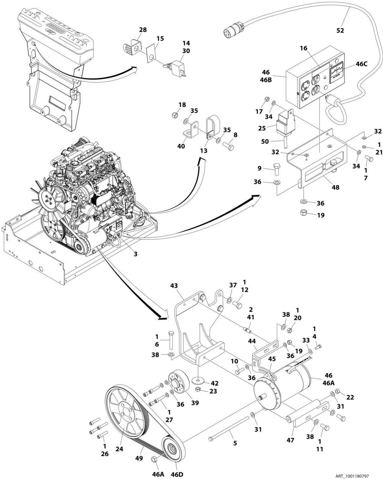
FIGURE 3-48. GENERATOR INSTALLATION - 2500W/60HZ (DEUTZ D2.9L4 ENGINE)
