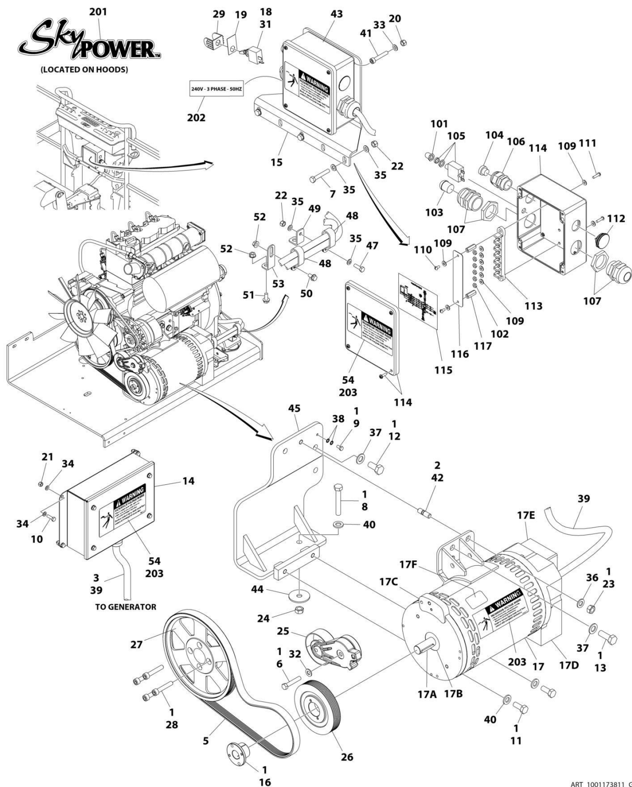
FIGURE 3-54. GENERATOR INSTALLATION - 7500W/50HZ (DEUTZ D2011 ENGINE)
