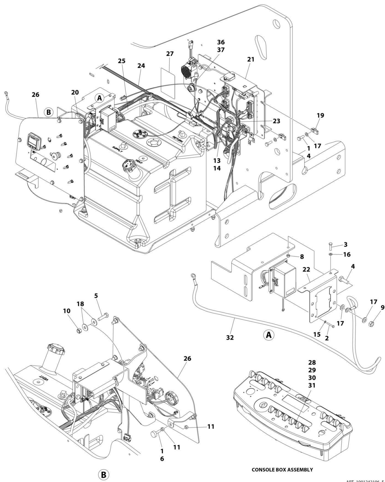
FIGURE 2-23. ELECTRICAL INSTALLATION - 460SJ
