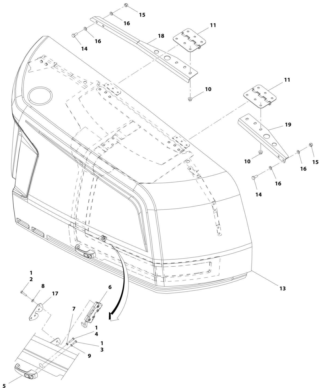
FIGURE 2-46. ABS HOOD ASSEMBLY - ENGINE SIDE
