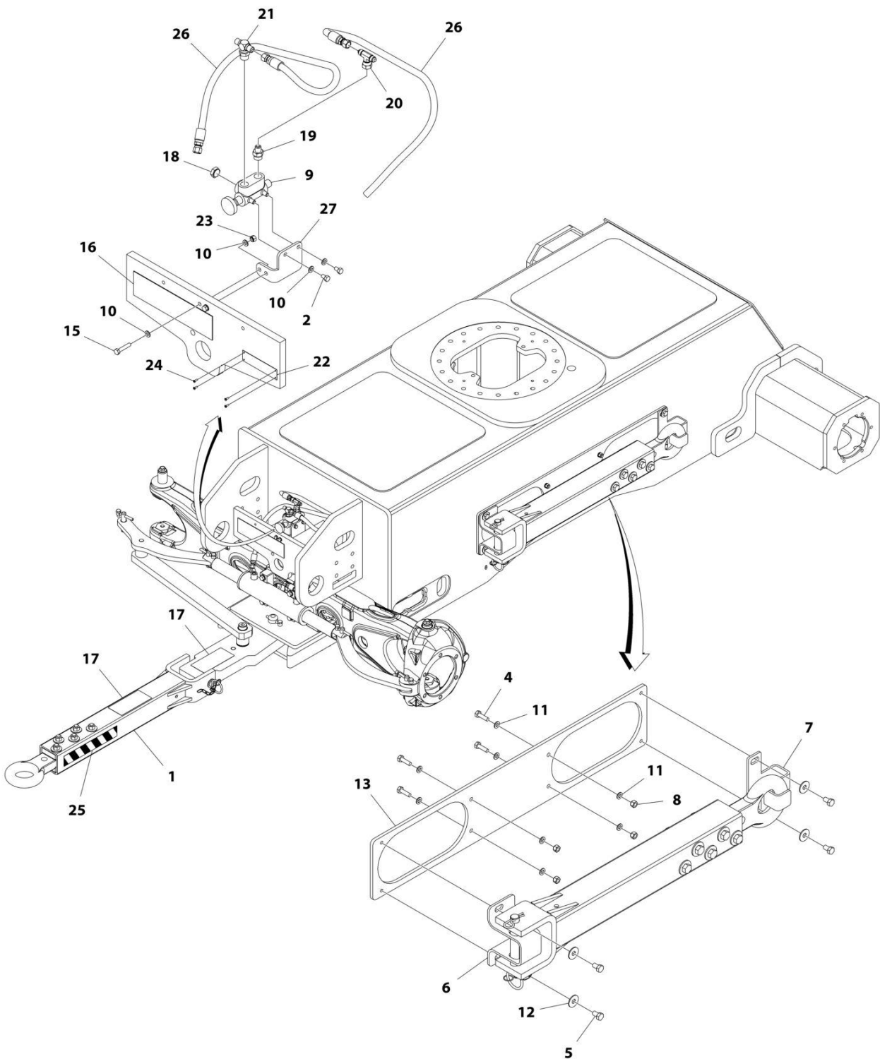
FIGURE 1-17. TOW BAR INSTALLATION
