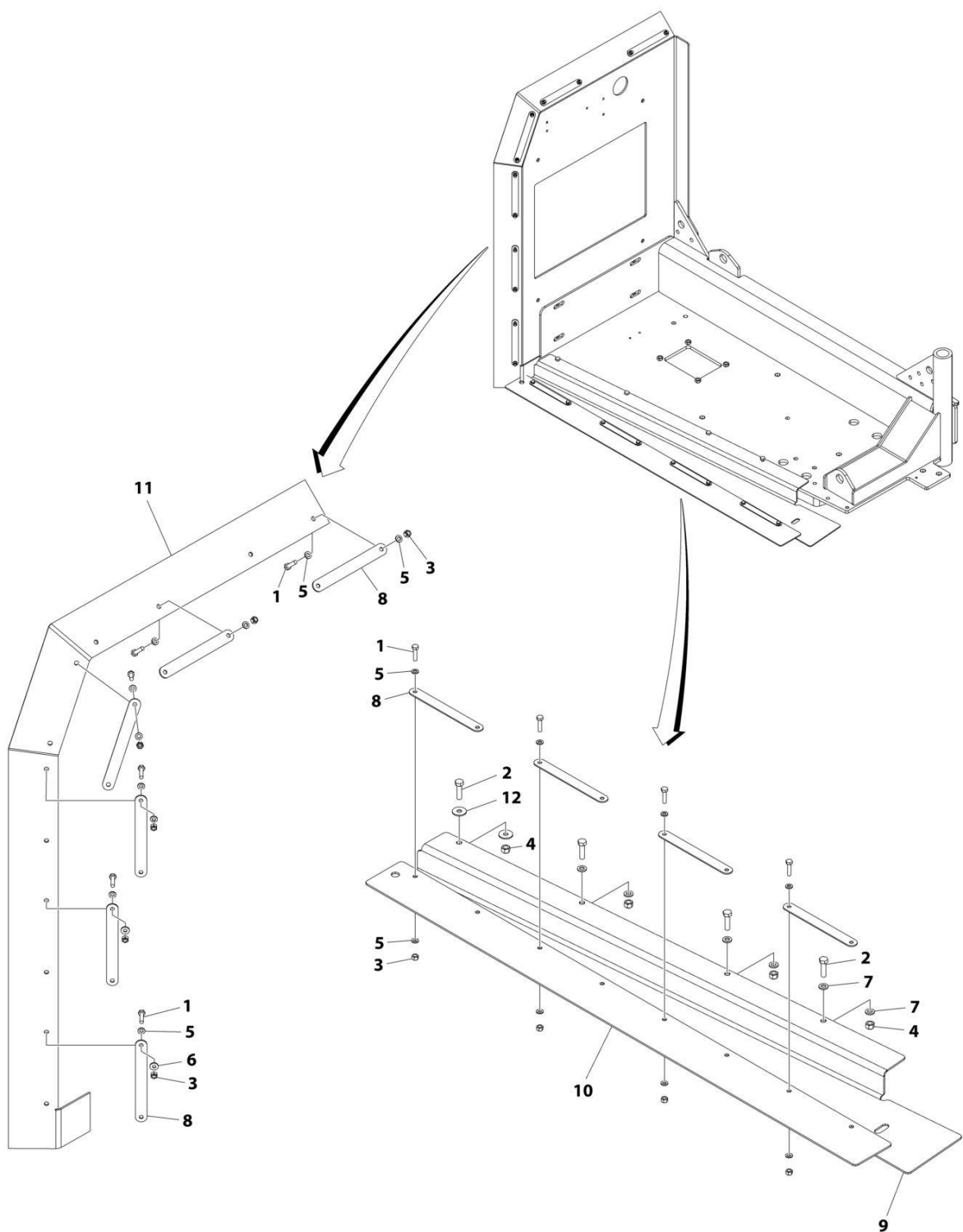
FIGURE 3-17. ENGINE HOOD Baffles INSTALLATION
