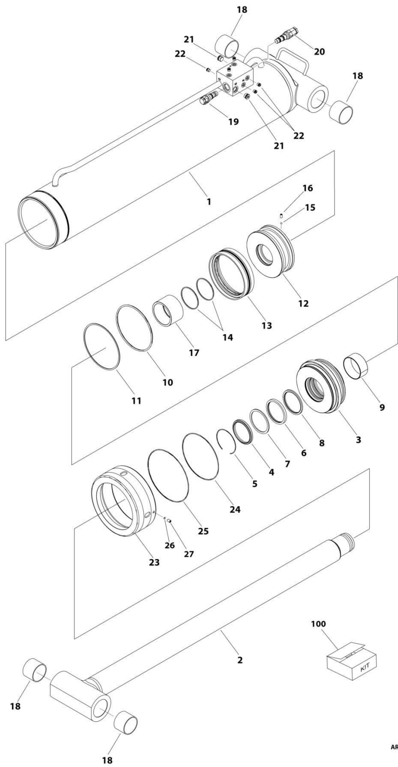
FIGURE 6-6. LEVEL (SLAVE) CYLINDER ASSEMBLY - UPRIGHT (SN 0300261402 through 0300270863)
