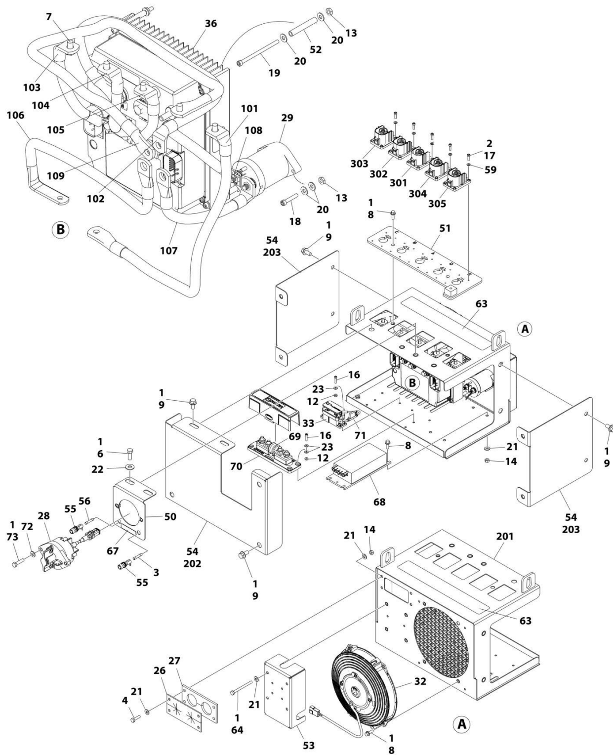
FIGURE 2-20. IMG CONTROL BOX ASSEMBLY
