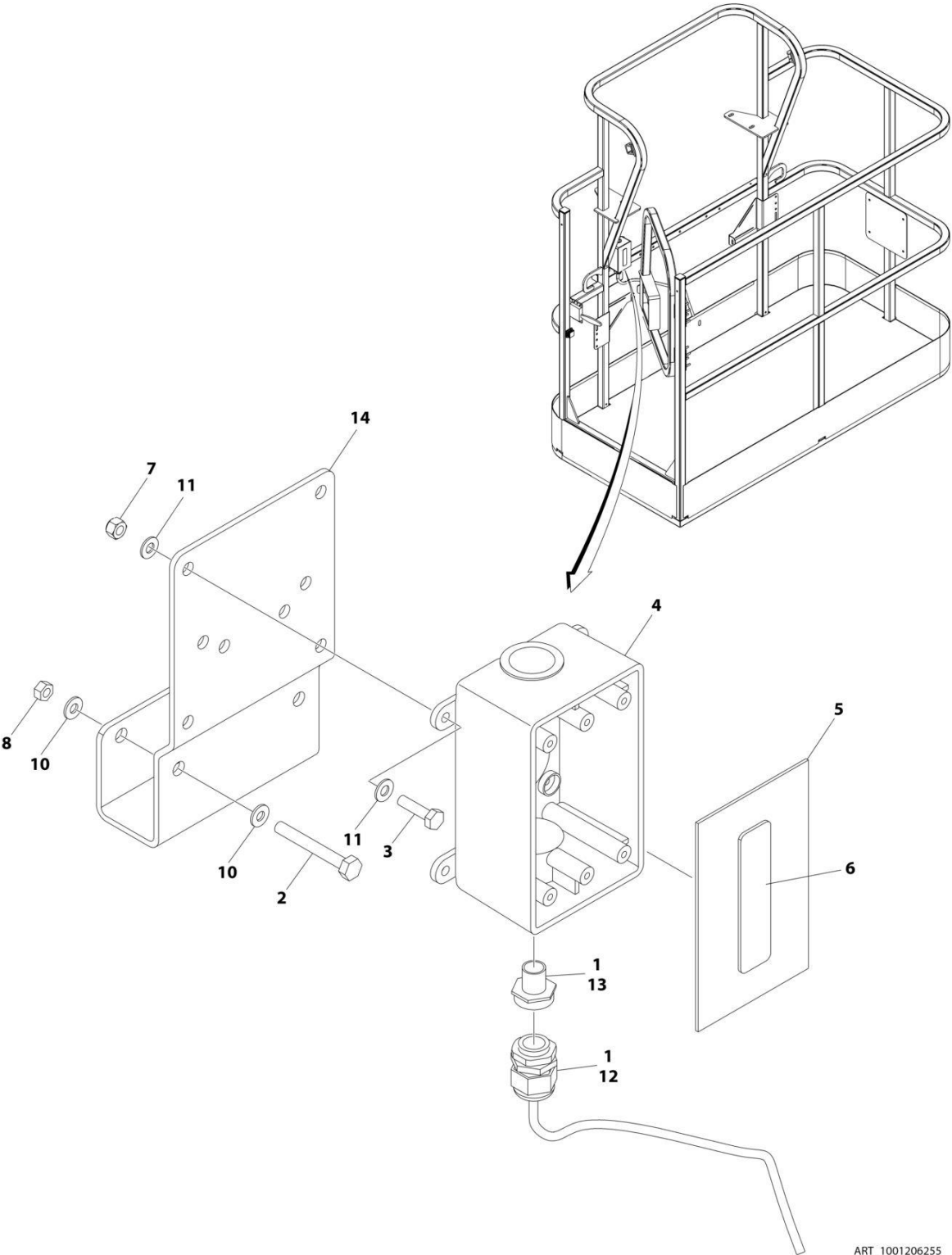
FIGURE 8-14. AC BOX AT PLATFORM INSTALLATION - BOX WITH COVER (ANSI EXPORT, AUSTRALIAN, CHINA & JAPANESE SPECS)
