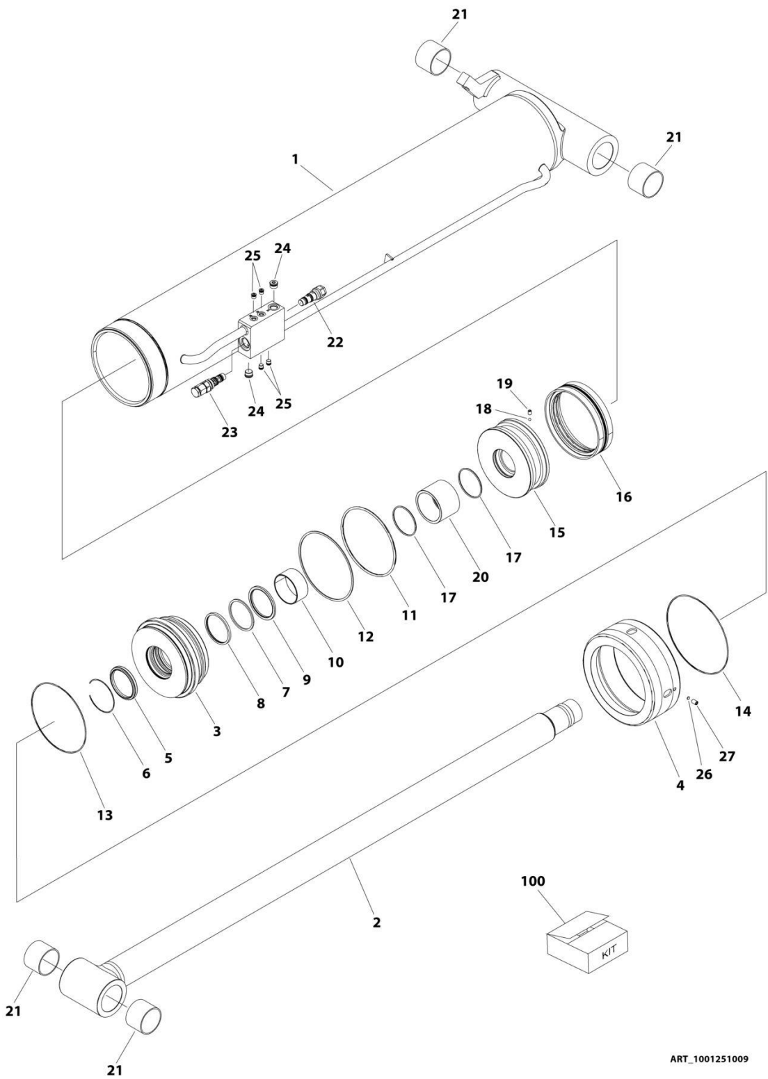
FIGURE 6-14. LIFT CYLINDER ASSEMBLY - TOWER BOOM (SN 0300261402 through 0300270863)
