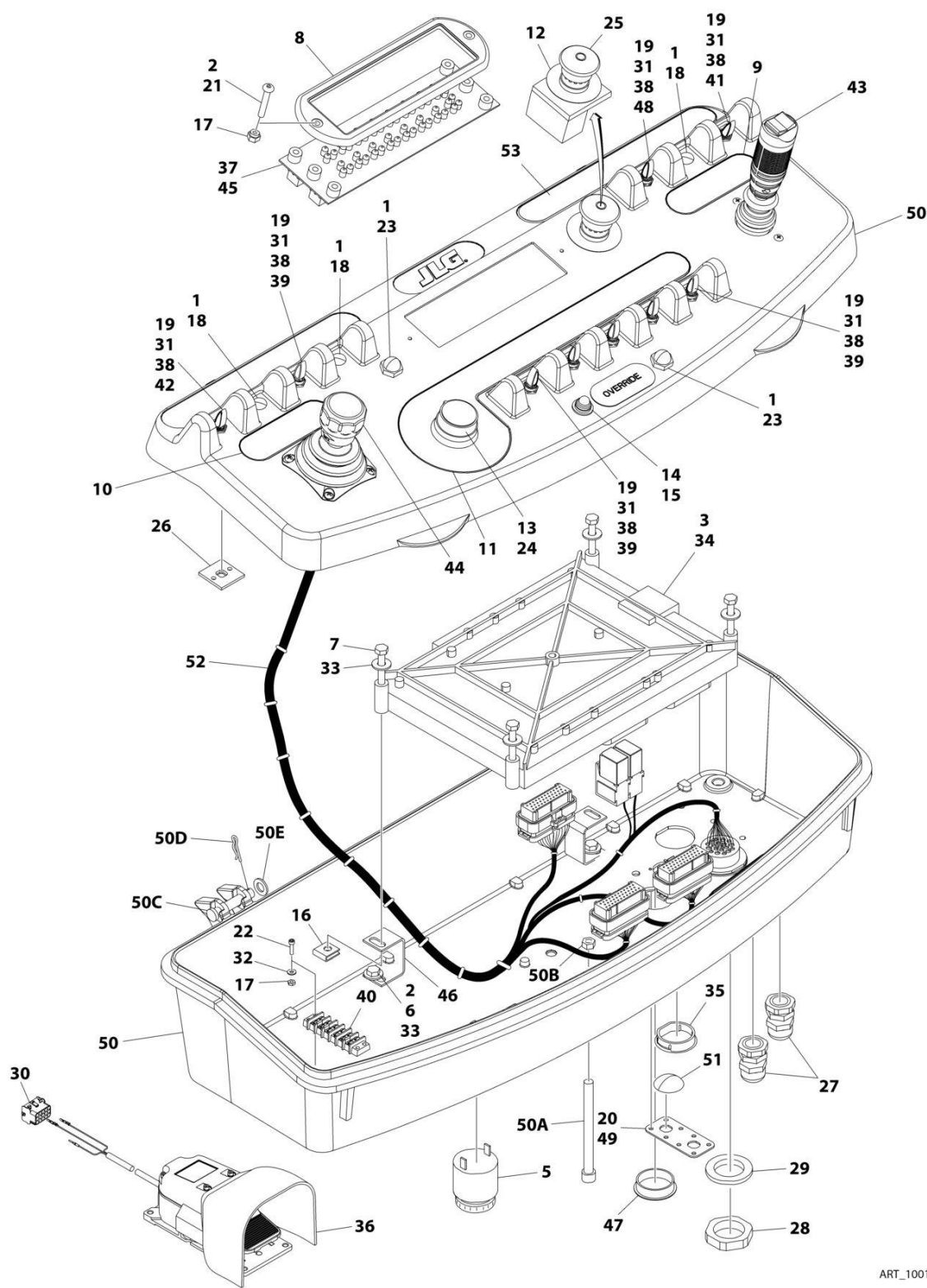
FIGURE 5-15. CONSOLE BOX ASSEMBLY (SN 0300259698 through 0300270863)
