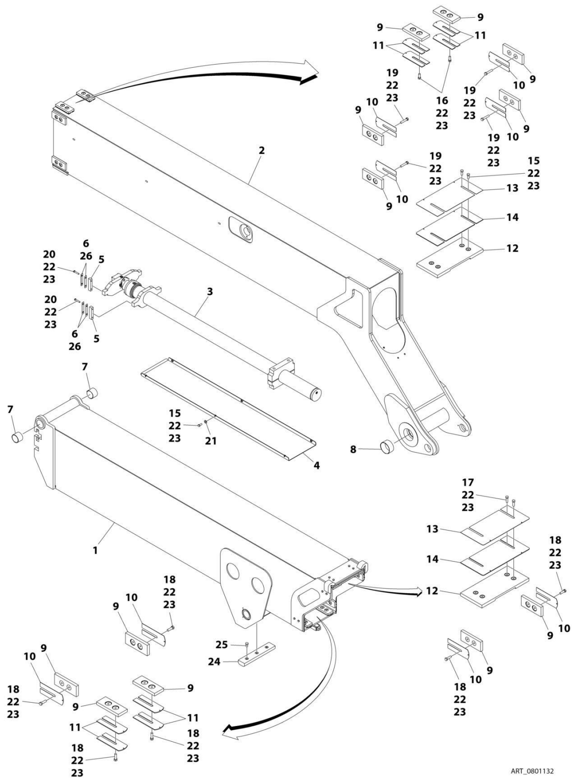
FIGURE 4-5. TOWER BOOM ASSEMBLY
