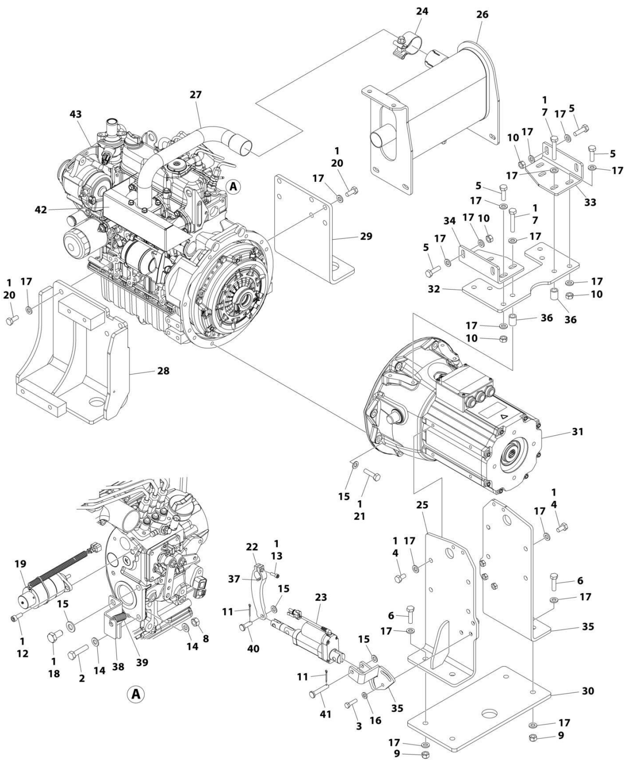
FIGURE 3-7. ENGINE AND GENERATOR ASSEMBLY (SN 0300259343 through 0300270863)
