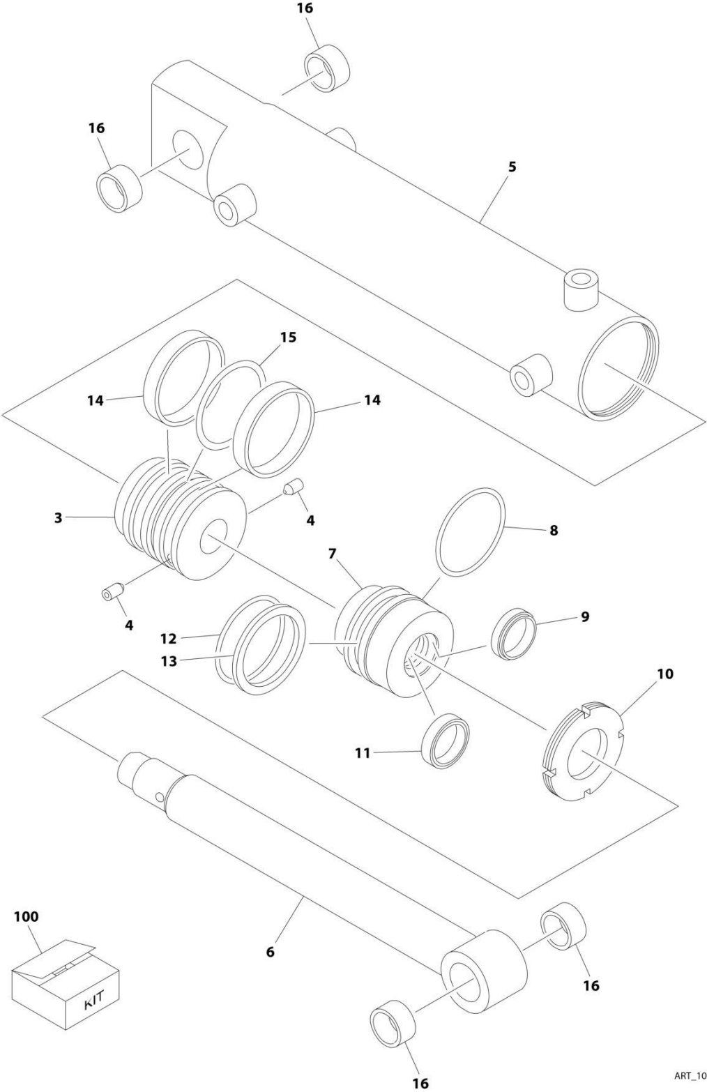
FIGURE 6-17. STEER CYLINDER ASSEMBLY
