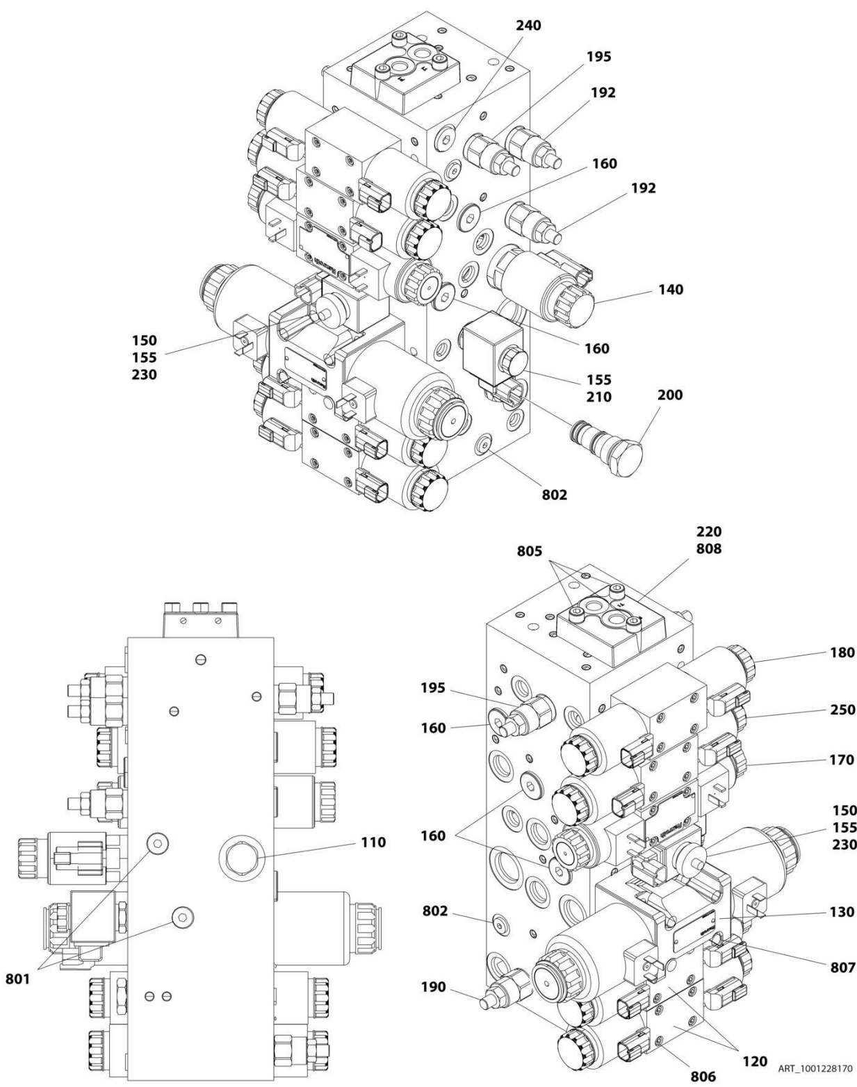
FIGURE 2-4. MAIN VALVE ASSEMBLY (SN 0300247156 through 0300270863)
