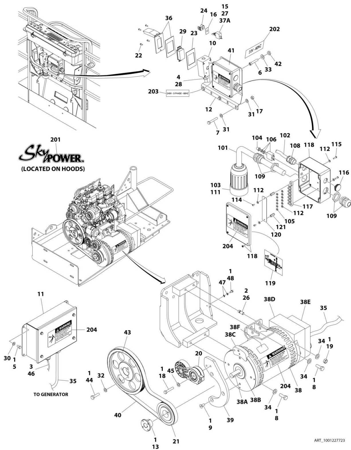
FIGURE 3-21. 7500W SKYPOWER GENERATOR INSTALLATION - 110V/60HZ (OPTIONAL)
