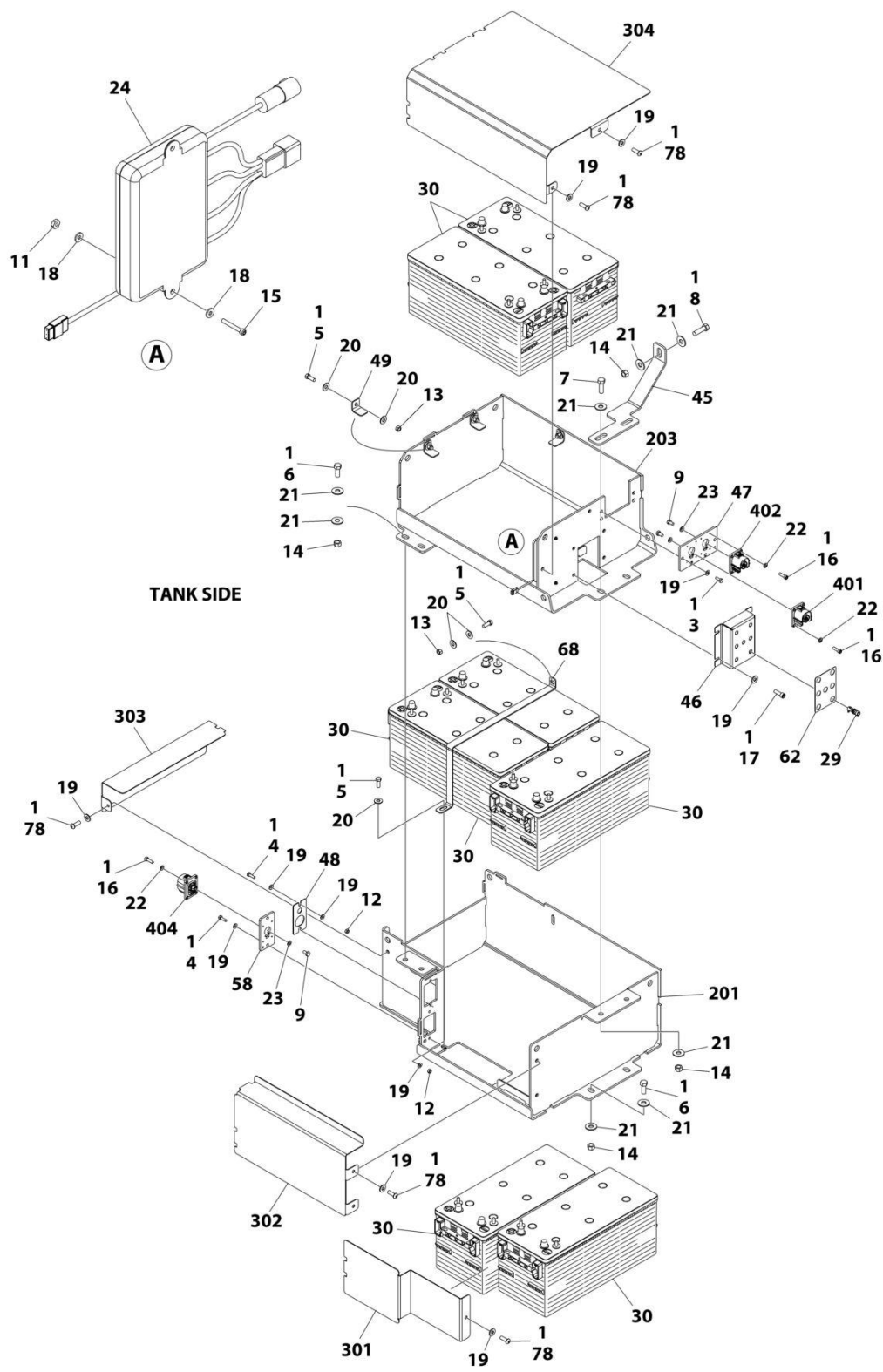
FIGURE 2-16. BATTERY BOXES INSTALLATION
