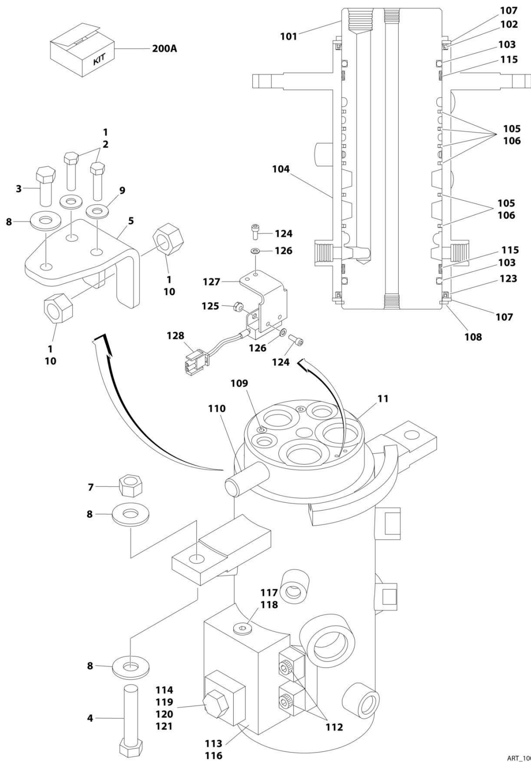
FIGURE 2-11. ROTARY COUPLING INSTALLATION
