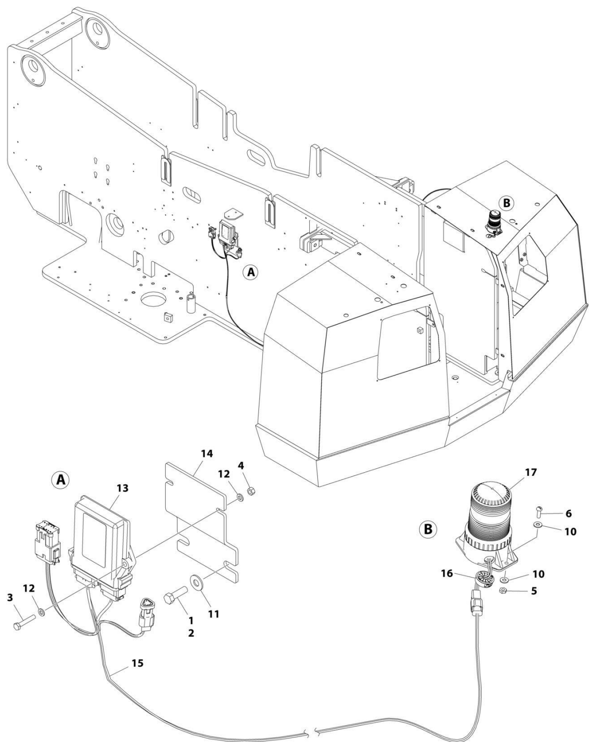
FIGURE 2-30. STROBE LIGHT INSTALLATION - RED (OPTIONAL) (SN 0300259698 through 0300270863)
