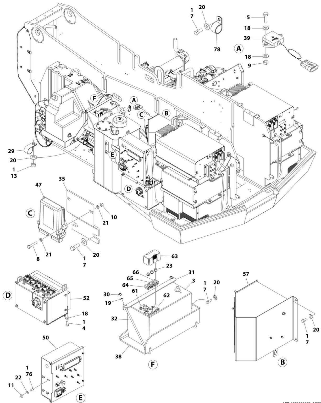
FIGURE 2-19. ELECTRICAL SYSTEM INSTALLATION
