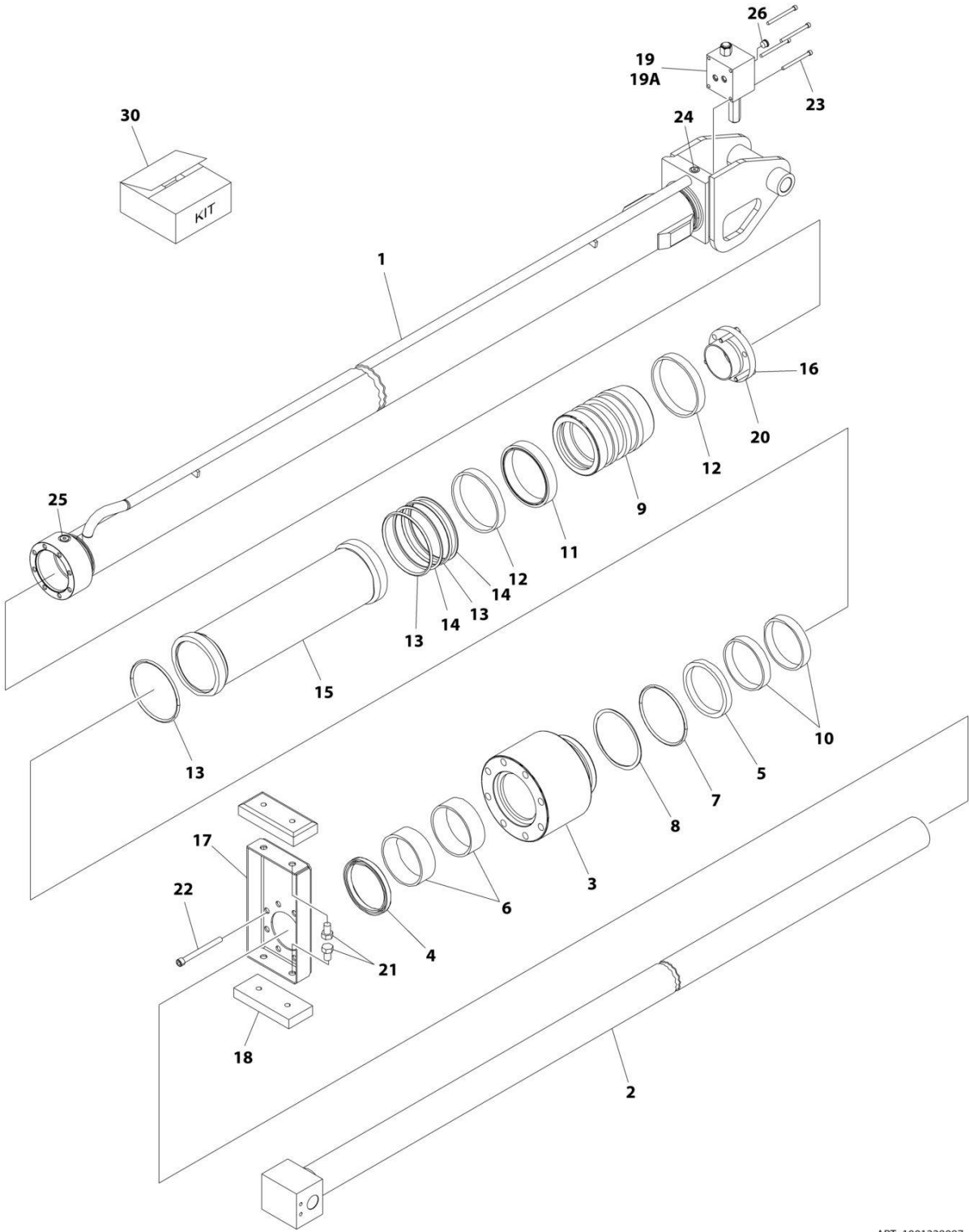
FIGURE 6-19. TELESCOPE CYLINDER ASSEMBLY - MAIN BOOM (SN 0300247156 through 0300270863)
