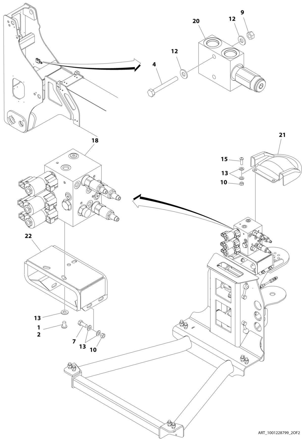
FIGURE 4-10. BOOM VALVES INSTALLATION - WITH LSS
