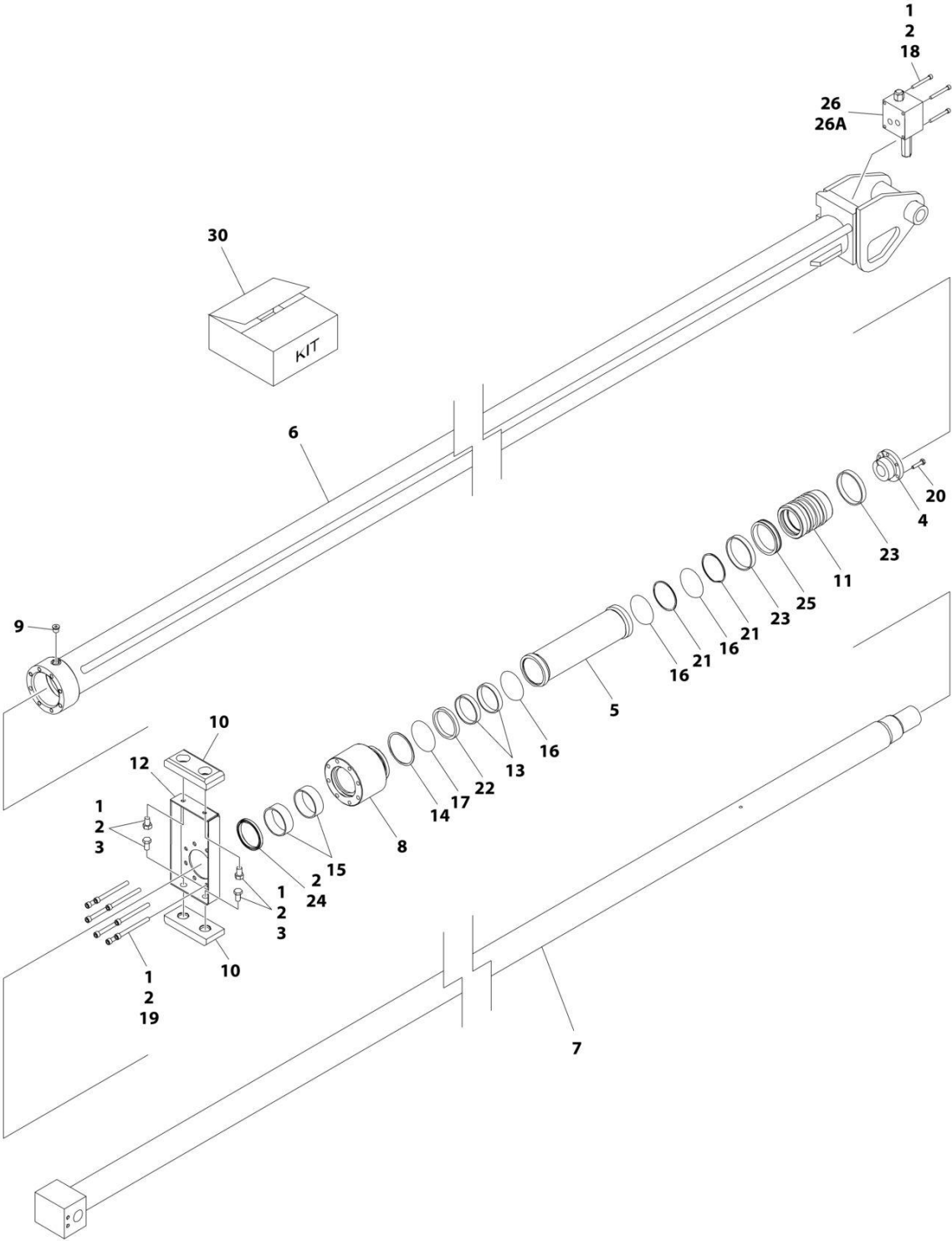
FIGURE 6-18. TELESCOPE CYLINDER ASSEMBLY - MAIN BOOM (Prior to SN 0300247156)
