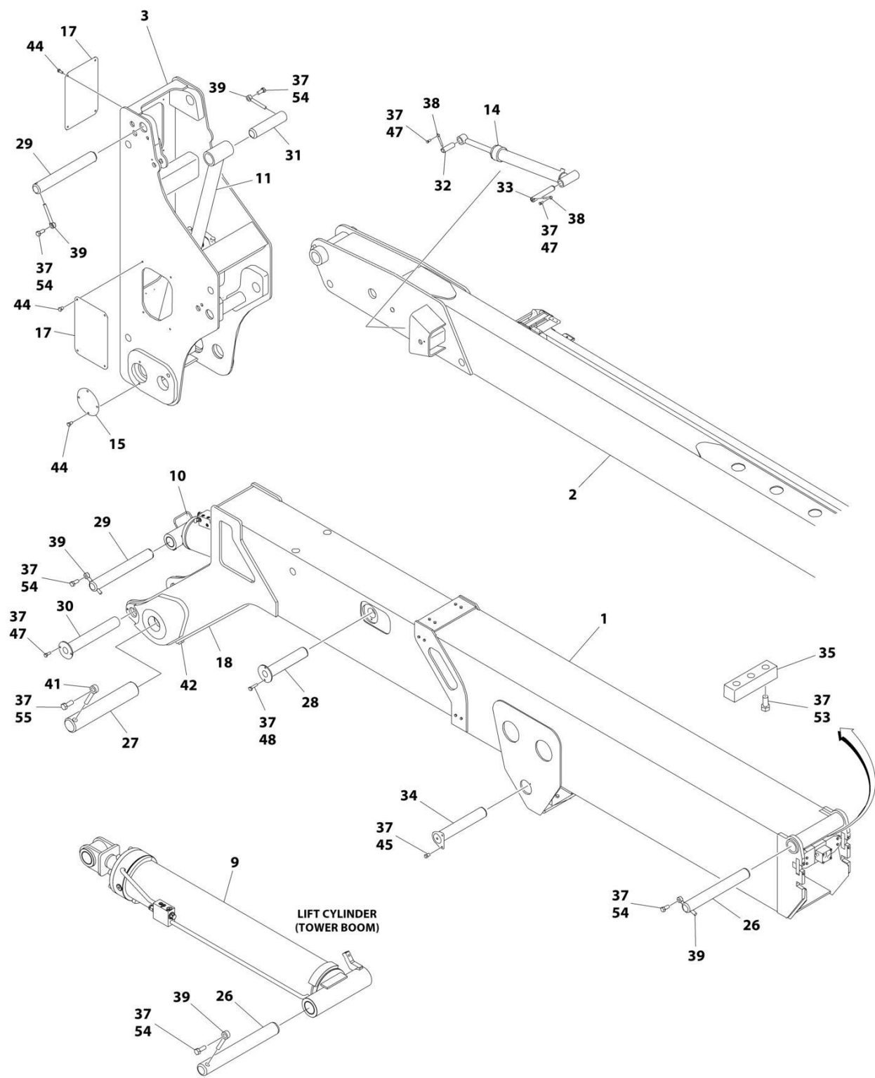
FIGURE 4-1. BOOM AND CYLINDER INSTALLATION (Prior to SN 0300261401)
