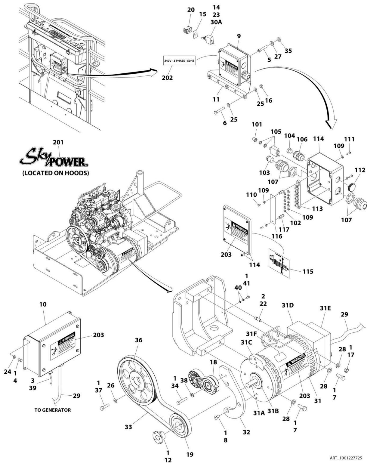
FIGURE 3-20. 7500W SKYPOWER GENERATOR INSTALLATION - 220V/50HZ (OPTIONAL)
