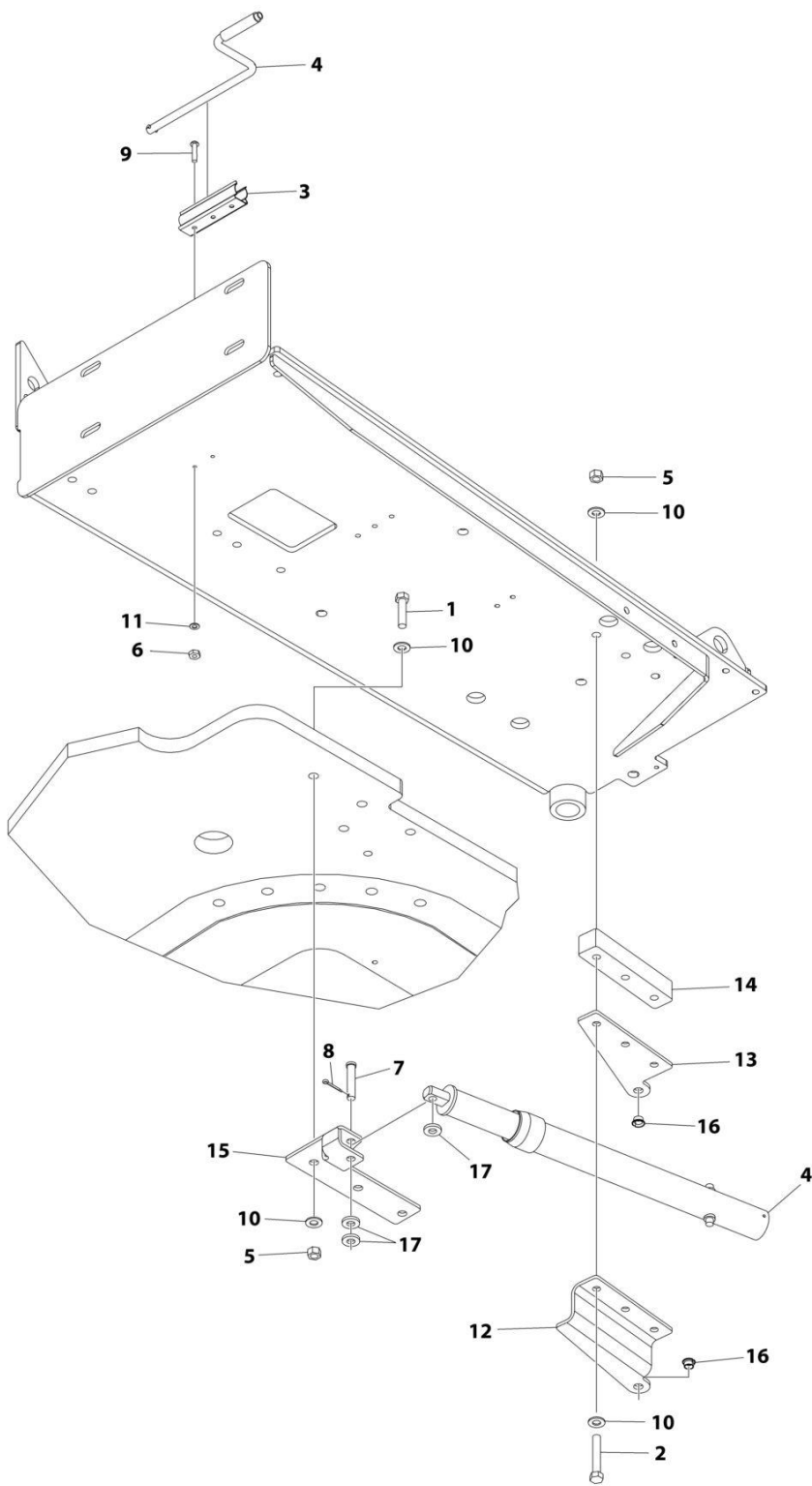
FIGURE 3-18. TRAY JACK INSTALLATION
