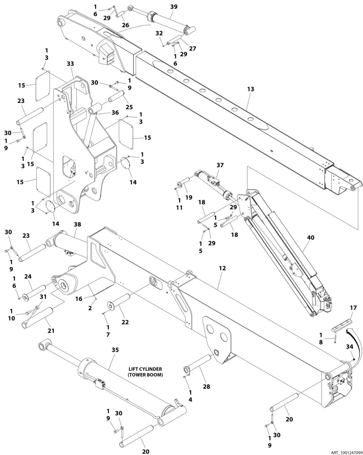
FIGURE 4-2. BOOM AND CYLINDER INSTALLATION (SN 0300261401 through 0300270863)
