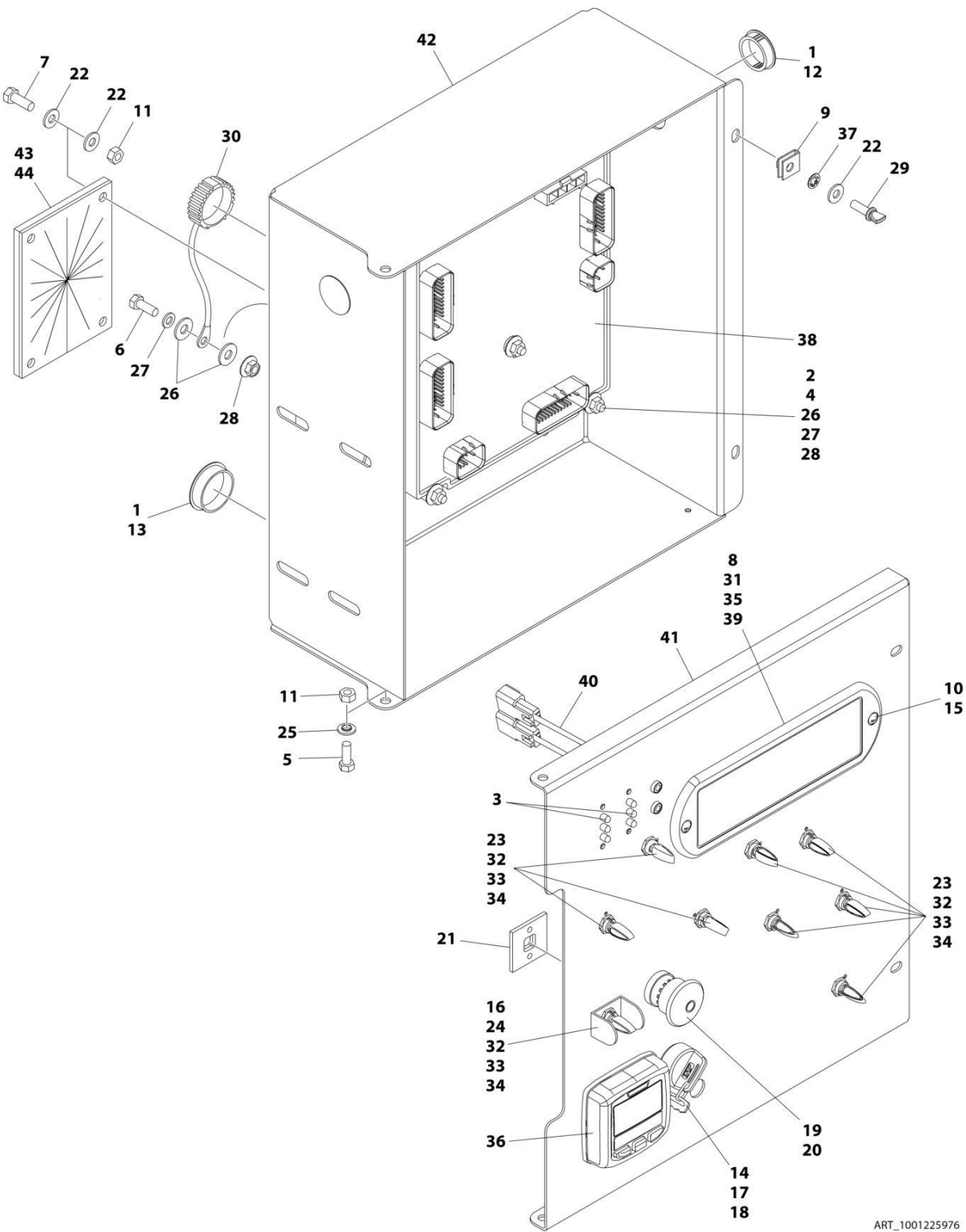
FIGURE 2-22. GROUND CONTROL BOX ASSEMBLY
