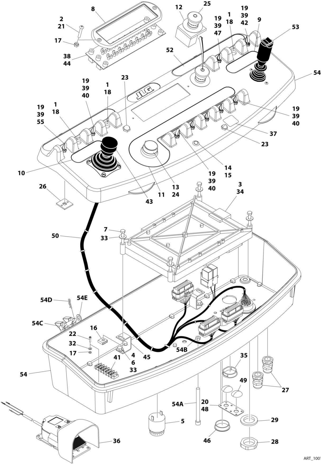
FIGURE 5-14. CONSOLE BOX ASSEMBLY (Prior to SN 0300259698)
