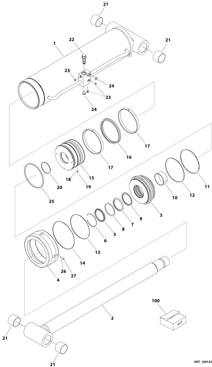
FIGURE 6-11. LIFT CYLINDER ASSEMBLY - MAIN BOOM (SN 0300261402 through 0300270863)
