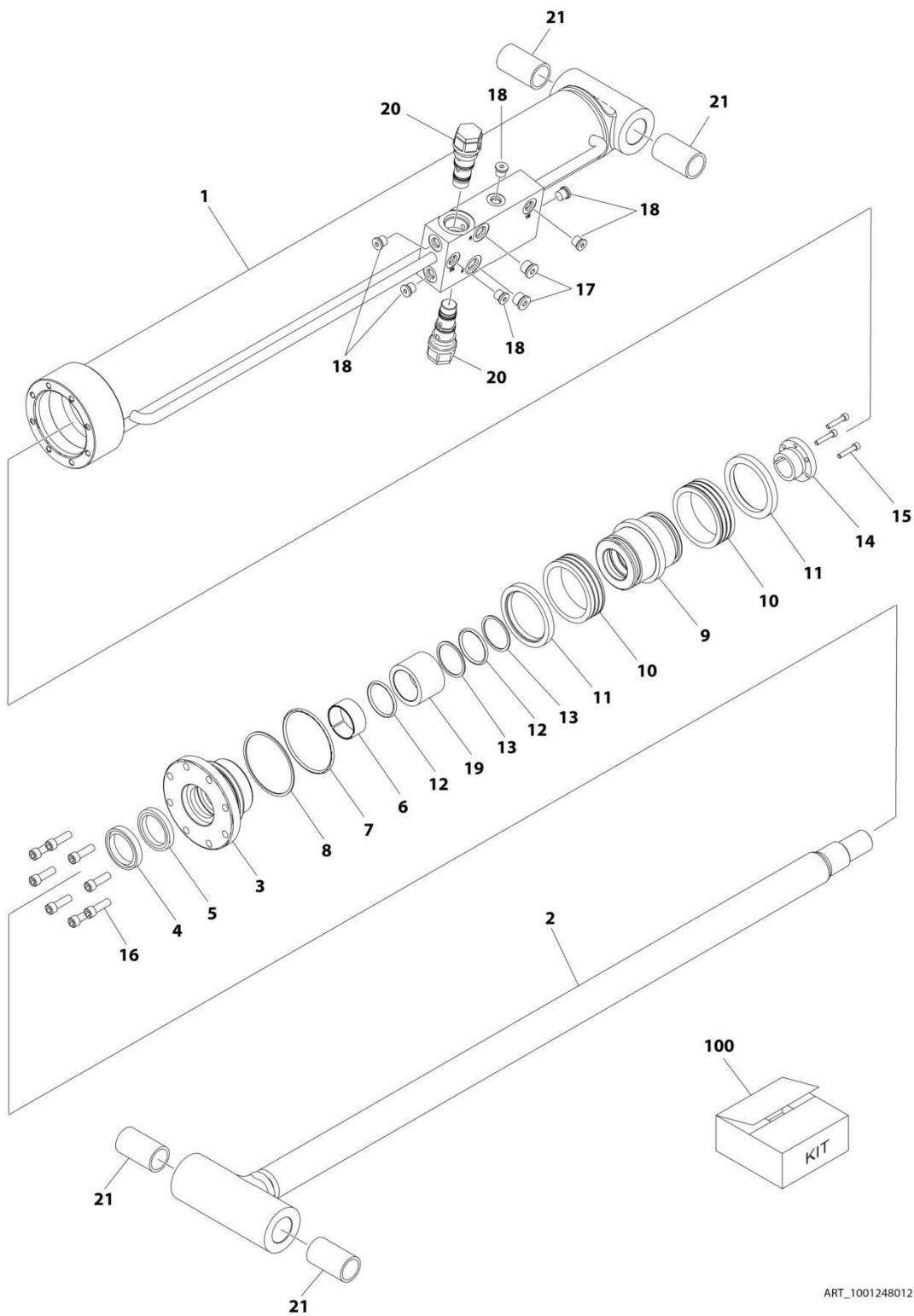
FIGURE 6-8. LIFT CYLINDER ASSEMBLY - JIB (SN 0300247156 through 0300270863)
