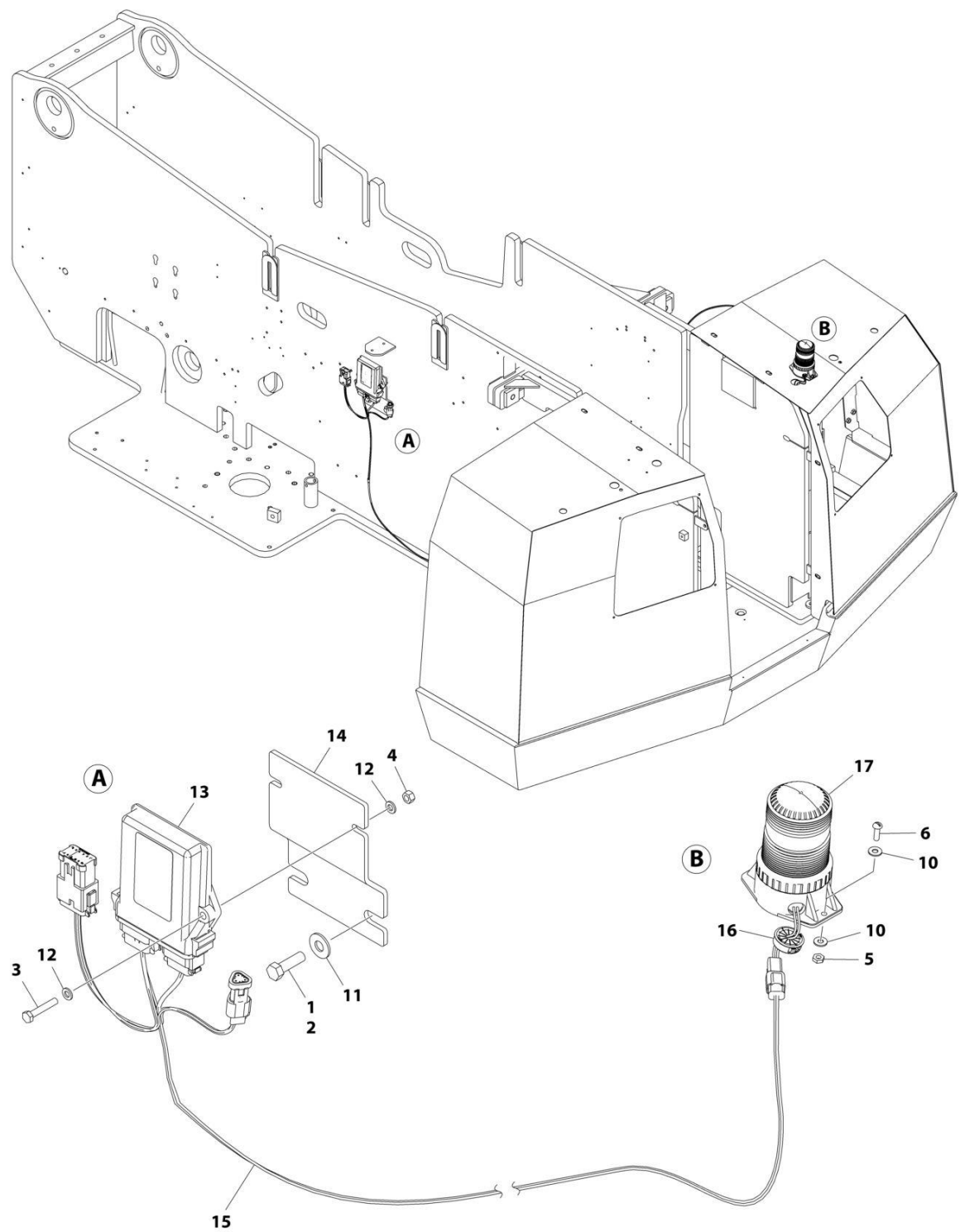
FIGURE 2-28. STROBE LIGHT INSTALLATION - BLUE (OPTIONAL) (SN 0300259698 through 0300270863)
