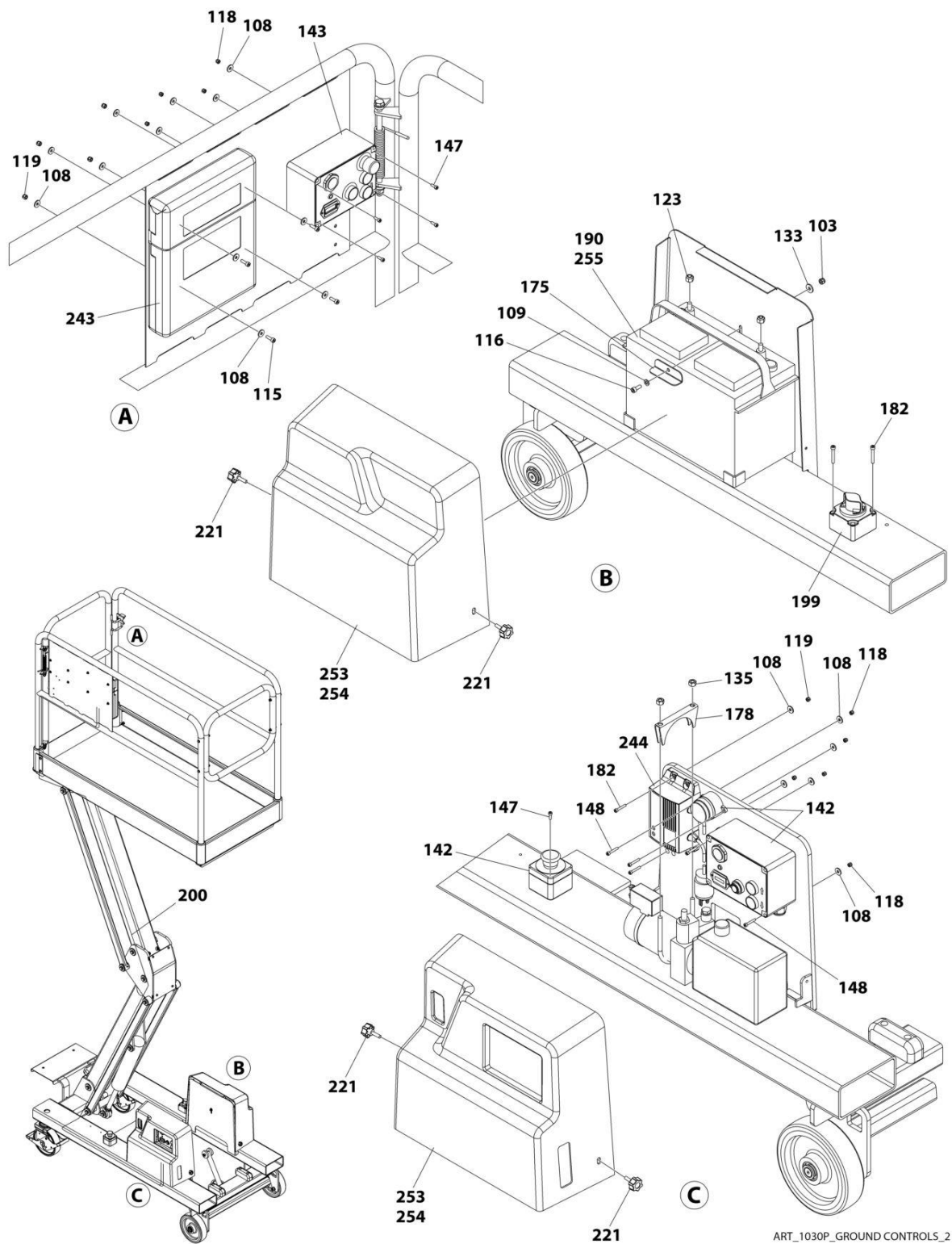
FIGURE 2-6. GROUND CONTROLS INSTALLATION
