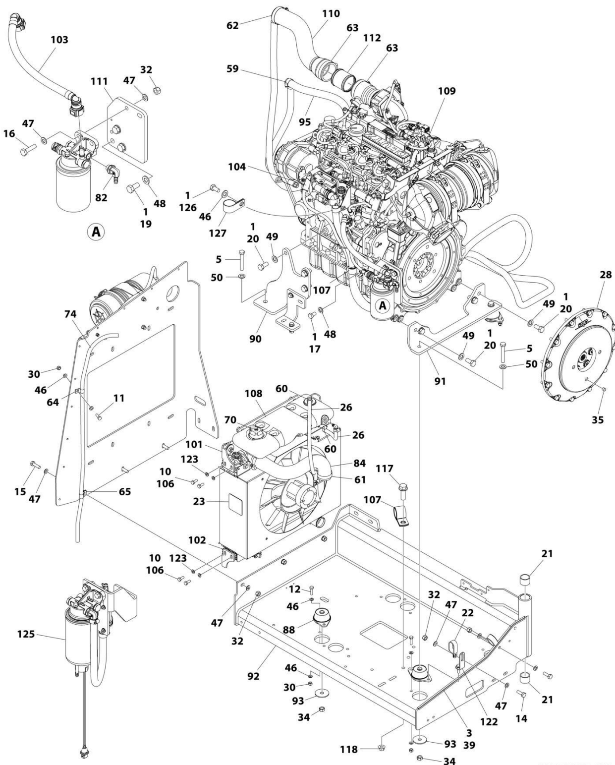
FIGURE 3-17. ENGINE ASSEMBLY - DEUTZ D2.9L4 (STAGE V) ENGINE (WITHOUT ARCTIC PACKAGE) (CE SPECS)
