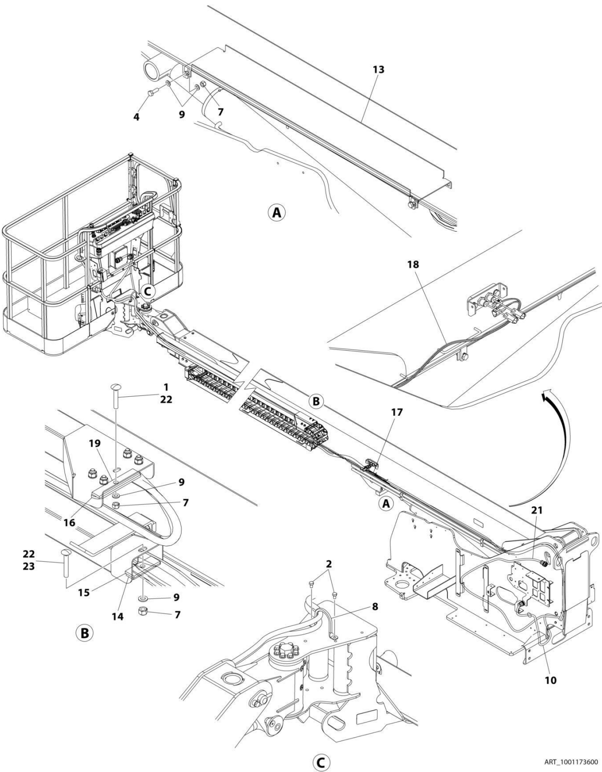
FIGURE 8-29. CABLES AND CLAMPS INSTALLATION - 400SC WITH 7500W GENERATOR
