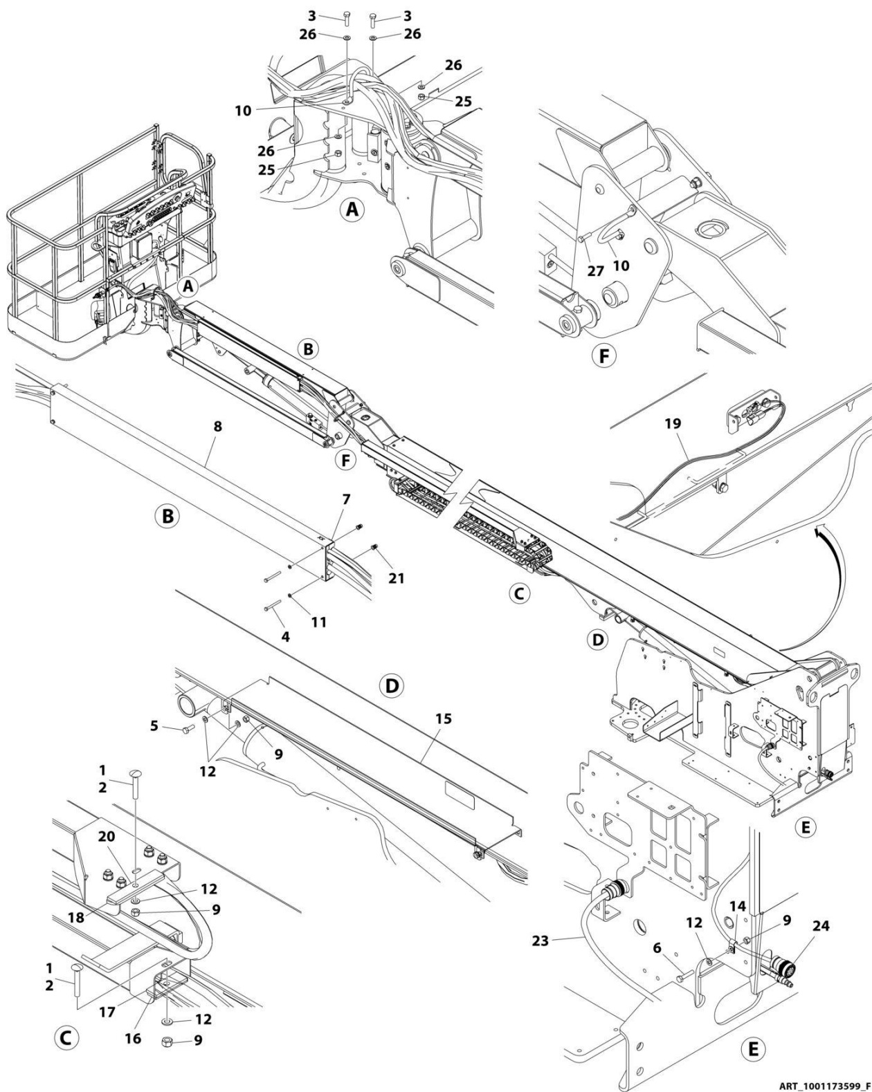
FIGURE 8-31. CABLES AND CLAMPS INSTALLATION - 460SJC WITH 4000W GENERATOR 50HZ
