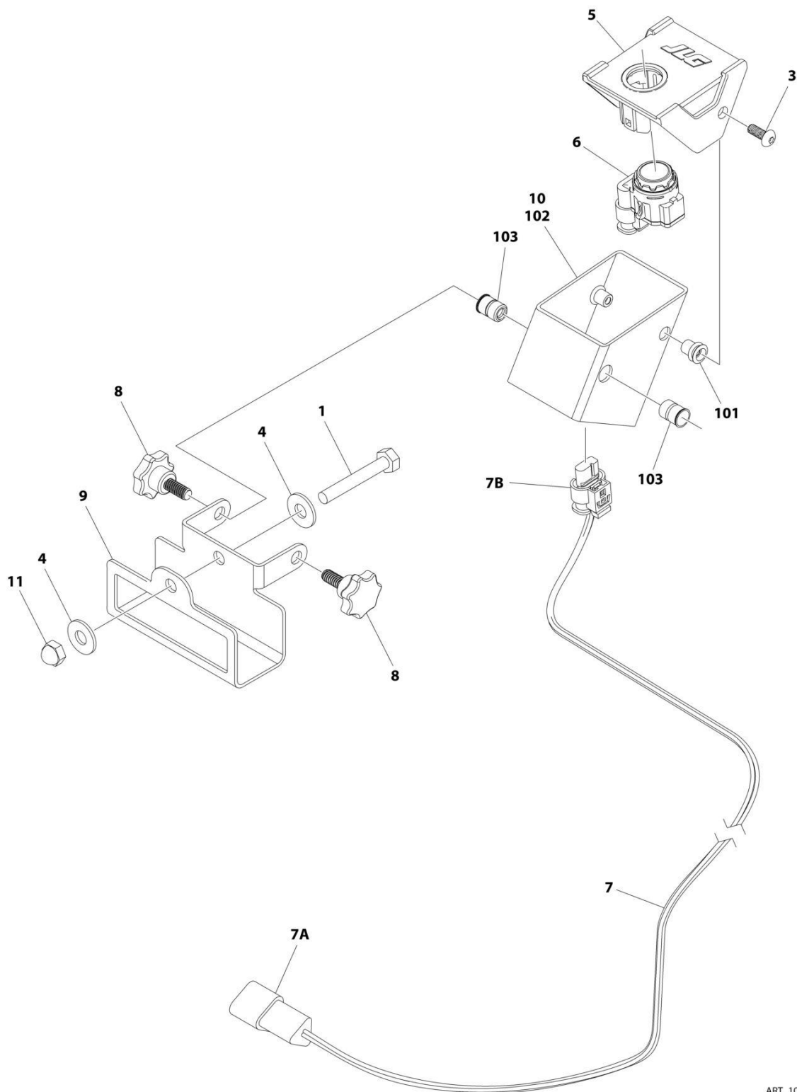
FIGURE 5-31. SKYSENSE OVERHEAD SENSOR ASSEMBLY
