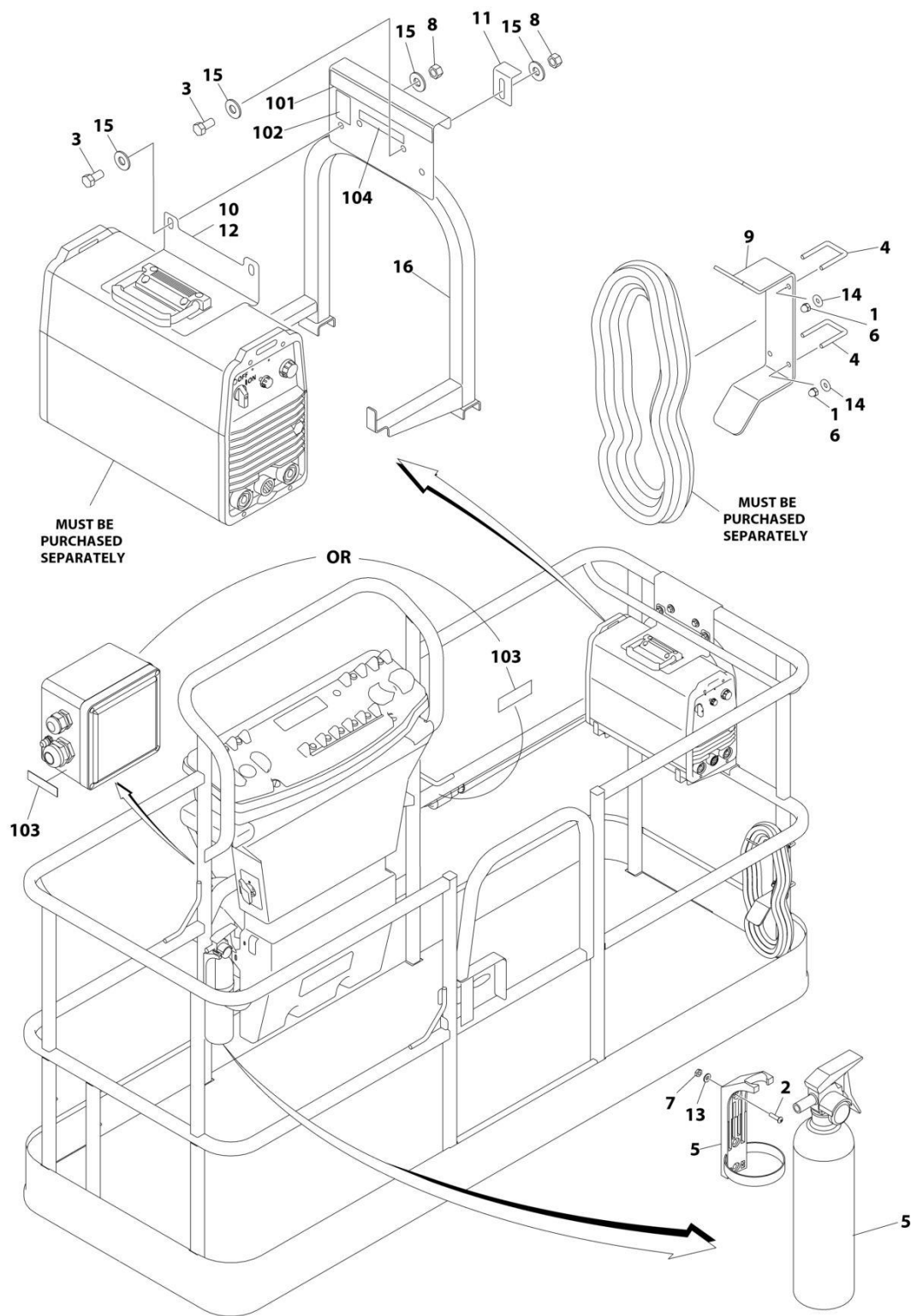
FIGURE 5-26. SKYWELDER PREP PACKAGE (60HZ) (ANSI, ANSI EXPORT, CSA AND JAPAN SPECS)
