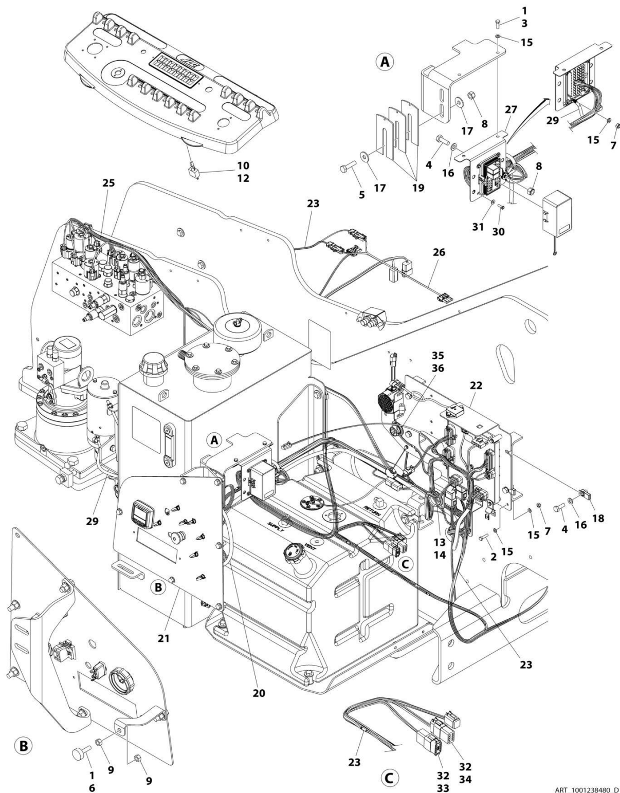
FIGURE 2-8. ELECTRICAL INSTALLATION - 460SJC
