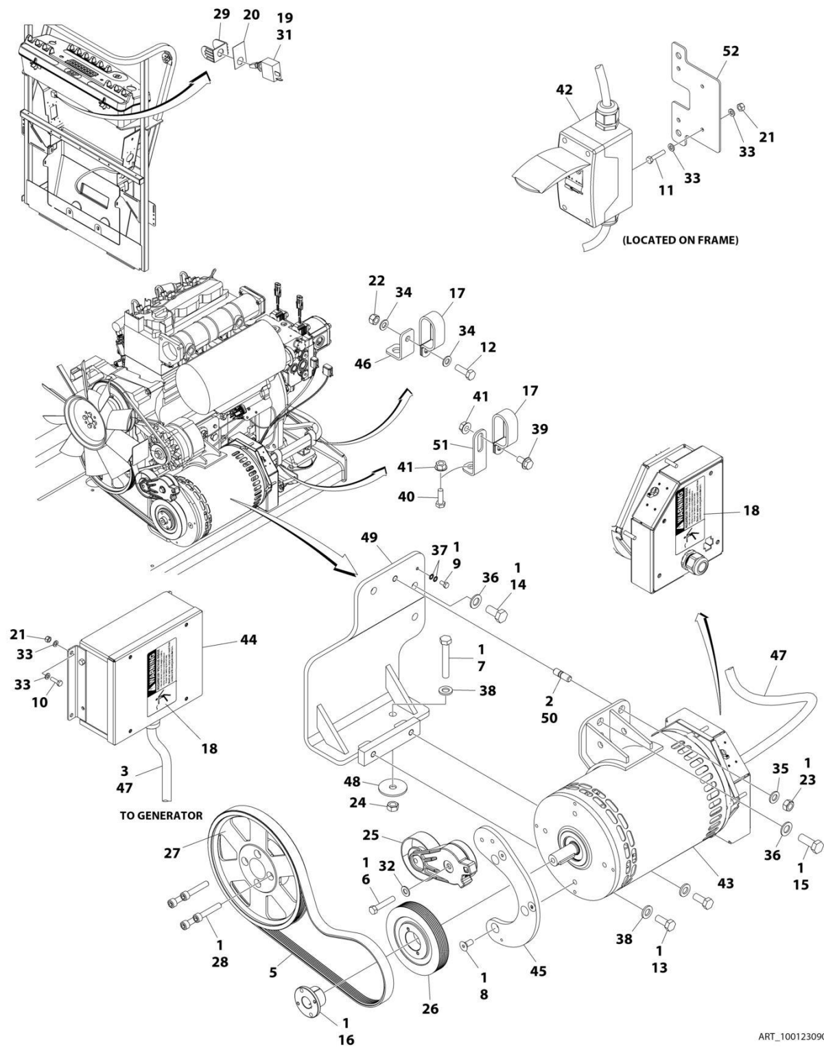
FIGURE 3-34. GENERATOR INSTALLATION - 4000W/50HZ (DEUTZ D2011 ENGINE) (ANSI EXPORT AND CE(LRC) SPECS)
