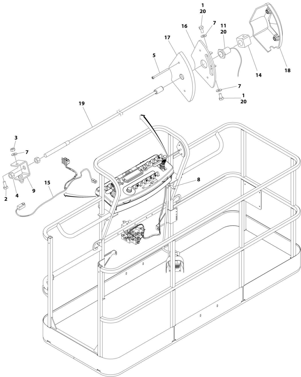
FIGURE 5-29. SKYLINE INSTALLATION
