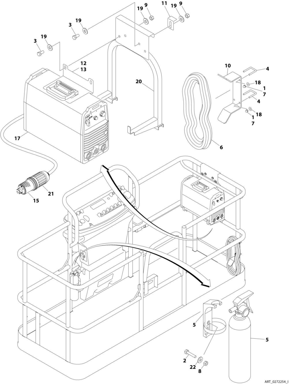
FIGURE 5-25. SKYWELDER INSTALLATION (60HZ) (ANSI, ANSI EXPORT, CSA AND JAPAN SPECS)
