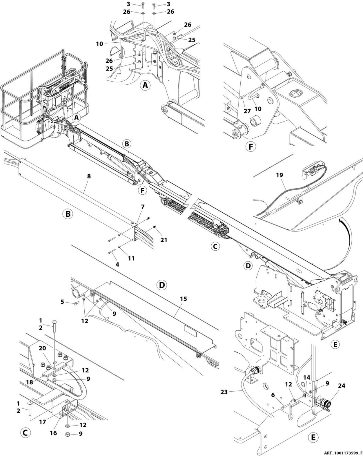
FIGURE 8-30. CABLES AND CLAMPS INSTALLATION - 460SJC WITHOUT GENERATOR
