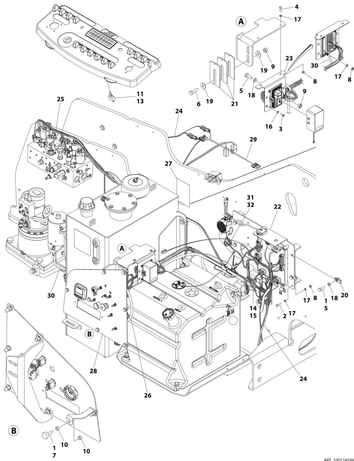
FIGURE 2-9. ELECTRICAL INSTALLATION - 460SJC WITH DEUTZ (STAGE V) ENGINE
