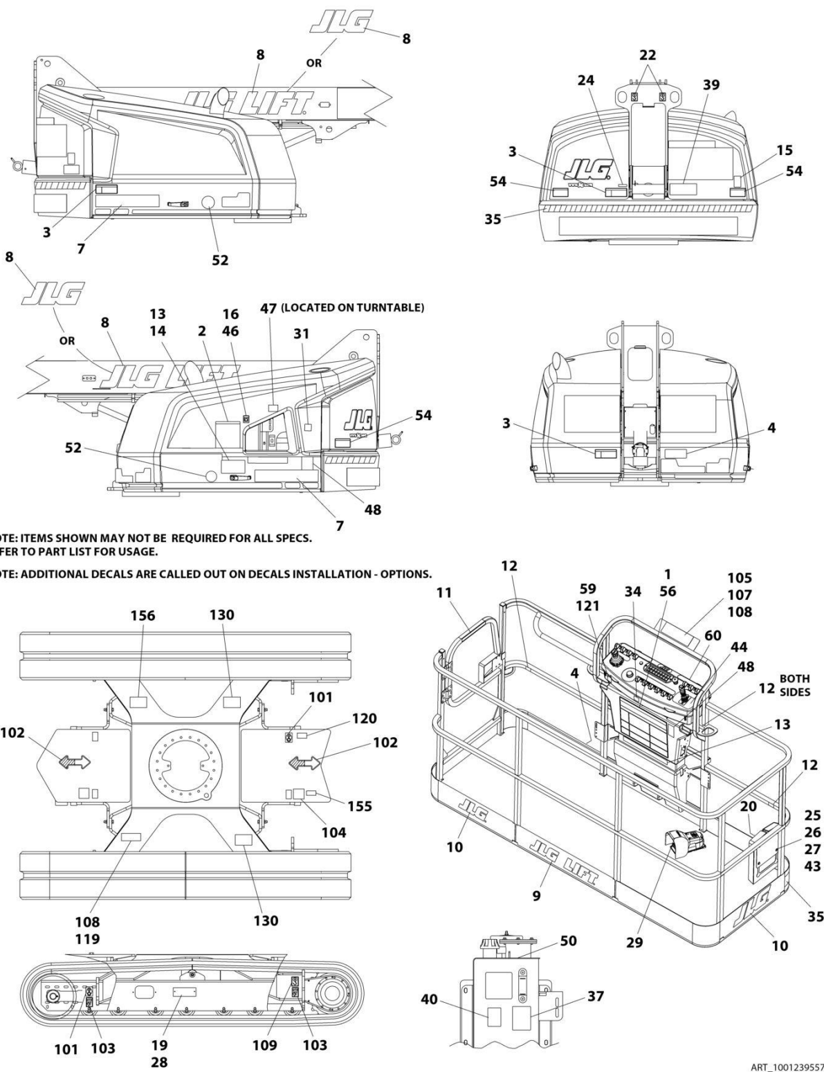
FIGURE 9-1. DECAL INSTALLATION - ANSI AND ANSI EXPORT SPECS - 400SC
