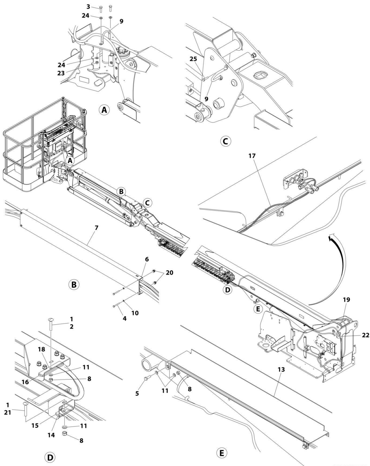
FIGURE 8-33. CABLES AND CLAMPS INSTALLATION - 460SJC WITH 7500W GENERATOR
