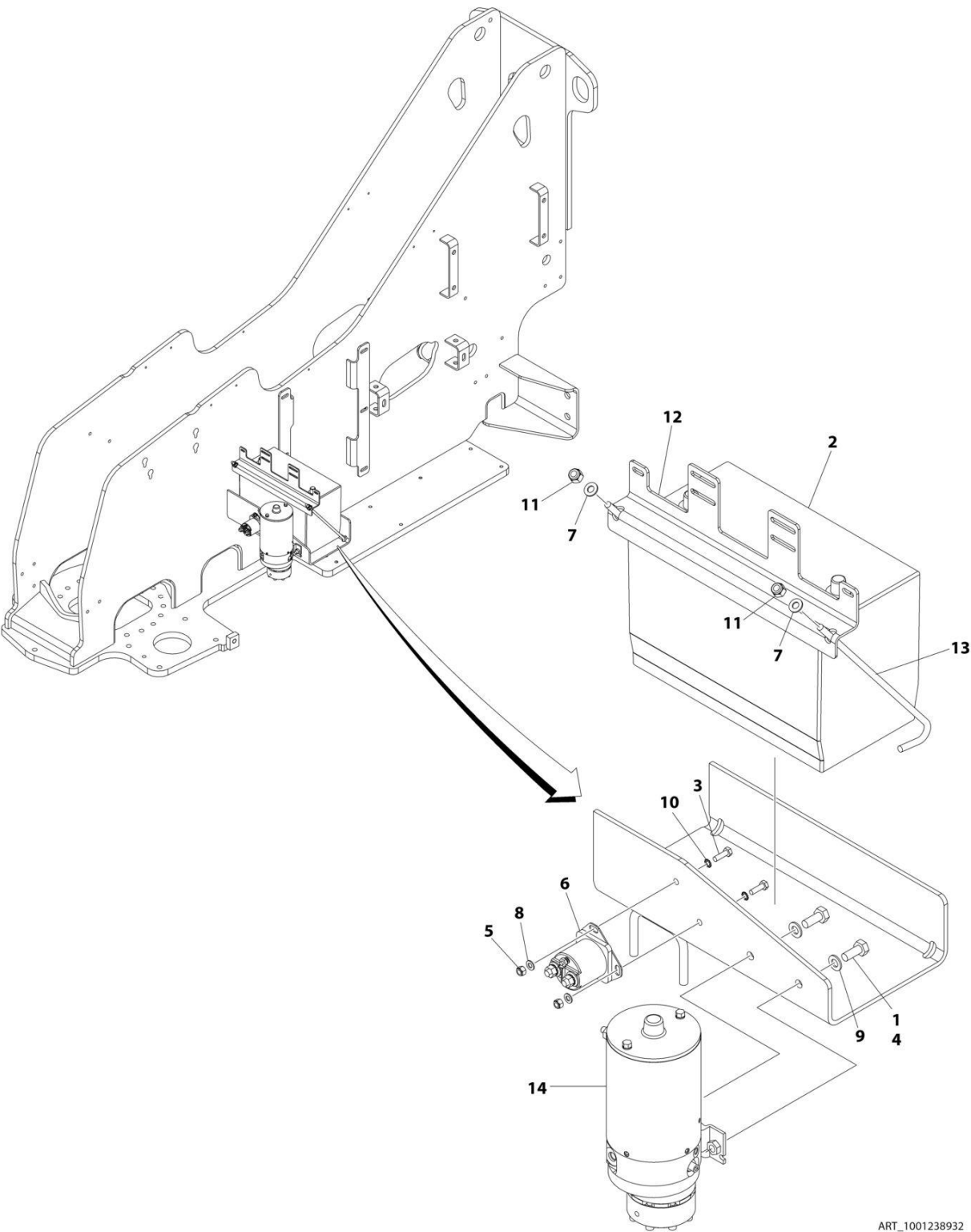
FIGURE 2-19. AUXILIARY PUMP AND BATTERY INSTALLATION (WITH DISCONNECT)
