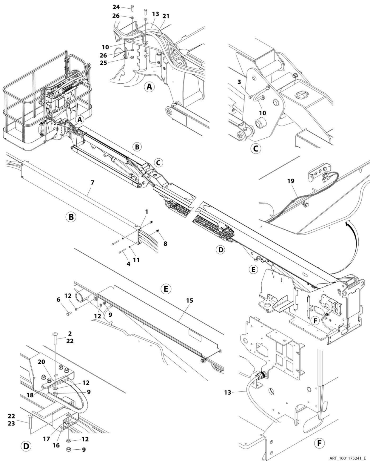
FIGURE 8-32. CABLES AND CLAMPS INSTALLATION - 460SJC WITH 4000W GENERATOR 60HZ
