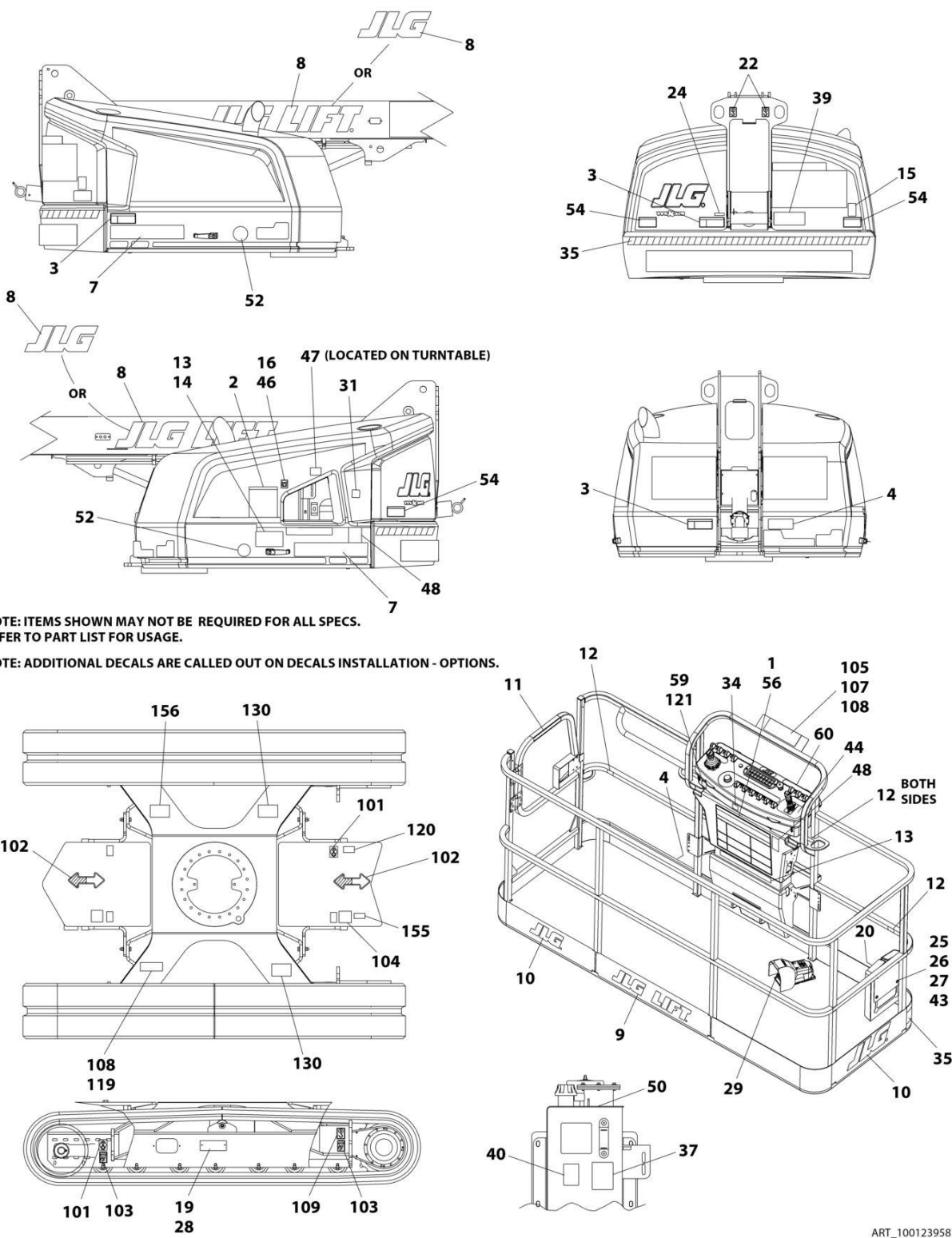
FIGURE 9-7. DECAL INSTALLATION - ANSI EXPORT - 400SC (JAPANESE SPECS)
