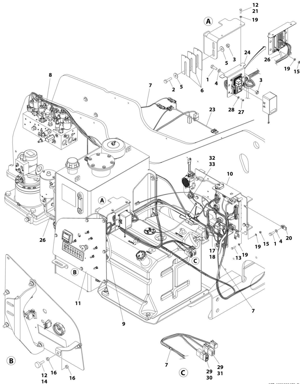
FIGURE 2-6. ELECTRICAL INSTALLATION - 400SC
