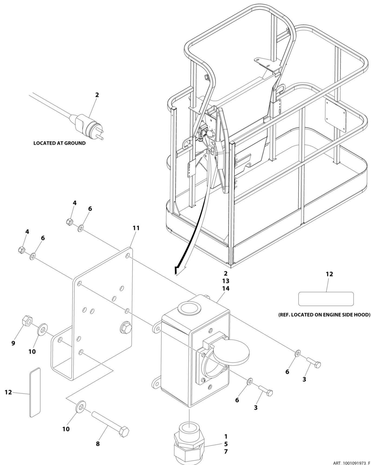
FIGURE 8-6. AC BOX AT PLATFORM - 220V CEE7 2IN X 4IN POST GROUND (CE SPEC WITHOUT GENERATOR)
