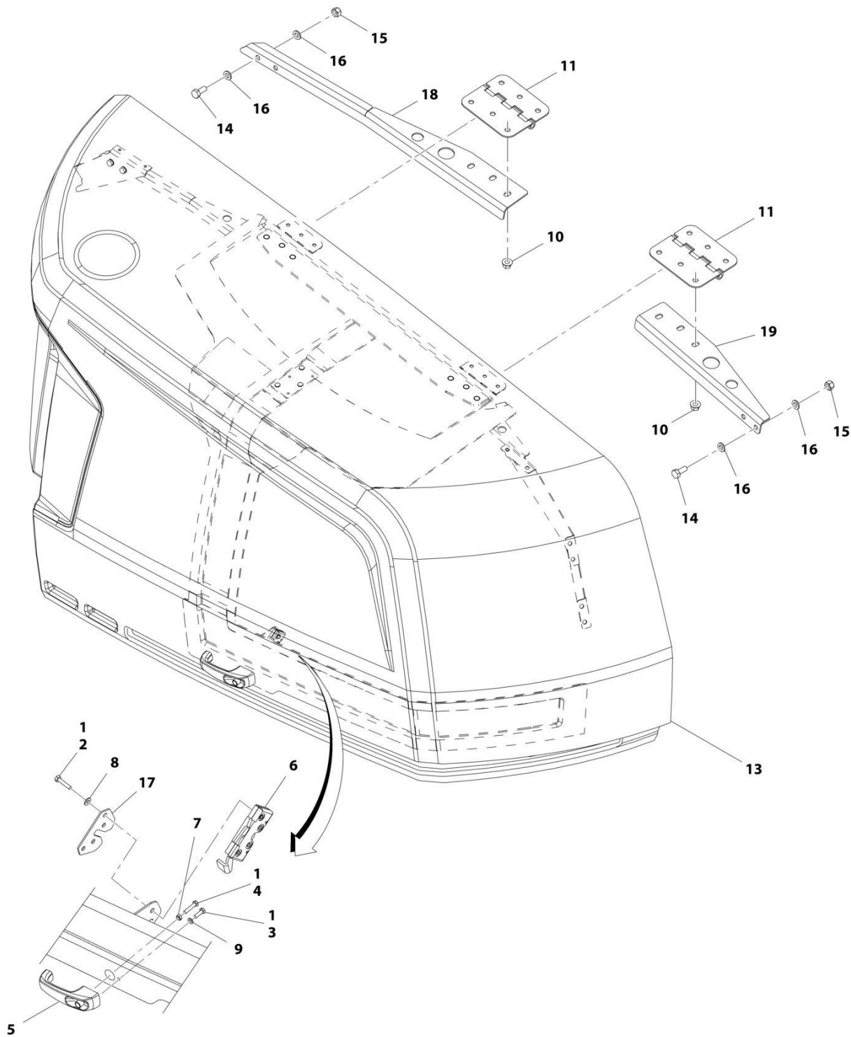
FIGURE 2-27. HOOD ASSEMBLY - ENGINE SIDE
