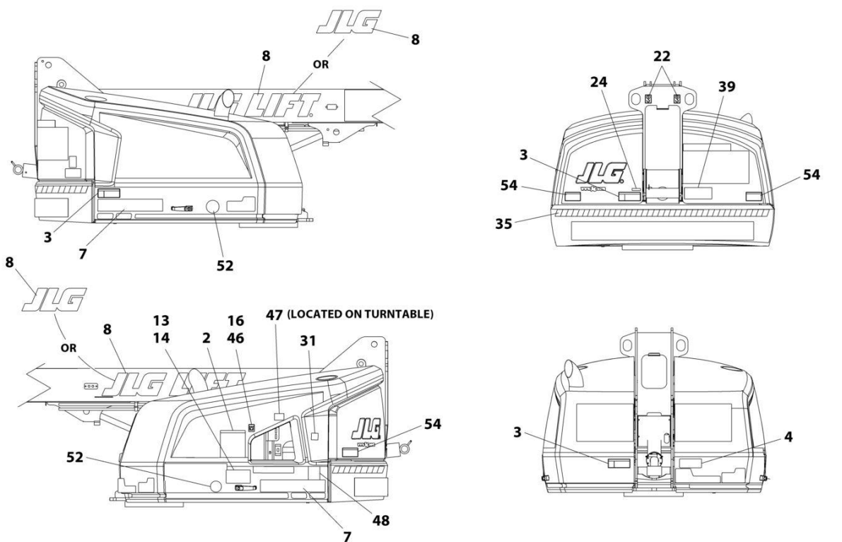
FIGURE 9-4. DECAL INSTALLATION - CE SPEC - 460SJC
