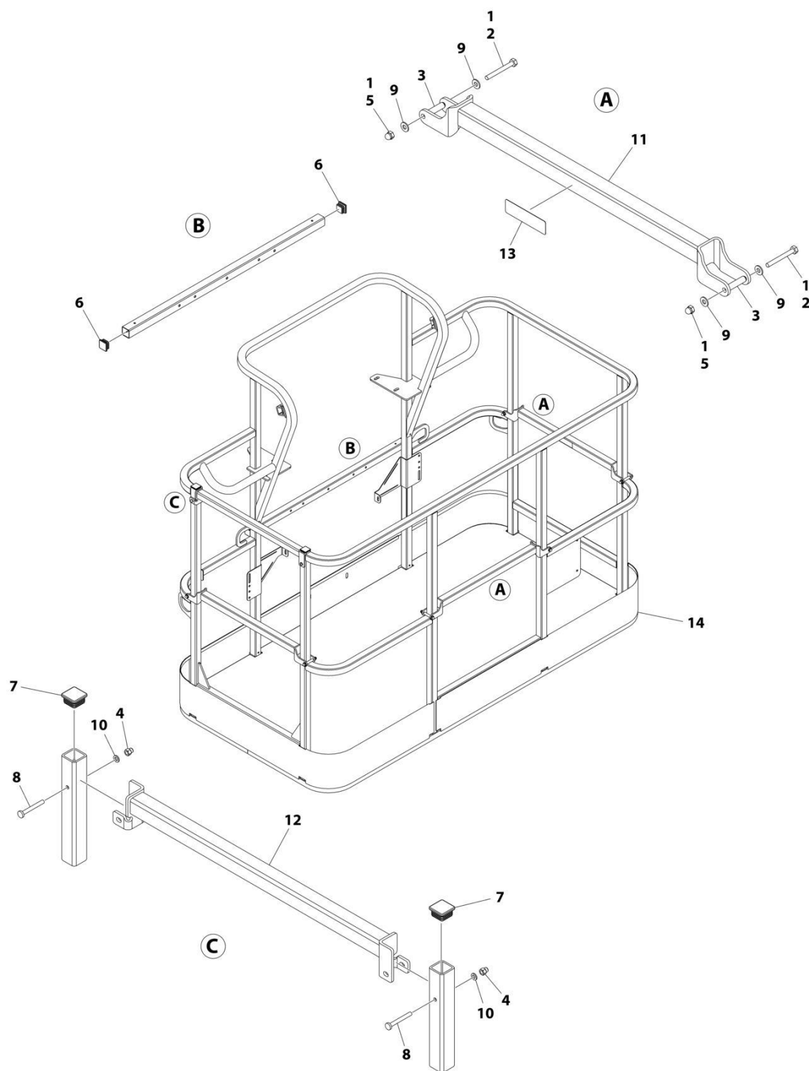
FIGURE 5-9. PLATFORM ASSEMBLY - 36IN X 6FT (91.5CM X 1.83M) TRI-ENTRY WITH DROPBAR
