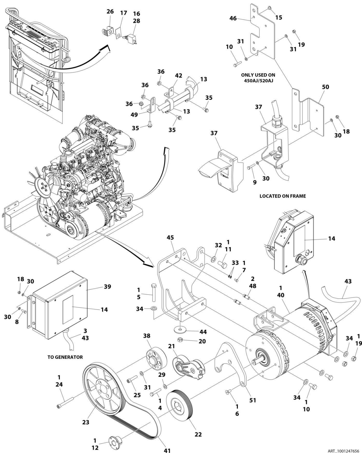
FIGURE 3-36. GENERATOR INSTALLATION - 4000W/50HZ (DEUTZ (STAGE V) ENGINE) (CE SPEC)
