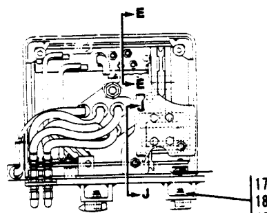
VIEW D-D
