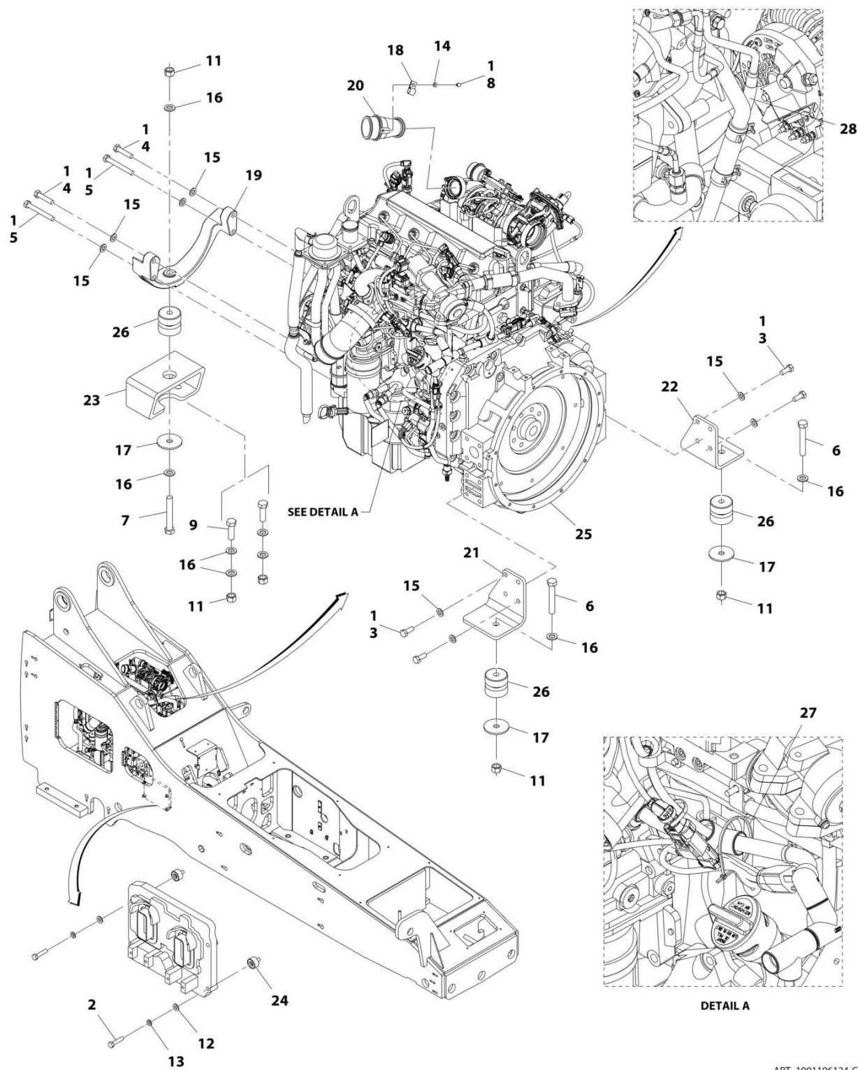
FIGURE 4-4. ENGINE INSTALLATION (74HP ULS)
