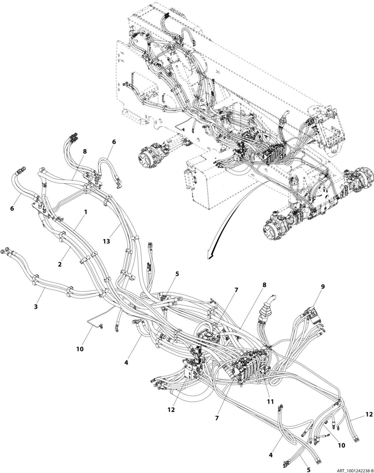
FIGURE 8-1. HYDRAULIC INSTALLATION
