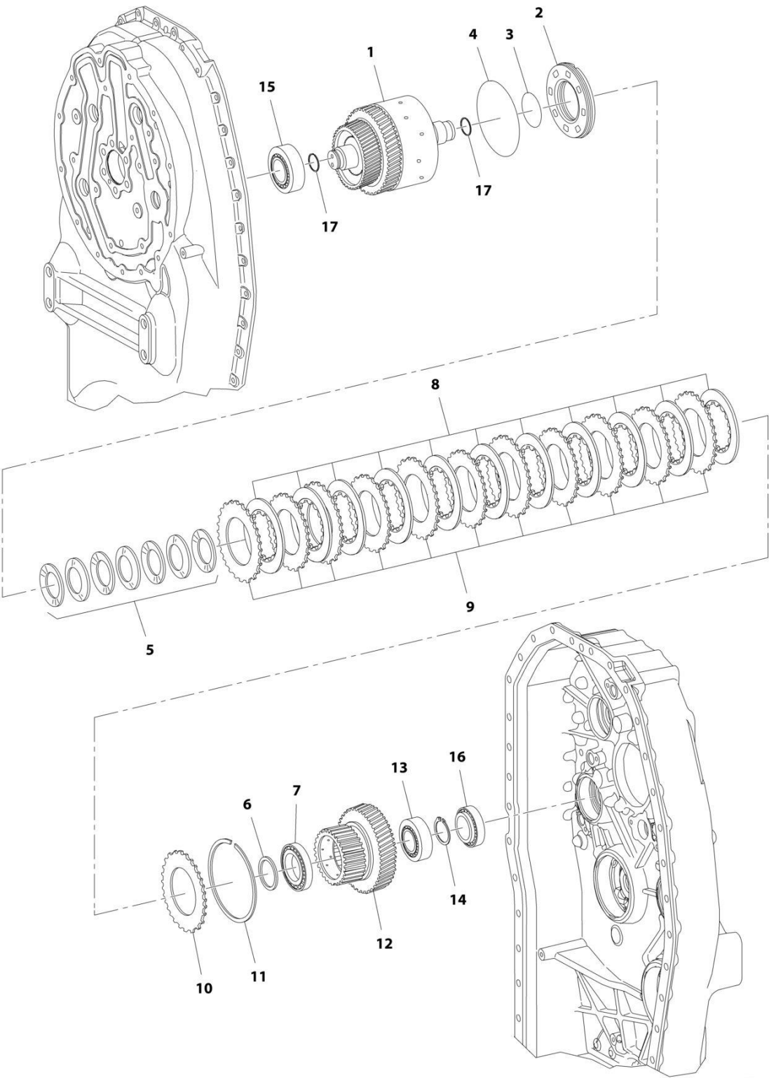
FIGURE 5-26. TRANSMISSION, REVERSING GEAR GROUP 1
