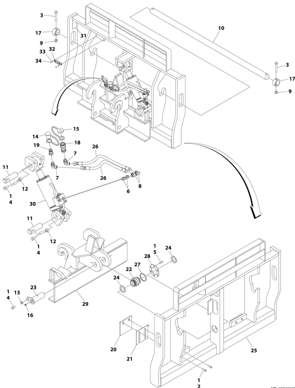
FIGURE 3-15. CARRIAGE ASSEMBLY (60 INCH 12K) (SIDE TILT)
