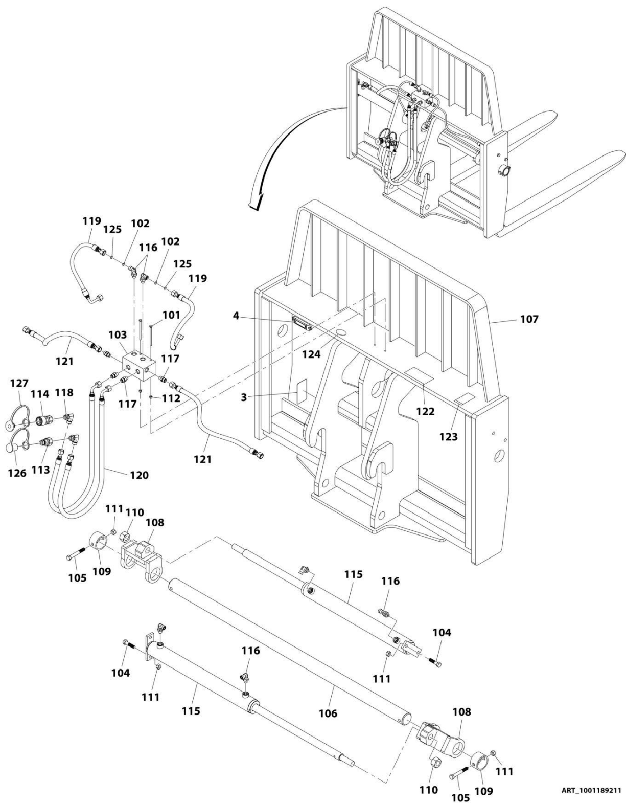
FIGURE 3-12. CARRIAGE (50 INCH 12K) (DUAL FORK)
