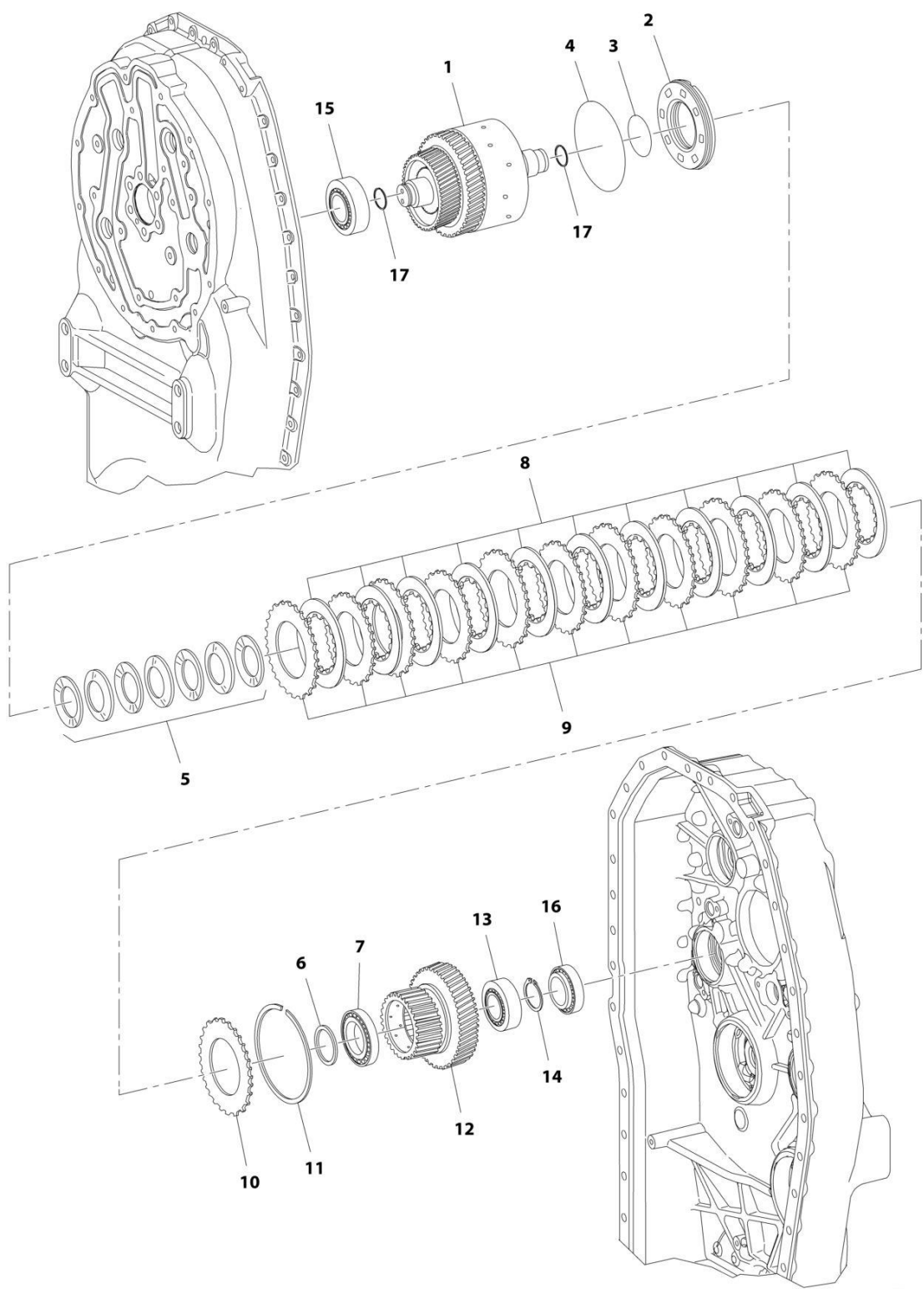
FIGURE 5-27. TRANSMISSION, REVERSING GEAR GROUP 2
