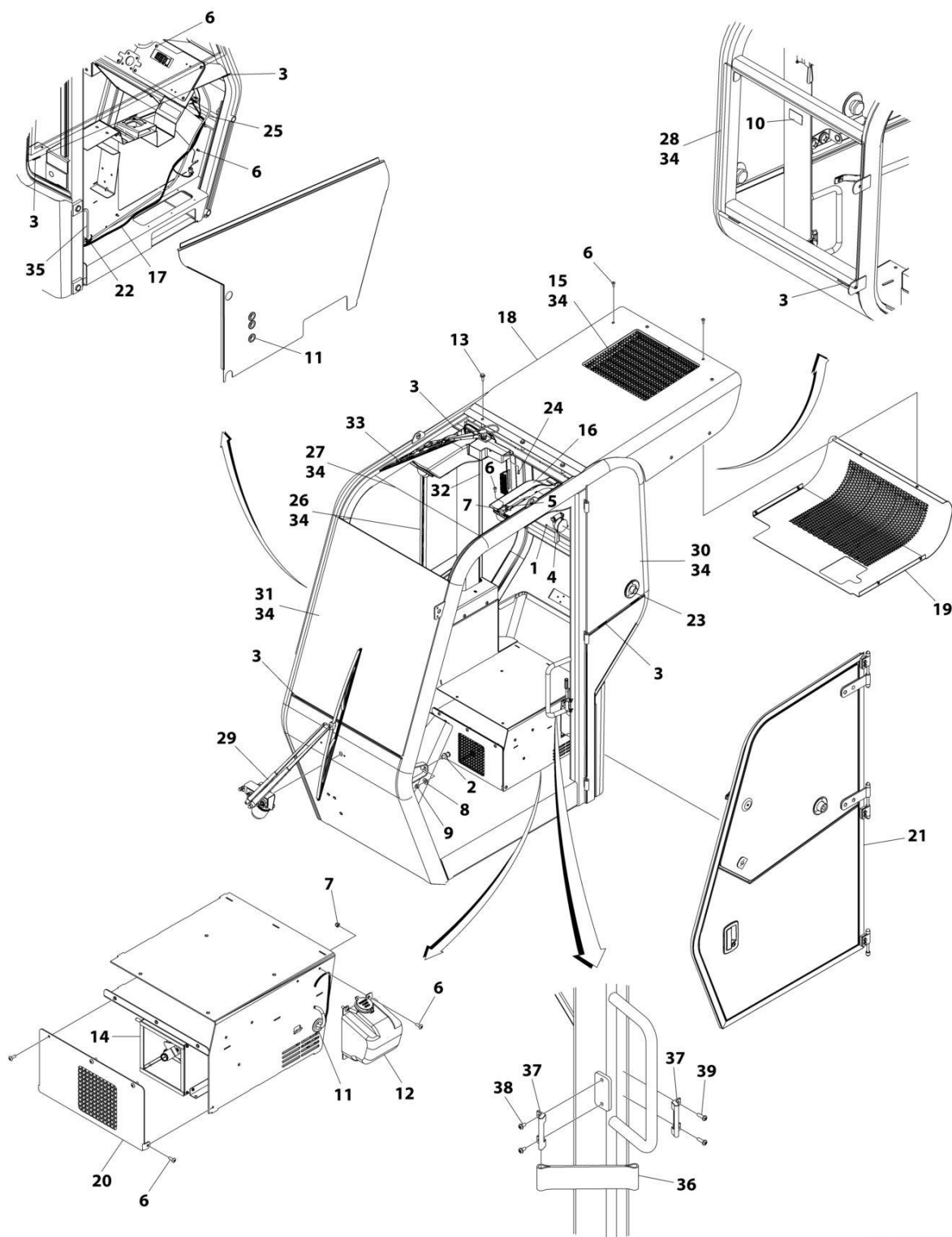
FIGURE 6-11. CAB HVAC ENCLOSURE
