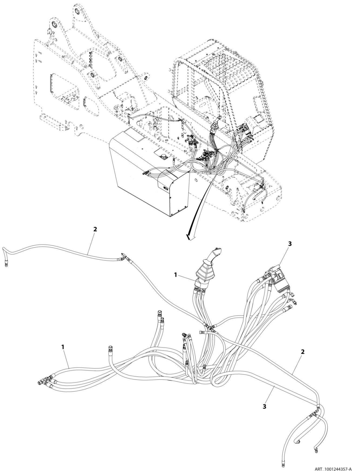
FIGURE 8-10. CAB HYDRAULICS INSTALLATION
