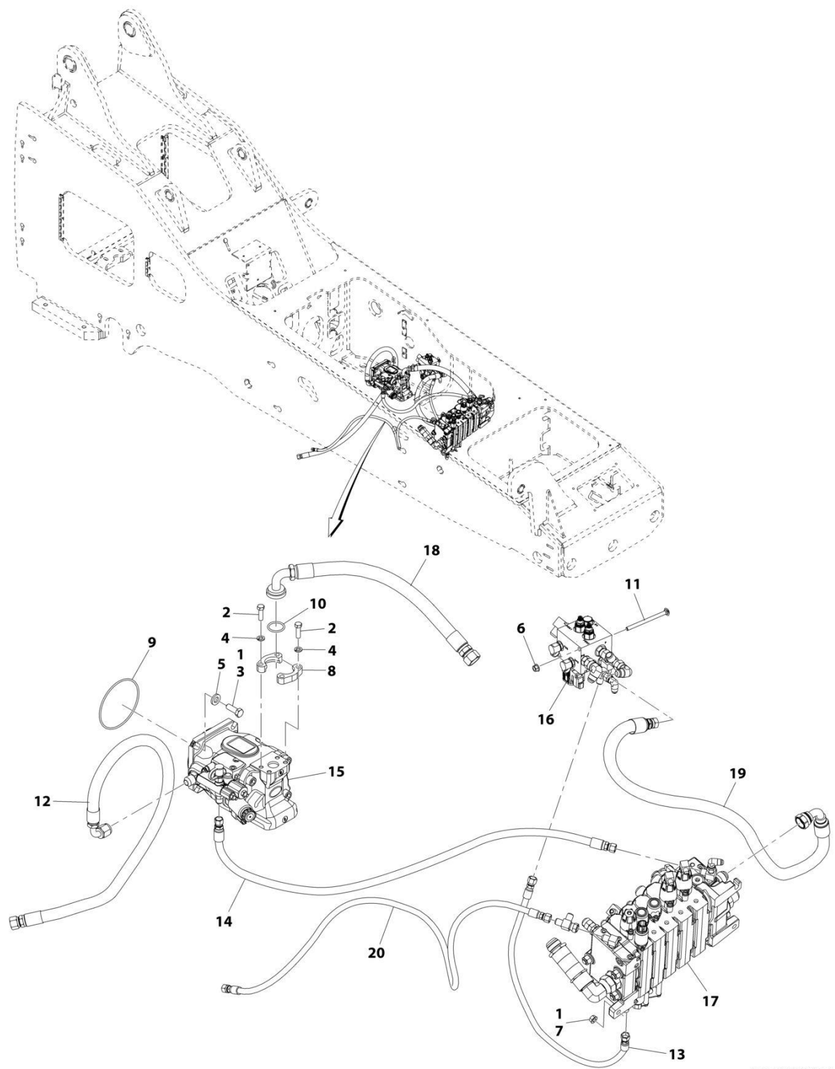
FIGURE 8-23. PUMP HYDRAULICS INSTALLATION
