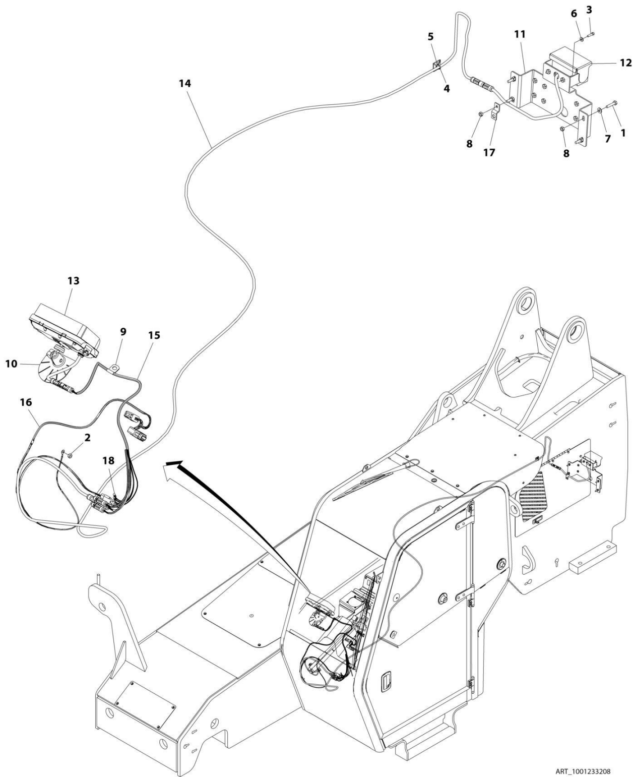
FIGURE 10-44. REVERSE CAMERA
