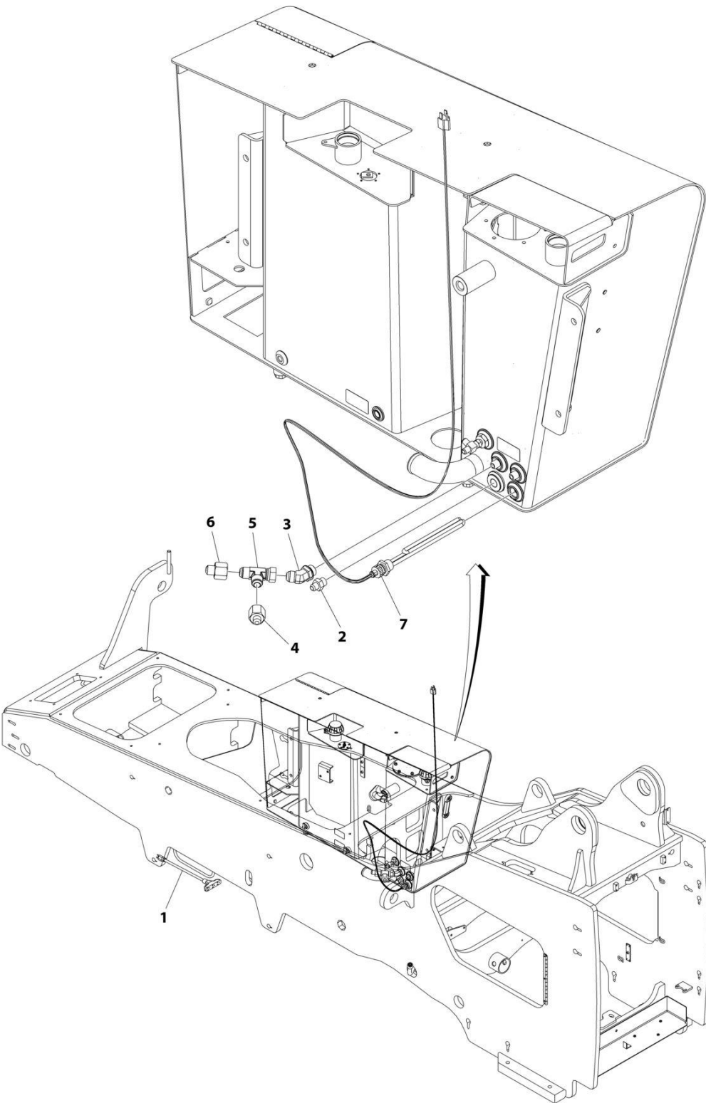
FIGURE 10-48. TANK HEATER INSTALLATION - HYDRAULIC TANK
