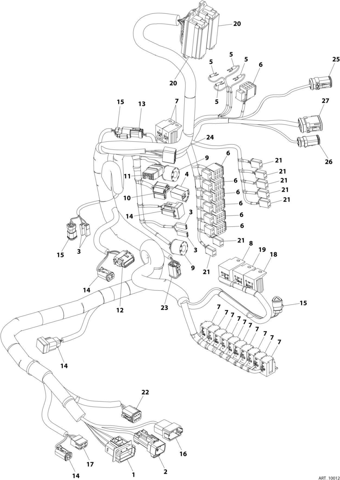
FIGURE 10-7. CAB HARNESS
