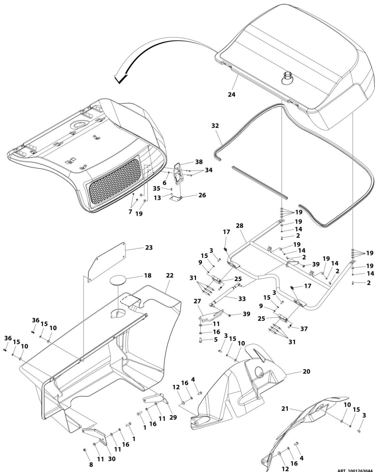
FIGURE 1-2. ENGINE ENCLOSURE INSTALLATION
