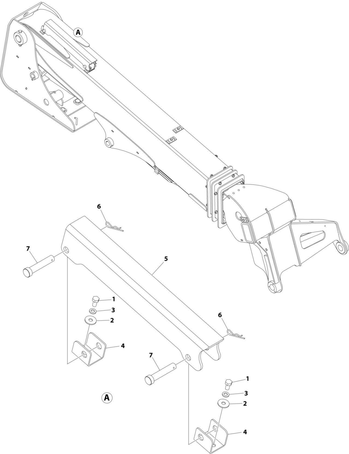
FIGURE 2-8. BOOM PROP INSTALLATION
