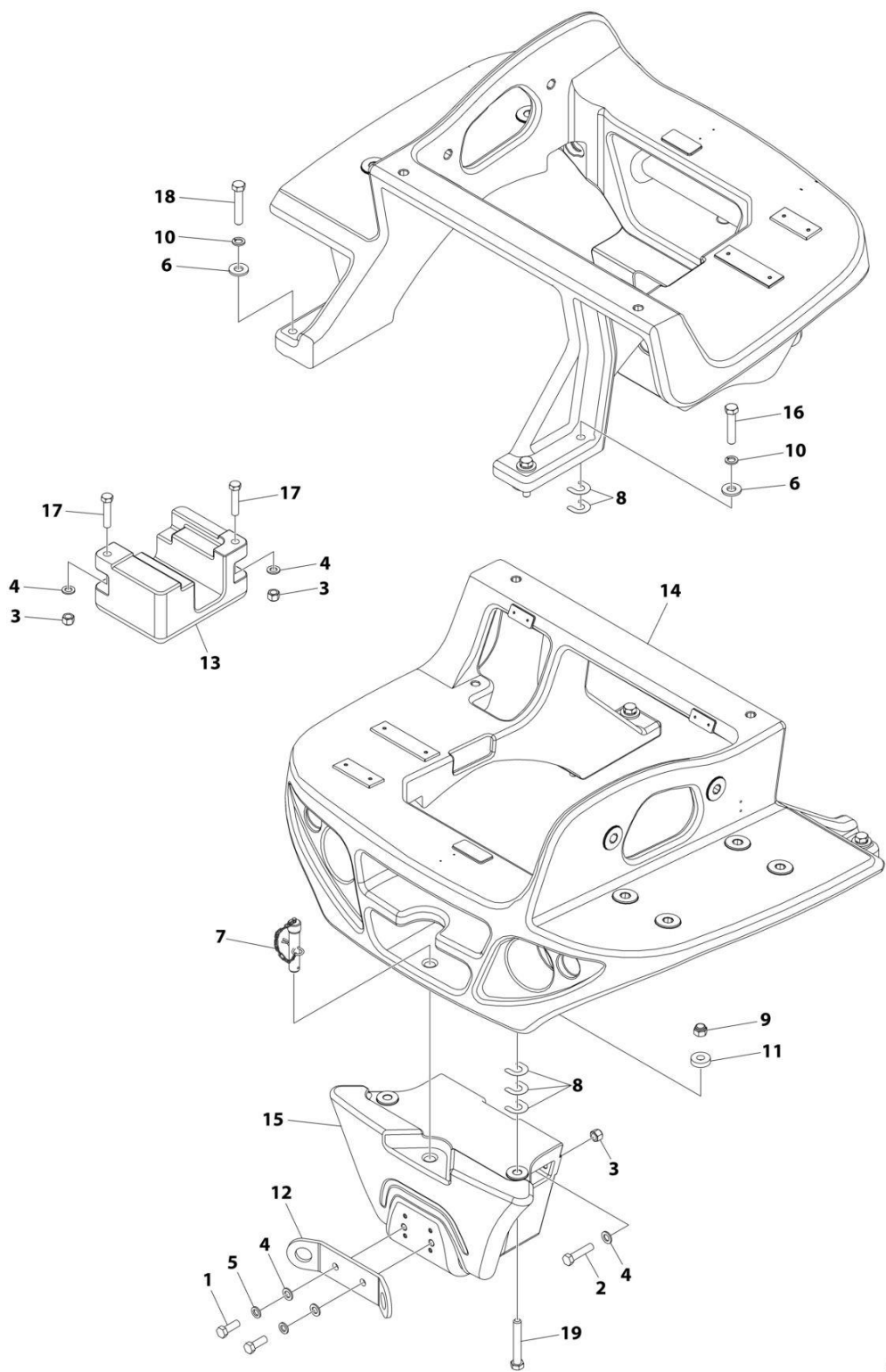
FIGURE 1-1. COUNTERWEIGHT INSTALLATION
