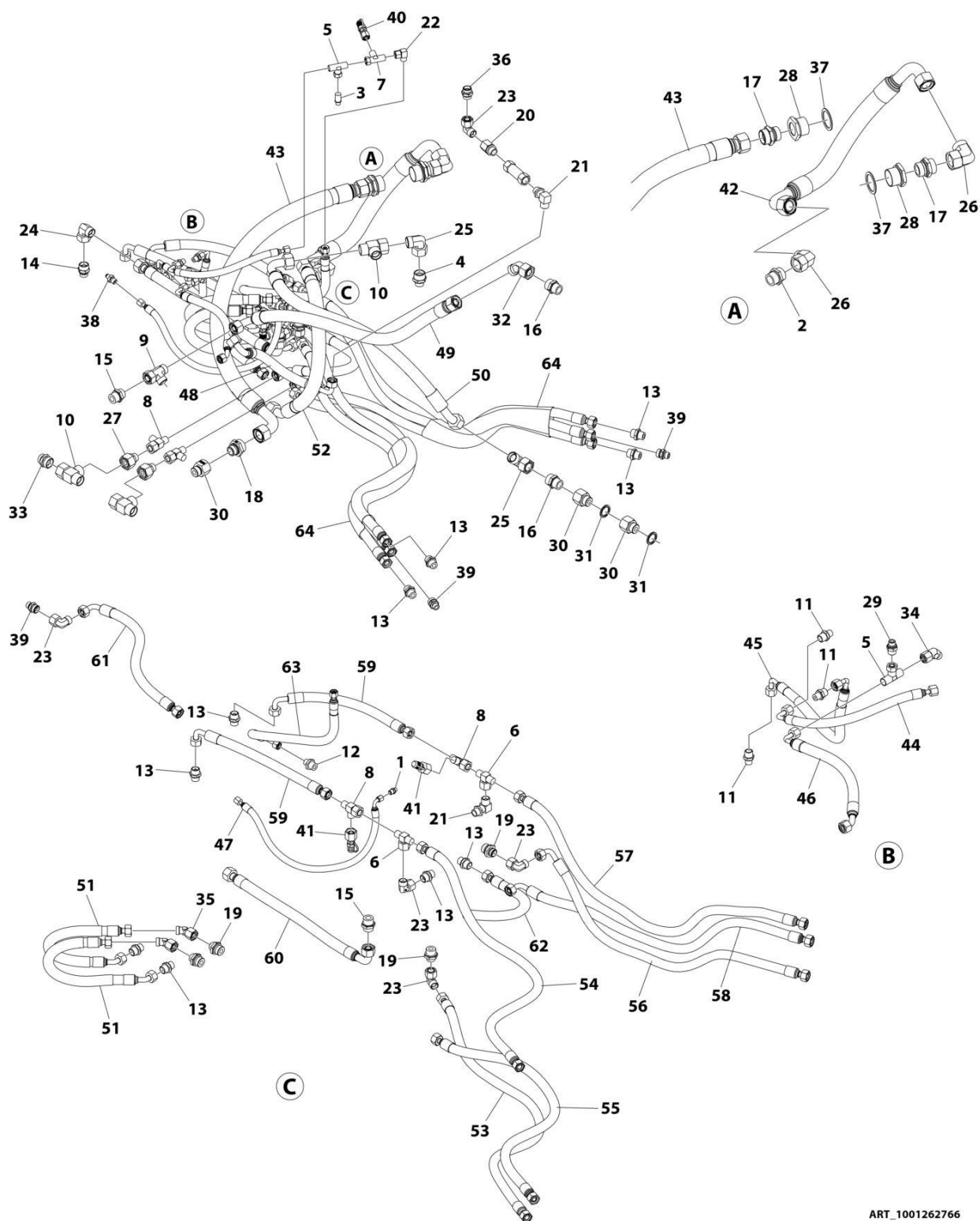
FIGURE 8-7. TRANSMISSION HOSES INSTALLATION
