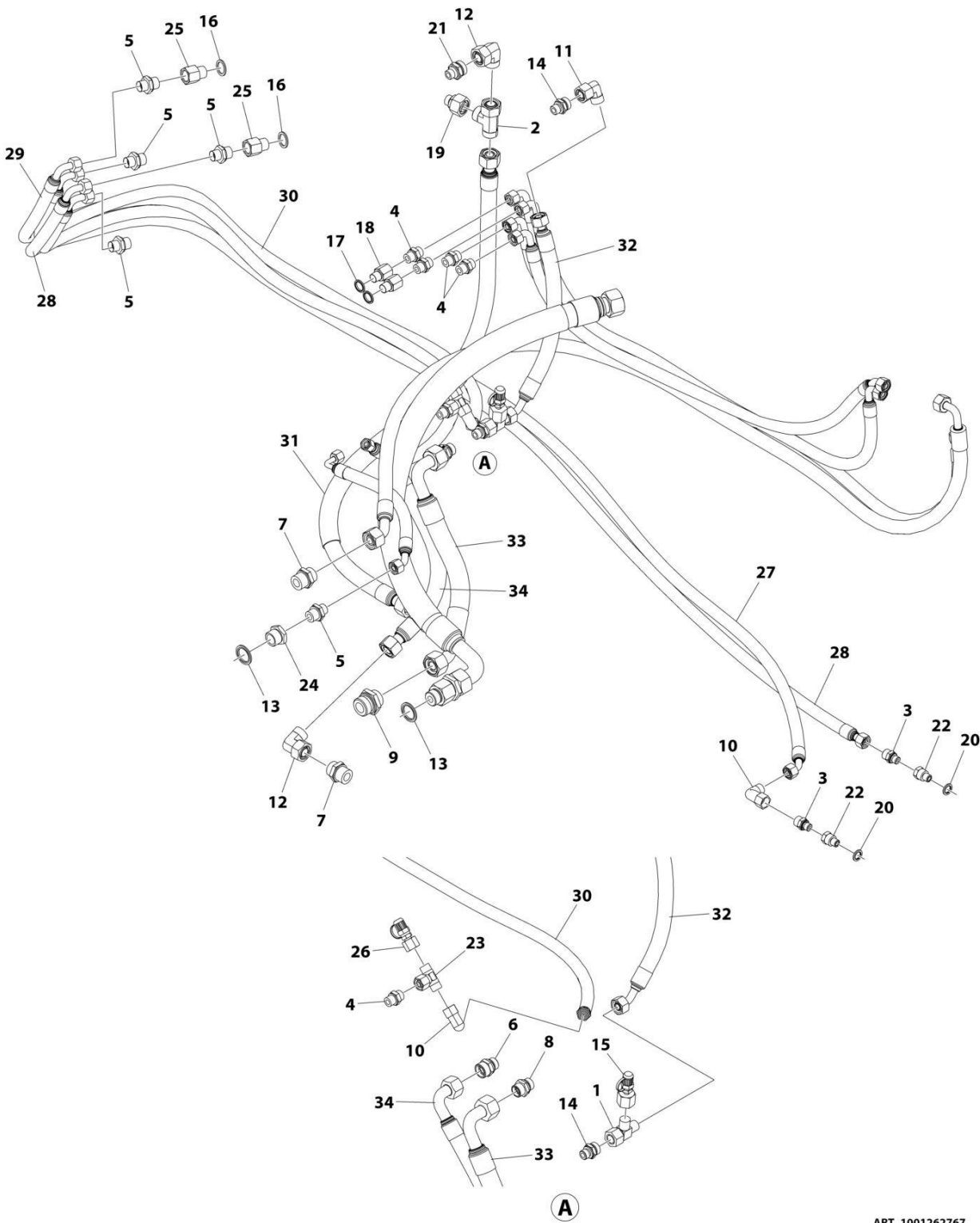
FIGURE 8-6. JOYSTICK HOSES INSTALLATION
