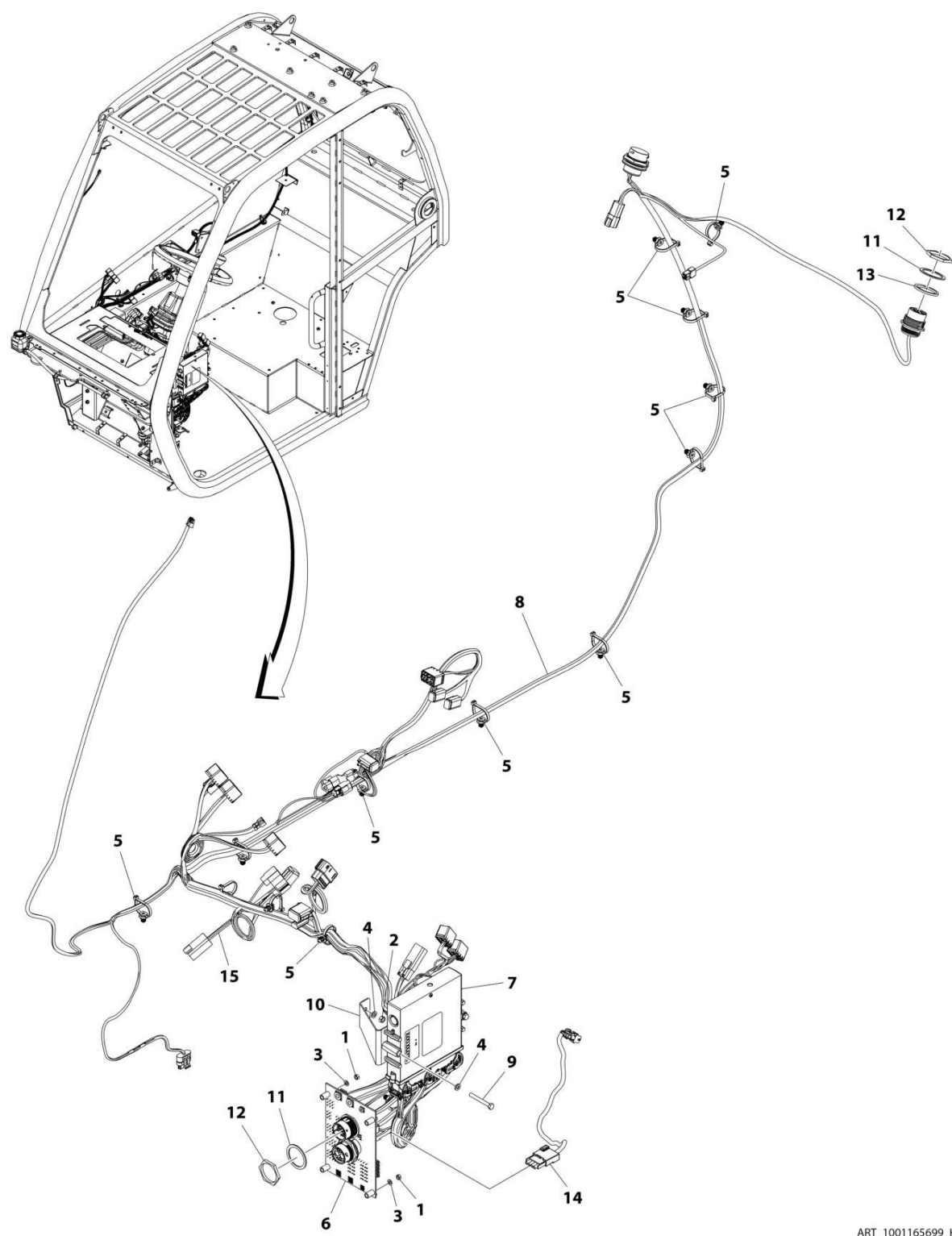
FIGURE 10-17. CAB ELECTRICAL INSTALLATION
