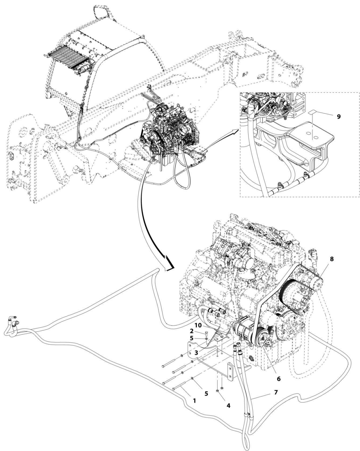
FIGURE 4-41. A/C PUMP INSTALLATION (LS)
