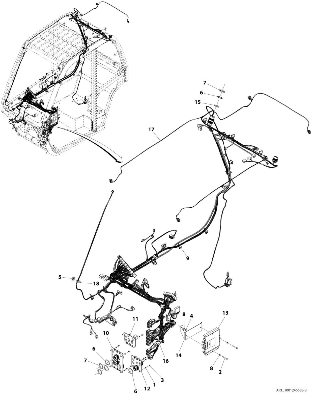
FIGURE 10-18. CAB ELECTRICAL INSTALLATION
