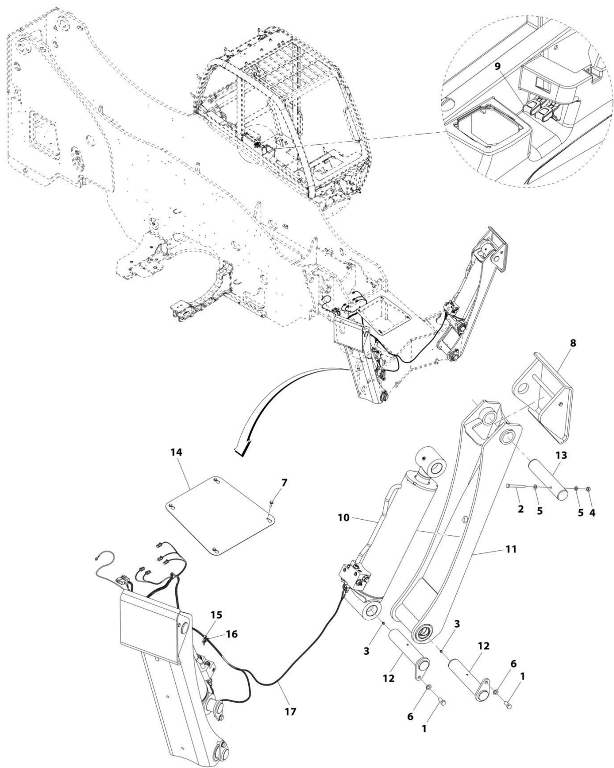
FIGURE 1-15. OUTRIGGERS INSTALLATION
