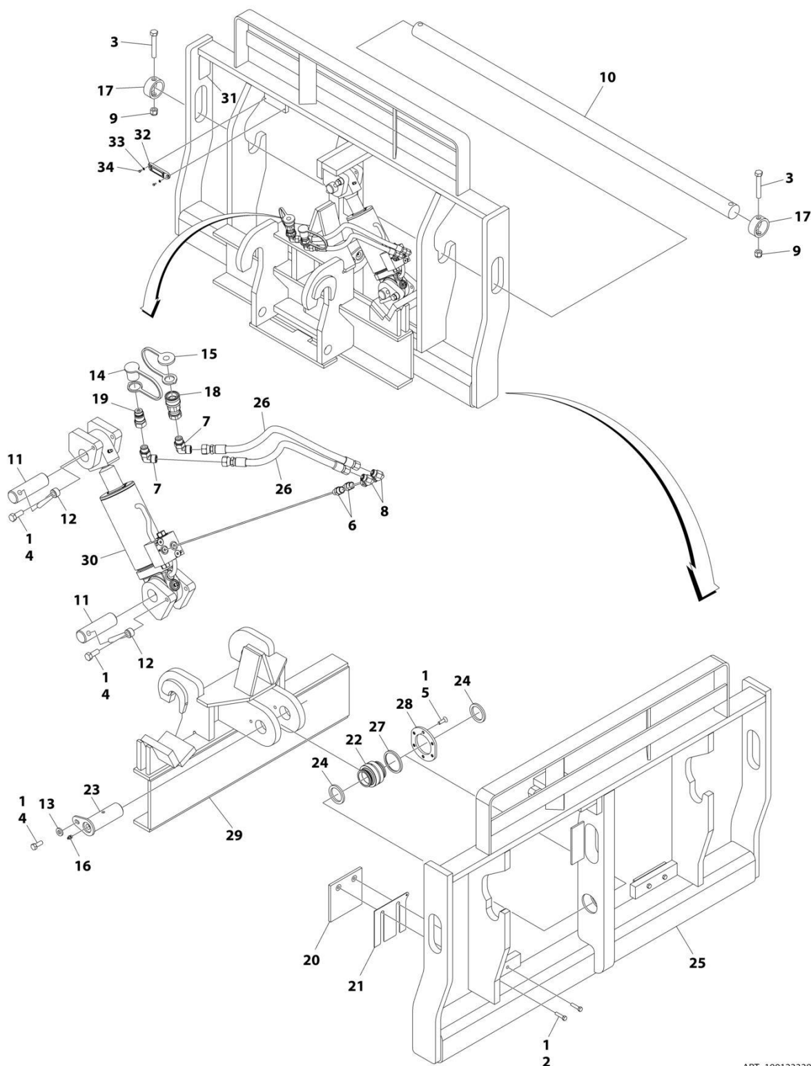
FIGURE 3-13. CARRIAGE ASSEMBLY - SIDE TILT (60 INCH)
