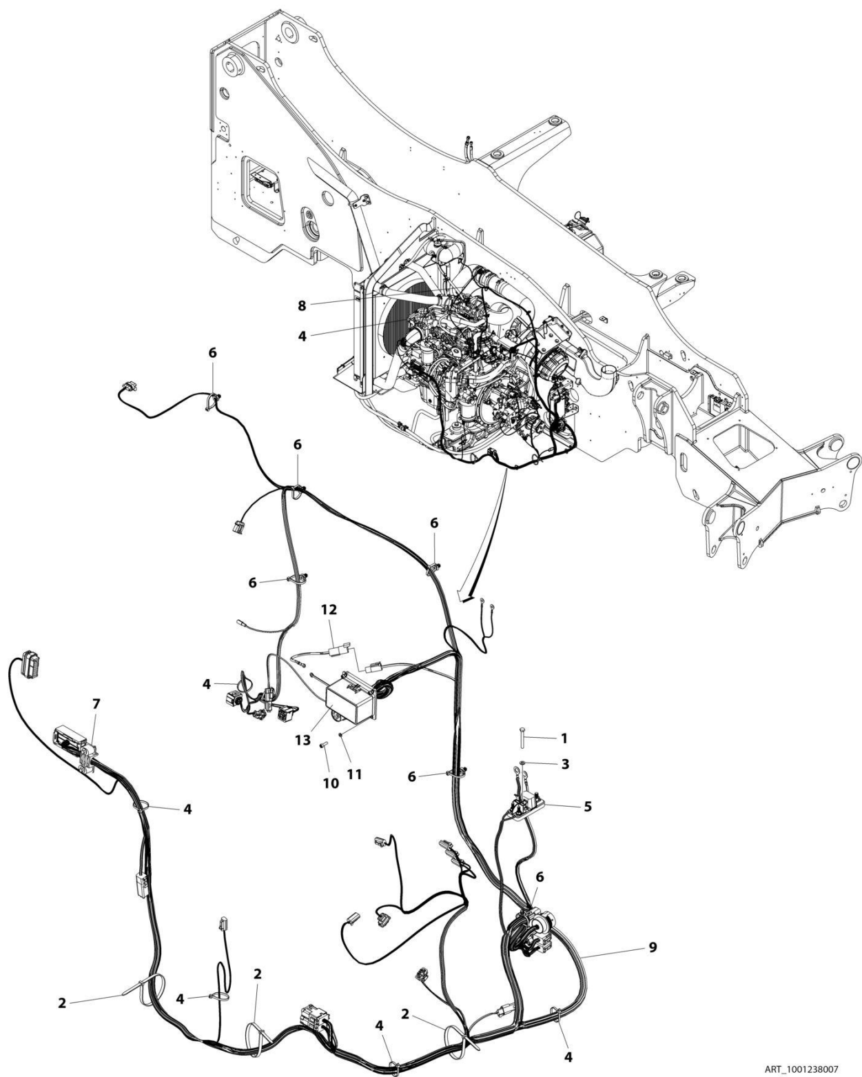
FIGURE 10-42. ENGINE WIRING INSTALLATION
