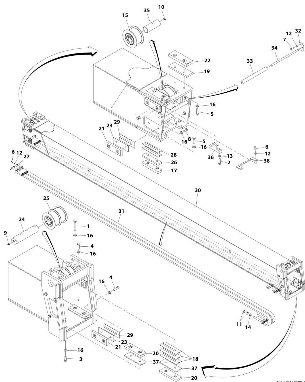
FIGURE 2-6. FOURTH BOOM SECTION ASSEMBLY
