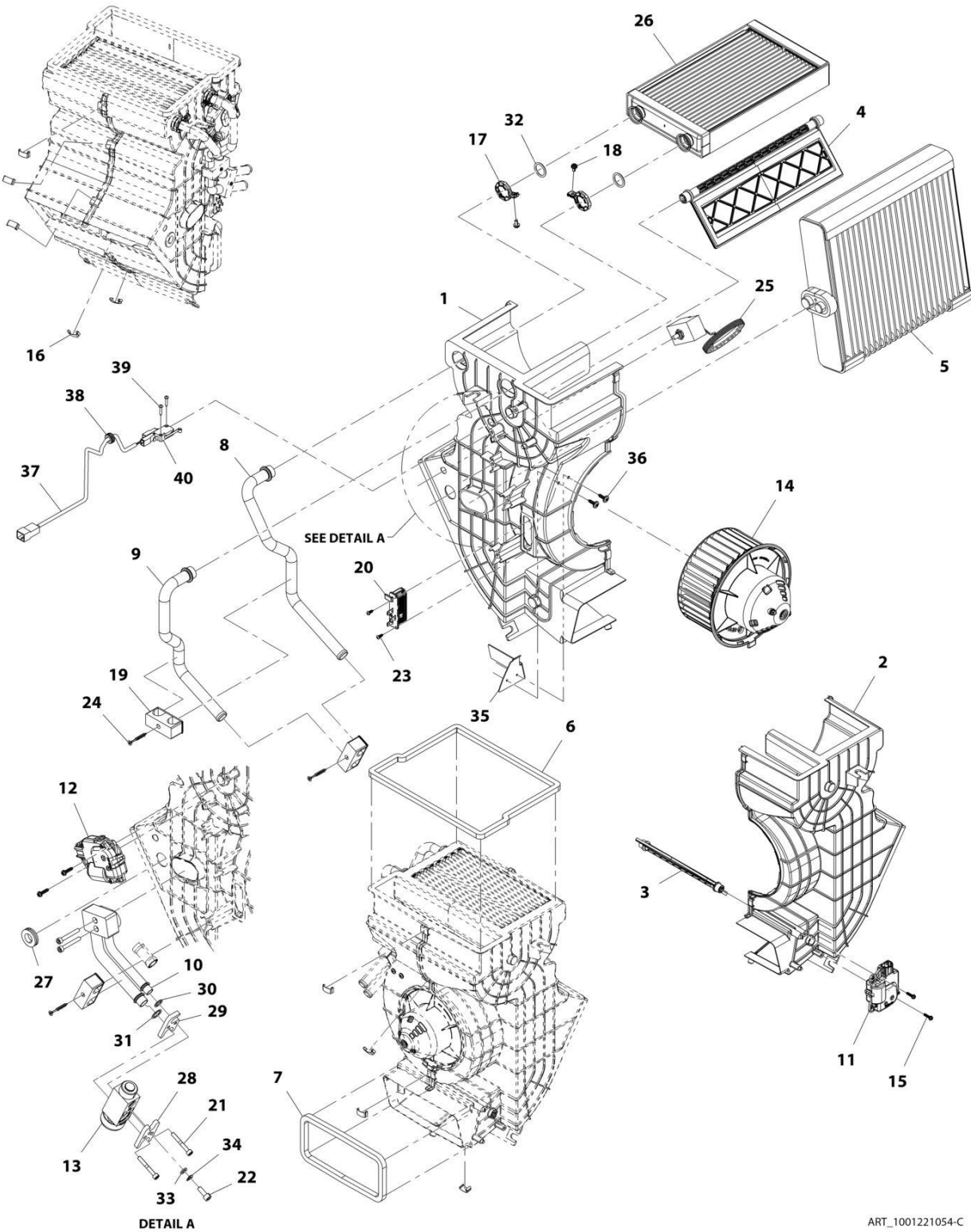
FIGURE 6-47. HEATER AND A/C
