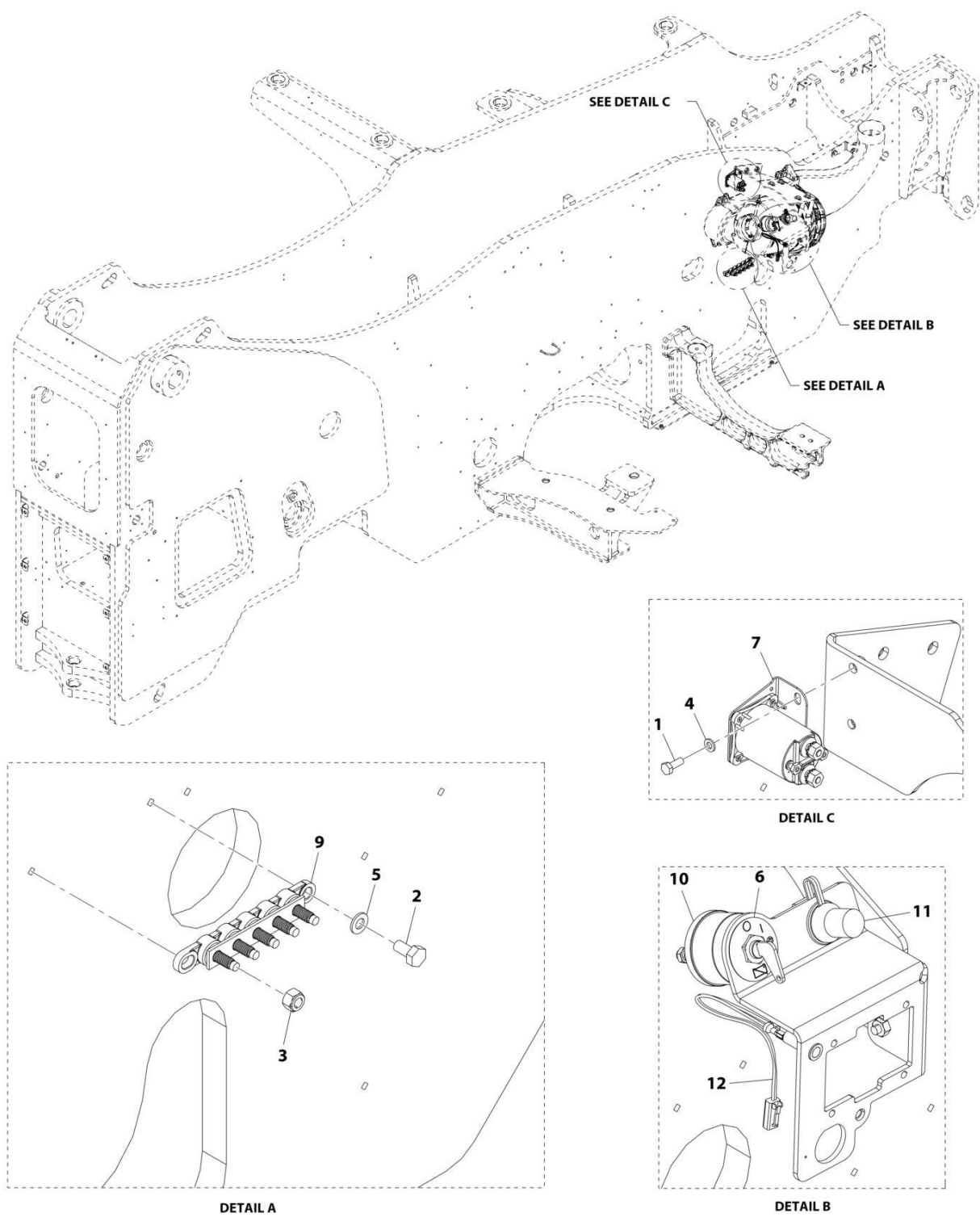
FIGURE 10-37. ENGINE BAY ELECTRICAL INSTALLATION
