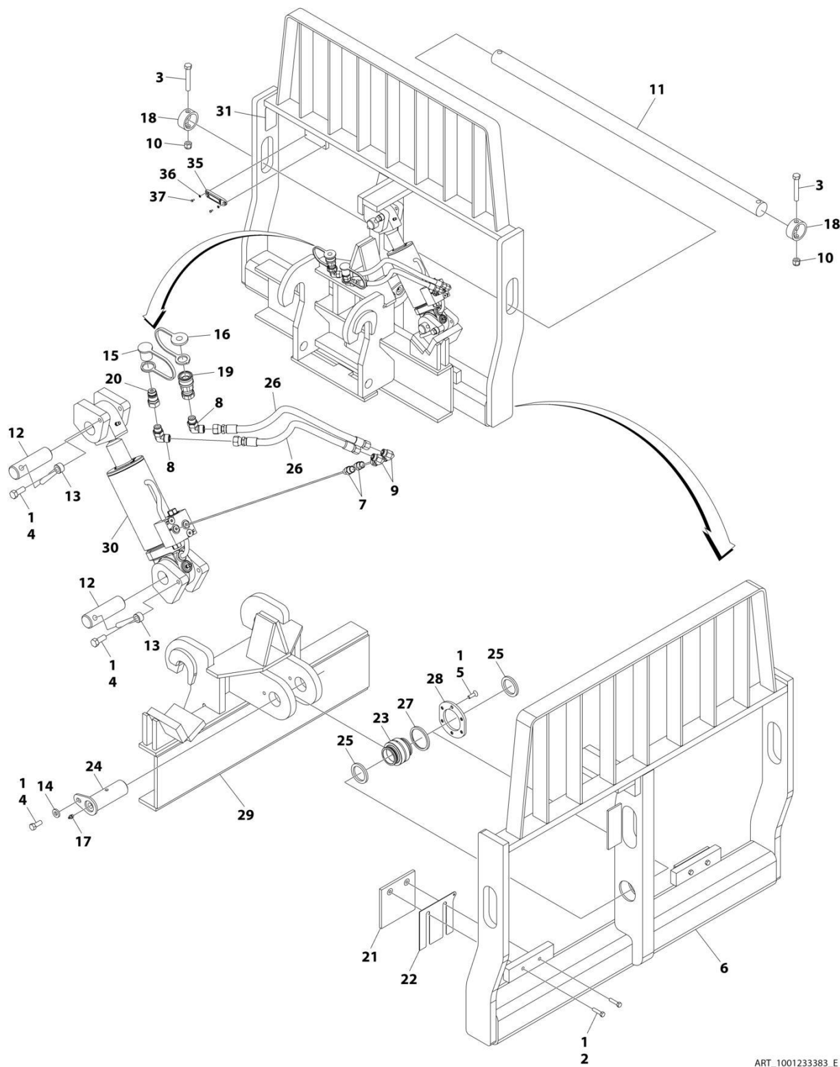
FIGURE 3-12. CARRIAGE ASSEMBLY - SIDE TILT (50 INCH)
