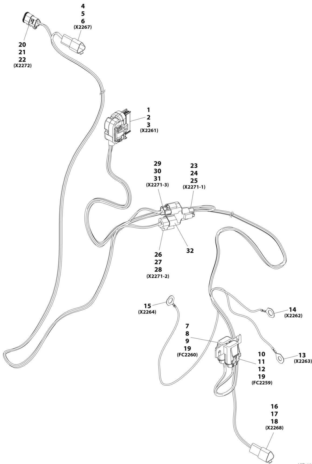
FIGURE 10-86. TELEMATICS CLEARSKY HARNESS - CANBUS
