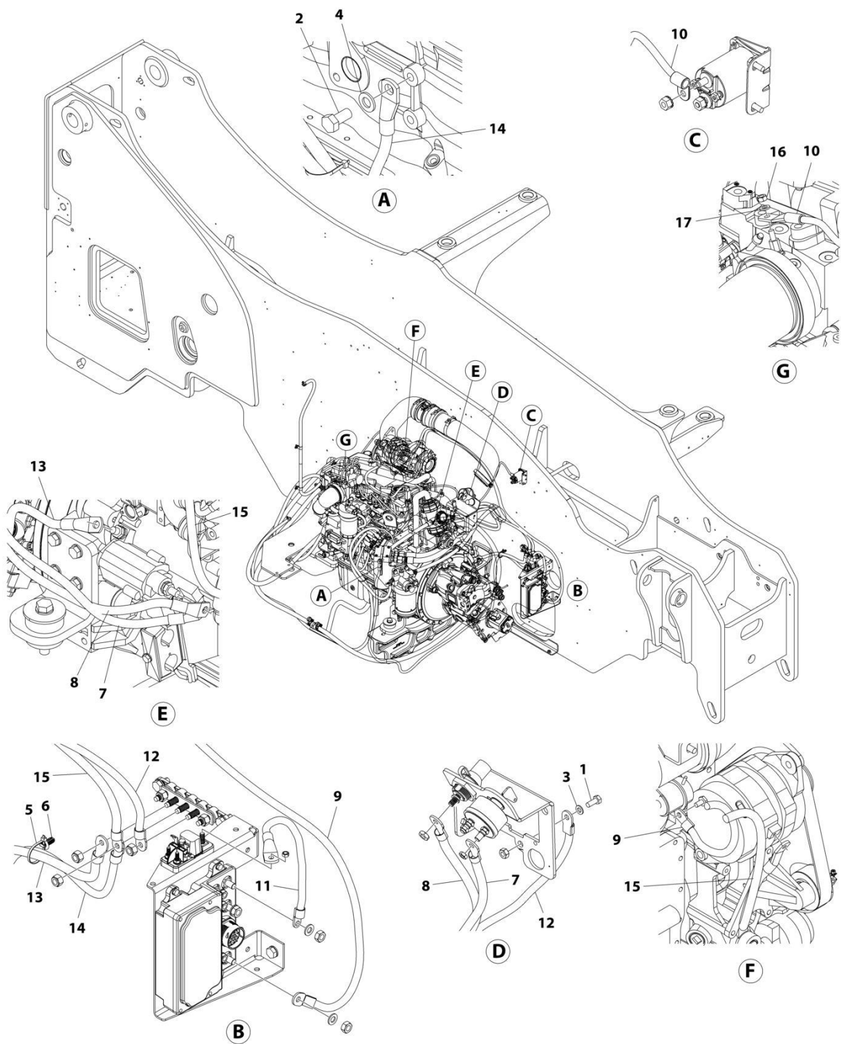
FIGURE 10-38. ENGINE BAY WIRING INSTALLATION
