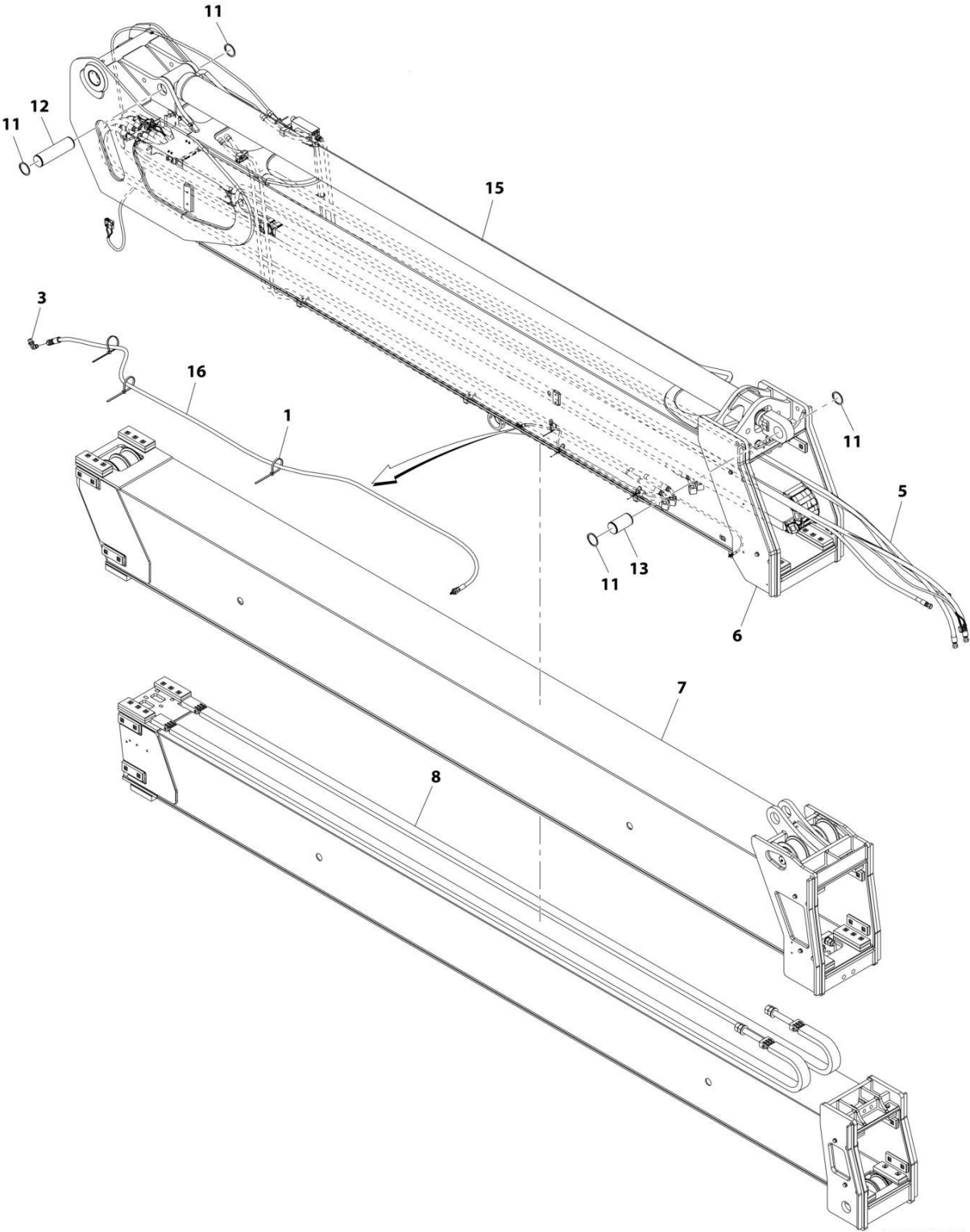
FIGURE 2-2. BOOM ASSEMBLY
