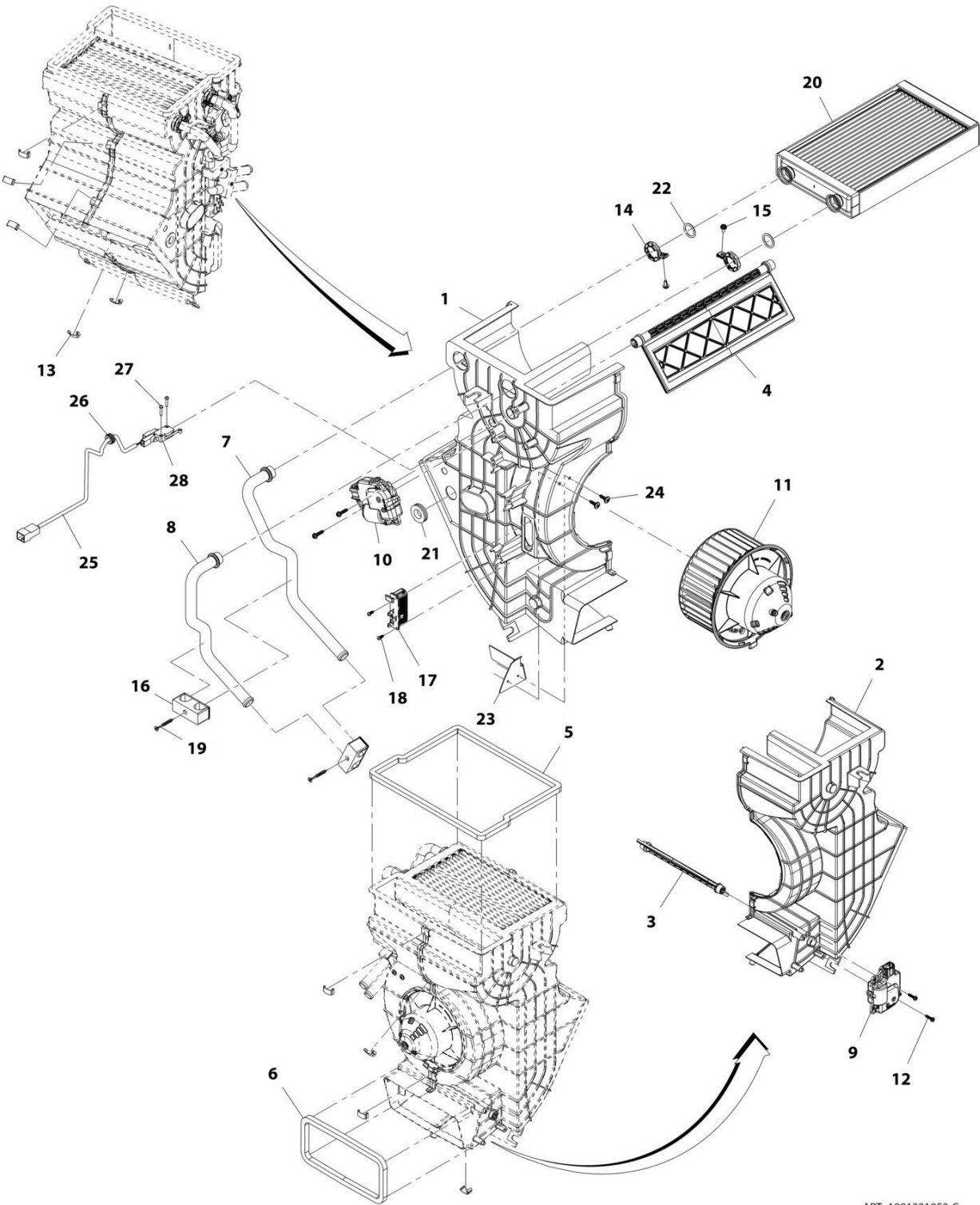
FIGURE 6-46. HEATER
