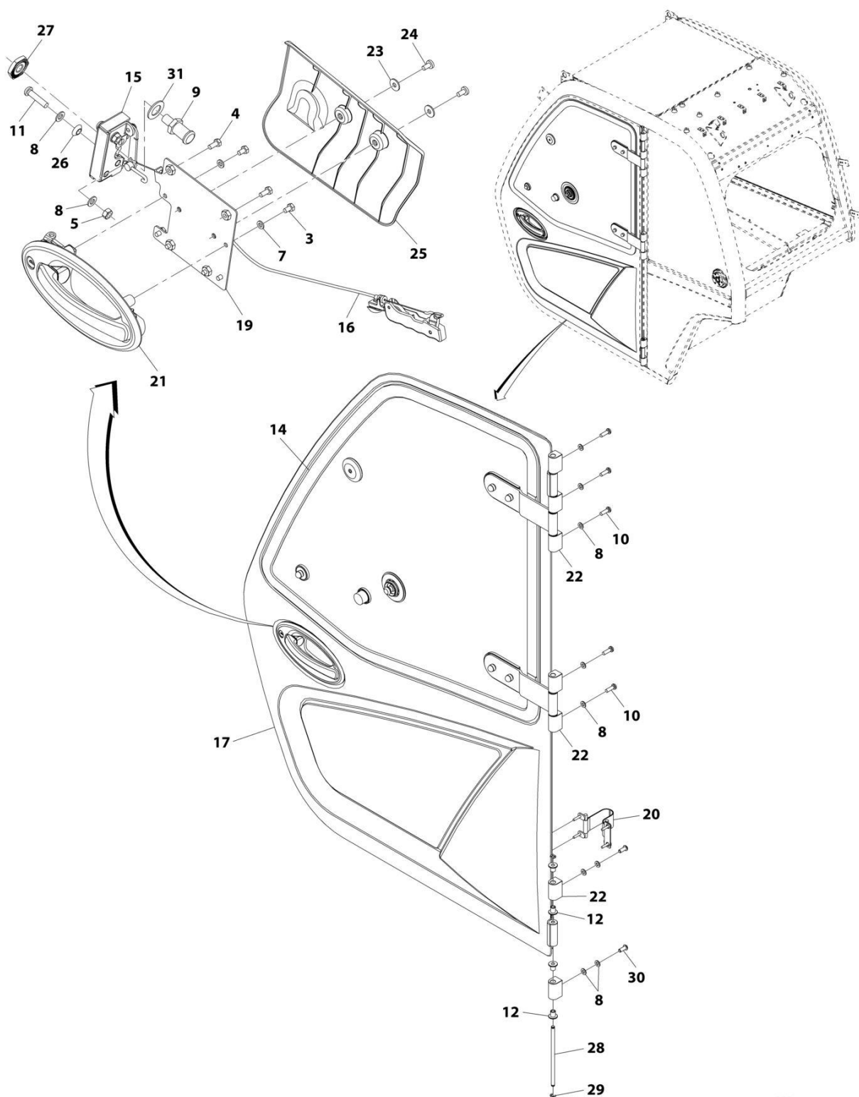
FIGURE 6-5. DOOR INSTALLATION
