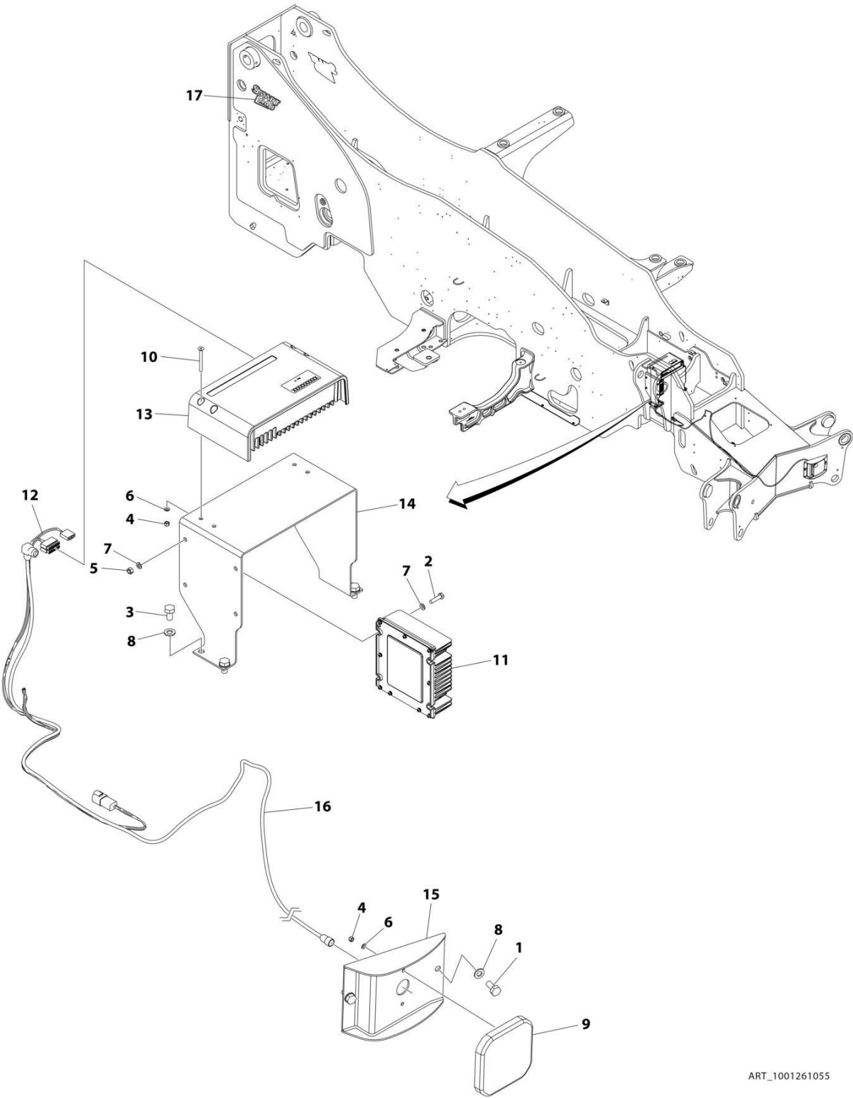
FIGURE 3-1. ATTACHMENT RECOGNITION INSTALLATION
