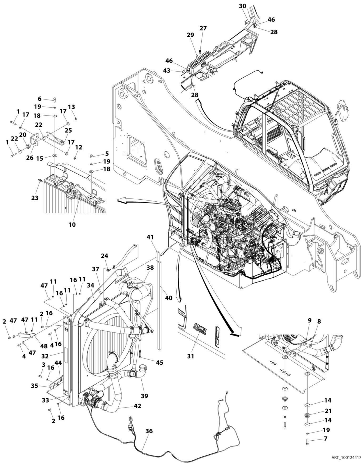
FIGURE 4-19. COOLING PACKAGE INSTALLATION (ASOV)
