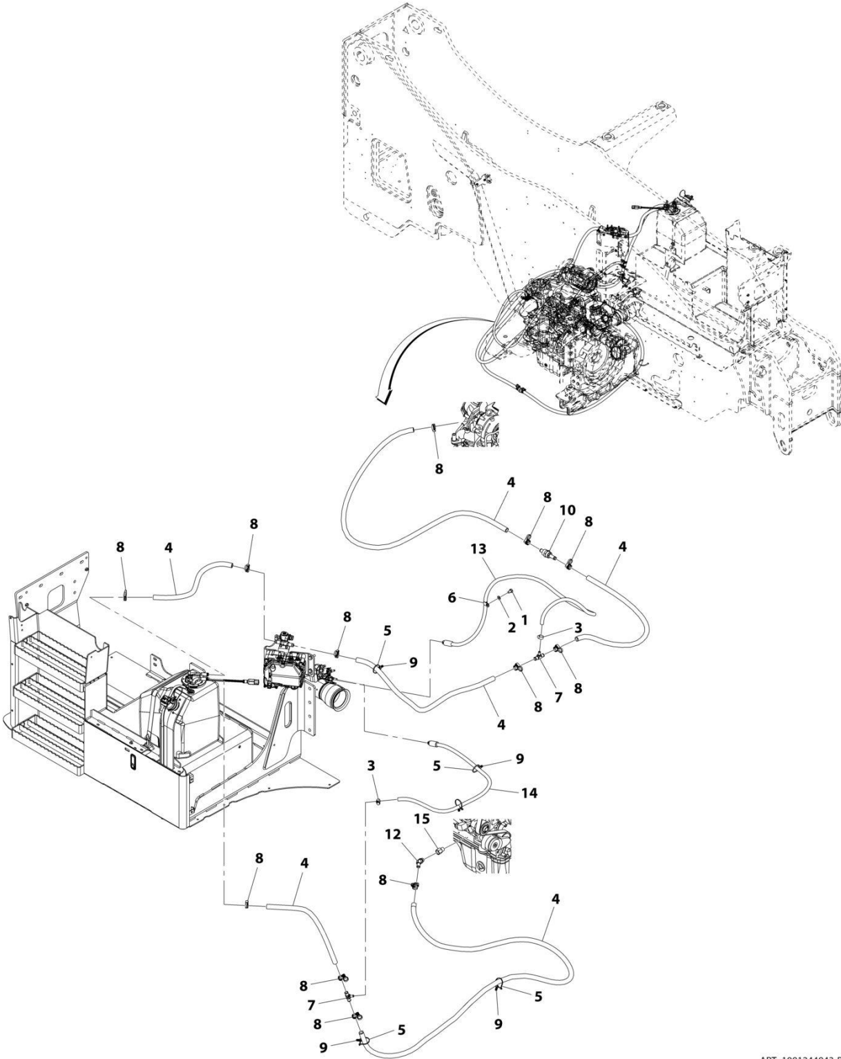
FIGURE 4-14. DEF COOLANT LINES INSTALLATION
