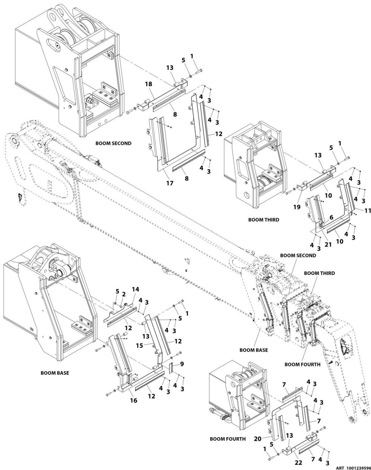
FIGURE 2-21. BOOM BRUSHES INSTALLATION
