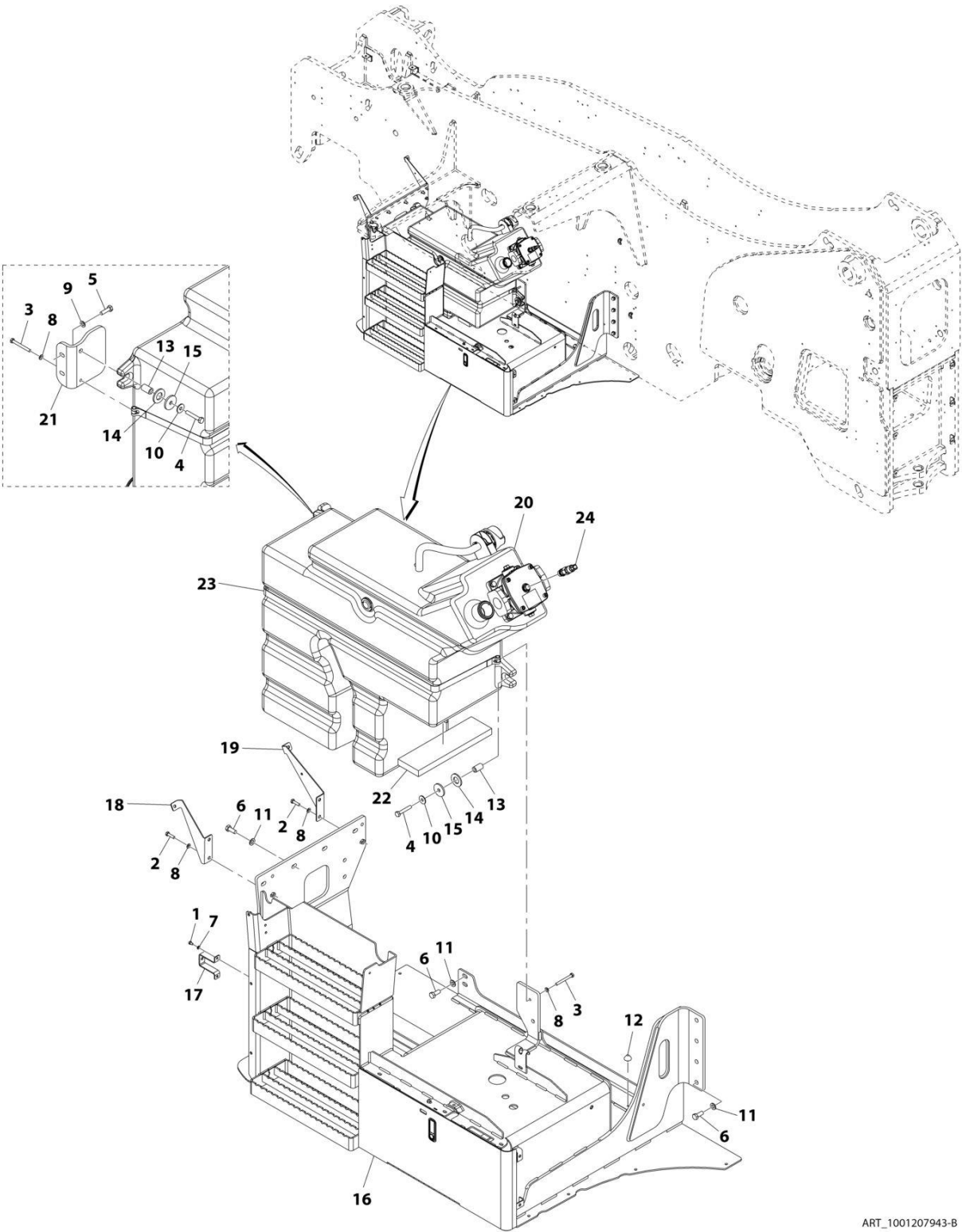
FIGURE 1-8. HYDRAULIC TANK INSTALLATION
