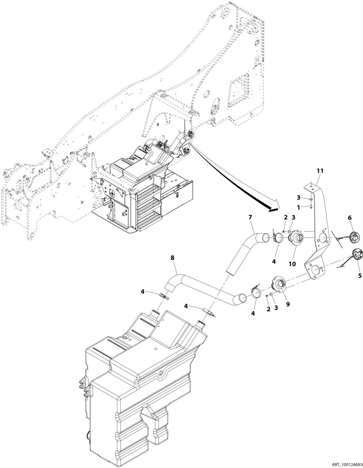
FIGURE 1-12. REMOTE FILL INSTALLATION
