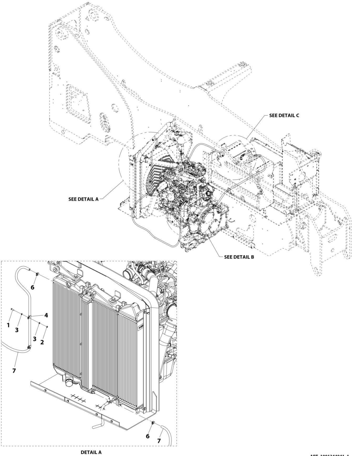
FIGURE 4-9. FUEL LINES INSTALLATION
