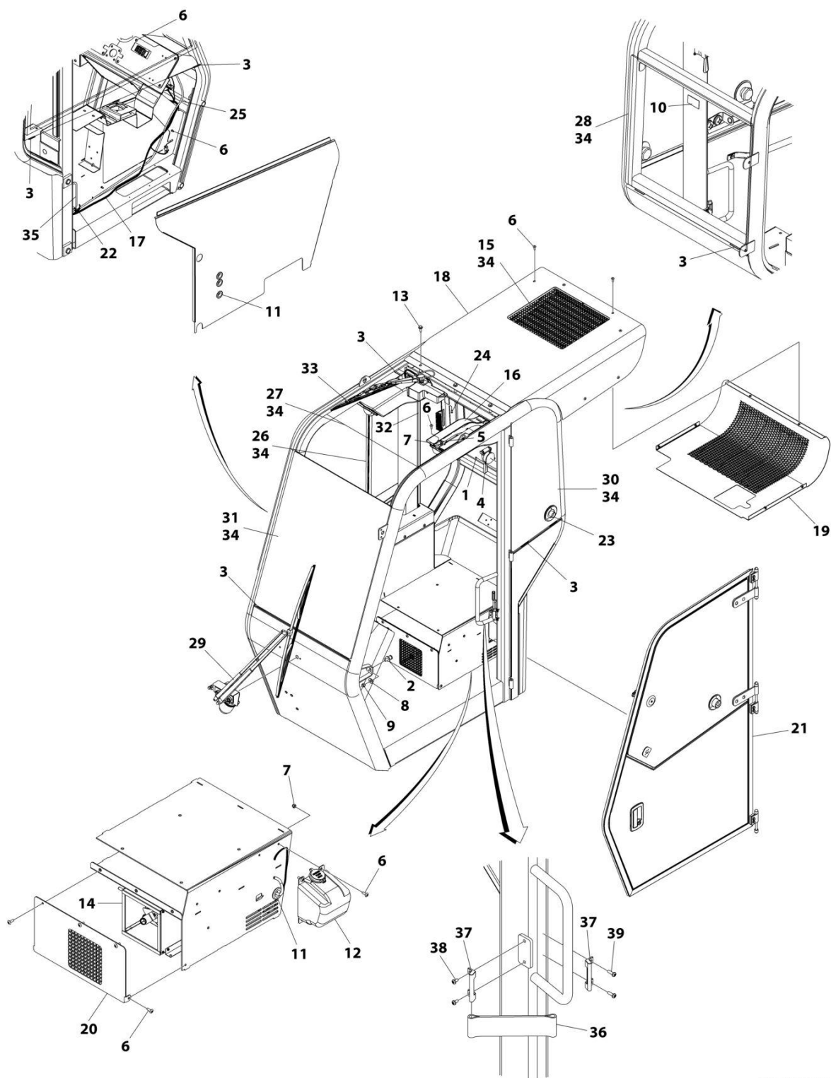
FIGURE 6-10. CAB ENCLOSURE INSTALLATION - WITH HVAC
