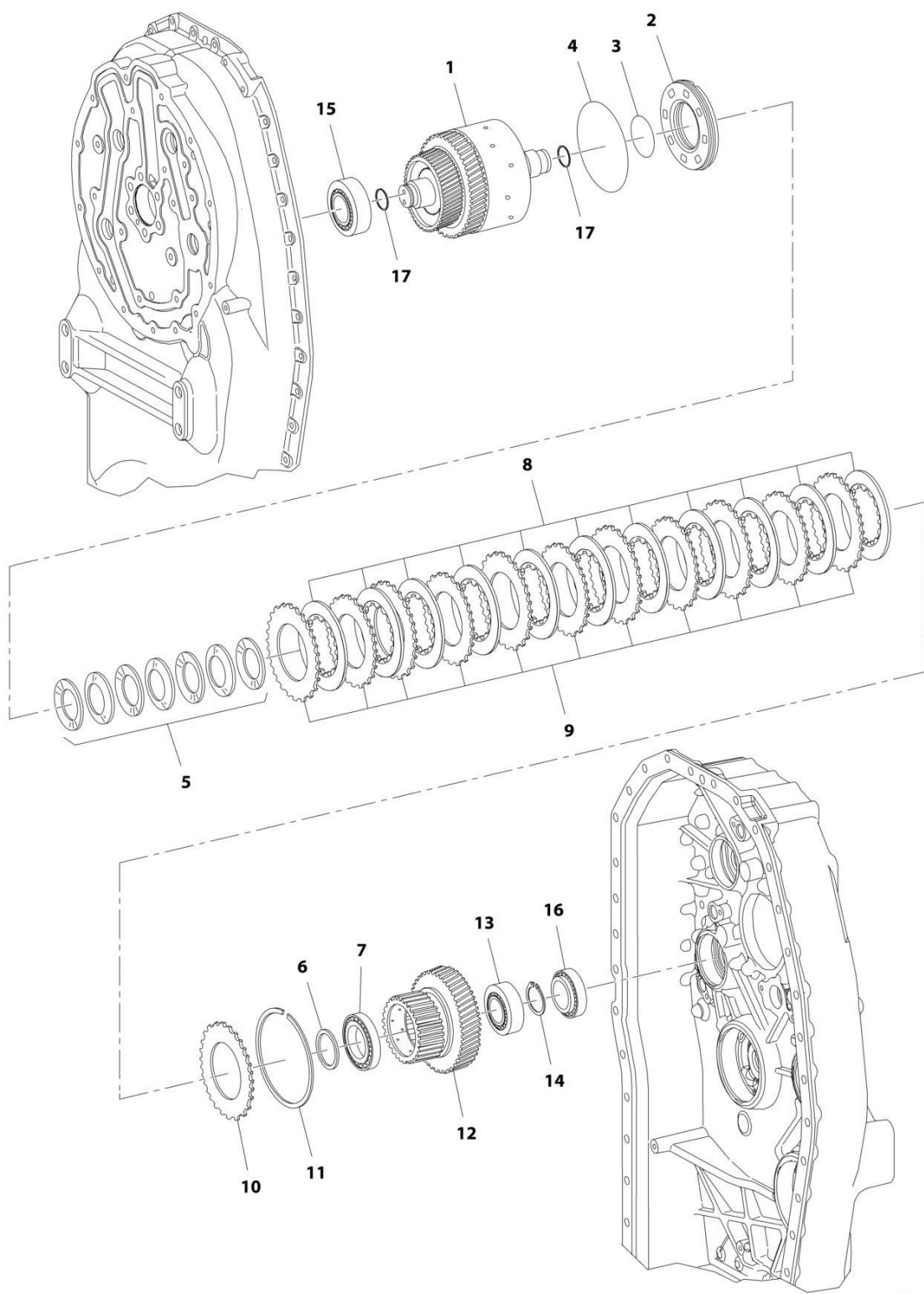
FIGURE 5-14. TRANSMISSION, REVERSING GEAR GROUP 2
