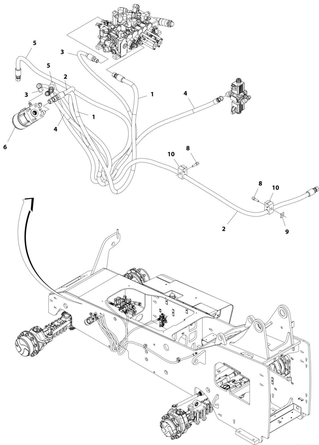
FIGURE 8-26. STEERING HYDRAULICS
