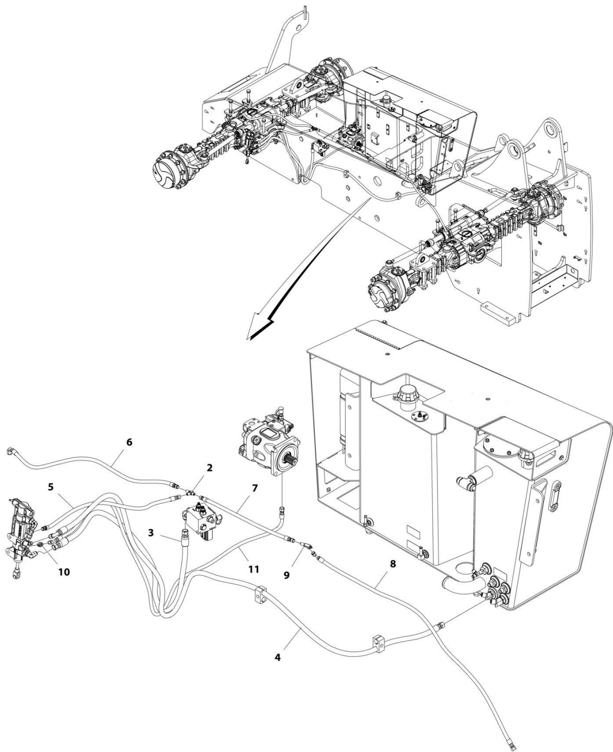
FIGURE 8-9. BRAKE HYDRAULICS
