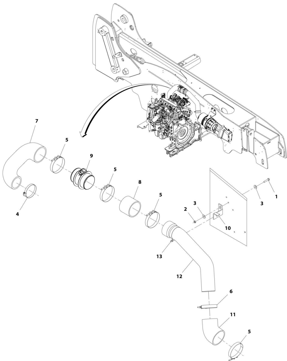
FIGURE 4-15. AIR CLEANER LINES INSTALLATION (ULS)
