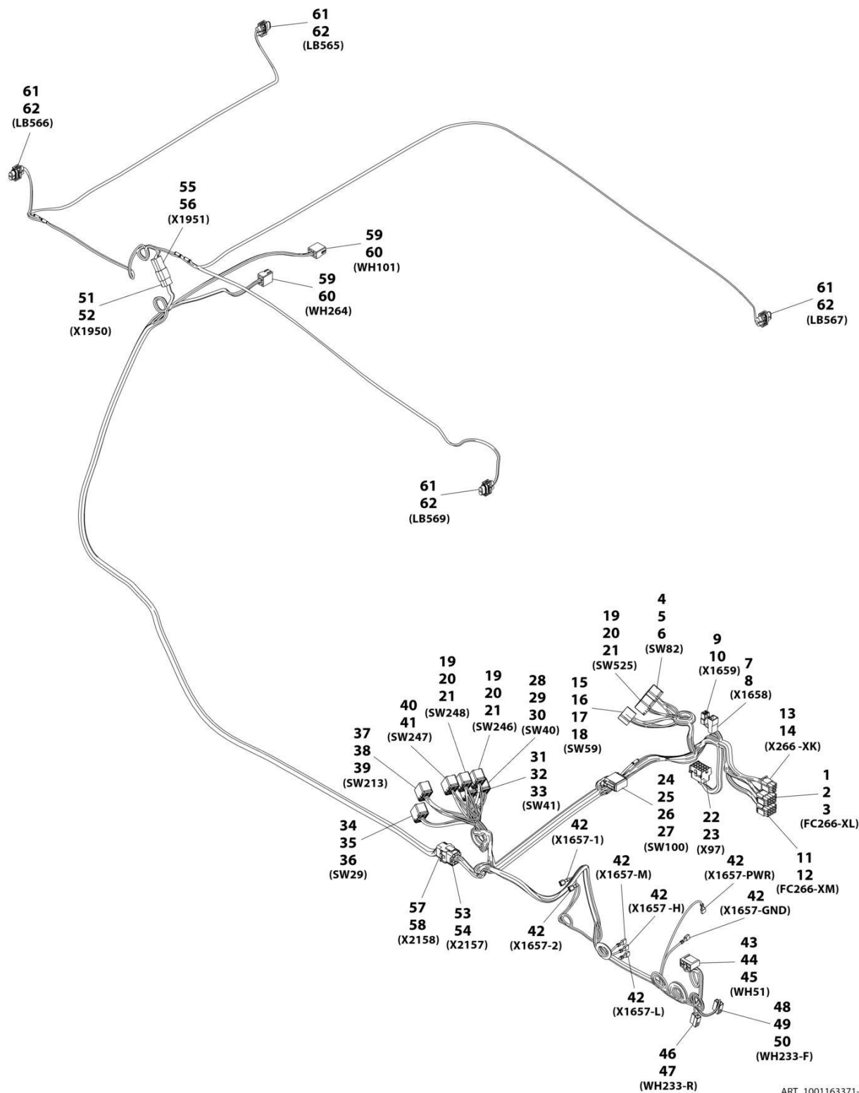
FIGURE 10-34. CAB OPTION 1 HARNESS
