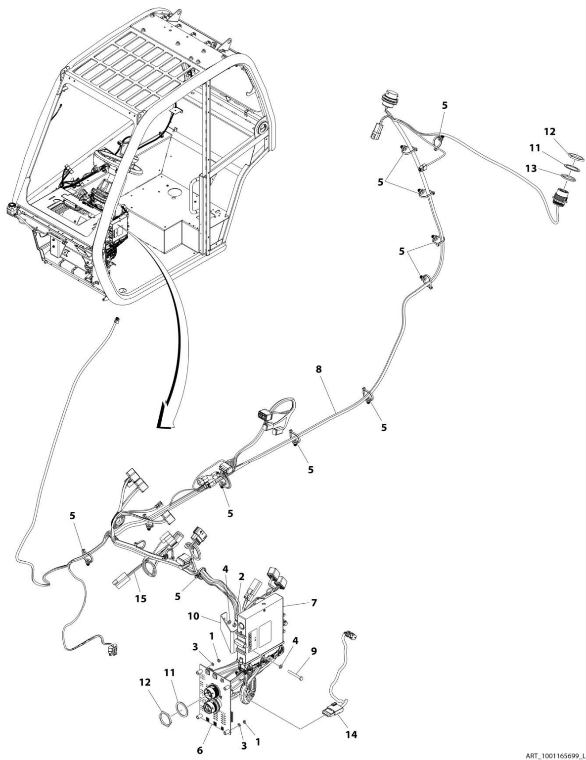
FIGURE 10-24. CAB ELECTRICAL INSTALLATION (SN 016011822 to Present)
