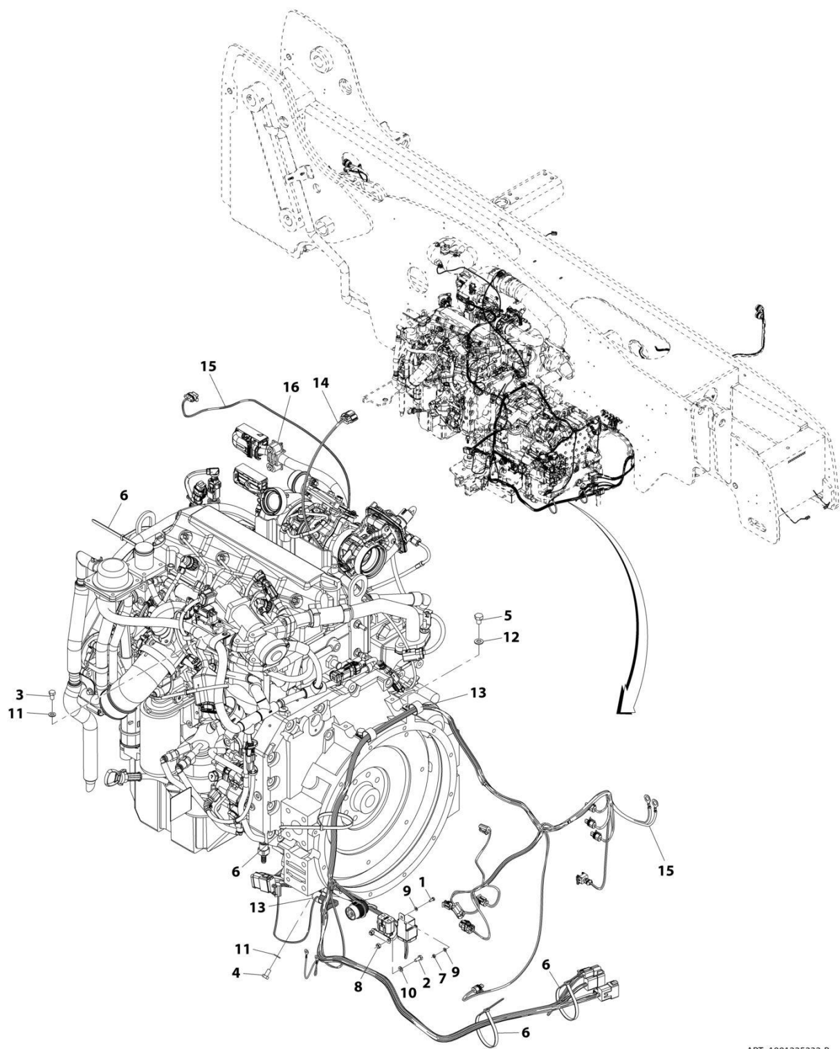
FIGURE 10-48. ENGINE - WIRING INSTALLATION (74HP) (ULS)
