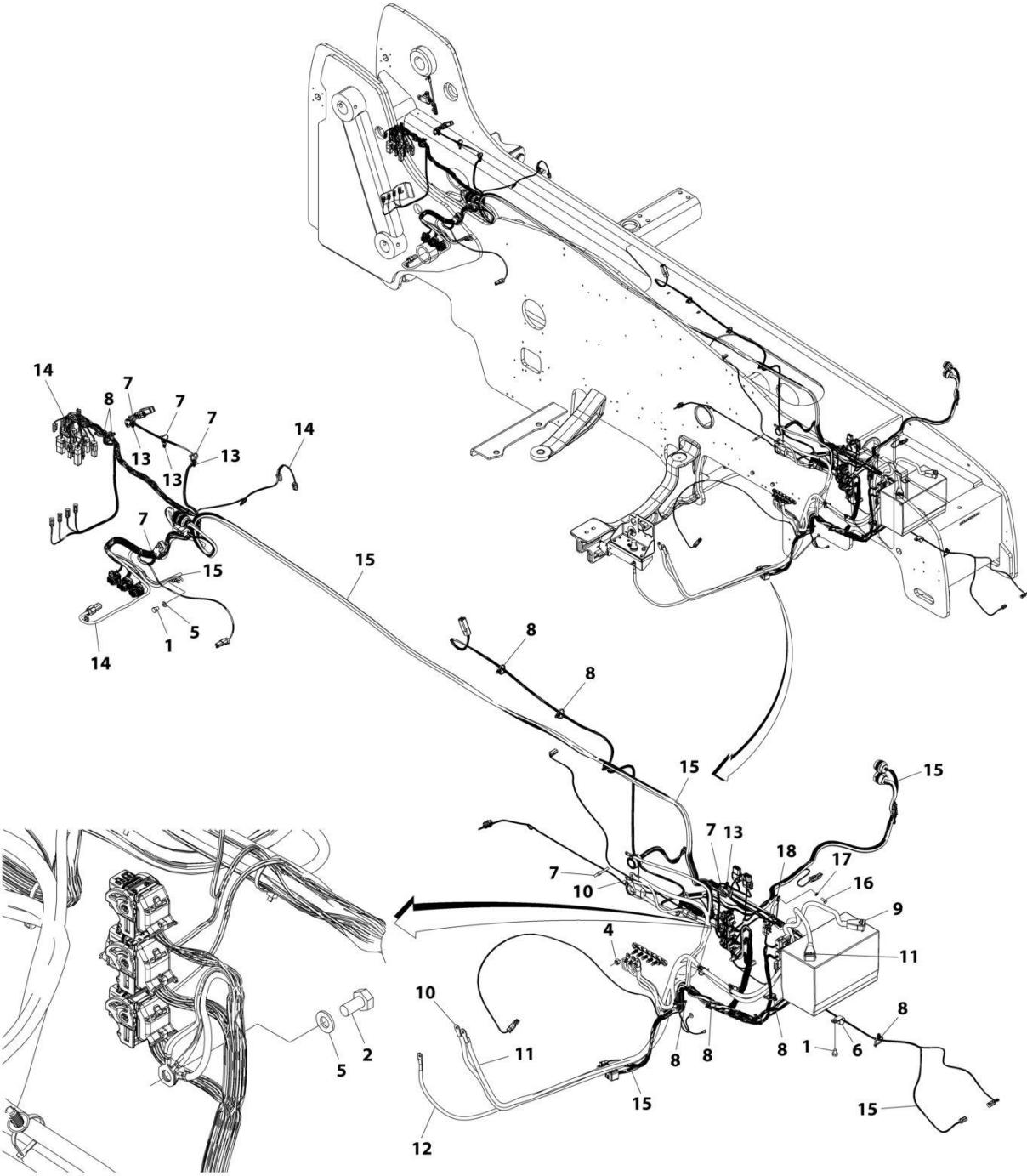
FIGURE 10-67. FRAME - WIRING INSTALLATION (74HP) (ULS)
