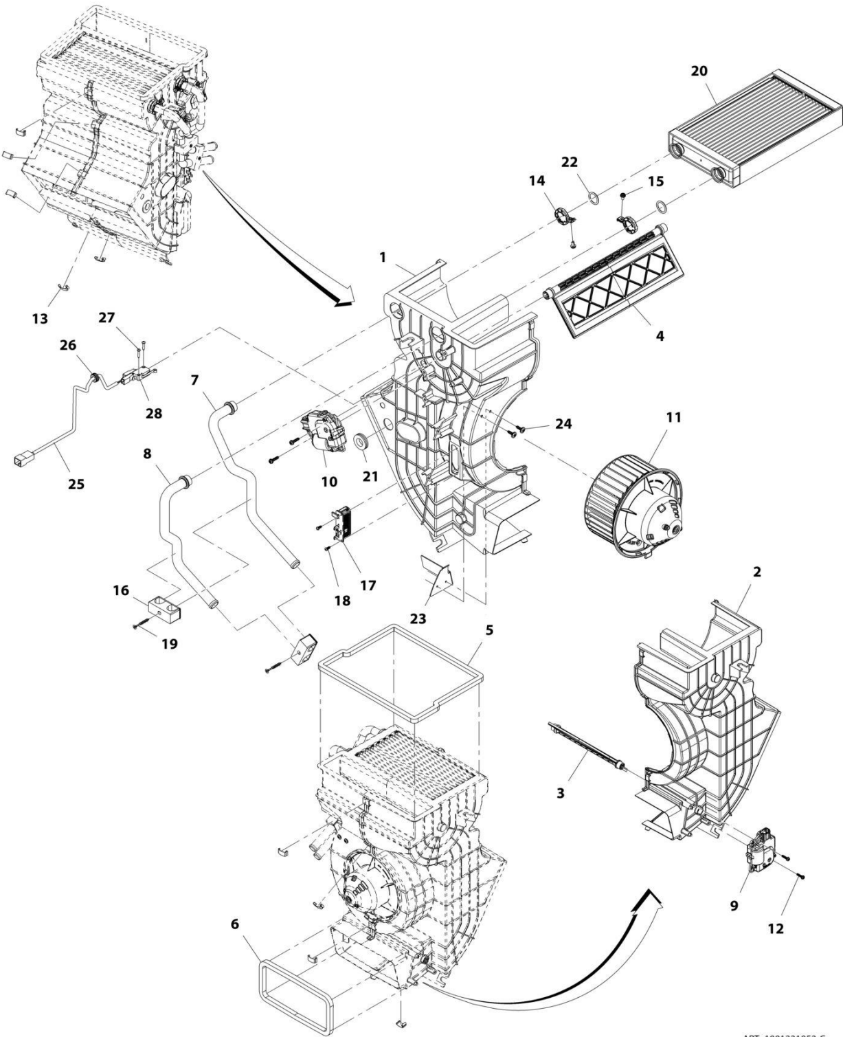
FIGURE 6-46. HEATER (Prior to SN 0160110882)
