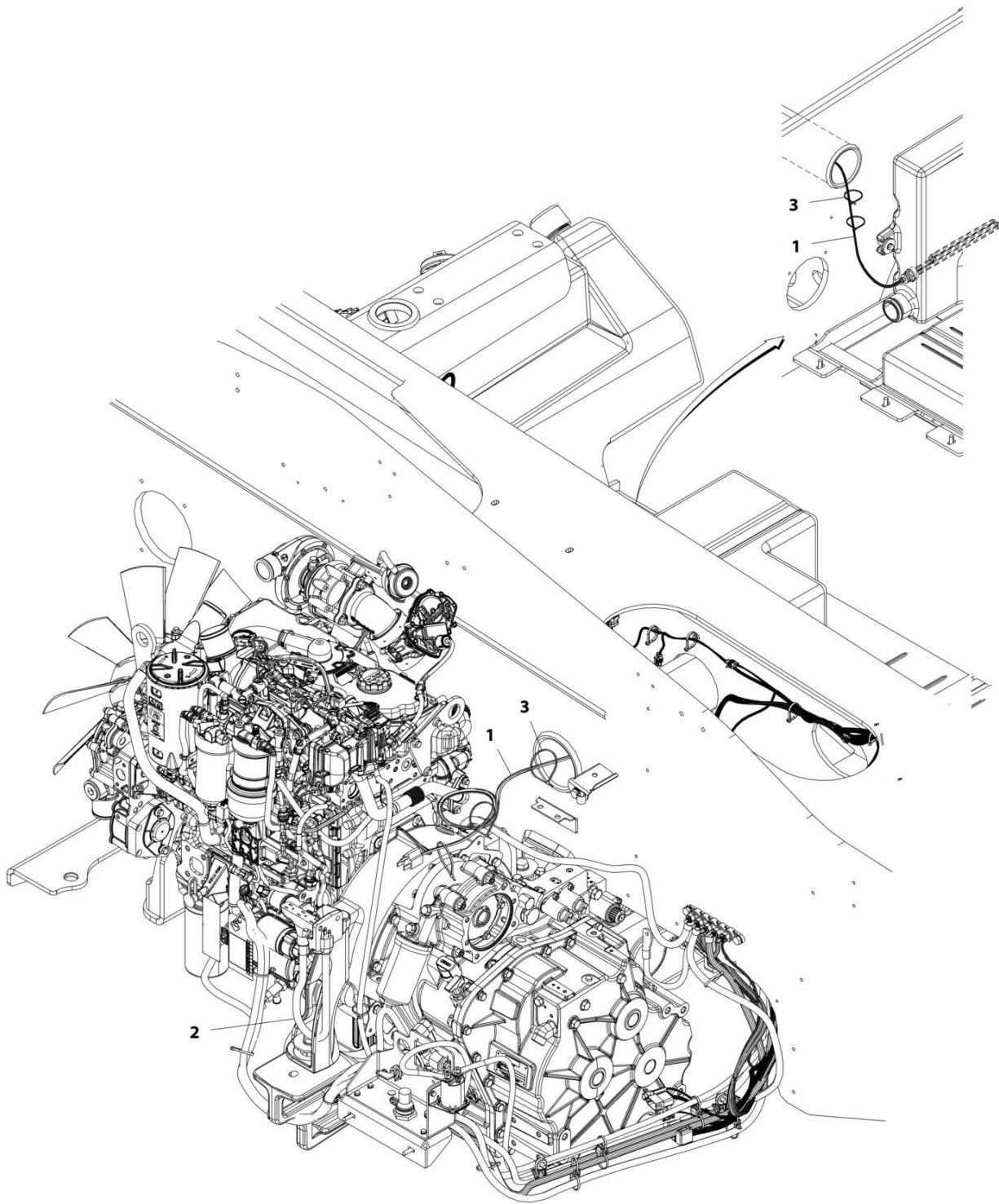
FIGURE 10-77. HEATER HARNESS - HYDRAULIC TANK
