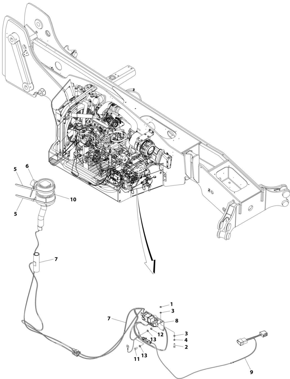
FIGURE 10-75. HEATER HARNESS - CUMMINS BREATHER (110HP) (ULS)
