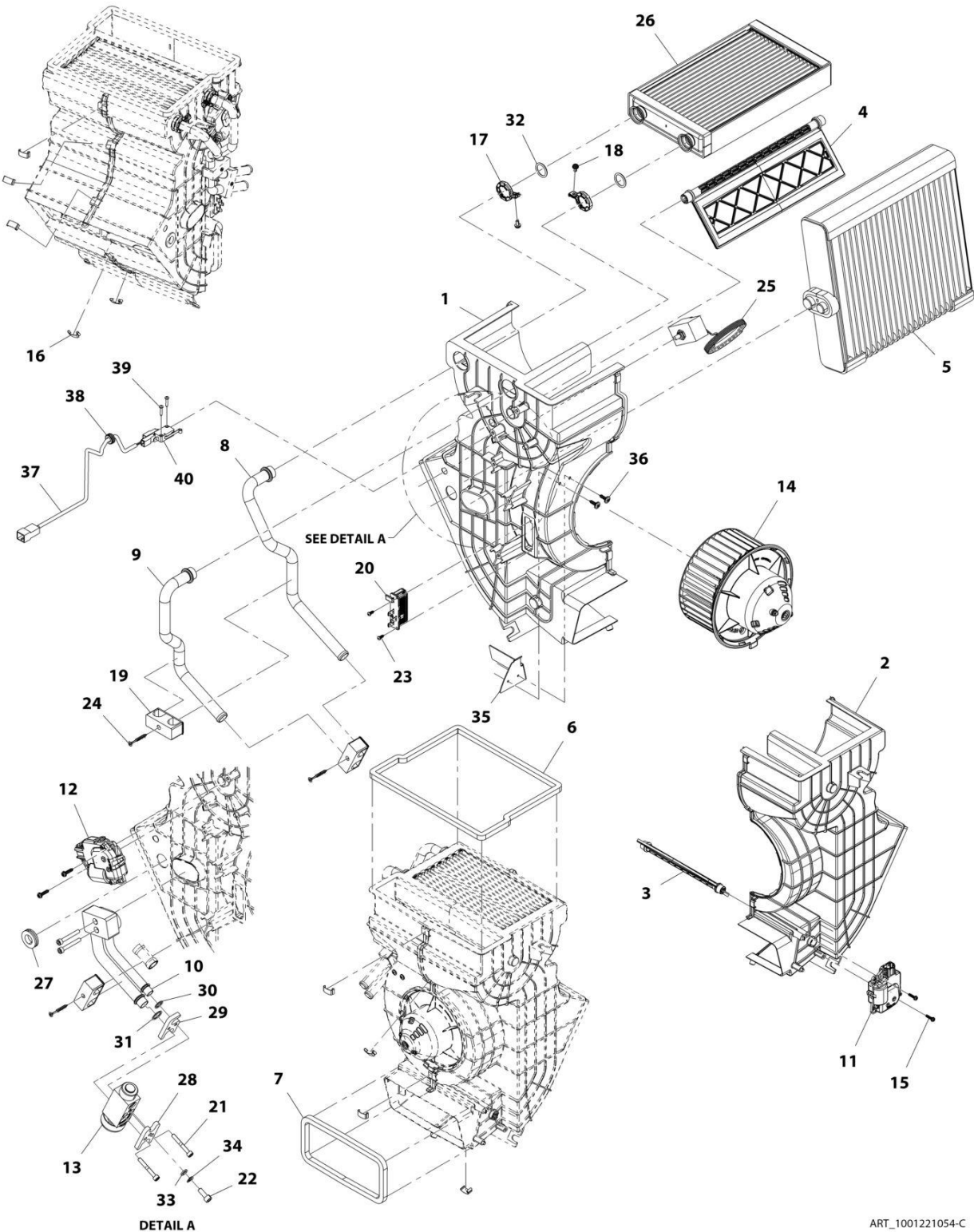
FIGURE 6-50. HEATER AND A/C (Prior to SN 0160110882)
