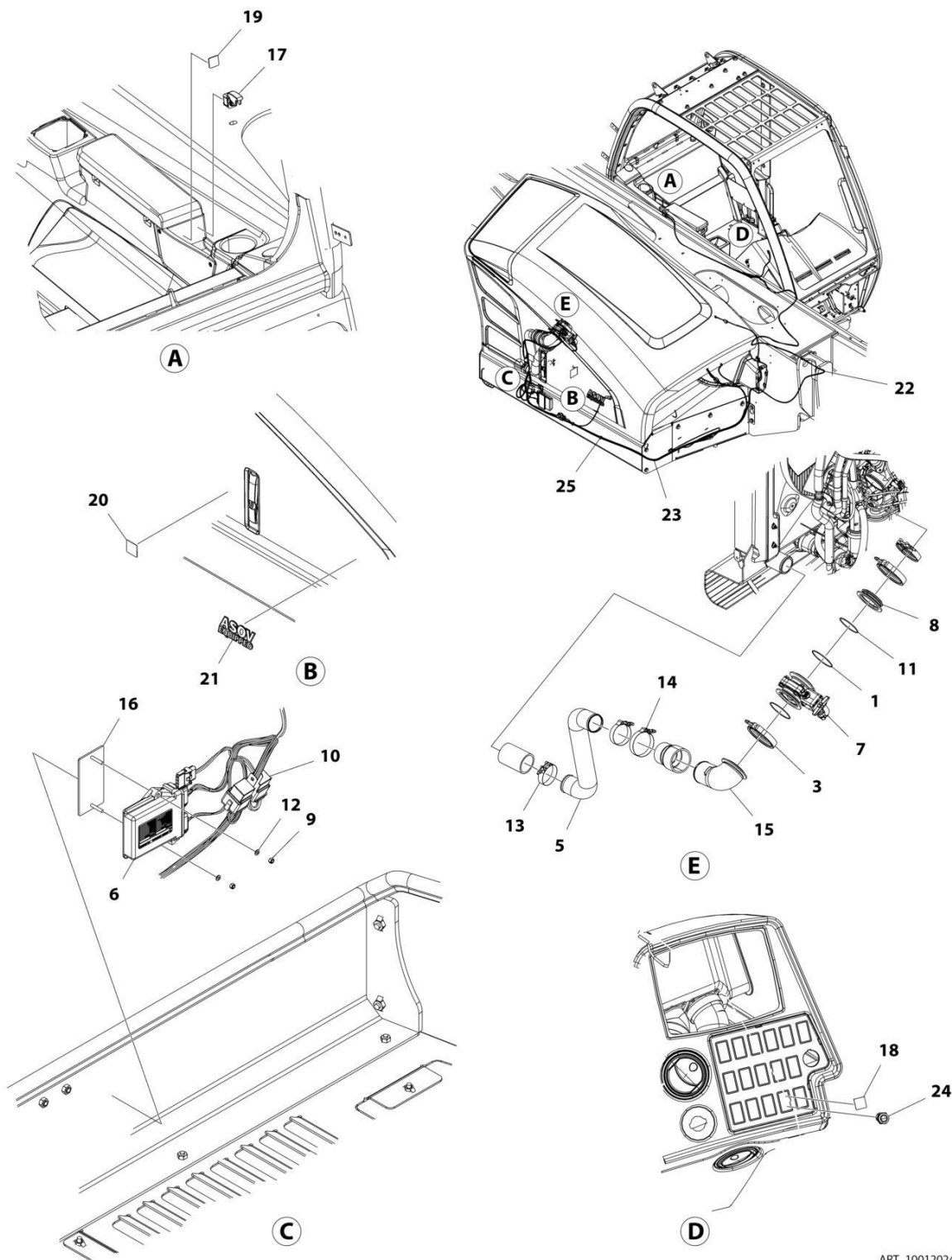
FIGURE 4-17. AIR INTAKE SHUT OFF VALVE INSTALLATION
