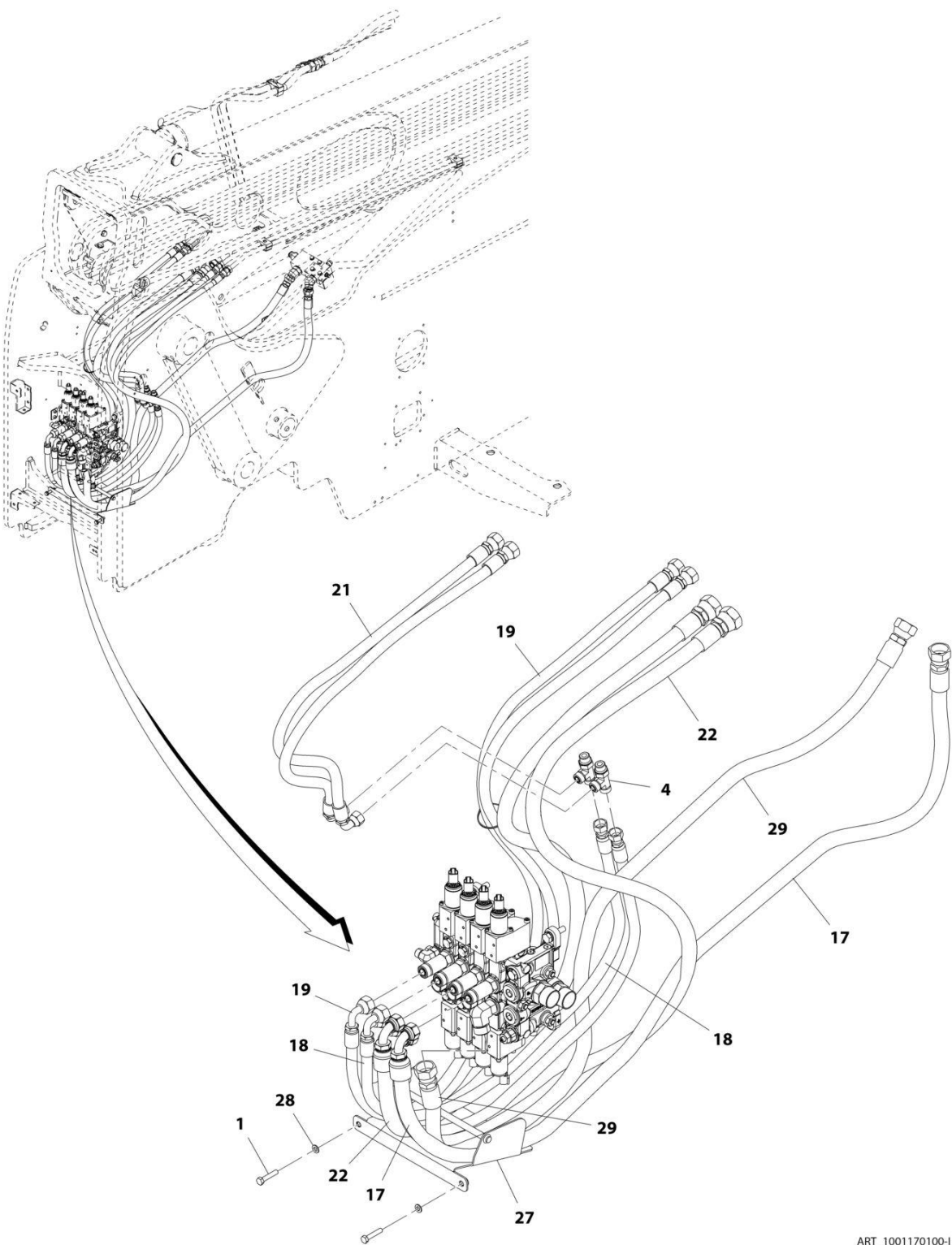
FIGURE 8-3. BOOM HYDRAULIC INSTALLATION
