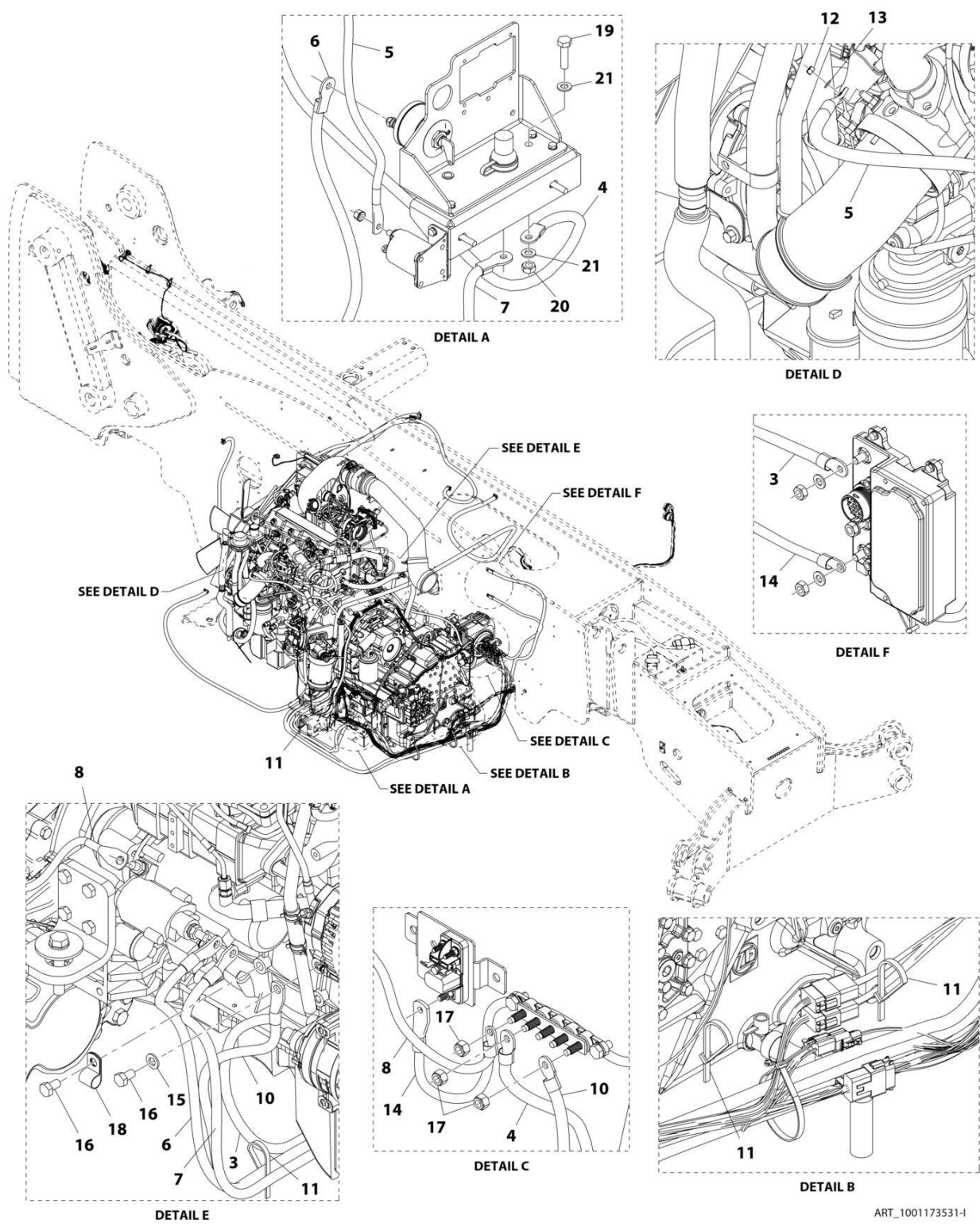
FIGURE 10-58. ENGINE BAY - WIRING INSTALLATION (110HP) (ULS)
