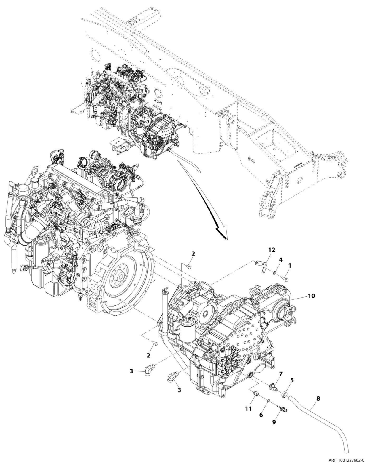
FIGURE 5-1. TRANSMISSION INSTALLATION, 74 HP
