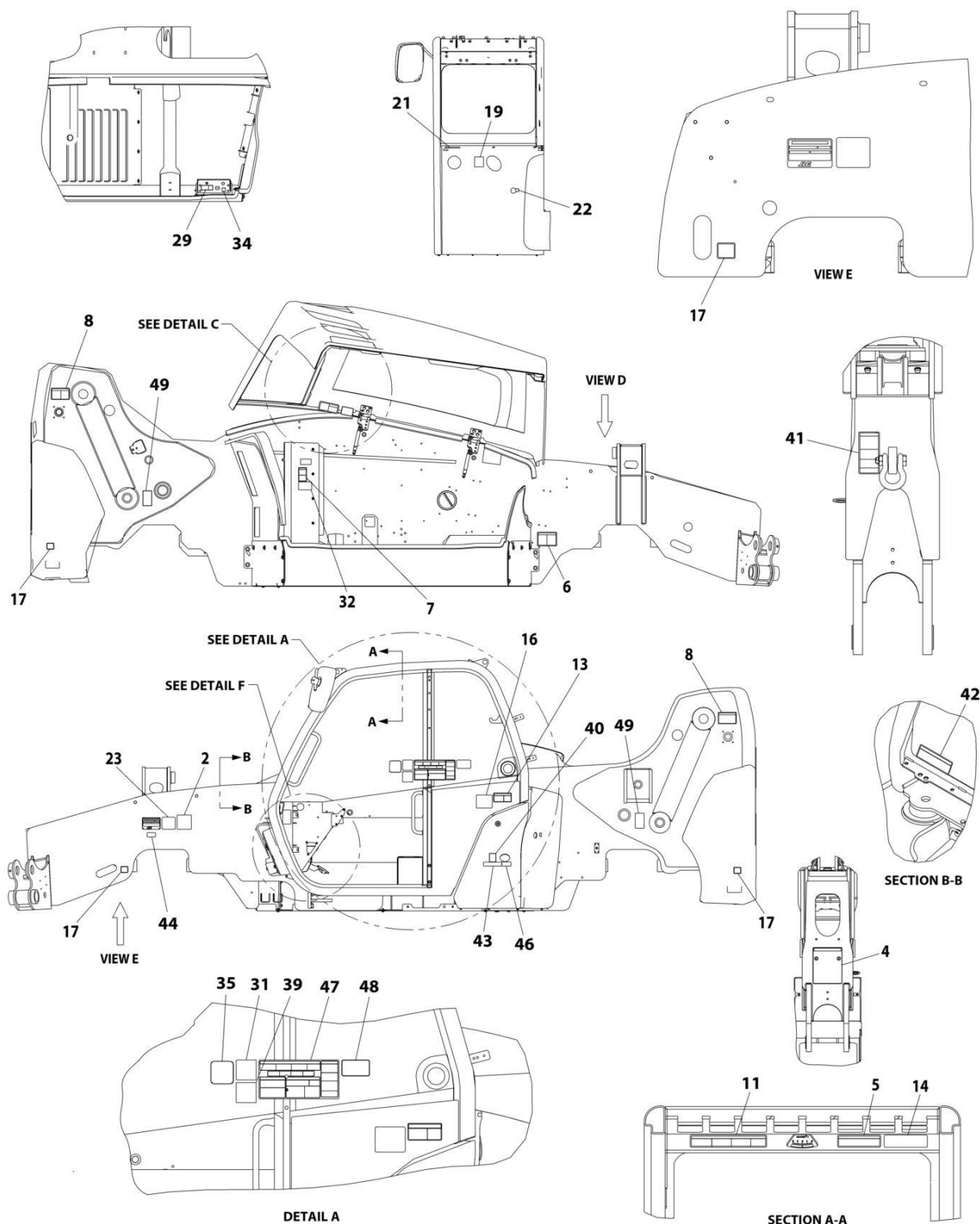
FIGURE 11-2. DECAL INSTALLATION (ANSI) (110 HP)
