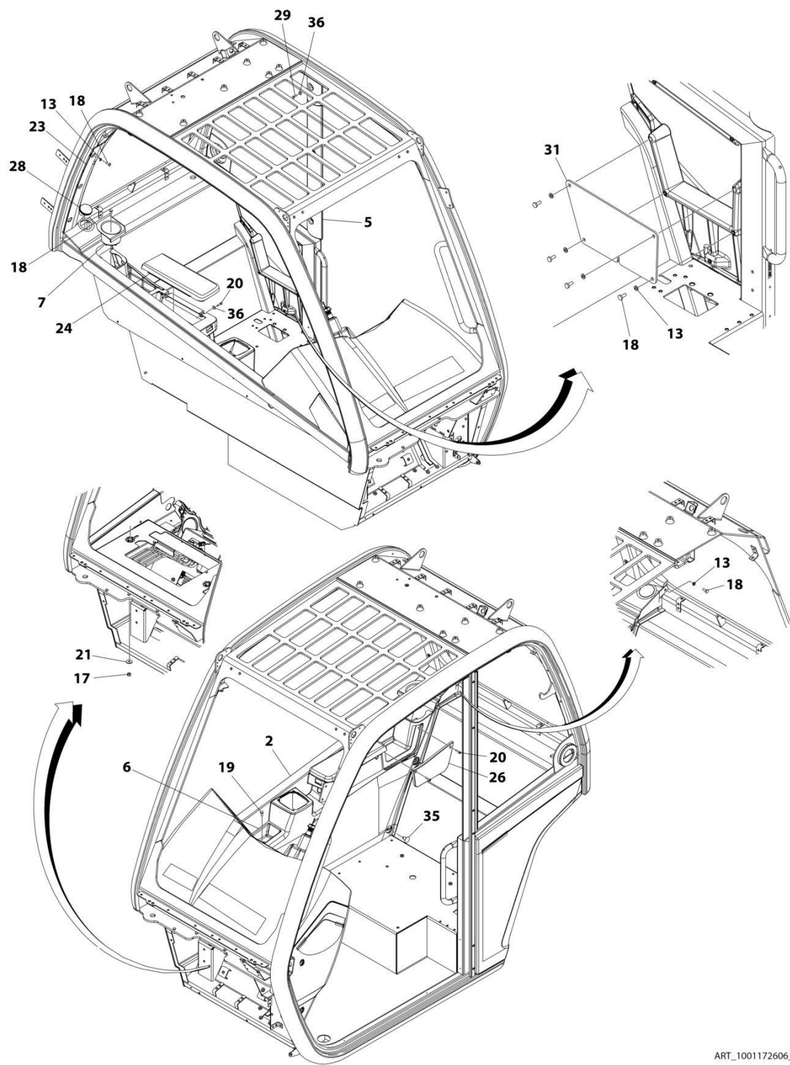
FIGURE 6-60. TRIM INSTALLATION - OPEN CAB
