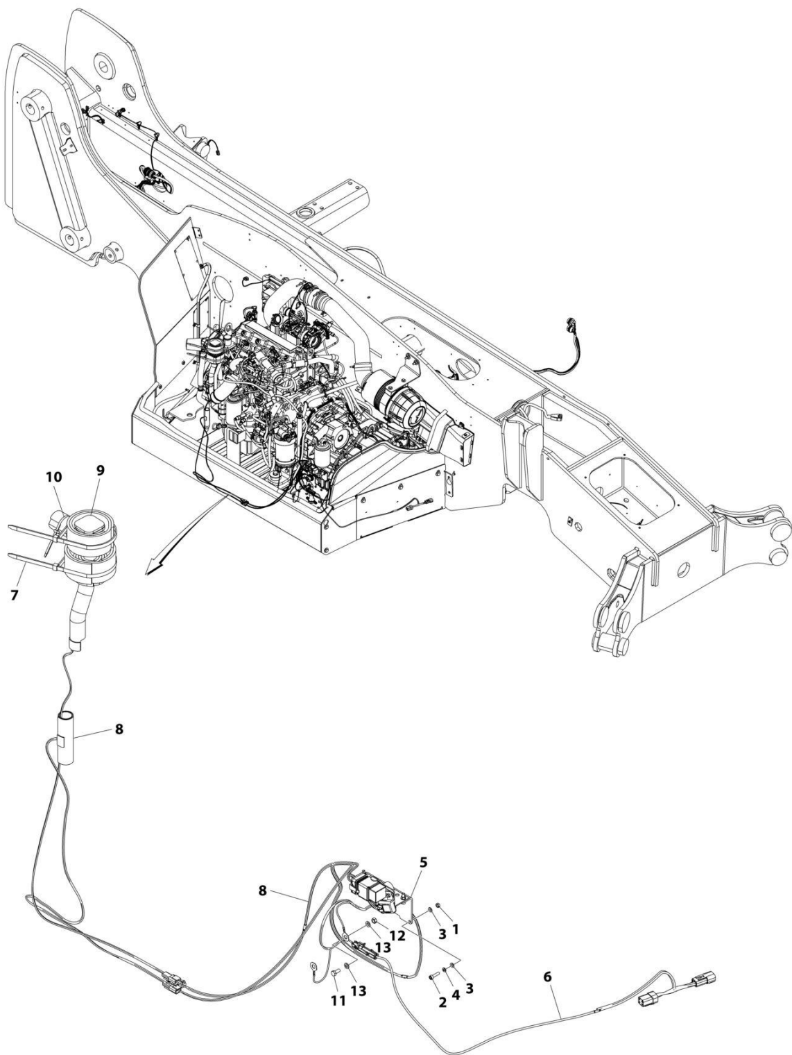
FIGURE 4-18. HEATER BREATHER - 74 HP
