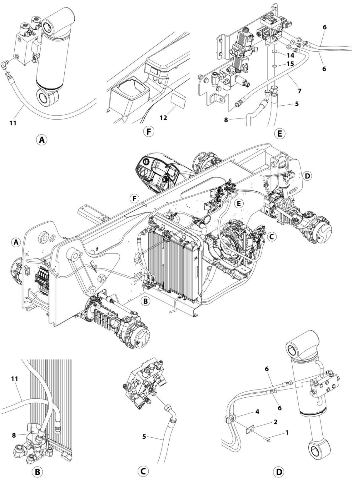
FIGURE 8-16. FRAME LEVEL HYDRAULICS INSTALLATION (NO OUTRIGGERS)
