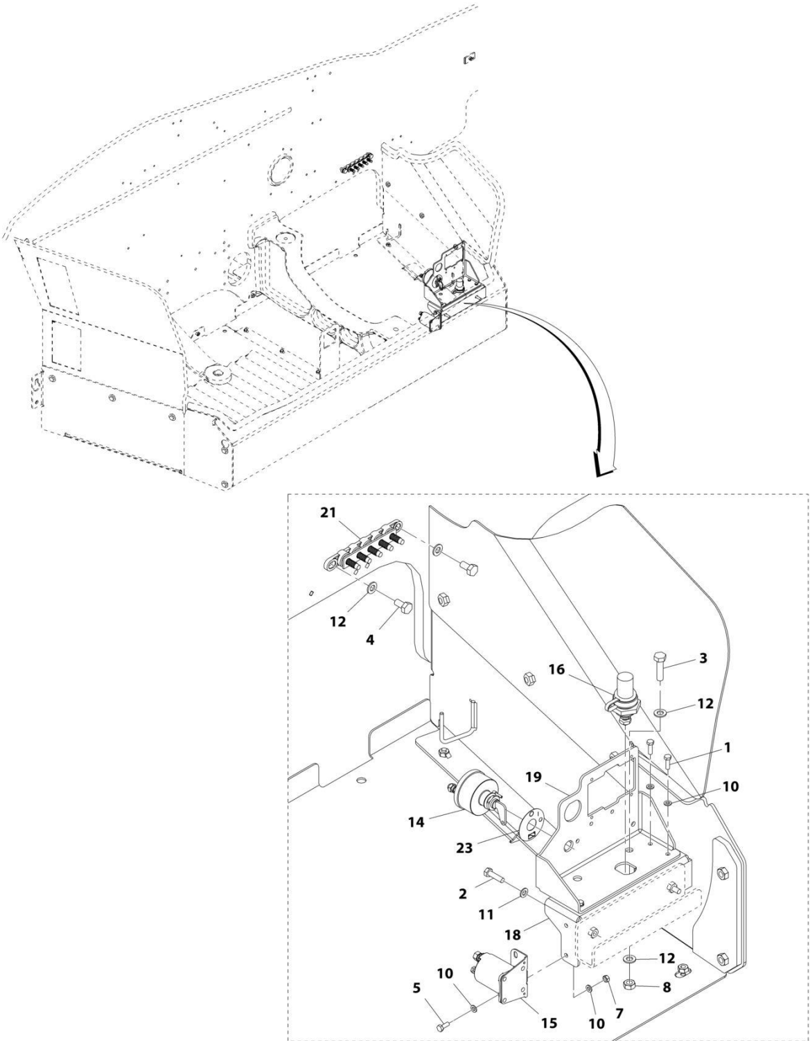
FIGURE 10-56. ENGINE BAY - ELECTRICAL INSTALLATION (110HP) (LS)
