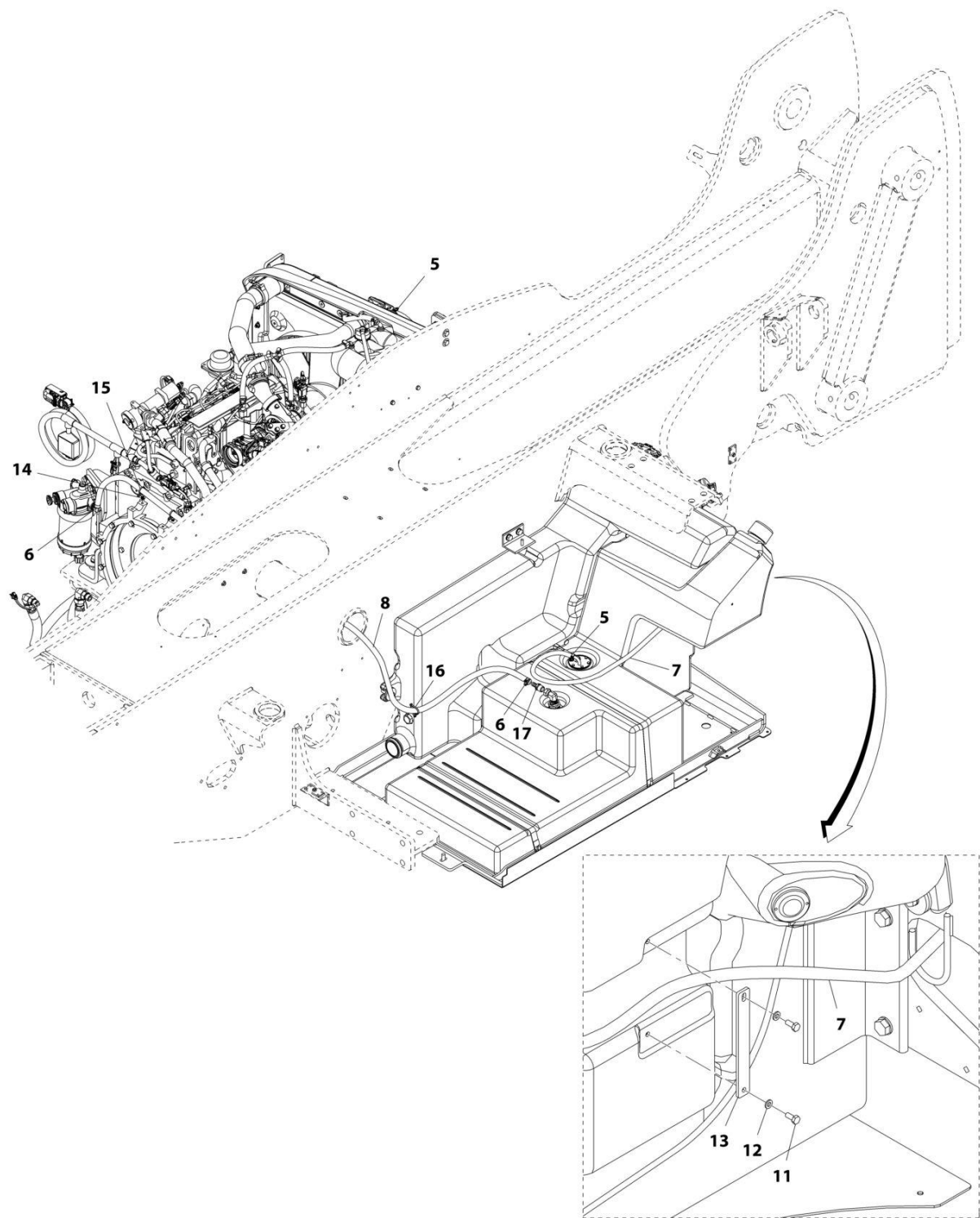
FIGURE 4-33. FUEL LINES INSTALLATION (LS)
