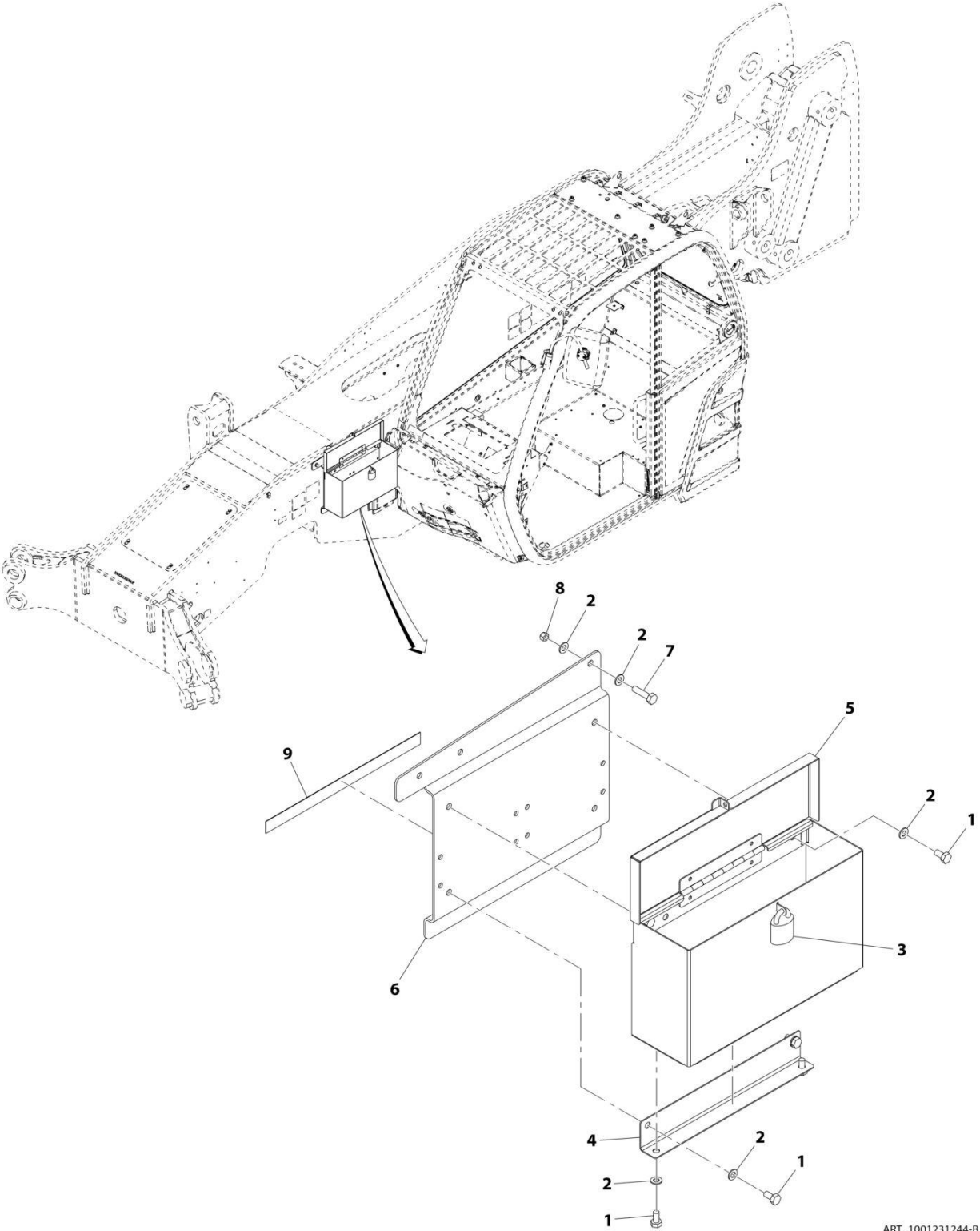
FIGURE 5-78. TOOLBOX INSTALLATION
