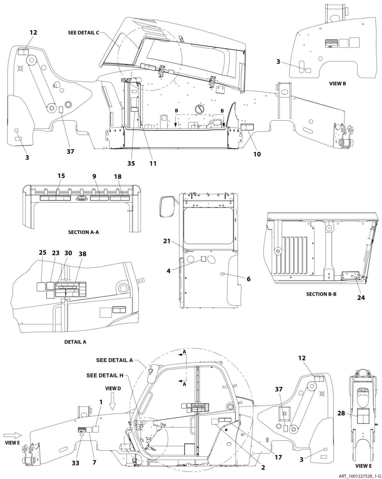
FIGURE 11-3. DECAL INSTALLATION (CSA ENGLISH/FRENCH) (74 HP)
