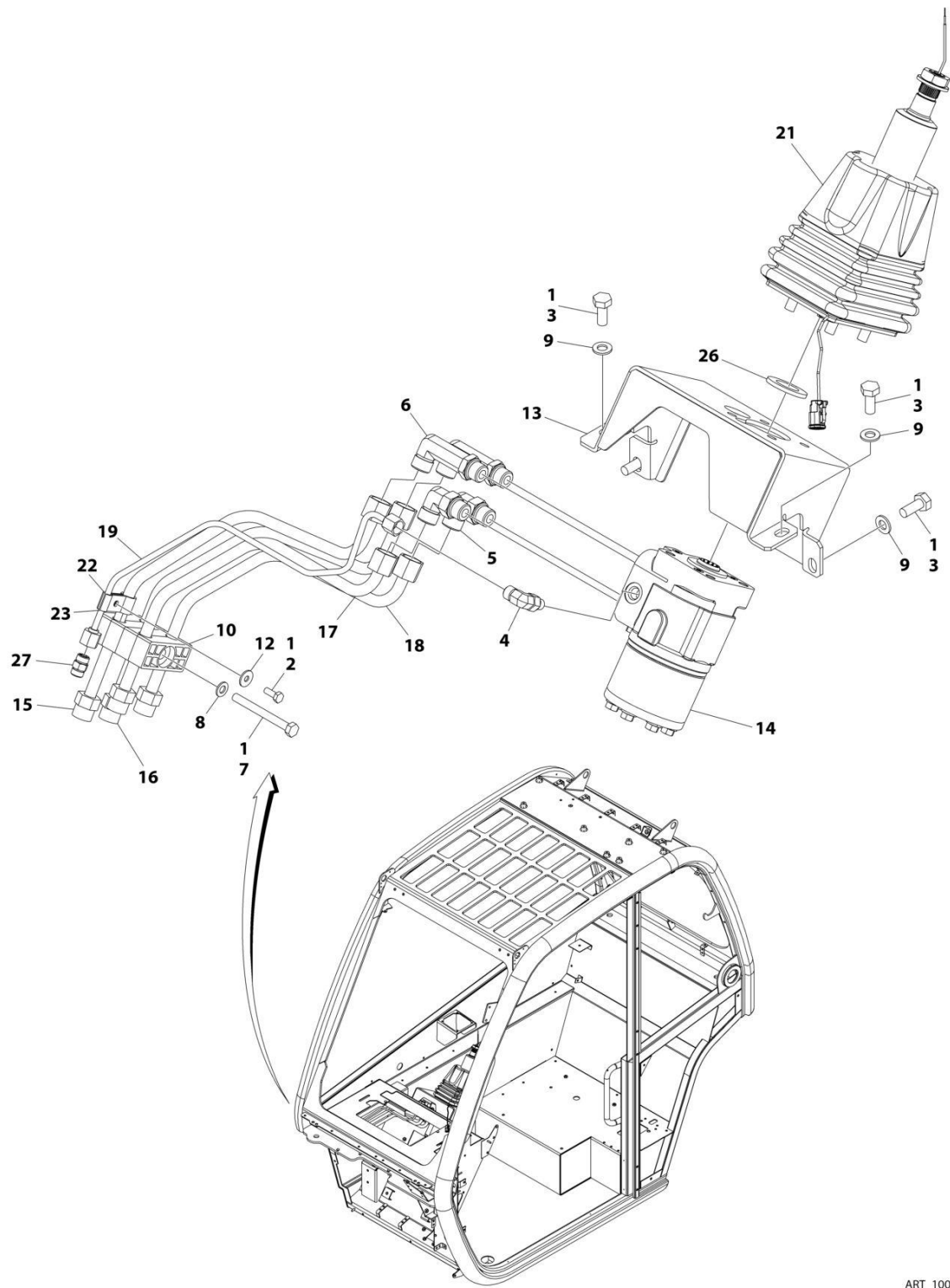
FIGURE 7-10. STEERING COLUMN INSTALLATION
