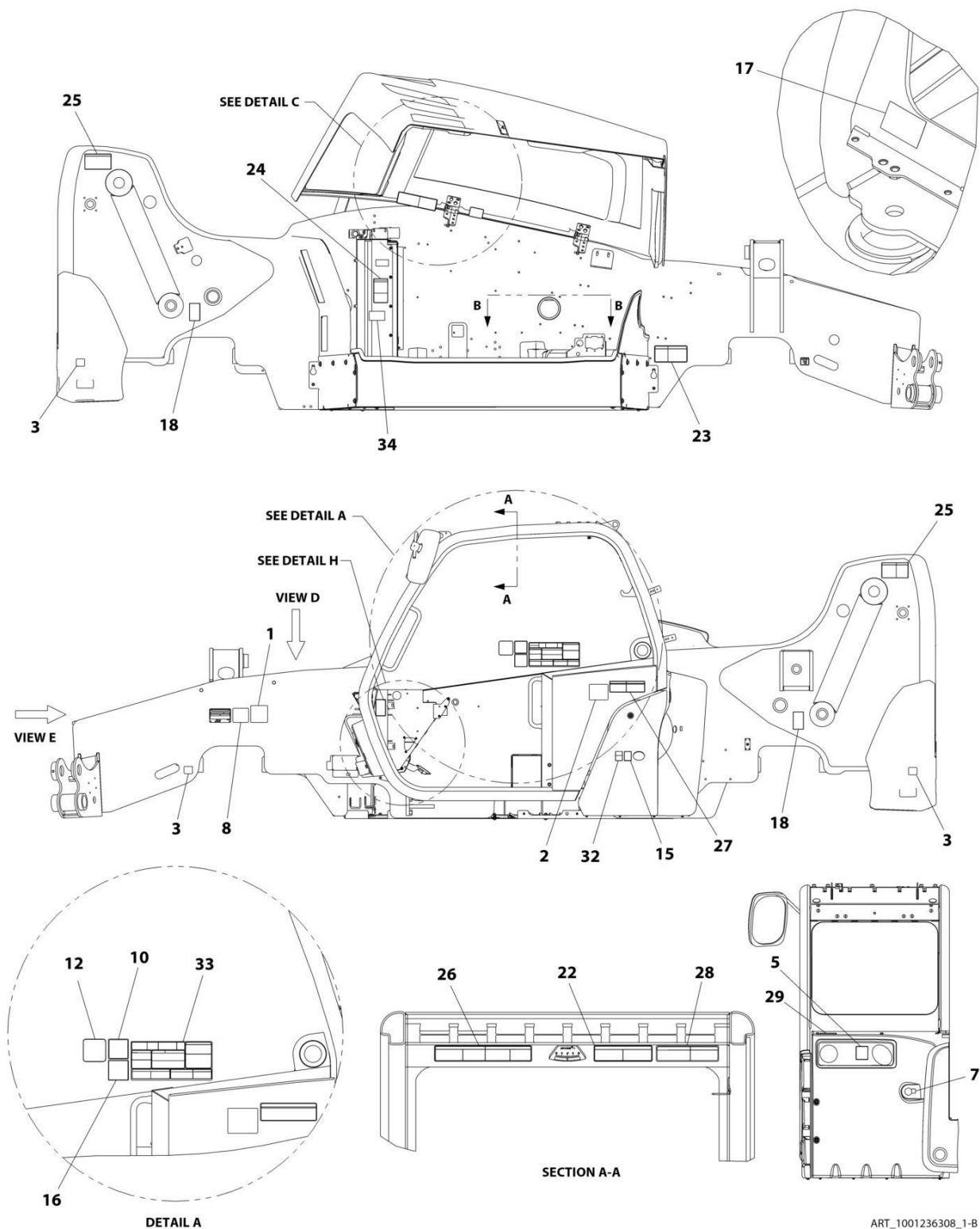
FIGURE 11-8. DECAL INSTALLATION (LATIN AMERICAN ENGLISH/SPANISH) (110HP)
