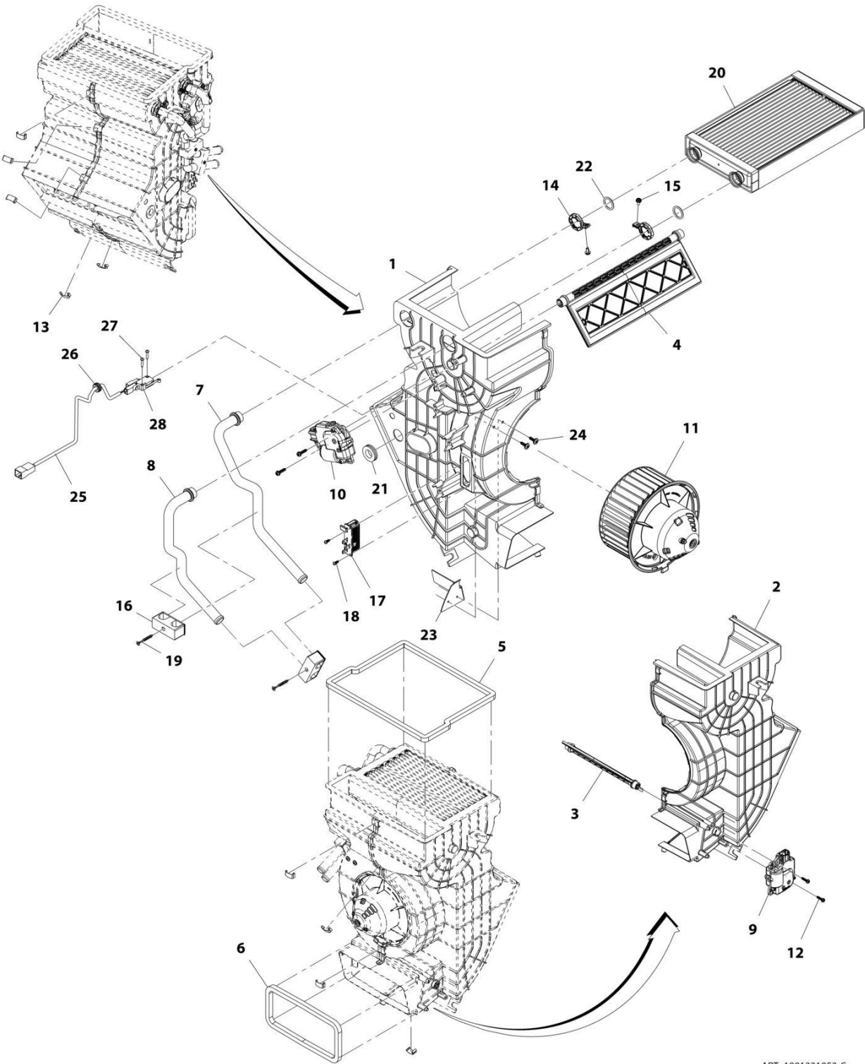
FIGURE 6-46. HEATER (Prior to SN 0160111362)
