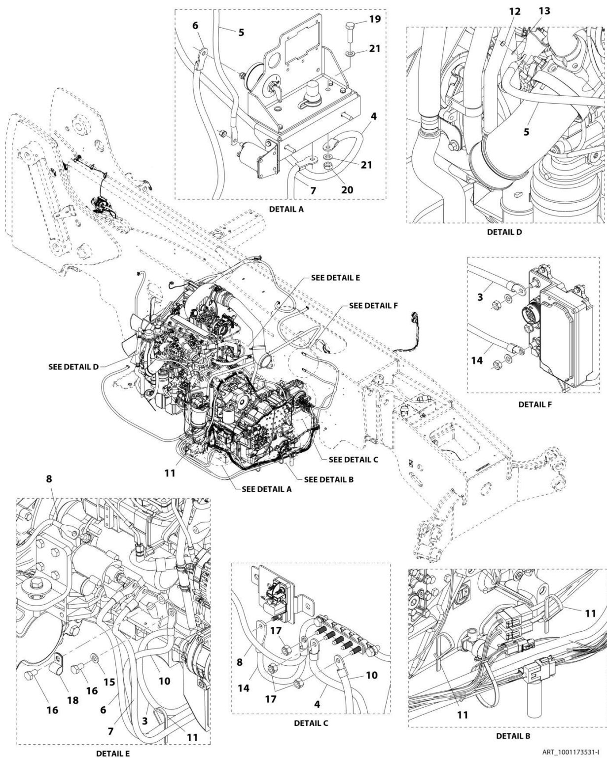
FIGURE 10-53. ENGINE BAY - WIRING INSTALLATION (ULS)
