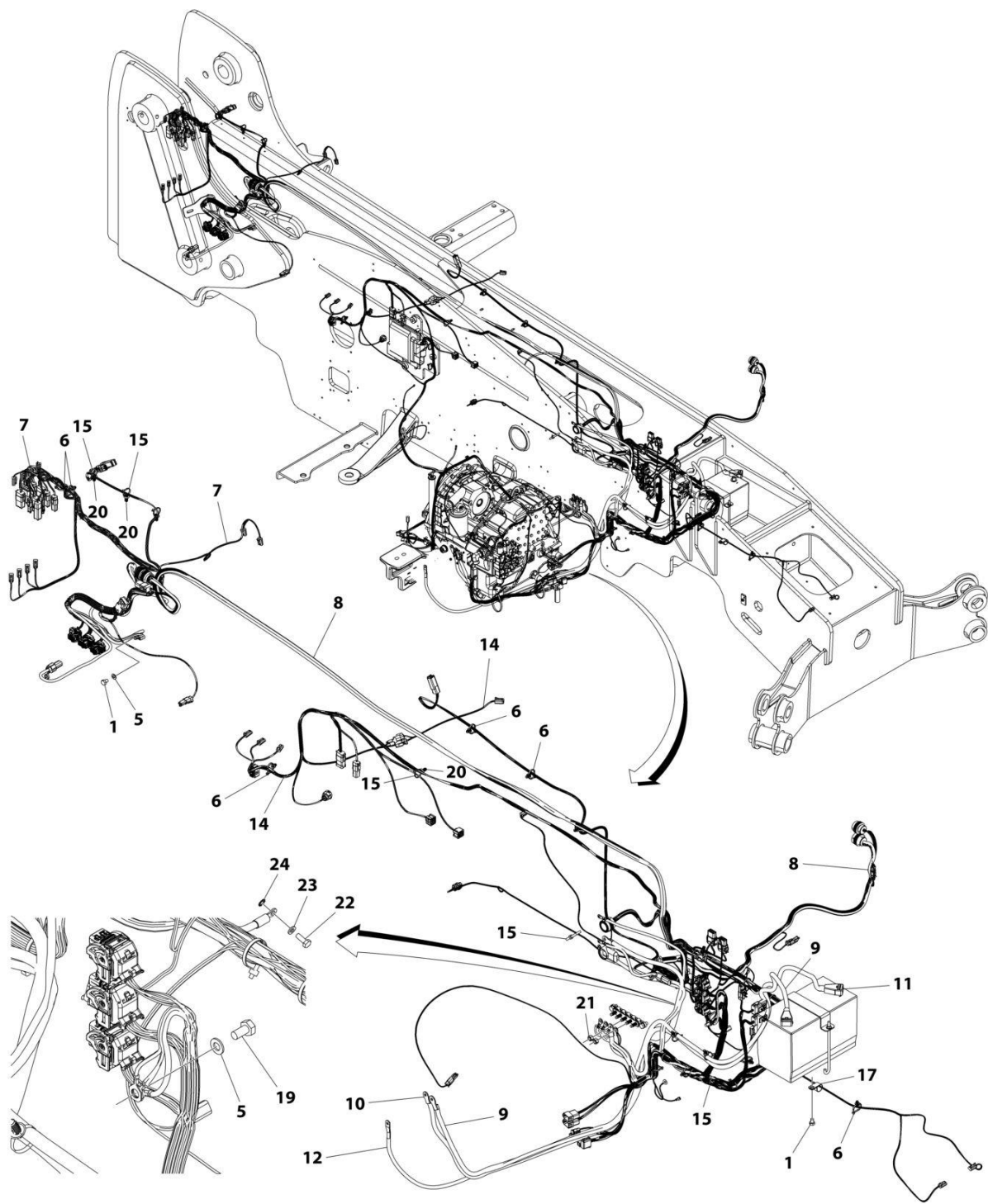
FIGURE 10-62. FRAME - WIRING INSTALLATION (ULS)
