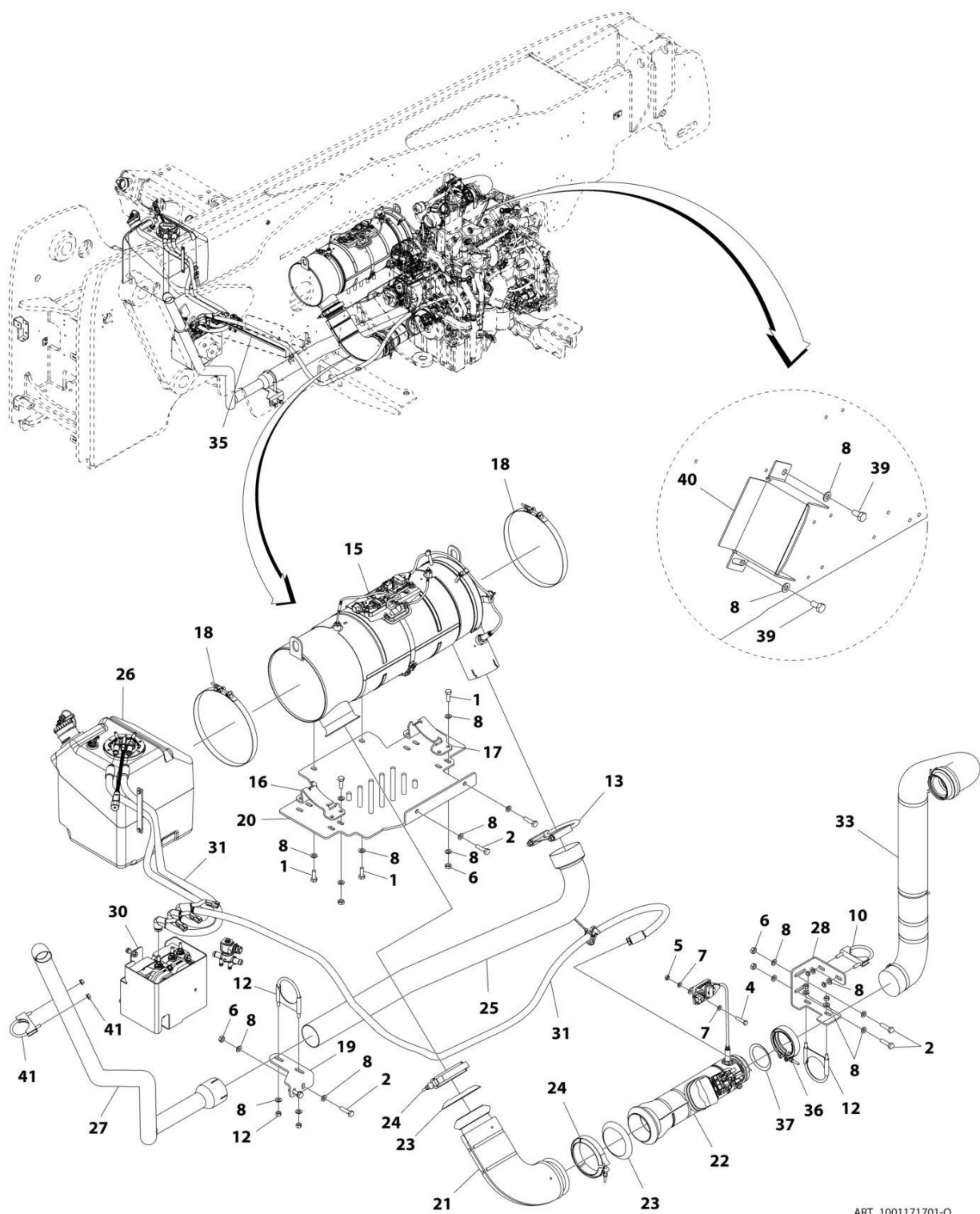
FIGURE 4-16. EXHAUST INSTALLATION, 110HP (ULS)
