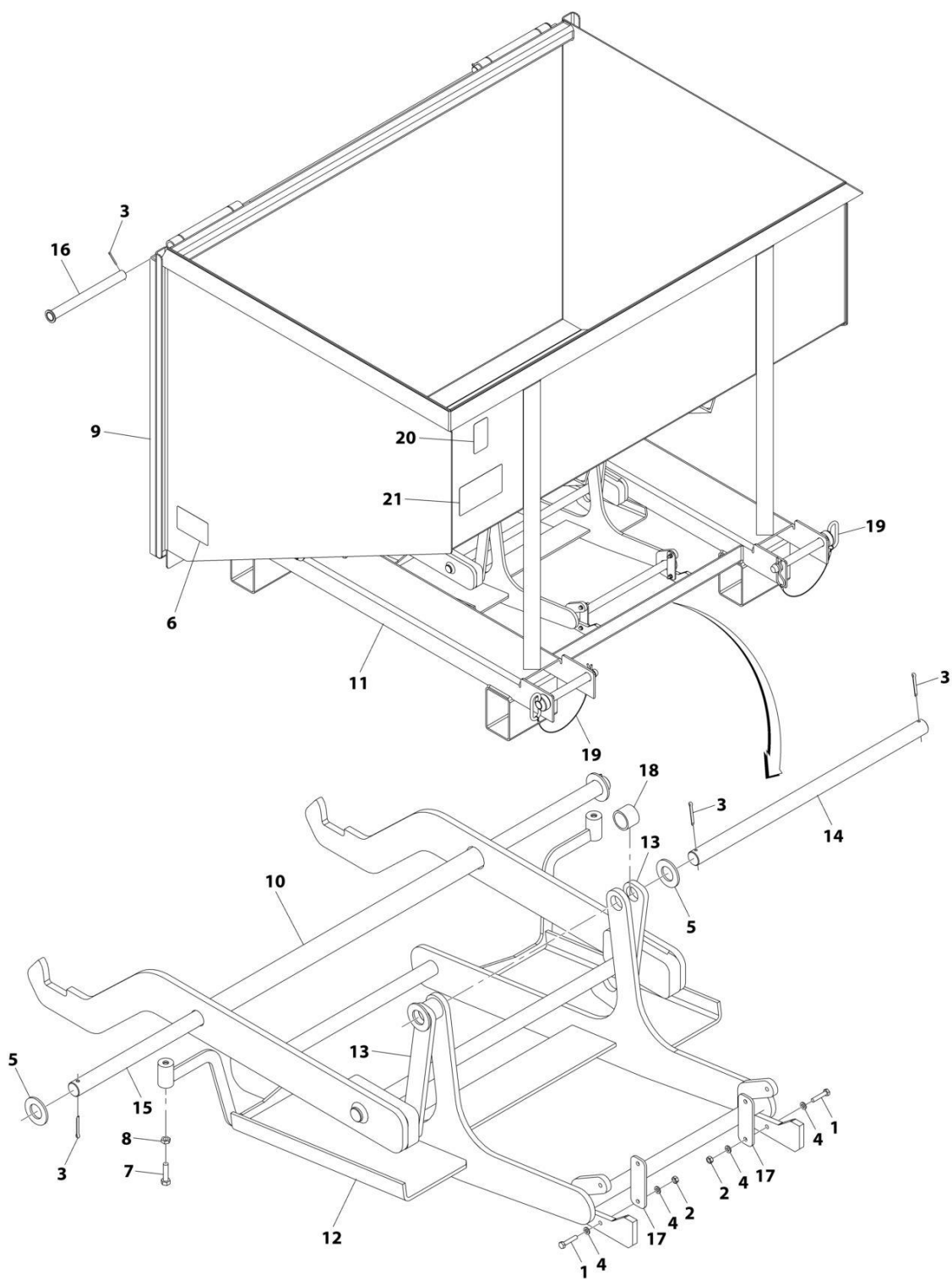
FIGURE 3-61. TRASH HOPPER
