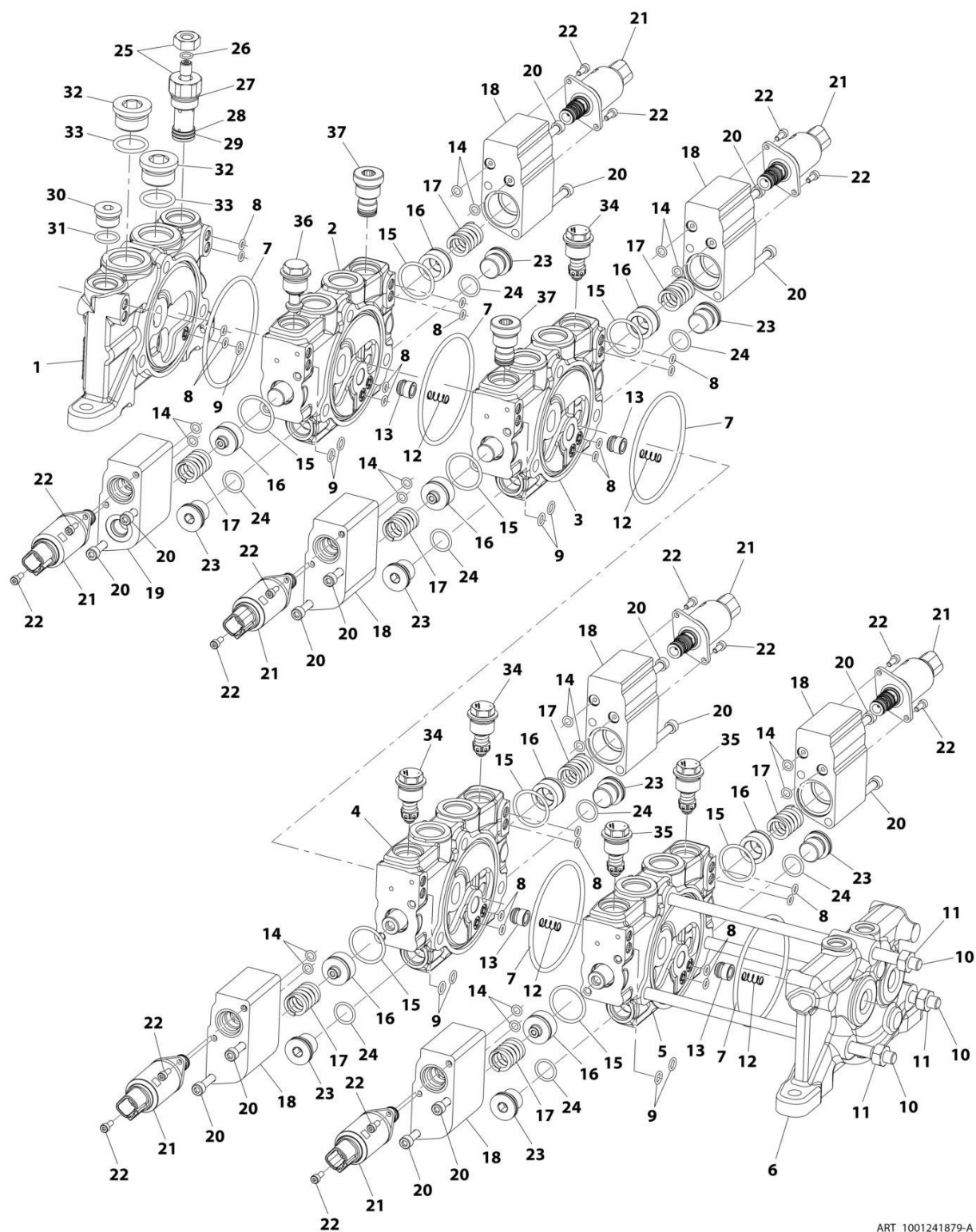
FIGURE 9-33. VALVE ASSEMBLY - MAIN CONTROL
