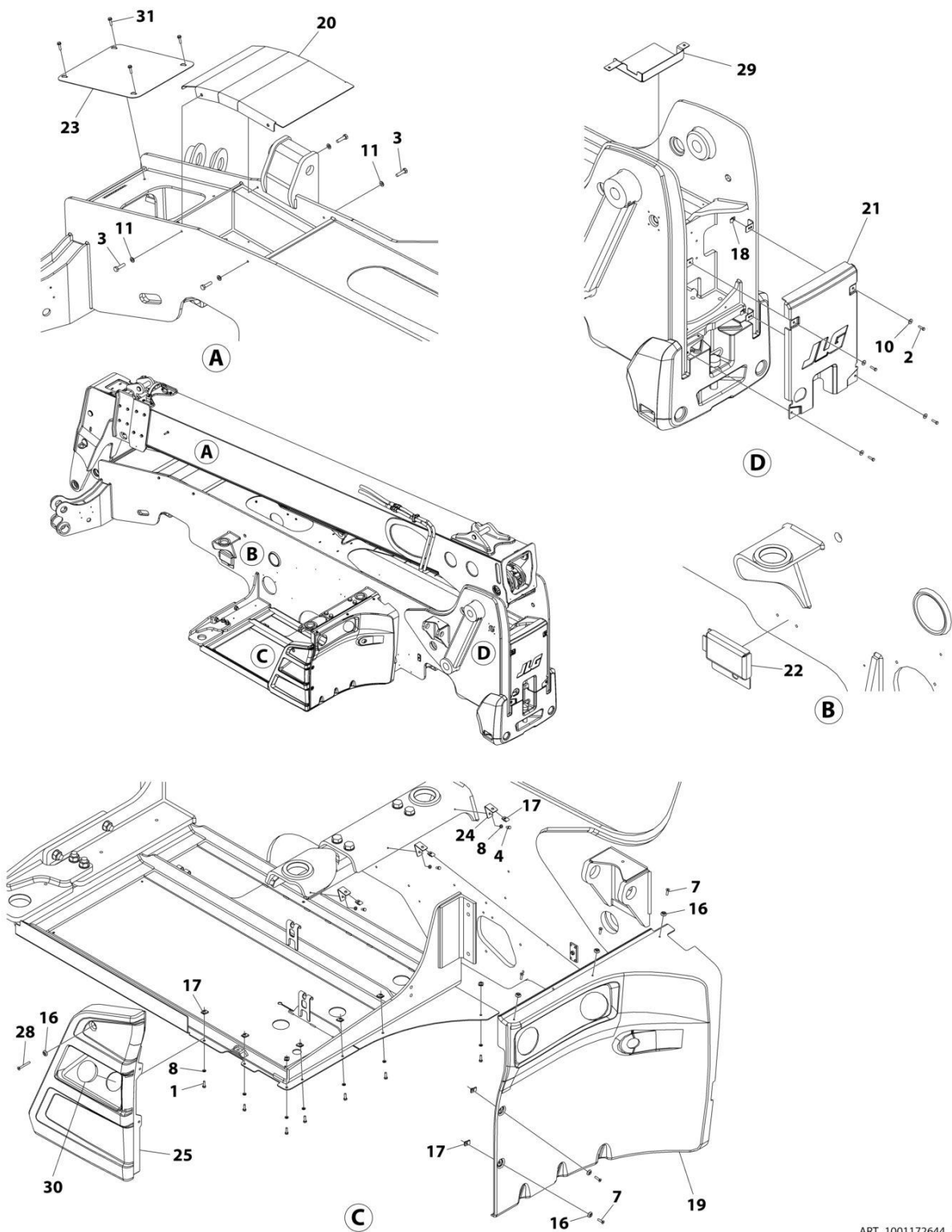
FIGURE 1-5. COVER INSTALLATION (OUTRIGGERS) (LS)
