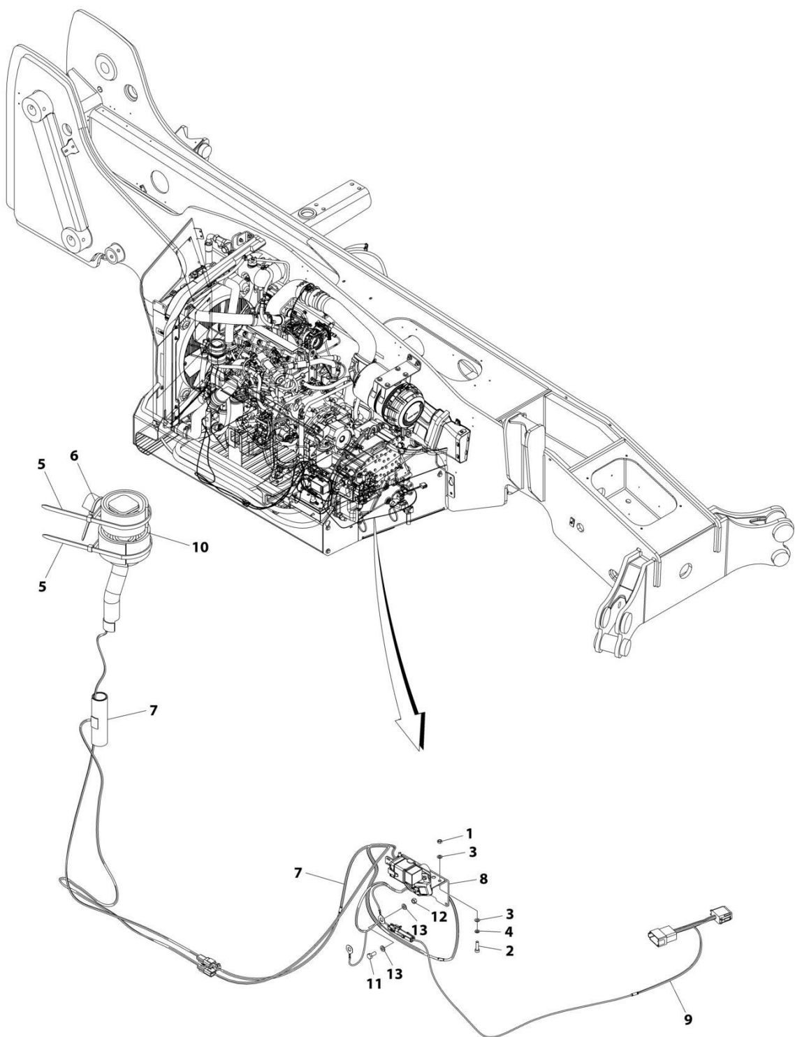
FIGURE 10-68. HEATER HARNESS - CUMMINS BREATHER (ULS)
