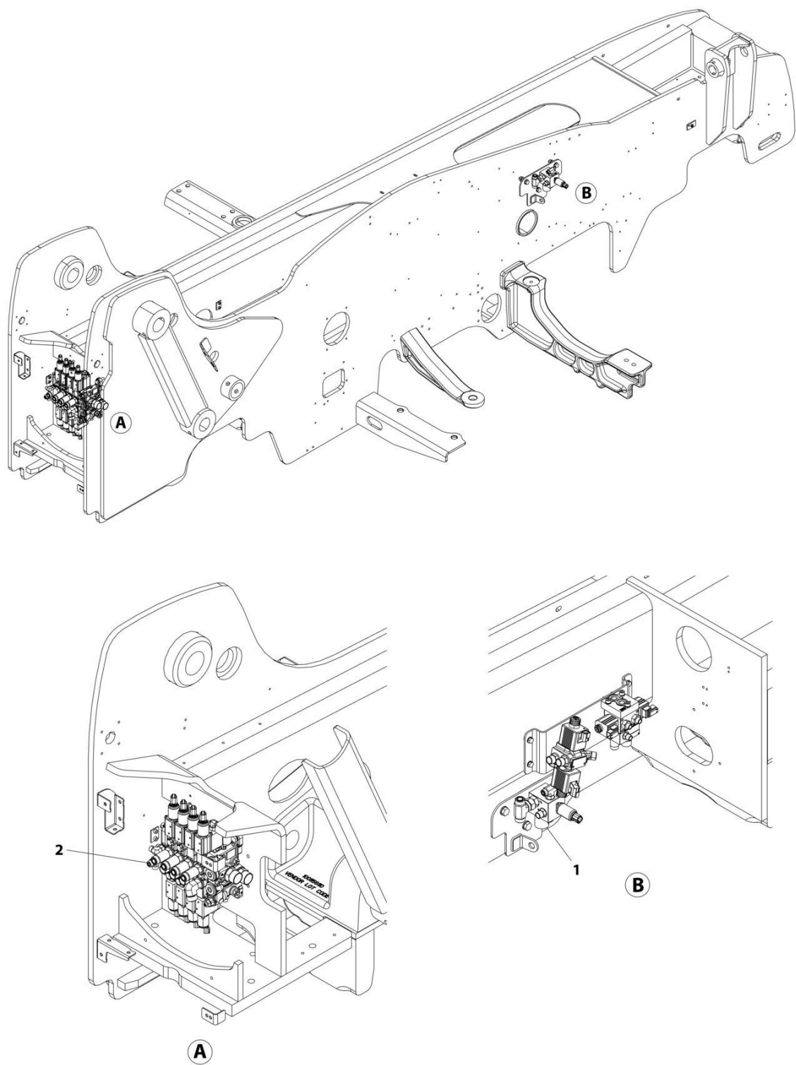
FIGURE 8-23. VALVES INSTALLATION - MAIN & PRIORITY
