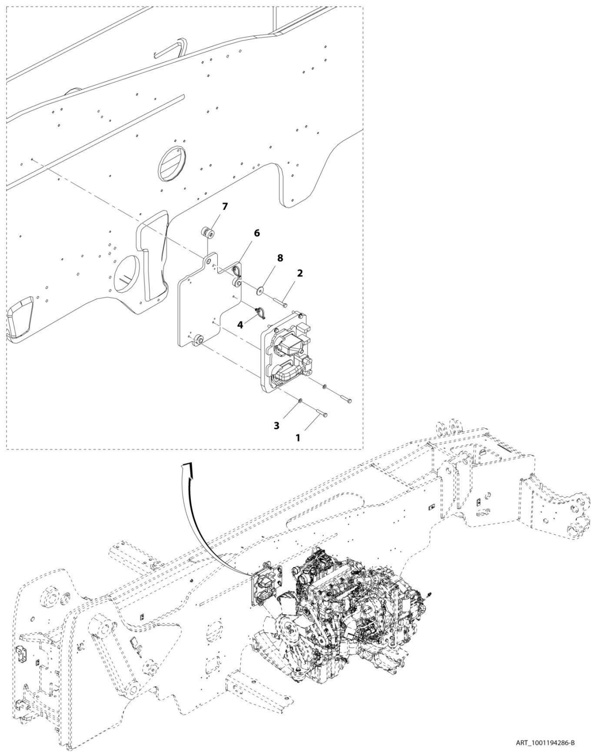
FIGURE 10-56. ENGINE - ECU INSTALLATION (ULS)
