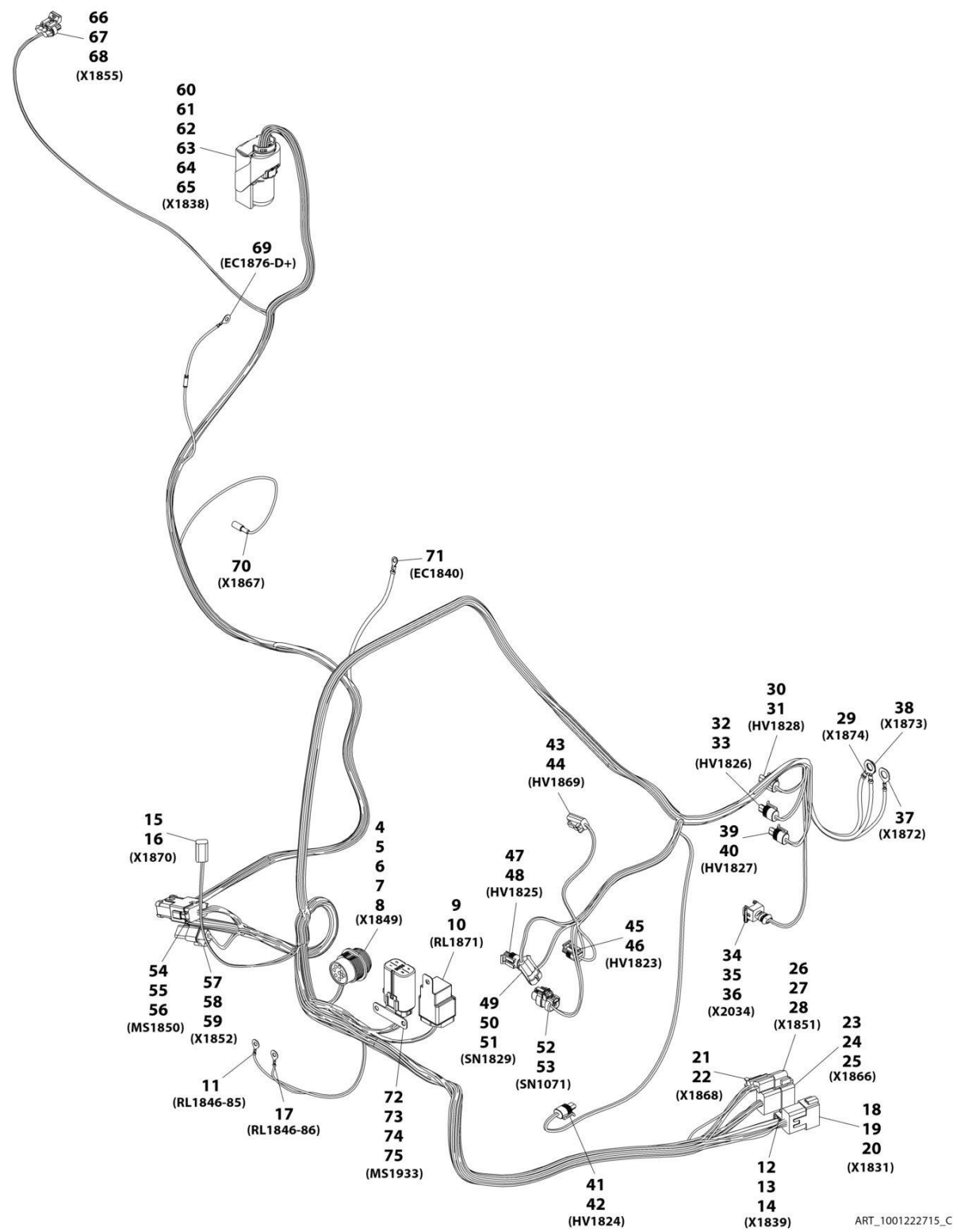
FIGURE 10-50. ENGINE HARNESS (LS)
