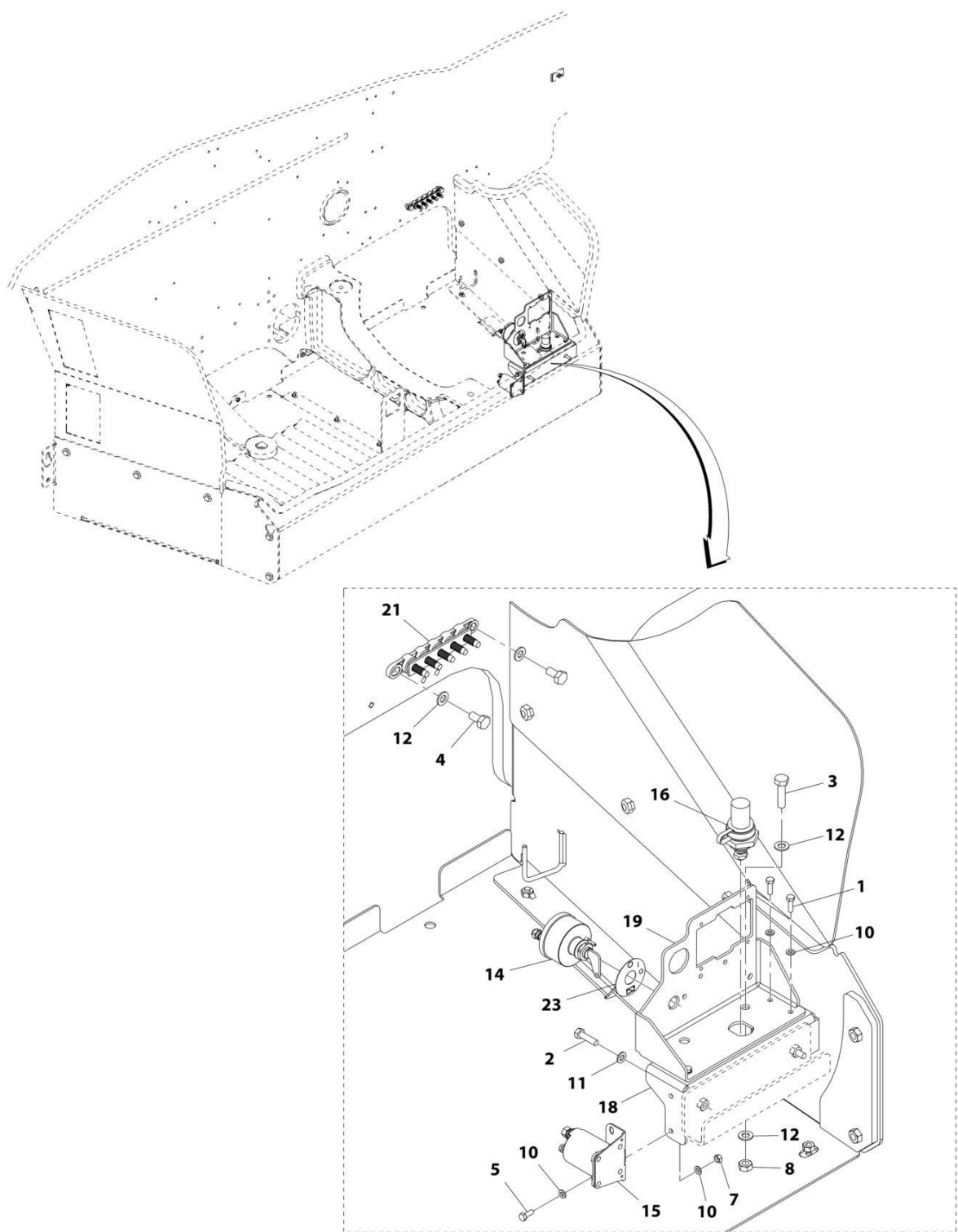
FIGURE 10-52. ENGINE BAY - ELECTRICAL INSTALLATION (LS)
