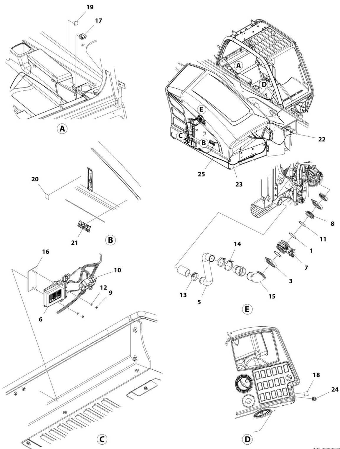
FIGURE 4-15. AIR INTAKE SHUT OFF VALVE INSTALLATION
