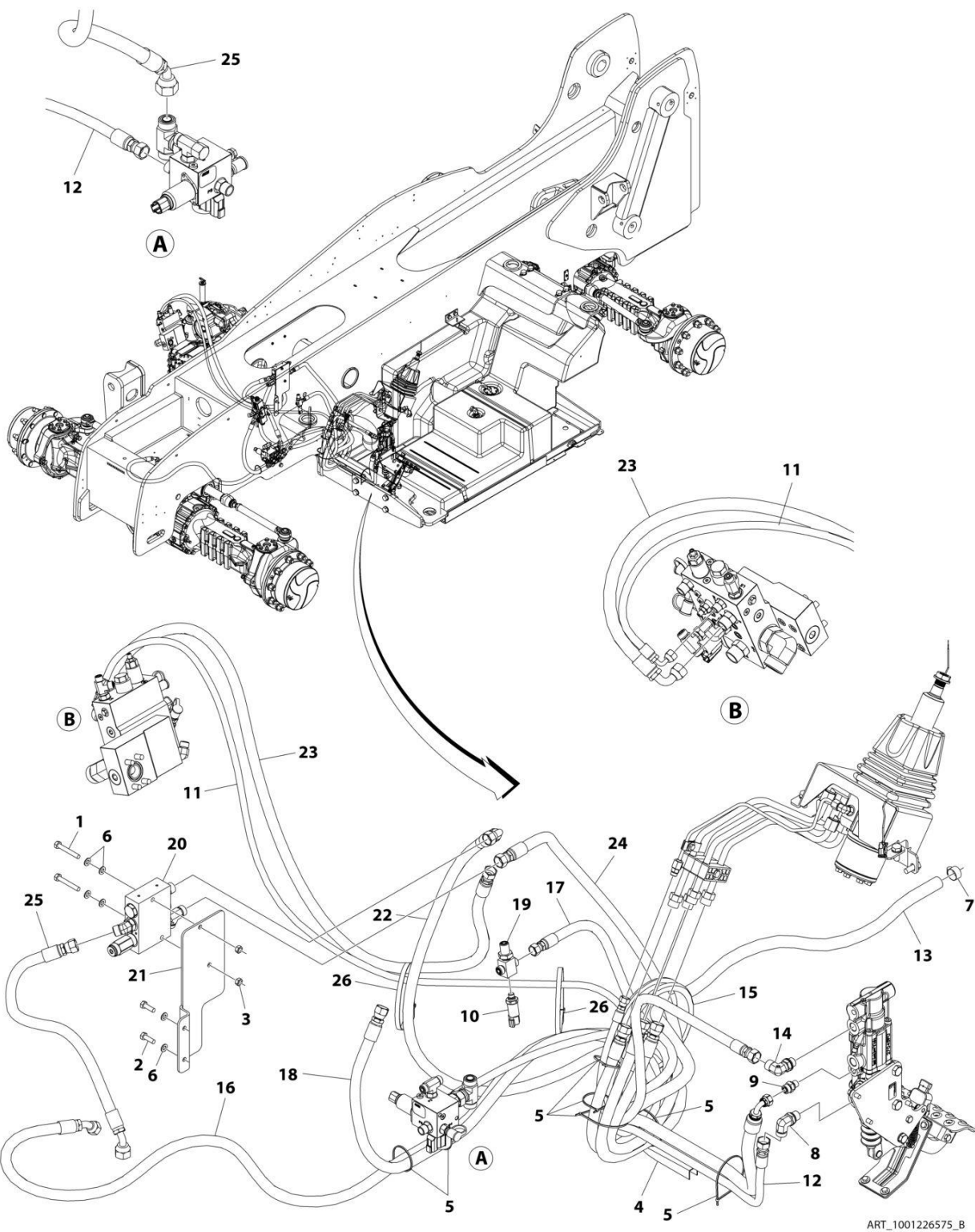
FIGURE 8-9. CAB HYDRAULIC INSTALLATION, EMERGENCY STEERING
