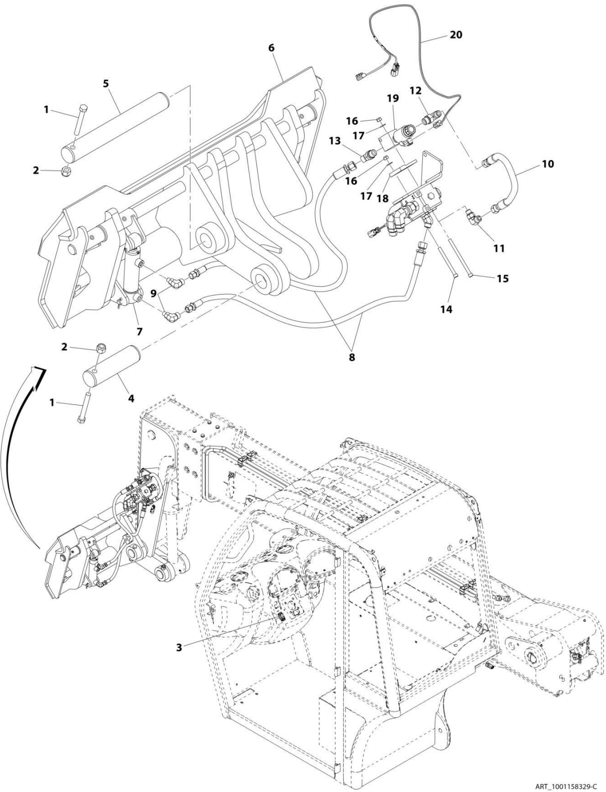
FIGURE 3-27. HYDRAULIC QUICK SWITCH INSTALLATION
