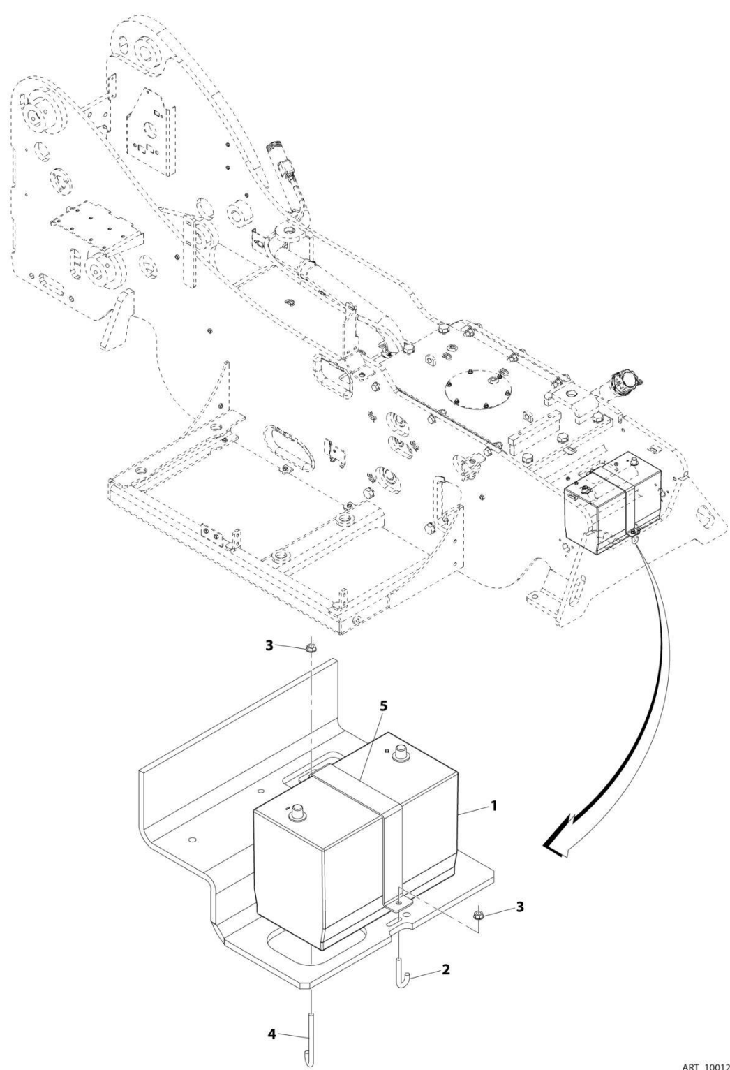
FIGURE 10-9. BATTERY INSTALLATION
