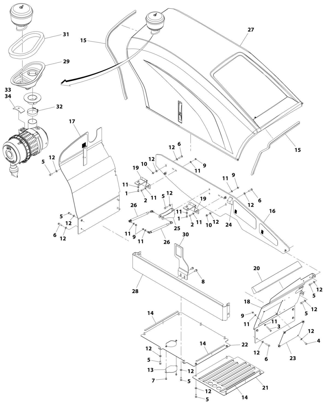
FIGURE 1-1. HOODS INSTALLATION
