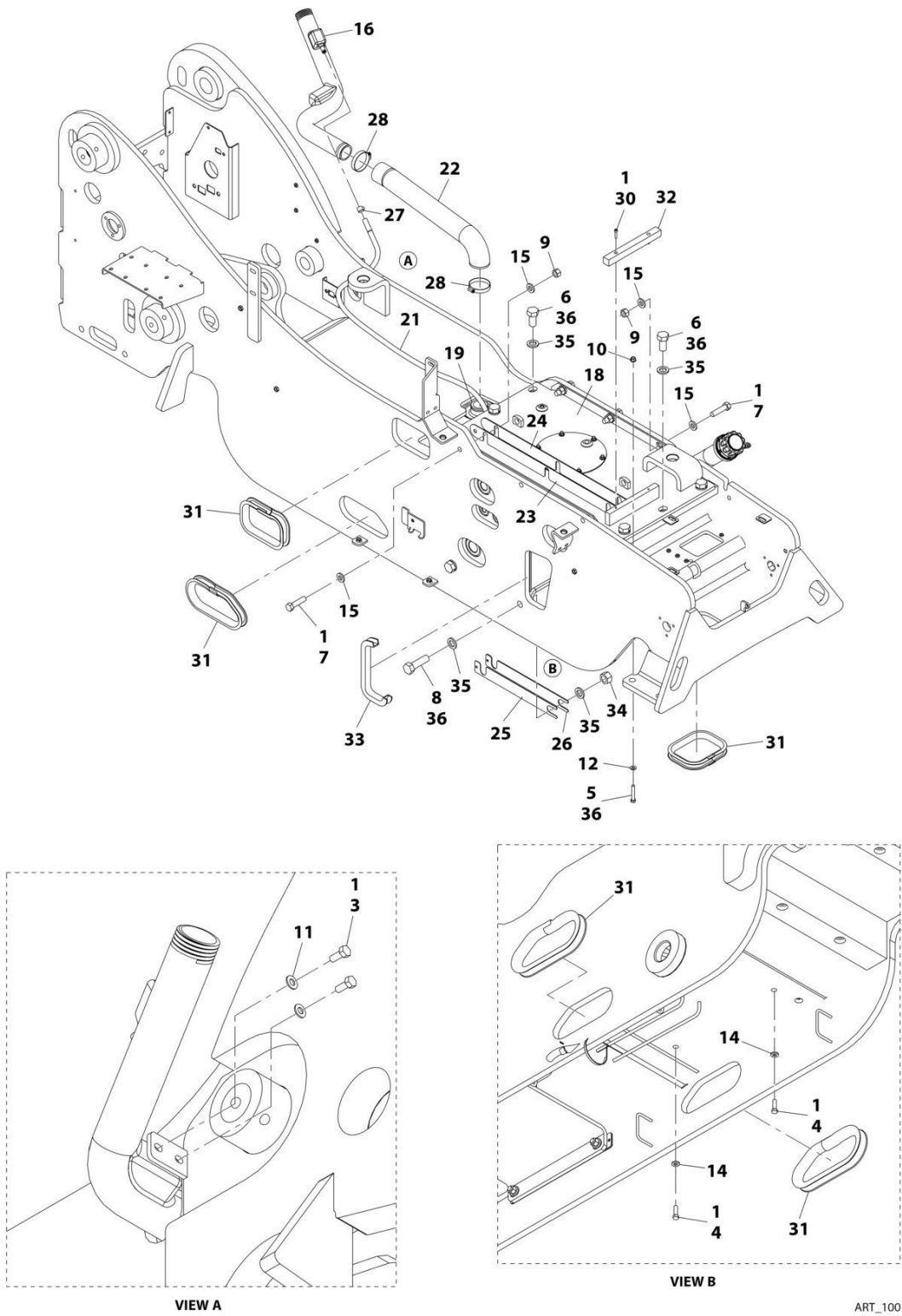
FIGURE 1-4. TANK INSTALLATION
