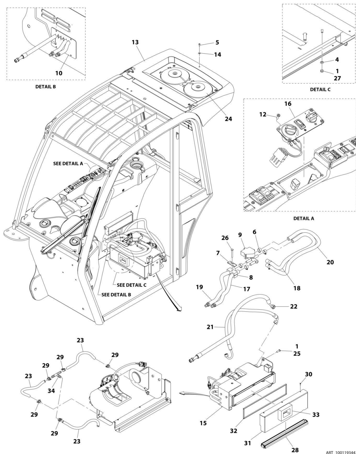
FIGURE 6-33. HEATER AND A/C INSTALLATION (CAB PARTS)
