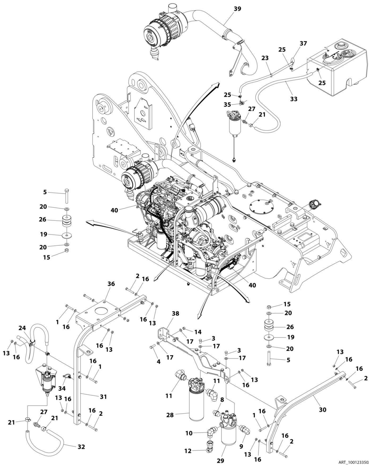
FIGURE 4-1. ENGINE INSTALLATION
