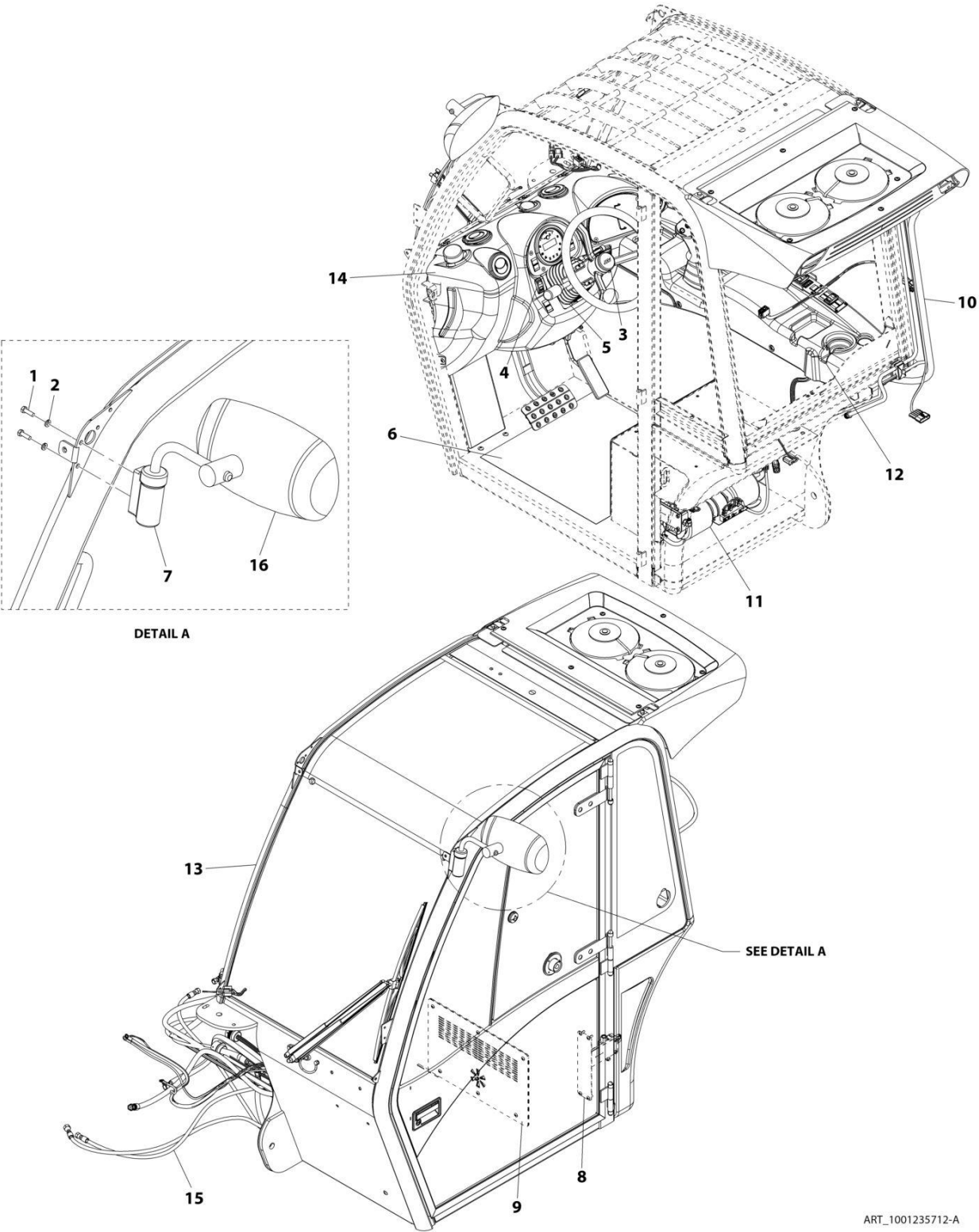
FIGURE 6-5. ENCLOSED CAB INSTALLATION (ANSI - TILT STEERING) (HEAT & A/C)
