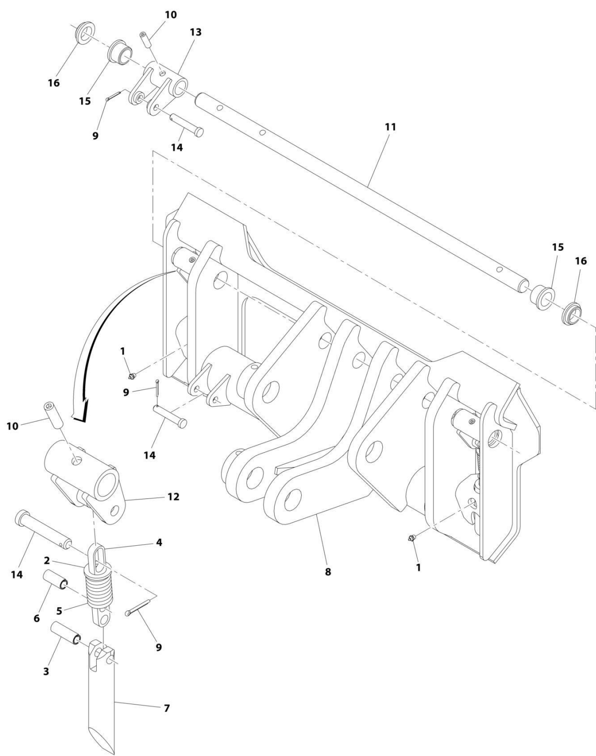
FIGURE 3-28. QUICK SWITCH ASSEMBLY
