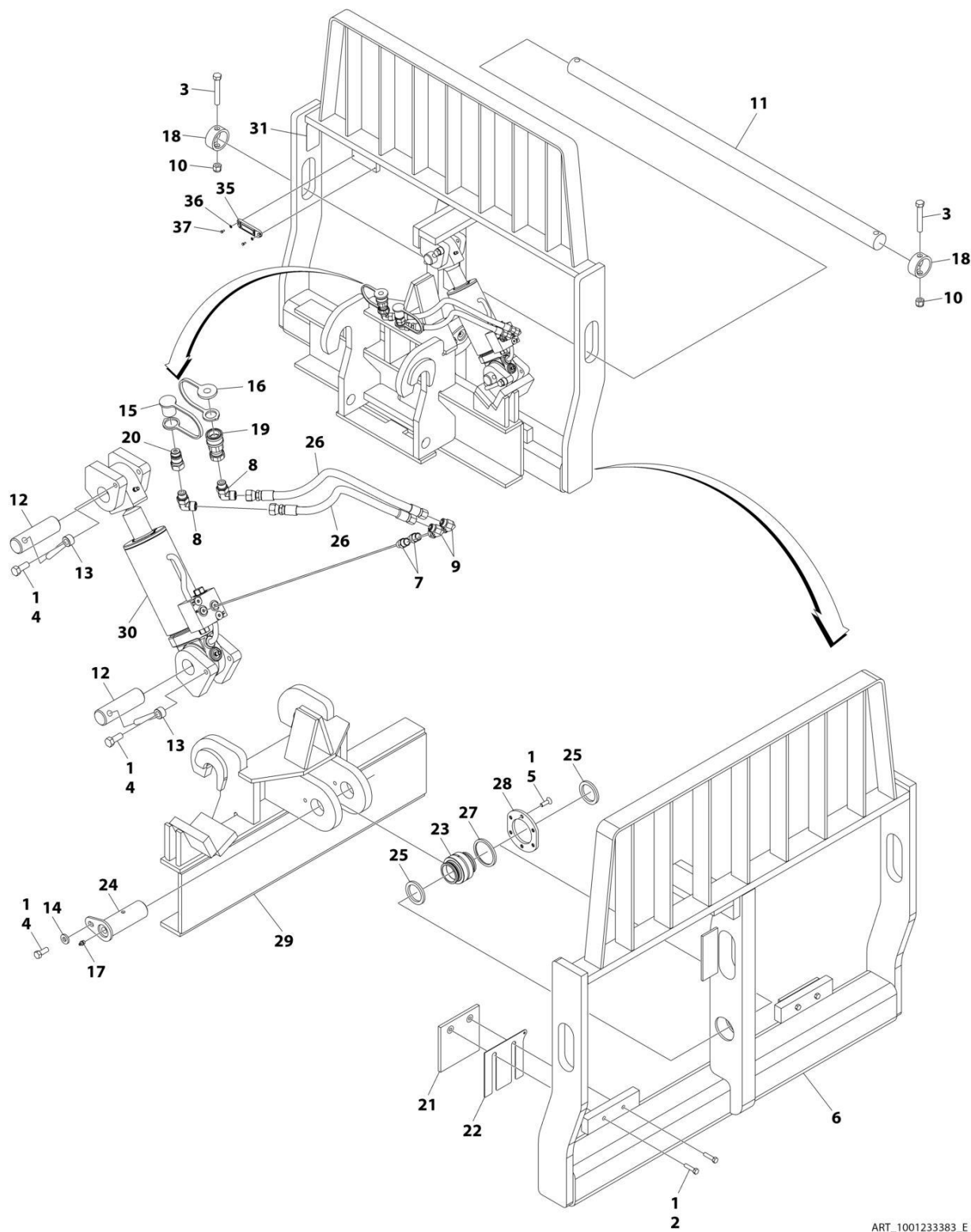
FIGURE 3-20. SIDE TILT CARRIAGE ASSEMBLY (50 INCH)
