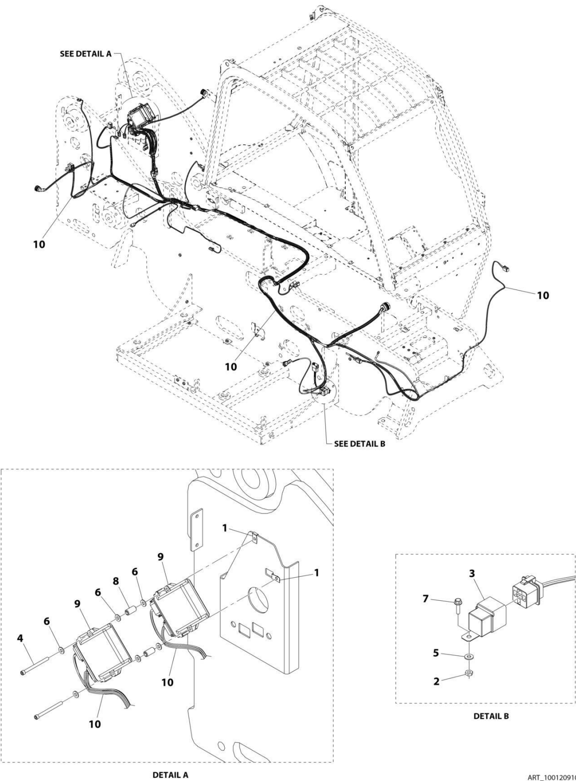
FIGURE 10-4. FRAME OPTIONS HARNESS INSTALLATION (CE)
