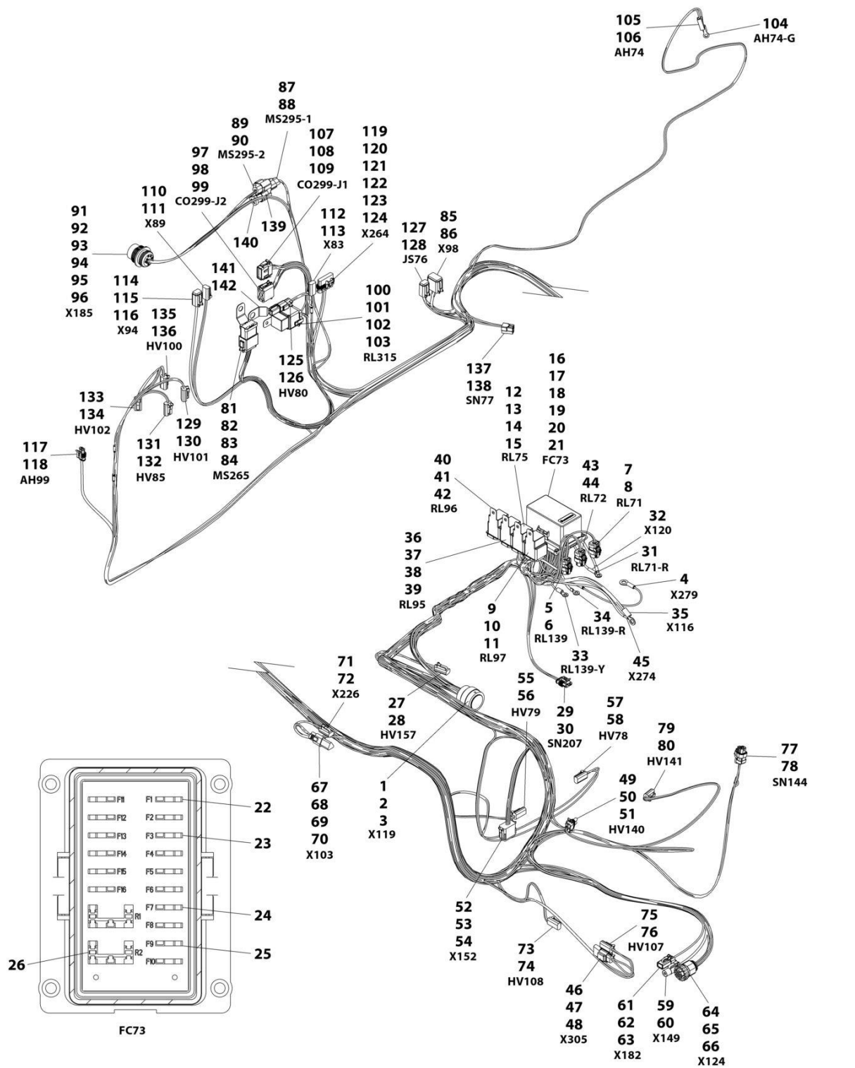
FIGURE 10-32. FRAME HARNESS
