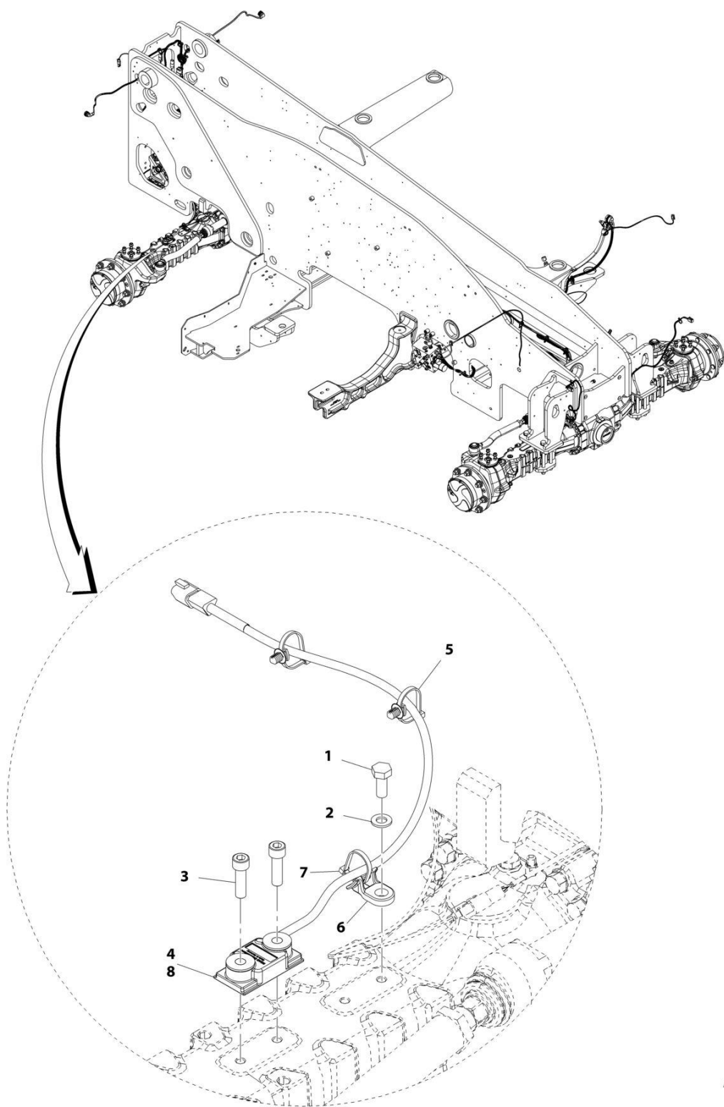
FIGURE 10-49. LSI SENSOR INSTALLATION
