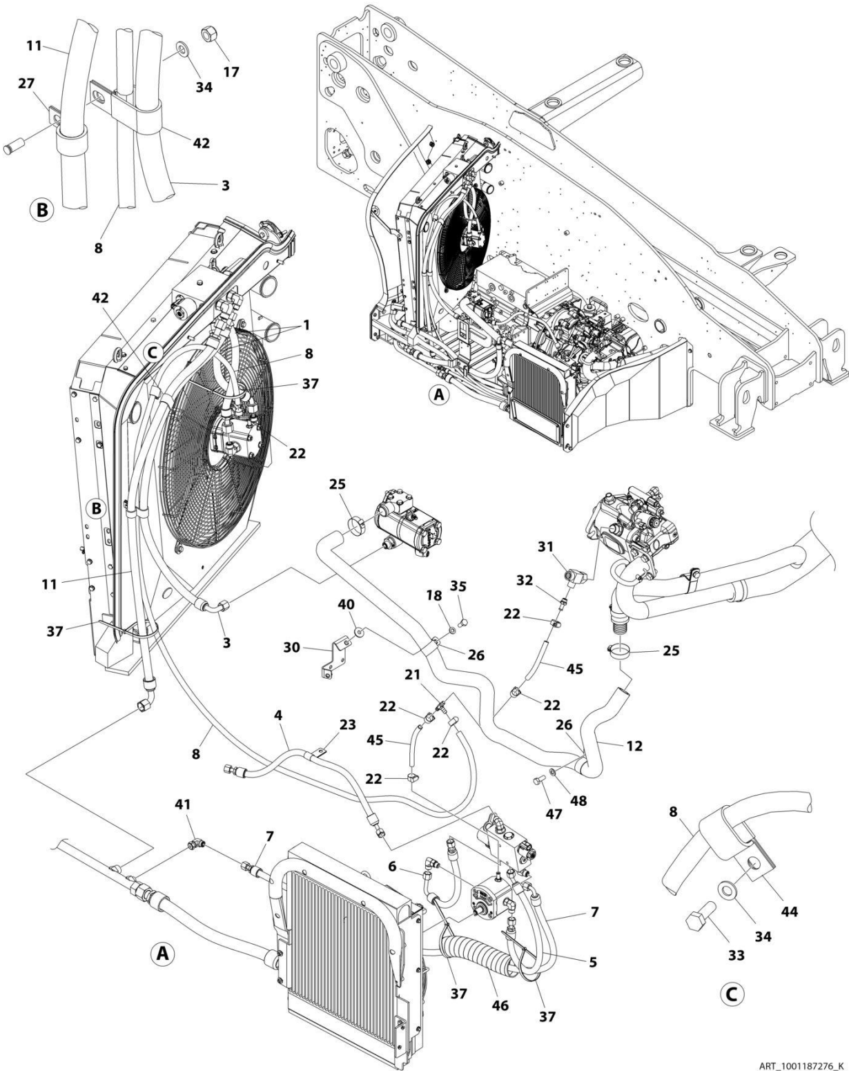
FIGURE 4-21. FAN LINES INSTALLATION (90KW)
