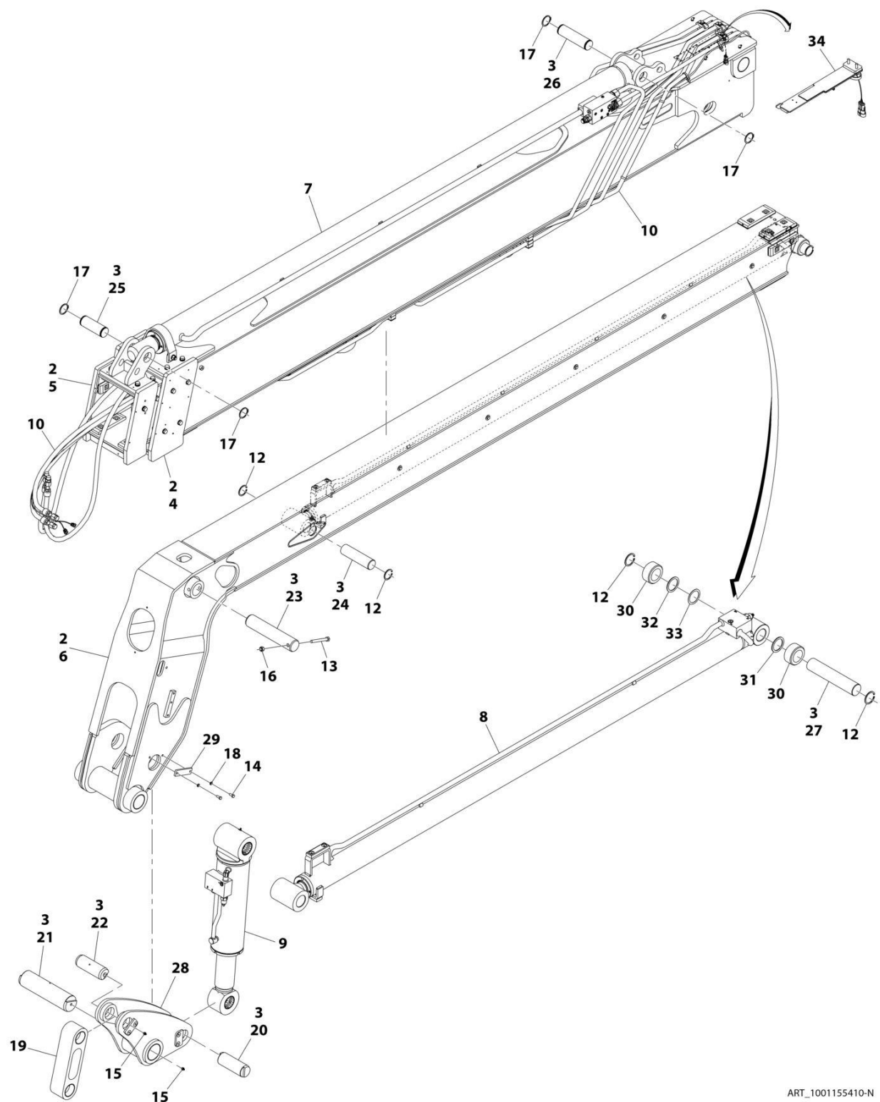
FIGURE 2-5. BOOM ASSEMBLY
