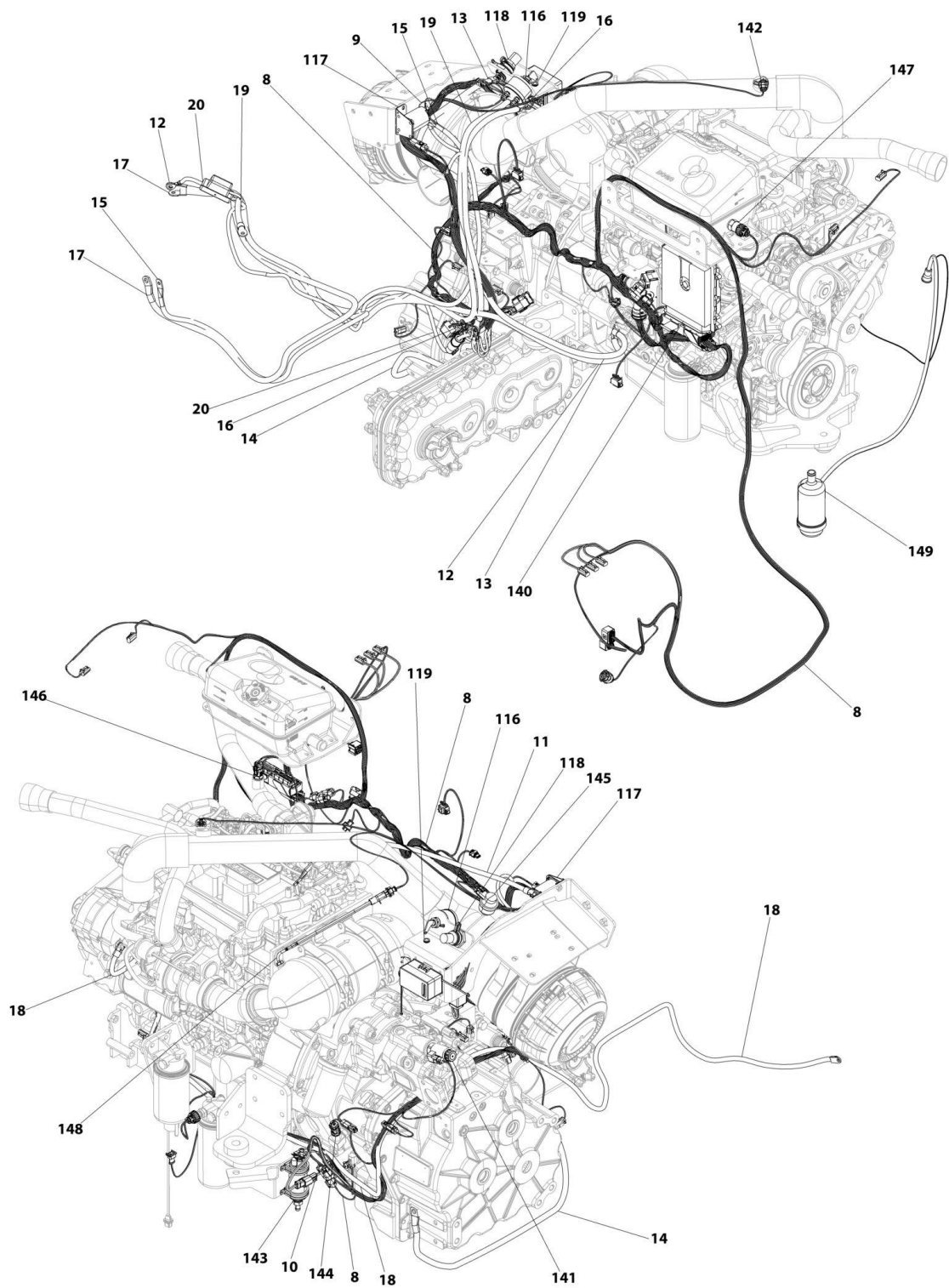
ART_925-ELECTRICAL_ENGINE_DEUTZ3-6-90KW
