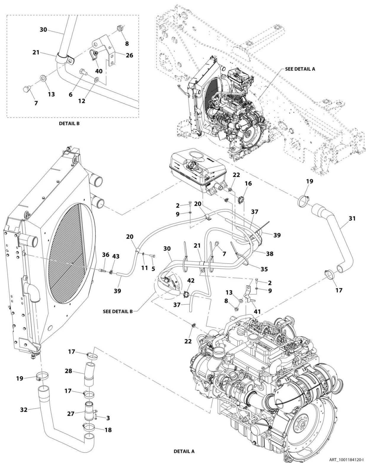
FIGURE 4-29. COOLANT LINES INSTALLATION (ULS)
