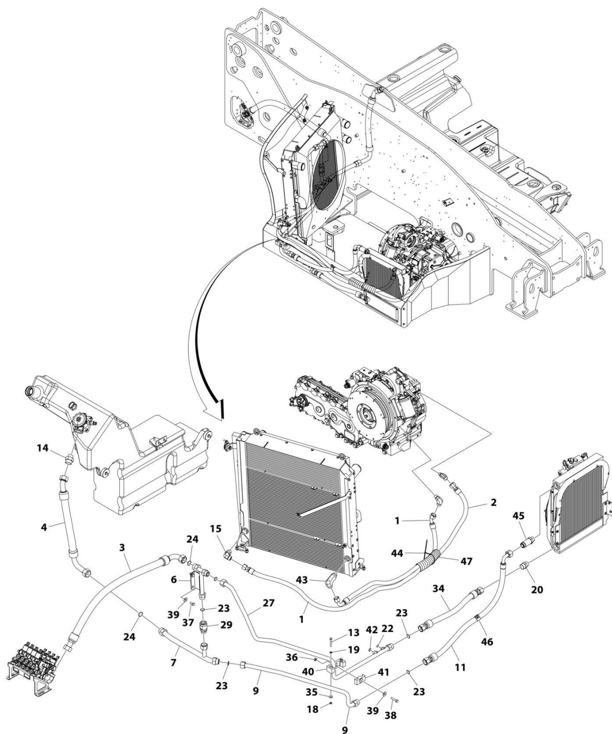
FIGURE 4-30. COOLER LINES INSTALLATION (90KW)
