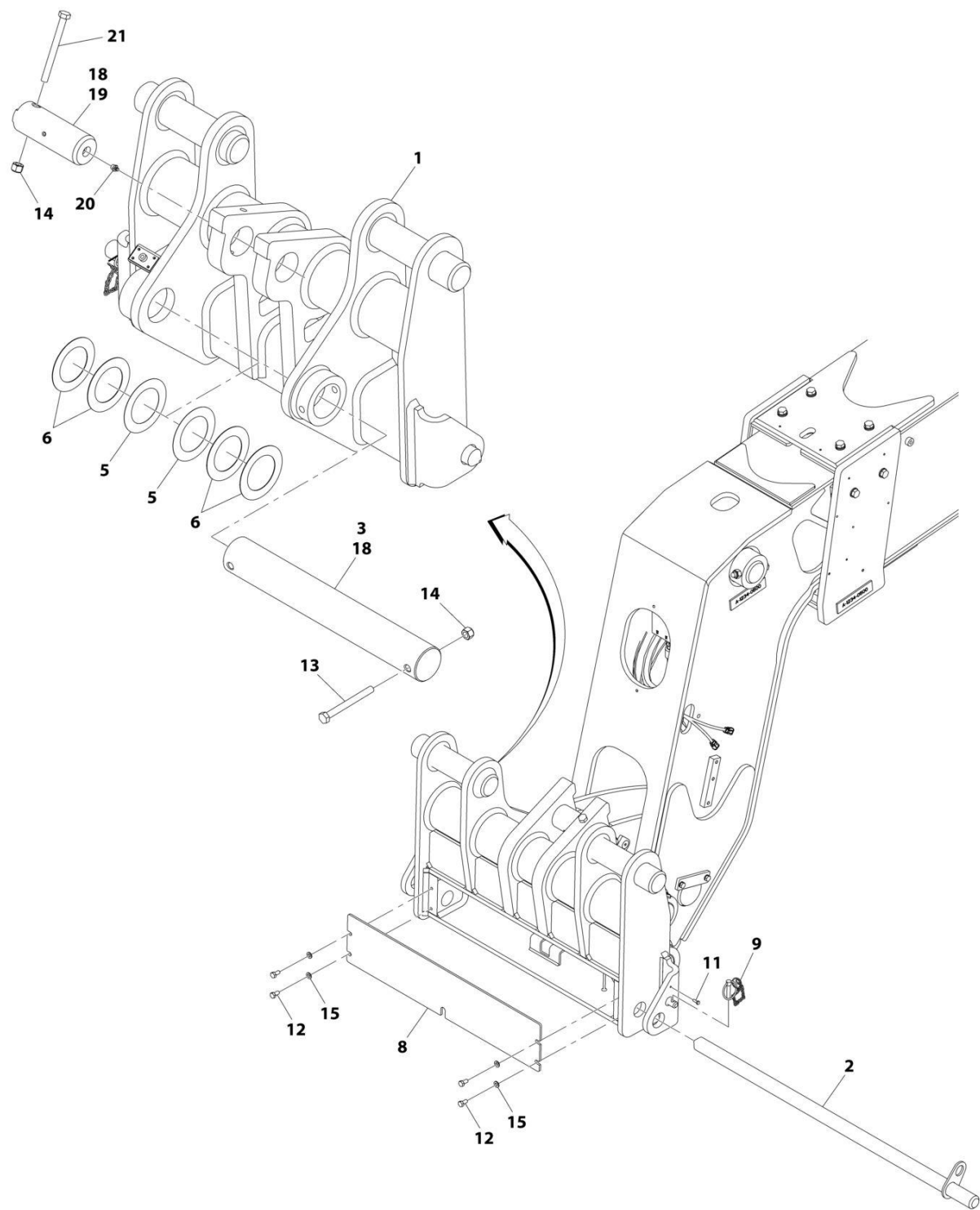
FIGURE 2-11. MANUAL QUICK COUPLER INSTALLATION
