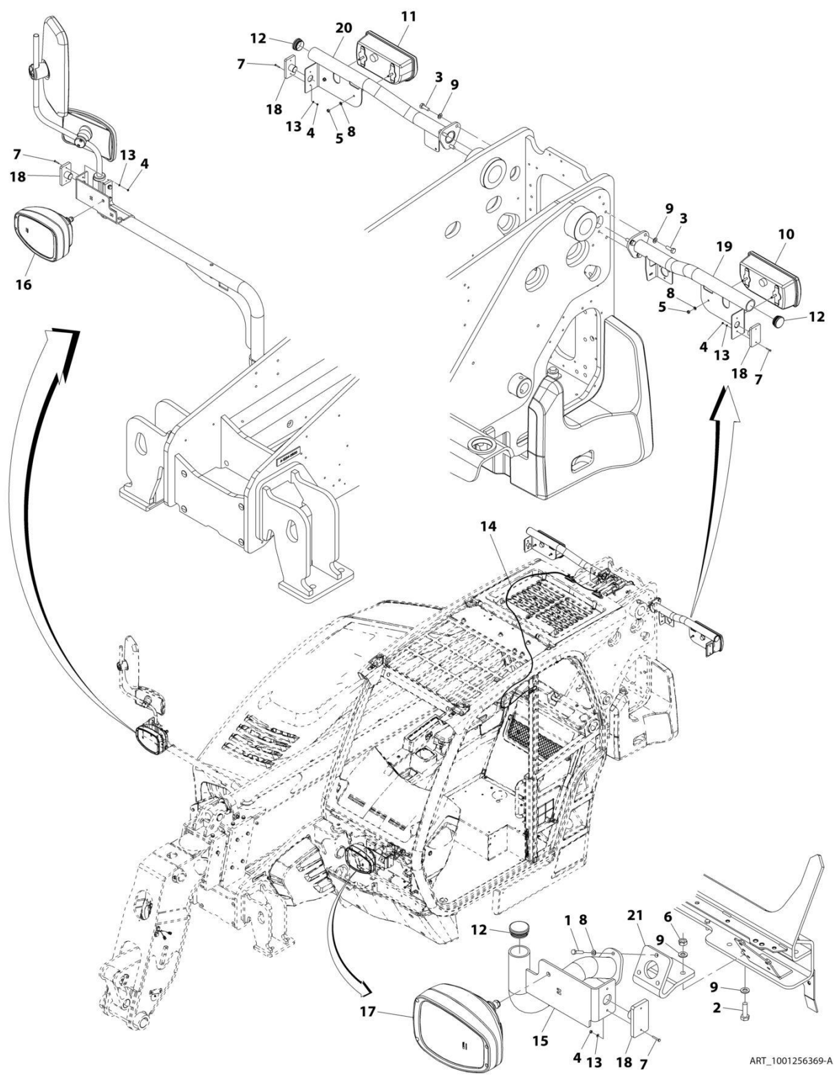
FIGURE 10-36. LIGHTS - DIP LIGHTS INSTALLATION (RH)
