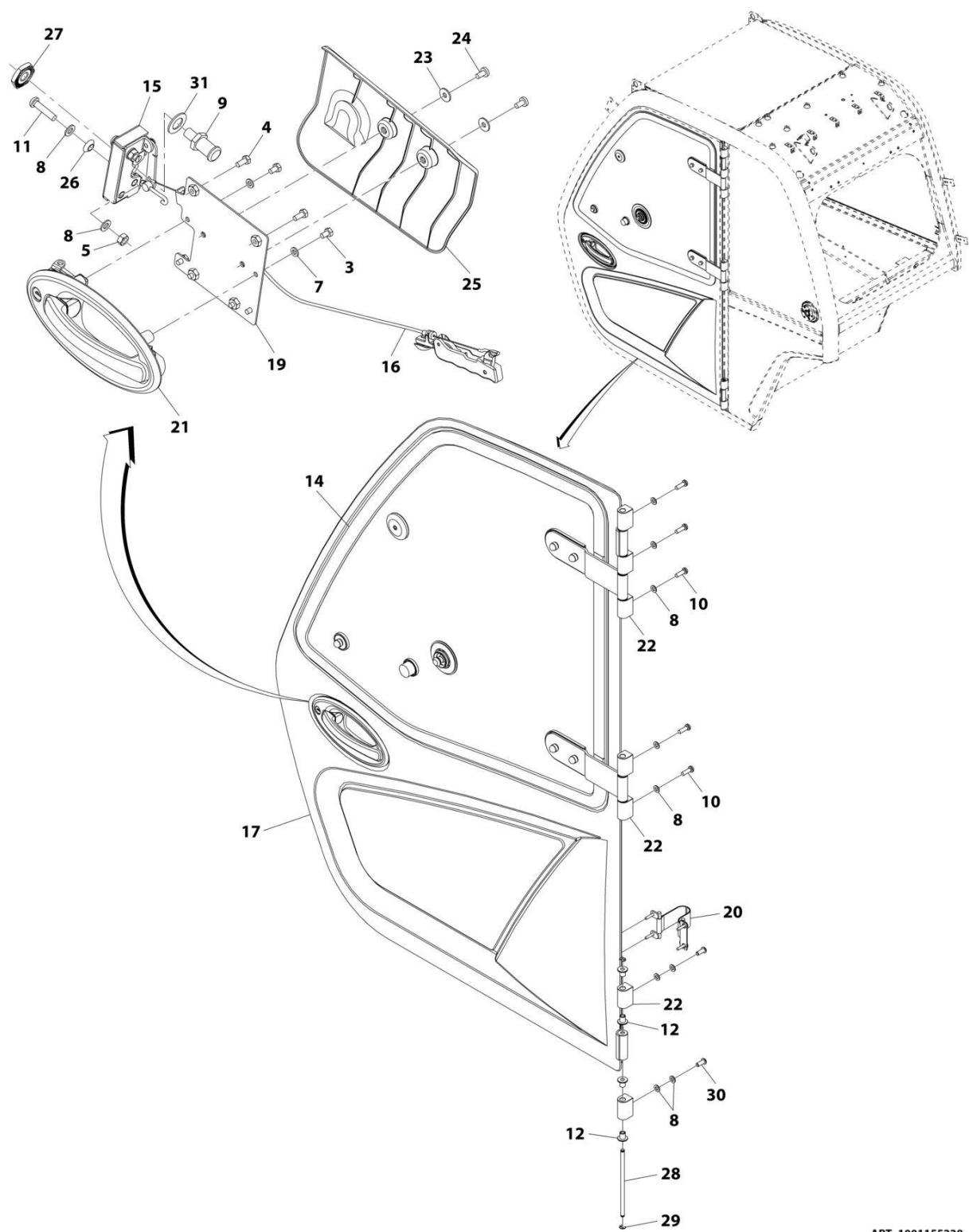
FIGURE 6-6. DOOR INSTALLATION
