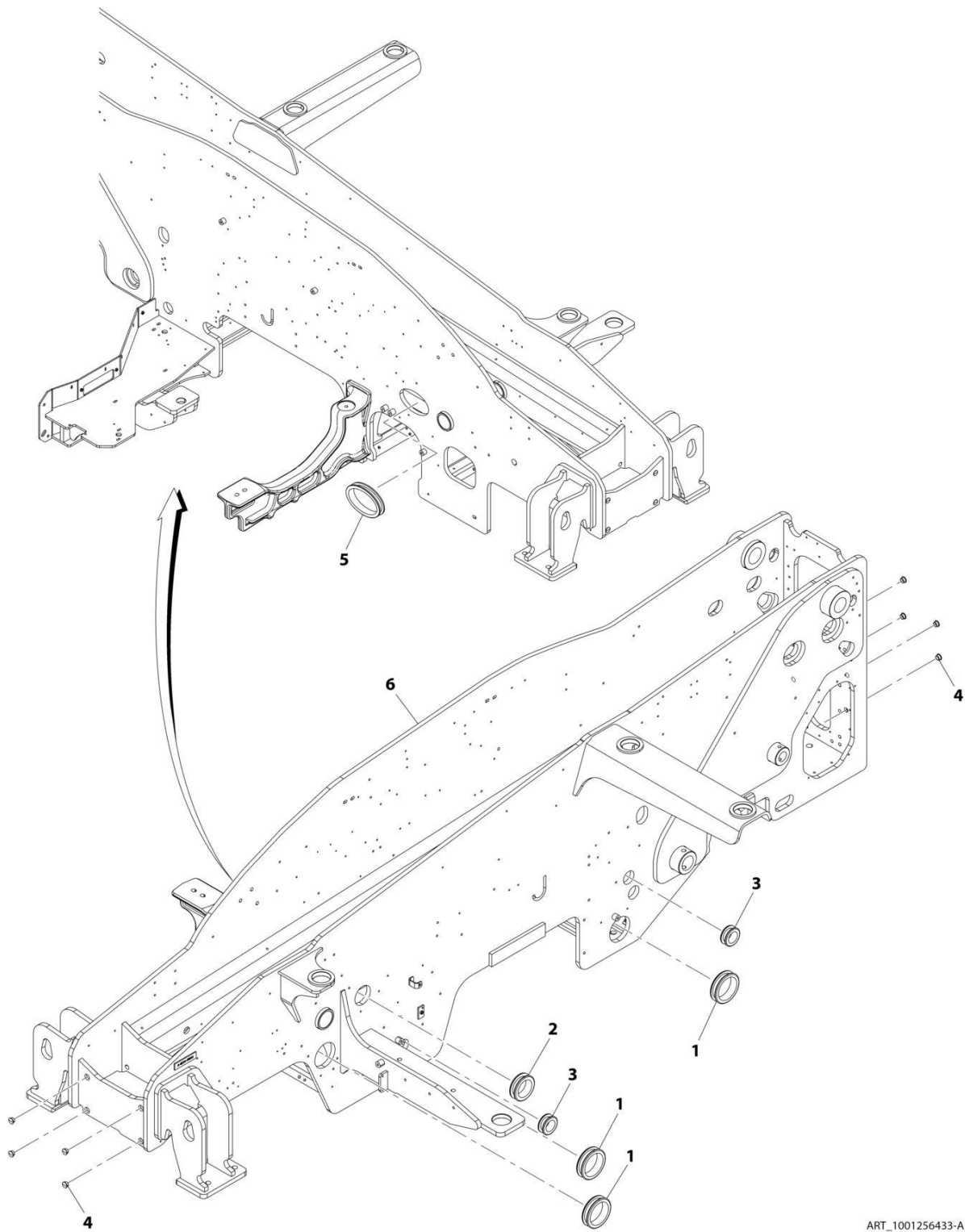
FIGURE 1-1. FRAME INSTALLATION
