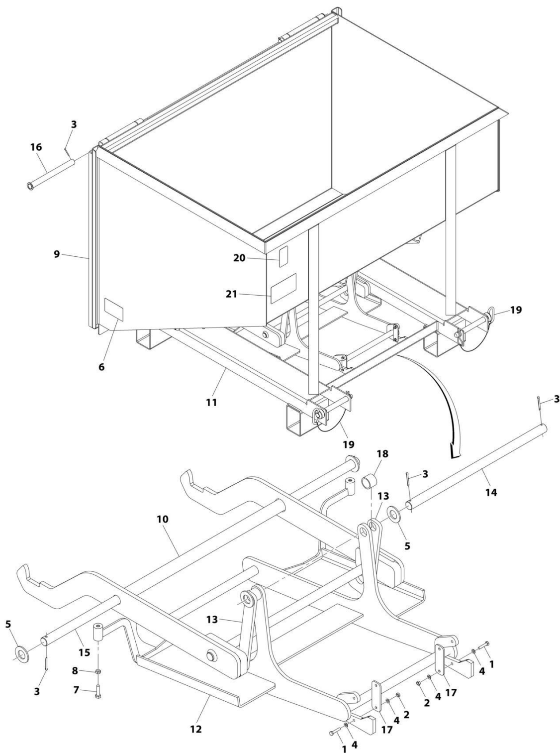
FIGURE 3-49. TRASH HOPPER INSTALLATION
