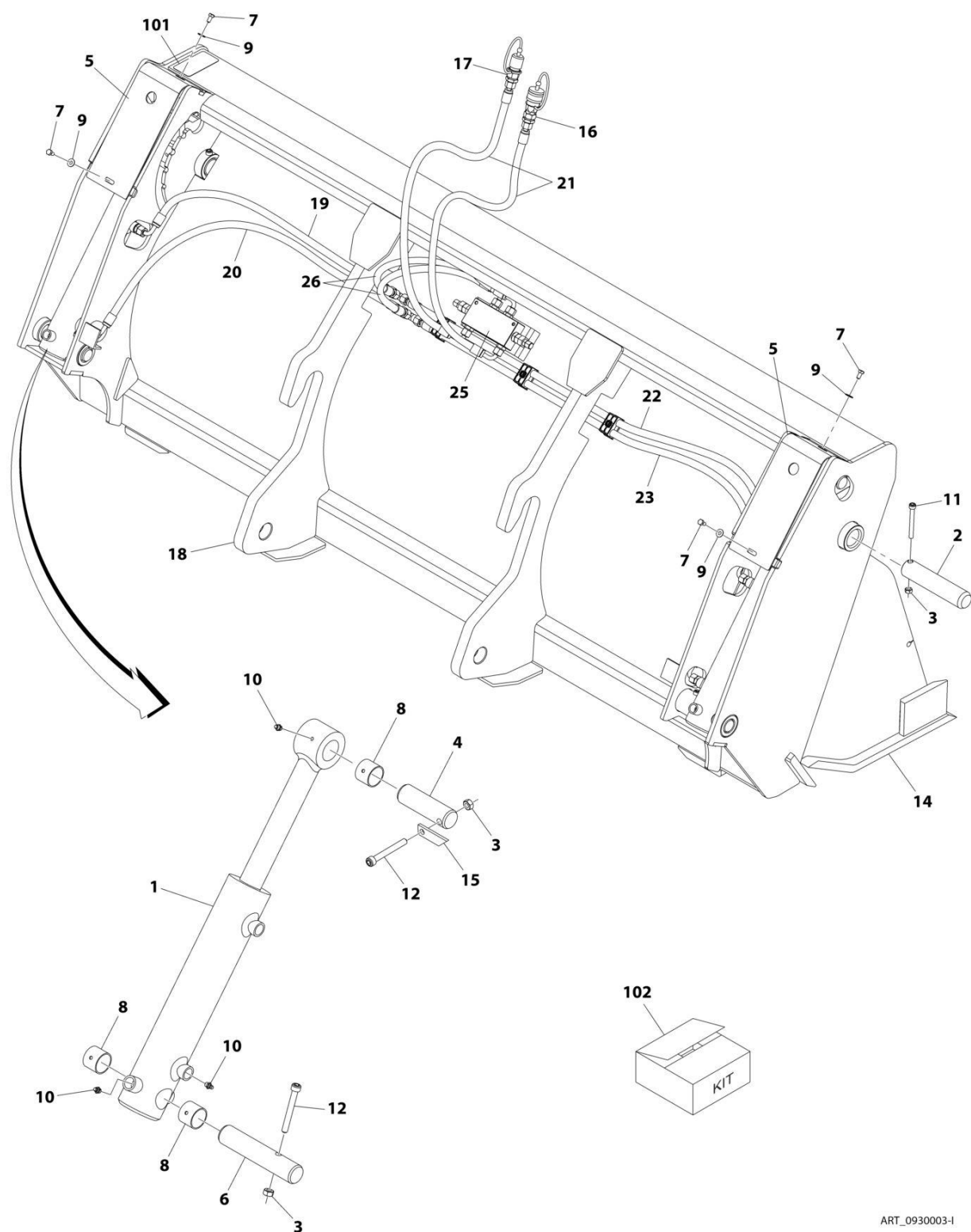
FIGURE 3-23. BUCKET(1 M³) (MULTI-PURPOSE 4 IN 1)
