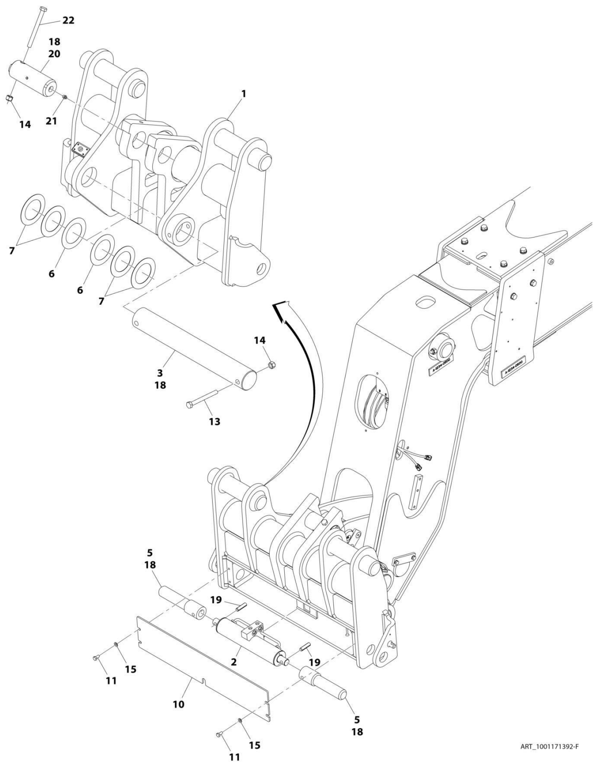
FIGURE 2-12. HYDRAULIC QUICK COUPLER INSTALLATION
