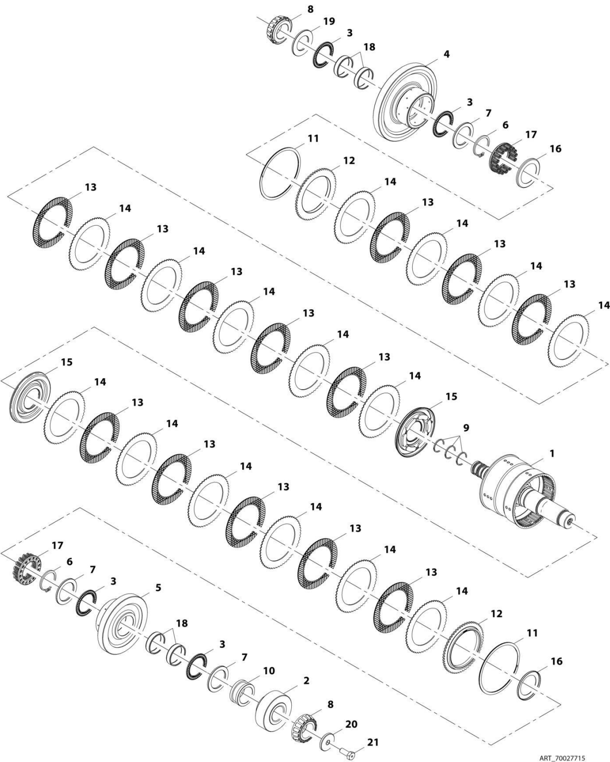
FIGURE 5-20. CLUTCH AND GEAR GROUP
