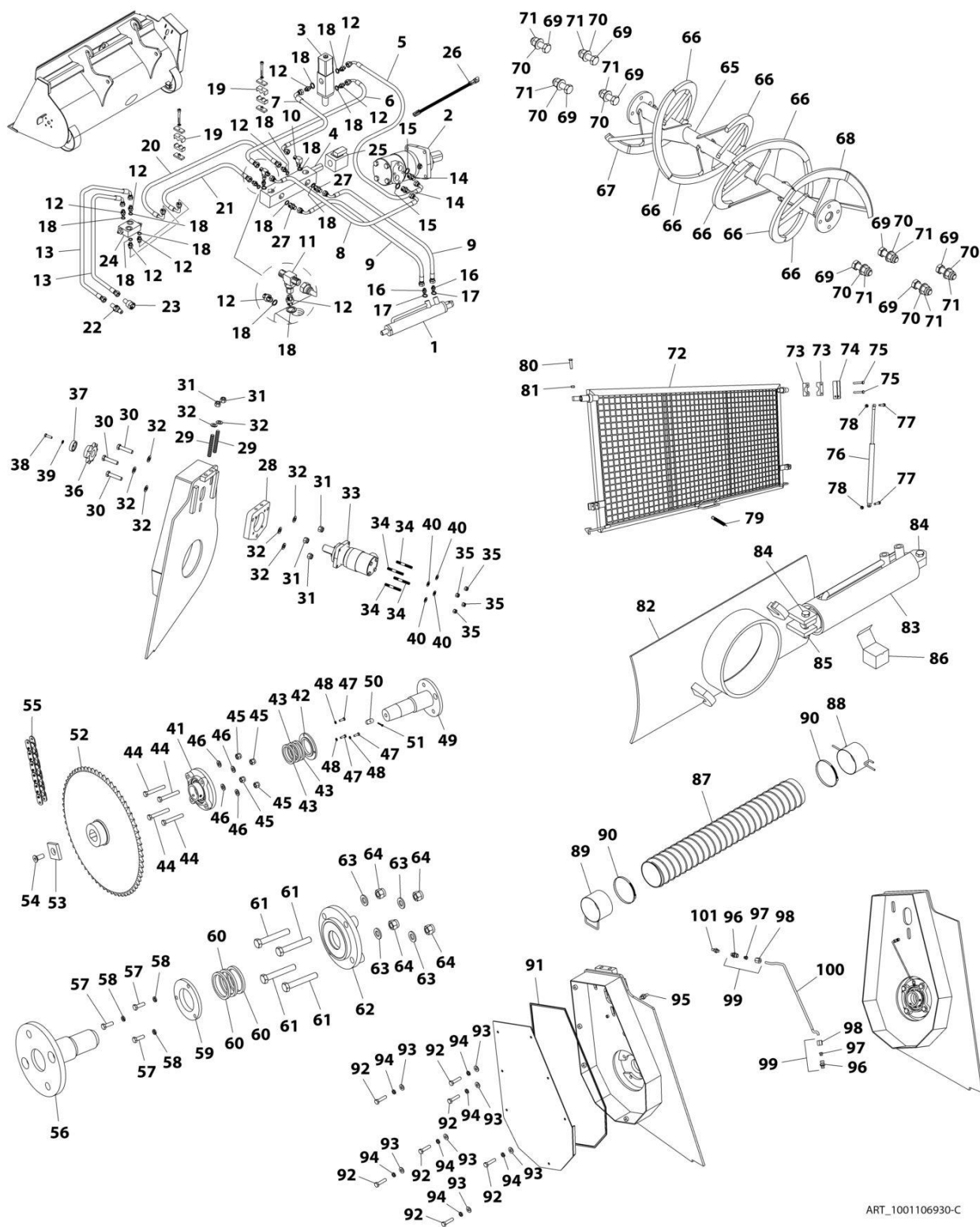
FIGURE 3-17. BUCKET (CONCRETE)
