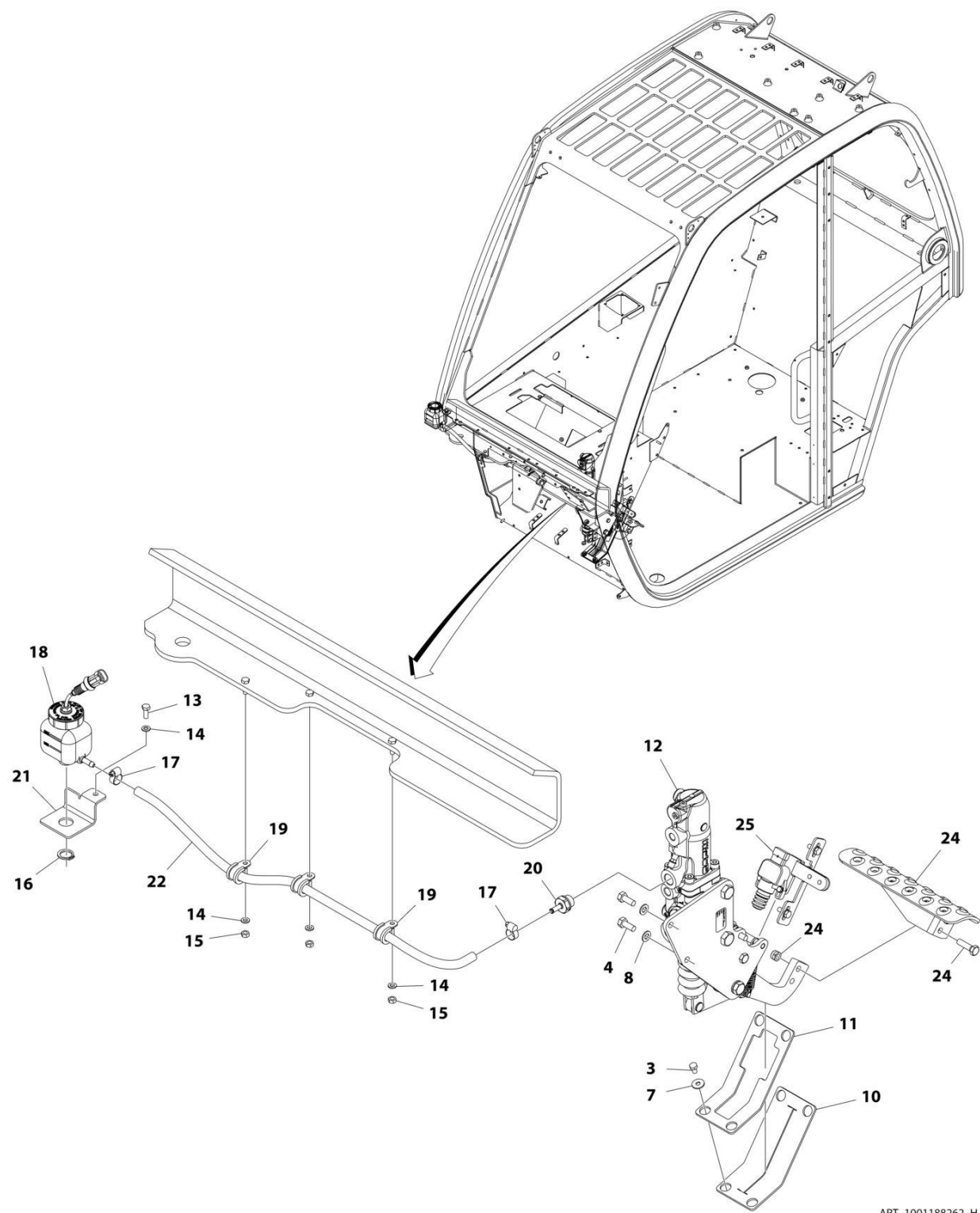
FIGURE 7-3. BRAKE PEDAL INSTALLATION
