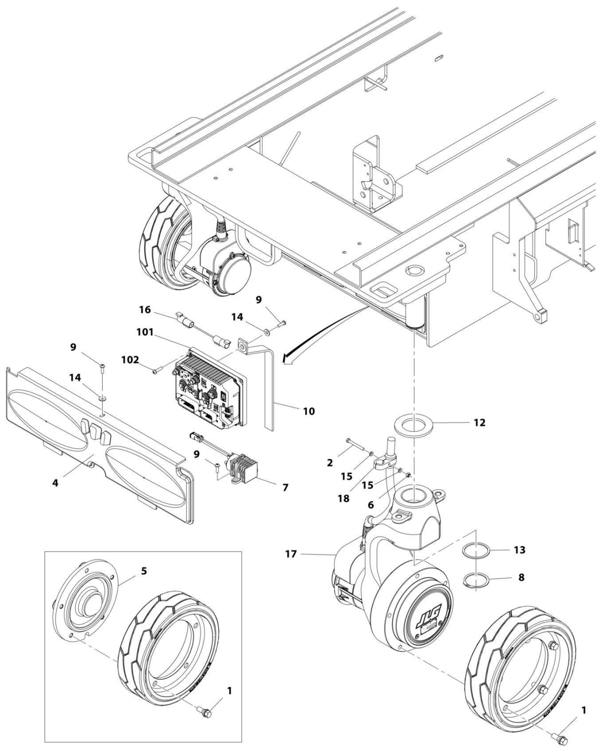
FIGURE 1-3. DRIVE HUB AND MODULE INSTALLATION (BELGIUM BUILT MACHINES ONLY)
