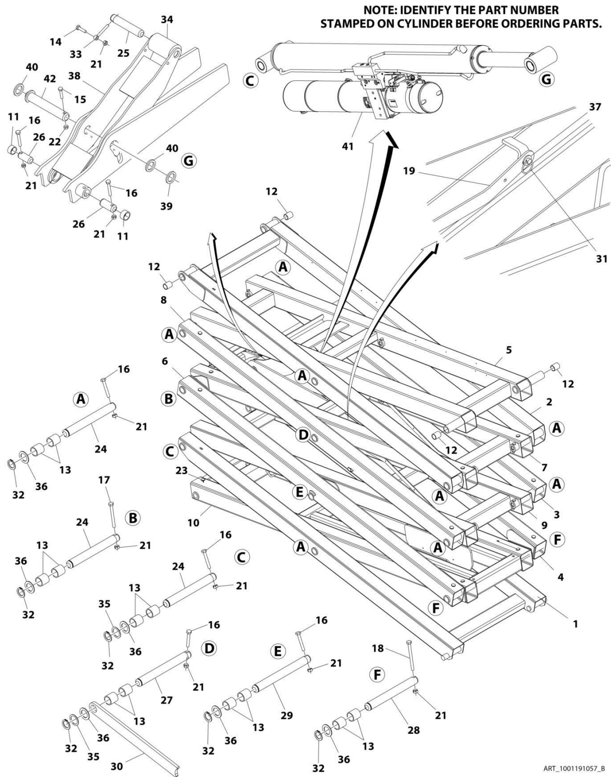
FIGURE 3-6. SCISSORS ARMS ASSEMBLY - 2646ES BIODEGRADABLE HYDRAULIC OIL (CHINA BUILT MACHINES)
