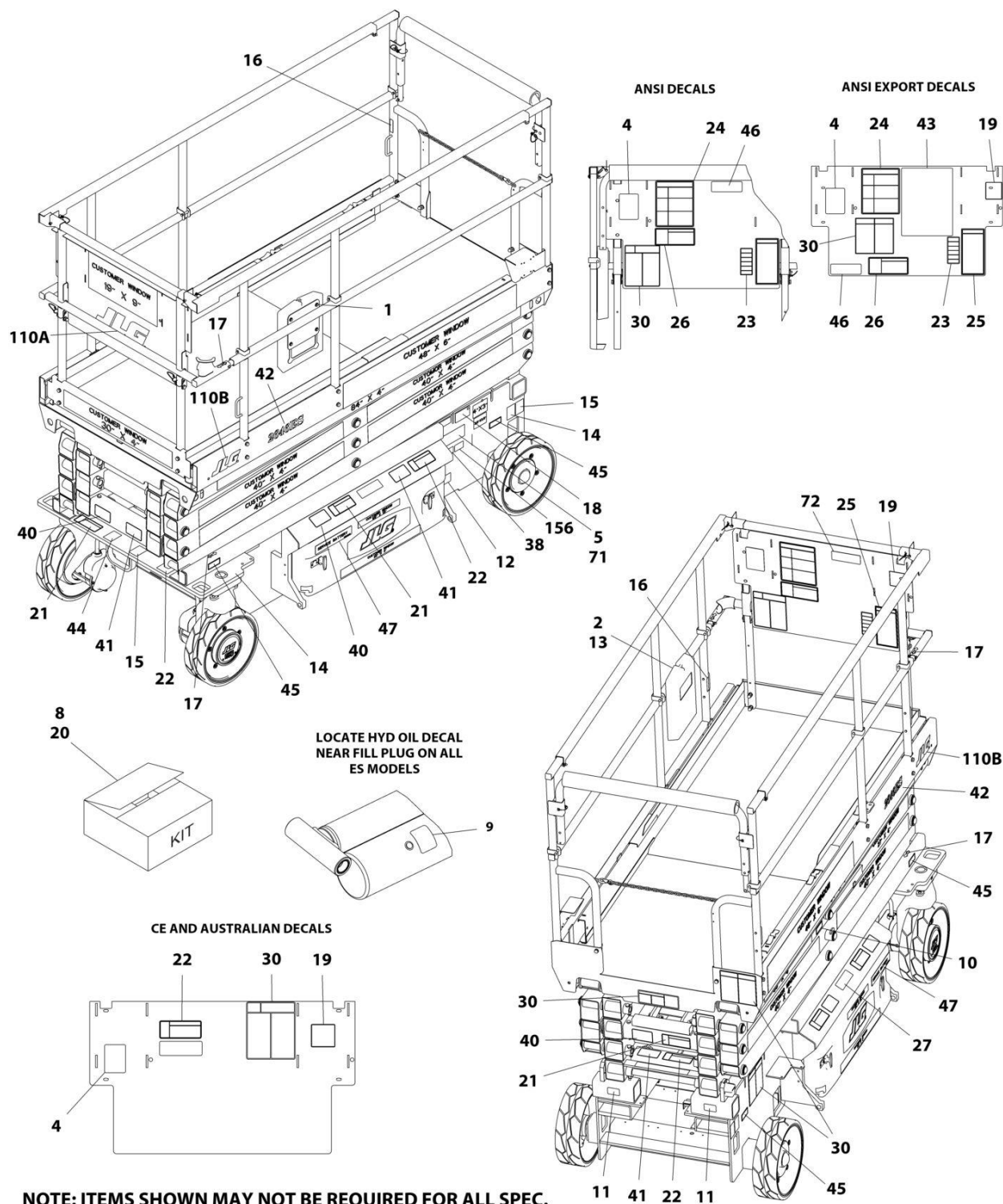
FIGURE 8-10. DECAL INSTALLATION – OPTIONS
