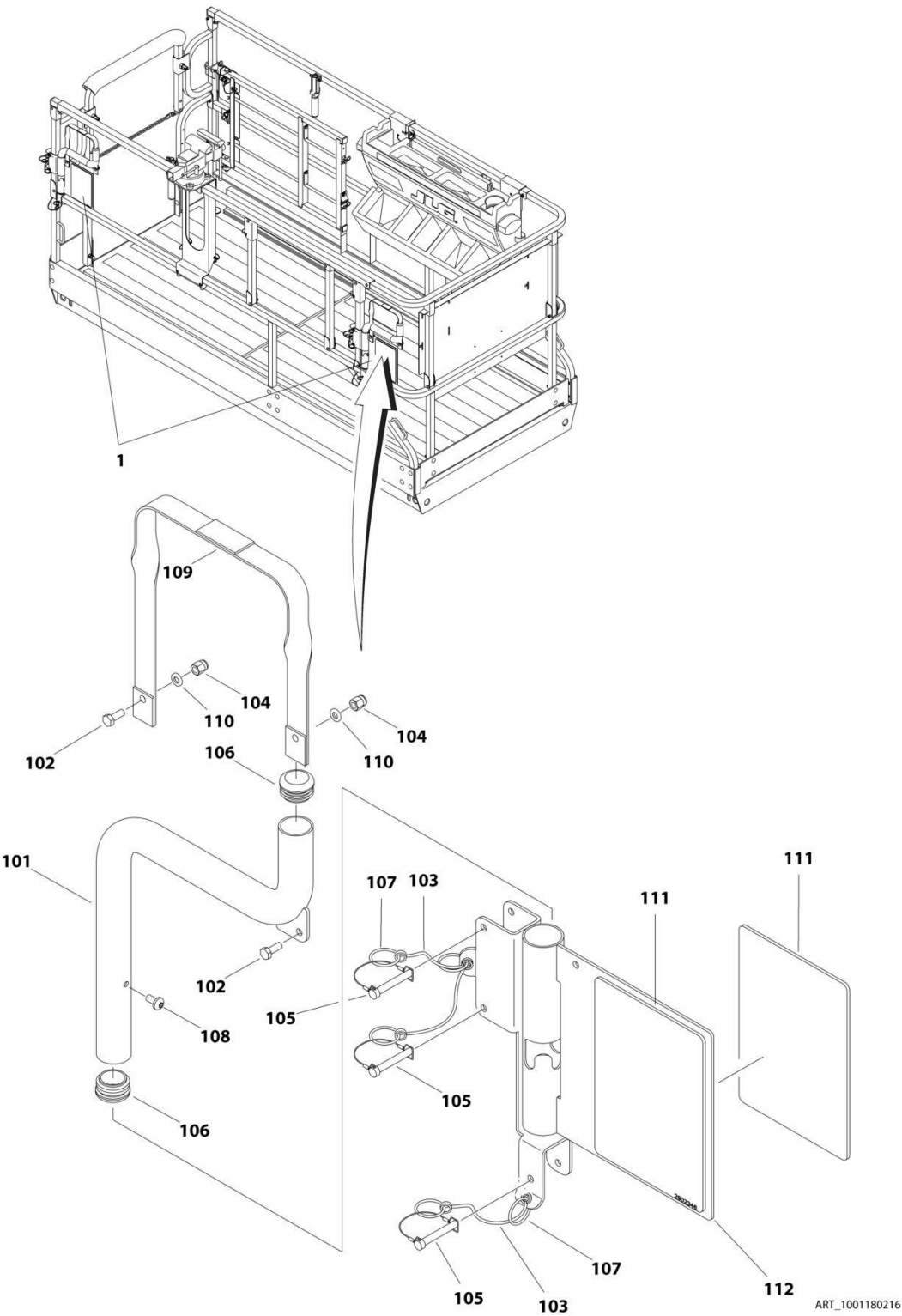
FIGURE 4-25. PIPE RACKS INSTALLATION (FACTORY INSTALLED)
