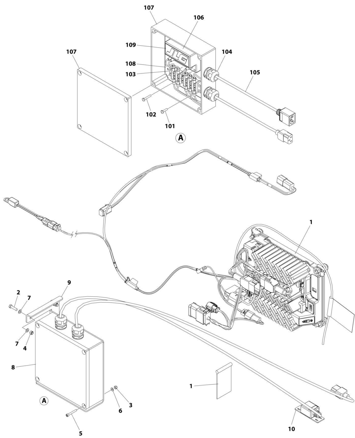
FIGURE 1-14. BATTERY CHARGER INSTALLATION - DELTA-Q WITH VOLTAGE GUARD (LOCALLY SUPPLIED PLUG) (ANSI EXPORT AND KOREA SPECS)
