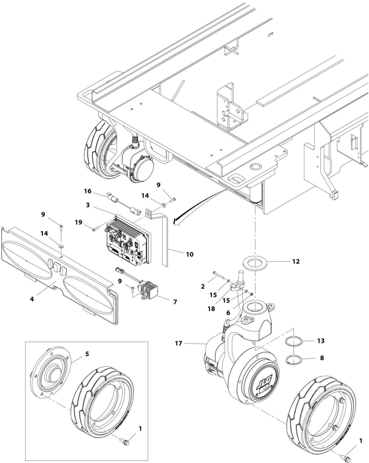
FIGURE 1-2. DRIVE HUB AND MODULE INSTALLATION (CHINA AND MEXICO BUILT MACHINES)
