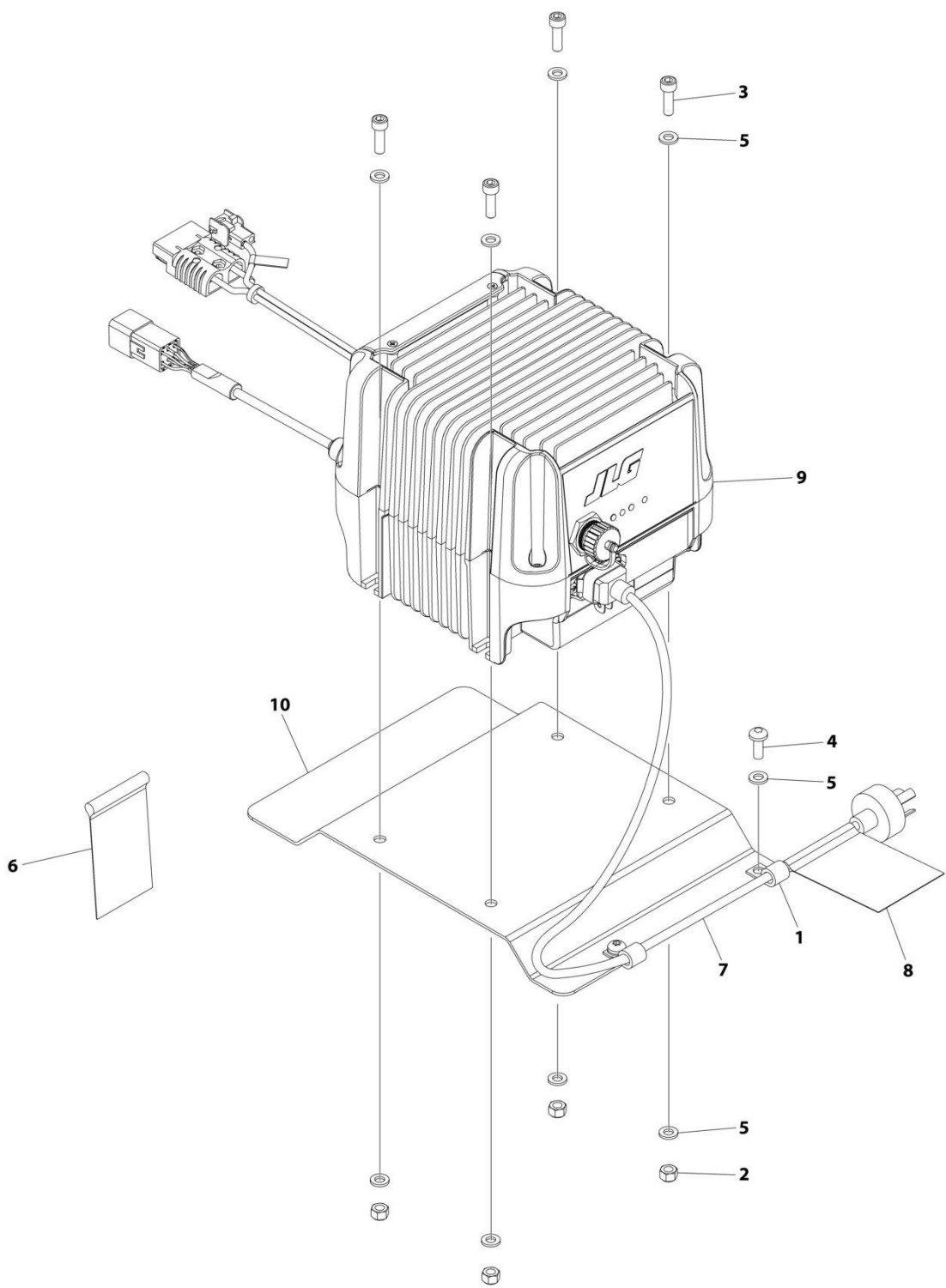
FIGURE 1-20. BATTERY CHARGER INSTALLATION - GREEN POWER (CHINESE PLUG) (CHINA SPECS)
