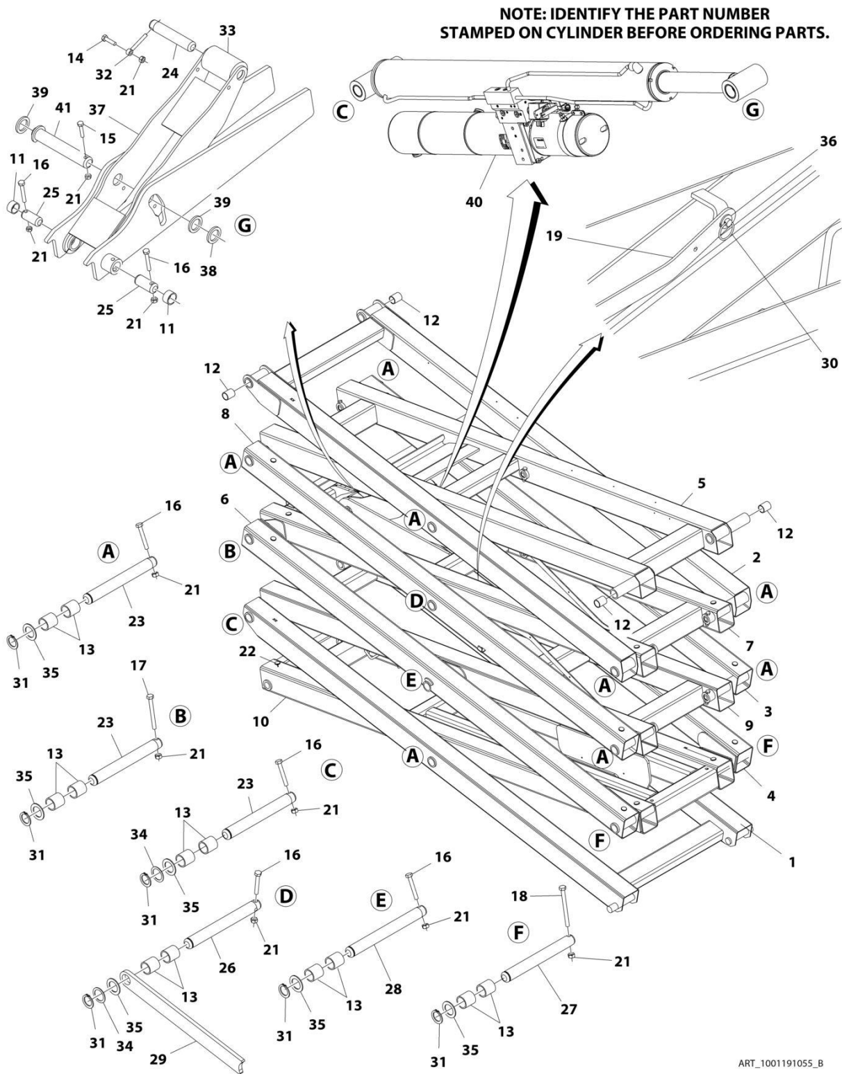
FIGURE 3-2. SCISSORS ARMS ASSEMBLY - 2646ES STANDARD HYDRAULIC OIL (BELGIUM, CHINA AND MEXICO BUILT MACHINES)
