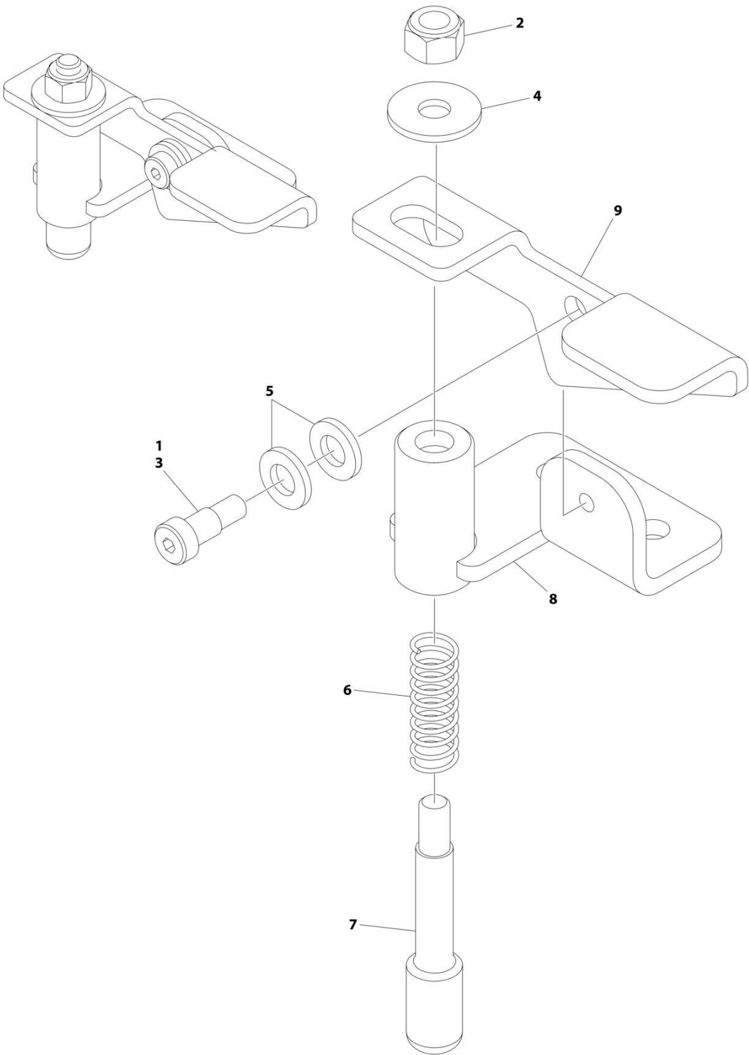
FIGURE 4-5. LATCH ASSEMBLY - WITH INSIDE EXTENSION RAILS
