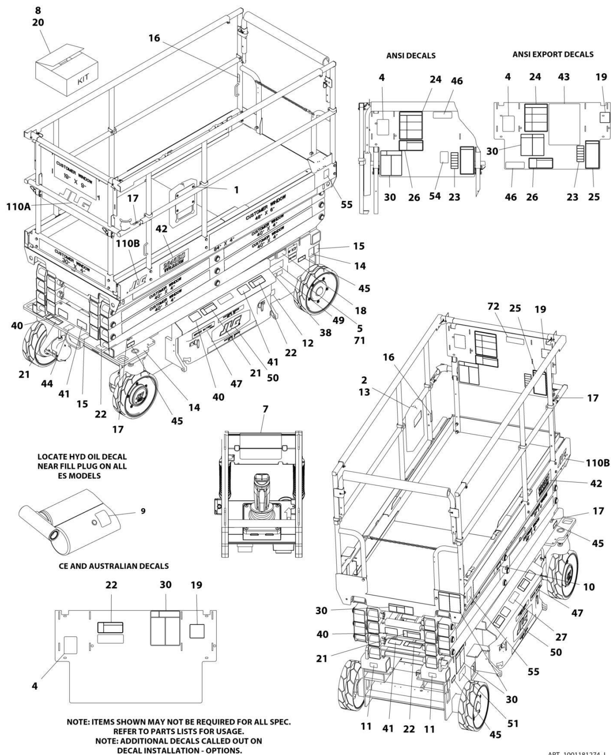
FIGURE 8-6. DECAL INSTALLATION - CHINA SPEC (CHINESE/ENGLISH)
