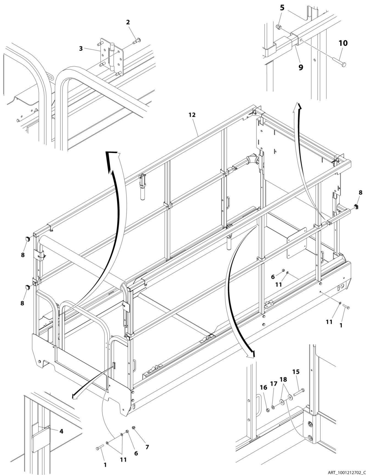
FIGURE 4-8. RAILS INSTALLATION - WITH INSIDE EXTENSION RAILS, HANDLE AND SELF CLOSING GATE
