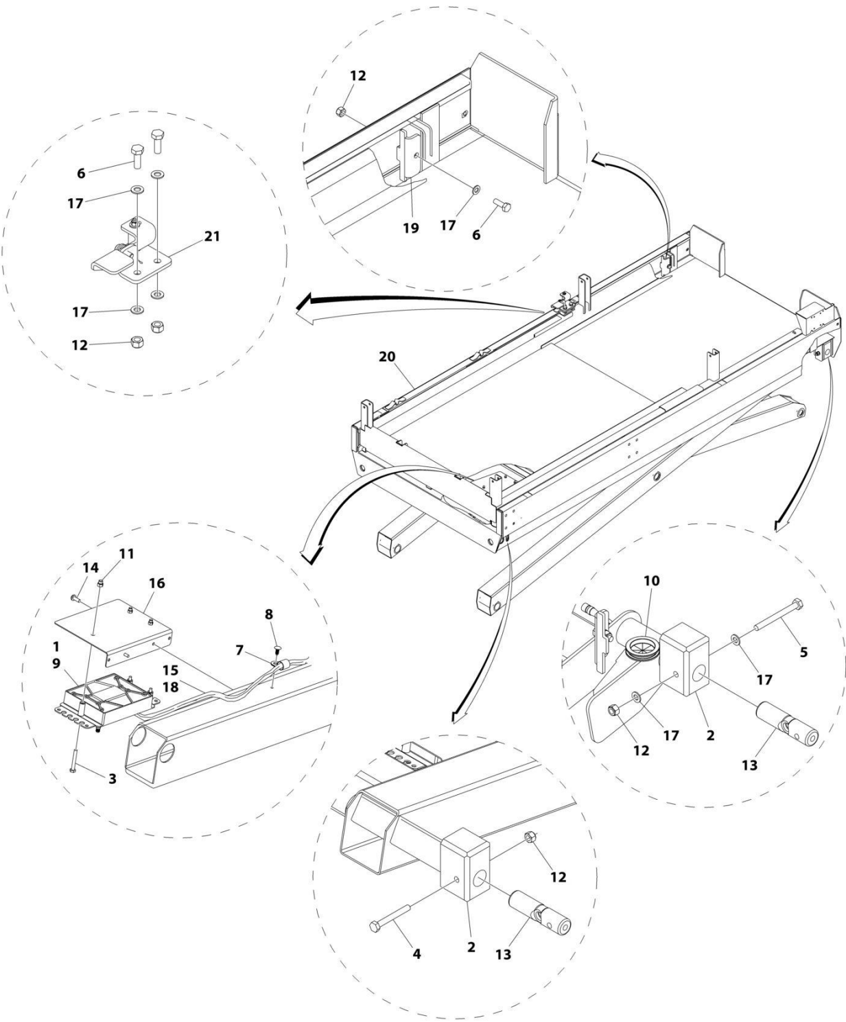
FIGURE 4-2. PLATFORM INSTALLATION - WITH OUTSIDE EXTENSION RAILS AND WITH LSS
