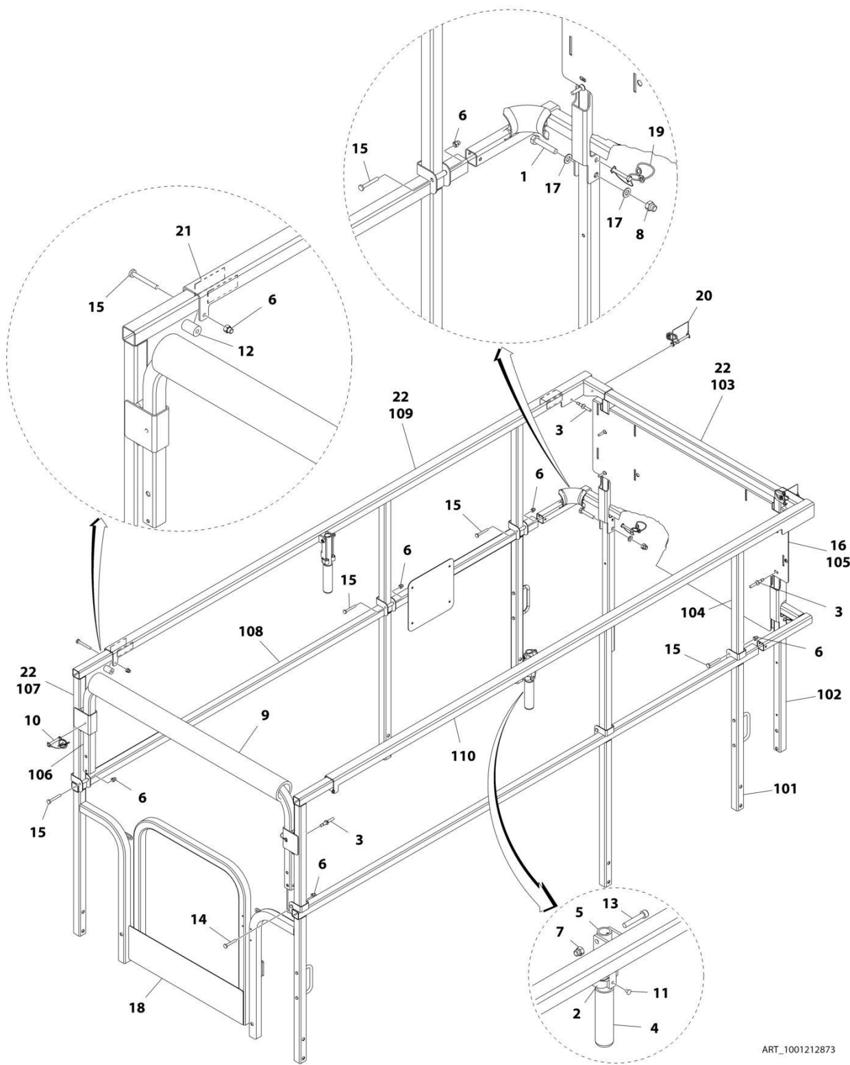
FIGURE 4-11. RAIL KIT - WITH INSIDE EXTENSION RAILS, HANDLE AND SELF CLOSING GATE
