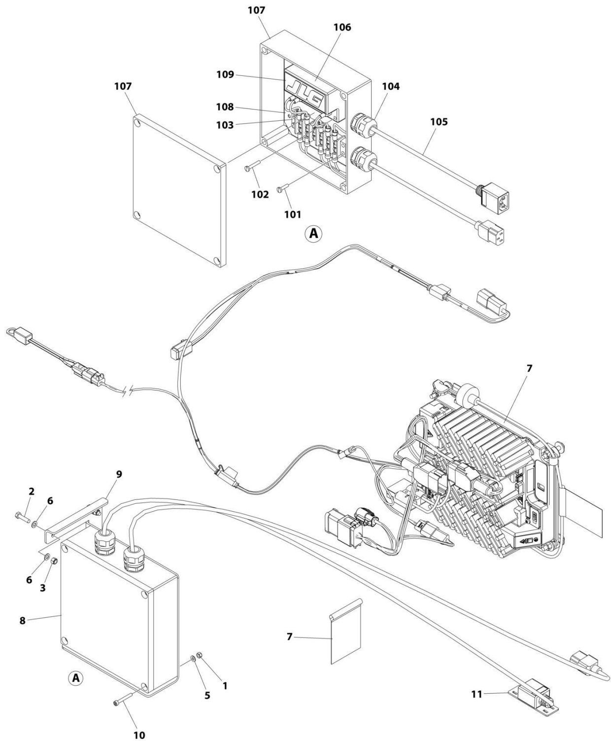
FIGURE 1-15. BATTERY CHARGER INSTALLATION - DELTA-Q WITH VOLTAGE GUARD AND CHINESE PLUG (ANSI EXPORT AND KOREA SPECS)
