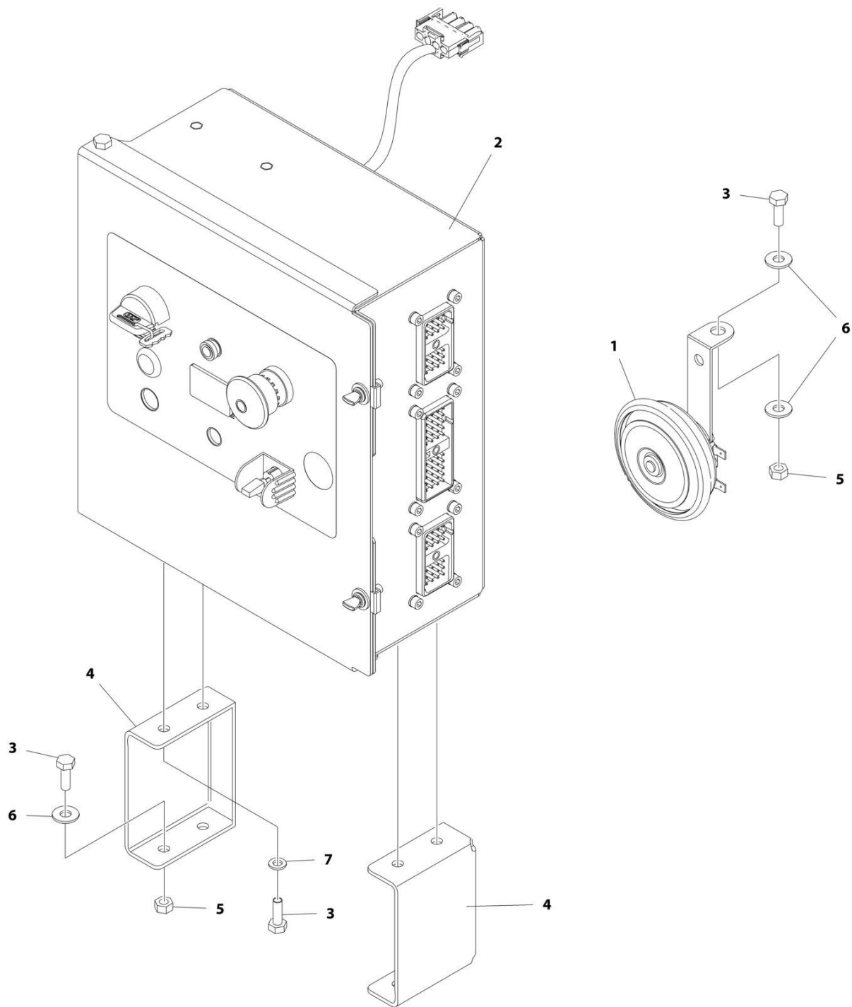
FIGURE 2-9. GROUND CONTROL BOX AND HORN INSTALLATIONS - M3369/M4069 (2WD - ALL SPECS EXCEPT CE SPEC)
