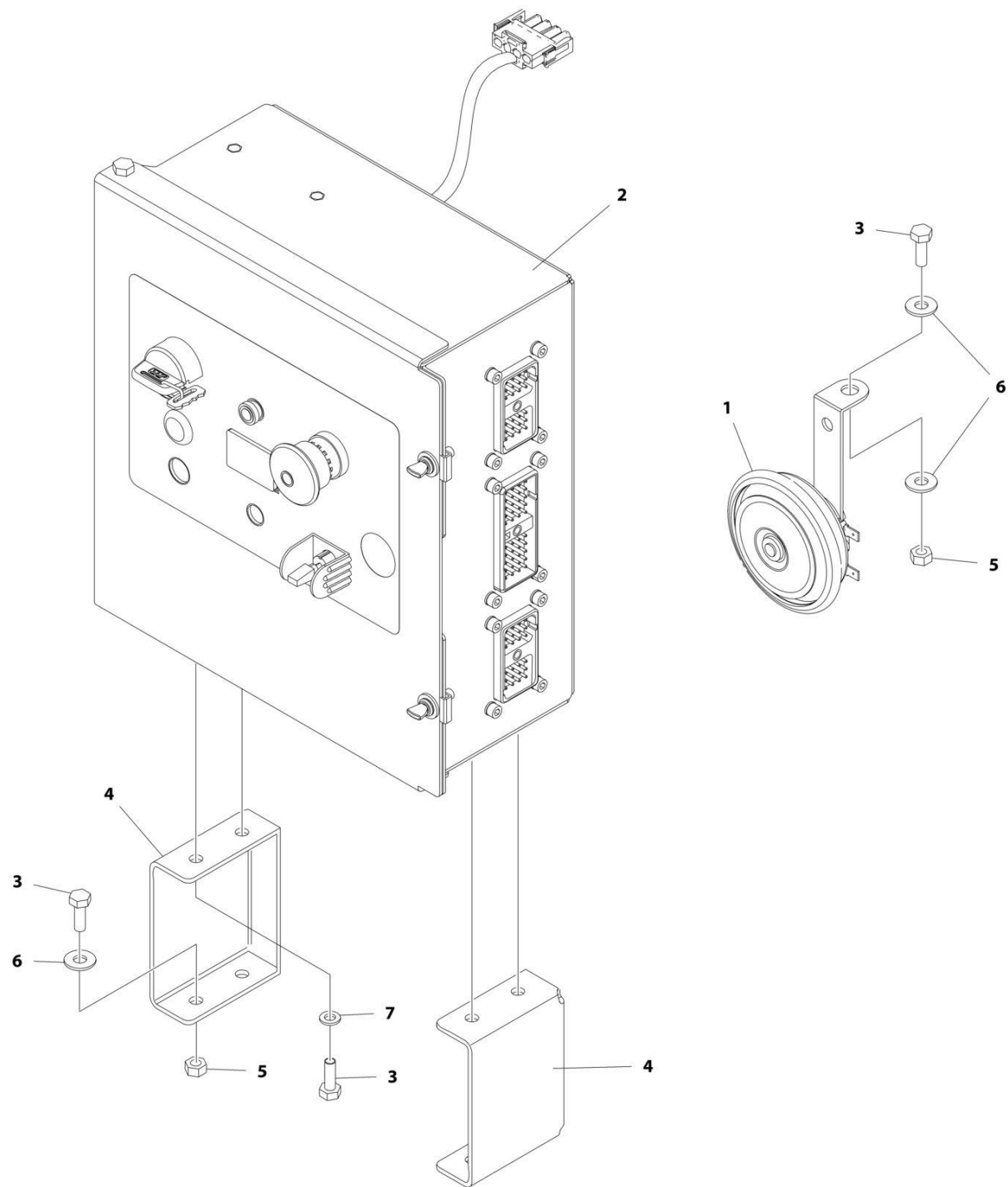
FIGURE 2-8. GROUND CONTROL BOX AND HORN INSTALLATIONS - 3369LE/4069LE WITH LEVELING JACKS (CE SPEC)
