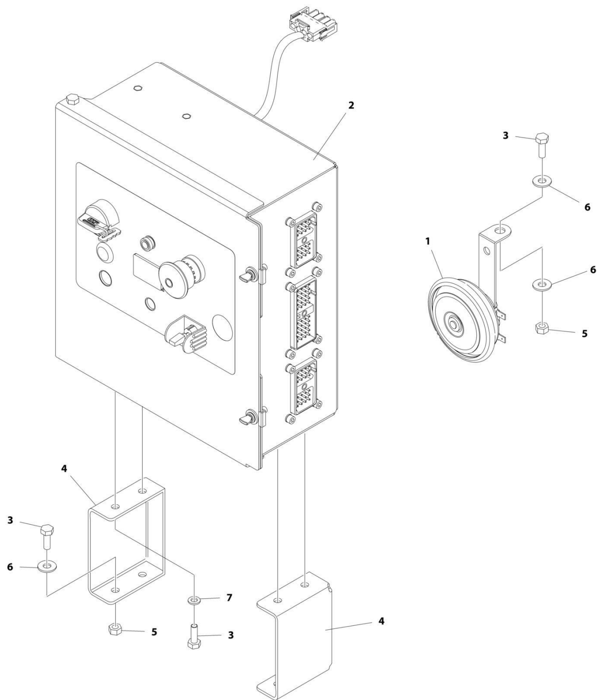
FIGURE 2-5. GROUND CONTROL BOX AND HORN INSTALLATIONS - 3369LE/4069LE WITHOUT LEVELING JACKS (ALL SPECS EXCEPT CE SPEC)
