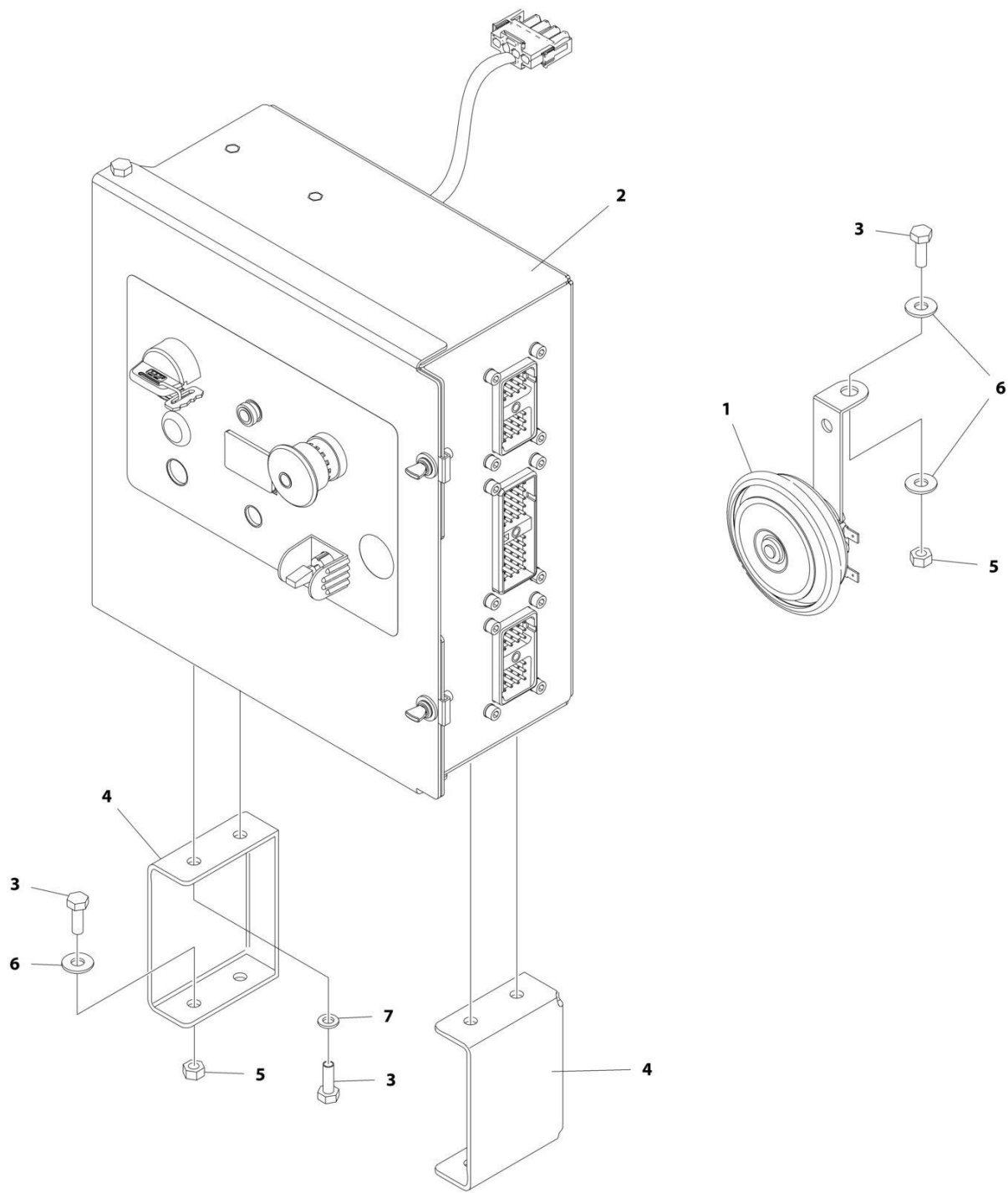
FIGURE 2-12. GROUND CONTROL BOX AND HORN INSTALLATIONS - M3369/M4069 (4WD - CE SPEC)
