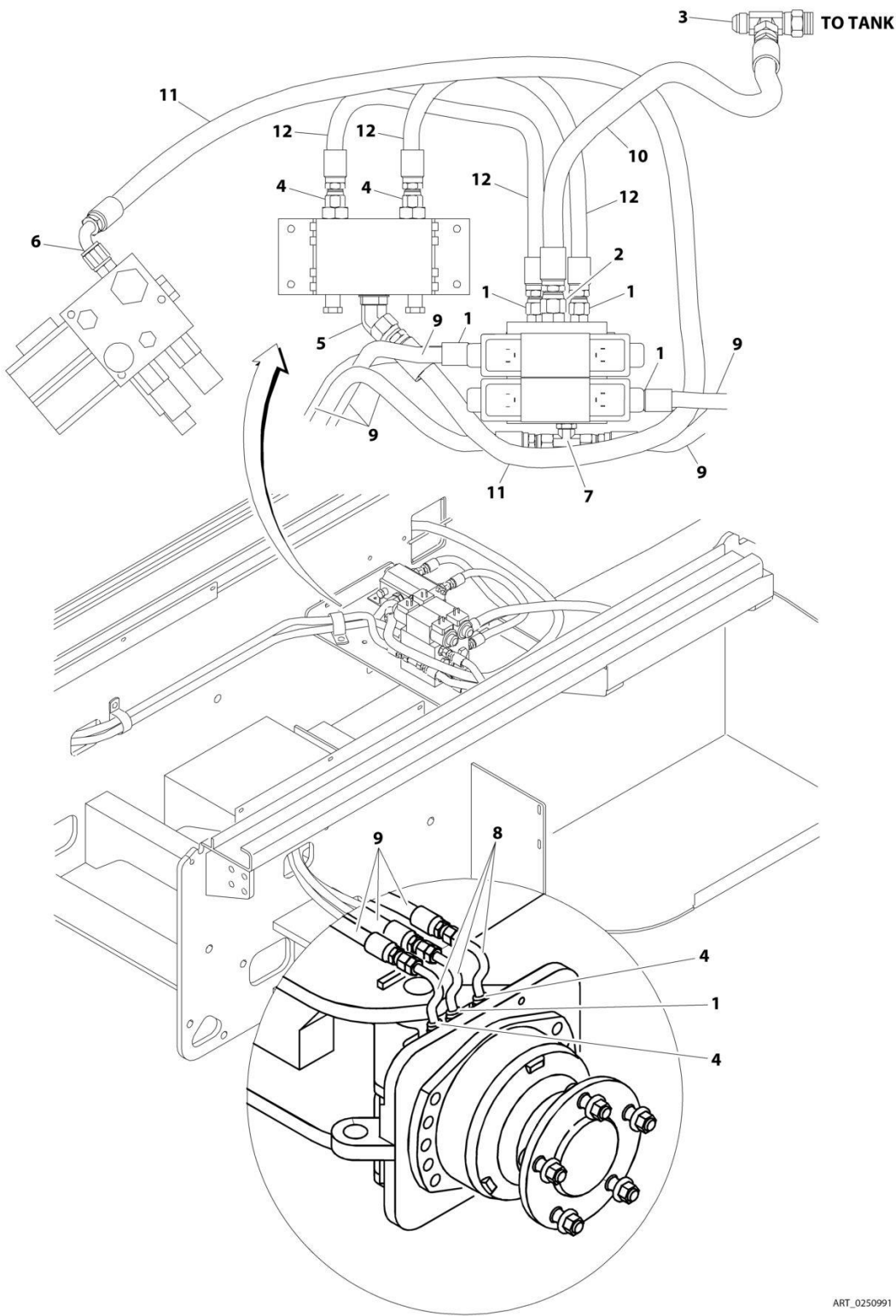
FIGURE 7-1. HYDRAULIC DIAGRAM - 4WD
