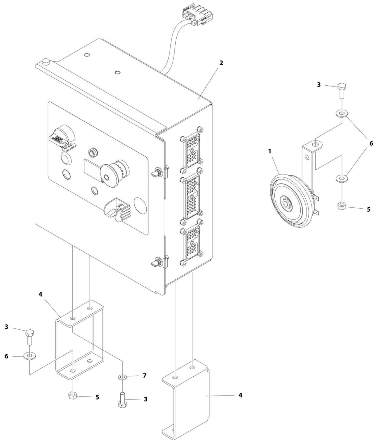
FIGURE 2-7. GROUND CONTROL BOX AND HORN INSTALLATIONS - 3369LE/4069LE WITH LEVELING JACKS (ALL SPECS EXCEPT CE SPEC)
