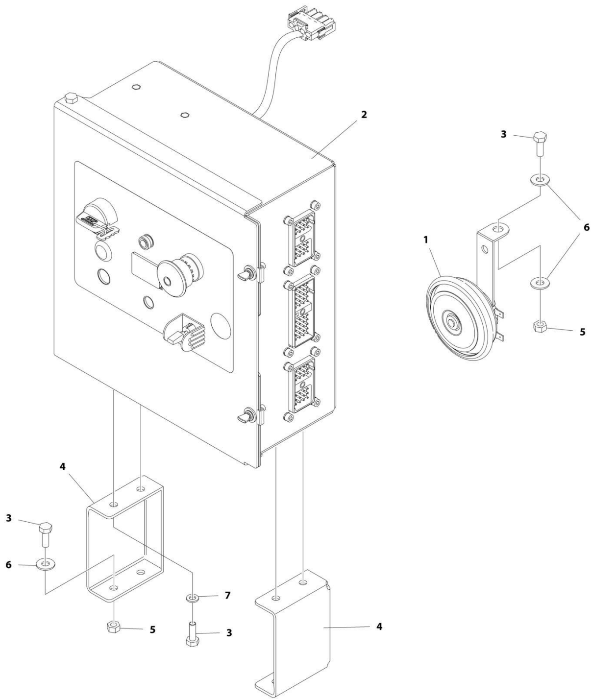
FIGURE 2-13. GROUND CONTROL BOX AND HORN INSTALLATIONS - M4069 (DRIVE AT FULL HEIGHT)
