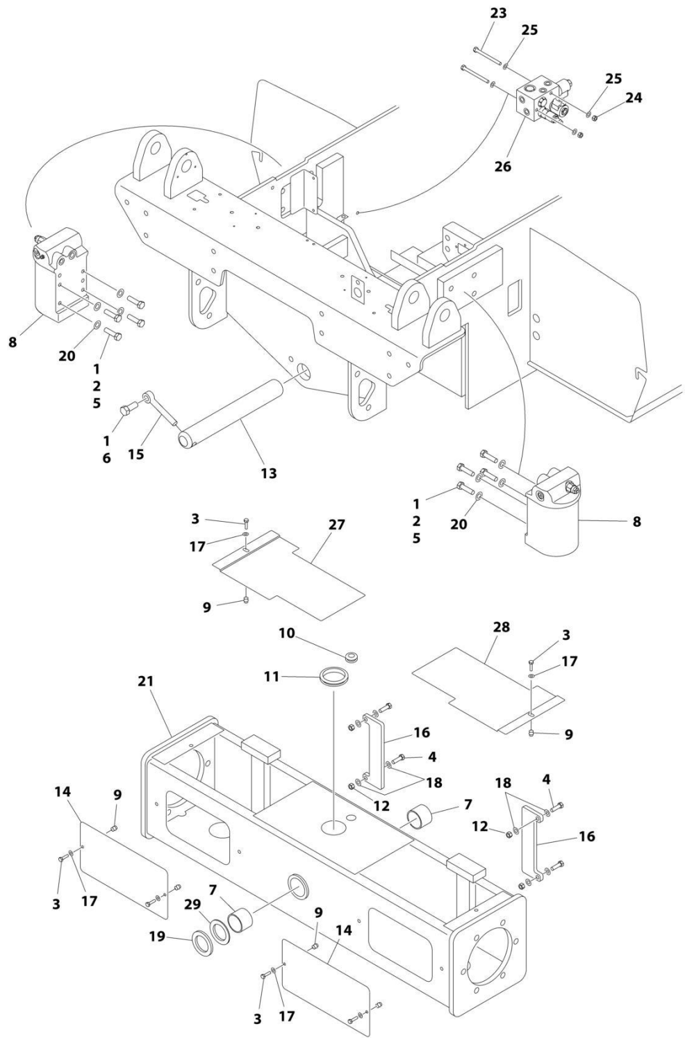
FIGURE 1-2. REAR AXLE INSTALLATION - OSCILLATING (ALL SPECS EXCEPT CE SPEC)
