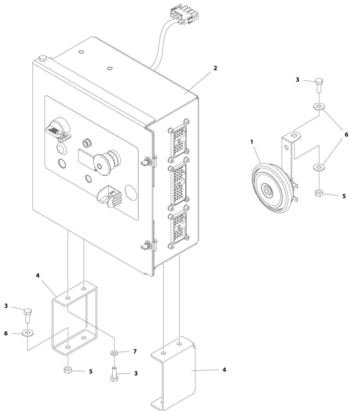
FIGURE 2-11. GROUND CONTROL BOX AND HORN INSTALLATIONS - M3369/M4069 (4WD - ALL SPECS EXCEPT CE SPEC)
