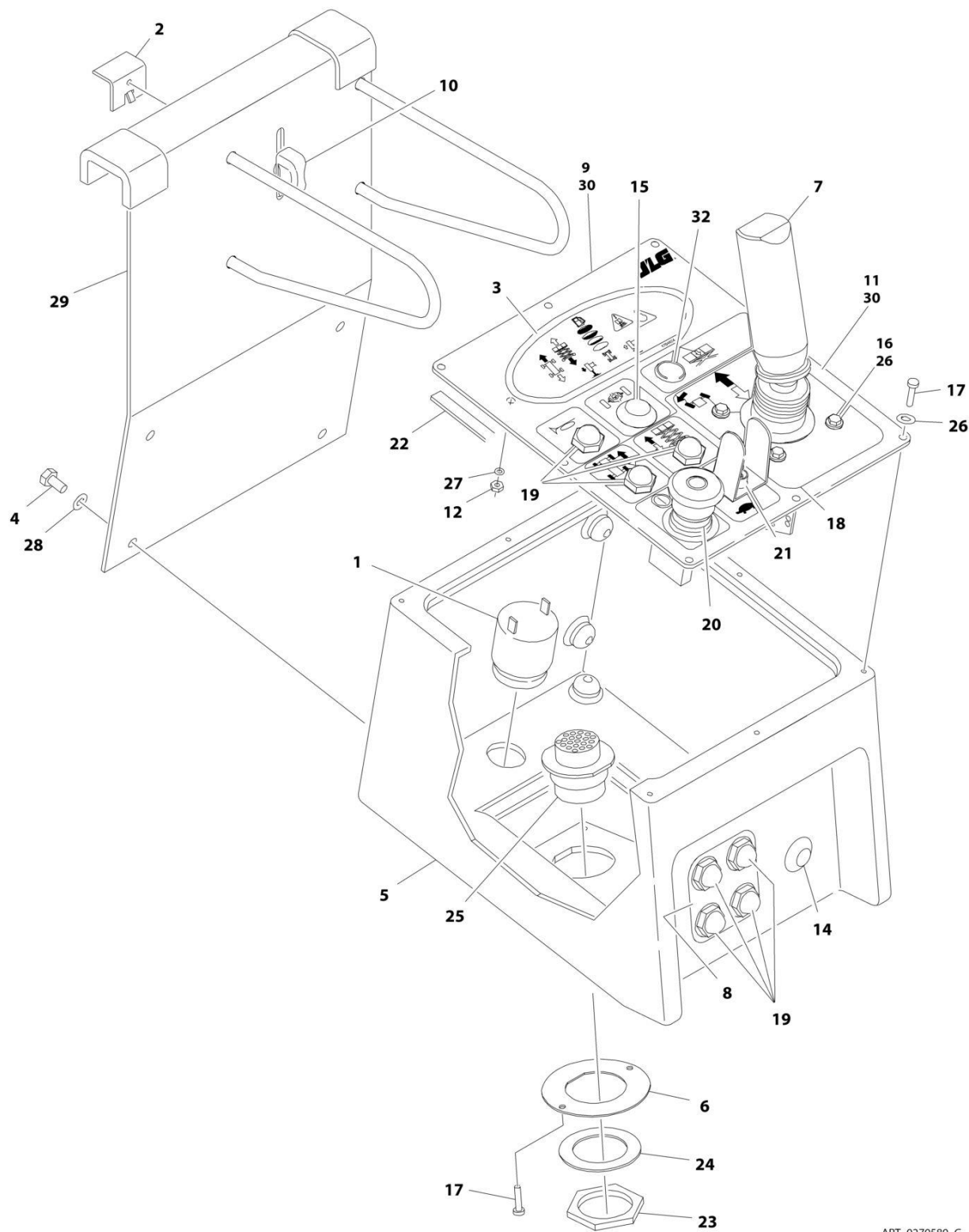
FIGURE 5-6. CONSOLE BOX ASSEMBLY - 3369LE/4069LE WITH LEVELING JACKS
