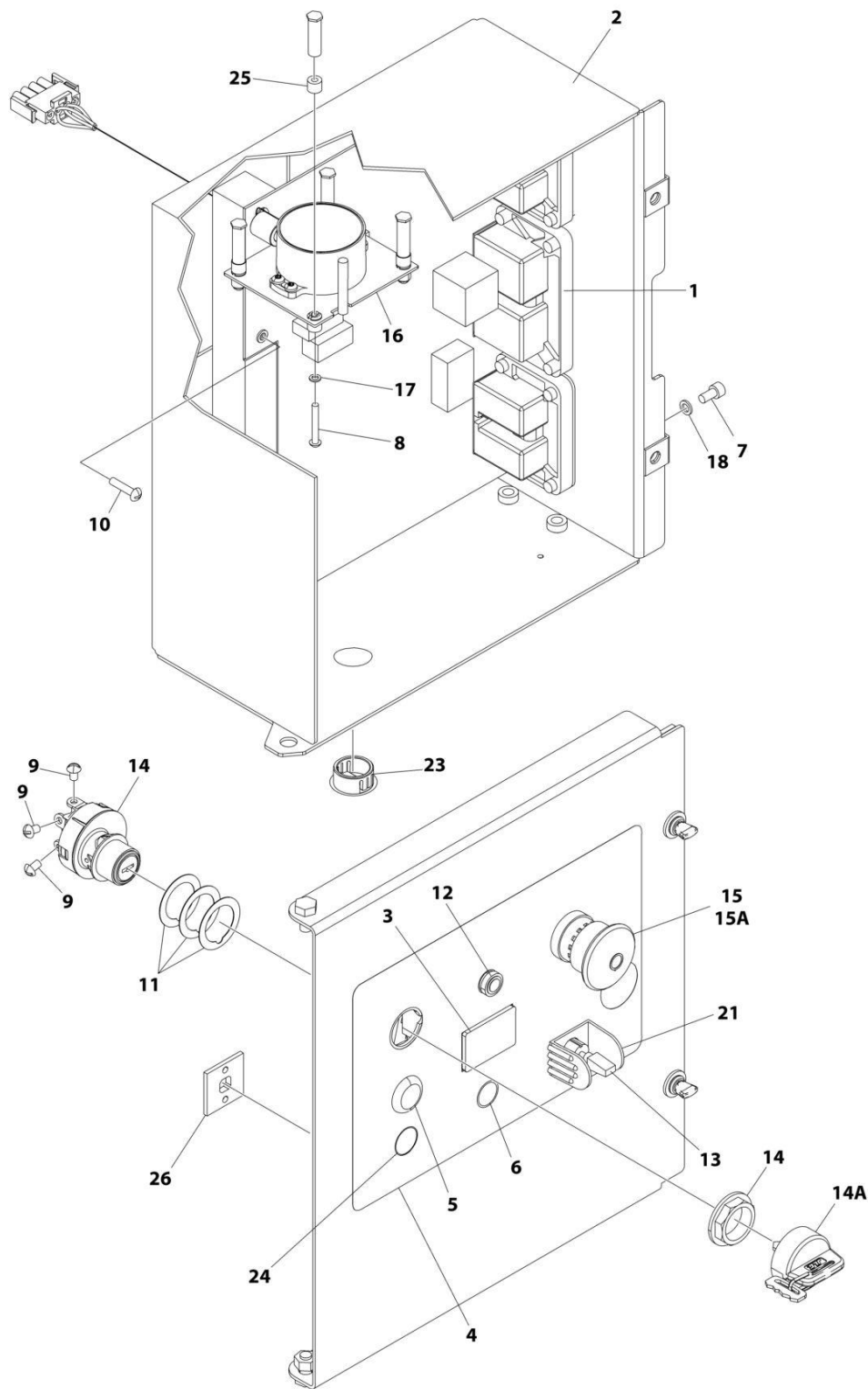
FIGURE 2-14. GROUND CONTROL BOX ASSEMBLY - 3369LE/4069LE (ALL SPECS EXCEPT CE SPEC)
