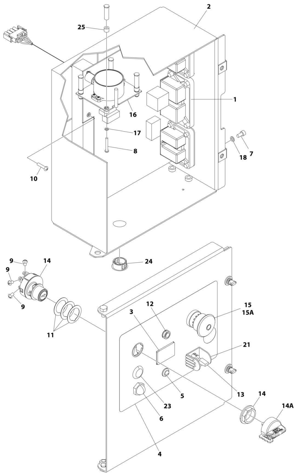
FIGURE 2-16. GROUND CONTROL BOX ASSEMBLY - M3369/M4069 (ALL SPECS EXCEPT CE SPEC)
