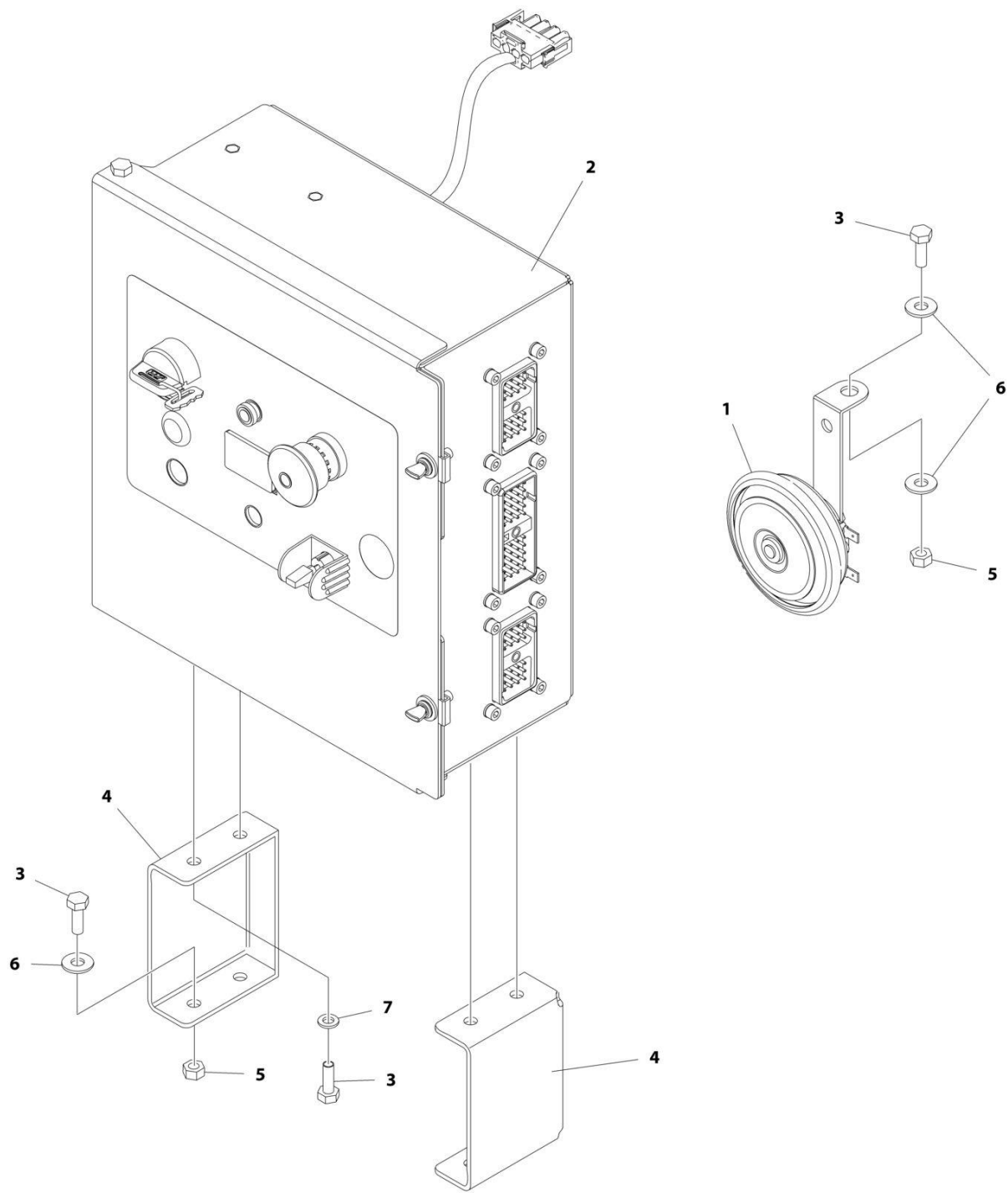
FIGURE 2-6. GROUND CONTROL BOX AND HORN INSTALLATIONS - 3369LE/4069LE WITHOUT LEVELING JACKS (CE SPEC)
