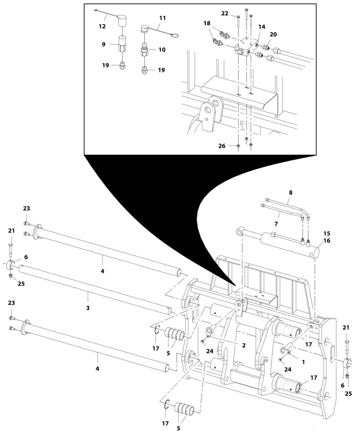
FIGURE 3-10. SIDE SHIFT CARRIAGE ASSEMBLY (50 INCH)
