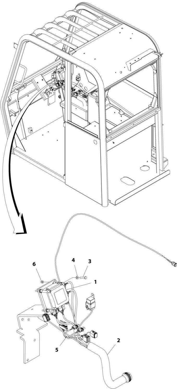
FIGURE 6-5. ELECTRICAL OPTIONS INSTALLATION
