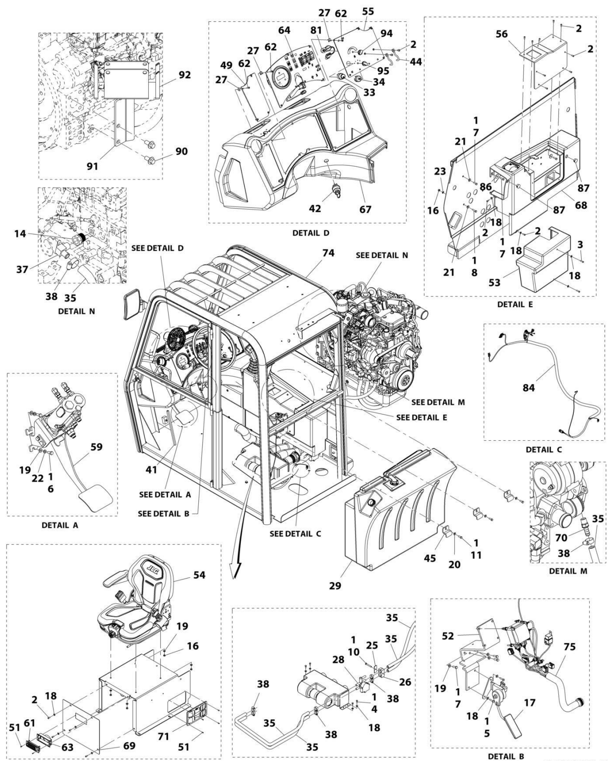
FIGURE 6-9. ENCLOSED CAB
