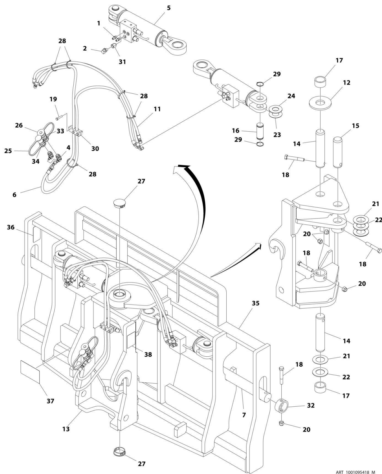
FIGURE 3-14. 90 SWING CARRIAGE ASSEMBLY (72 INCH)
