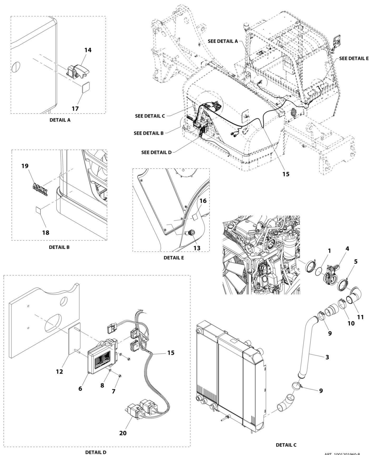
FIGURE 4-15. AIR INTAKE SHUT OFF VALVE INSTALLATION
