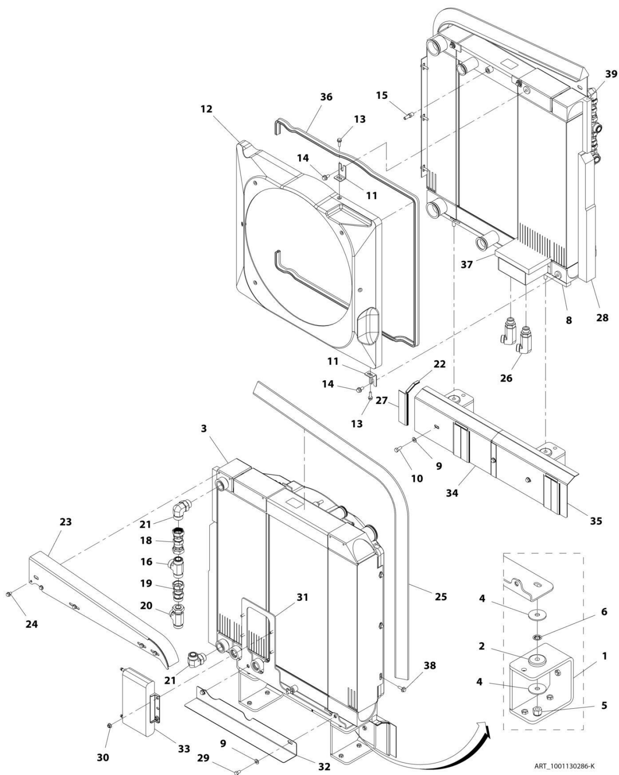
FIGURE 4-5. COOLER INSTALLATION
