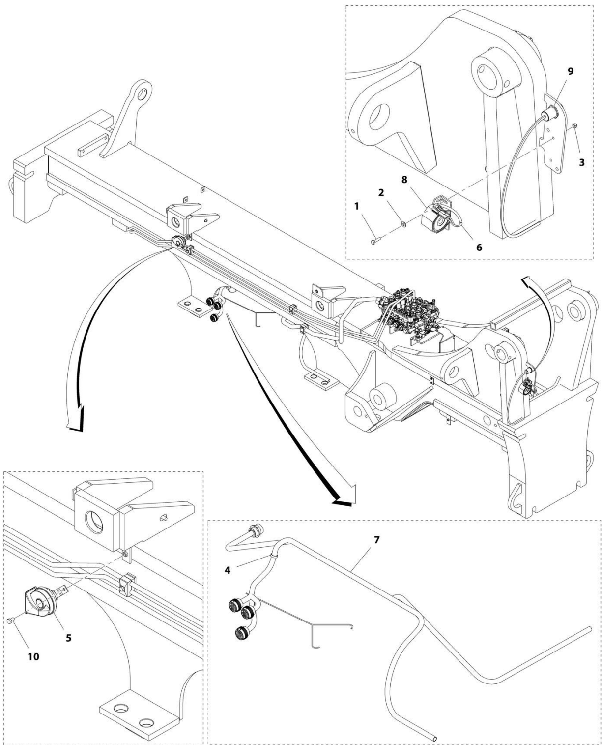
FIGURE 10-6. ELECTRICAL INSTALLATION
