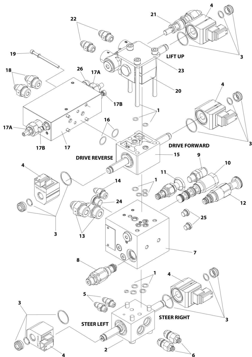
FIGURE 2-2. VALVE ASSEMBLY
