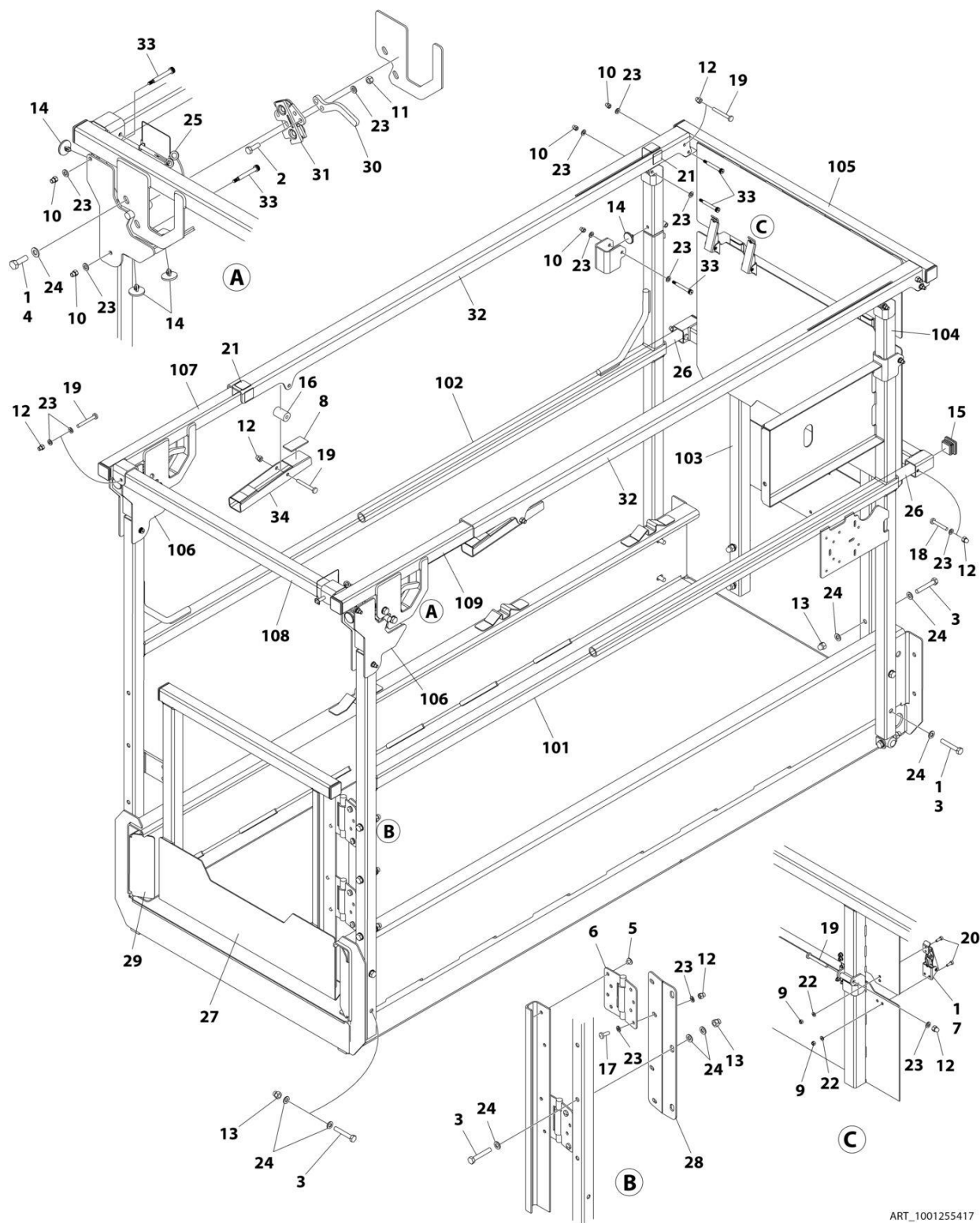
FIGURE 4-10. RAILS INSTALLATION - FOLD-DOWN RAILS/GATE ENTRY (QUIK FOLD) (INSIDE TUBE SLIDER)
