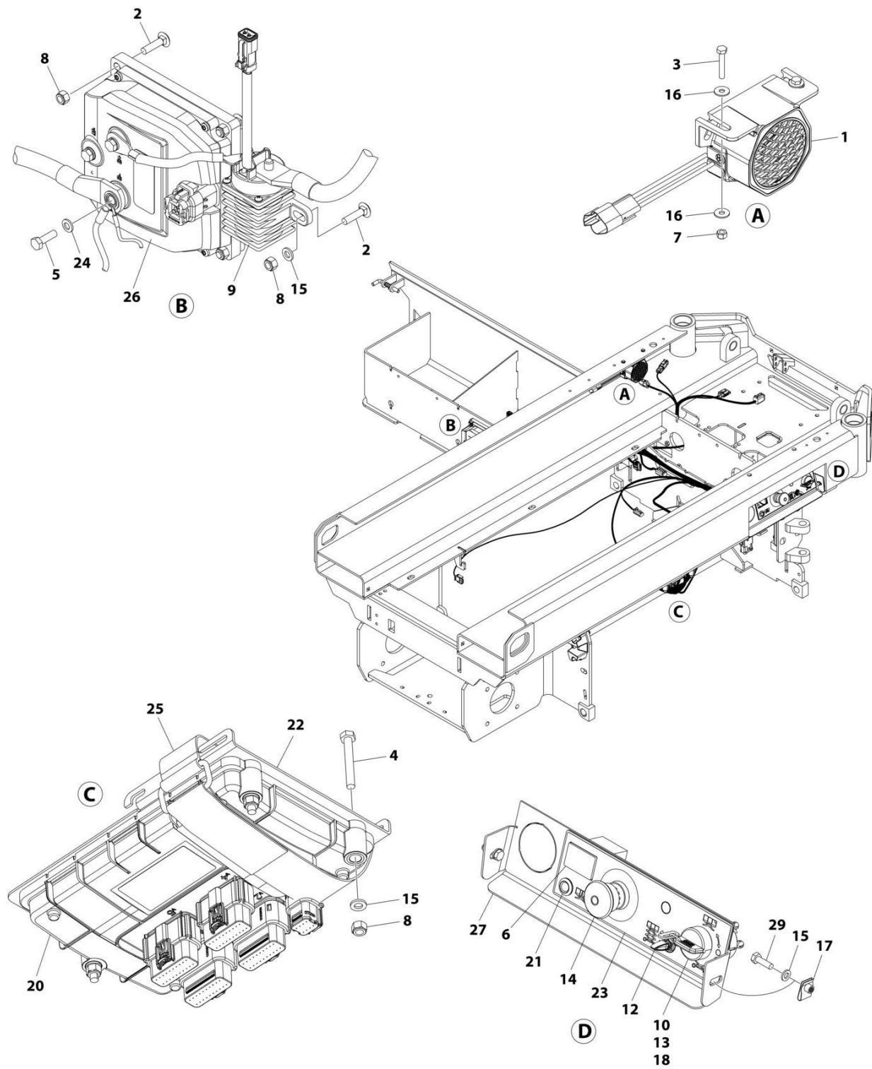
FIGURE 2-5. ELECTRICAL COMPONENTS INSTALLATION (MACHINES WITH SN STARTING WITH M2)
