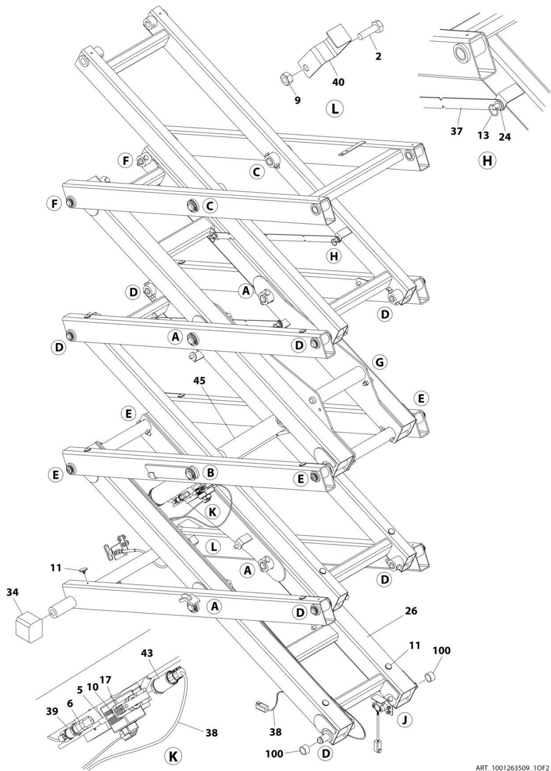
FIGURE 3-8. SCISSORS ARMS INSTALLATION – R1932/R1932i (MACHINES WITH SN STARTING WITH G2)
