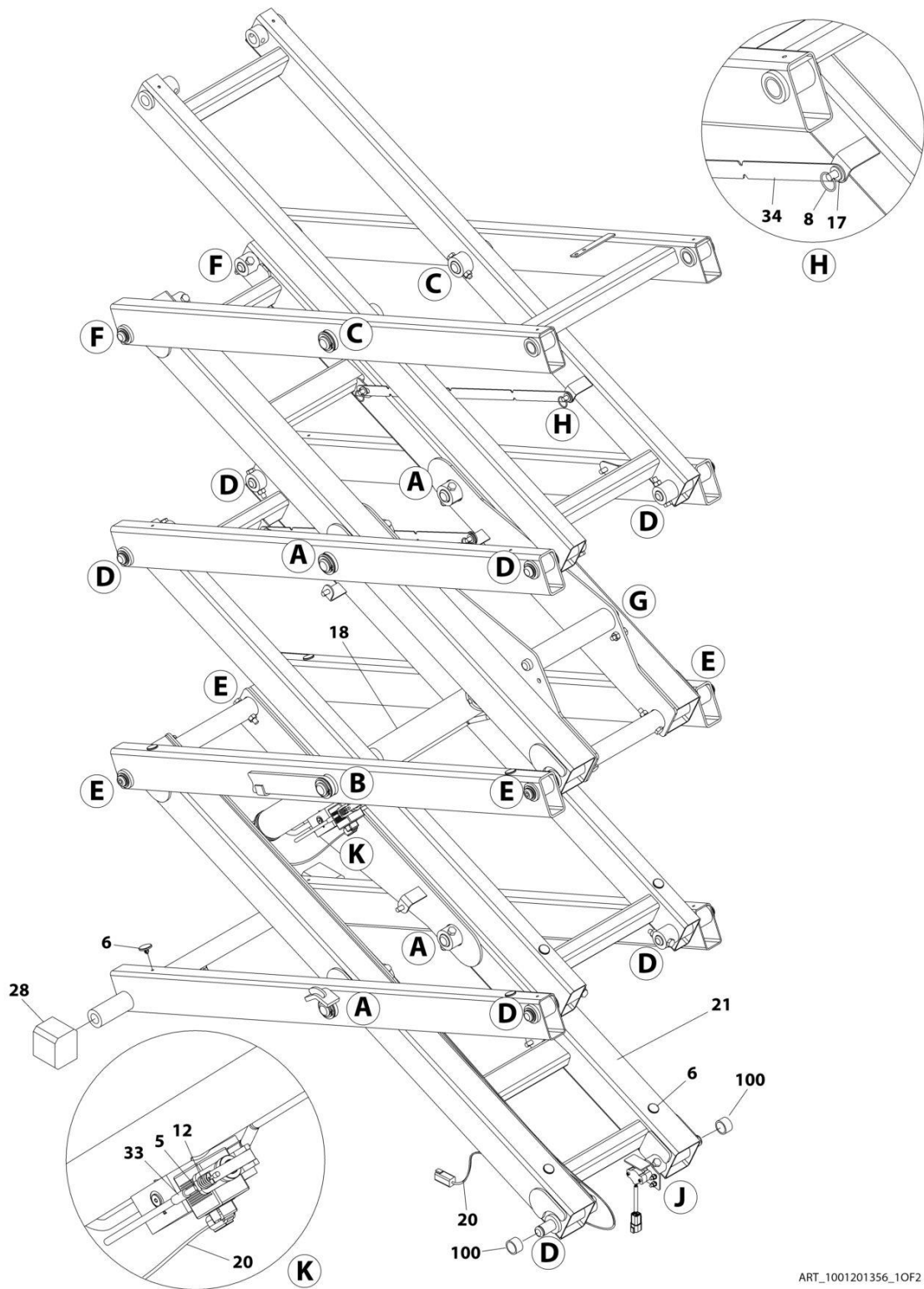
FIGURE 3-6. SCISSORS ARMS INSTALLATION - R1932 WITHOUT LSS
