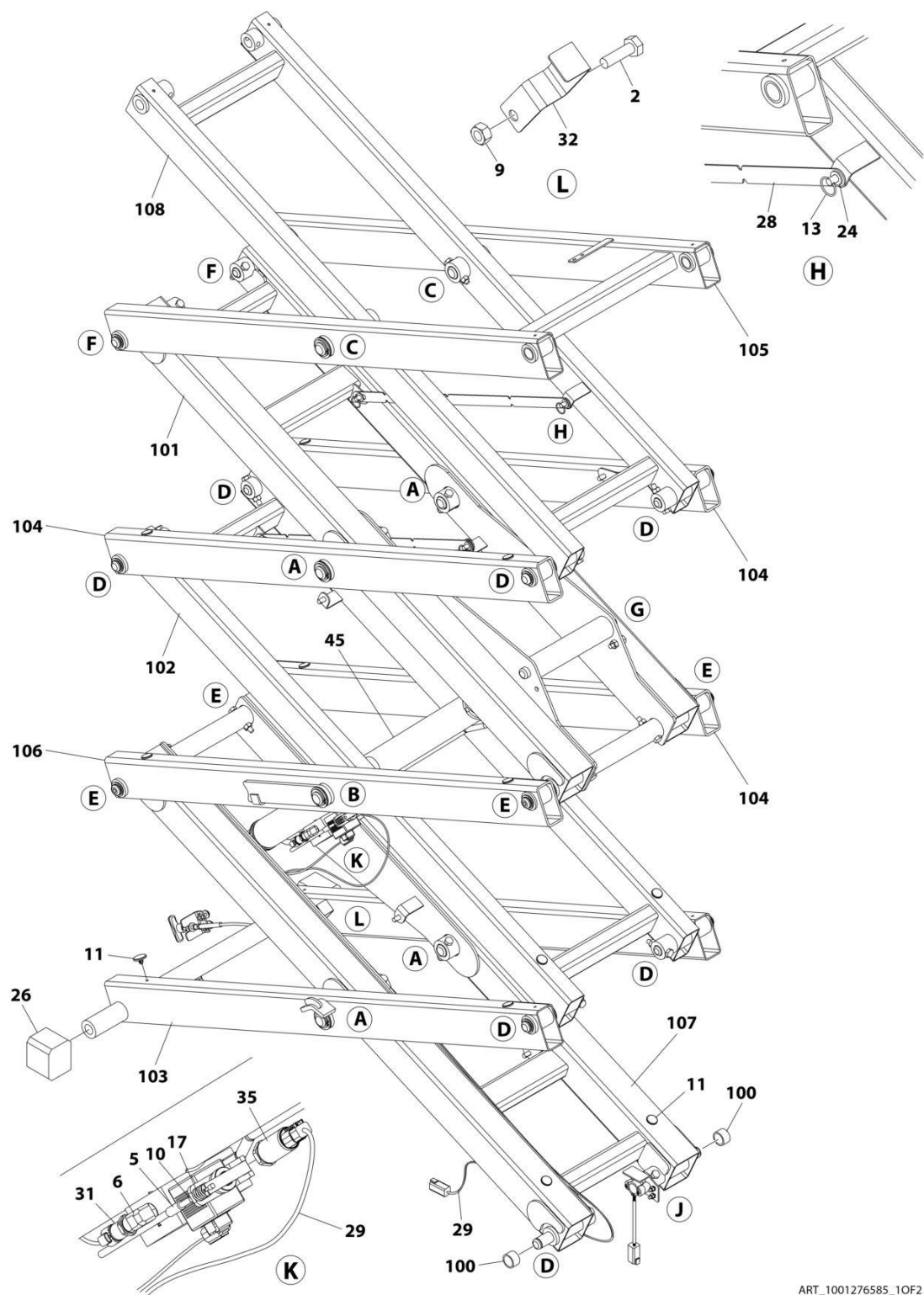
FIGURE 3-9. SCISSORS ARMS INSTALLATION (MACHINES WITH SN STARTING WITH 12)
