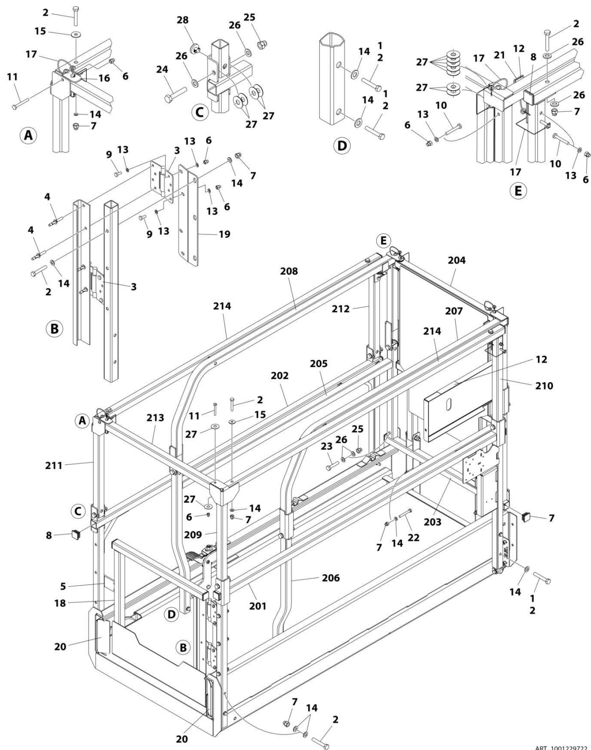
FIGURE 4-11. RAILS INSTALLATION - FOLD-DOWN RAILS/GATE ENTRY (OUTSIDE TUBE SLIDER)
