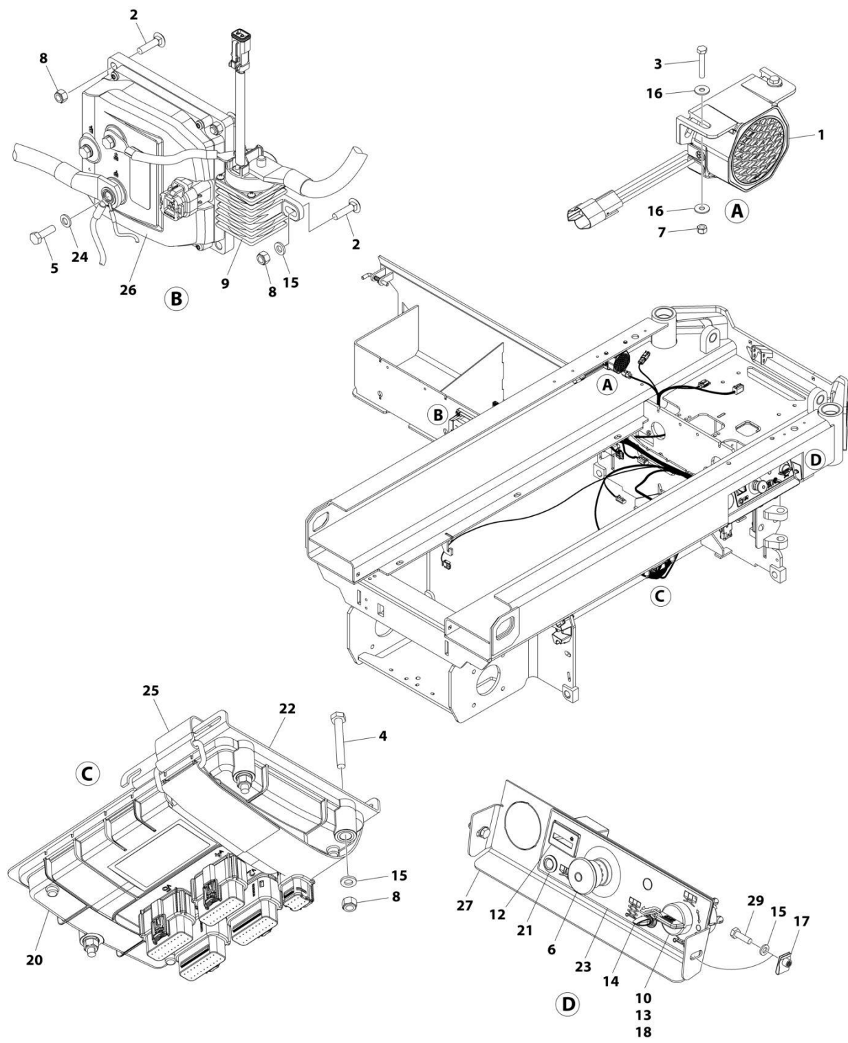
FIGURE 2-17. GROUND CONTROL INSTALLATION (MACHINES WITH SN STARTING WITH G2)
