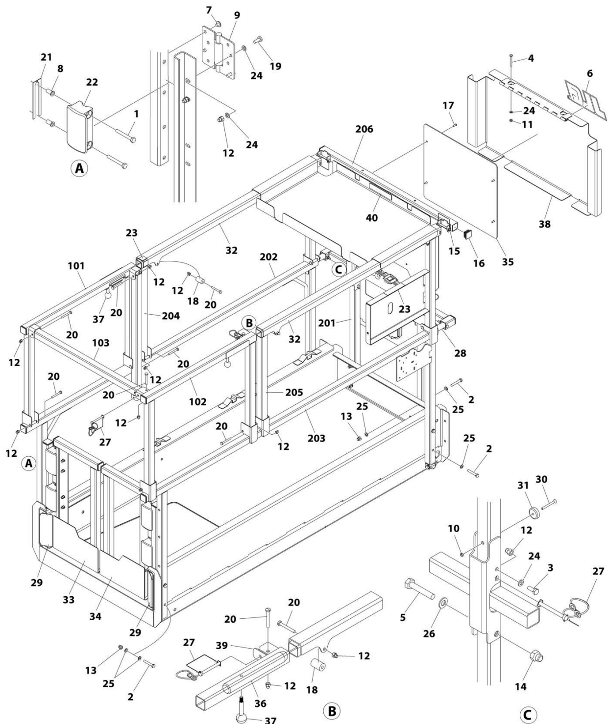
FIGURE 4-12. RAILS INSTALLATION - FOLD-DOWN RAILS/GATE ENTRY (NARROW ACCESS)
