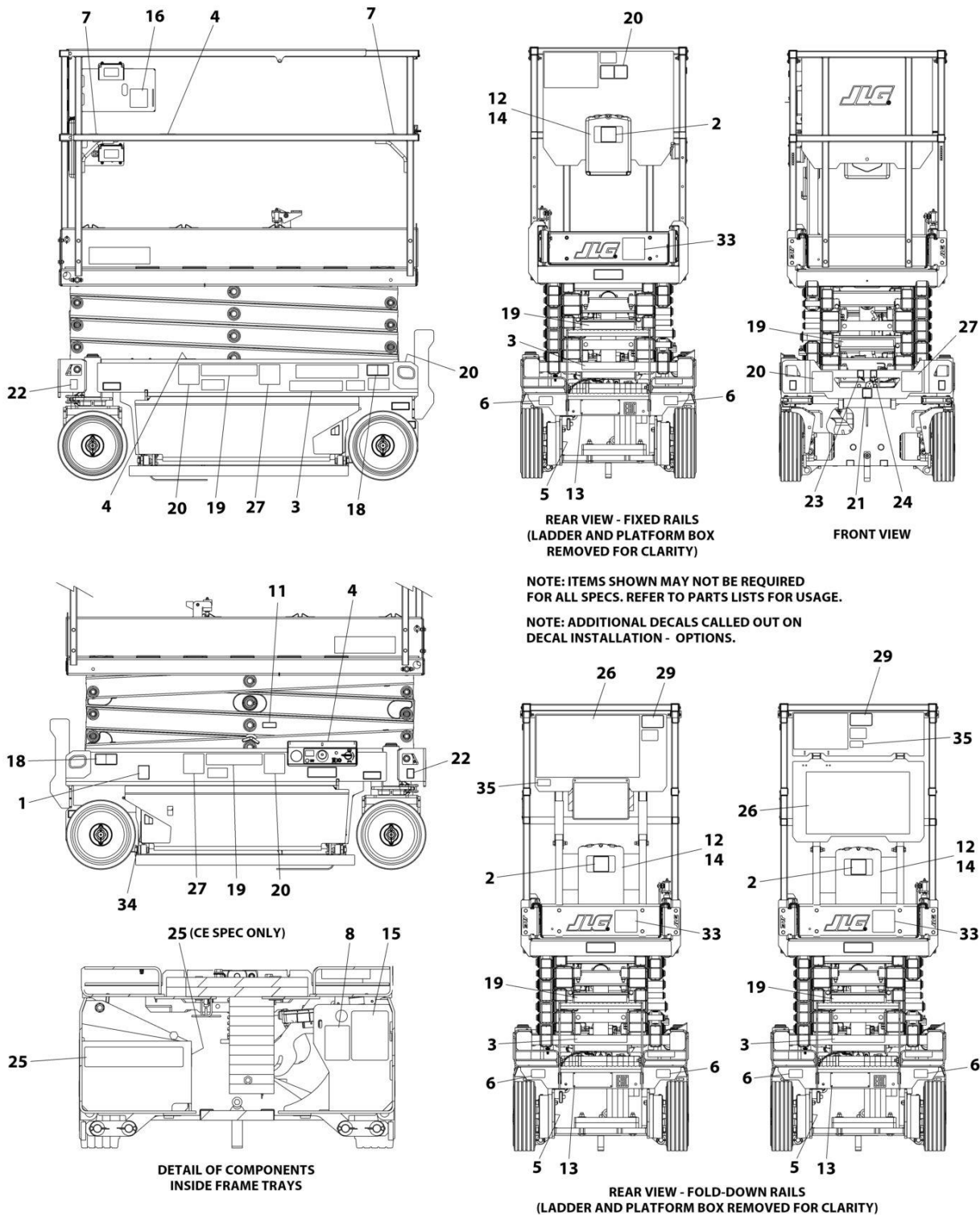
FIGURE 8-8. DECAL INSTALLATION (LATIN AMERICAN SPECS)
