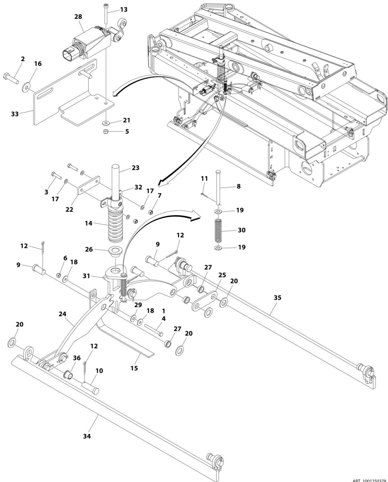
FIGURE 1-10. POTHOLE PROTECTION SYSTEM INSTALLATION
