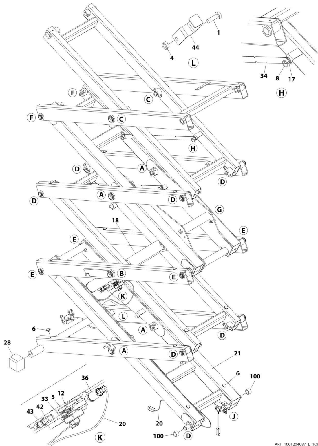
FIGURE 3-7. SCISSORS ARMS INSTALLATION – R1932/R1932i (MACHINES WITH SN STARTING WITH M2)
