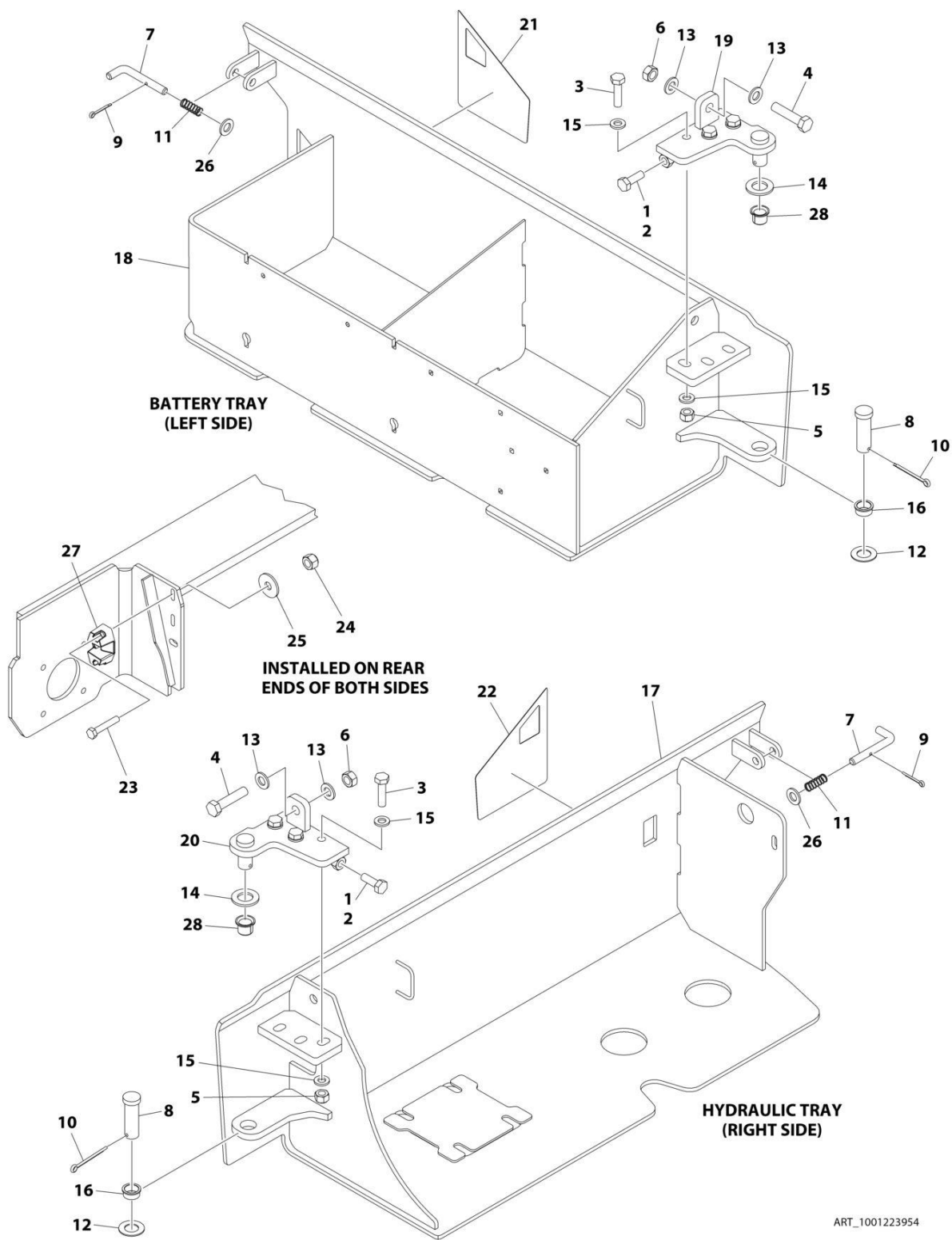
FIGURE 2-14. DOORS INSTALLATION (1532R)
