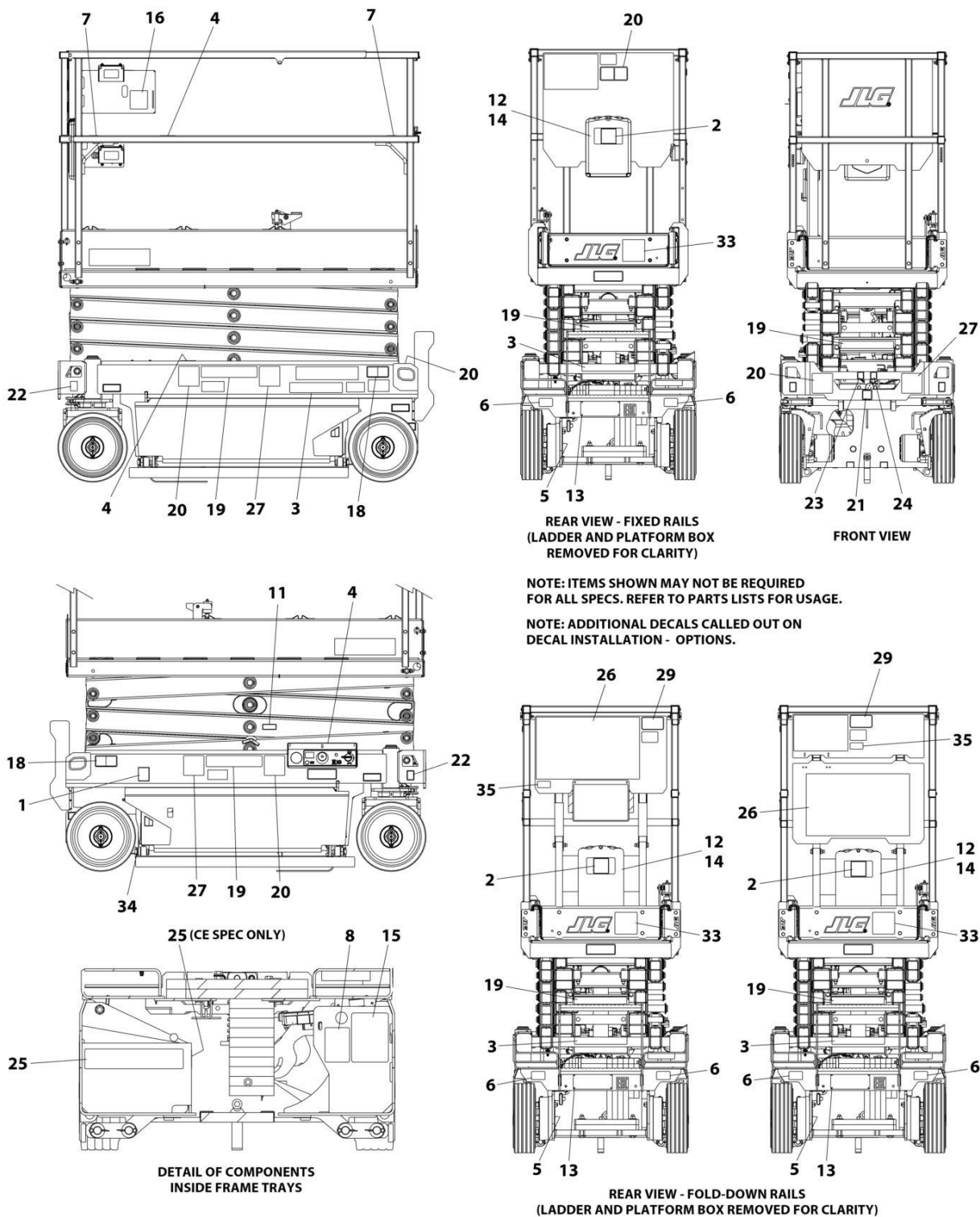
FIGURE 8-2. DECAL INSTALLATION (AUSTRALIAN SPECS)
