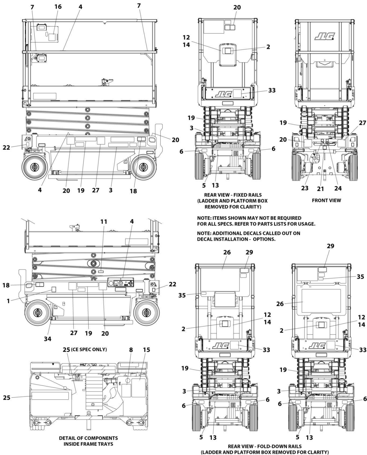
FIGURE 8-4. DECAL INSTALLATION (CE & UK CA SPECS)
