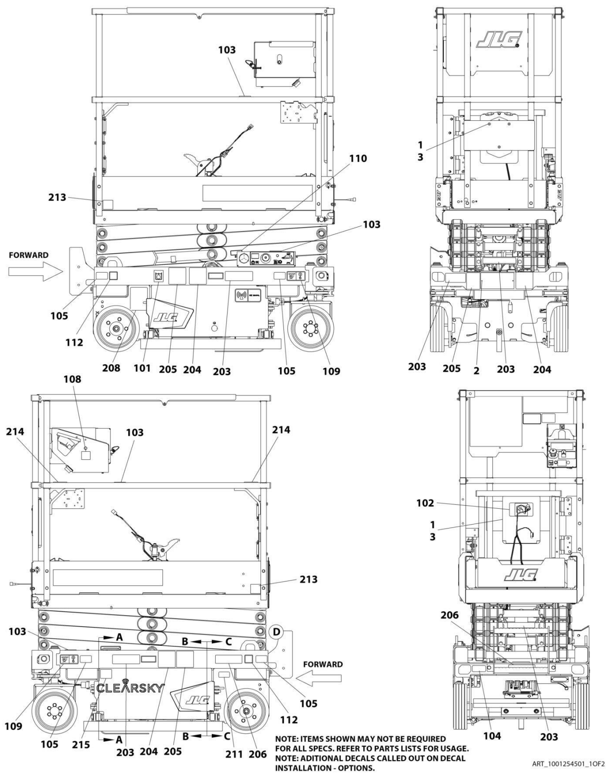
FIGURE 8-4. DECALS INSTALLATION (CSA SPECS)
