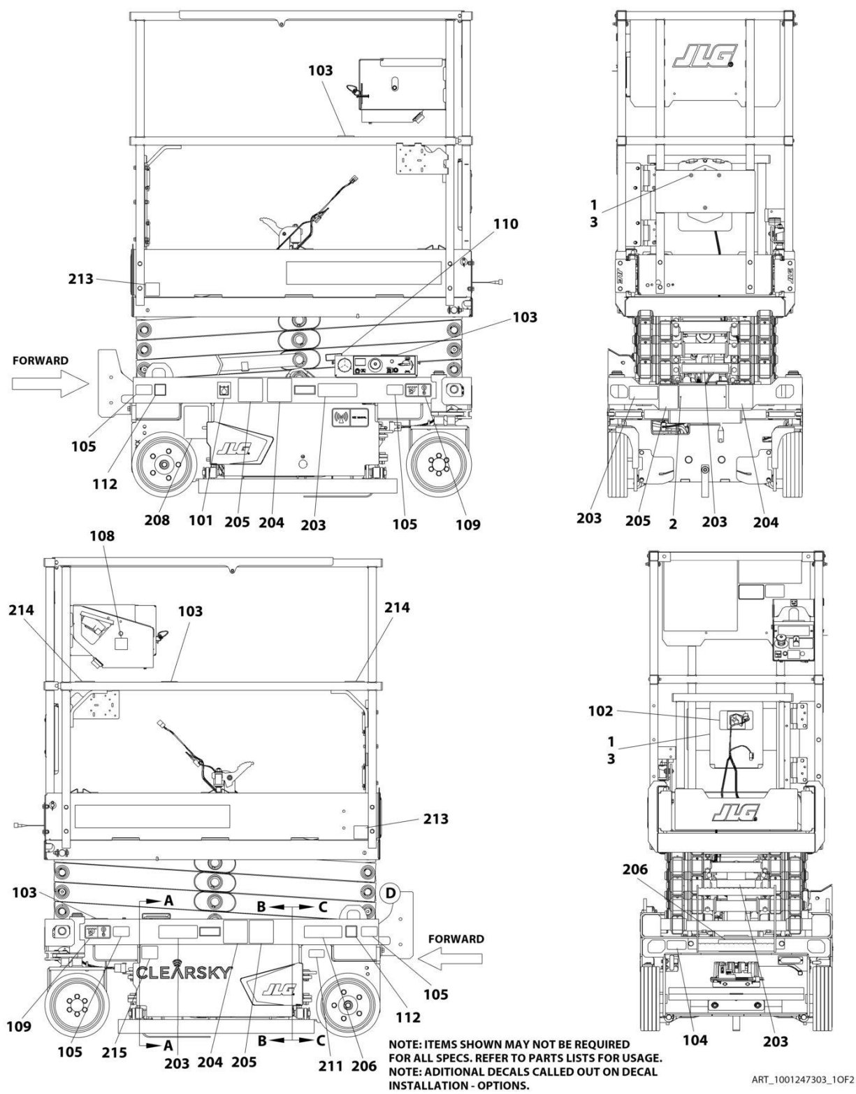
FIGURE 8-3. DECALS INSTALLATION (CHINA SPECS)
