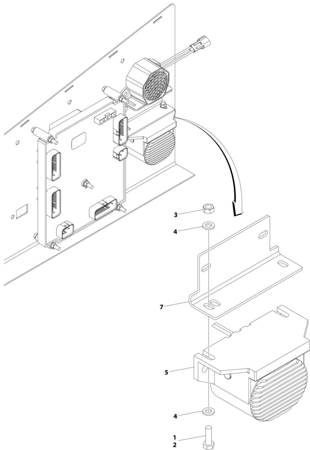
FIGURE 2-24. WHITE NOISE AMBIENT ALARM INSTALLATION
