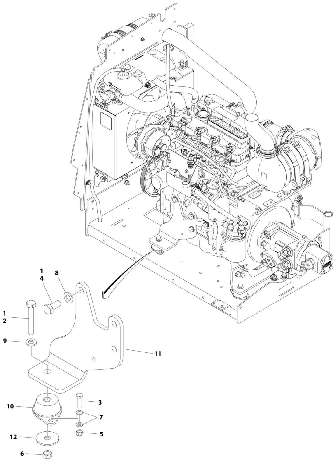
FIGURE 3-17. MOTOR MOUNT INSTALLATION (STAGE V ENGINES WITHOUT GENERATOR)
