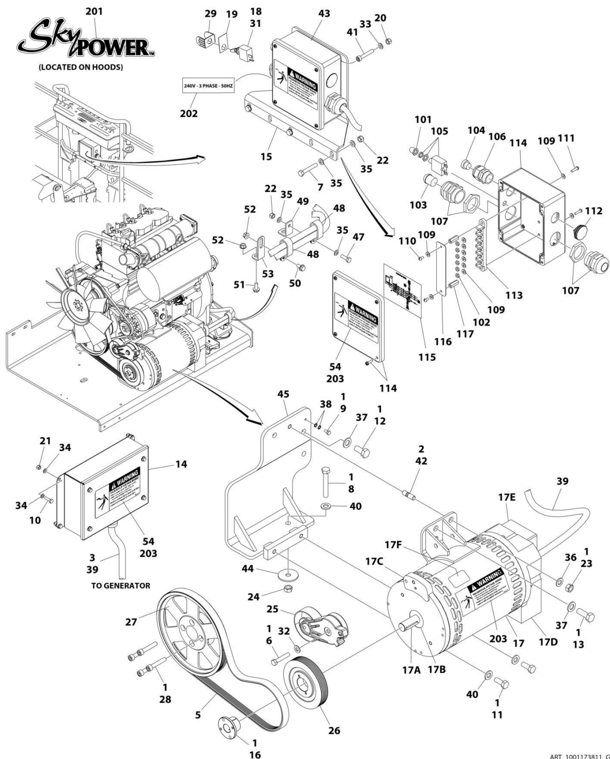
FIGURE 3-26. GENERATOR INSTALLATION - 7500W/50HZ (DEUTZ D2011 ENGINE)
