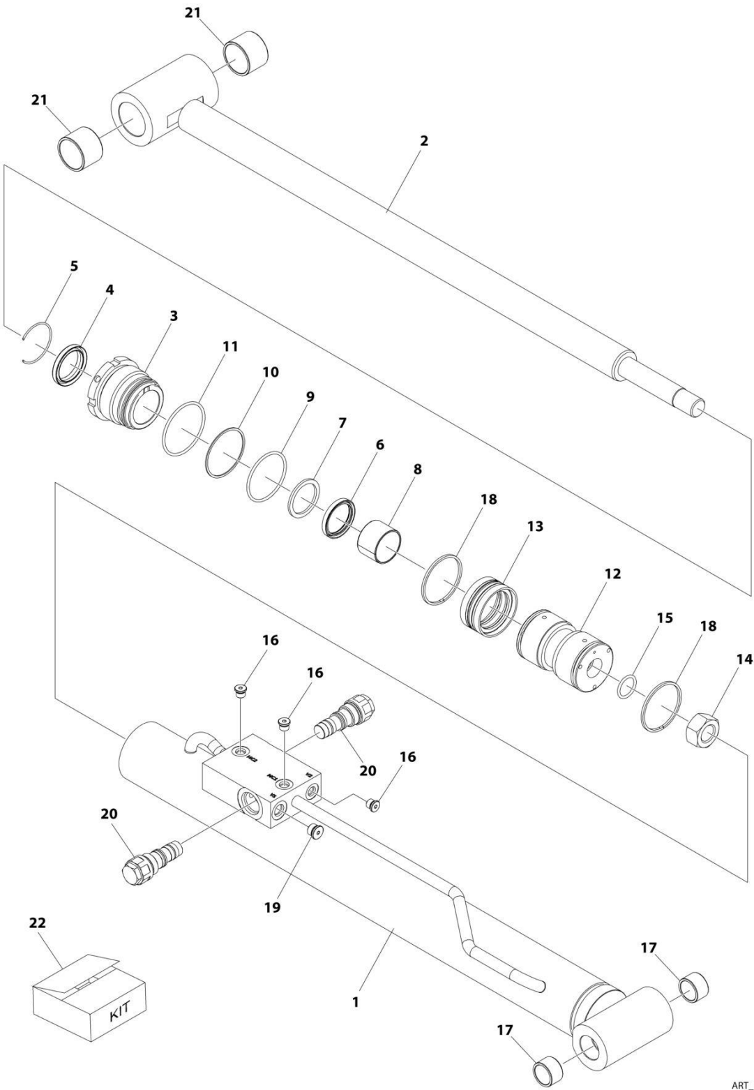
FIGURE 6-8. LIFT JIB CYLINDER ASSEMBLY
