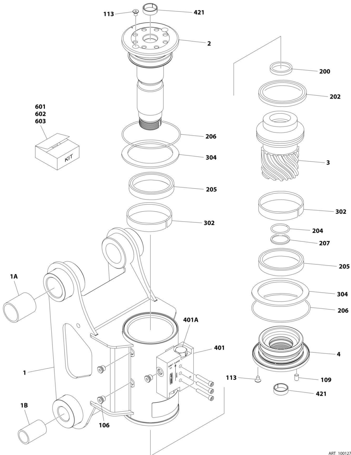
FIGURE 4-5. ROTATOR ASSEMBLY
