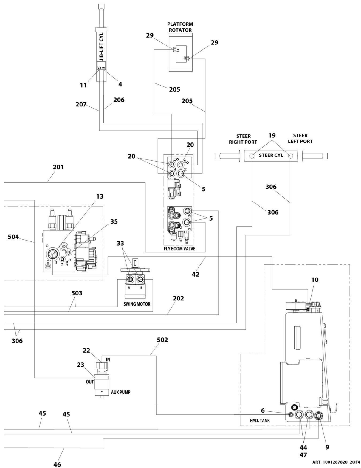
FIGURE 7-3. HYDRAULIC SYSTEM INSTALLATION - 450AJ 4WD
