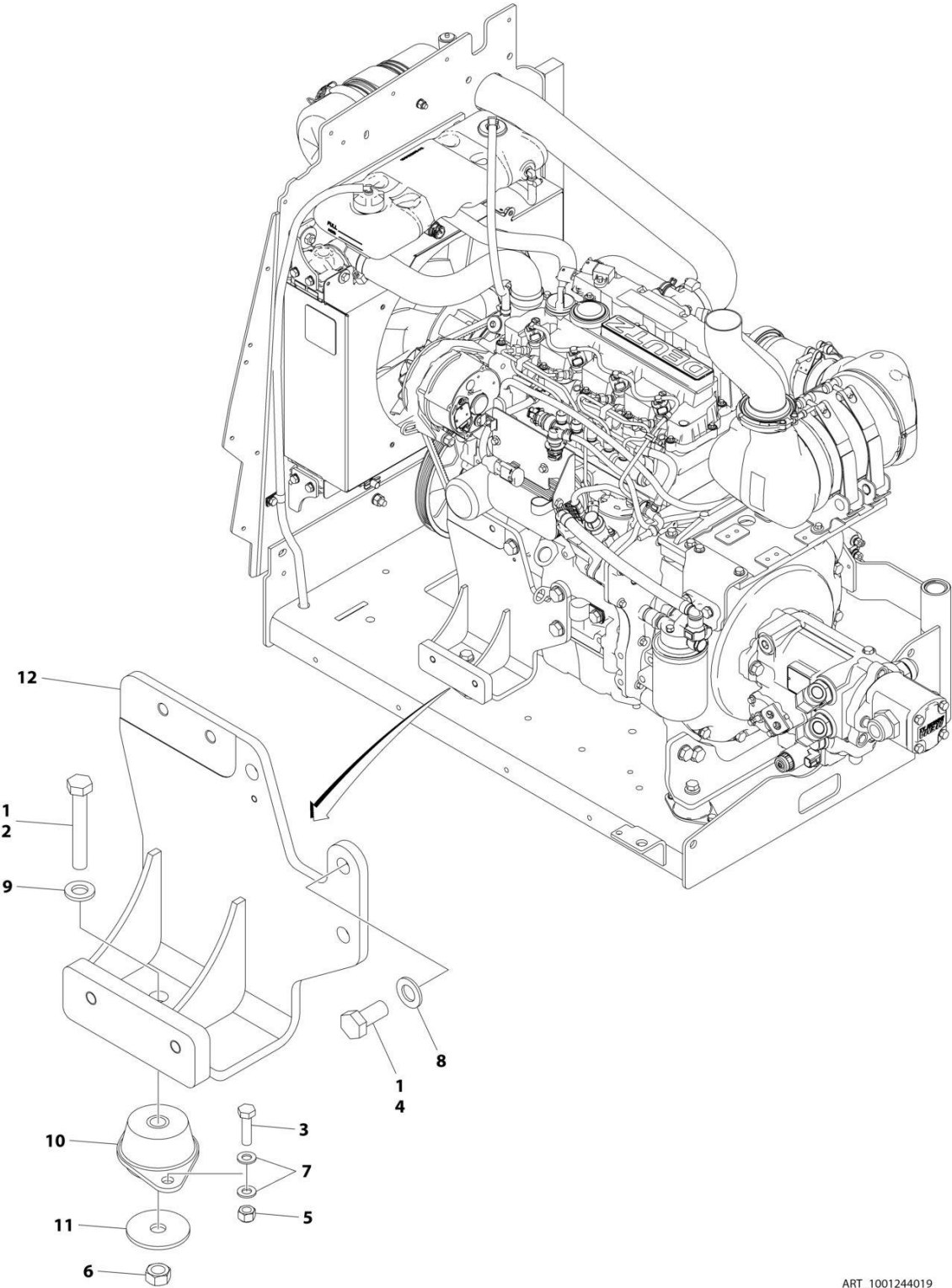
FIGURE 3-18. MOTOR MOUNT INSTALLATION (STAGE V ENGINES WITH GENERATOR)
