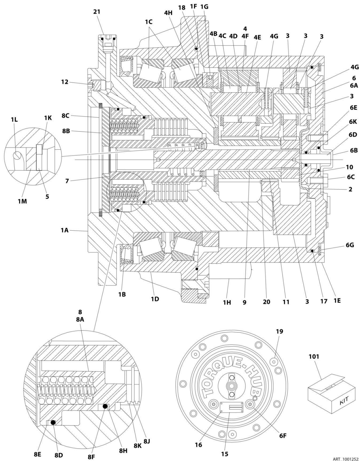
FIGURE 1-5. DRIVE HUB ASSEMBLY
