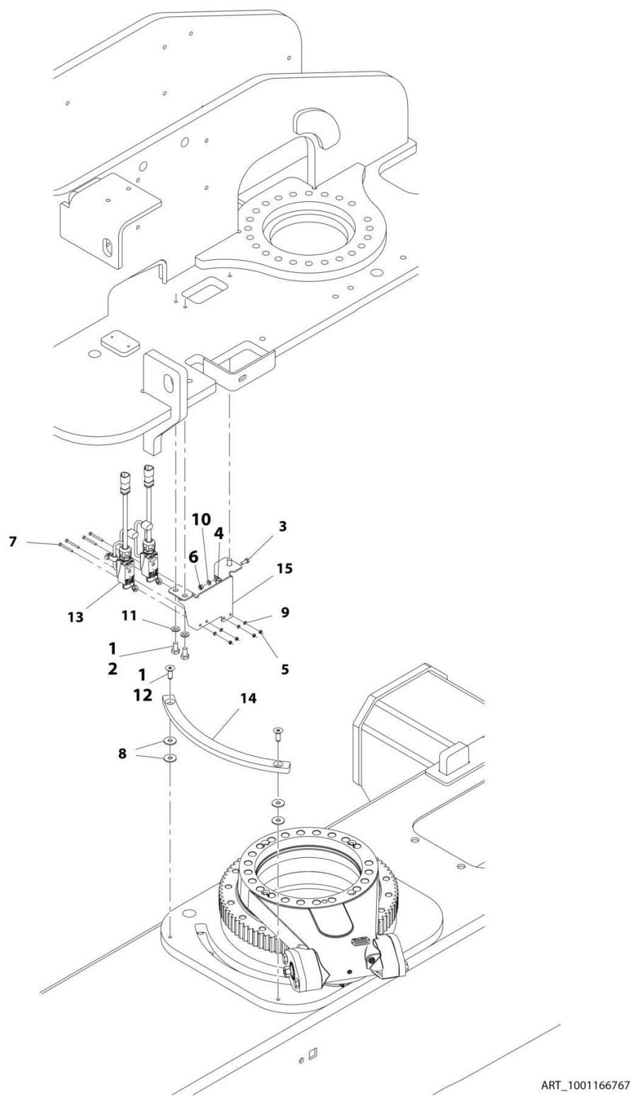
FIGURE 2-13. DRIVE ORIENTATION INSTALLATION
