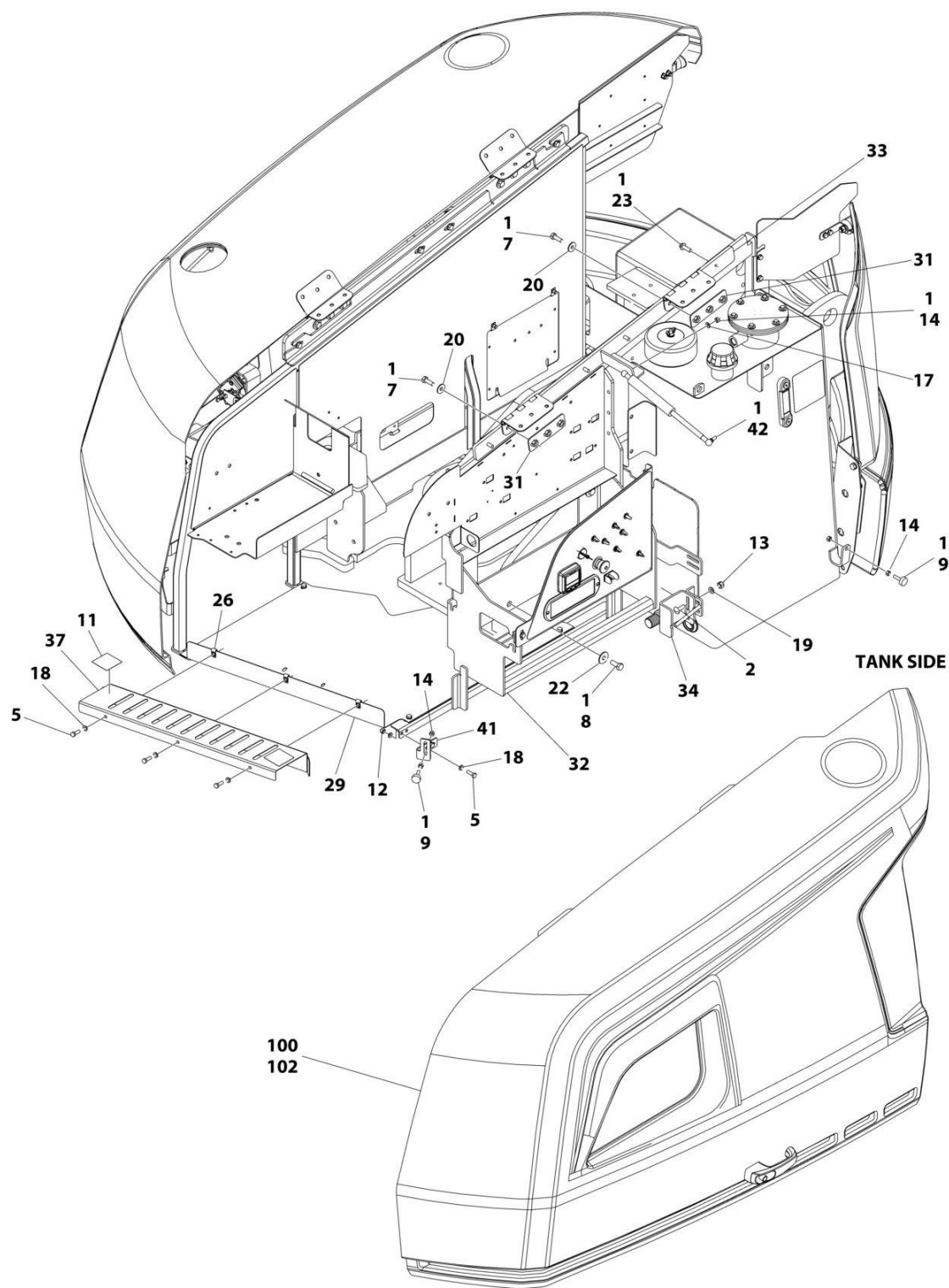
FIGURE 2-27. HOODS INSTALLATION
