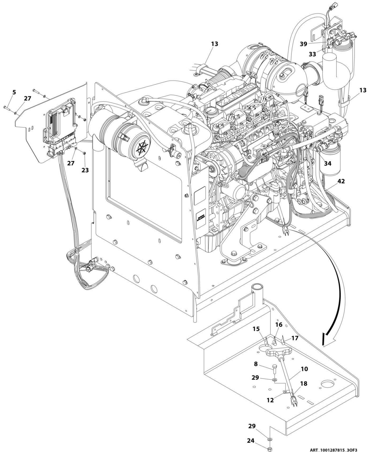
FIGURE 3-3. ENGINE INSTALLATION - DEUTZ D2.9L4 ENGINE (WITH ARCTIC PACKAGE) (ANSI EXPORT, AUSTRALIAN, CE (LRC), CIS/EAC & UK CA SPECS)
