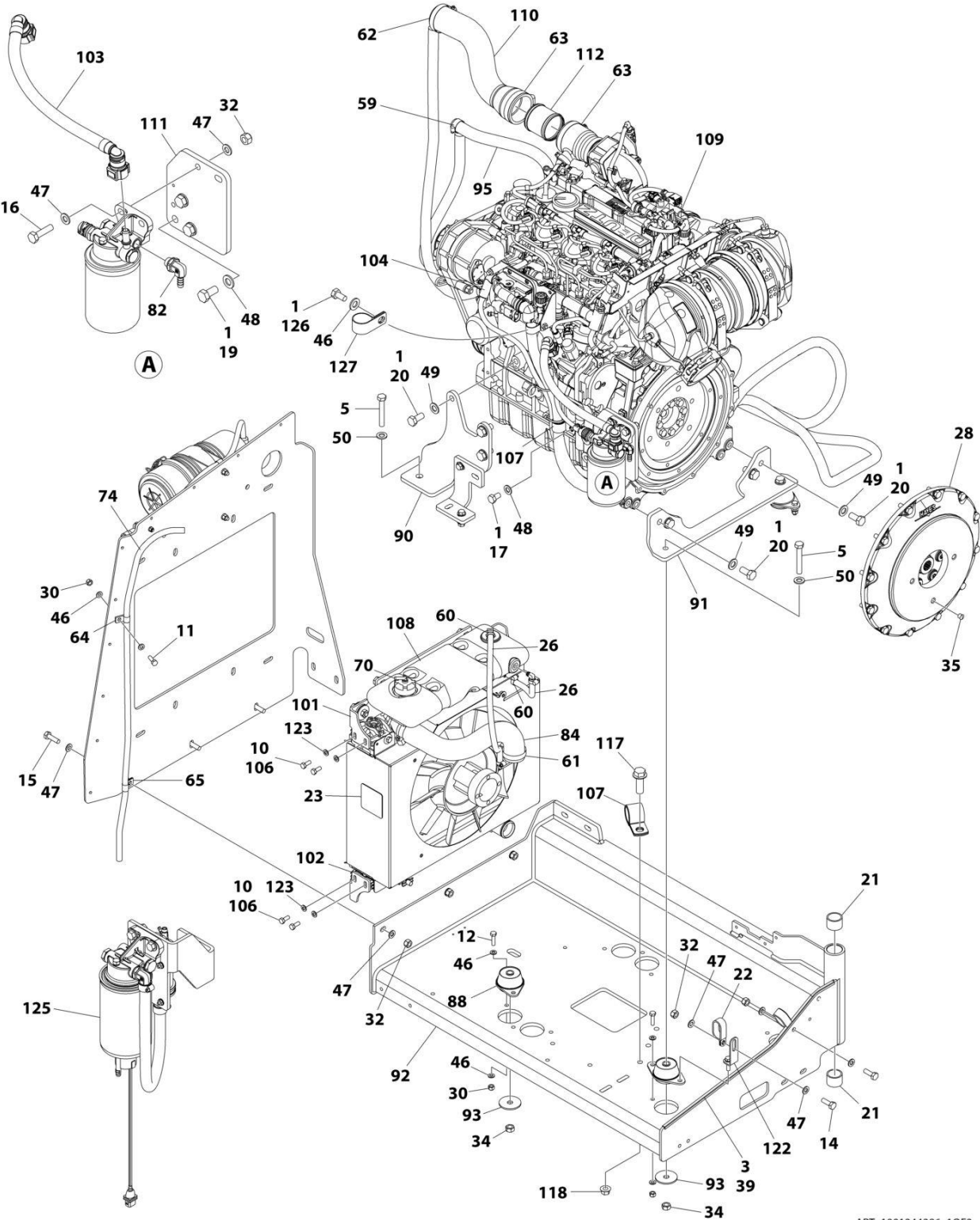
FIGURE 3-15. ENGINE ASSEMBLY – DEUTZ D2.9L4 ENGINE (STAGE V) (CE & UK CA SPECS)
