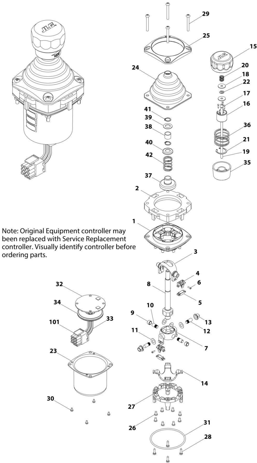
FIGURE 4-7. CONTROLLER ASSEMBLY - LIFT AND SWING (SN 0300188534 through 0300209000)
