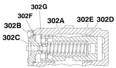
HYD. CONTROL FRONT & MID PUMPS (DETAIL OF ITEM 302)
