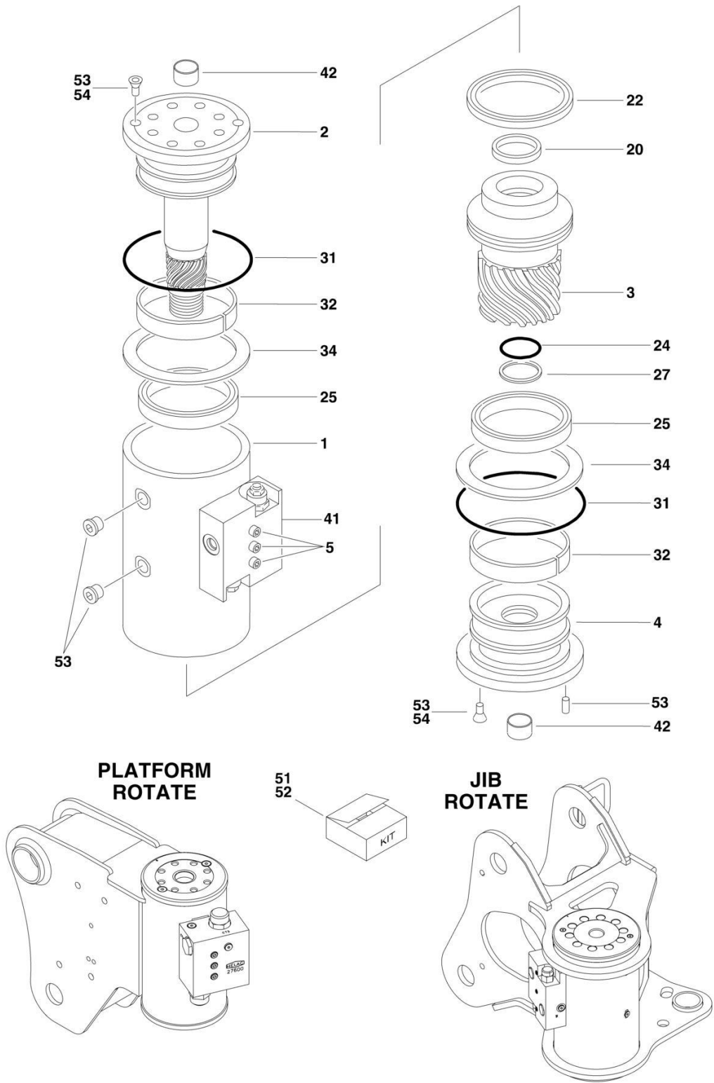
FIGURE 3-4. ACTUATOR ASSEMBLY
