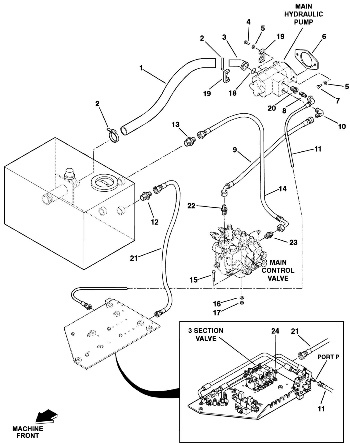
FIGURE 5-8. MAIN CONTROL VALVE CIRCUIT (W/CABLE CONTROLLED JOYSTICK) (SN 0E1180 to Present)
