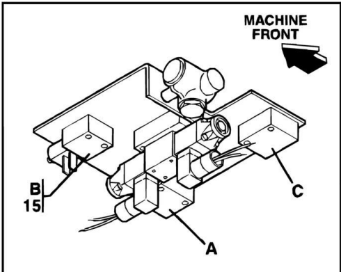
UNDERSIDE VIEW OF VALVE PLATE. REFER TO VALVE PLATE ASSEMBLY FOR BREAKDOWN.
