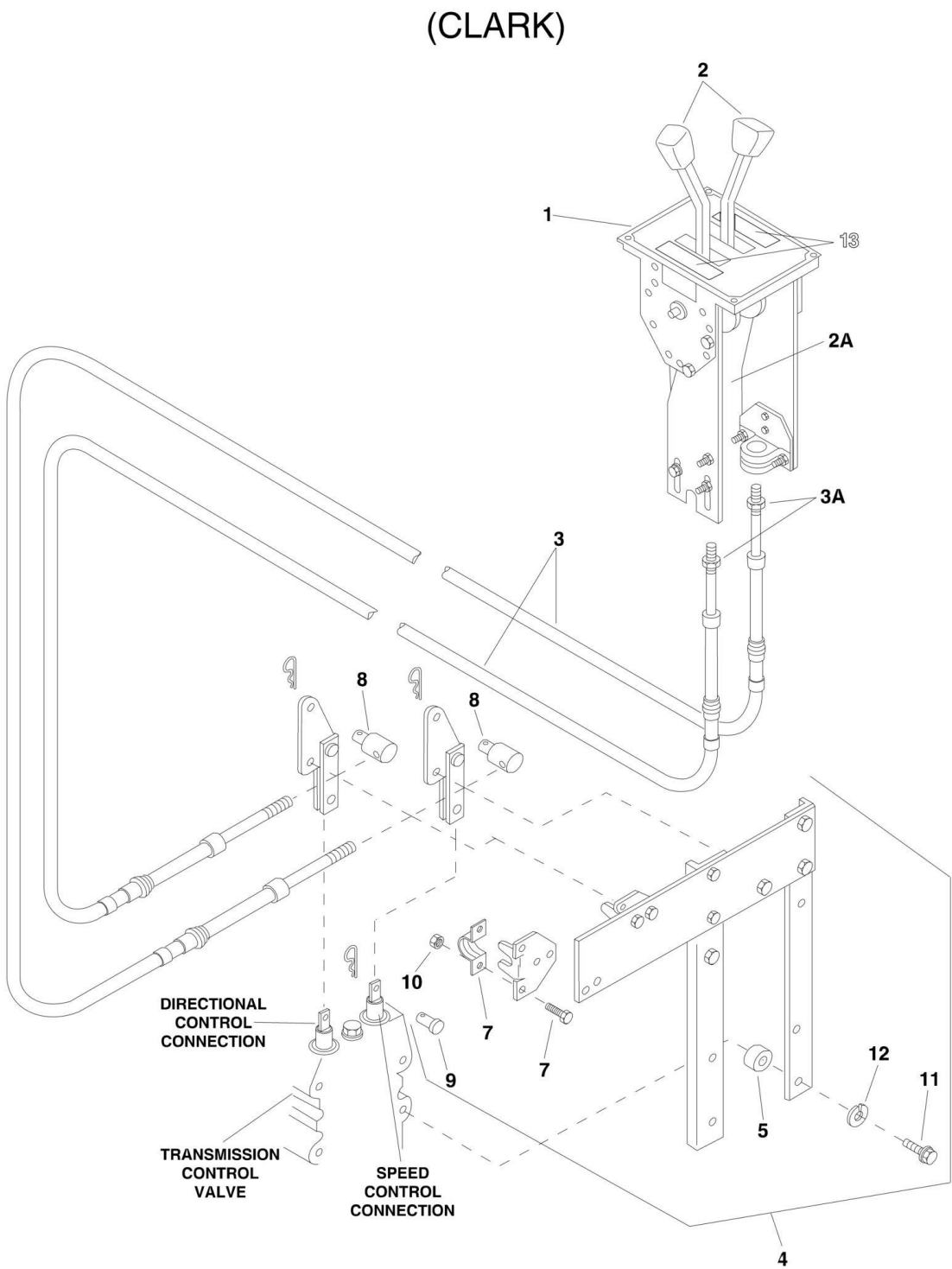
FIGURE 2-6. TRANSMISSION SHIFT CONTROLS (CLARK)
