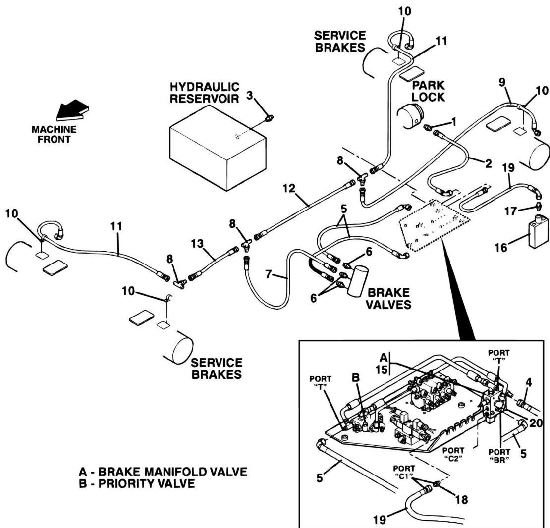
UNDERSIDE VIEW OF VALVE PLATE. REFER TO VALVE PLATE ASSEMBLY PAGE FOR BREAKDOWN.
