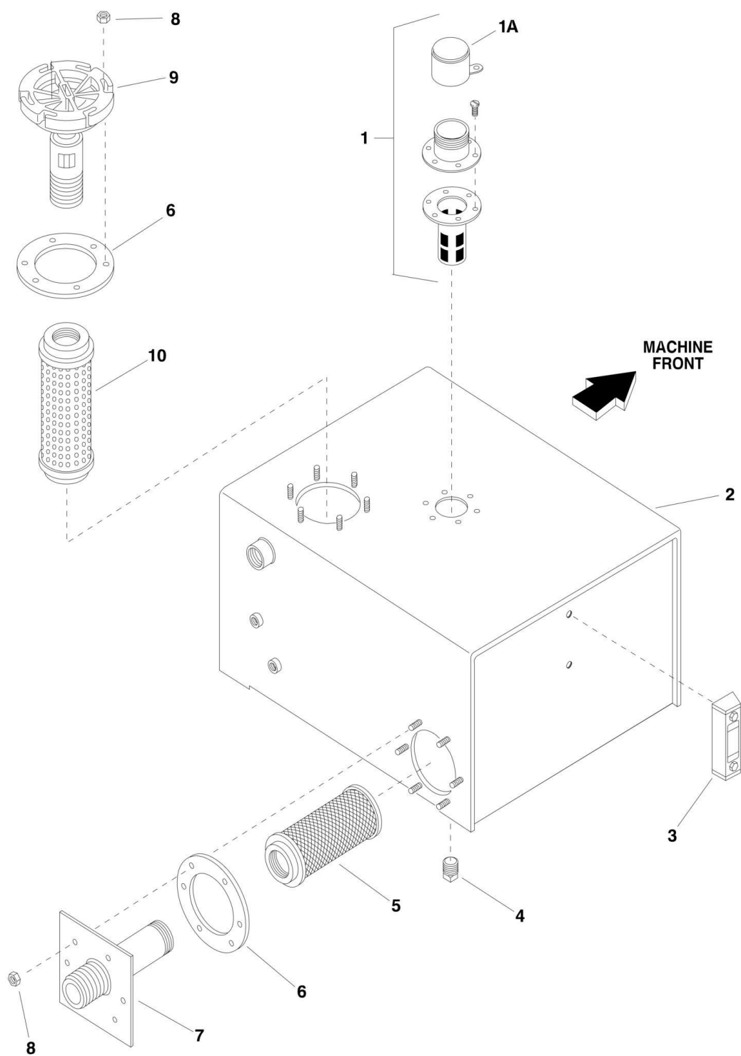
FIGURE 6-3. HYDRAULIC RESERVOIR (SN 1317 to Present)
