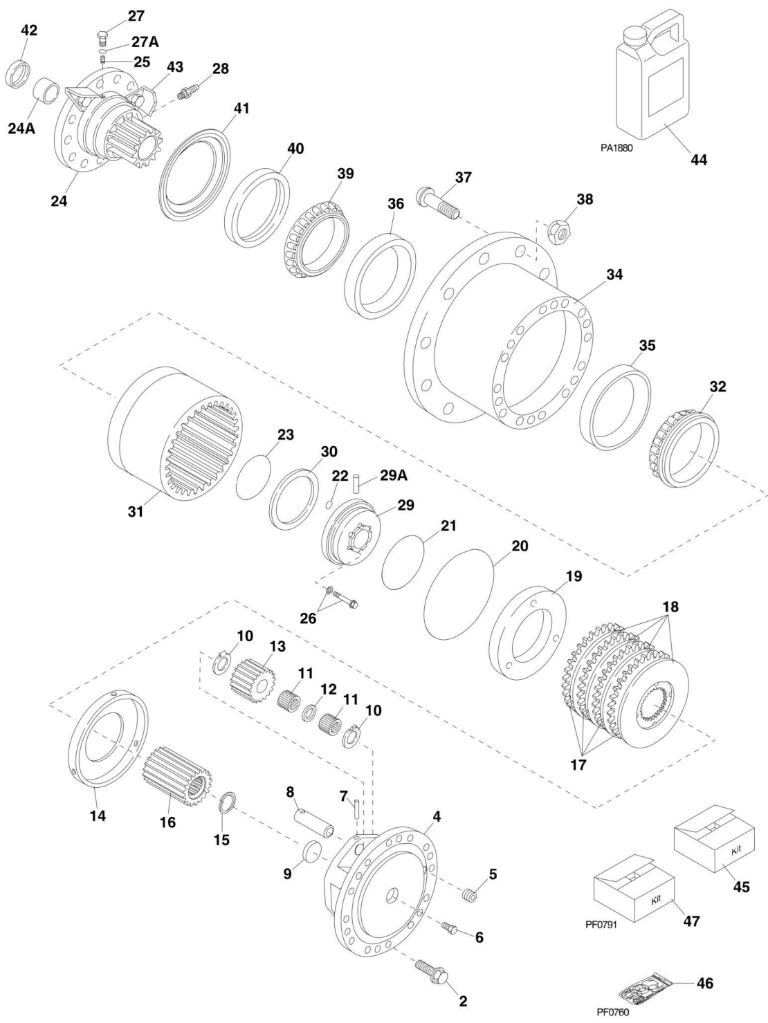
FIGURE 3-20. WHEEL END - WITH SERVICE BRAKES (FRONT AXLE ONLY) (SN 2344 to Present)
