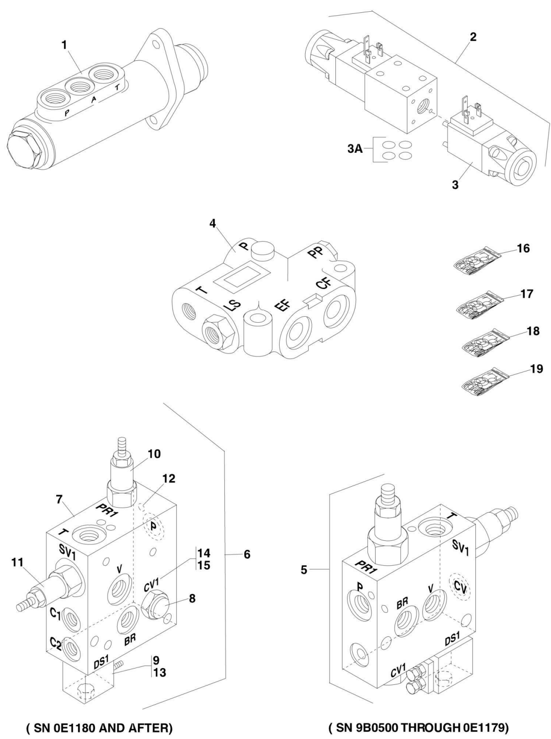
FIGURE 6-20. DIRECTIONAL CONTROL VALVES (SN 9B0500 to Present)
