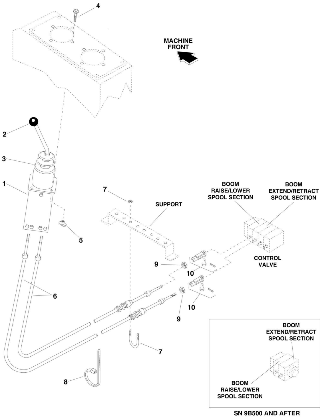
FIGURE 2-7. BOOM RAISE/LOWER AND BOOM EXTEND/RETRACT CONTROL (CABLE CONTROL JOYSTICK)
