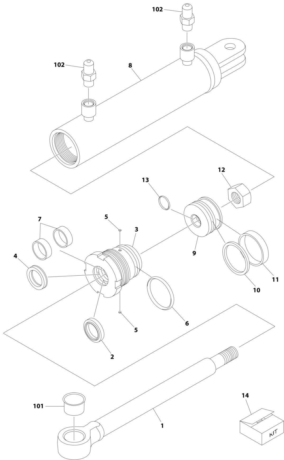
FIGURE 5-3. STEER CYLINDER ASSEMBLY (6RS/1932RS)
