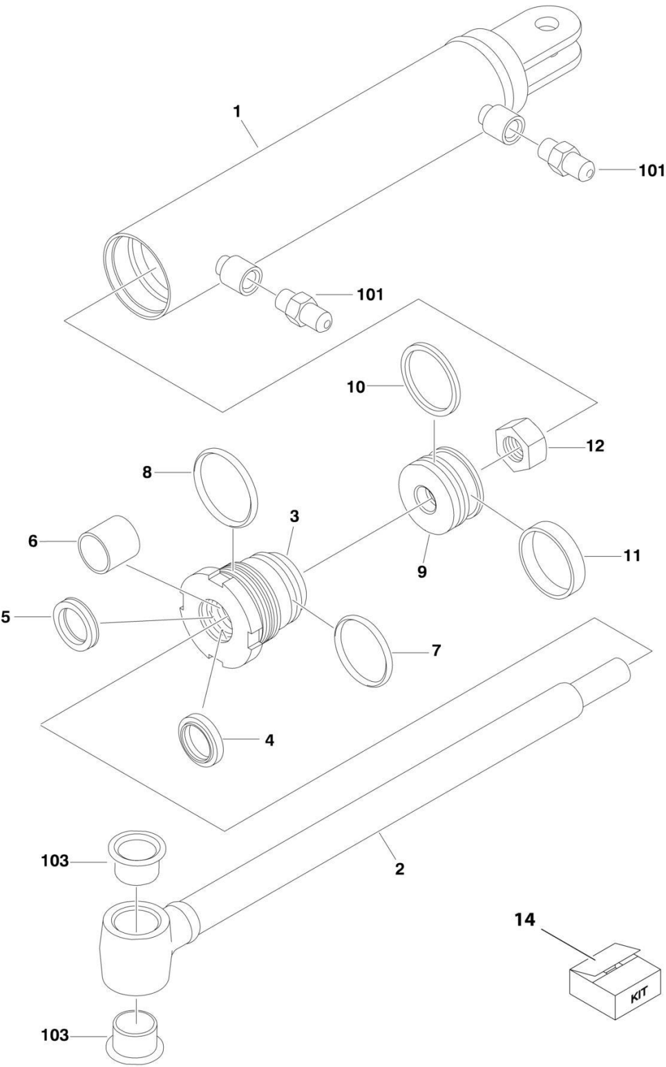
FIGURE 5-4. STEER CYLINDER ASSEMBLY (10RS/3248RS)
