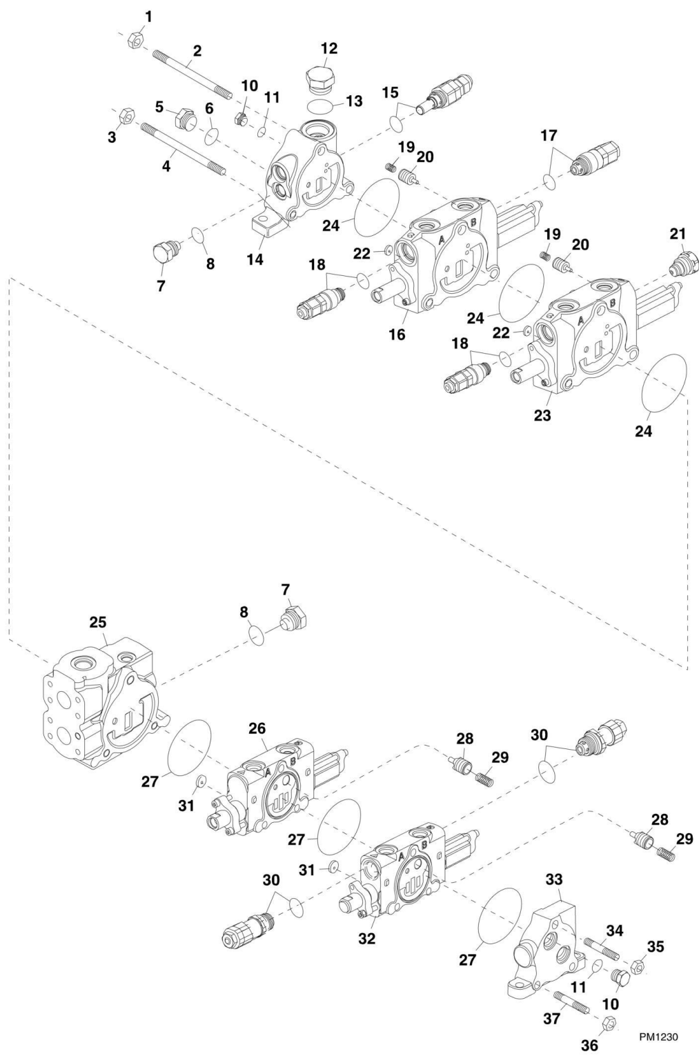
FIGURE 9-8. MAIN CONTROL VALVE
