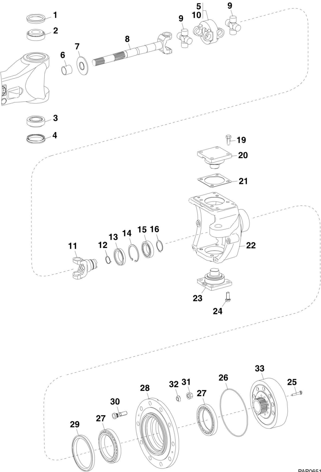
FIGURE 5-15. REAR AXLE - JOINT HOUSING
