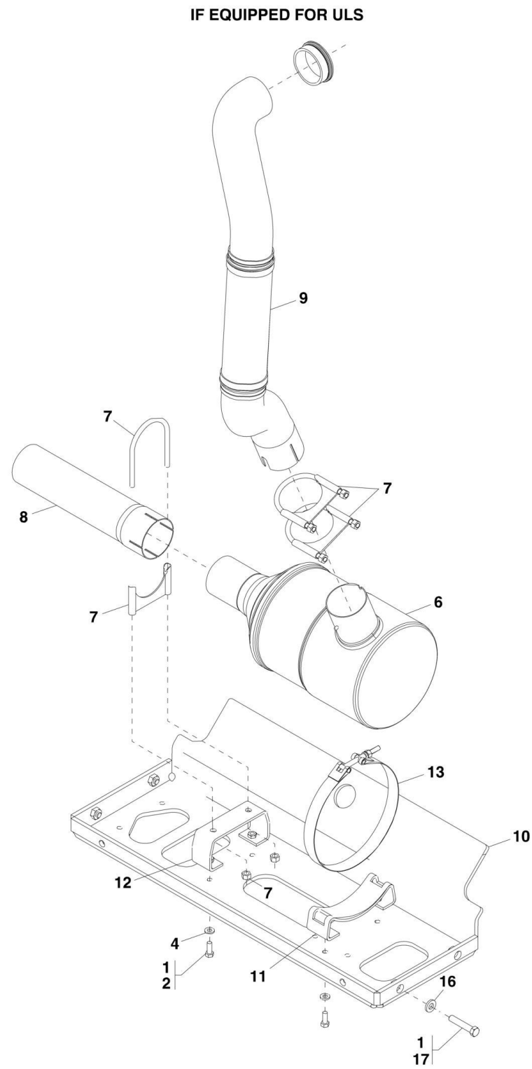
FIGURE 4-12. EXHAUST SYSTEM
