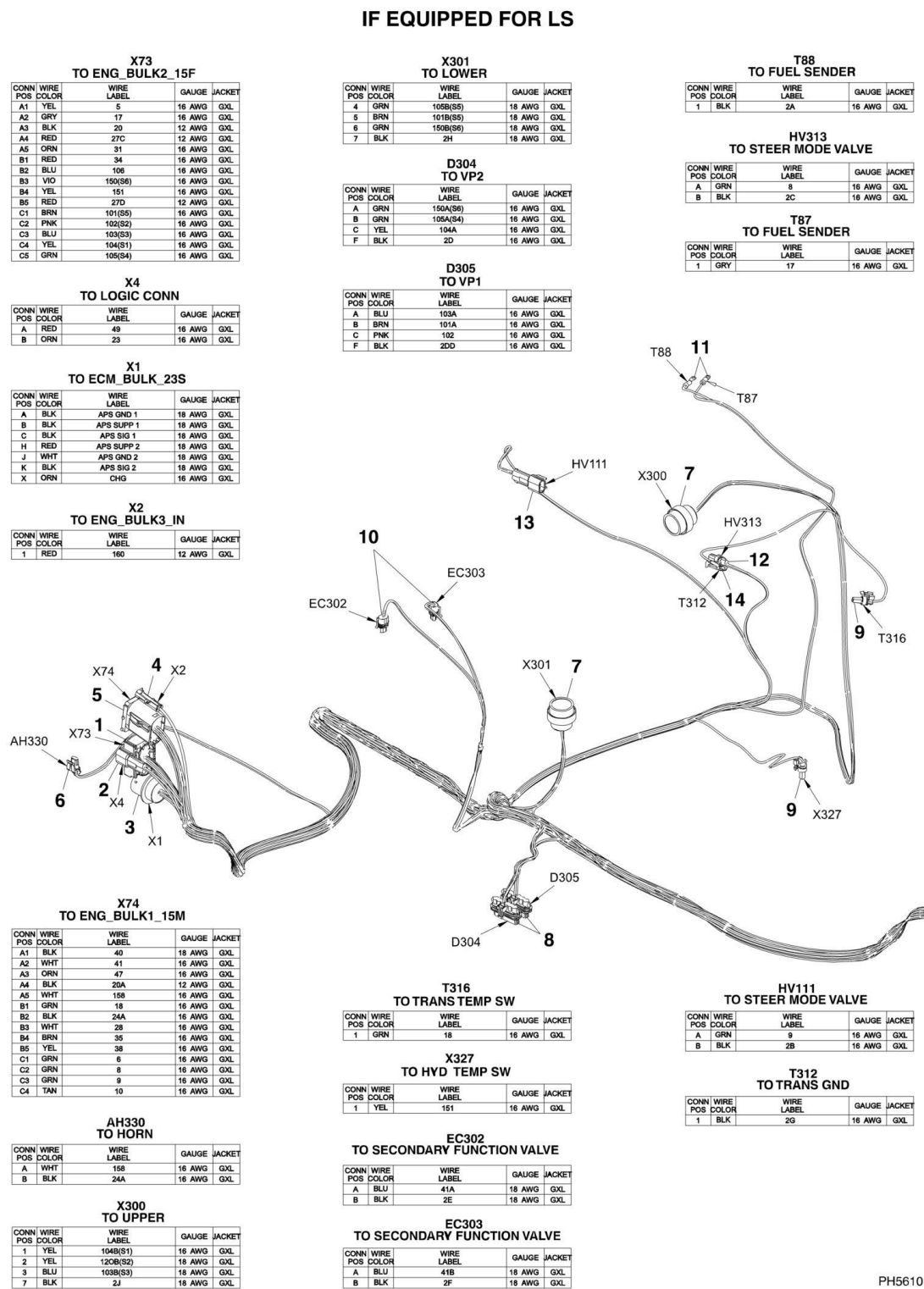
FIGURE 10-10. ENGINE HARNESS
