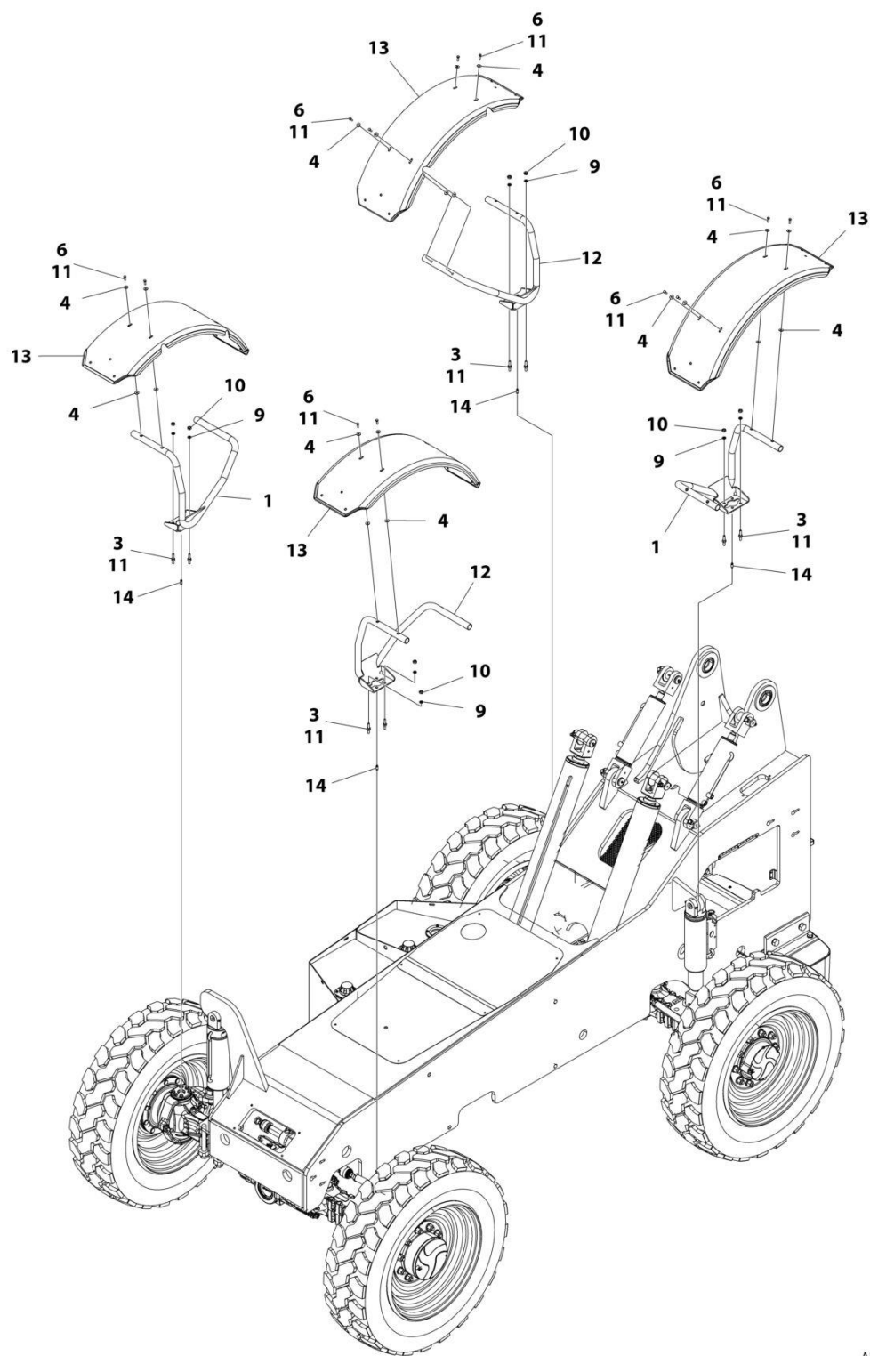
FIGURE 5-49. FENDER INSTALLATION (DANA)
