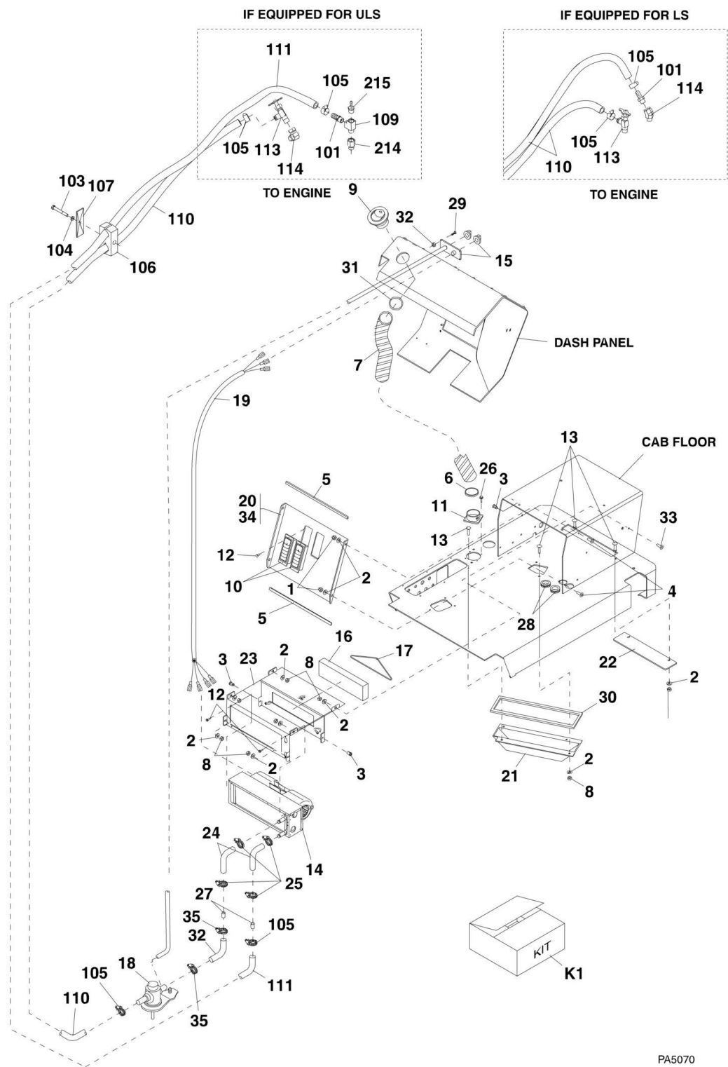
FIGURE 6-8. CAB HEATER
