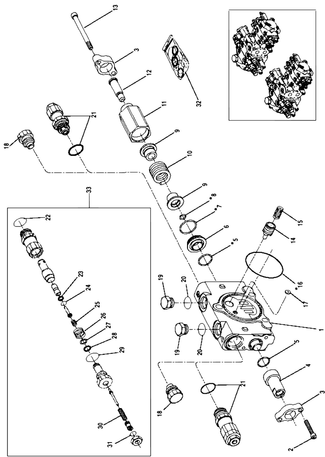
FIGURE 6-13. SECTION ASSEMBLY AUXILIARY
