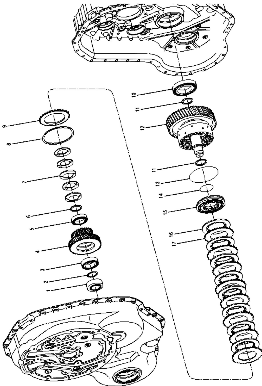
FIGURE 1-22. COUPLING GROUP 3
