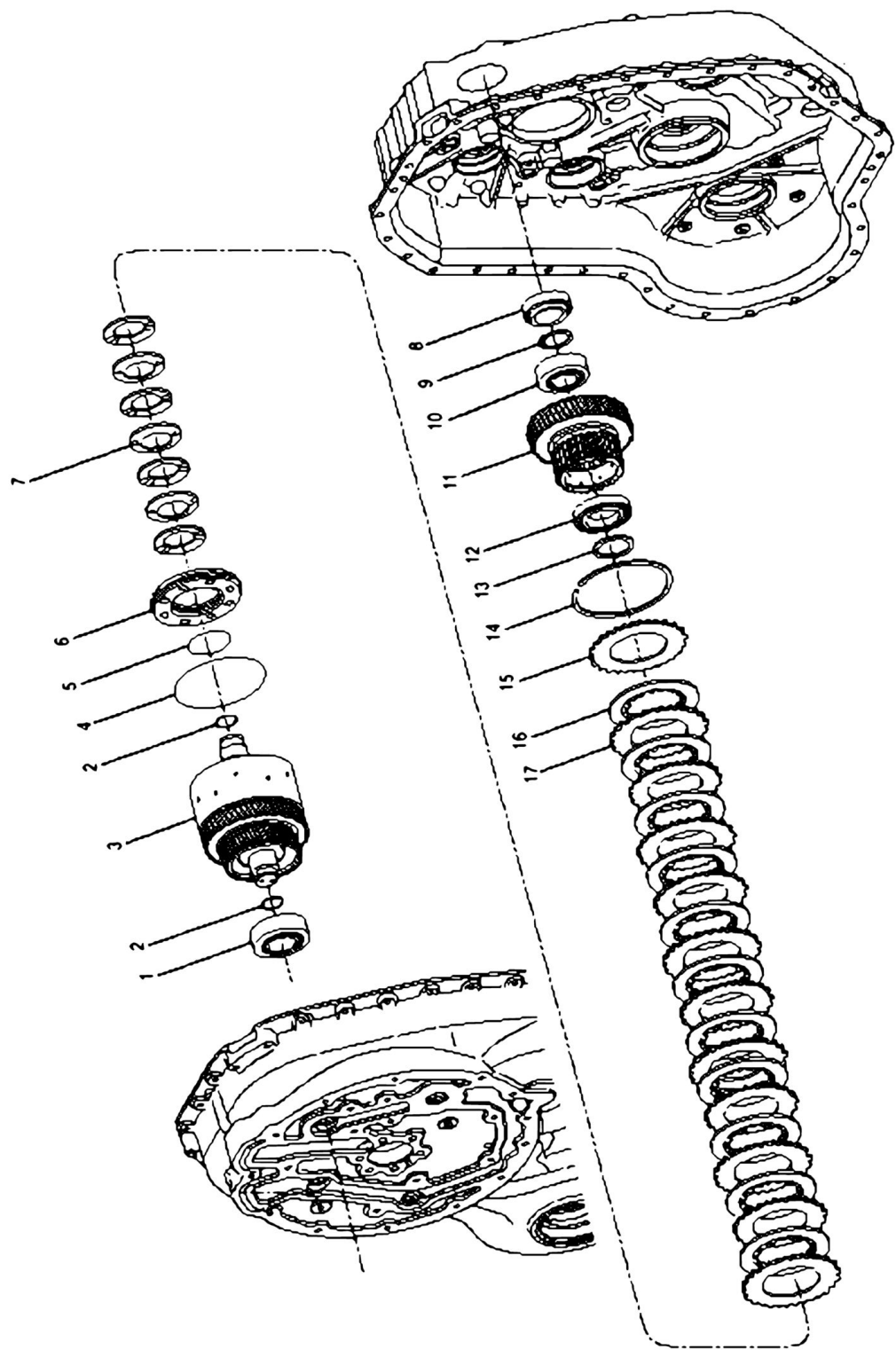
FIGURE 1-25. REVERSING GEAR GROUP 2
