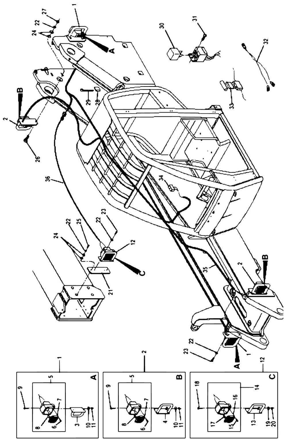
FIGURE 10-6. WORKLIGHTS ASSEMBLY
