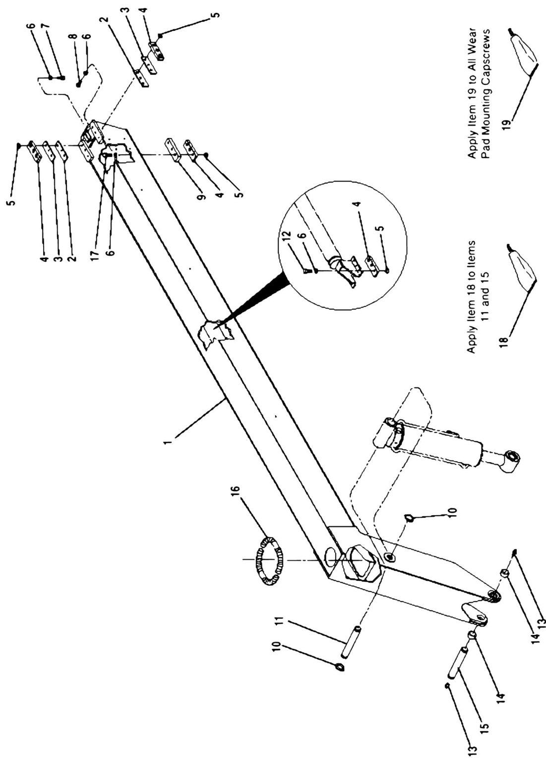
FIGURE 4-4. INNER BOOM ASSEMBLY (HIGH PIVOT)
