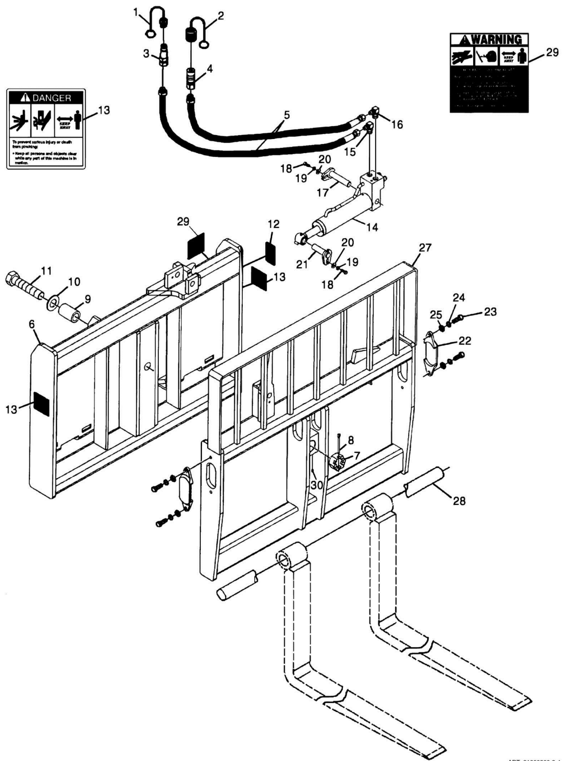
FIGURE 3-4. UNIVERSAL SIDE TILT CARRIAGE - G5-18A
