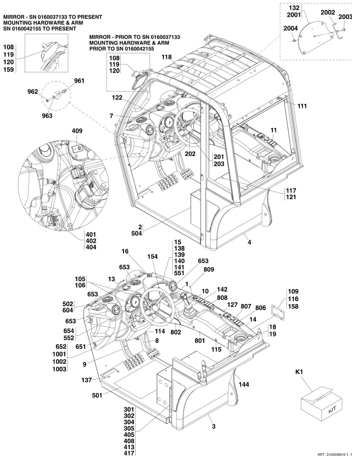
FIGURE 6-1. CAB INSTALLATION
