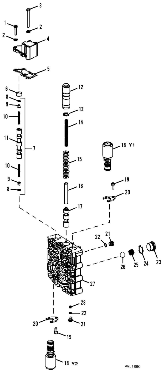
FIGURE 5-49. TRANSMISSION - GEARSHIFT SYSTEM
