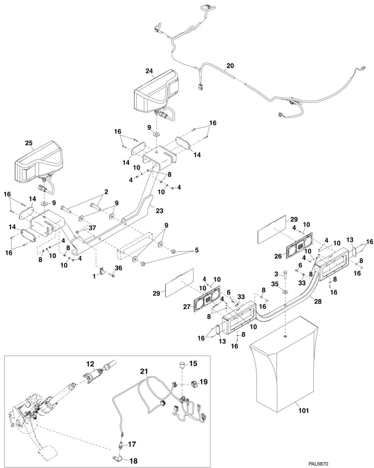
FIGURE 10-11. DRIVE LIGHTS
