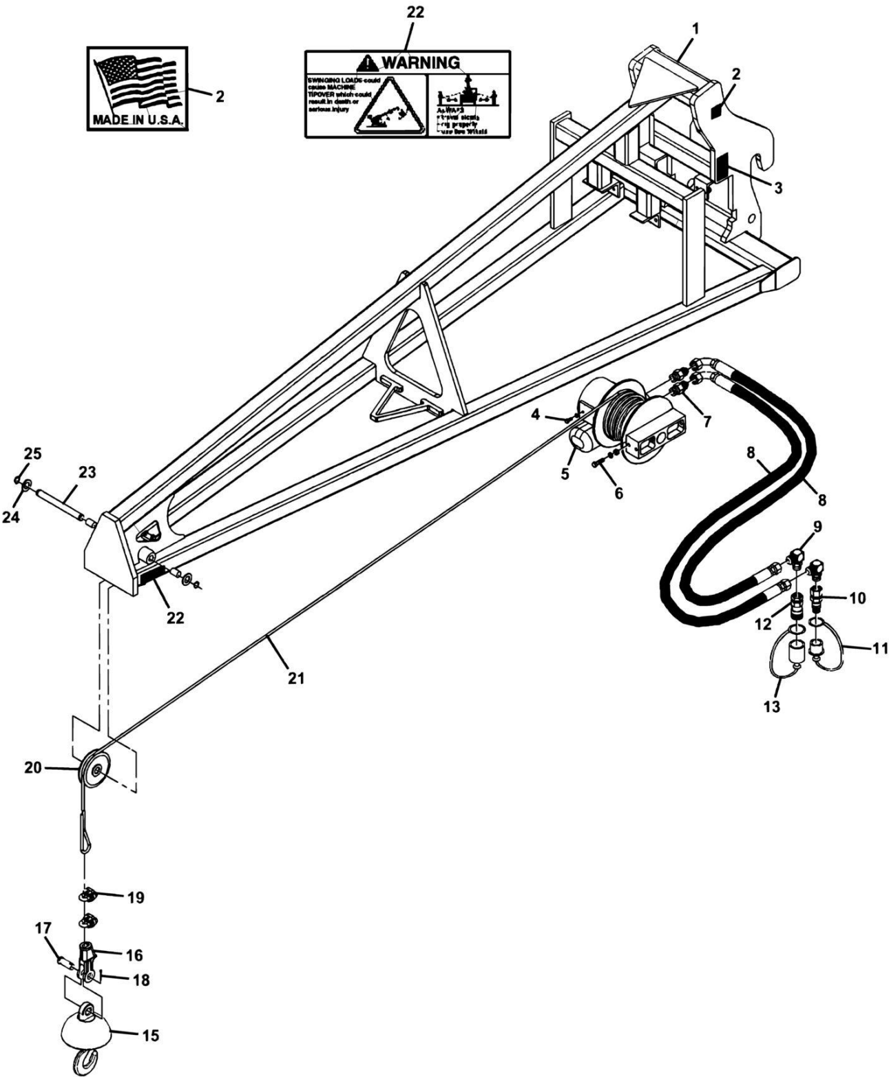
FIGURE 3-9. TRUSS BOOM WITH WINCH (SN 0160037689 to Present)
