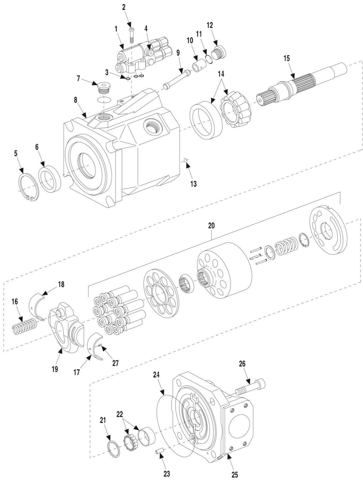
FIGURE 9-46. HYDRAULIC PUMP
