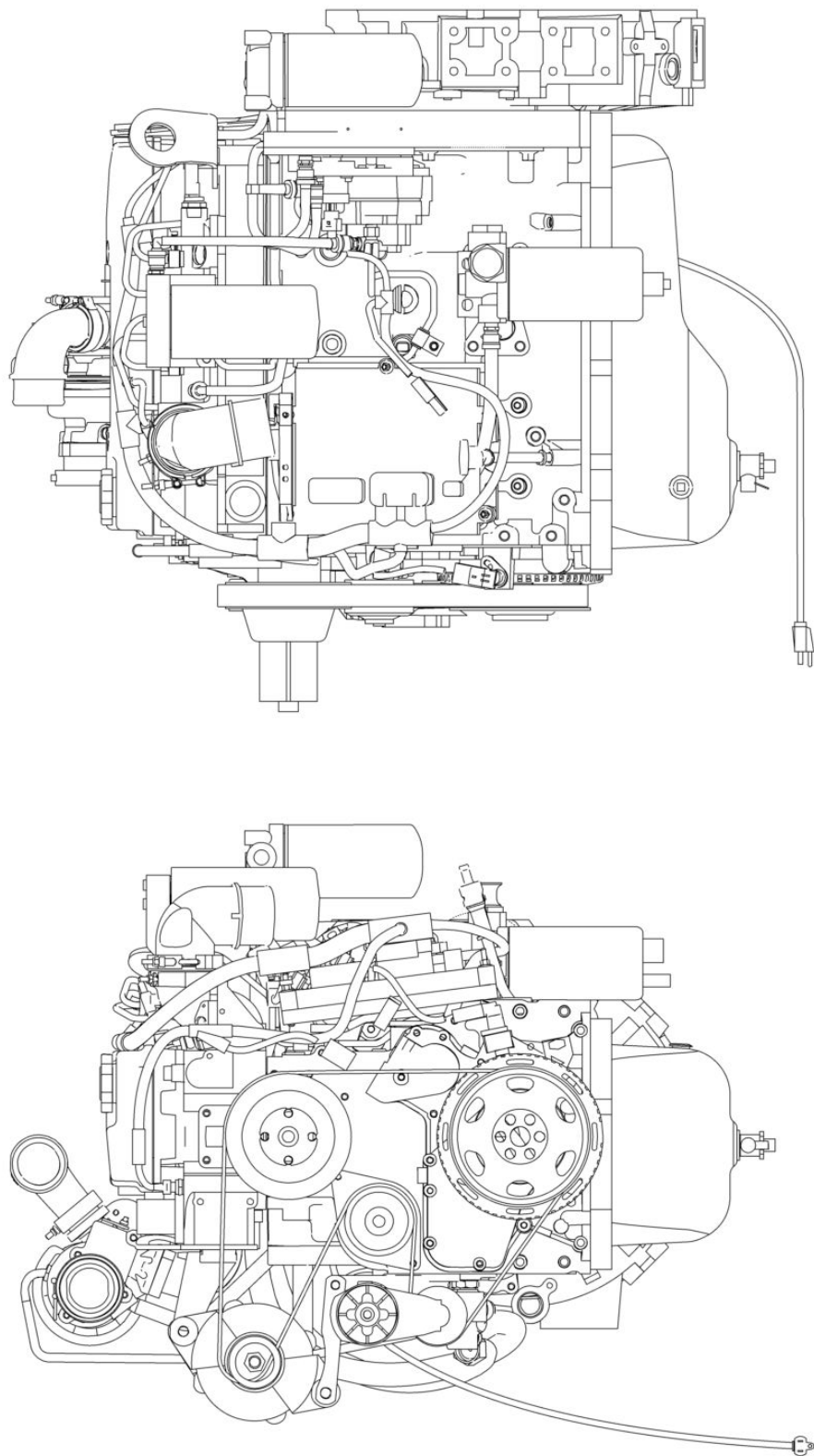
FIGURE 4-6. CUMMINS ENGINE
