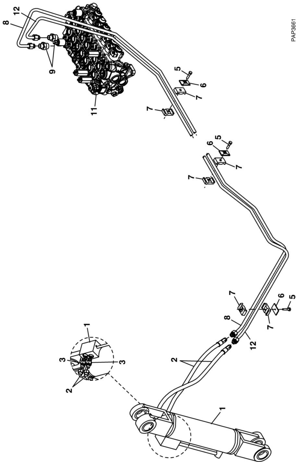
FIGURE 8-35. SWAY CYLINDER - CUMMINS ENGINE
