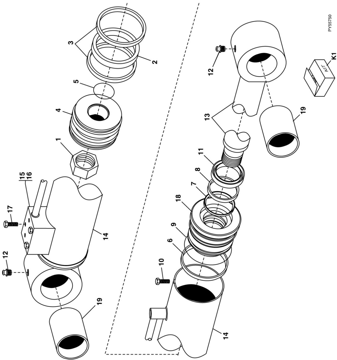
FIGURE 12-14. SWAY CYLINDER
