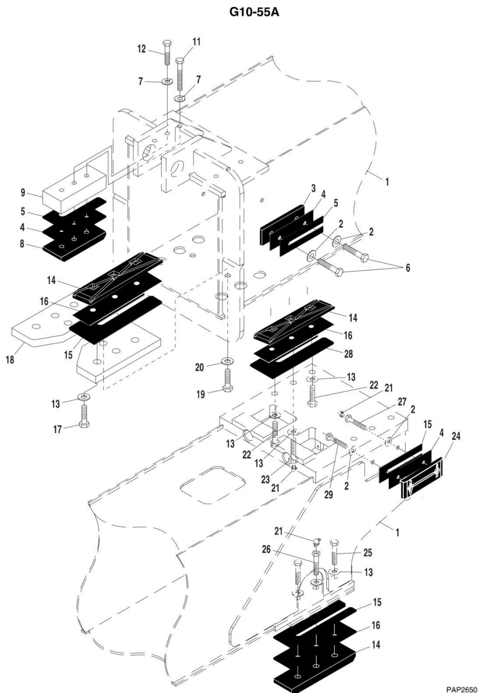
FIGURE 2-11. BEARINGS, PADS, SPACERS AND SHIMS, (THIRD BOOM SECTION) (G10-55A)
