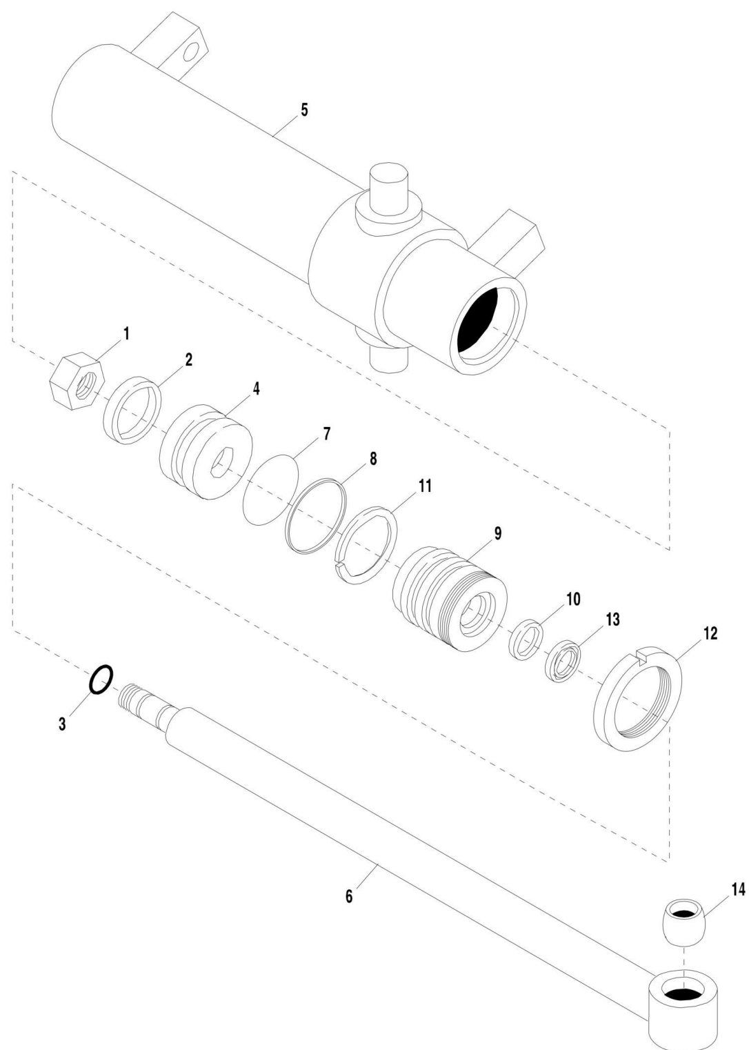
FIGURE 9-31. TRANSFORMER PLATFORM ROTATE CYLINDER (SN 0192001 through 0192007, SN 0160000052 through 0160000242, Including 0160000267 and 0160000322)
