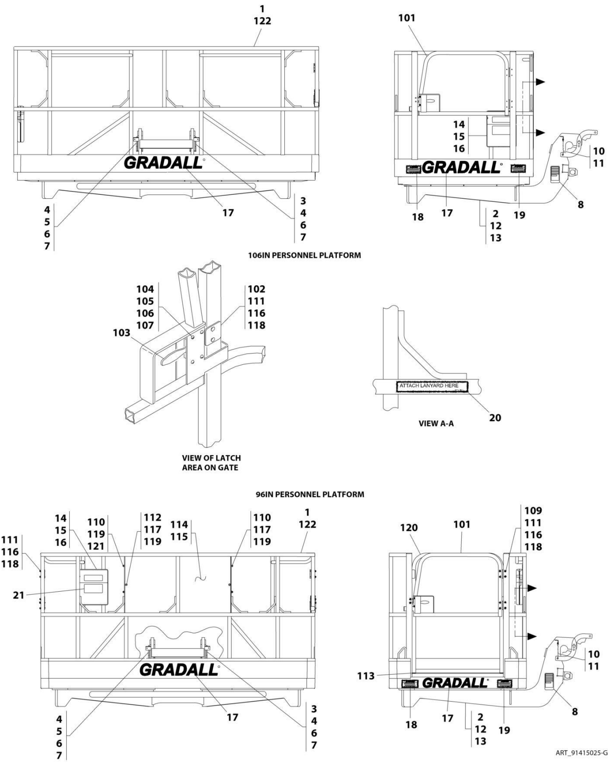
FIGURE 3-11. PERSONNEL PLATFORM ASSEMBLY
