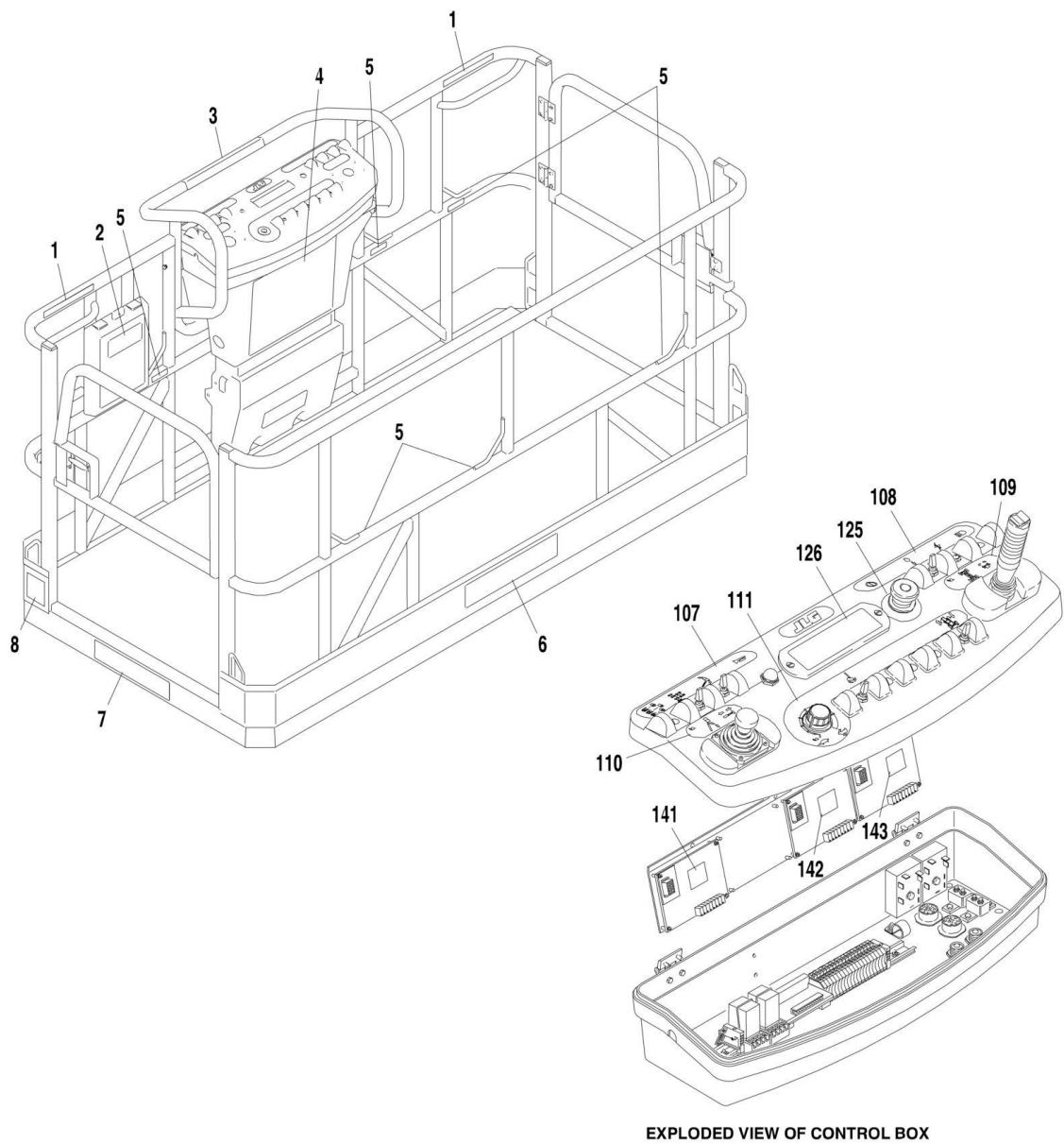
EXPLODED VIEW OF CONTROL BOX
