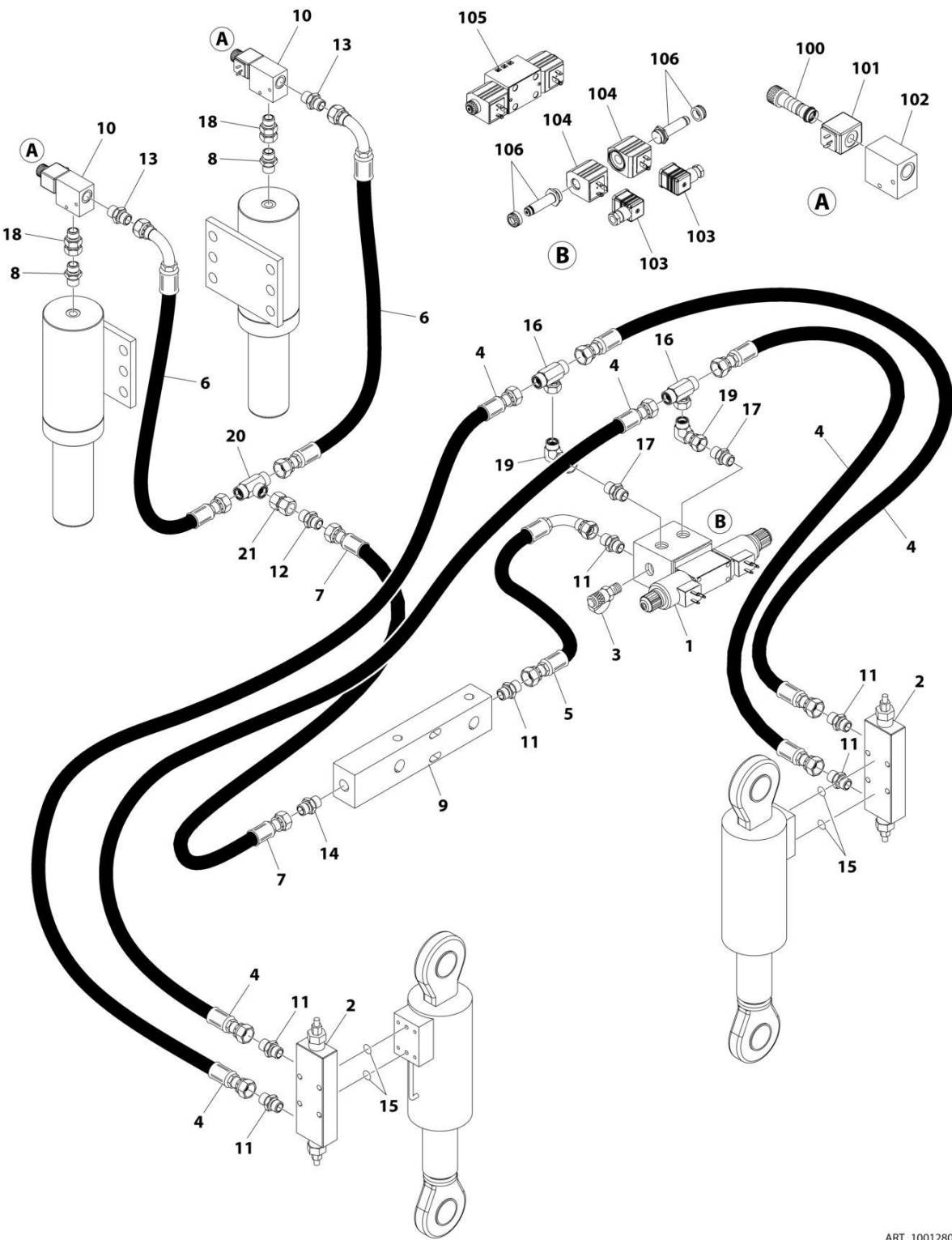
FIGURE 8-10. LEVELING CYLINDERS HYDRAULIC DIAGRAM
