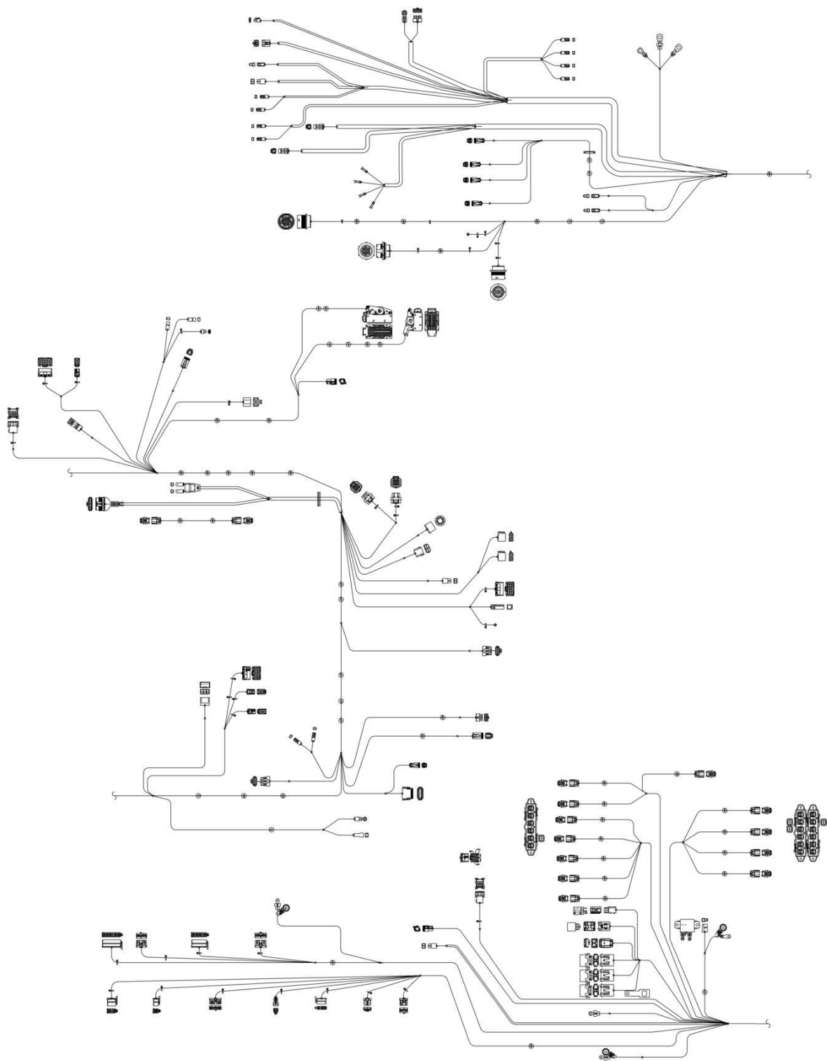
FIGURE 10-30. SEAT HARNESS
