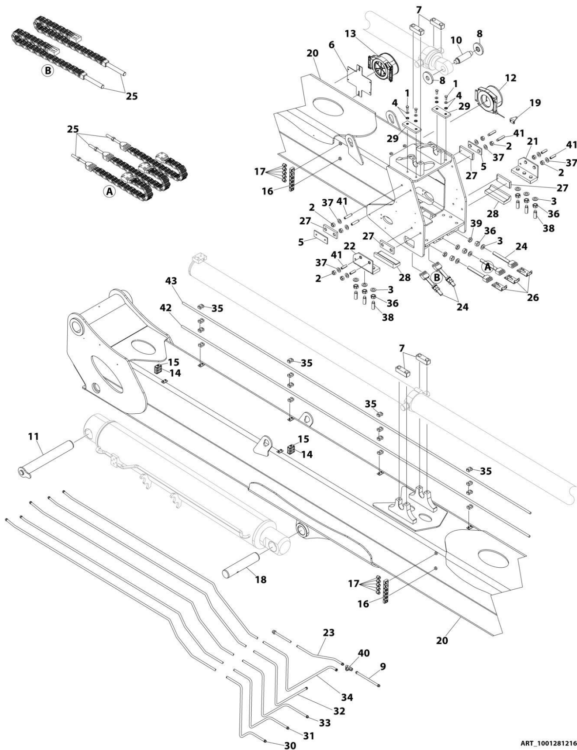
FIGURE 2-1. BASE BOOM ASSEMBLY
