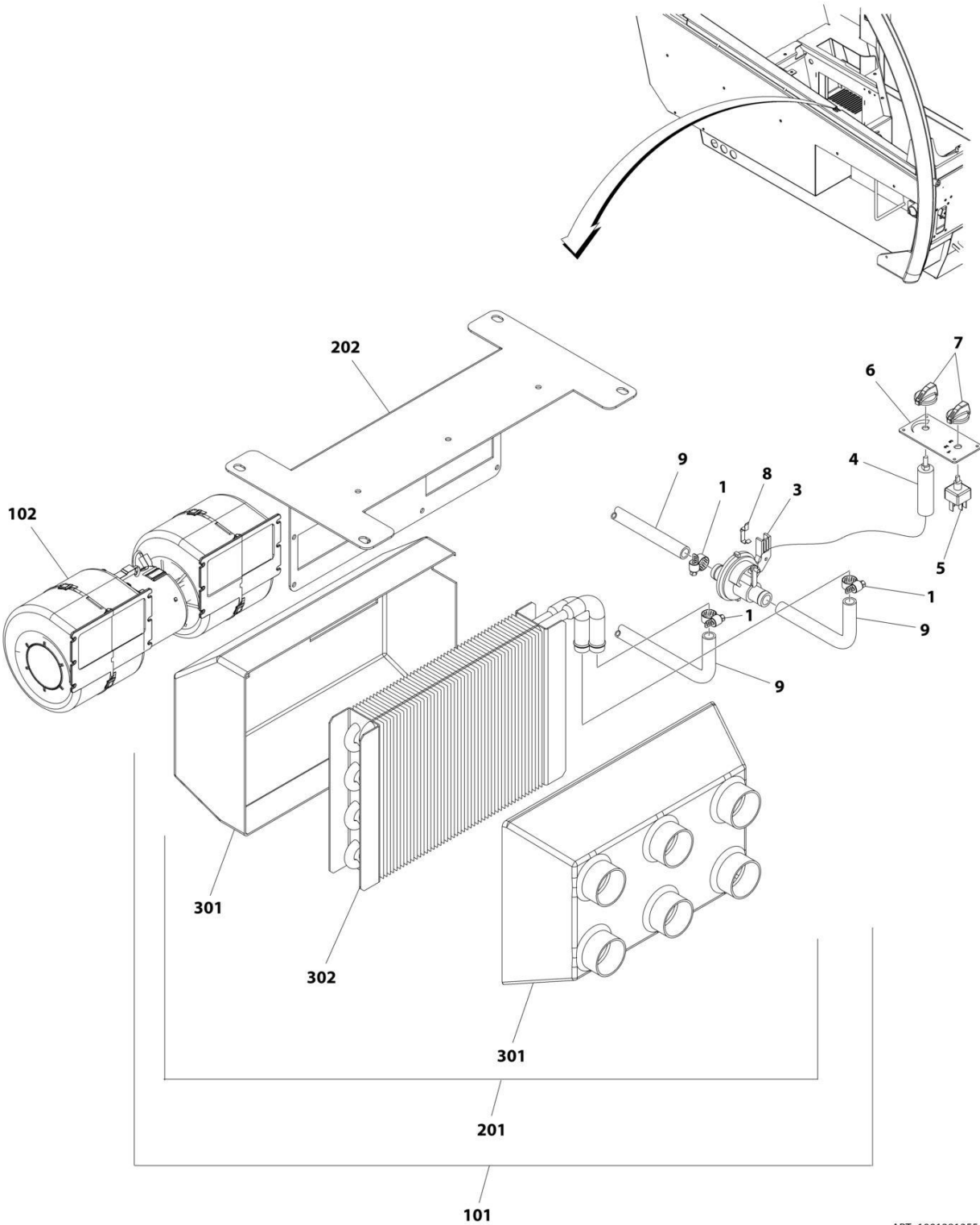
FIGURE 6-15. HEATER INSTALLATION
