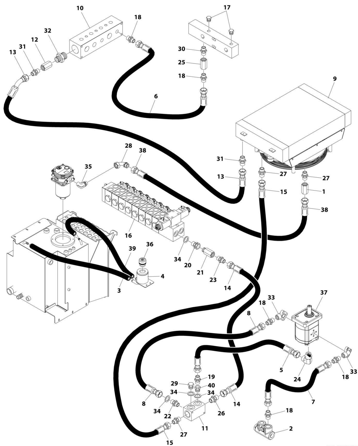
FIGURE 8-12. OIL COOLER HYDRAULIC DIAGRAM
