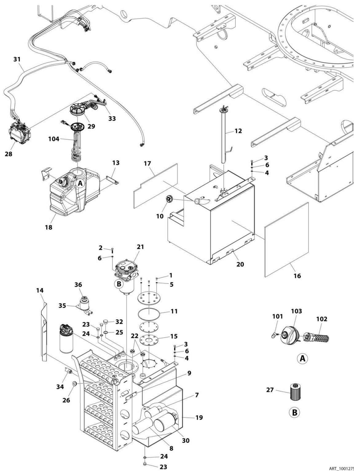
FIGURE 1-4. TANKS INSTALLATION
