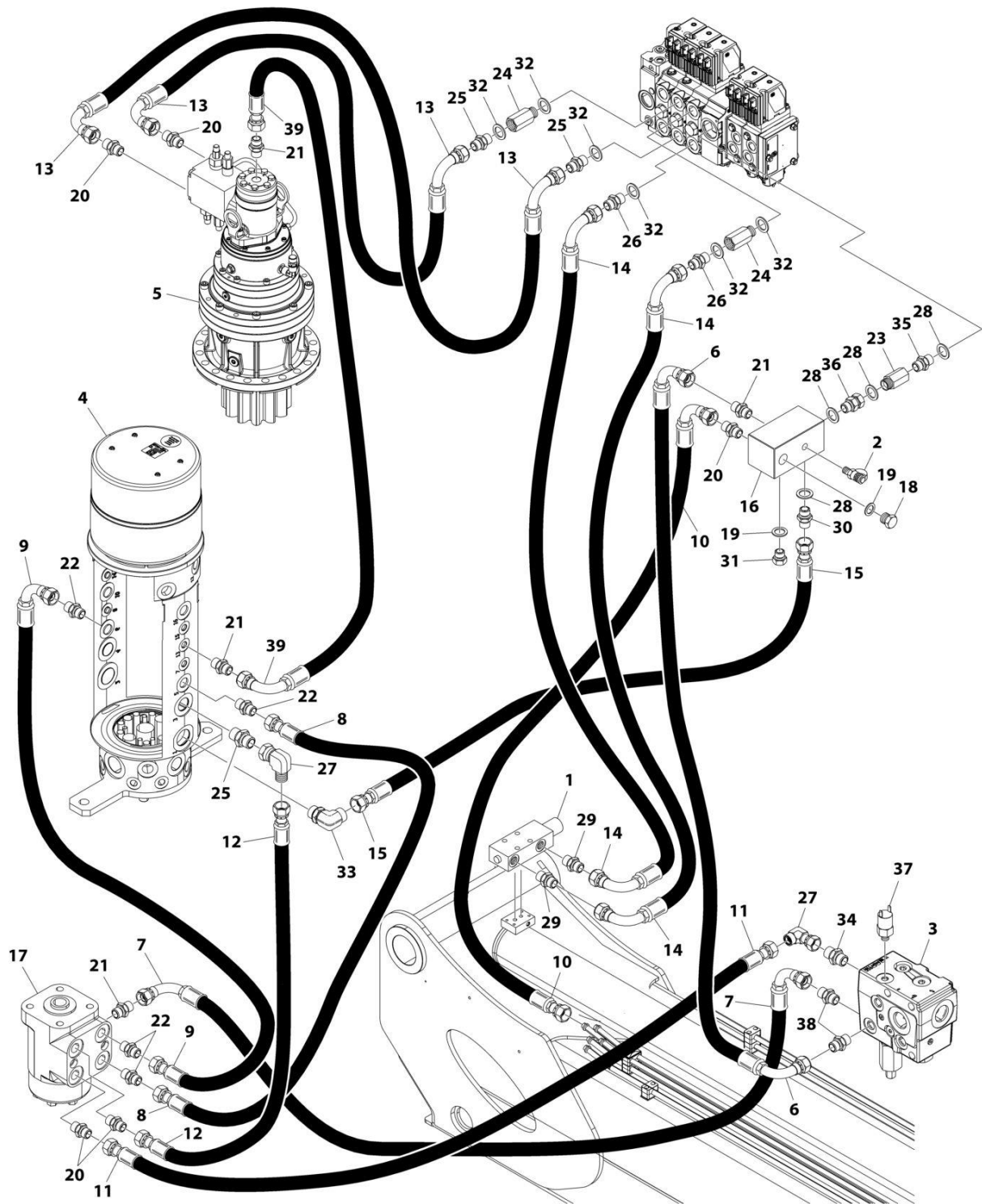
FIGURE 8-14. SWING HYDRAULIC DIAGRAM
