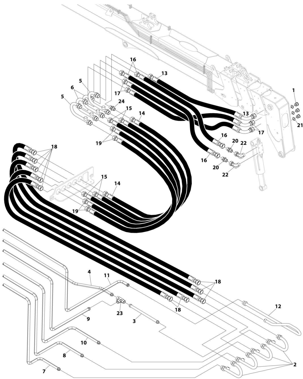
FIGURE 8-4. BOOM HYDRAULICS DIAGRAM
