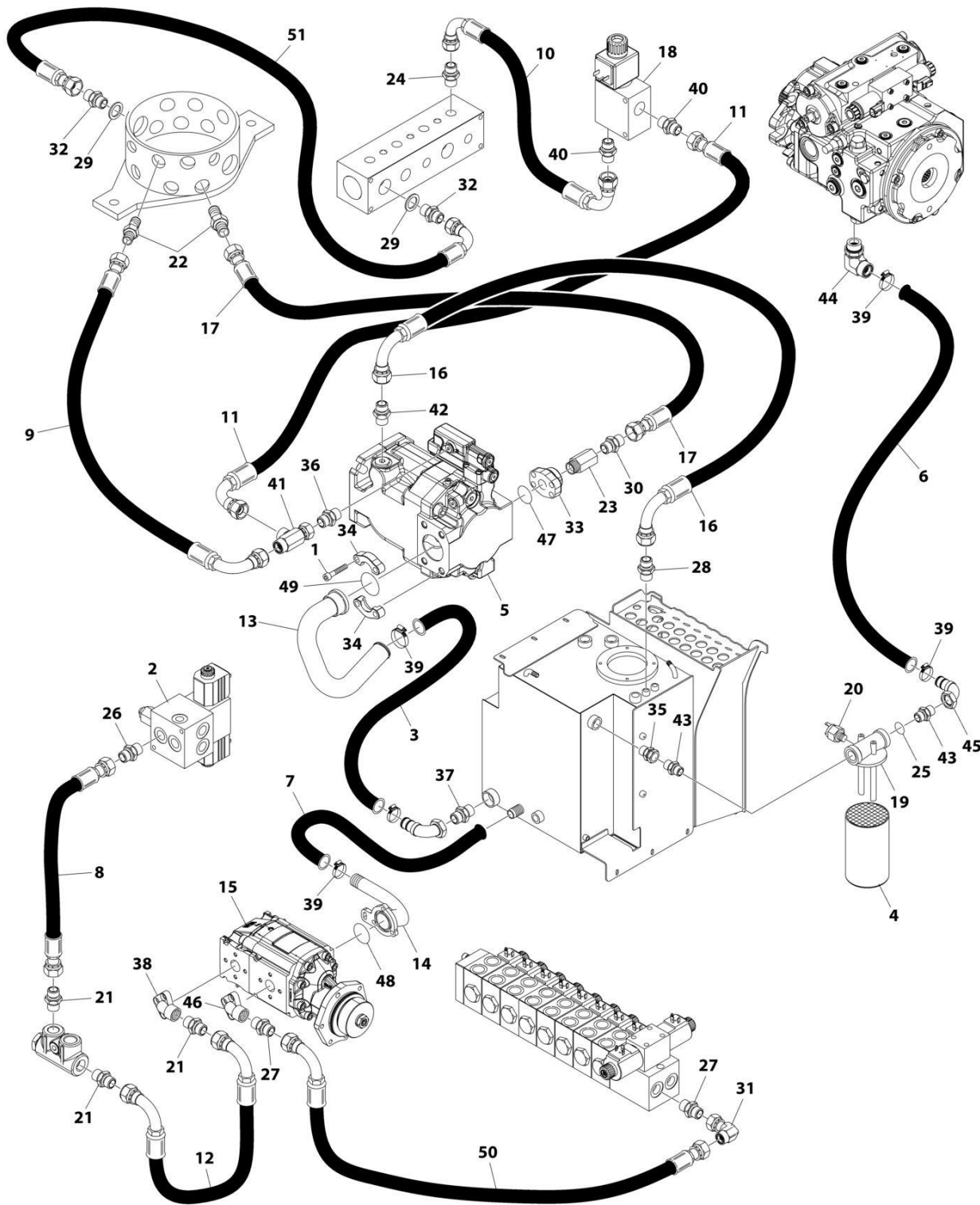
FIGURE 8-9. IMPLEMENT PUMP HYDRAULIC DIAGRAM
