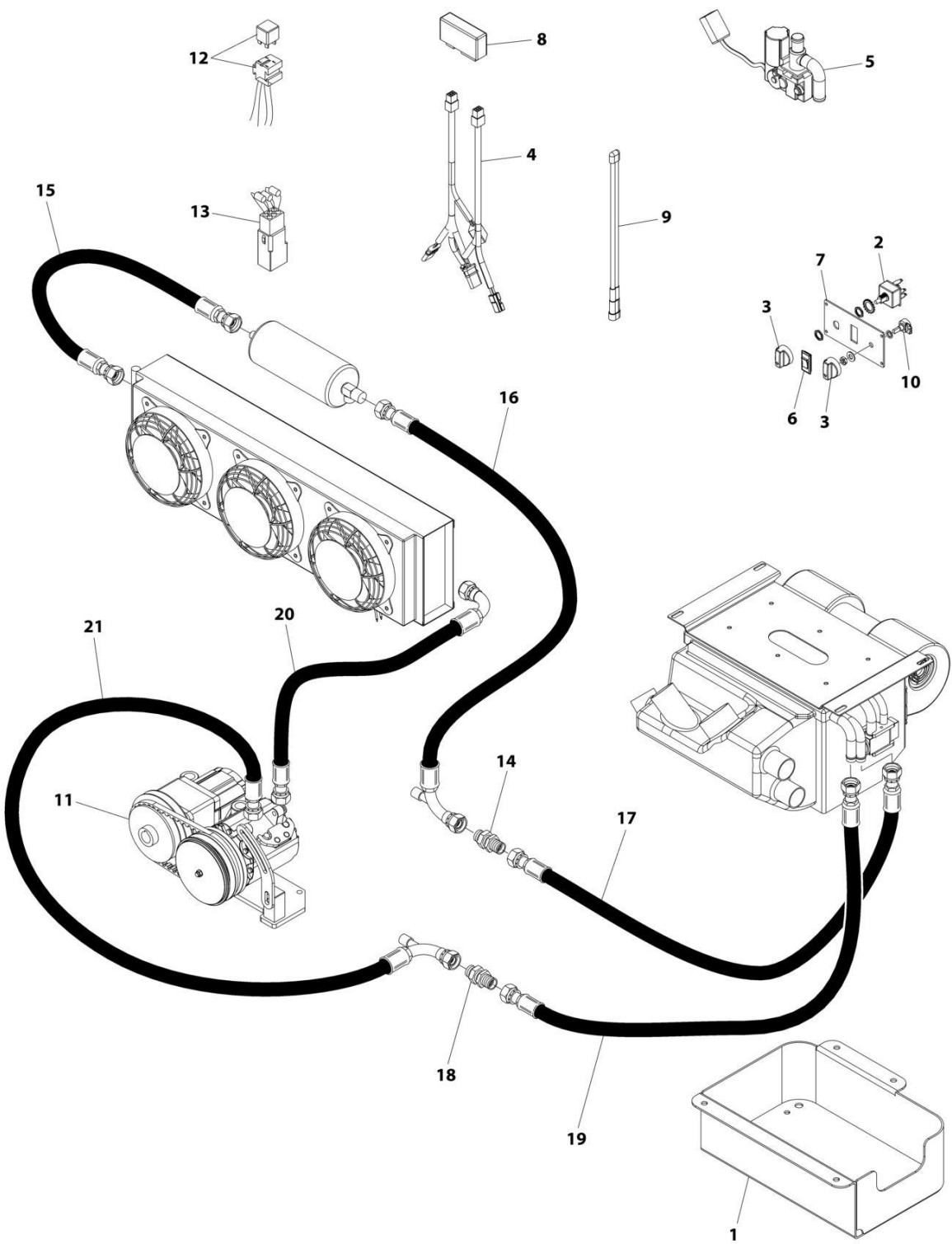
FIGURE 6-13. A/C PUMP INSTALLATION
