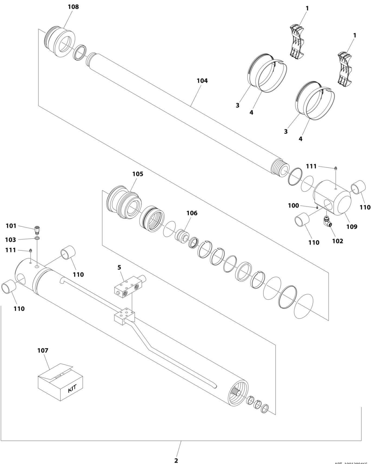
FIGURE 9-3. LIFT CYLINDER ASSEMBLY
