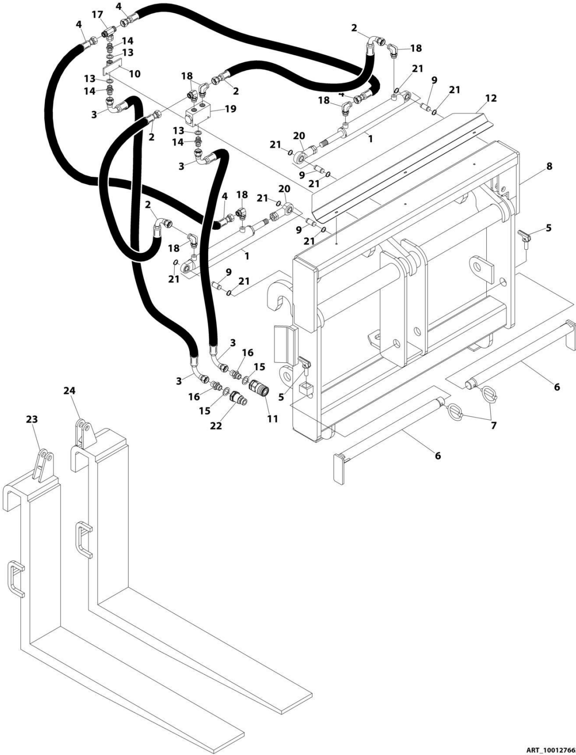
FIGURE 3-5. DUAL FORK CARRIAGE ASSEMBLY - SIDE SHIFT
