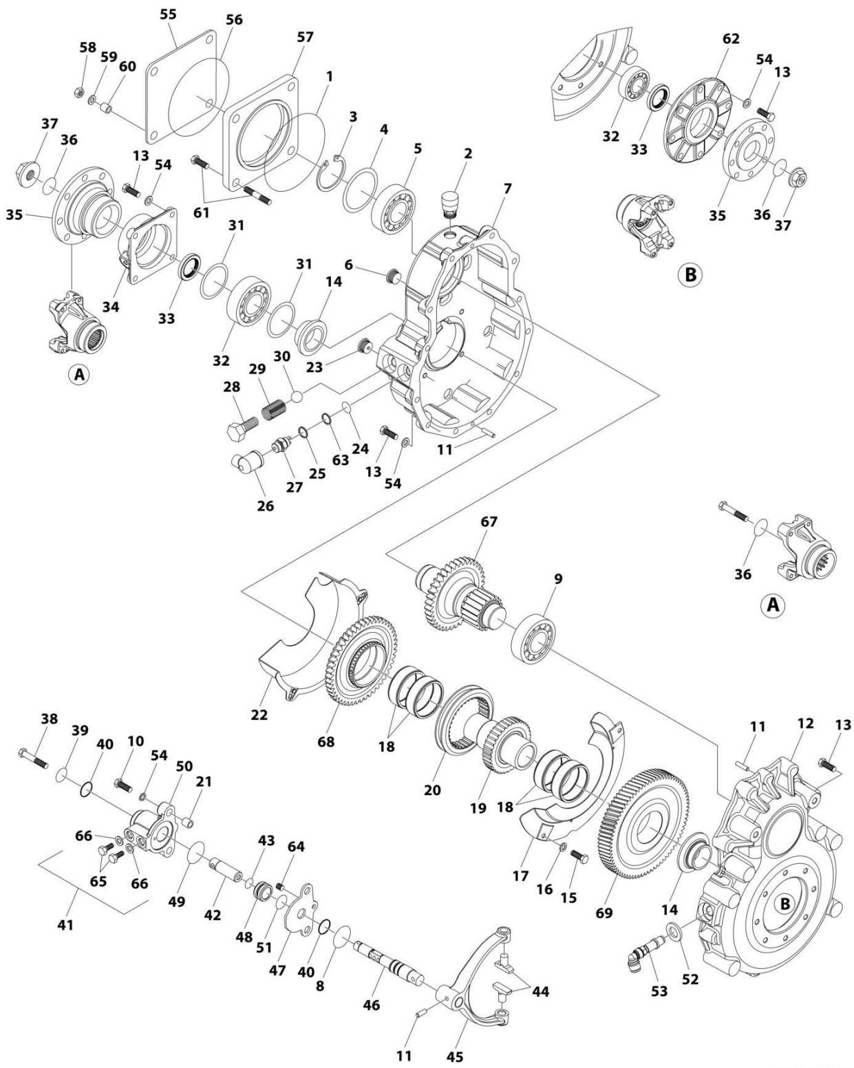
FIGURE 5-5. GEARBOX ASSEMBLY
