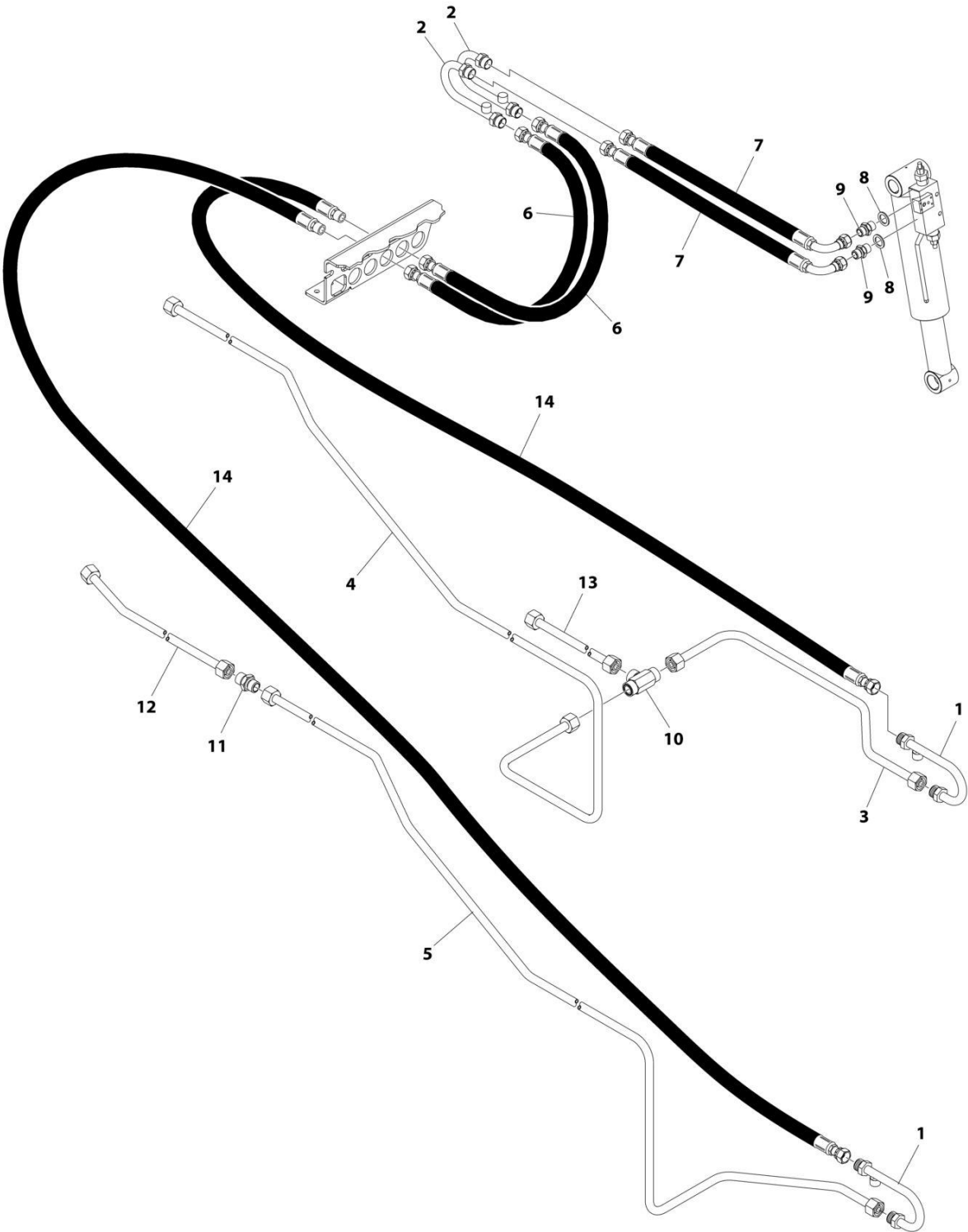
FIGURE 8-15. TILT CYLINDER HYDRAULIC DIAGRAM
