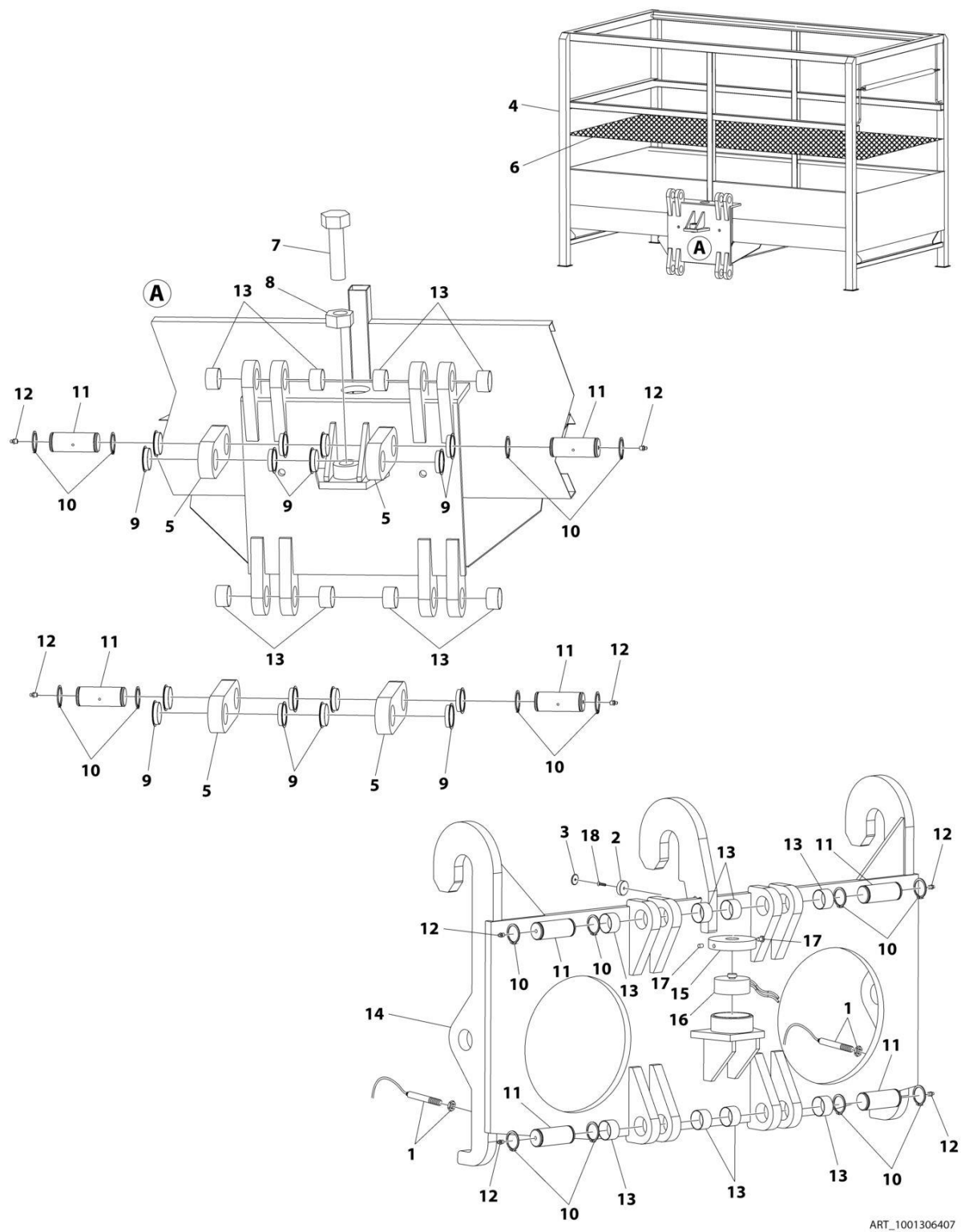
FIGURE 3-10. PLATFORM ASSEMBLY - STANDARD
