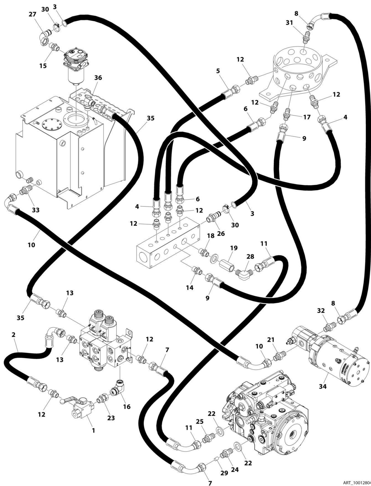
FIGURE 8-8. HYDROSTATIC PUMP HYDRAULIC DIAGRAM
