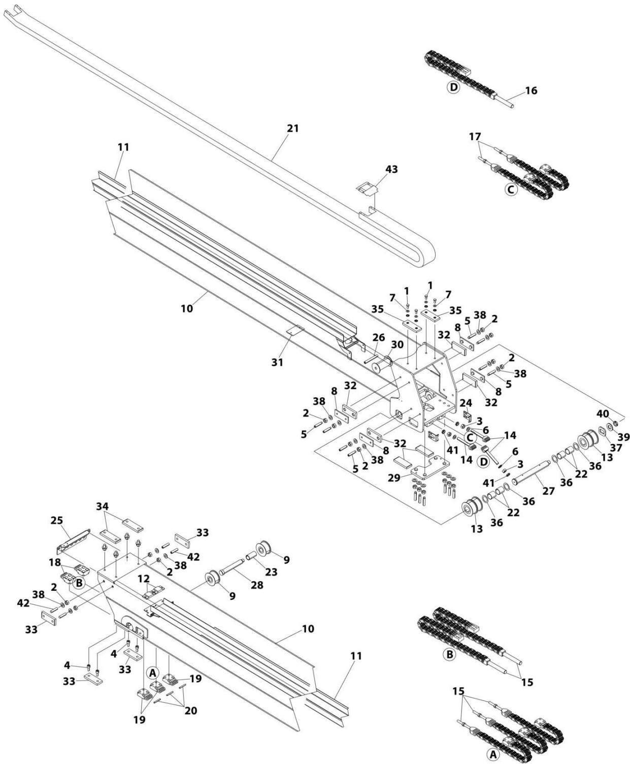
FIGURE 2-3. THIRD BOOM ASSEMBLY
