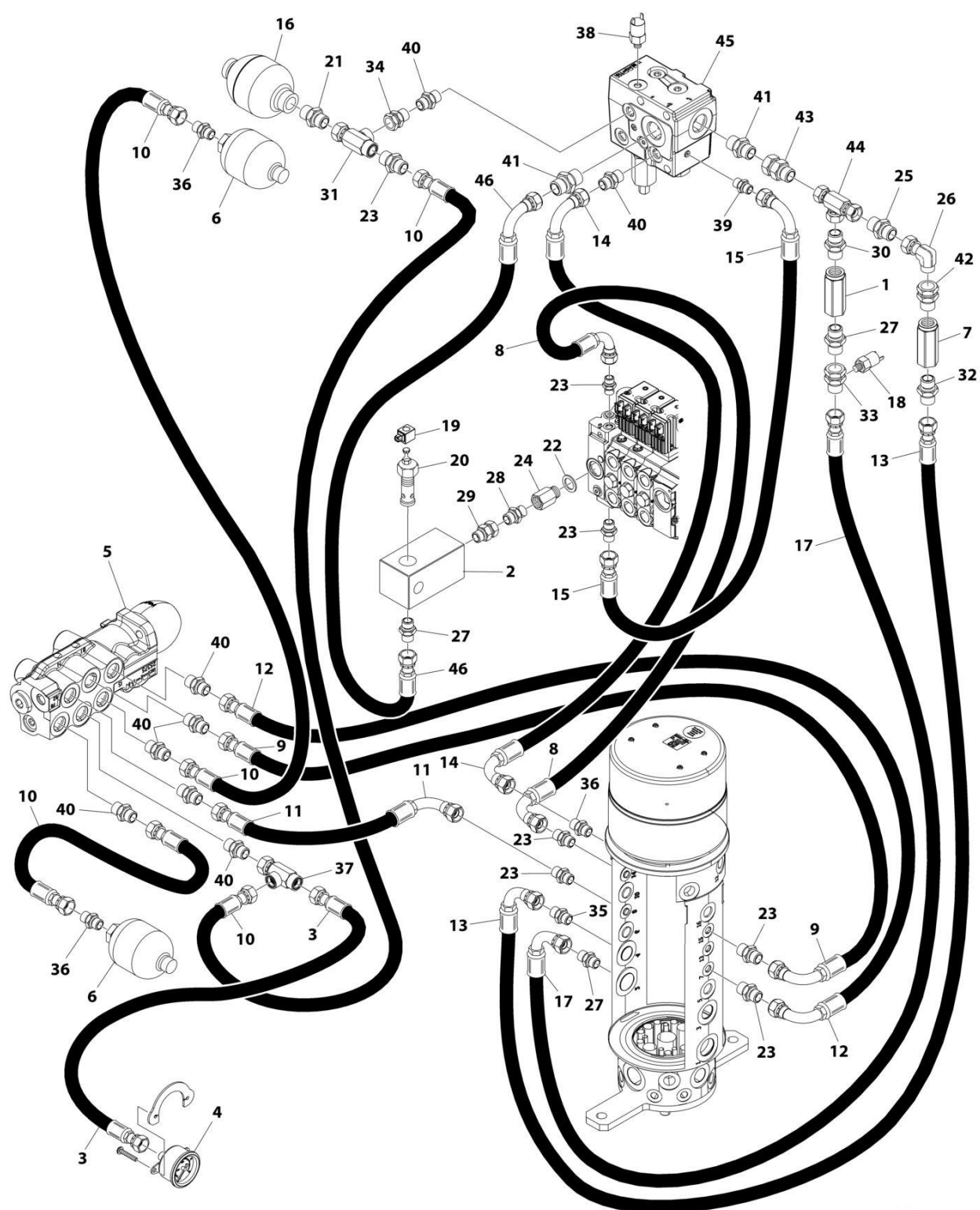
FIGURE 8-5. BRAKES HYDRAULIC DIAGRAM
