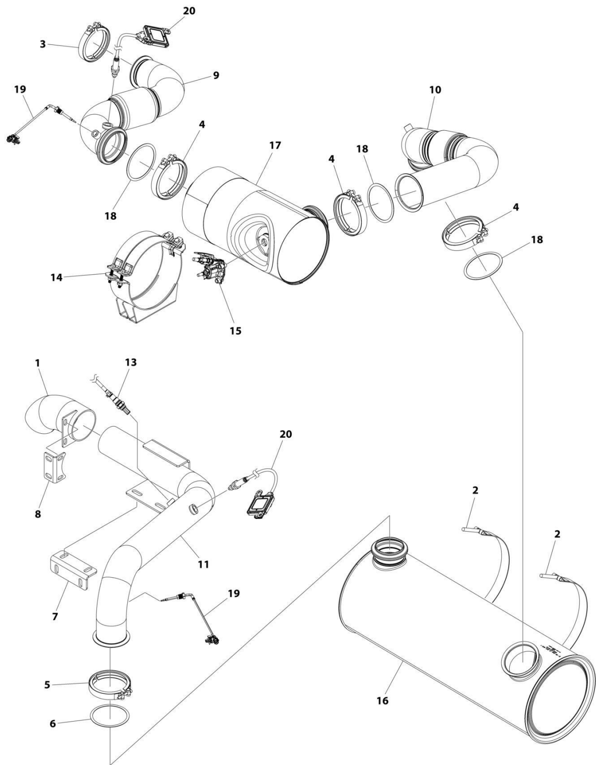
FIGURE 4-5. EXHAUST INSTALLATION
