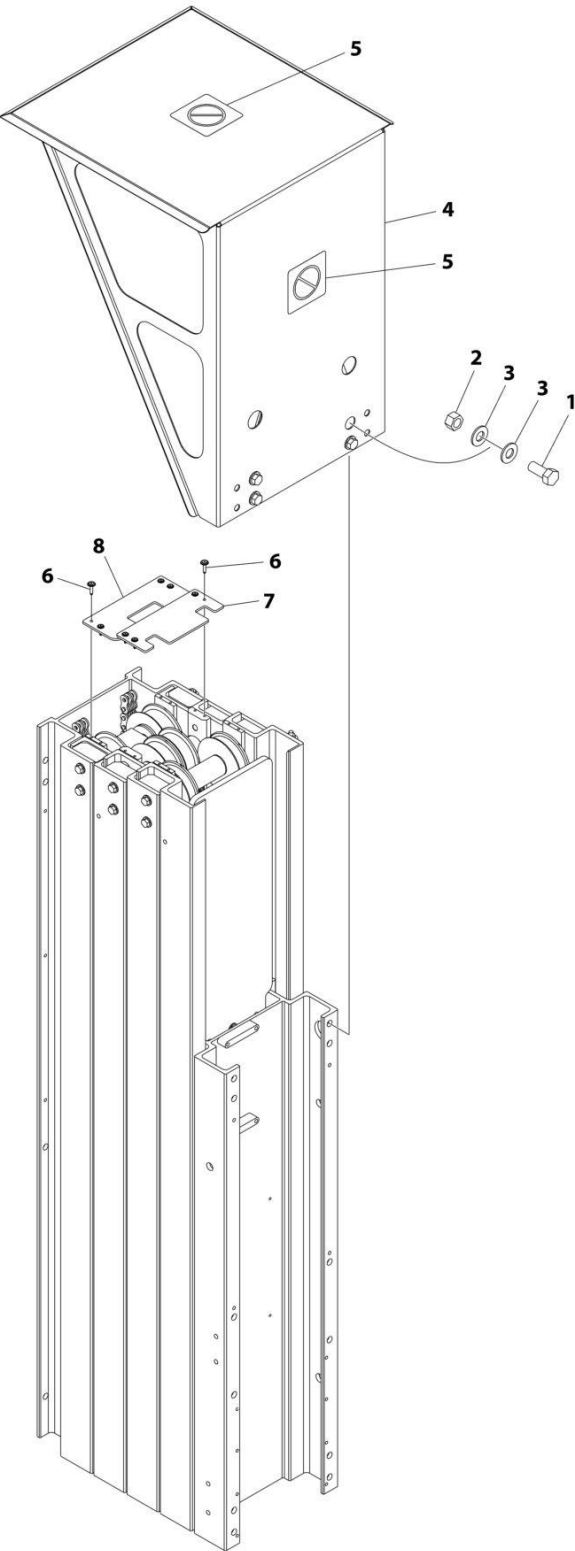
FIGURE 1-7. MAST PROTECTION INSTALLATION
