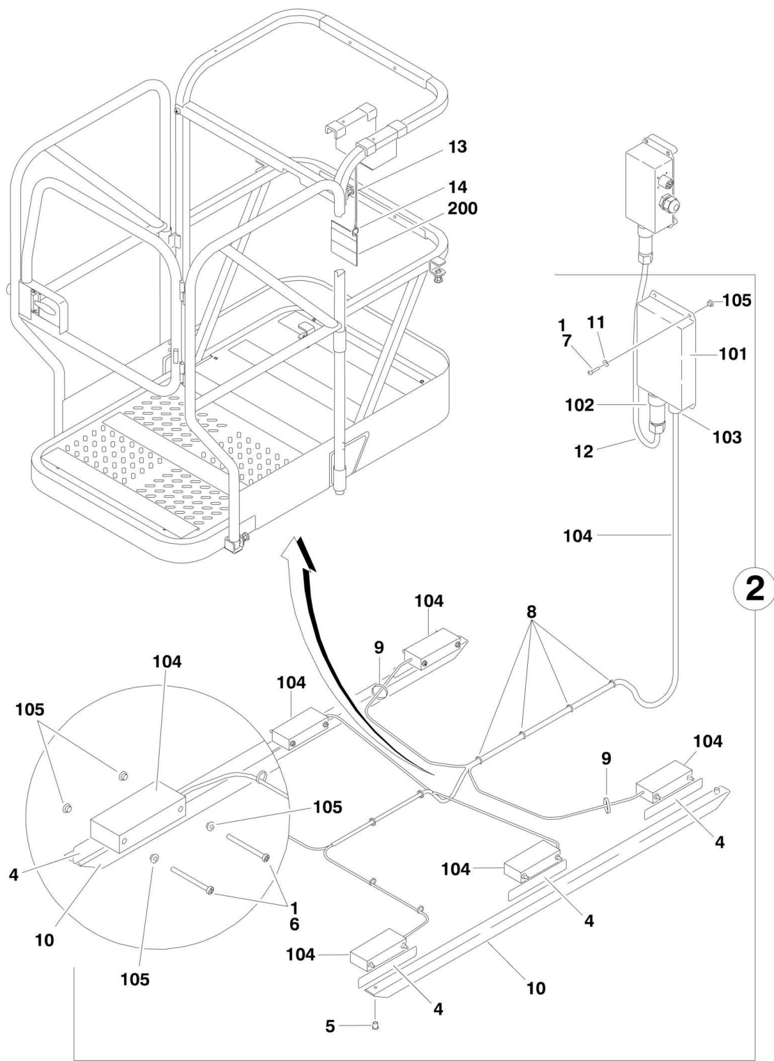
FIGURE 4-11. OBSTRUCTION SENSOR INSTALLATION (MSP ONLY) (OPTIONAL) (SN 0130000001 through 0130033830)
