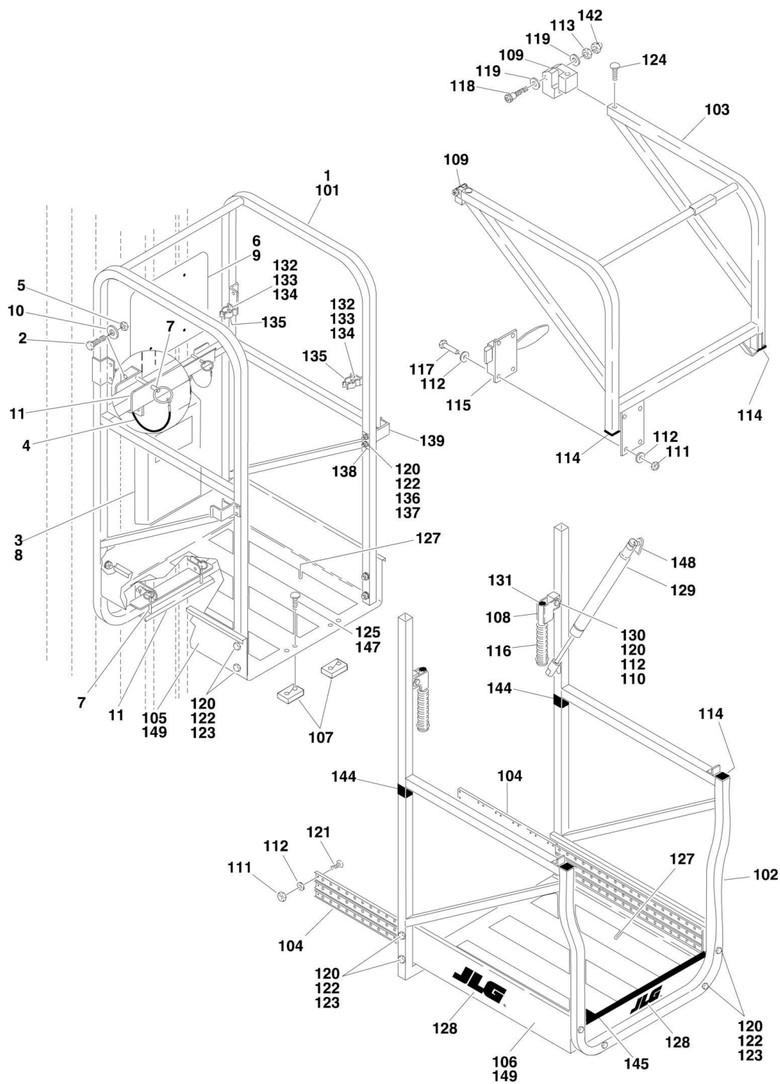
FIGURE 4-4. PLATFORM WITH FRONT ENTRY GULLWING GATE AND ROLLING EXTENSION
