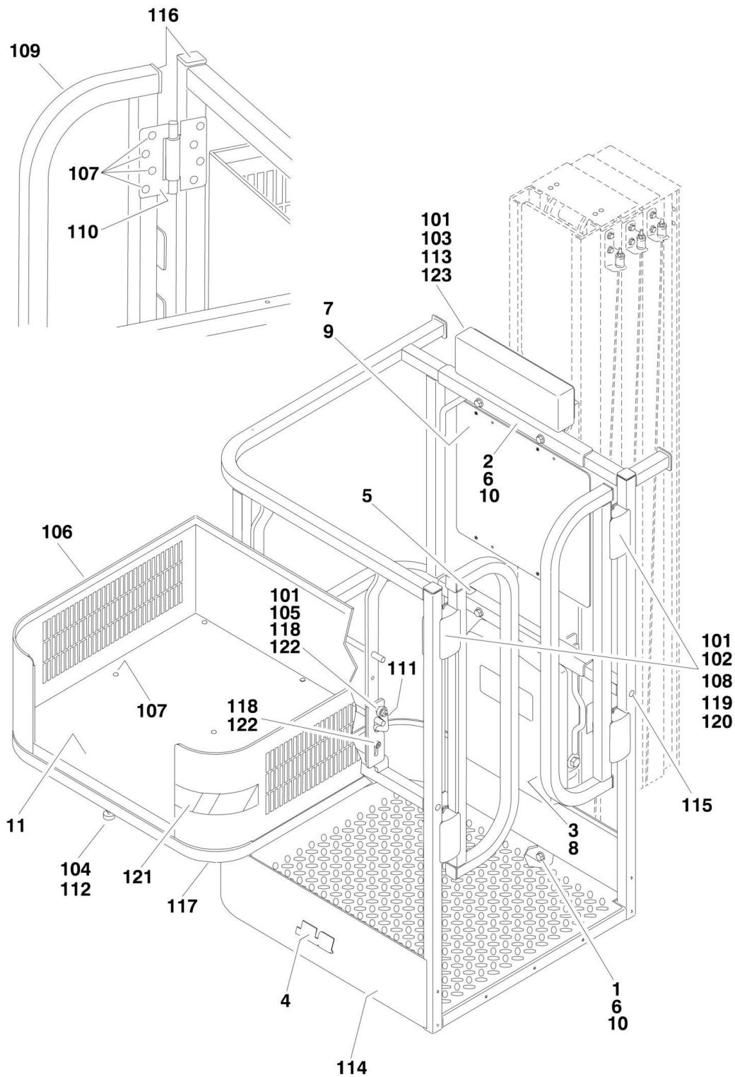
FIGURE 4-9. PLATFORM WITH SIDE ENTRY GATE AND FOLDING MATERIAL TRAY (SN 0130010824 through 0130037734)
